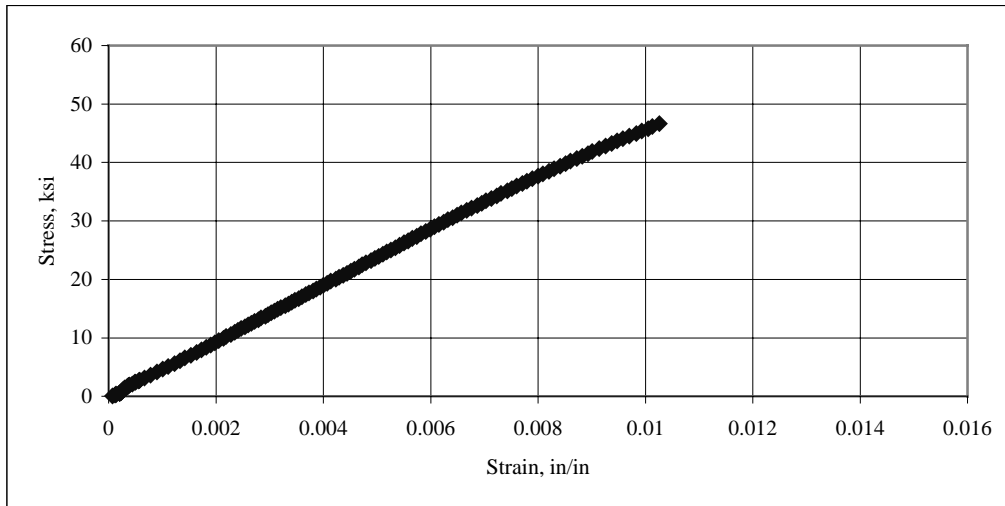
Figure A.7: Stress-Strain Curve for 0°/90° CFRP Coupon #7
