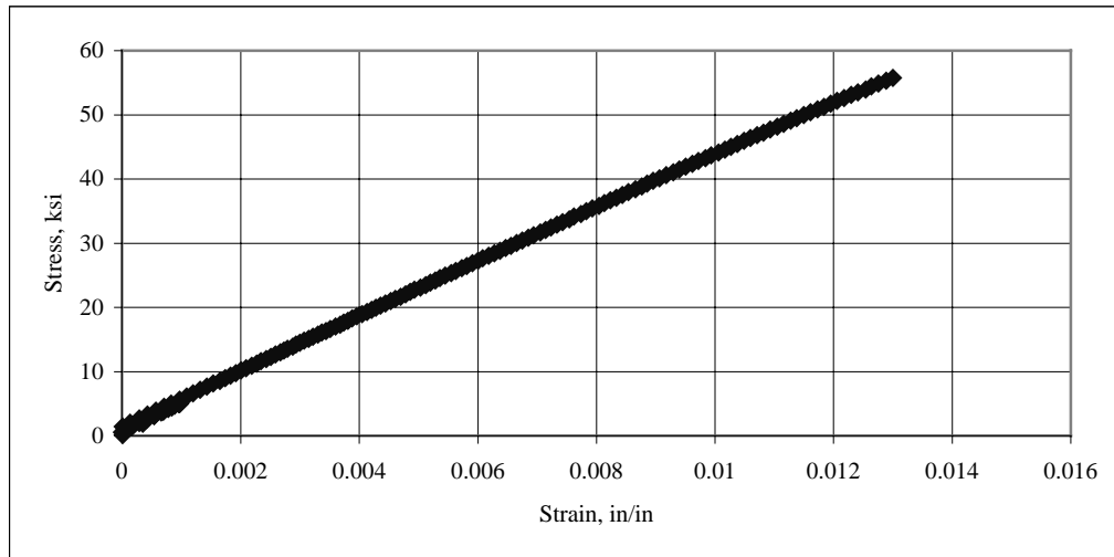
Figure A.5: Stress-Strain Curve for 0°/90° CFRP Coupon #5
