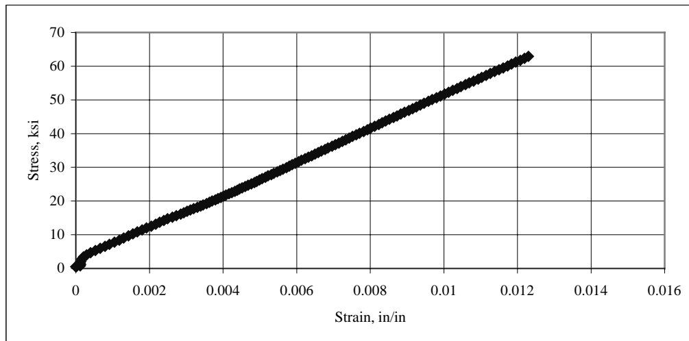
Figure A.8: Stress-Strain Curve for 0°/90° CFRP Coupon #8
