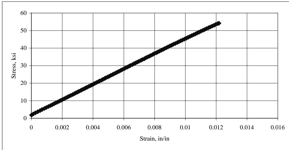
Figure A.2: Stress-Strain Curve for 0°/90° CFRP Coupon #2
