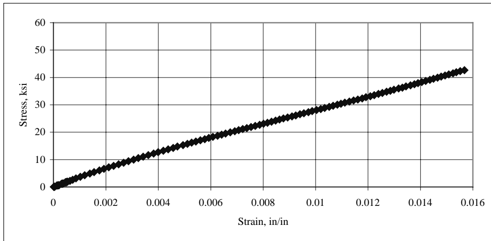
Figure A.11: Stress-Strain Curve for 0°/90° CFRP Coupon #11
