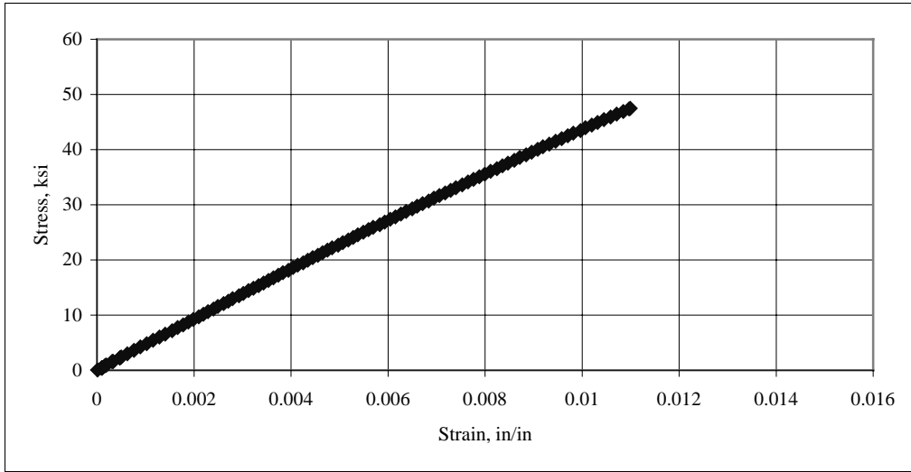
Figure A.1: Stress-Strain Curve for 0°/90° CFRP Coupon #1
