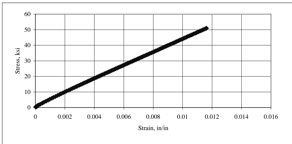
Figure A.12: Stress-Strain Curve for 0°/90° CFRP Coupon #12
