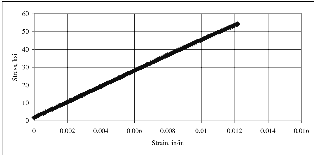
Figure A.10: Stress-Strain Curve for 0°/90° CFRP Coupon #10
