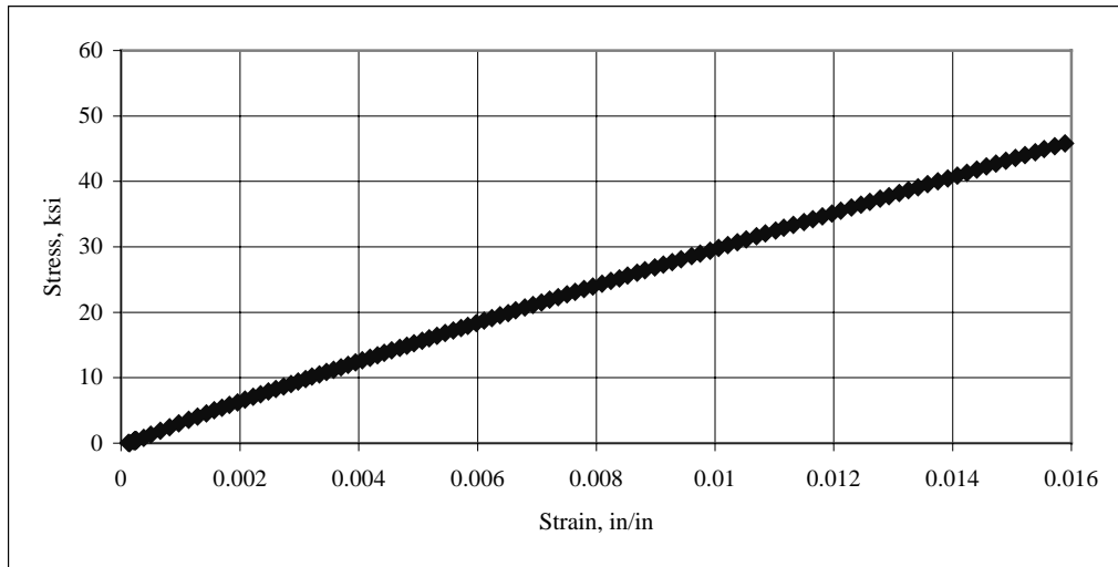
Figure A.3: Stress-Strain Curve for 0°/90° CFRP Coupon #3
