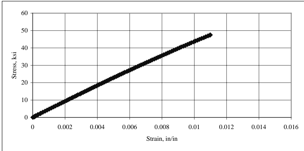
Figure A.9: Stress-Strain Curve for 0°/90° CFRP Coupon #9
