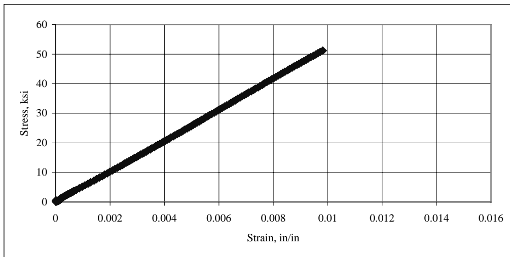
Figure A.6: Stress-Strain Curve for 0°/90° CFRP Coupon #6
