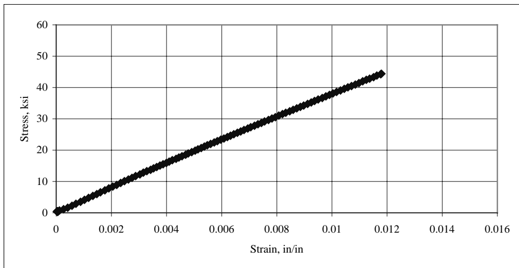
Figure A.4: Stress-Strain Curve for 0°/90° CFRP Coupon #4
