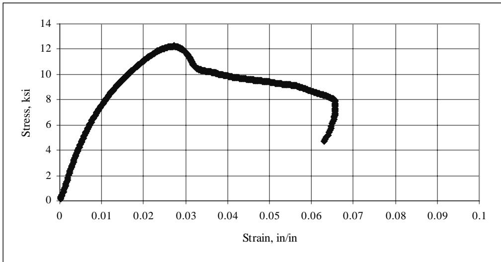
Figure B.6: Stress-Strain Curve for \pm 45^\circ CFRP Coupon #6
