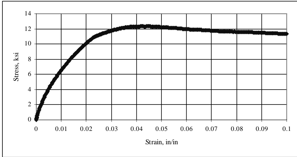
Figure B.11: Stress-Strain Curve for \pm 45^\circ CFRP Coupon #11
