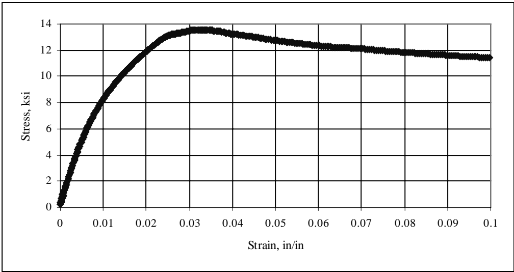
Figure B.3: Stress-Strain Curve for \pm 45^\circ CFRP Coupon #3
