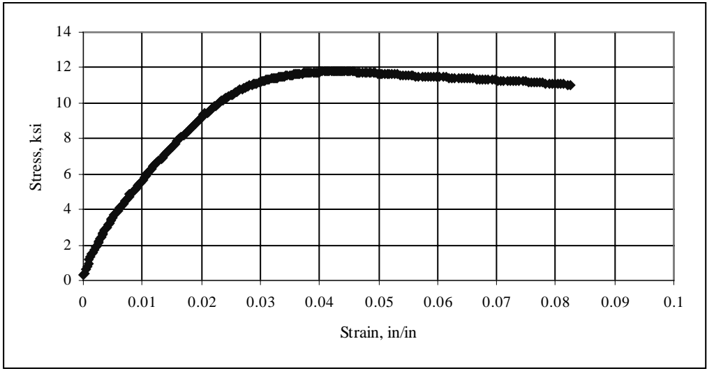
Figure B.9: Stress-Strain Curve for \pm 45^\circ CFRP Coupon #9
