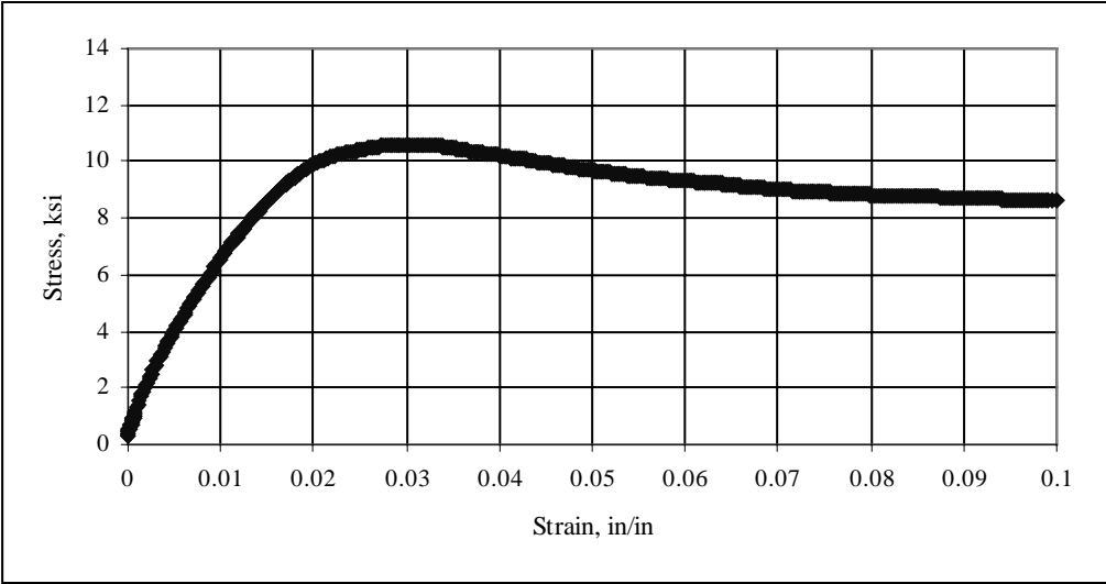
Figure B.7: Stress-Strain Curve for \pm 45^\circ CFRP Coupon #7
