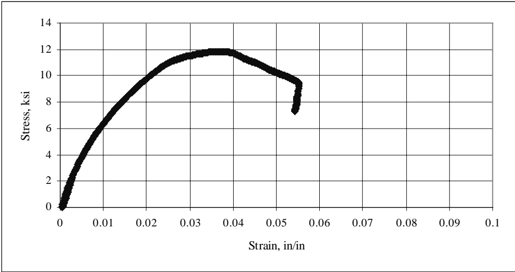
Figure B.8: Stress-Strain Curve for \pm 45^\circ CFRP Coupon #8
