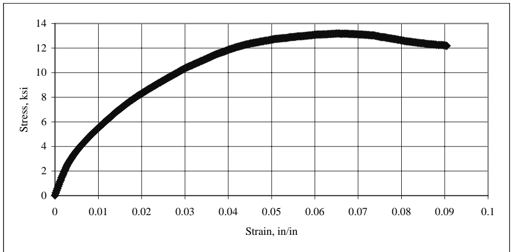
Figure B.10: Stress-Strain Curve for \pm 45^\circ CFRP Coupon #10
