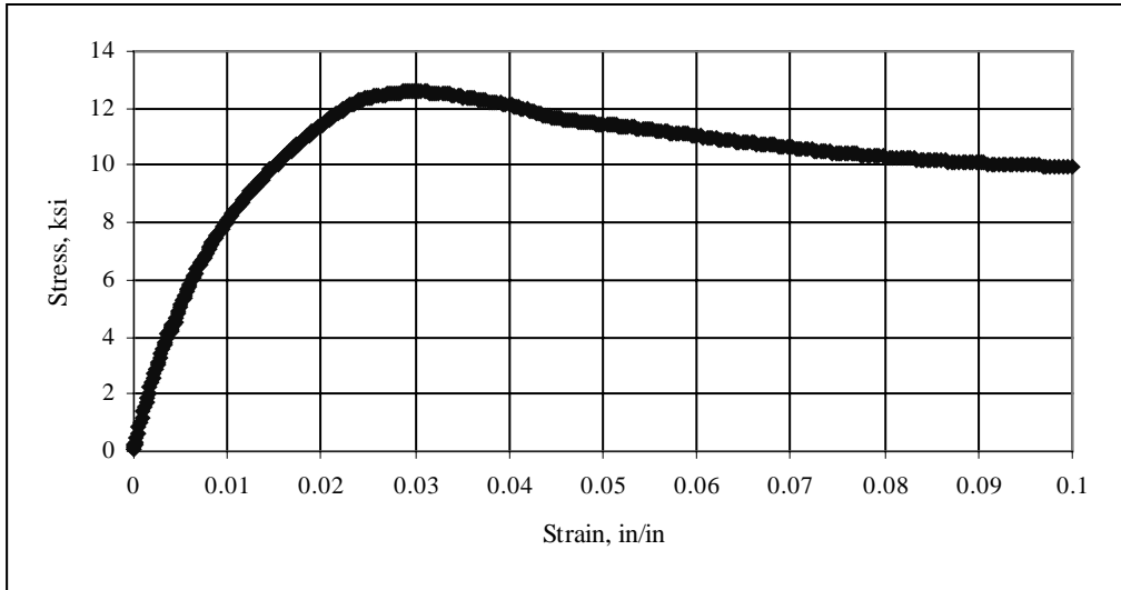
Figure B.5: Stress-Strain Curve for \pm 45^\circ CFRP Coupon #5
