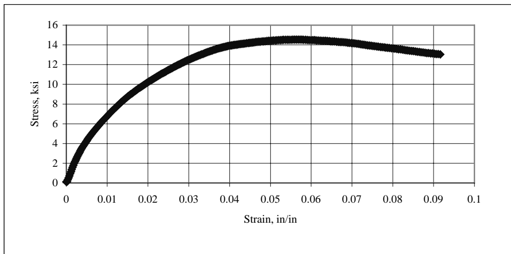
Figure B.12: Stress-Strain Curve for \pm 45^\circ CFRP Coupon #12
