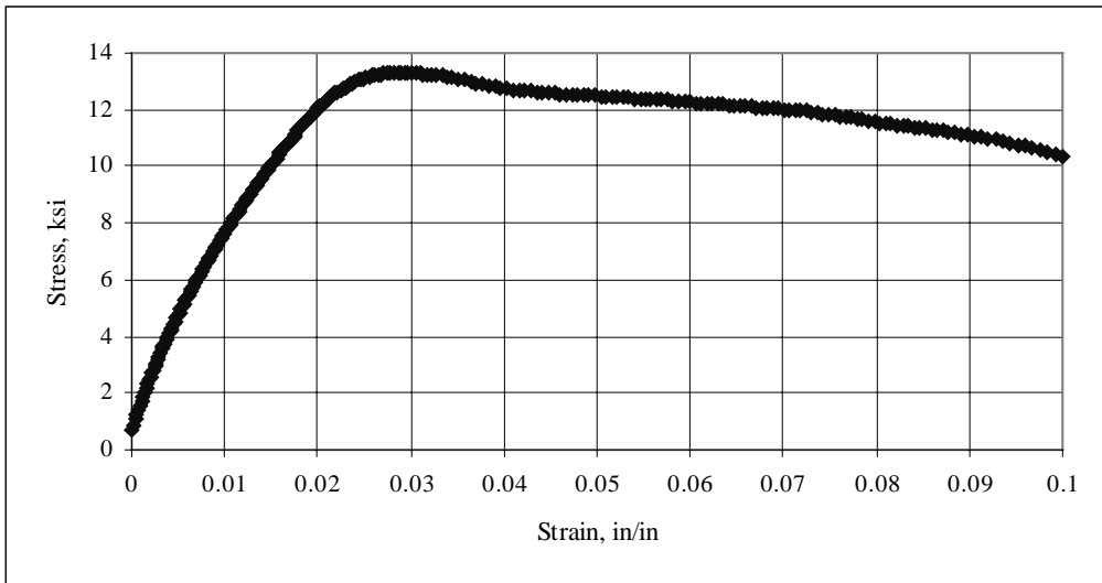
Figure B.2: Stress-Strain Curve for \pm 45^\circ CFRP Coupon #2
