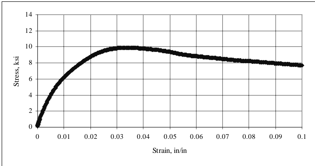
Figure B.4: Stress-Strain Curve for \pm 45^\circ CFRP Coupon #4
