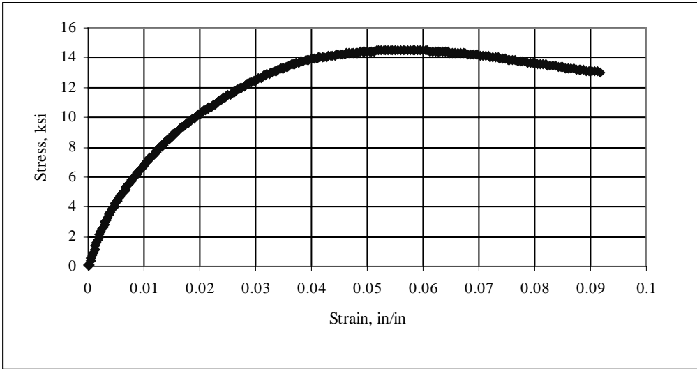
Figure B.1: Stress-Strain Curve for \pm 45^\circ CFRP Coupon #1
