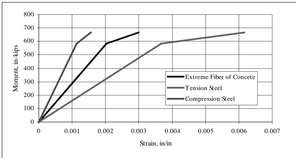
Figure C.4: Theoretical Moment-Strain Curves for Four Layer, 0°/90° Strengthened Beam
