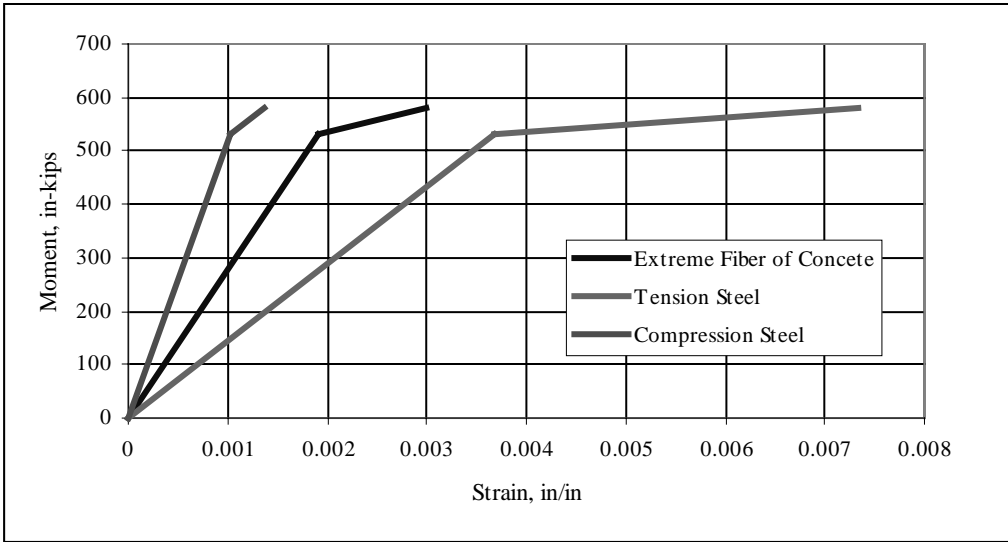
Figure C.5: Theoretical Moment-Strain Curves for Two Layer, ±45° Strengthened Beam
