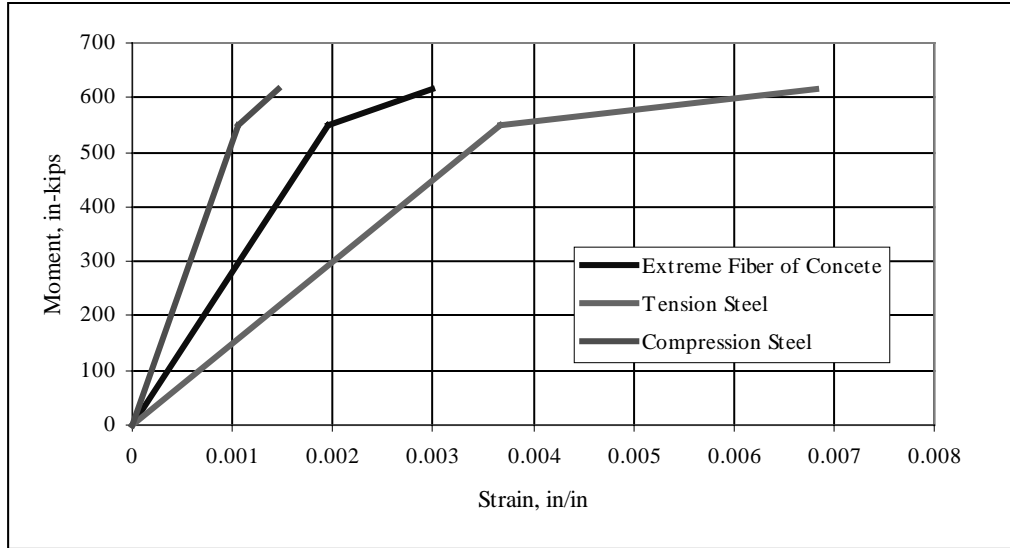
Figure C.7: Theoretical Moment-Strain Curves for Four Layer, ±45° Strengthened Beam
