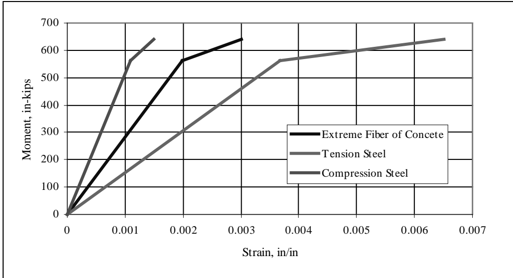
Figure C.3: Theoretical Moment-Strain Curves for Three Layer, 0°/90° Strengthened Beam
