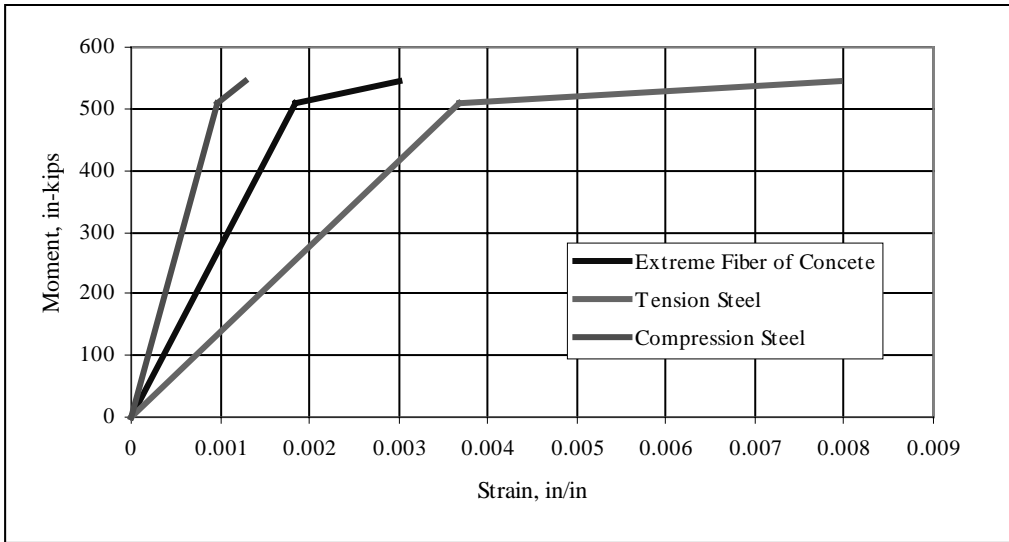
Figure C.1: Theoretical Moment-Strain Curves for Control Beam
