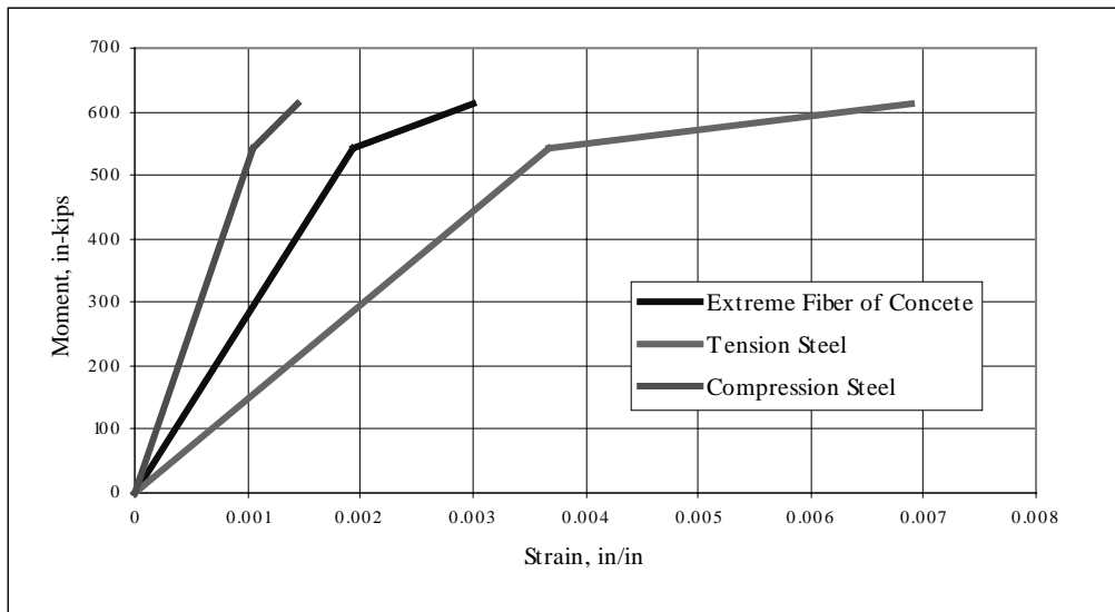
Figure C.2: Theoretical Moment-Strain Curves for Two Layer, 0°/90° Strengthened Beam
