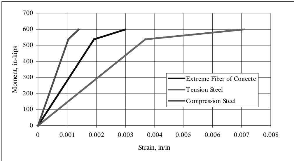
Figure C.6: Theoretical Moment-Strain Curves for Three Layer, ±45° Strengthened Beam
