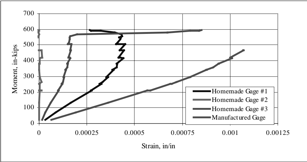
Figure D.6: Moment-Steel Strain Plot for Three-Layer, ±45° Strengthened Beam
