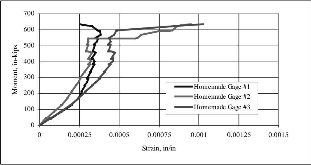
Figure D.7: Moment-Steel Strain Plot for Four-Layer, \pm 45^\circ Strengthened Beam
