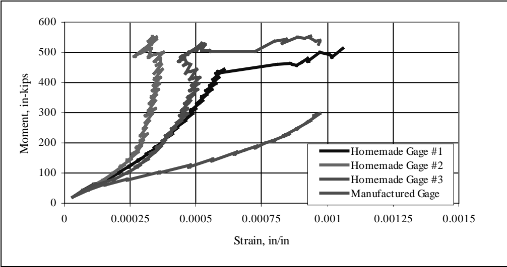
Figure D.5: Moment-Steel Strain Plot for Two-Layer, ±45° Strengthened Beam
