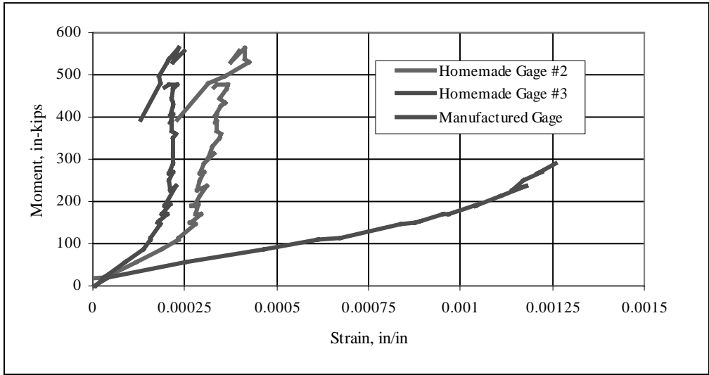
Figure D.1: Moment-Steel Strain Plot for Control
