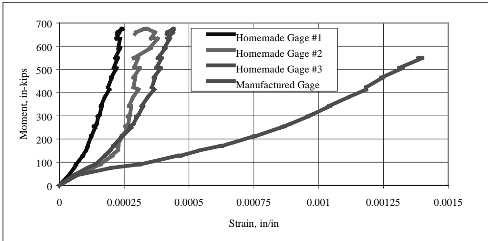
Figure D.4: Moment-Steel Strain Plot for Four-Layer, 0°/90° Strengthened Beam
