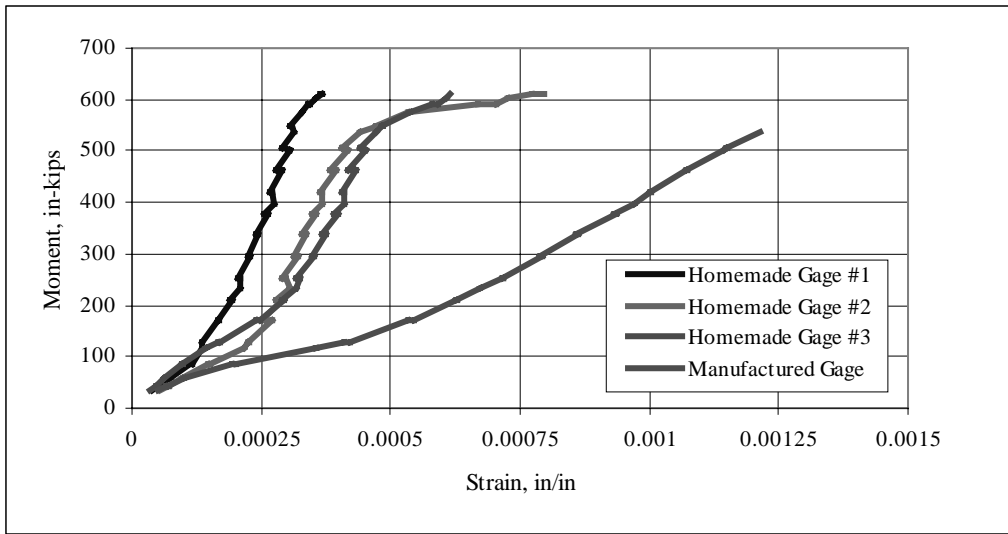
Figure D.2: Moment-Steel Strain Plot for Two-Layer, 0°/90° Strengthened Beam
