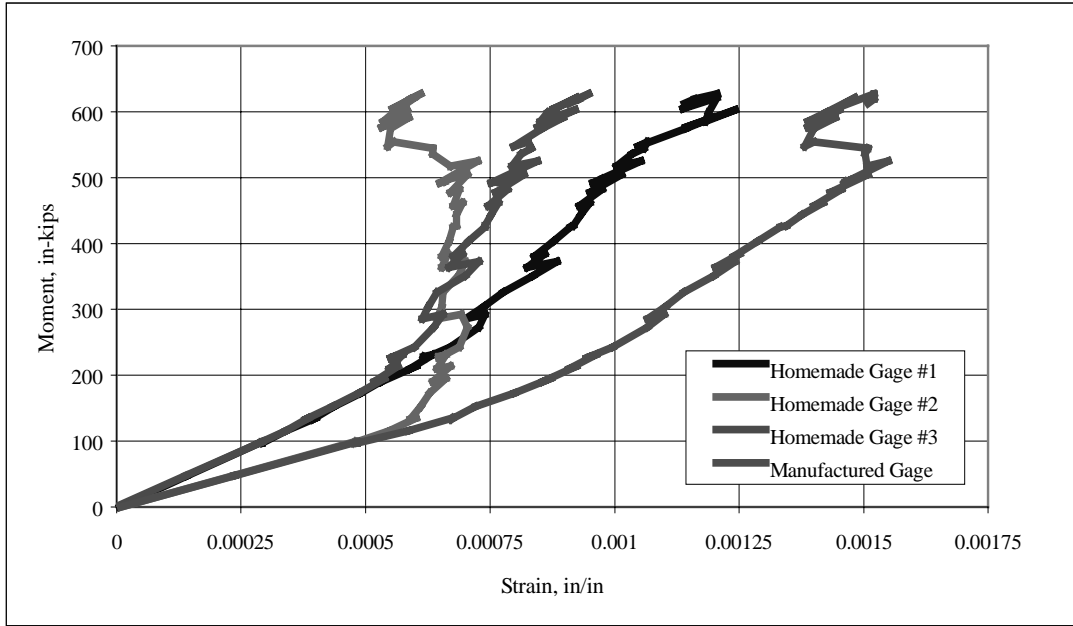
Figure D.3: Moment-Steel Strain Plot for Three-Layer, 0°/90° Strengthened Beam
