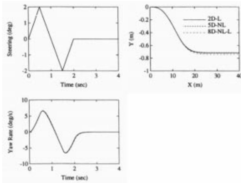
Figure 2.14 Smith Vehicle Response with Saw-Tooth Input after Smith [14]
