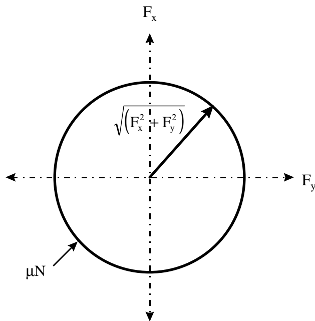
Figure 2.13 Friction Circle Diagram
