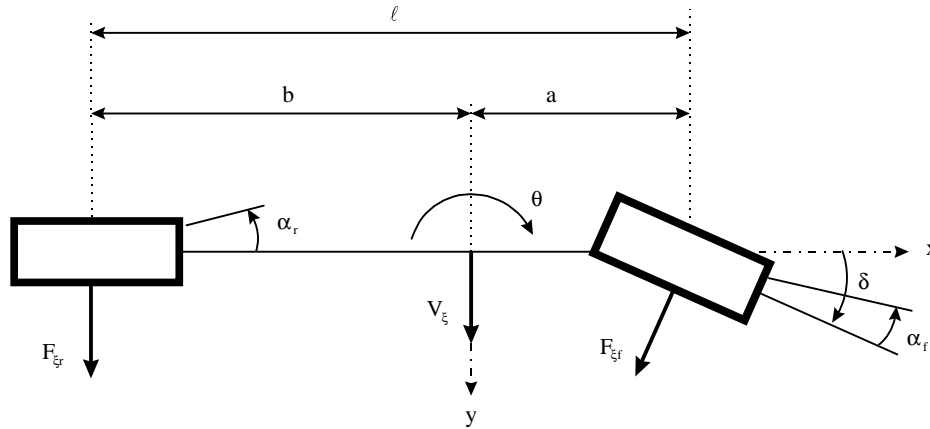
Figure 2.5 Two-Degree-of-Freedom Model
