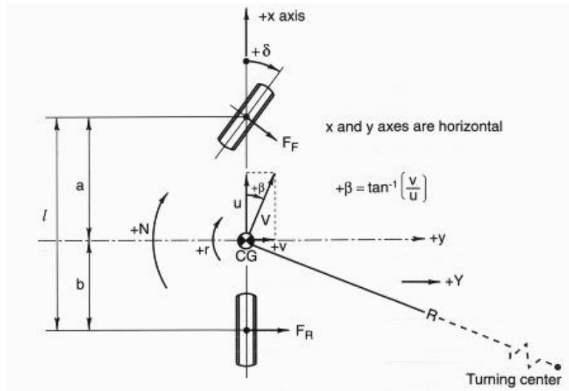
Figure 2.4 Body-Slip Angle after Milliken [19]
