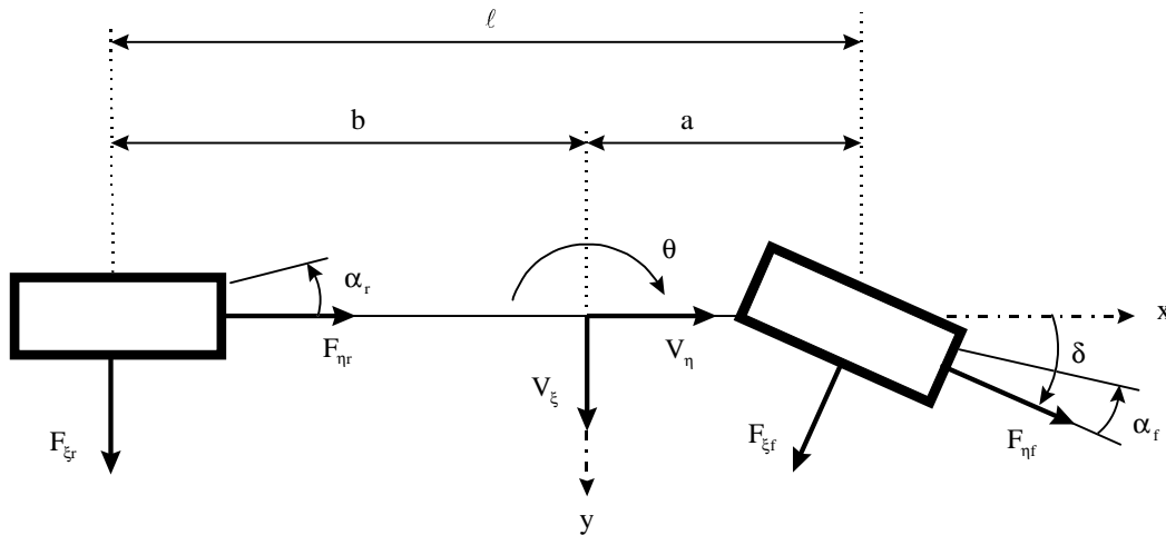
Figure 2.9 Three-Degree-of-Freedom Used for Simulation
