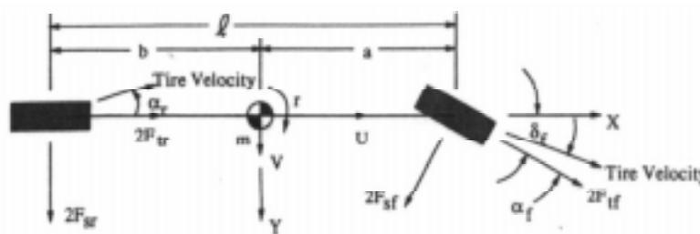
Figure 2.6 Three-Degree-of-Freedom Model after Smith [18]
