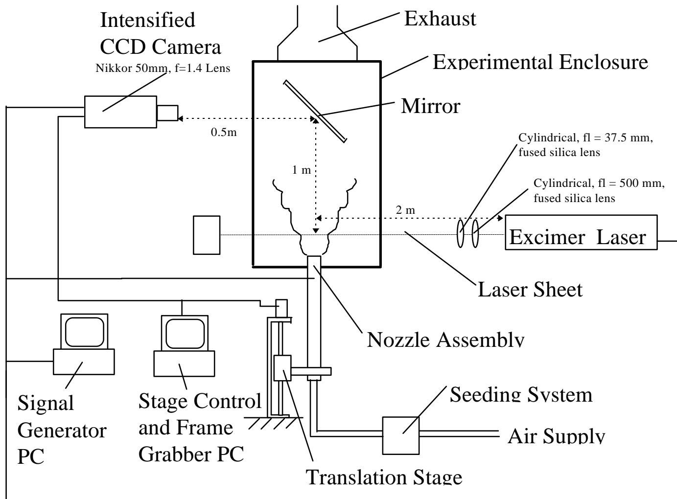
Figure 2.3: Schematic of Flow Visualization System for PLIF Experiments
