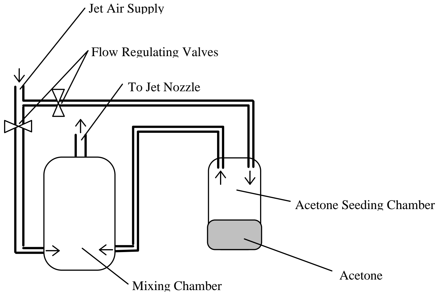
Figure 2.4 Acetone seeding system for PLIF experiments
