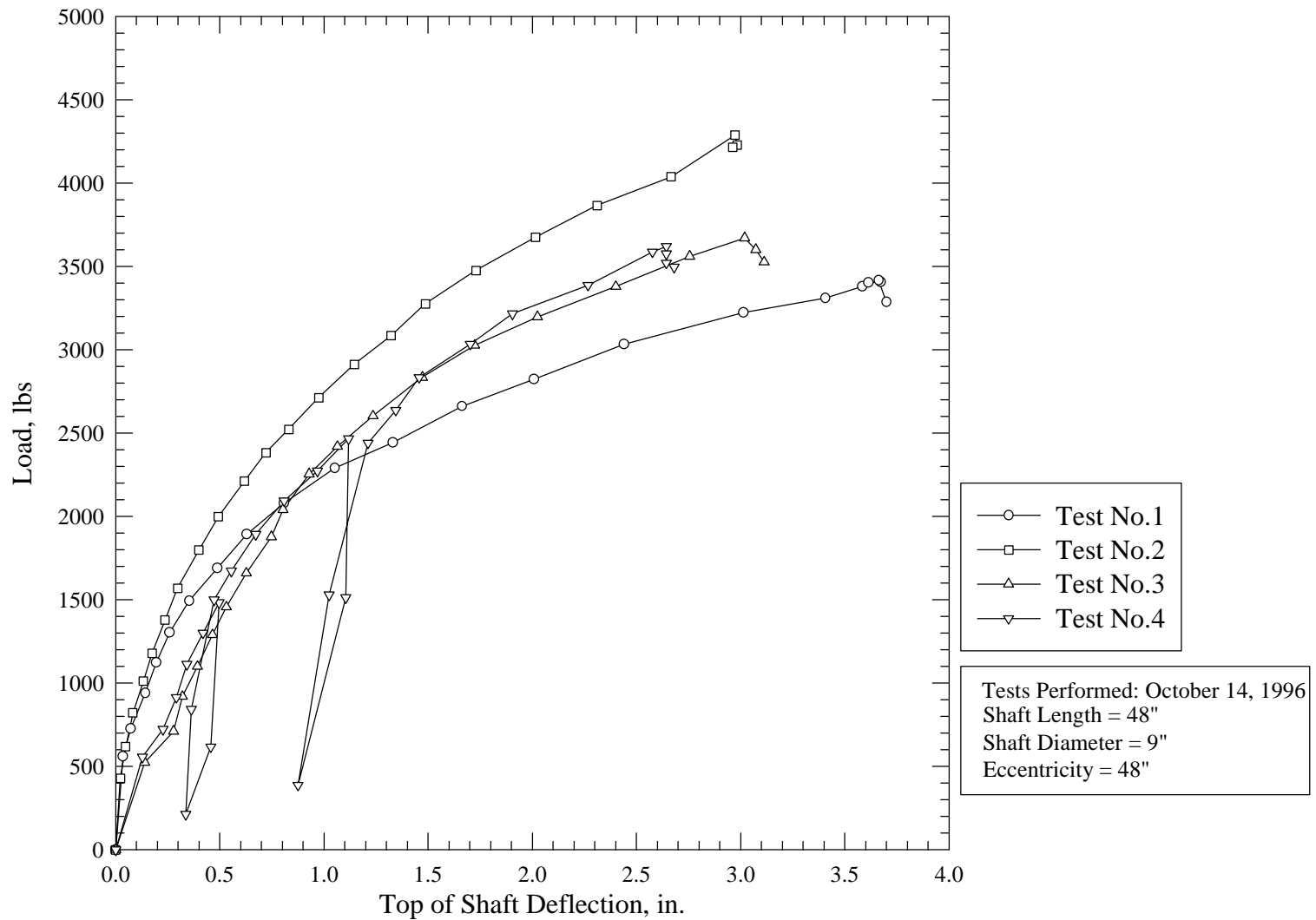
Figure 3.10: Fairfax County Parkway Load Deflection Curves
