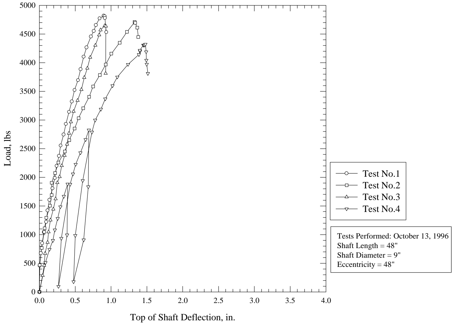
Figure 3.11: Roberts Road Load Deflection Curves
