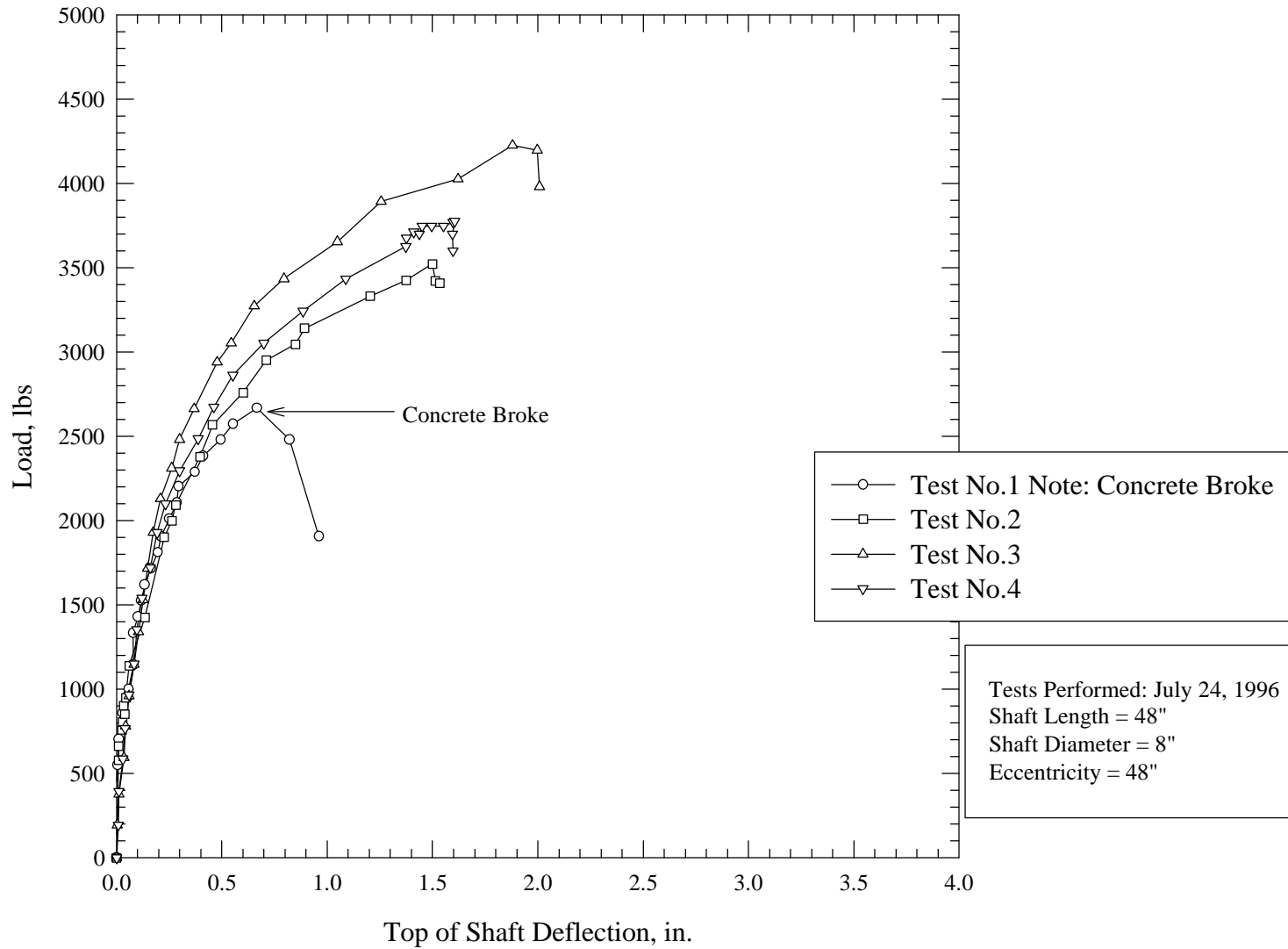
Figure 3.7: Prices Fork Load Deflection Curves
