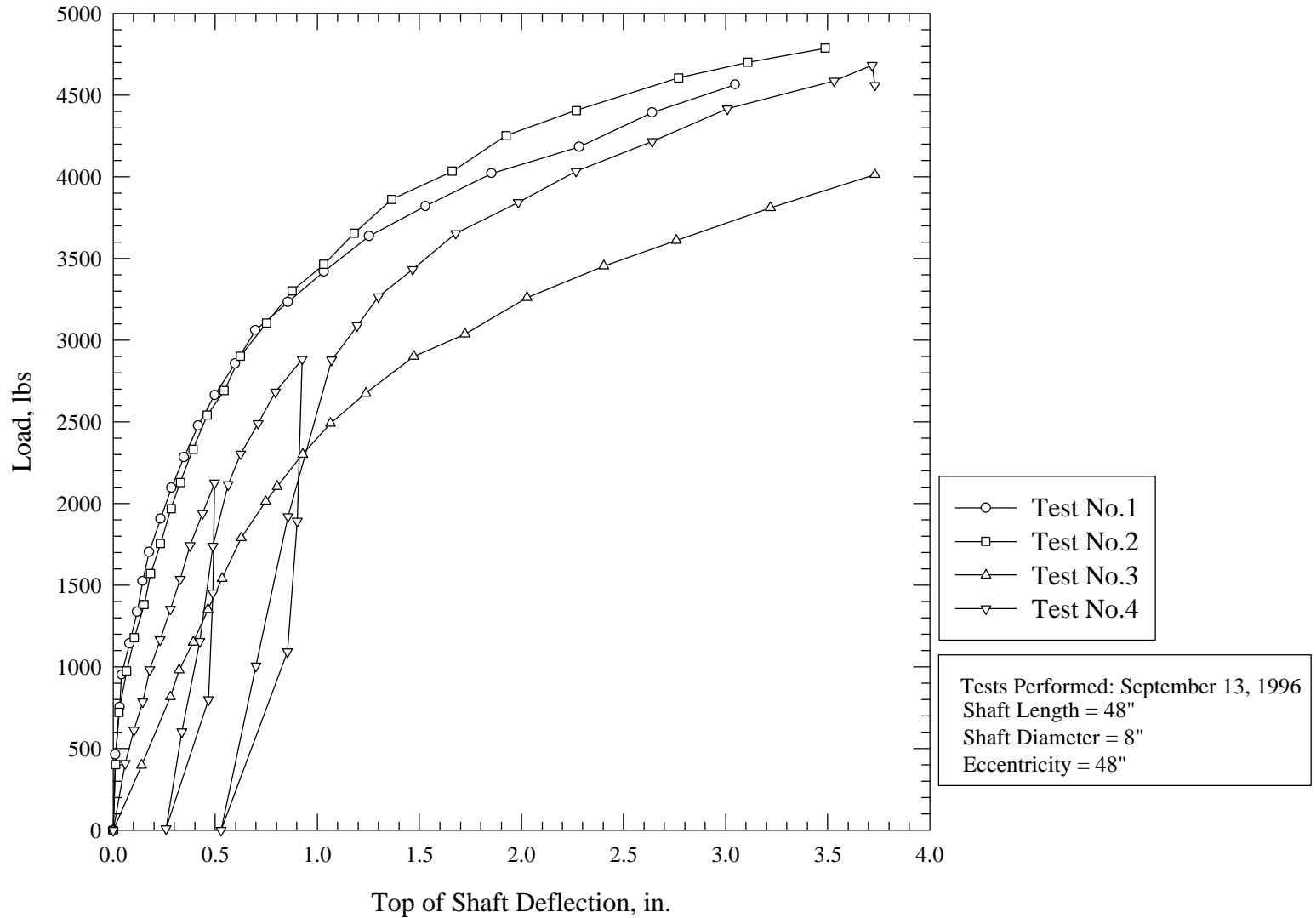
Figure 3.9: Suffolk Load Deflection Curves
