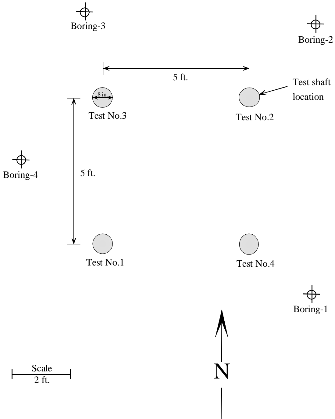
Figure 4.1: Site Plan, Prices Fork
