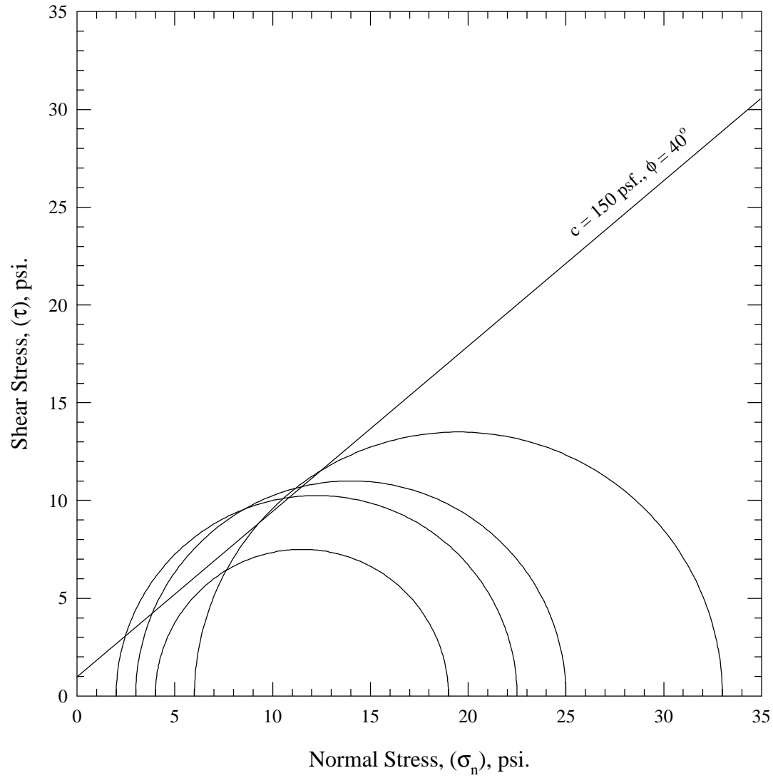
Figure 4.11b: Roberts Road, Strength Envelope
