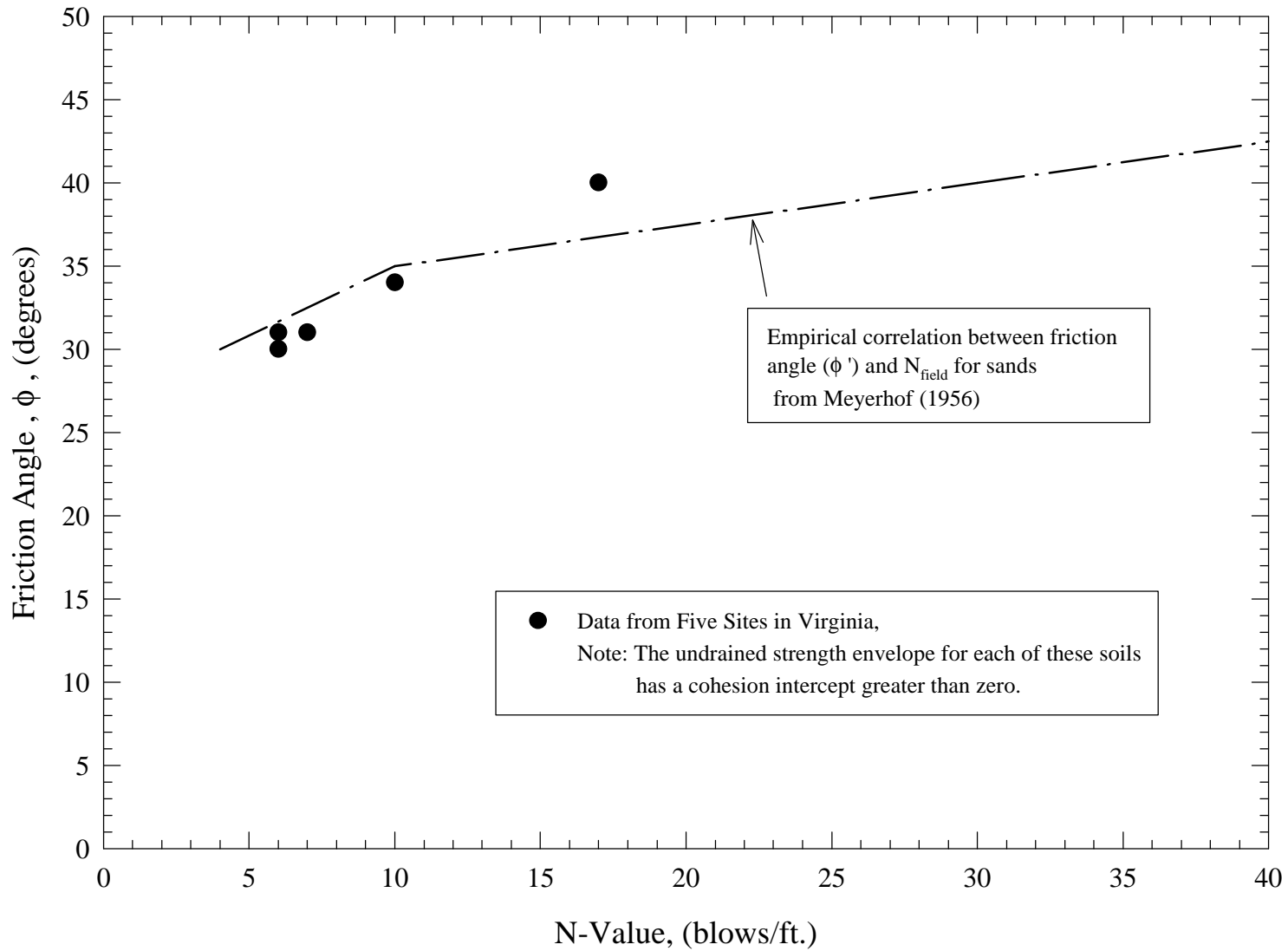
Figure 4.12: Variation of Friction Angle with N_{\text{field}}
