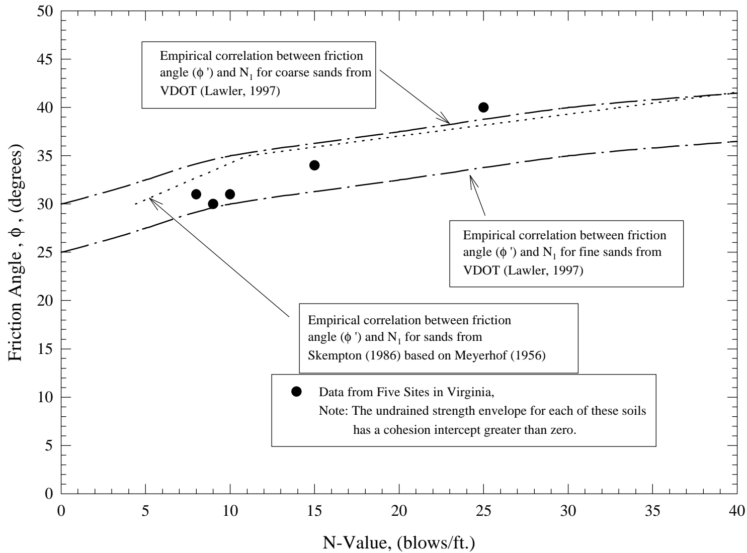
Figure 4.13: Variation of Friction Angle with N_1
