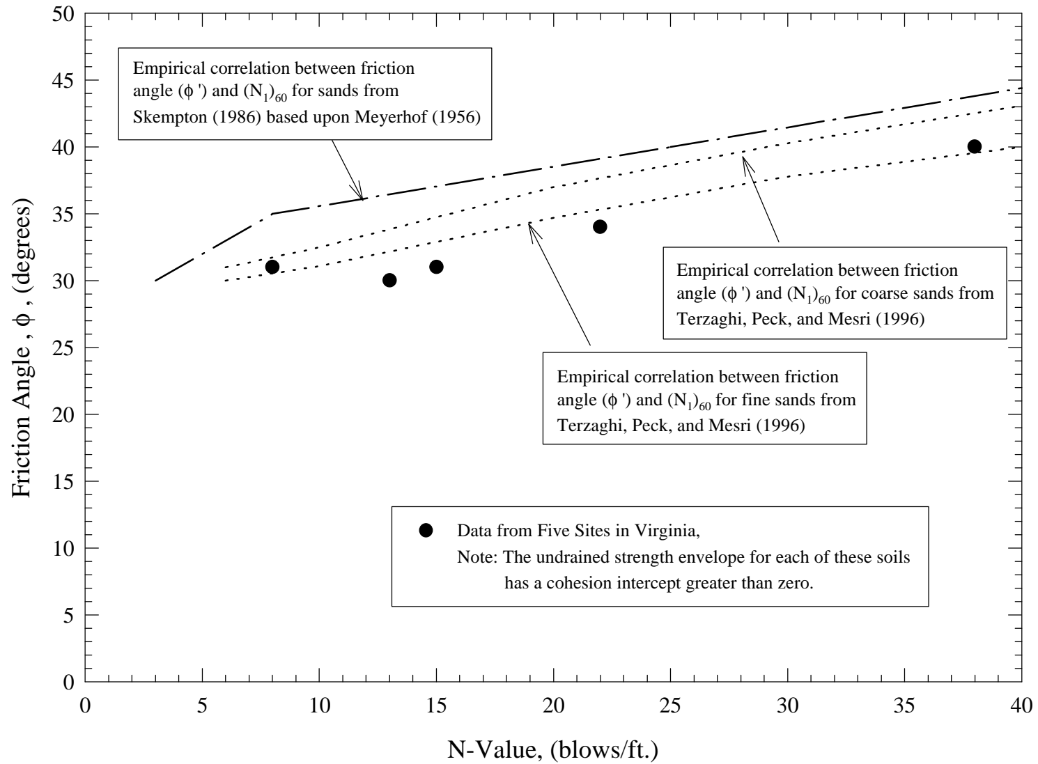
Figure 4.14: Variation of Friction Angle with (N_1)_{60}
