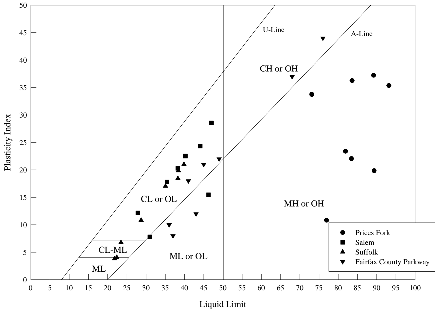
Figure 4.6: Summary of Atterberg Limits
