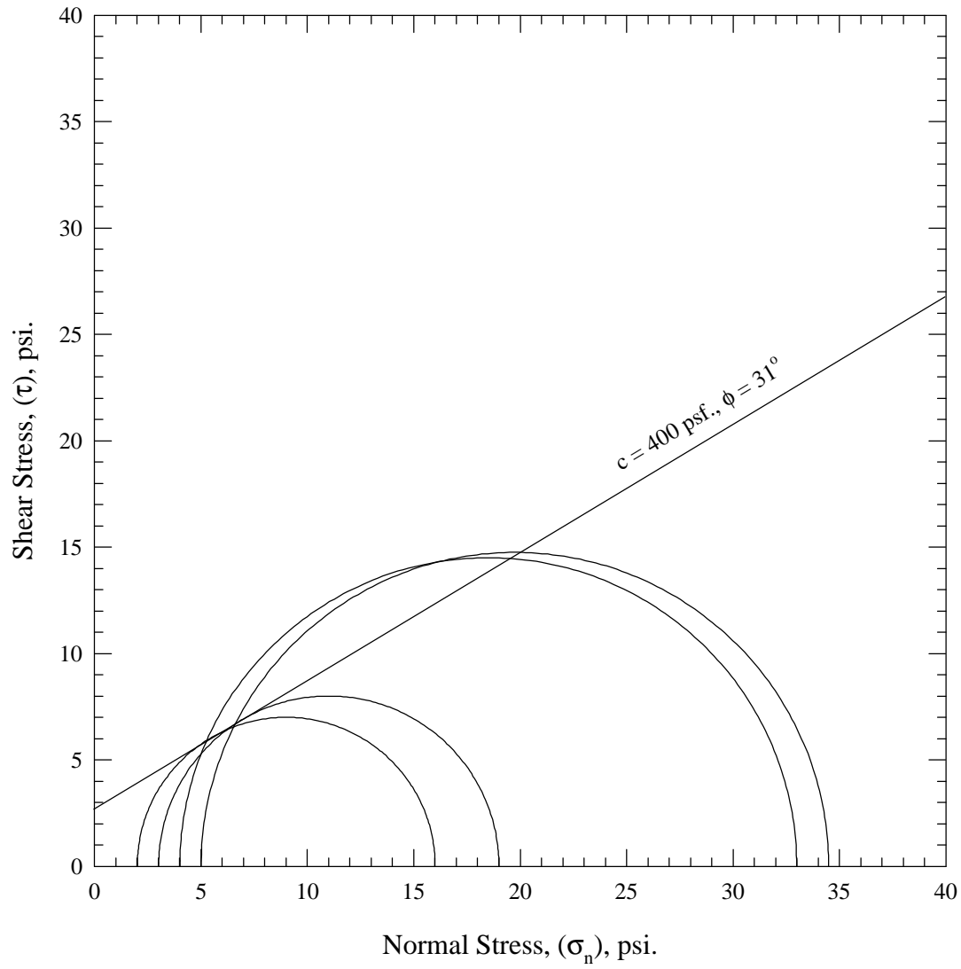
Figure 4.7b: Prices Fork, Strength Envelope
