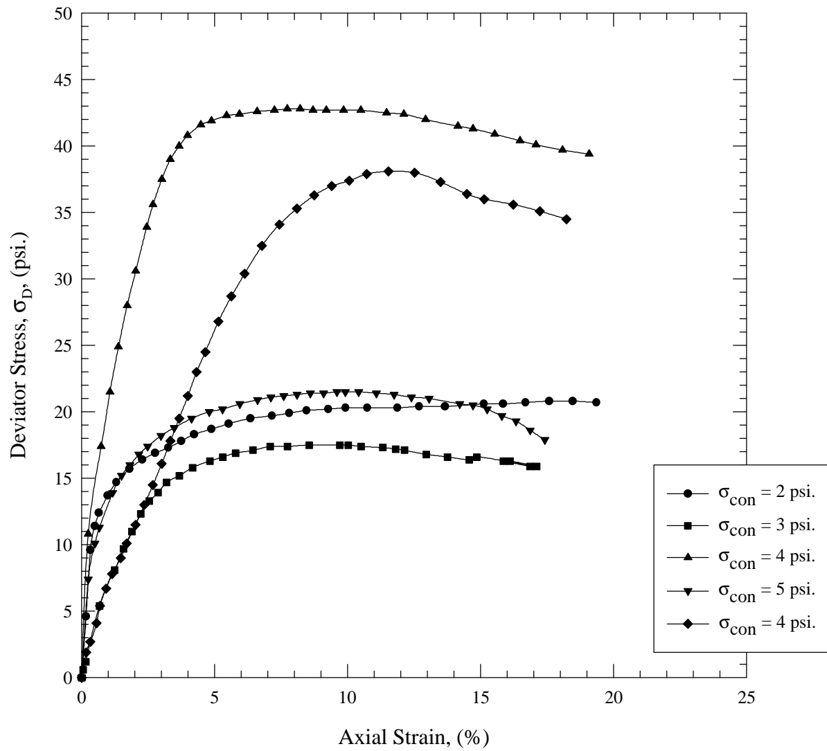
Figure 4.8a: Salem, Deviator Stress vs. Axial Strain Curves
