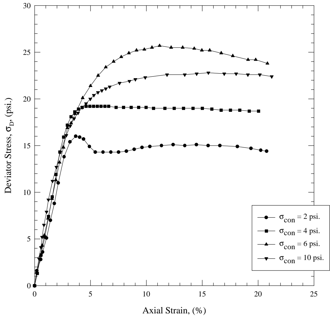
Figure 4.9a: Suffolk, Deviator Stress vs. Axial Strain Curves
