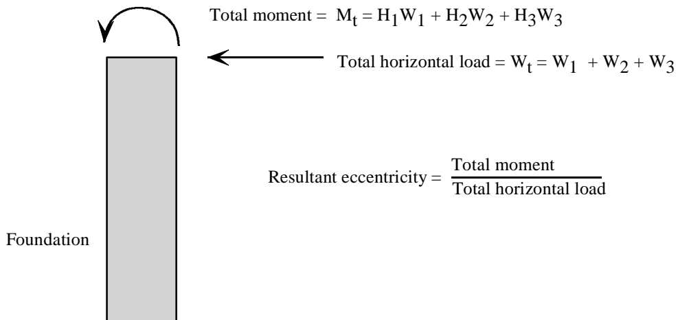
Figure B.1: Moments and Loads on Sound Wall Foundations due to Wind
