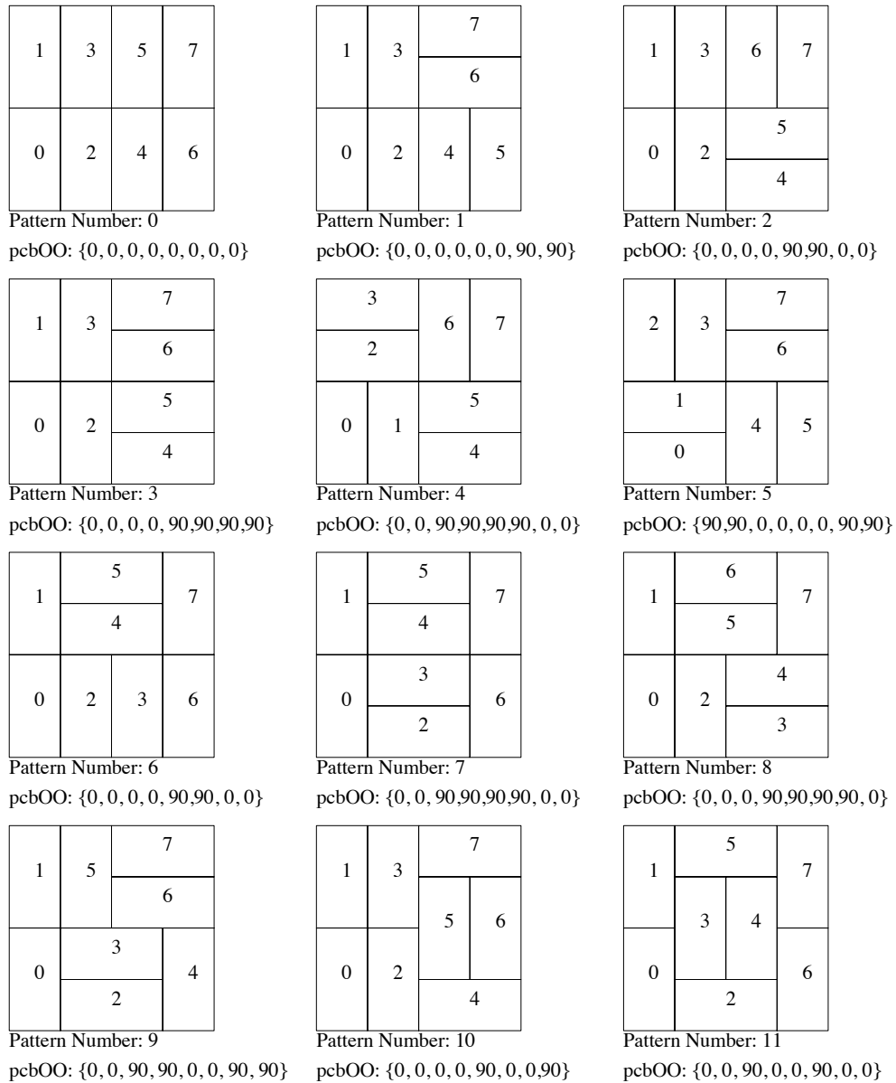
Figure 4.4: Pattern alternatives for the AIM type, 8-PCB experiments.
