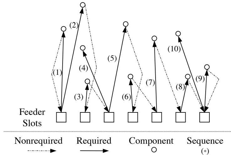
Figure 2.7: Required and nonrequired arcs for a PAPM [3].
