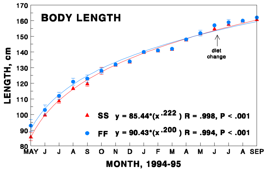
Figure 3.3. Girth circumference and growth curve for body length of 1994 Thoroughbred foals from May 1994 to September 1995 (birth to 16 mo of age).
