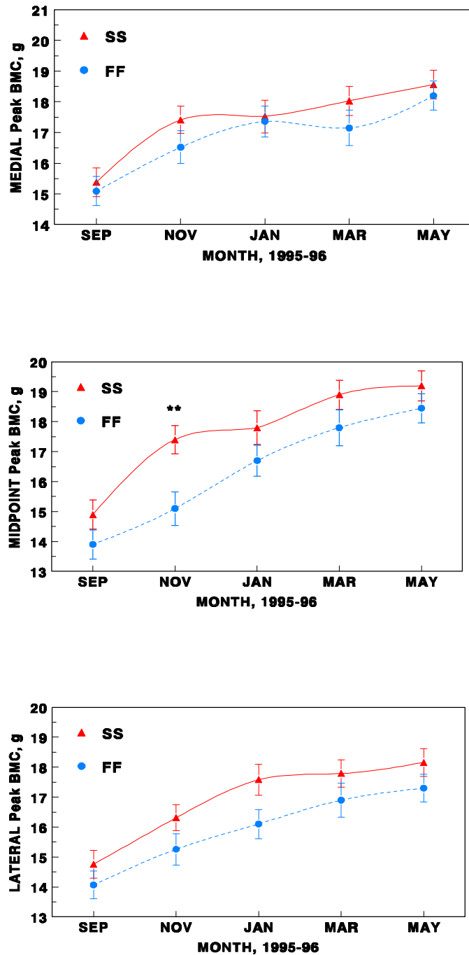
Figure 5.3. Estimated bone mineral content (BMC), expressed as grams per 2 cm section, in 1995 Thoroughbreds from approximately 4 to 12 mo of age. Data are summarized as means \pm standard errors. Dietary treatments were a starch and sugar concentrate (SS) or a fat and fiber supplement (FF).
