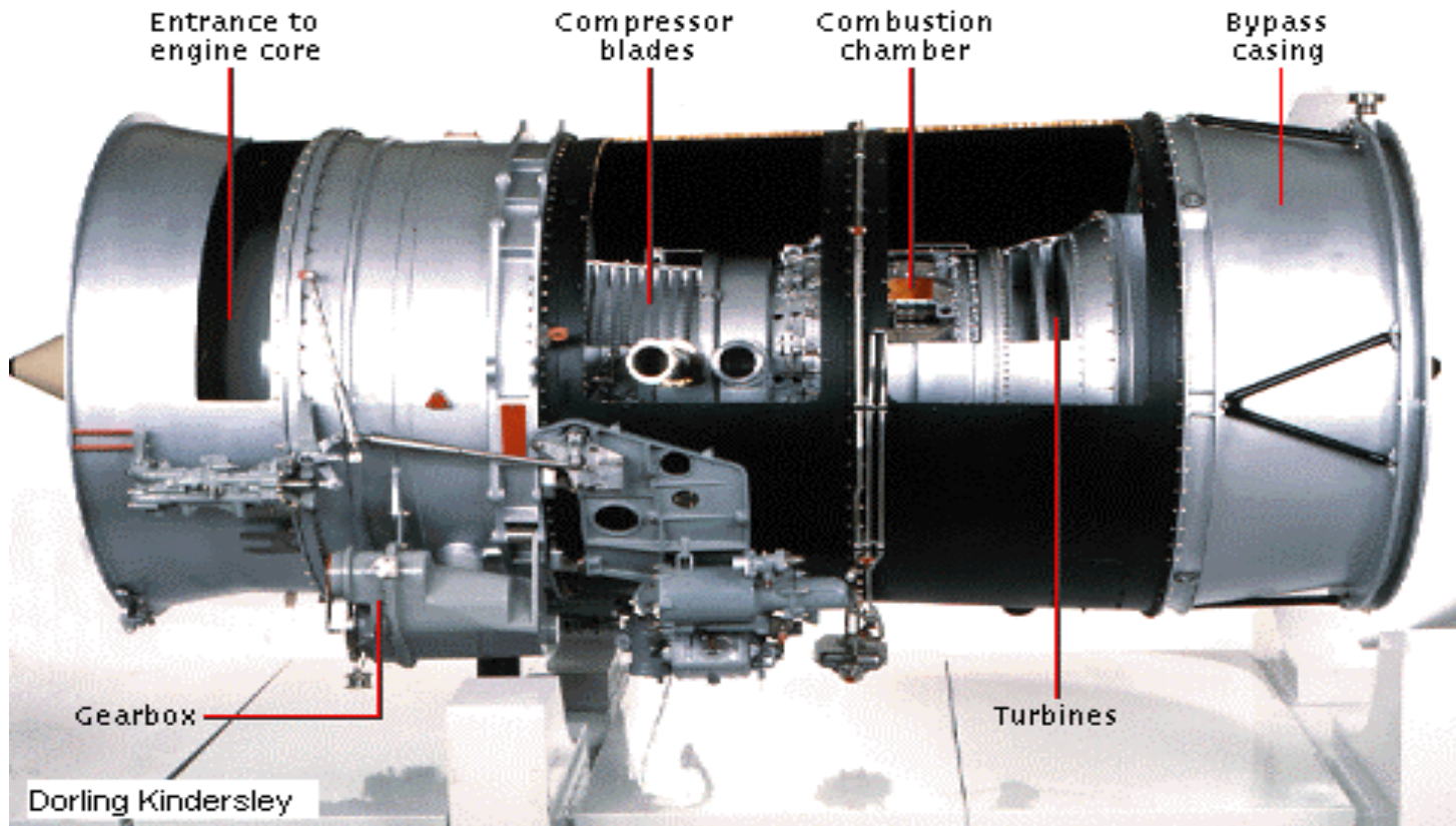
Figure A.1 Turbofan Engine
