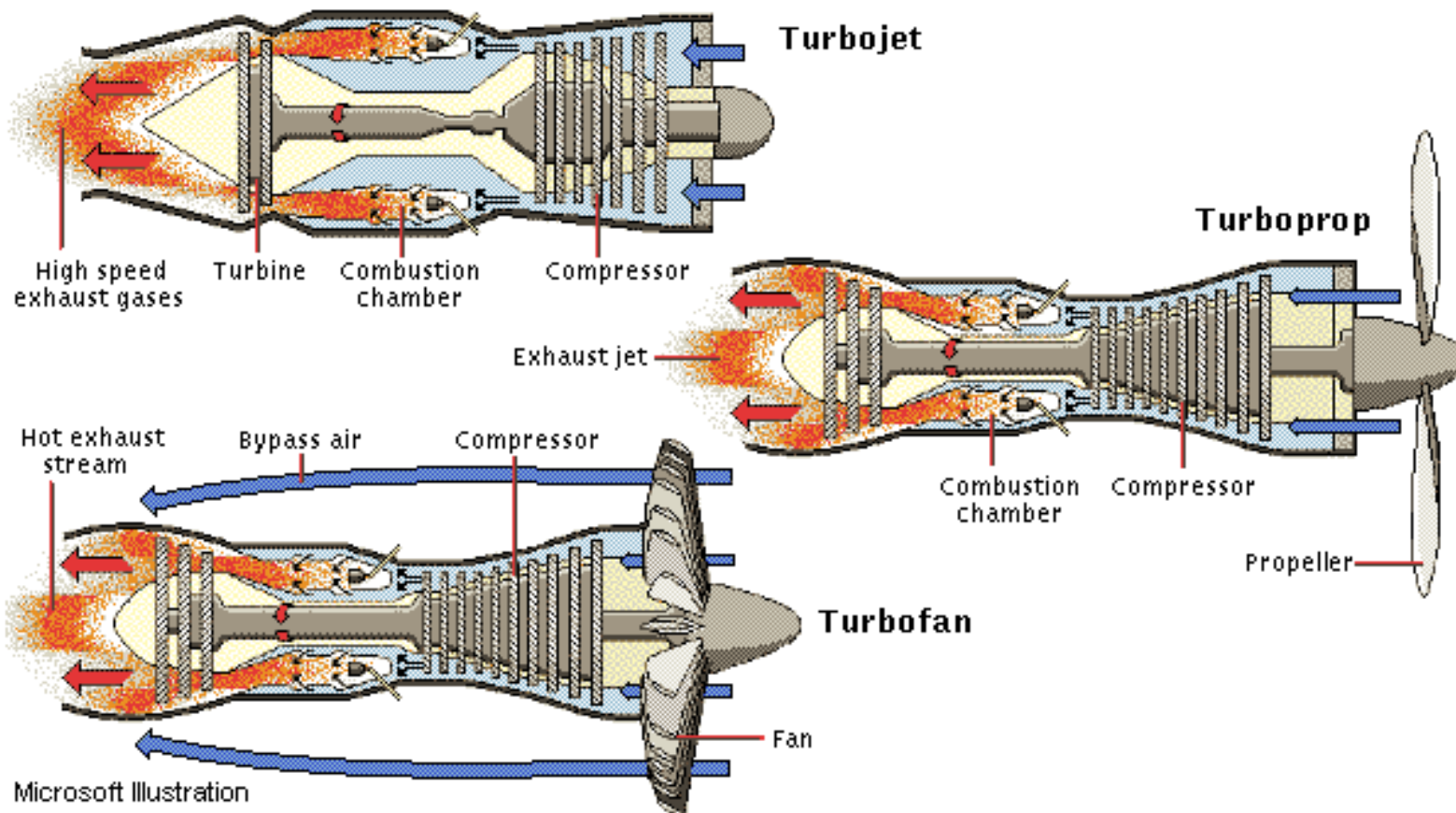
Figure A.2 Jet Engines
