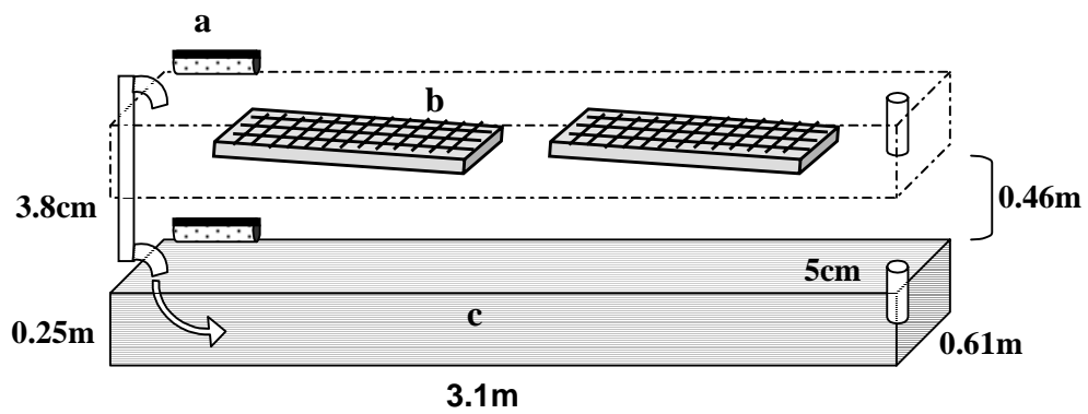
Figure 4.6. Yellow perch incubation troughs: a- fry collection lamp, b- egg ribbon screens, and c- incubation trough.
