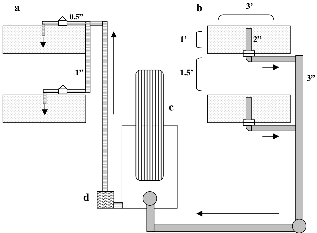
Figure 4.7. Vertical view of yellow perch fry culture system without drum filter: a- delivery line, b- drain line, c- RBC biofilter, d- pump.
