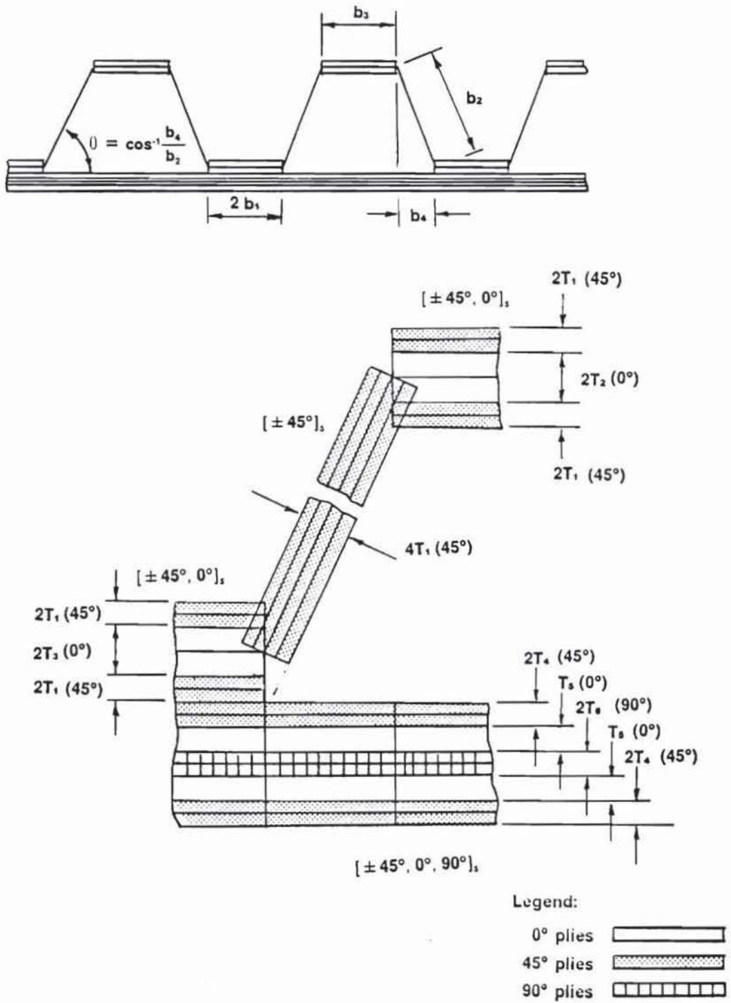
Figure 13. Hat Stiffened Panel Model.
