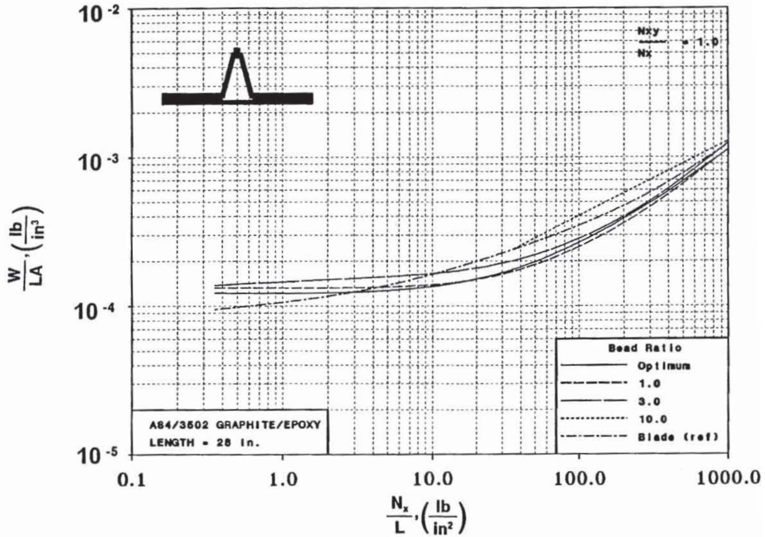
Figure 76. Beading Effect on the Hat Stiffened Panel Structural Efficiency for applied Axial Compression and Shear Loadings (Blade stiffened panel included for comparison).
