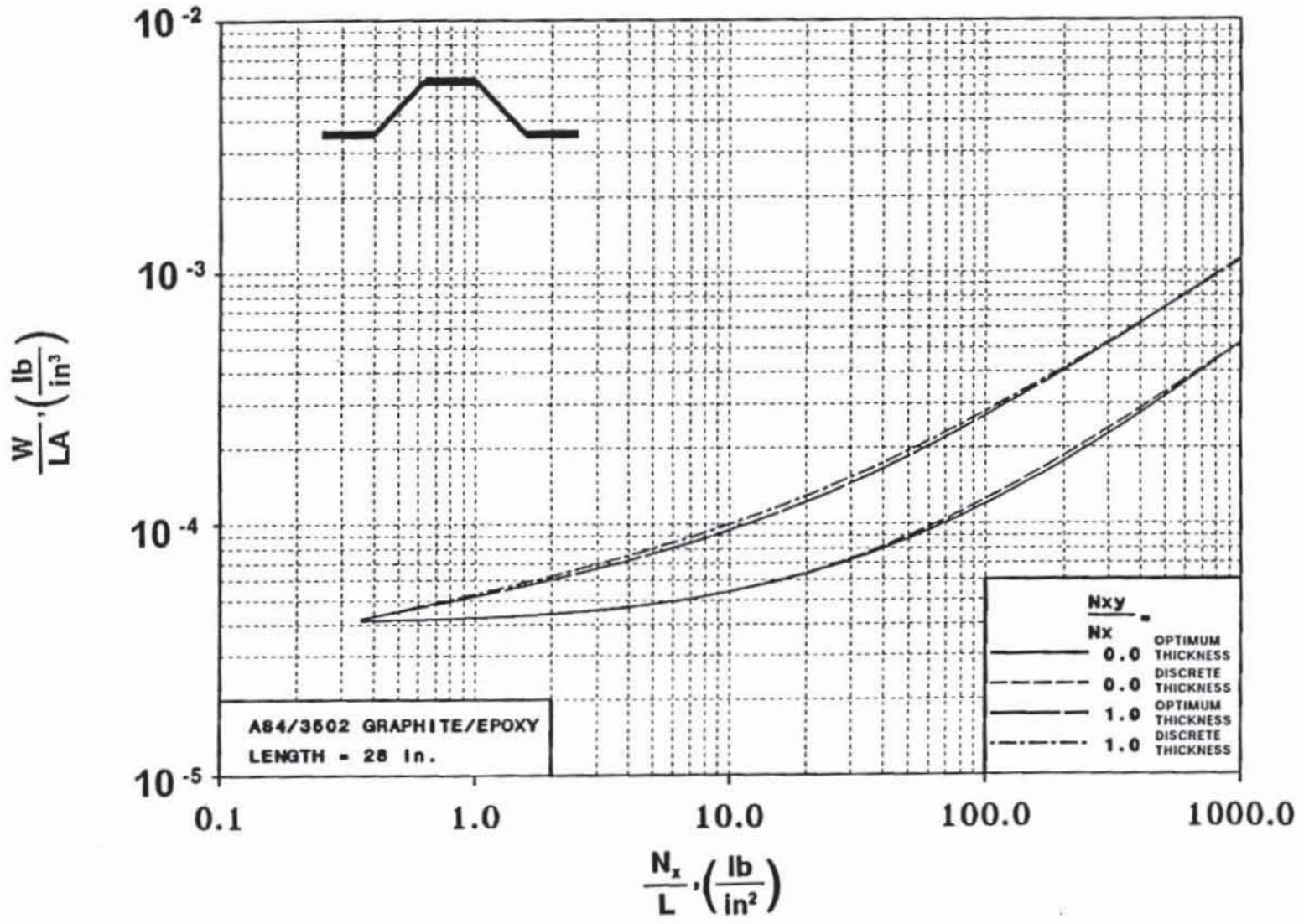
Figure 81. Effect of the Discrete Ply Thickness on Structural Efficiency.
