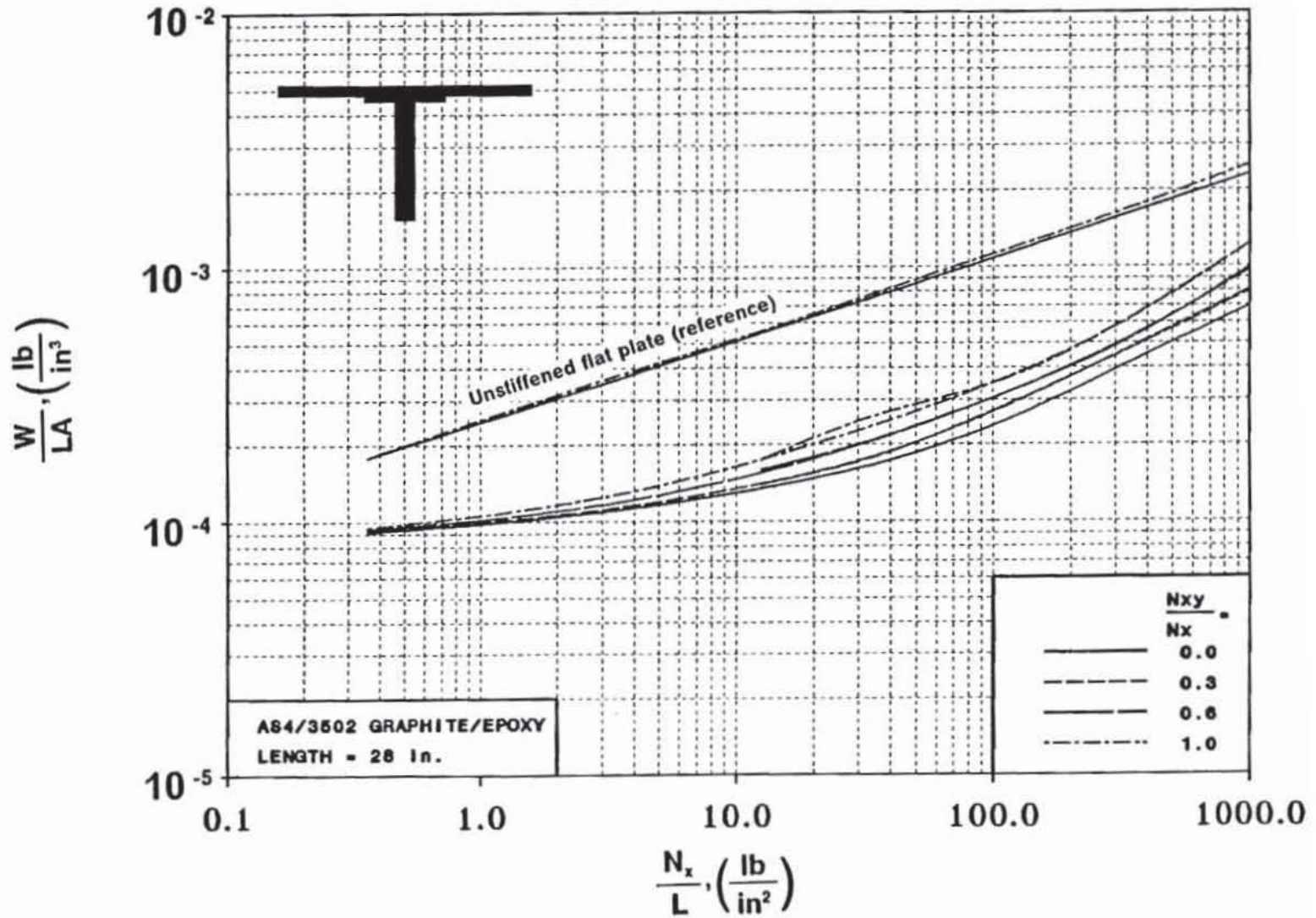
Figure 41. Structural Efficiency Curves for a Blade Stiffened Panel Loaded in Shear.
