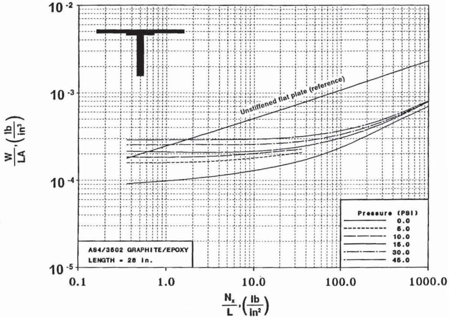
Figure 32. Structural Efficiency Curves of a Blade Stiffened Panel Loaded by Pressure.
