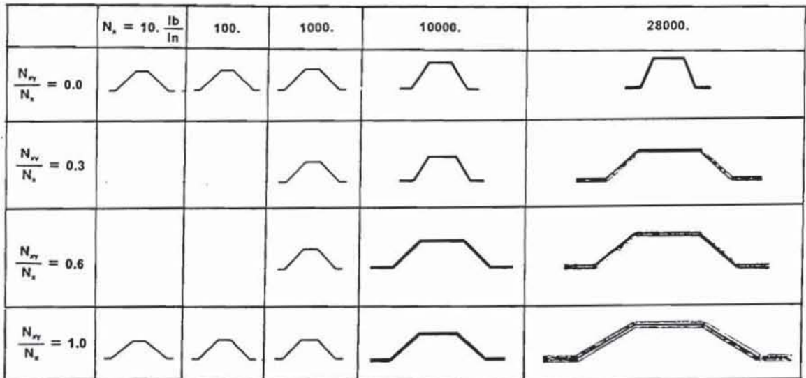
Figure 49. Corrugated Panel with a Continuous Laminate Loaded in Shear ( P=15 \text{ lb/in}^2 ): a) Structural Efficiency and b) Geometry.
