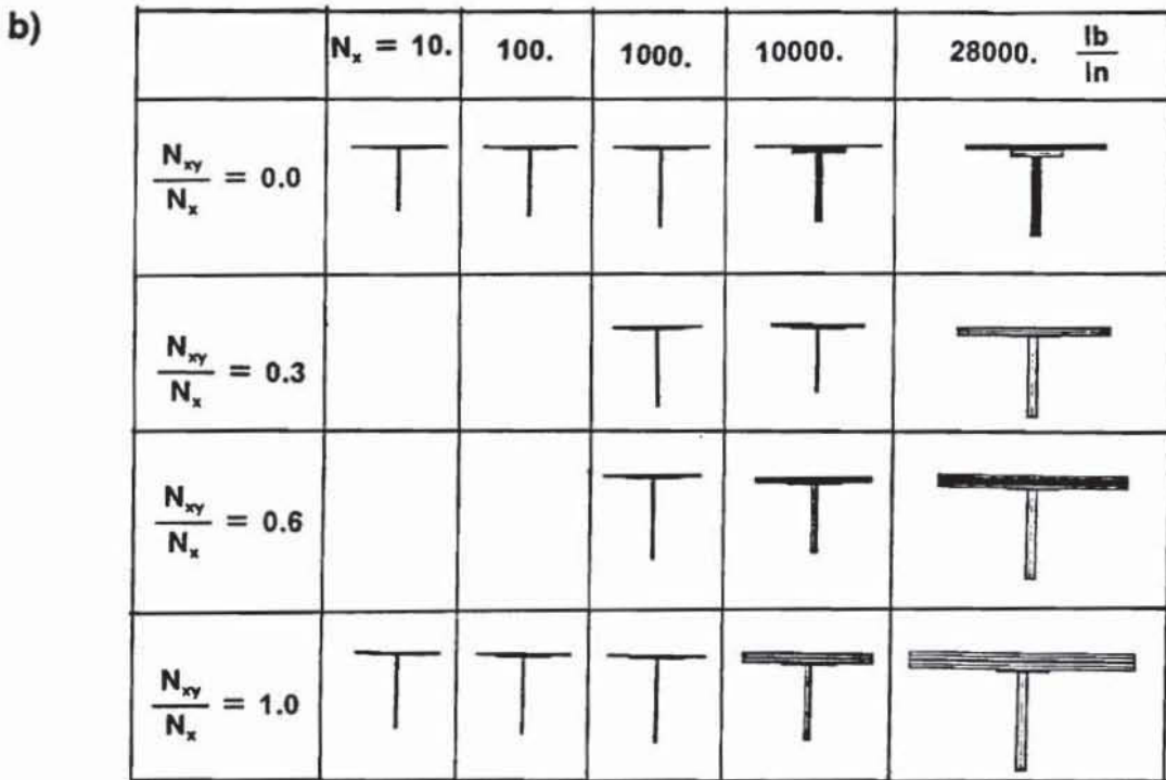
Figure 58. Blade Stiffened Panel Loaded in Shear ( P=30 \text{ lb/in}^2 ): a) Structural Efficiency and b) Geometry.
