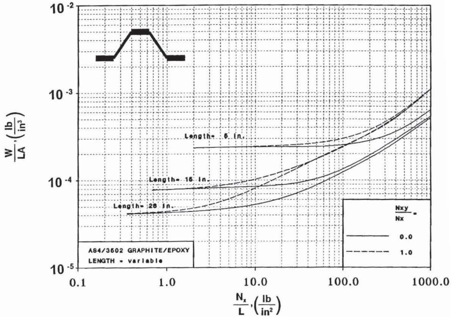
Figure 64. Effect of Panel Length on Structural Efficiency of the Tailored Corrugated Panel.
