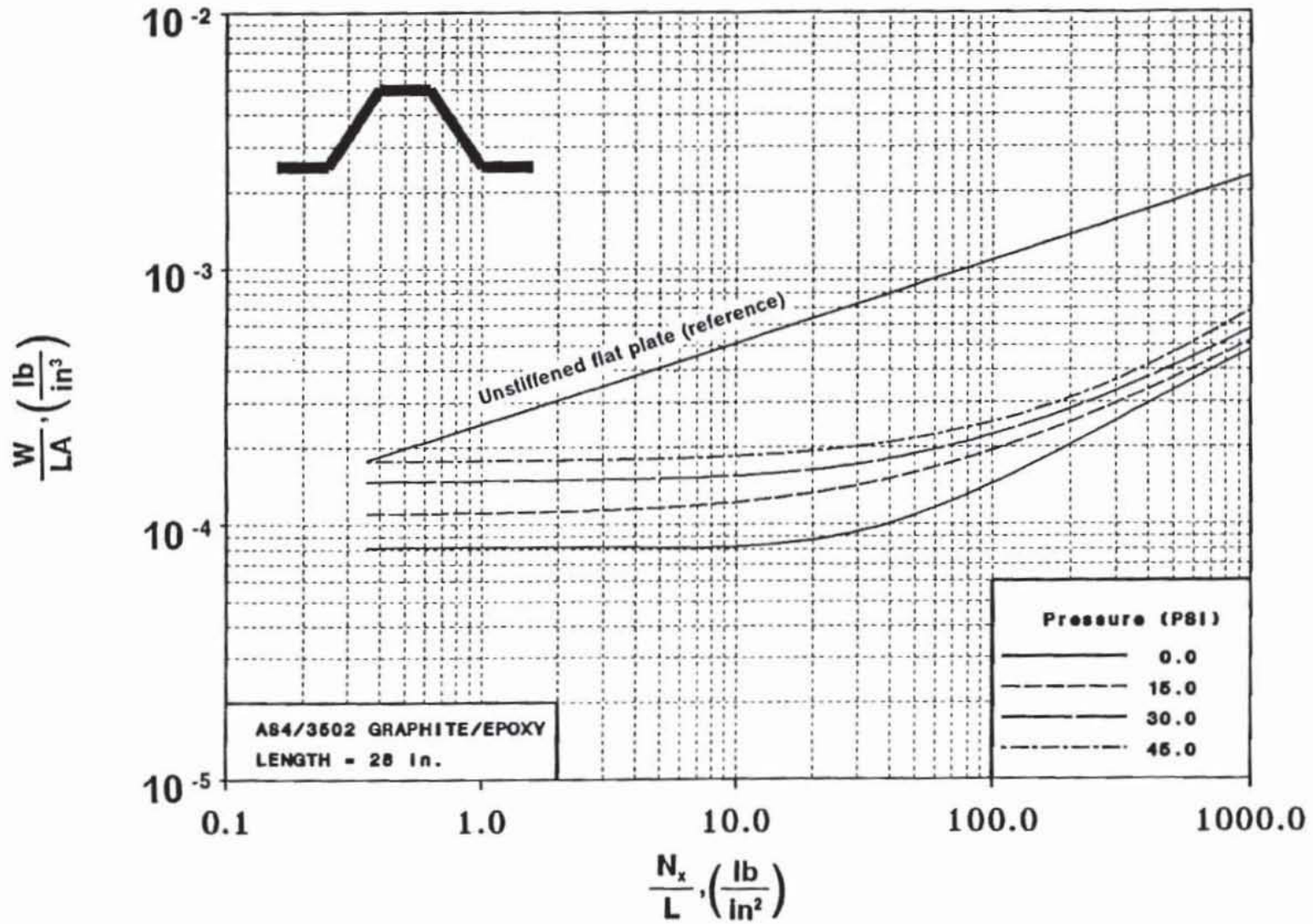
Figure 28. Structural Efficiency Curves for a Corrugated Panel with a Continuous Laminate Loaded by Pressure.
