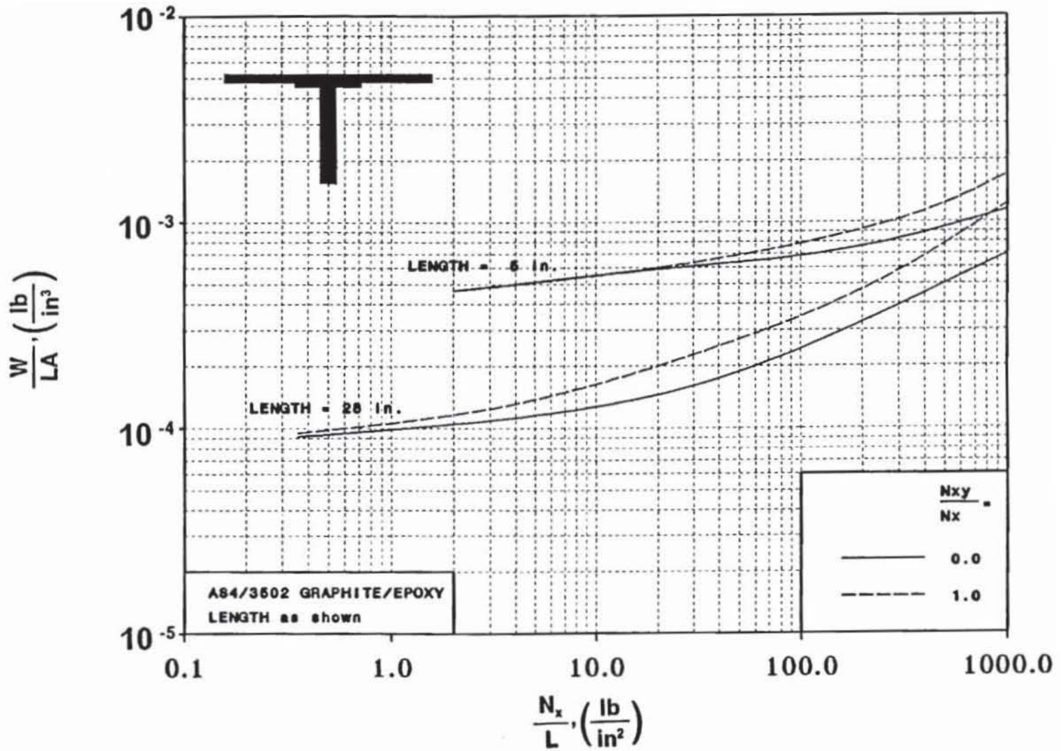
Figure 66. Effect of Panel Length on Structural Efficiency of the Blade Stiffened Panel.
