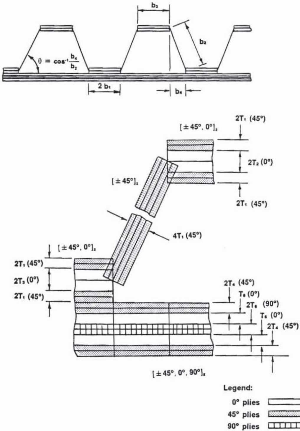
Figure 84. Hat Stiffened Panel Model
