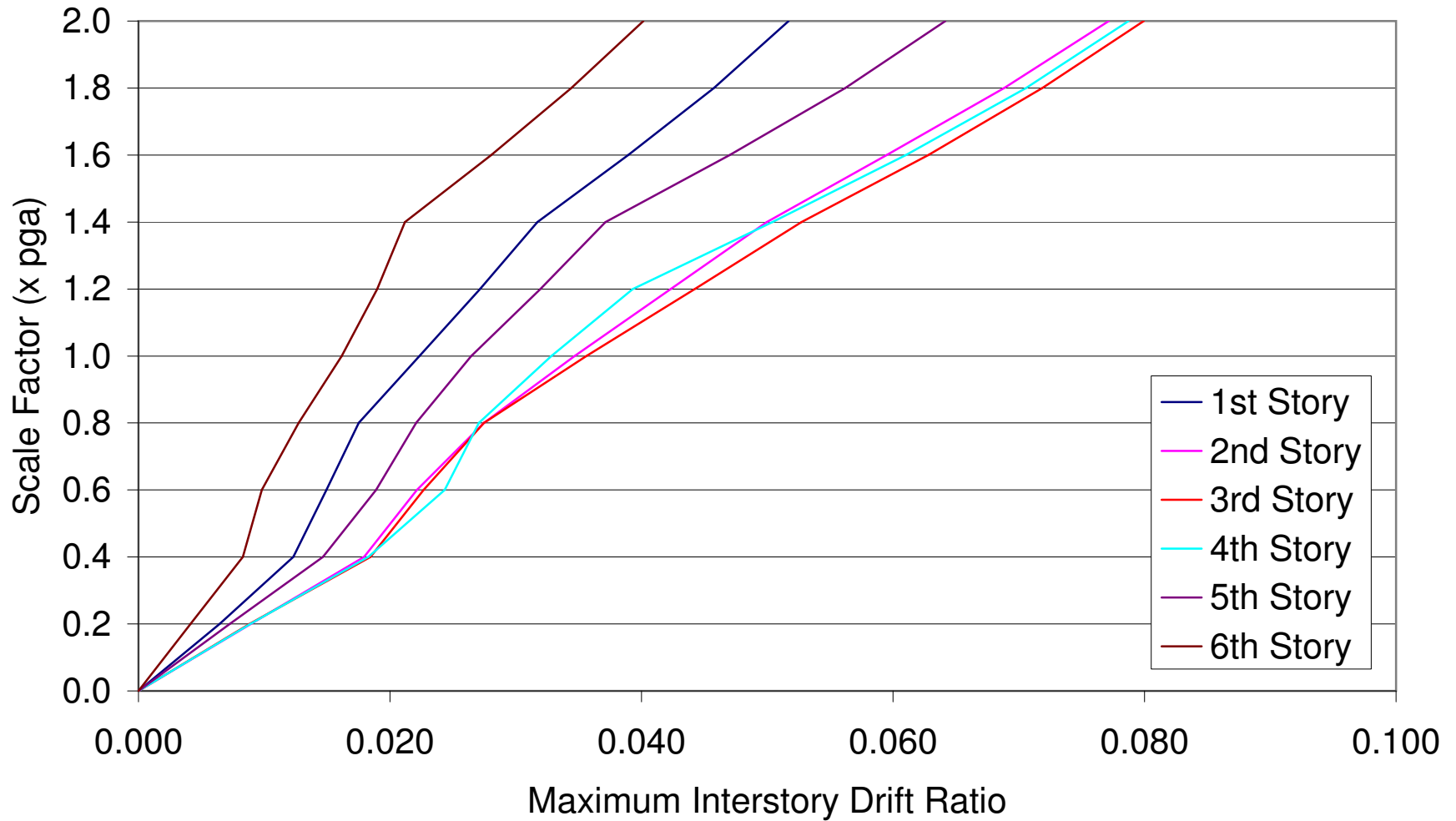
Figure D.12 - Interstory Drift Ratio IDA Curves for P-Delta Case 2 Hyper 1 Frame, Northridge
