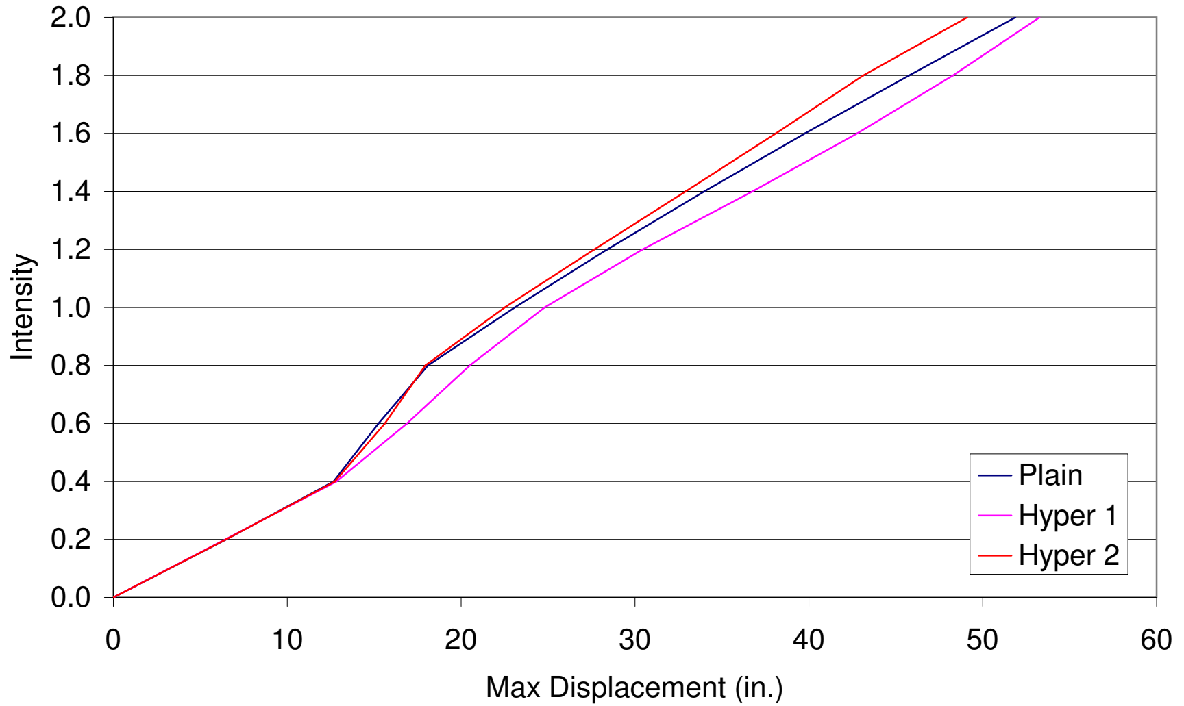
Figure D.7 - Max Displacement IDA Curves for P-Delta Case 1, Northridge
