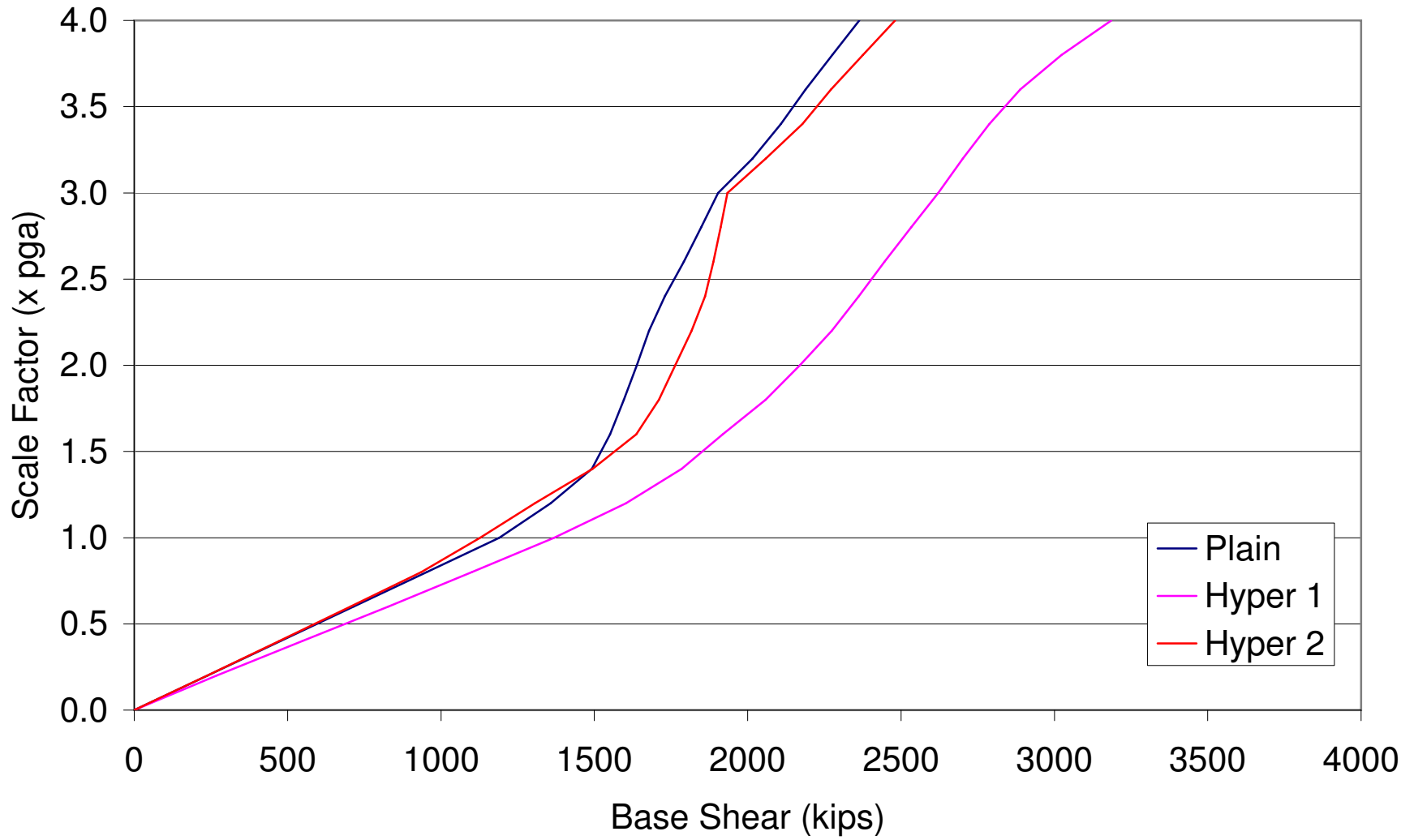
Figure D.9 - Base Shear IDA Curves for P-Delta Case 2 El Centro
