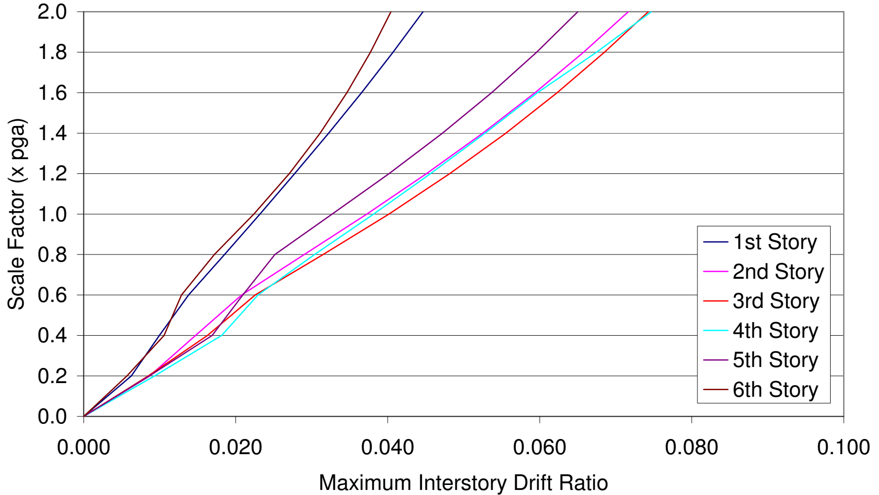
Figure D.13 - Interstory Drift Ratio IDA Curves for P-Delta Case 2 Hyper 2 Frame, Northridge
