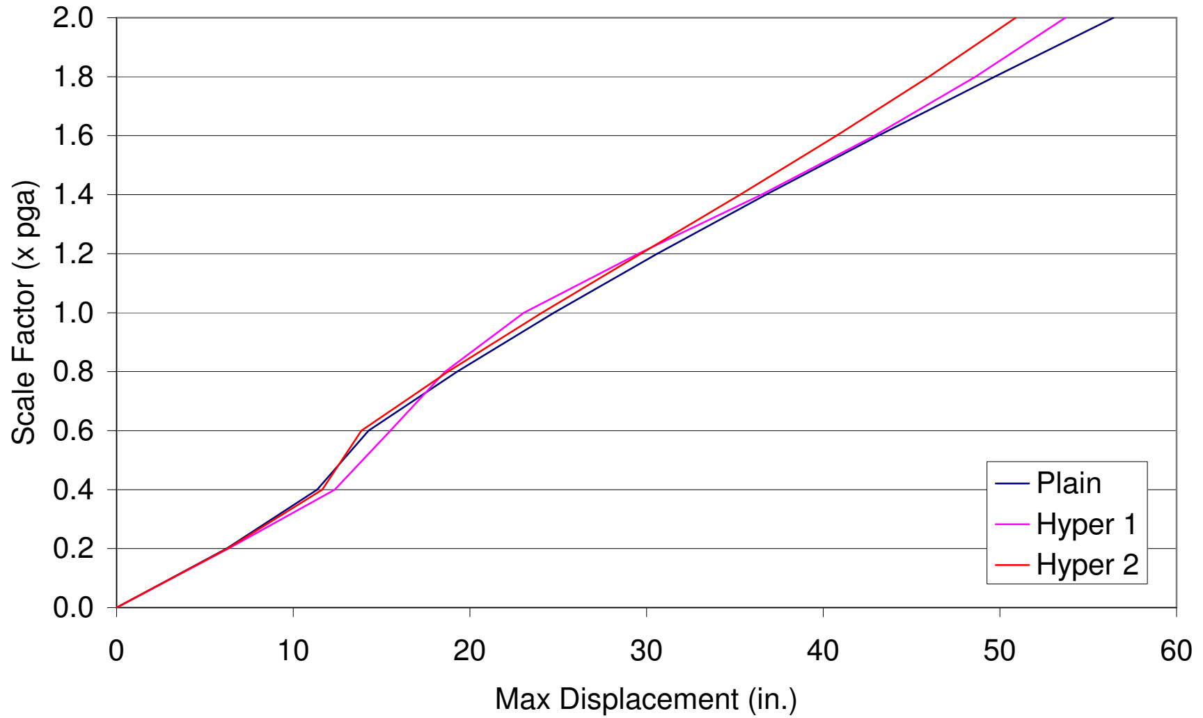
Figure D.14 - Max Displacement IDA Curves for P-Delta Case 2, Northridge
