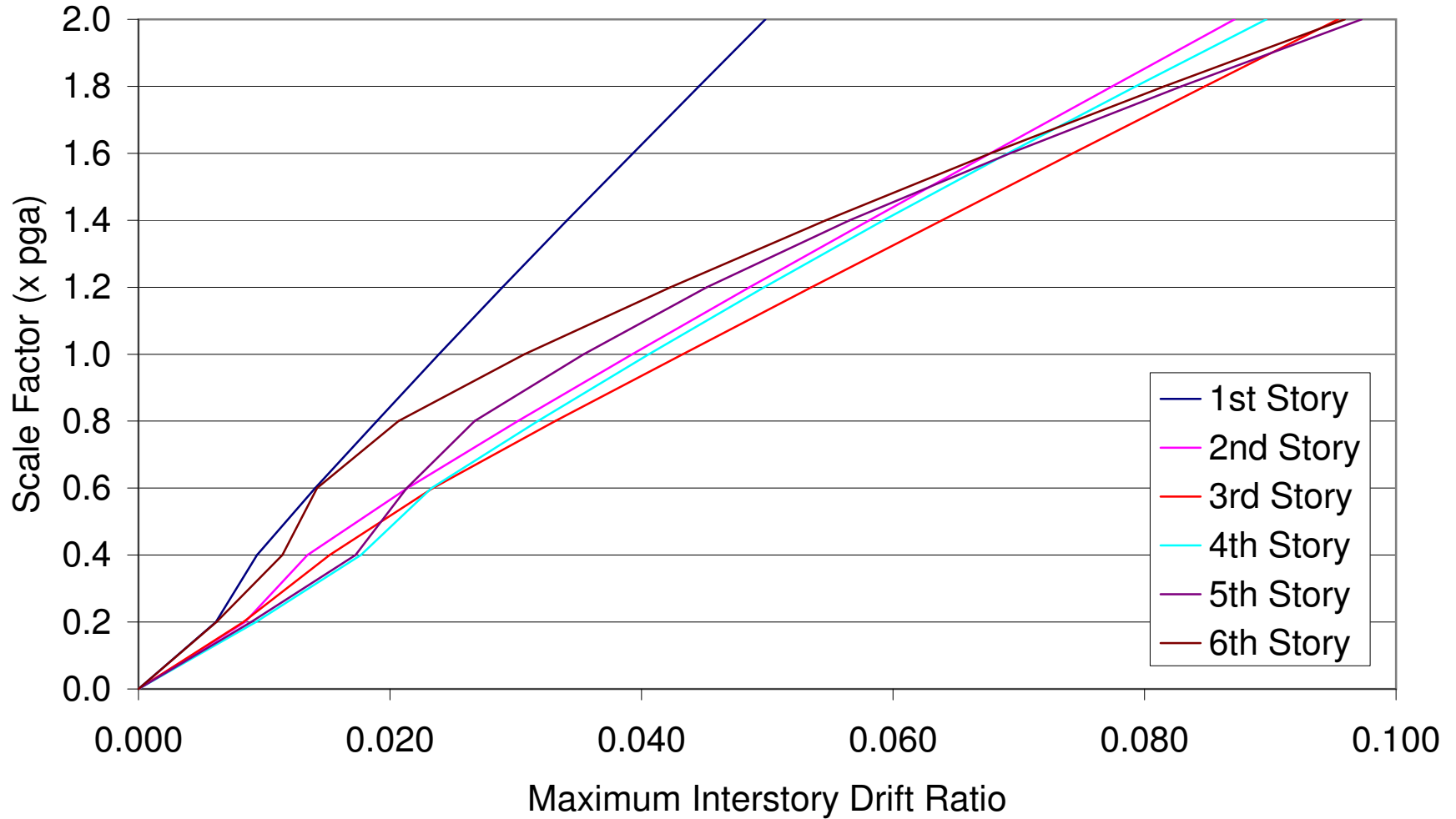
Figure D.11- Interstory Drift Ratio IDA Curves for P-Delta Case 2 Plain Frame, Northridge
