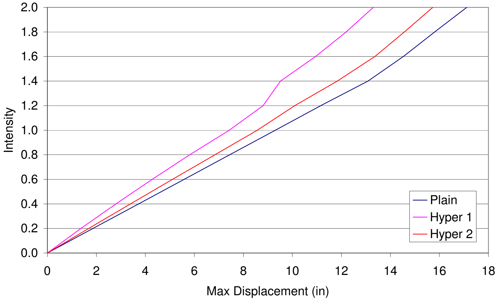
Figure D.3 - Max Displacement IDA Curves for P-Delta Case 1, El Centro
