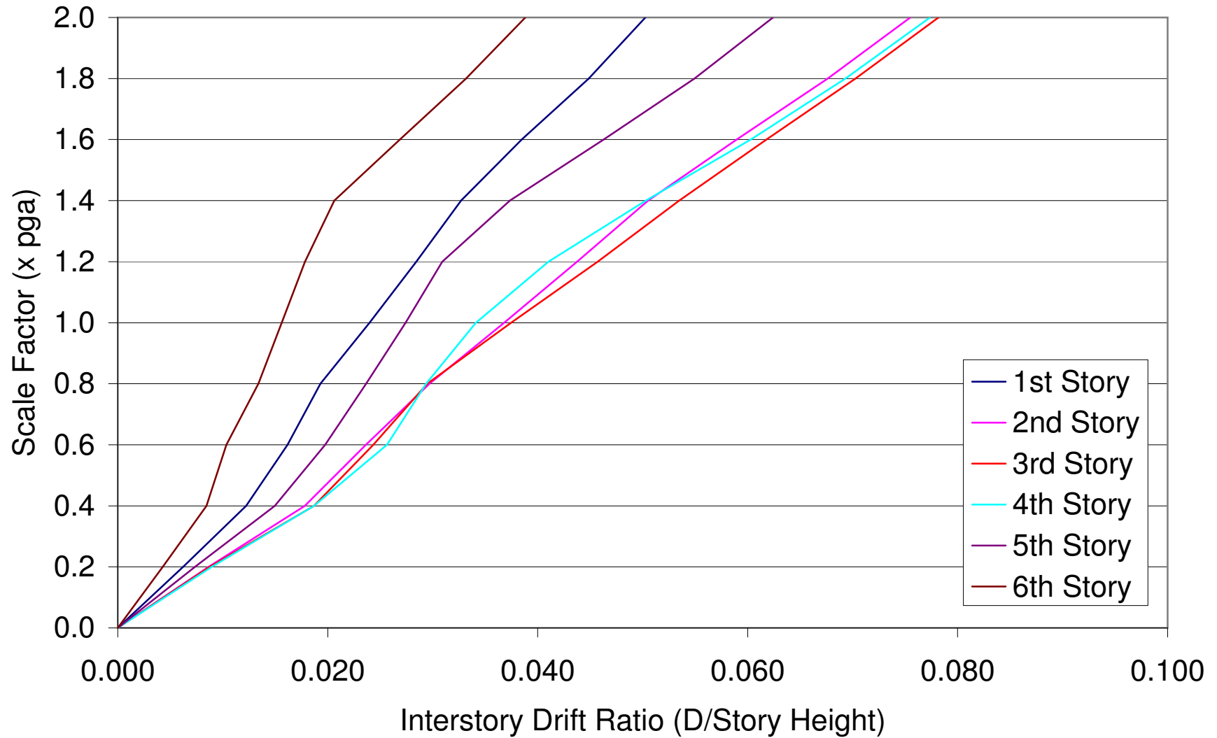
Figure D.5 - Interstory Drift Ratio IDA Curves for P-Delta Case 1 Hyper 1 Frame, Northridge
