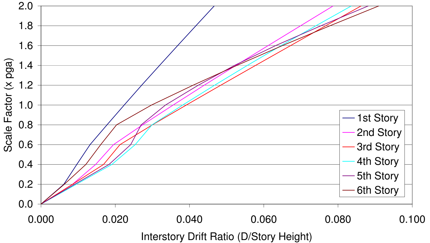
Figure D.4 - Interstory Drift Ratio IDA Curves for P-Delta Case 1 Plain Frame, Northridge
