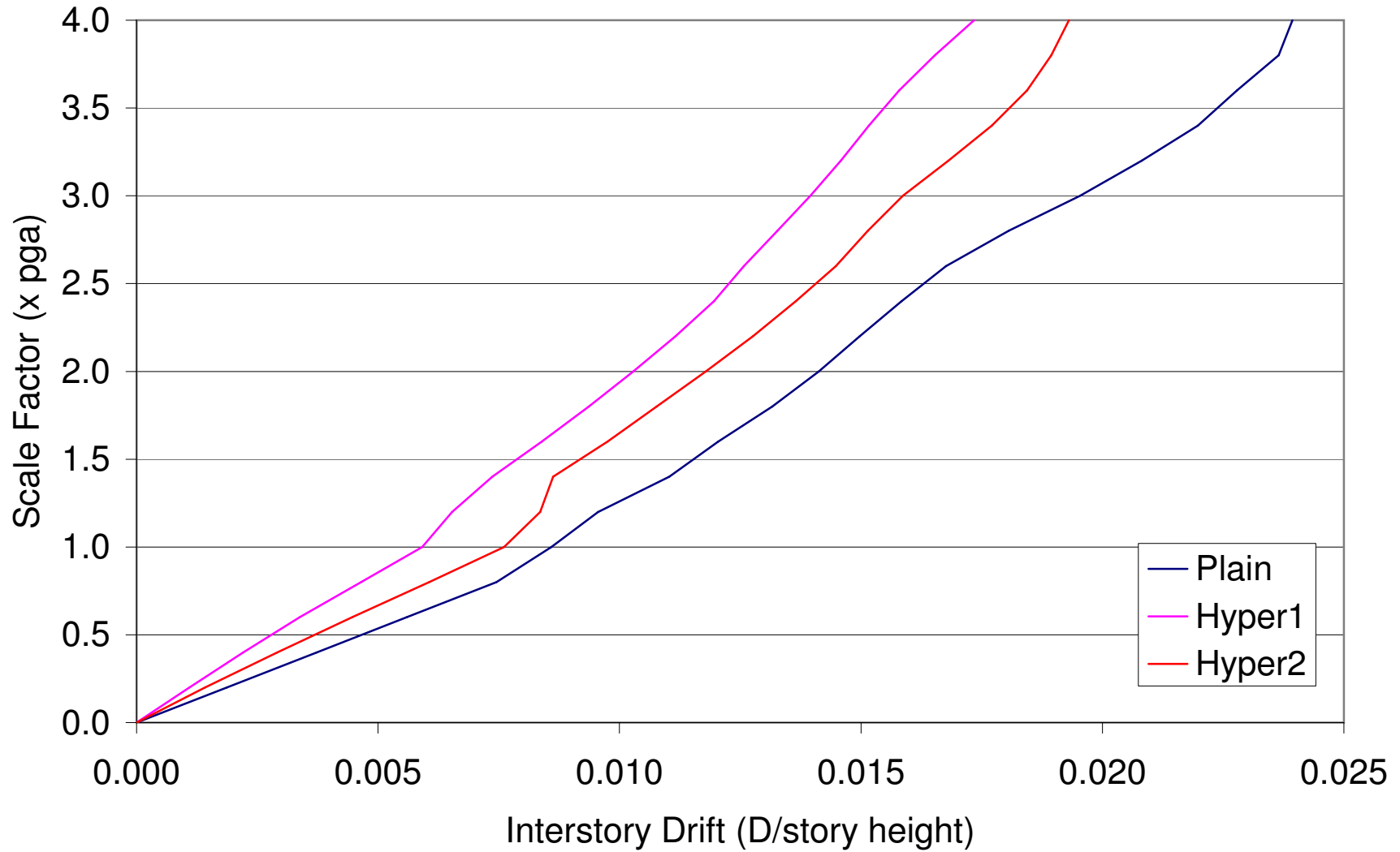
Figure D.8 - Interstory Drift Ratio IDA Curve Summary P-Delta Case 2, El Centro (Sixth Story)
