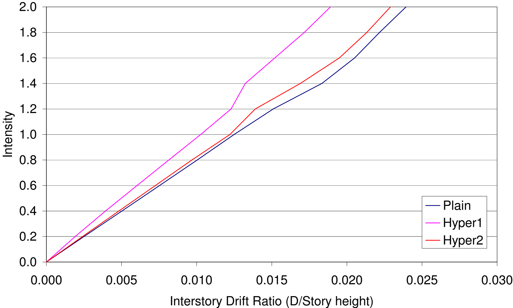
Figure D.1 - Interstory Drift IDA Curve Summary P-Delta Case 1 El Centro (Third Story)
