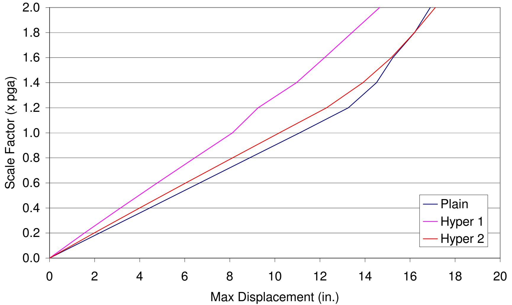
Figure D.10 - Max Displacement IDA Curves for P-Delta Case 2, El Centro
