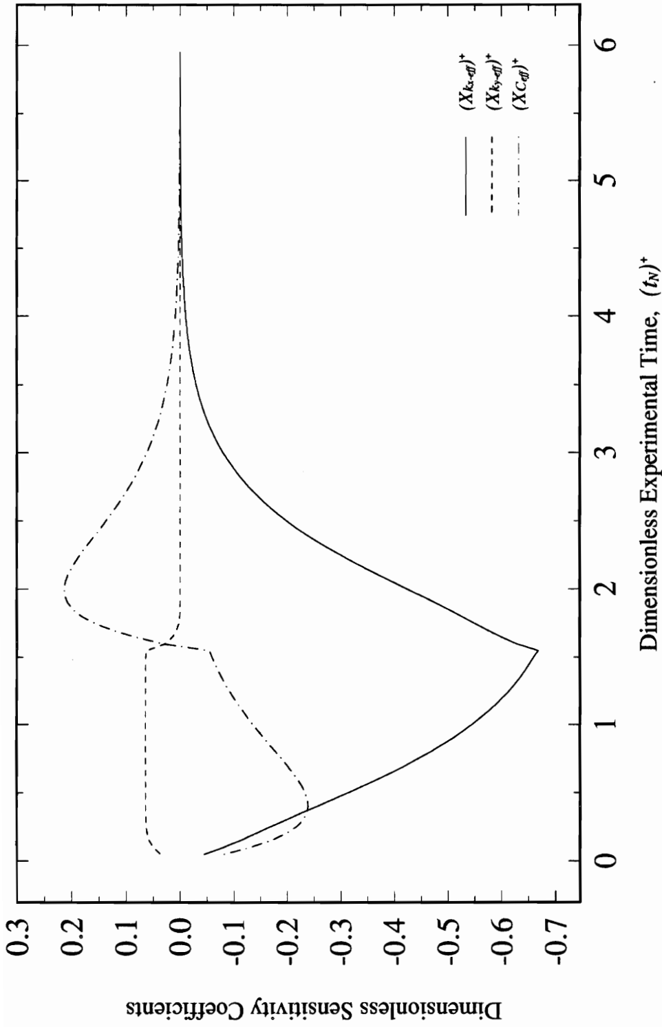
Figure 5.44. Sensitivity Coefficients for Configuration 2 Using a L_{xy} ( L_x/L_y ) of 0.5 and \kappa_{xy} ( k_{y, eff}/k_{x, eff} ) of 7.
