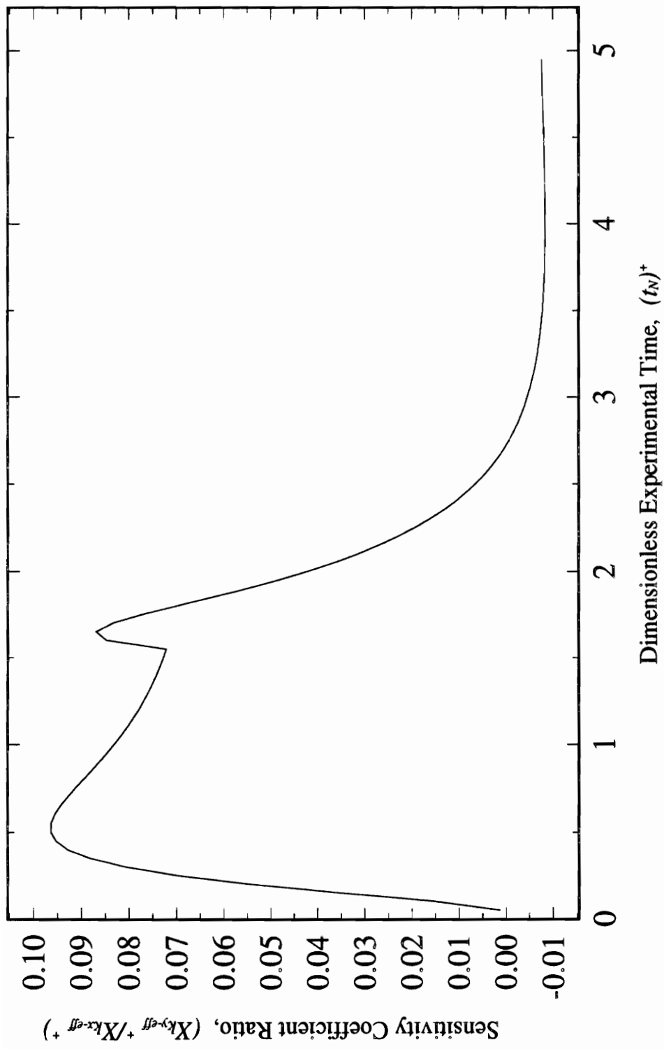
Figure 5.34. Sensitivity Coefficient Ratio, X_{k_y\text{-eff}}^+ / X_{k_x\text{-eff}}^+ to Check for Correlation Between k_{x\text{-eff}} and k_{y\text{-eff}}
