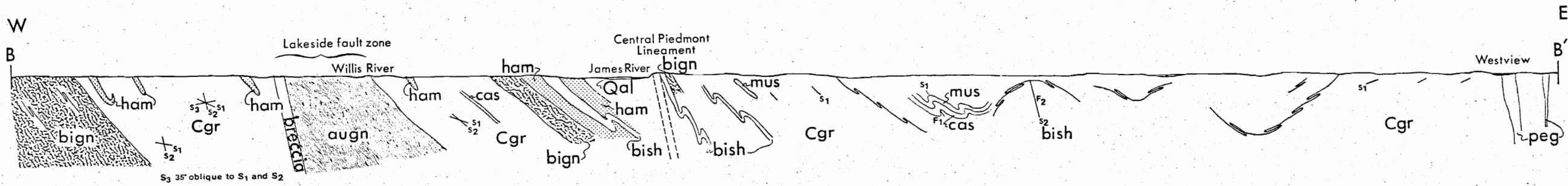
Cross Sections of the Piedmont Along the James River from Columbia to Westview, Virginia
