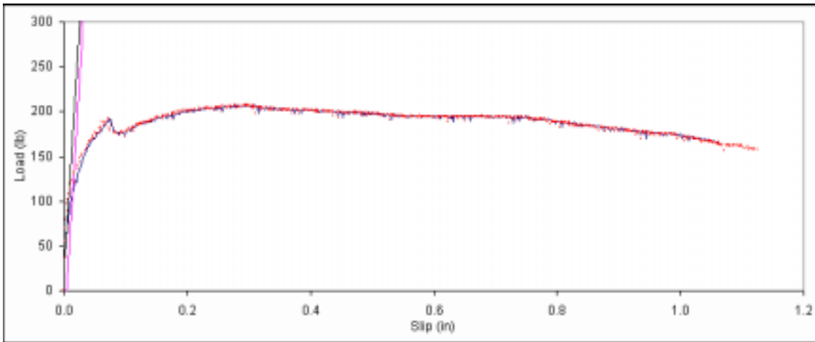
Figure B. 575: Load vs. slip plot for sample F4-13.
