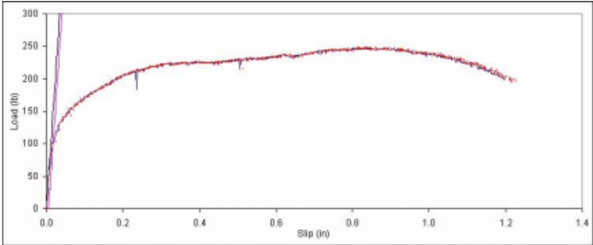
Figure B. 196: Load vs. slip plot for sample B7-4.
