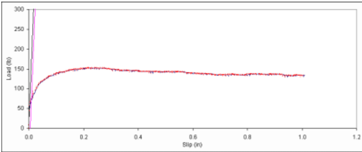
Figure B. 251: Load vs. slip plot for sample C3-15.
