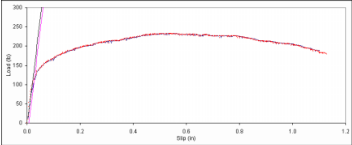
Figure B. 157: Load vs. slip plot for sample B4-10.
