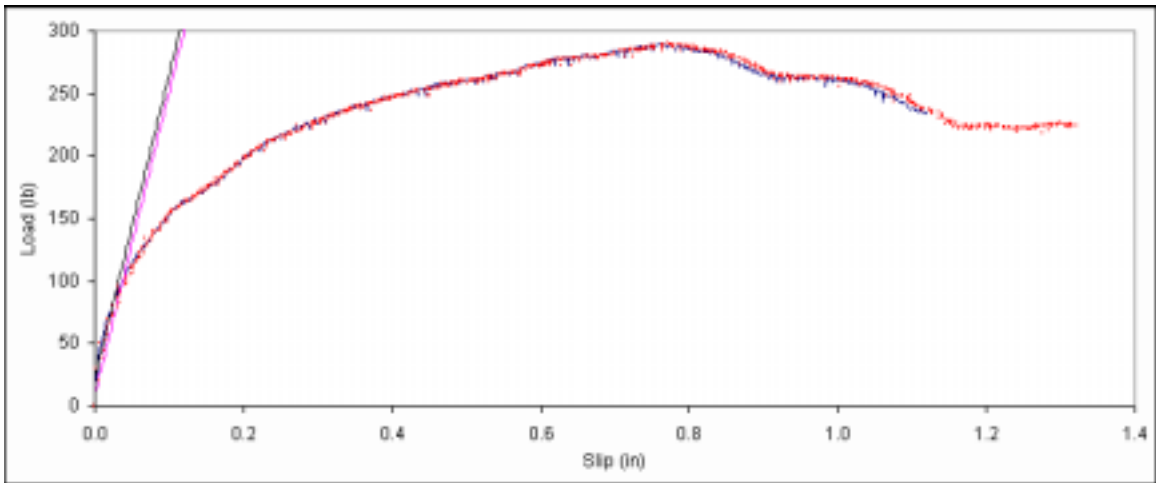
Figure B. 62: Load vs. slip plot for sample A5-3.
