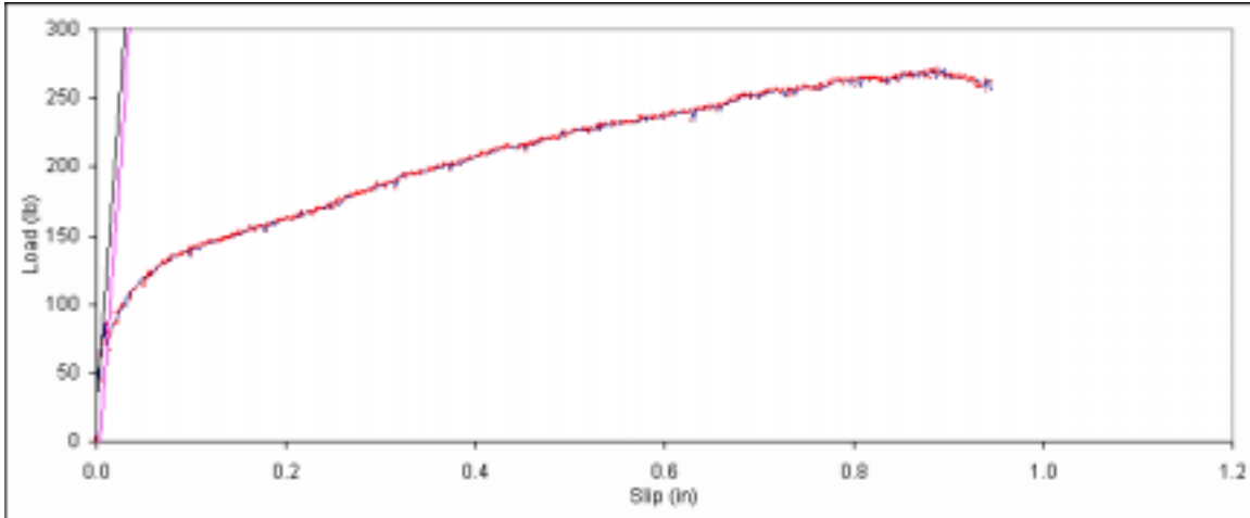
Figure B. 217: Load vs. slip plot for sample C1-10.
