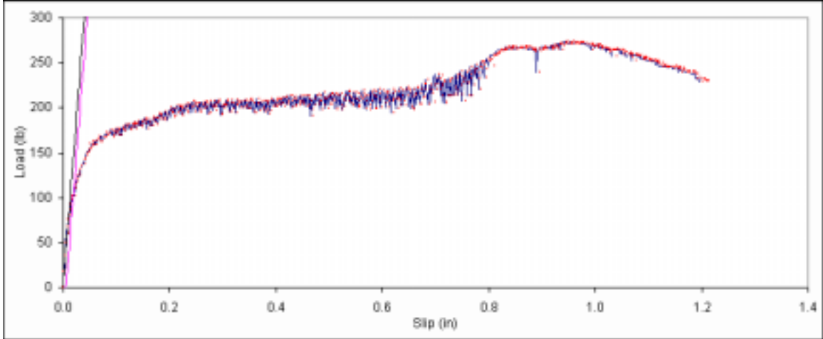
Figure B. 232: Load vs. slip plot for sample C2-10.
