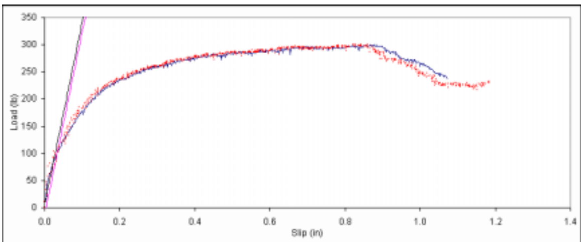
Figure B. 291: Load vs. slip plot for sample C6-10.
