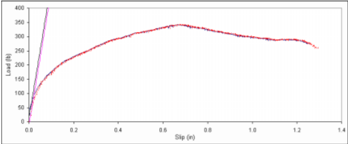
Figure B. 379: Load vs. slip plot for sample D5-9.
