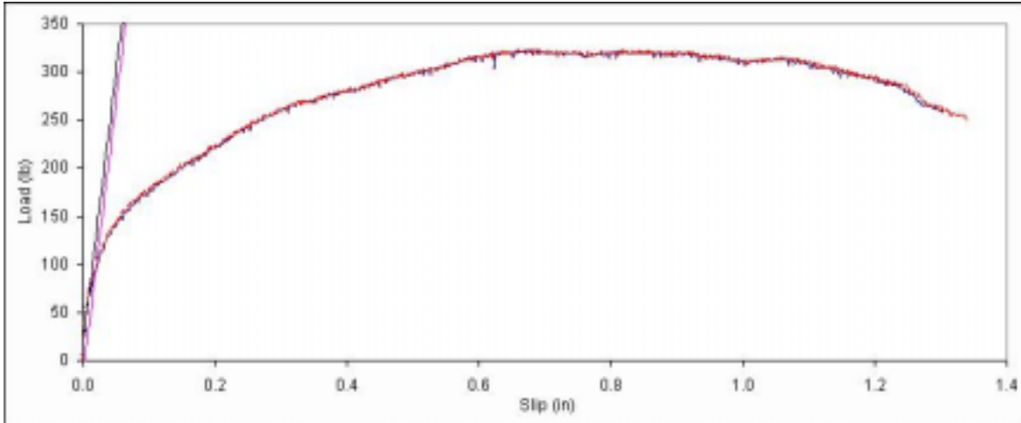
Figure B. 310: Load vs. slip plot for sample C7-14.
