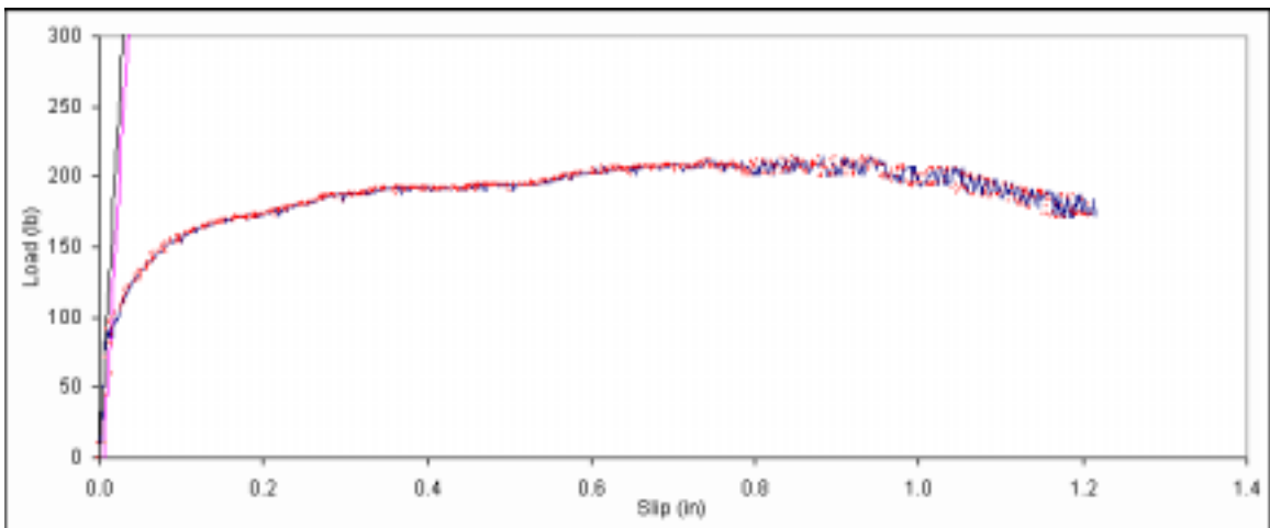
Figure B. 6: Load vs. slip plot for sample A1-6.
