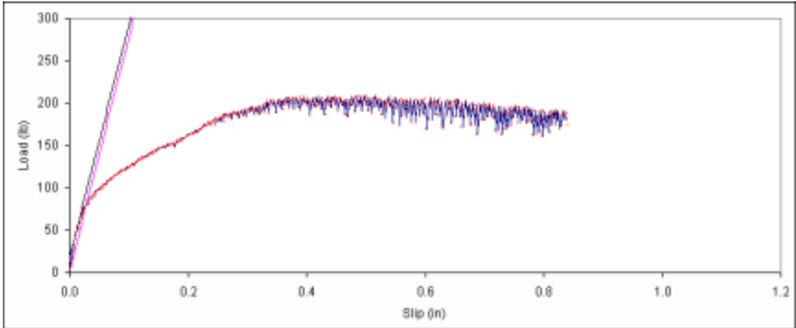
Figure B. 25: Load vs. slip plot for sample A2-11.
