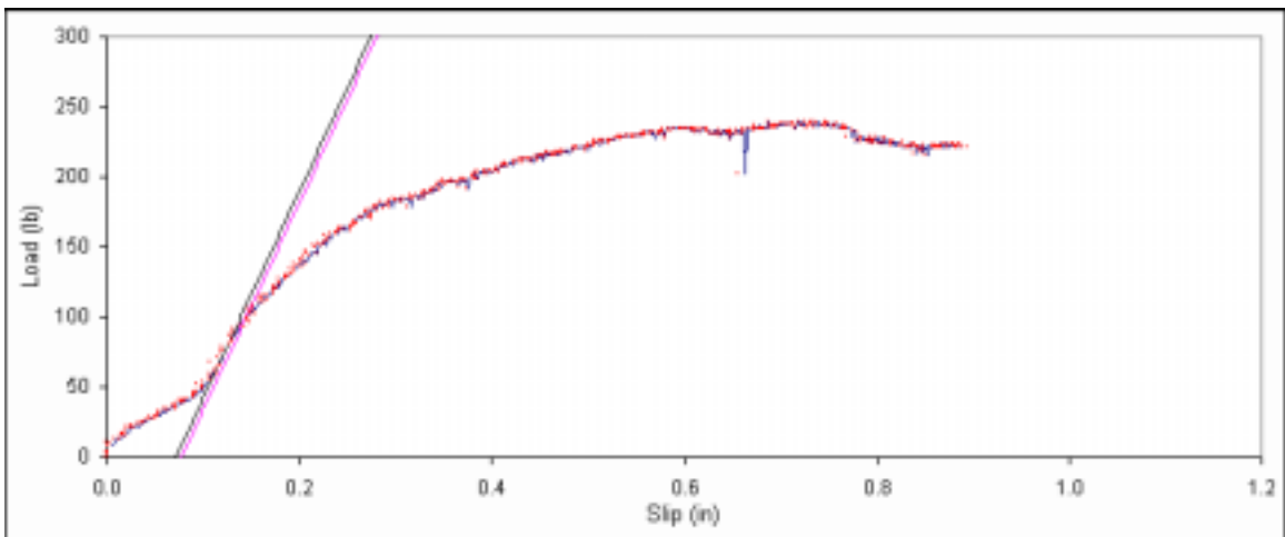
Figure B. 9: Load vs. slip plot for sample A1-9.
