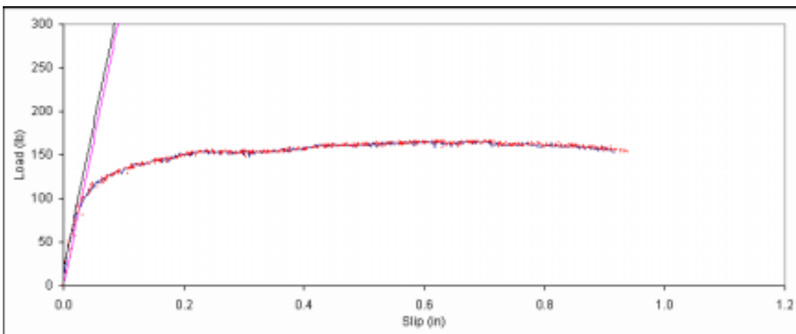
Figure B. 114: Load vs. slip plot for sample B1-12.
