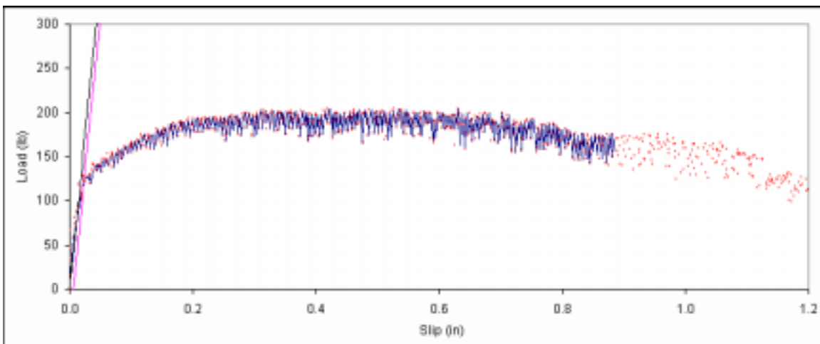
Figure B. 326: Load vs. slip plot for sample D2-1.
