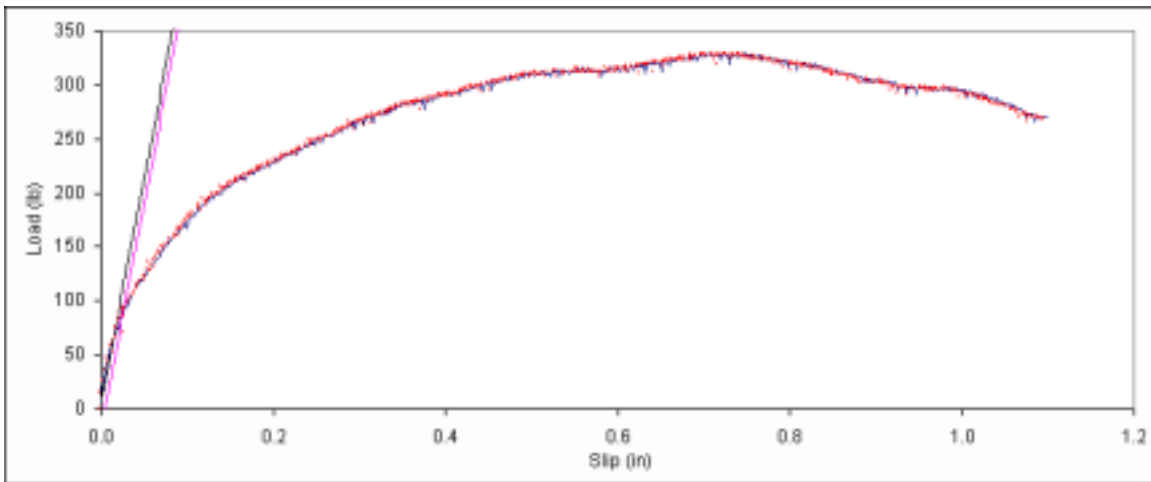
Figure B. 578: Load vs. slip plot for sample F5-1.
