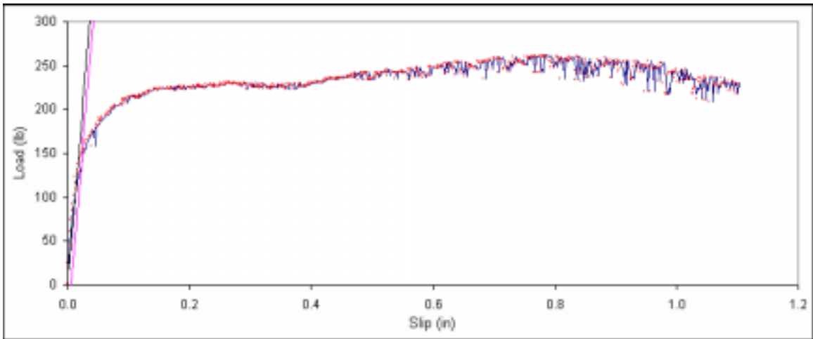
Figure B. 23: Load vs. slip plot for sample A2-9.
