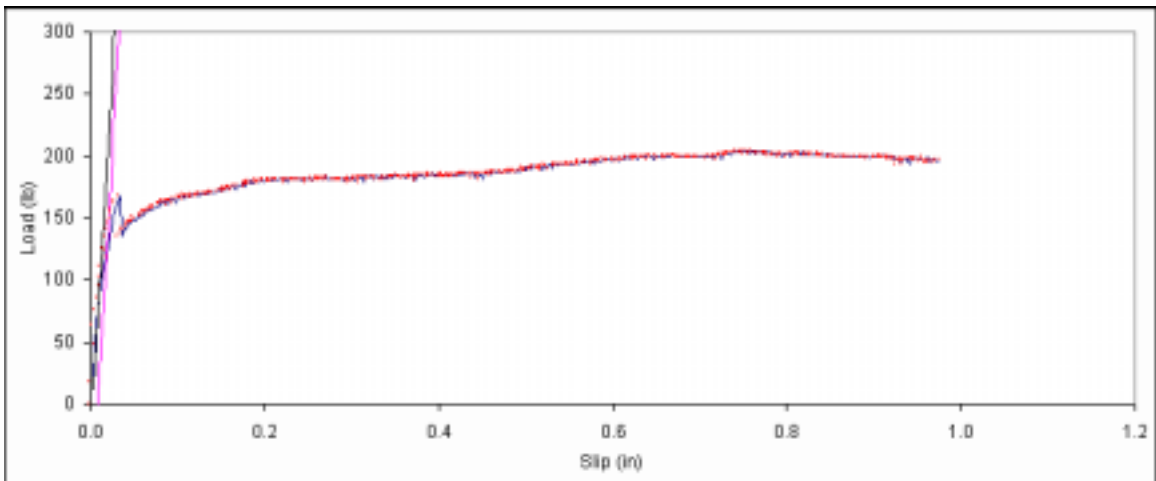
Figure B. 318: Load vs. slip plot for sample D1-7.
