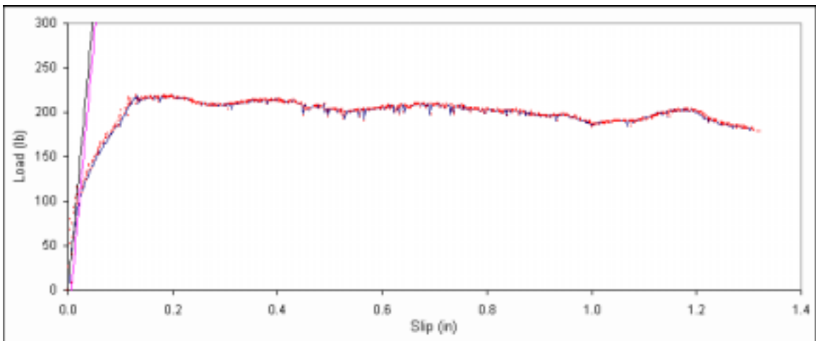
Figure B. 126: Load vs. slip plot for sample B2-9.
