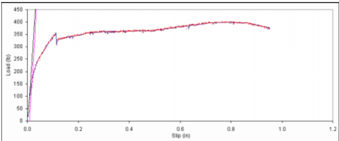
Figure B. 546: Load vs. slip plot for sample F2-14.
