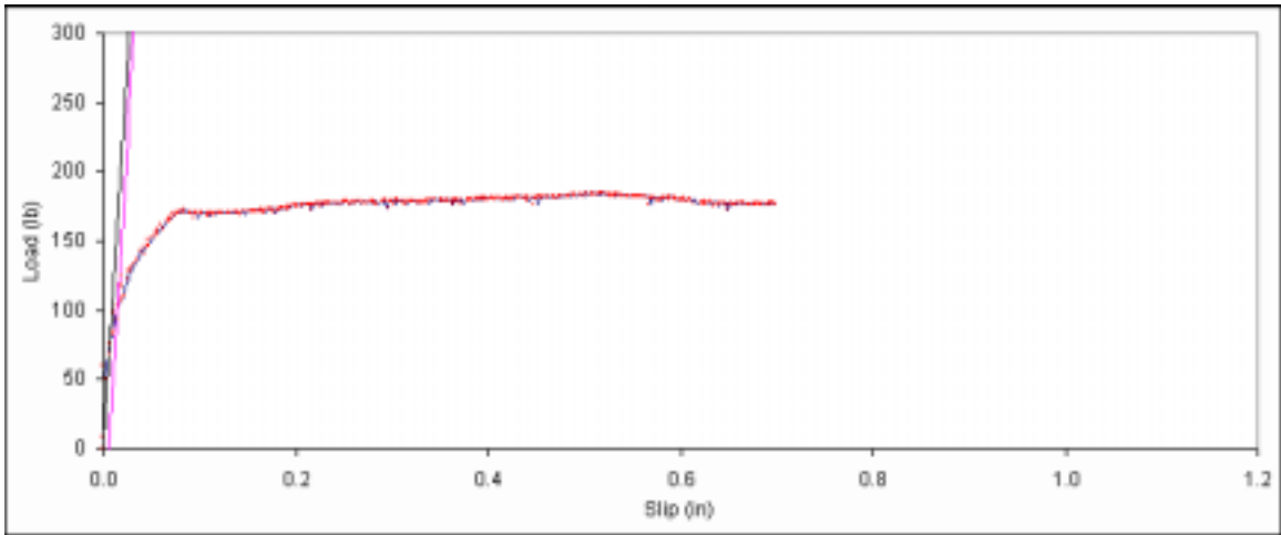
Figure B. 320: Load vs. slip plot for sample D1-10.
