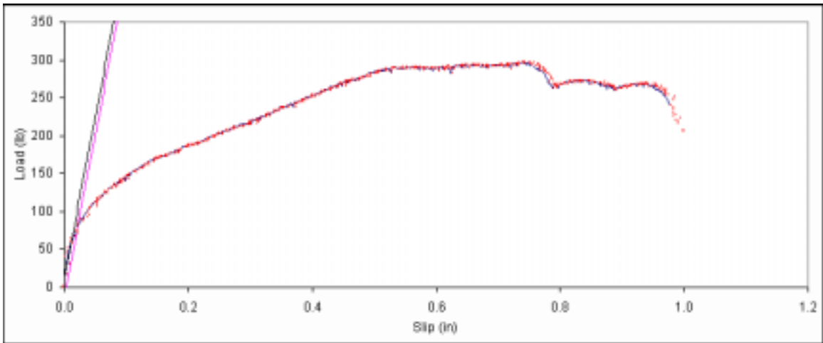
Figure B. 377: Load vs. slip plot for sample D5-7.
