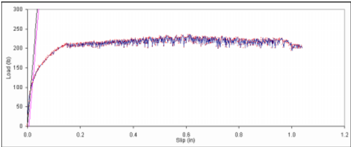
Figure B. 317: Load vs. slip plot for sample D1-6.
