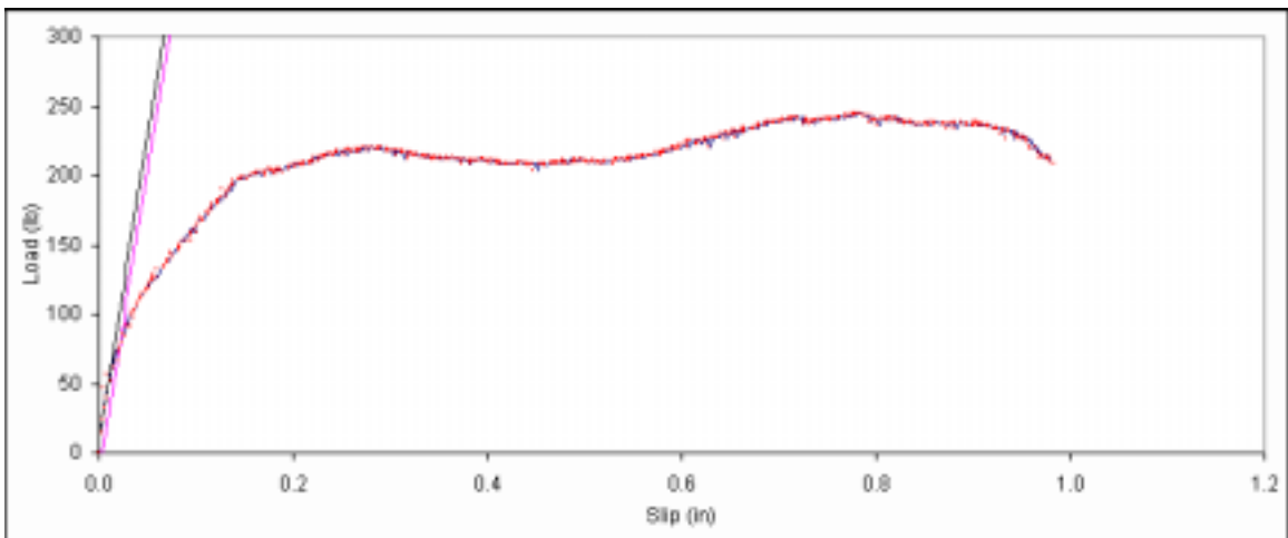
Figure B. 390: Load vs. slip plot for sample D6-5.
