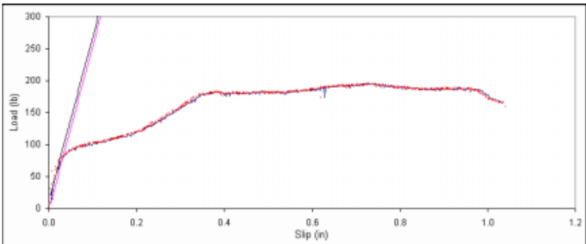
Figure B. 171: Load vs. slip plot for sample B5-9.
