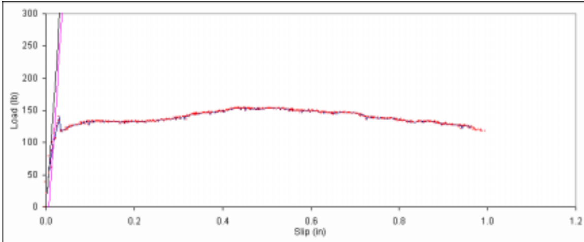
Figure B. 226: Load vs. slip plot for sample C2-4.
