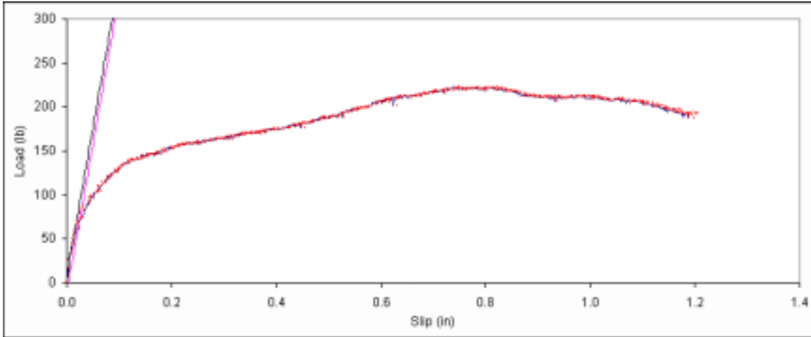
Figure B. 373: Load vs. slip plot for sample D5-3.
