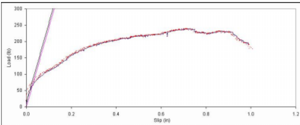
Figure B. 297: Load vs. slip plot for sample C7-1.
