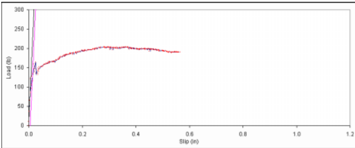
Figure B. 325: Load vs. slip plot for sample D1-15.
