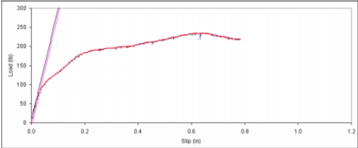
Figure B. 292: Load vs. slip plot for sample C6-11.
