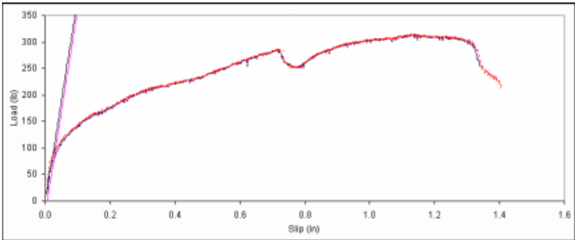
Figure B. 569: Load vs. slip plot for sample F4-7.
