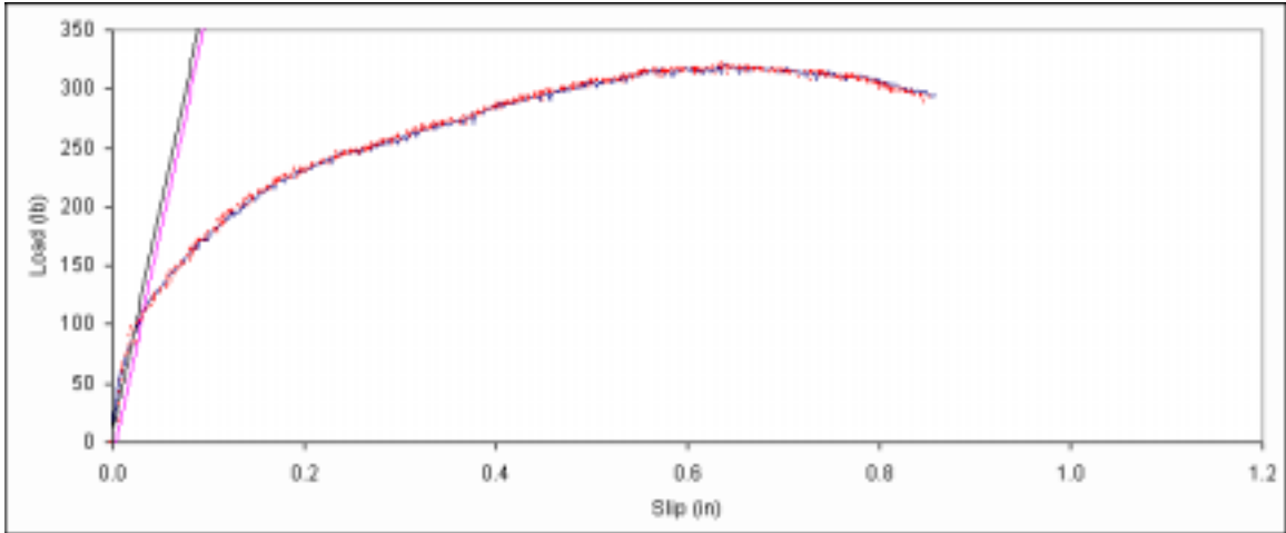
Figure B. 277: Load vs. slip plot for sample C5-11.
