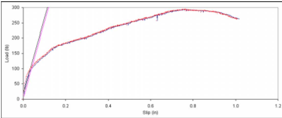
Figure B. 77: Load vs. slip plot for sample A6-3.
