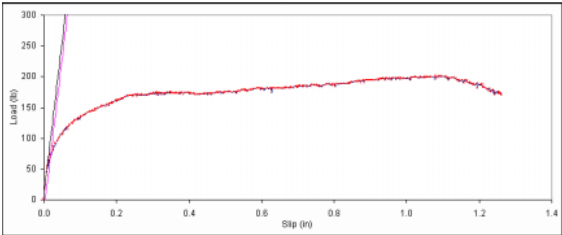
Figure B. 560: Load vs. slip plot for sample F3-13.
