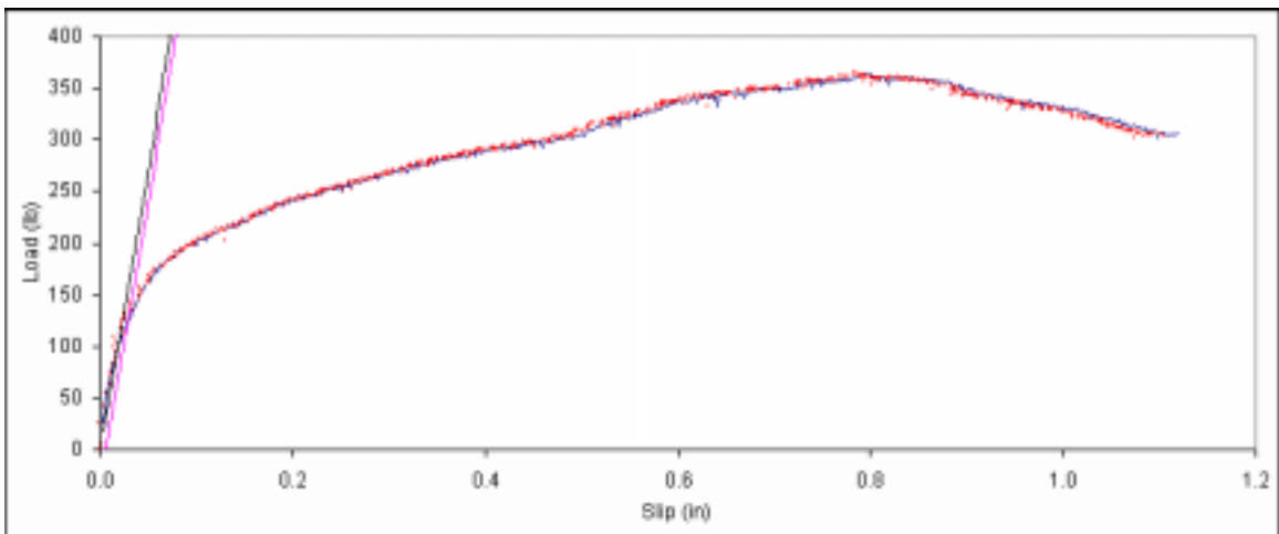
Figure B. 288: Load vs. slip plot for sample C6-7.
