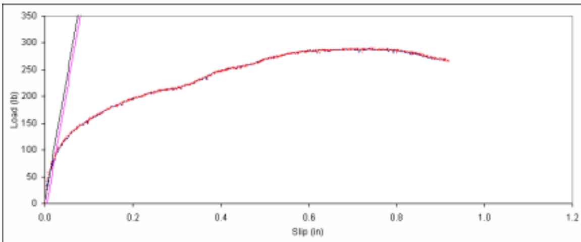
Figure B. 360: Load vs. slip plot for sample D4-5.
