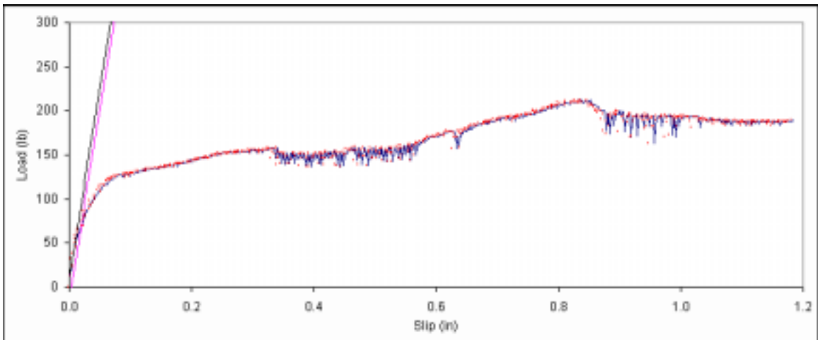
Figure B. 342: Load vs. slip plot for sample D3-2.
