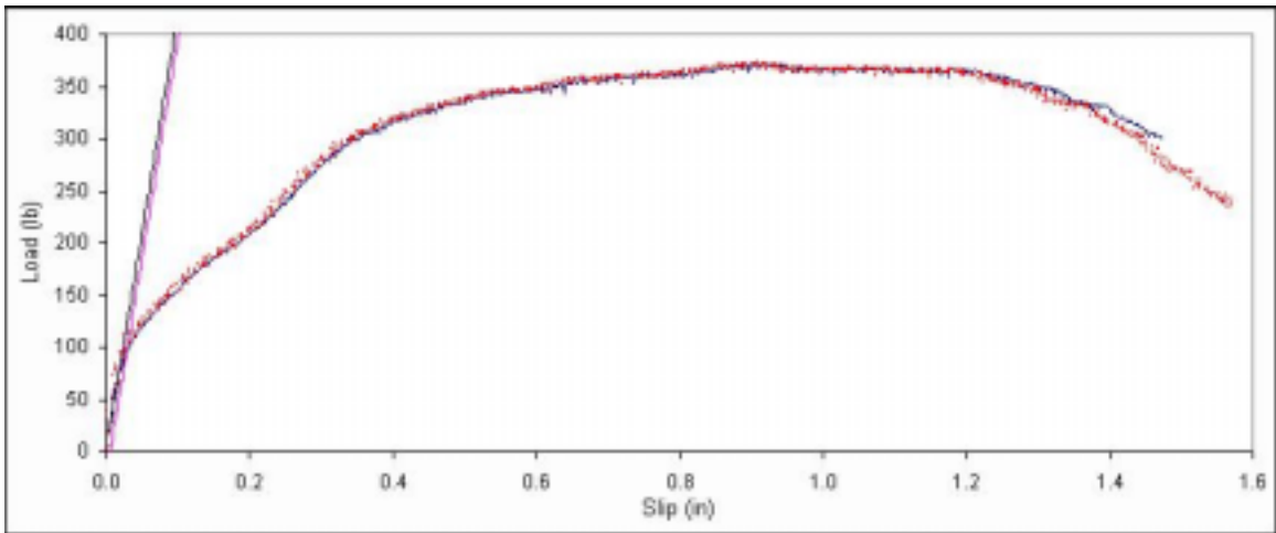
Figure B. 305: Load vs. slip plot for sample C7-9.
