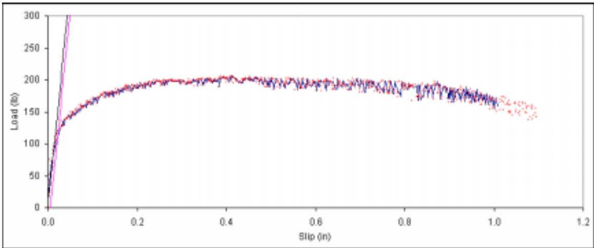
Figure B. 20: Load vs. slip plot for sample A2-6.
