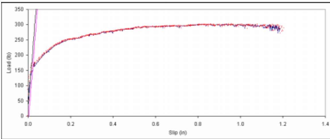
Figure B. 416: Load vs. slip plot for sample E1-1.
