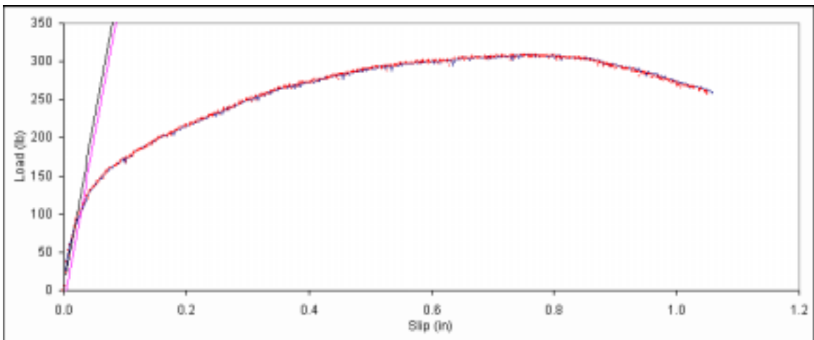
Figure B. 264: Load vs. slip plot for sample C4-13.
