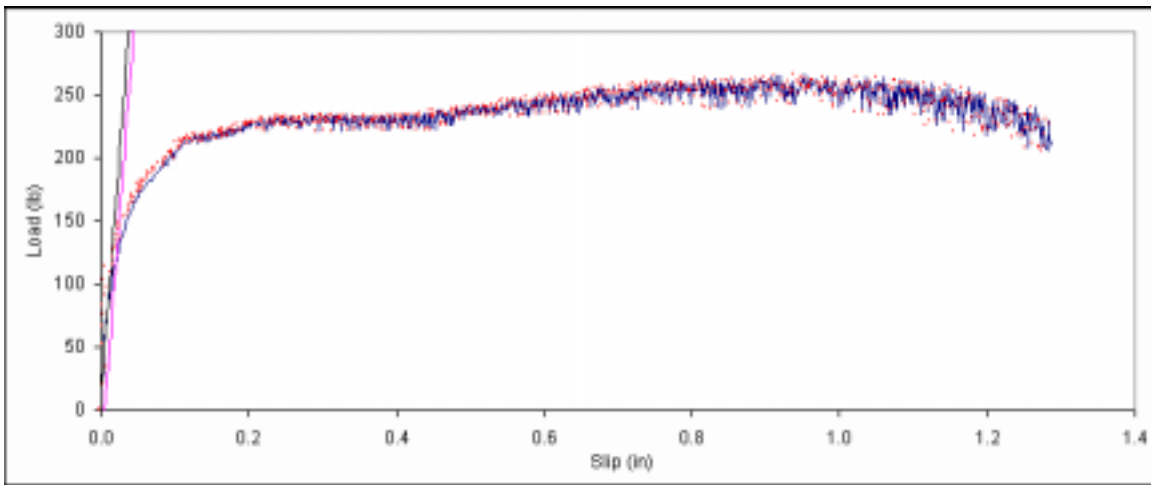
Figure B. 431: Load vs. slip plot for sample E2-1.
