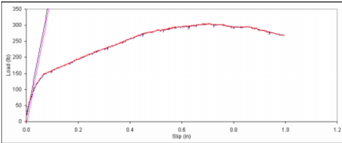
Figure B. 587: Load vs. slip plot for sample F5-10.
