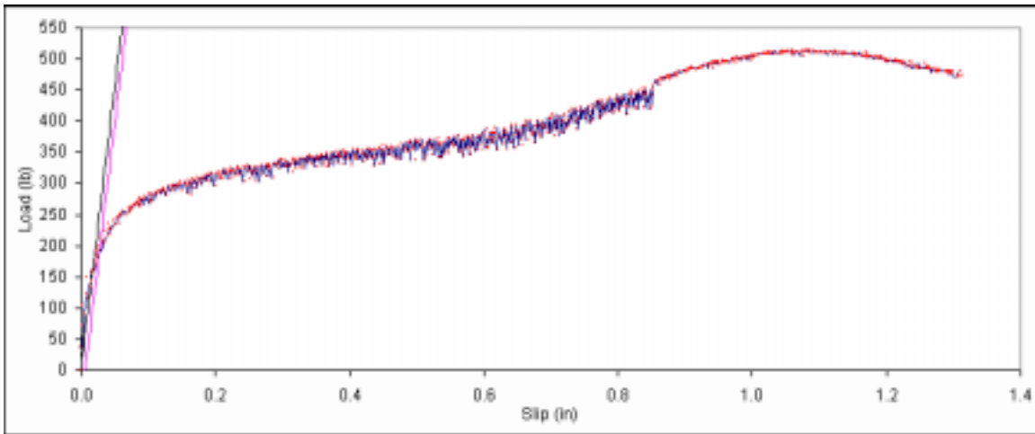
Figure B. 434: Load vs. slip plot for sample E2-4.
