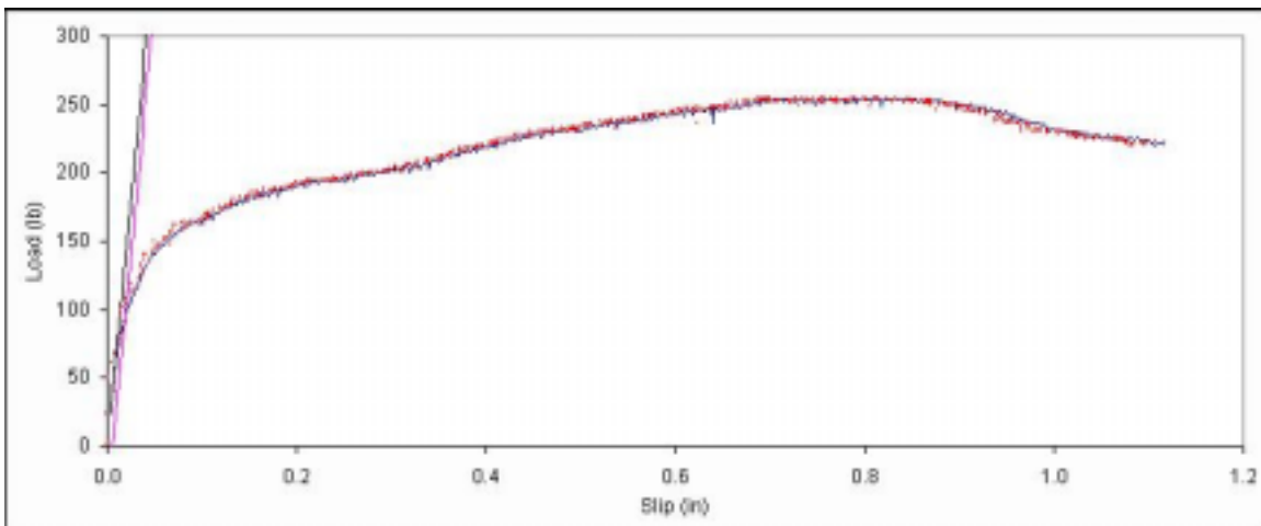
Figure B. 90: Load vs. slip plot for sample A7-2.
