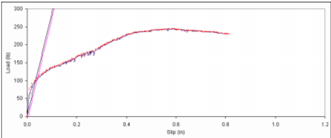
Figure B. 321: Load vs. slip plot for sample D1-11.
