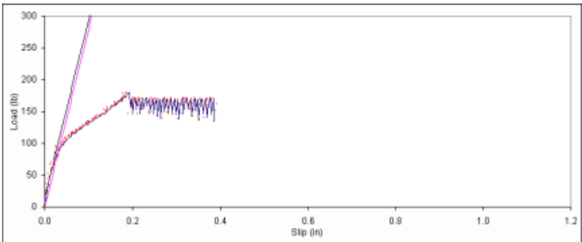
Figure B. 24: Load vs. slip plot for sample A2-10.
