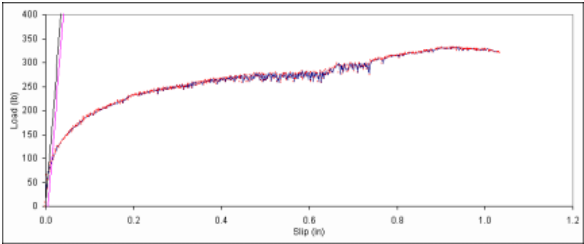
Figure B. 323: Load vs. slip plot for sample D1-13.
