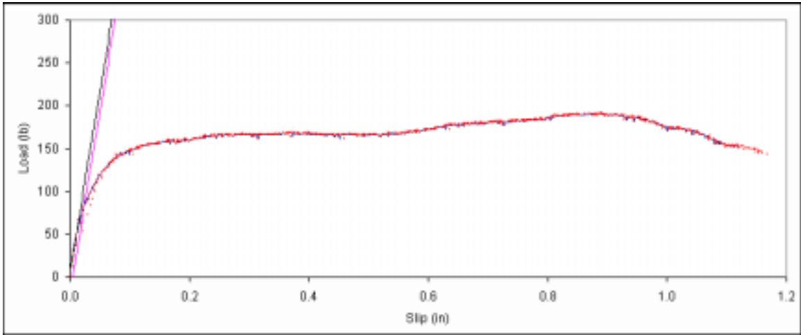
Figure B. 233: Load vs. slip plot for sample C2-11.
