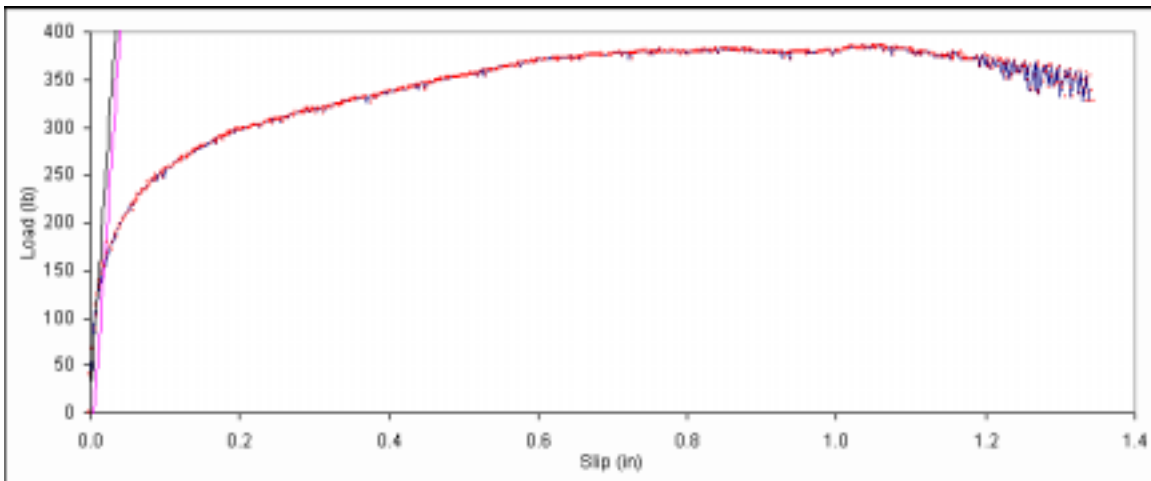
Figure B. 449: Load vs. slip plot for sample E3-4.
