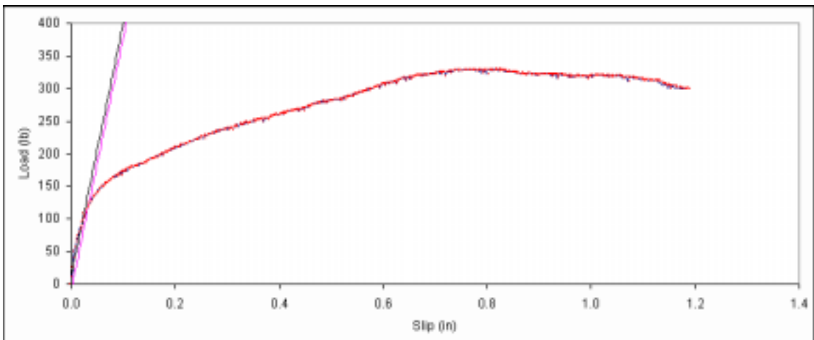
Figure B. 84: Load vs. slip plot for sample A6-11.
