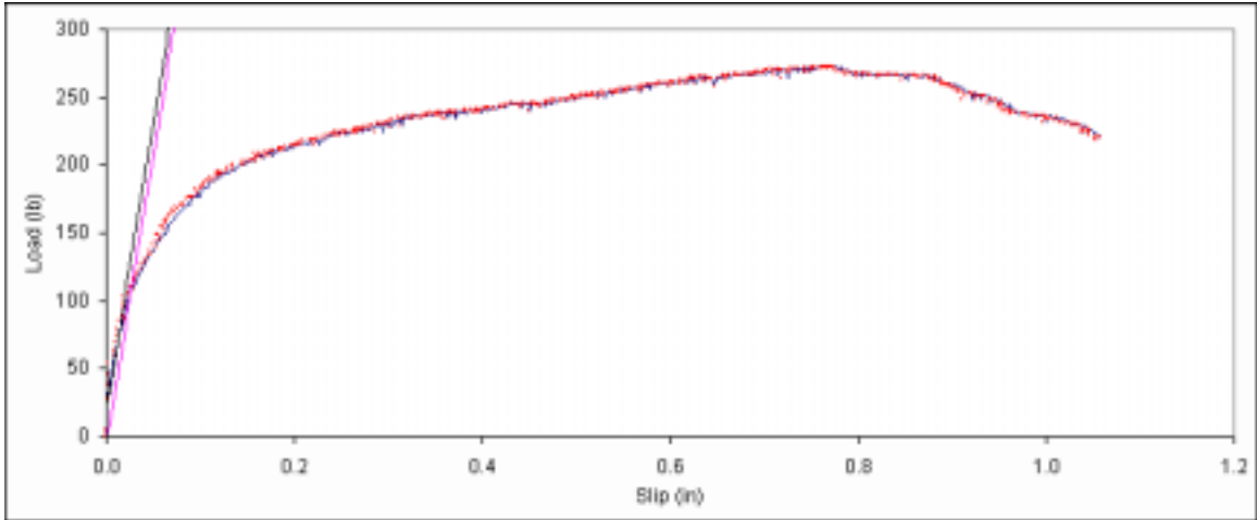
Figure B. 268: Load vs. slip plot for sample C5-2.
