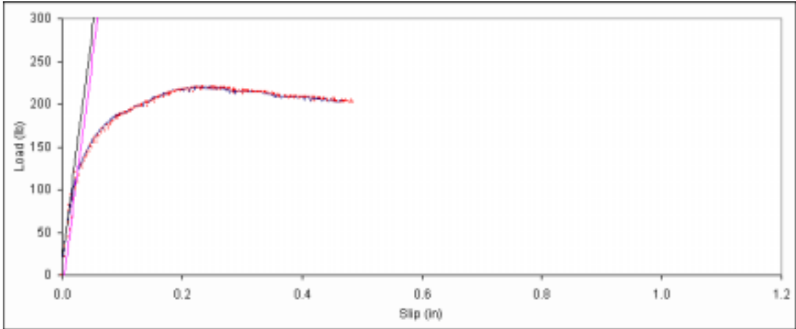
Figure B. 496: Load vs. slip plot for sample E6-7.
