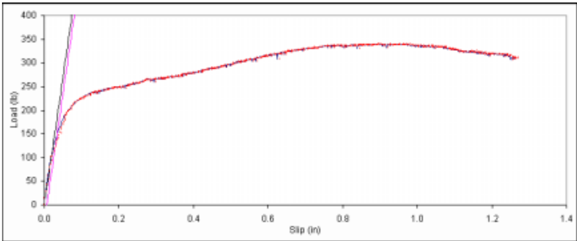
Figure B. 470: Load vs. slip plot for sample E4-10.
