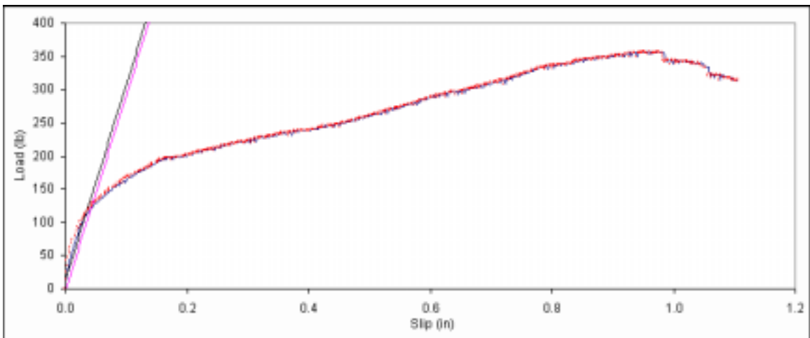
Figure B. 87: Load vs. slip plot for sample A6-14.
