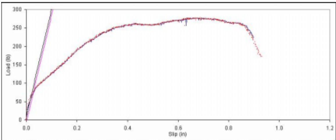
Figure B. 300: Load vs. slip plot for sample C7-4.
