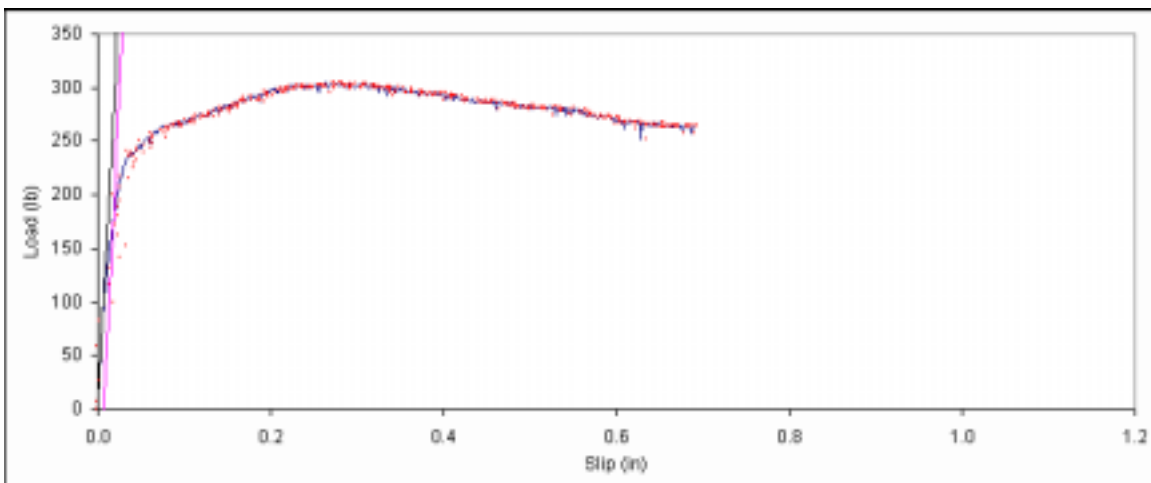
Figure B. 492: Load vs. slip plot for sample E6-2.
