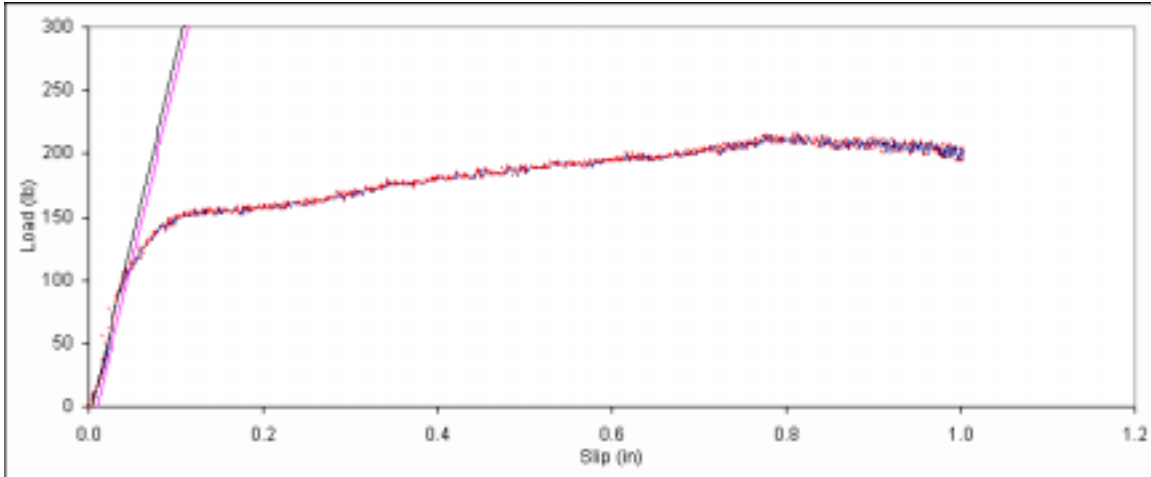
Figure B. 112: Load vs. slip plot for sample B1-10.
