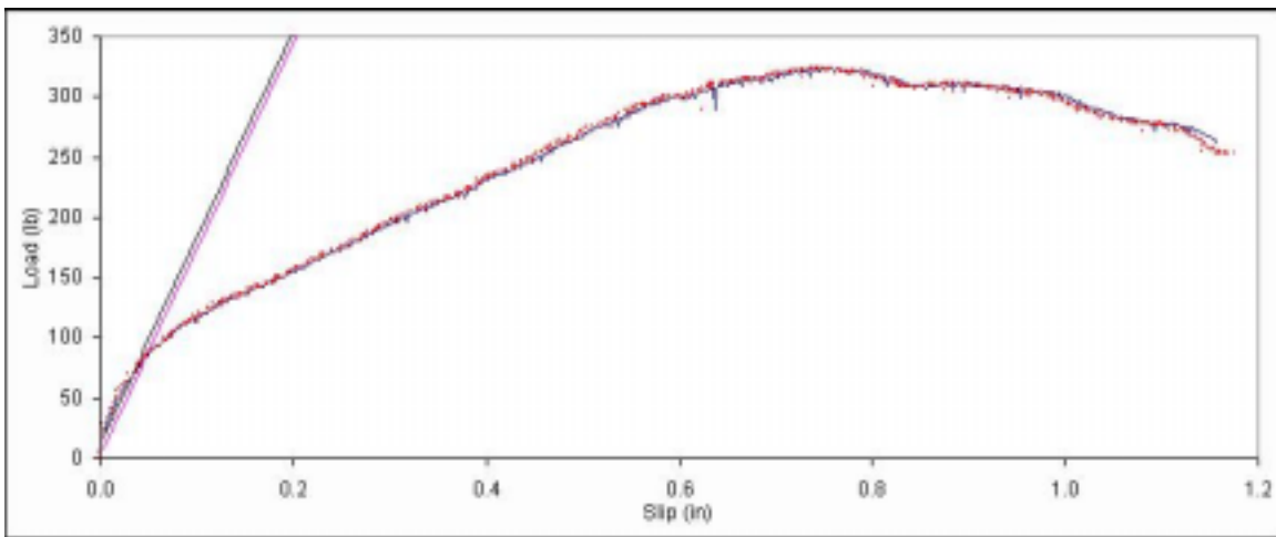
Figure B. 611: Load vs. slip plot for sample F7-4.
