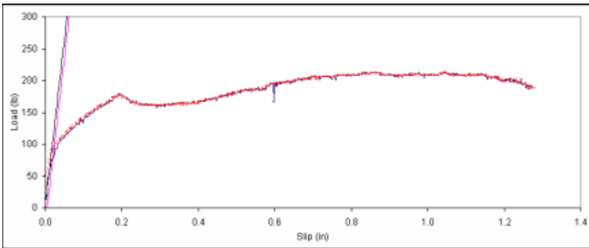
Figure B. 227: Load vs. slip plot for sample C2-5.
