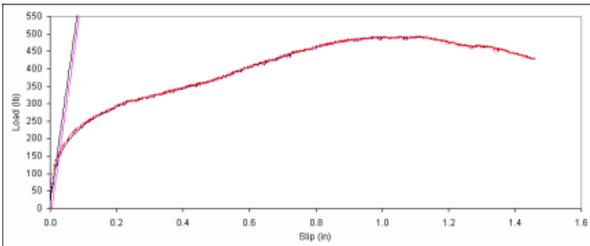
Figure B. 477: Load vs. slip plot for sample E5-2.
