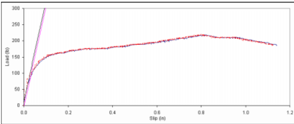
Figure B. 176: Load vs. slip plot for sample B5-14.
