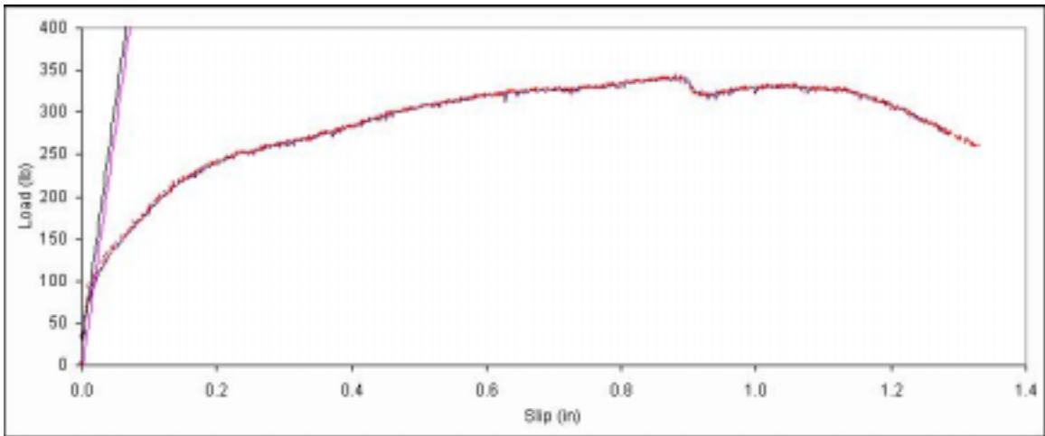
Figure B. 95: Load vs. slip plot for sample A7-7.
