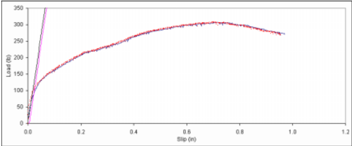
Figure B. 589: Load vs. slip plot for sample F5-12.
