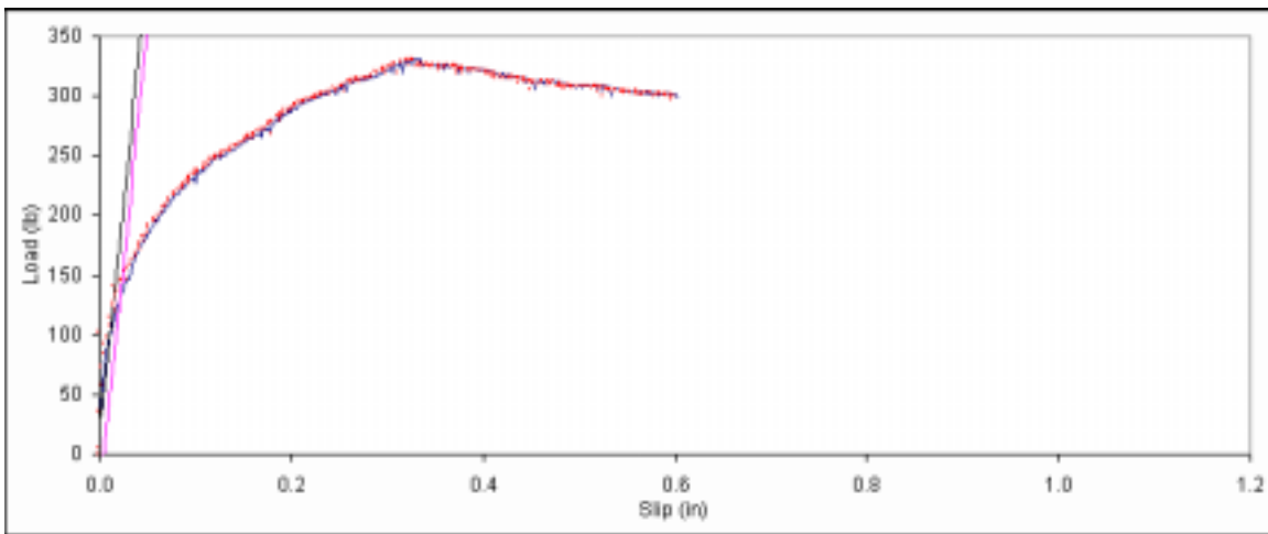
Figure B. 458: Load vs. slip plot for sample E3-13.
