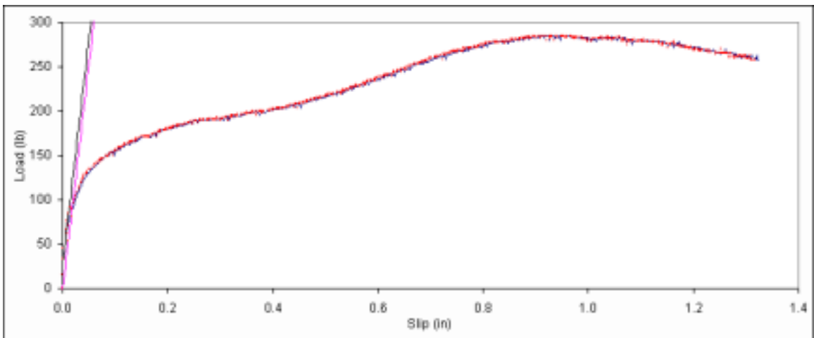
Figure B. 39: Load vs. slip plot for sample A3-10.
