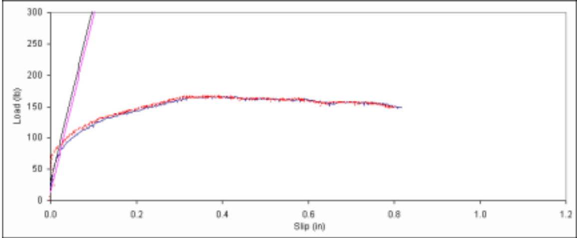
Figure B. 133: Load vs. slip plot for sample B3-1.
