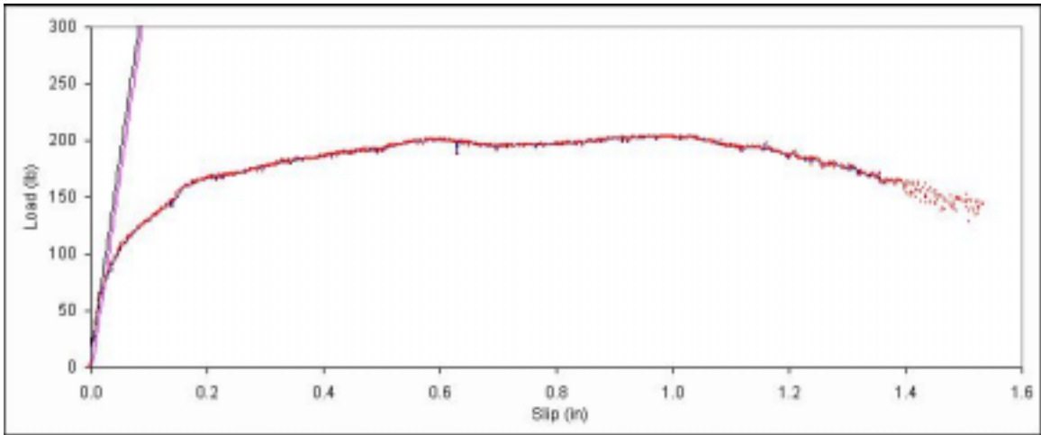
Figure B. 608: Load vs. slip plot for sample F7-1.
