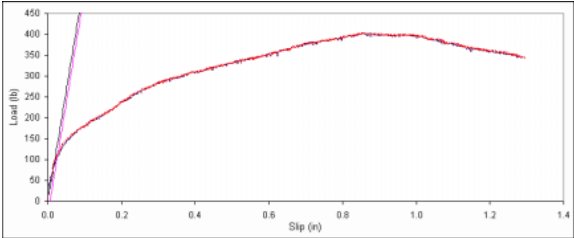
Figure B. 394: Load vs. slip plot for sample D6-9.
