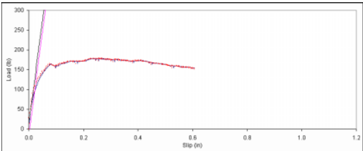
Figure B. 132: Load vs. slip plot for sample B2-15.
