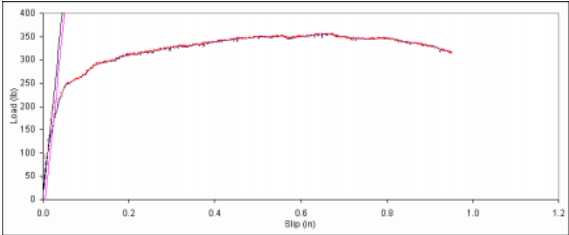
Figure B. 274: Load vs. slip plot for sample C5-8.
