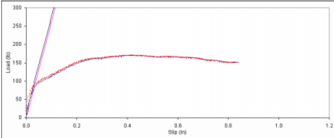
Figure B. 175: Load vs. slip plot for sample B5-13.
