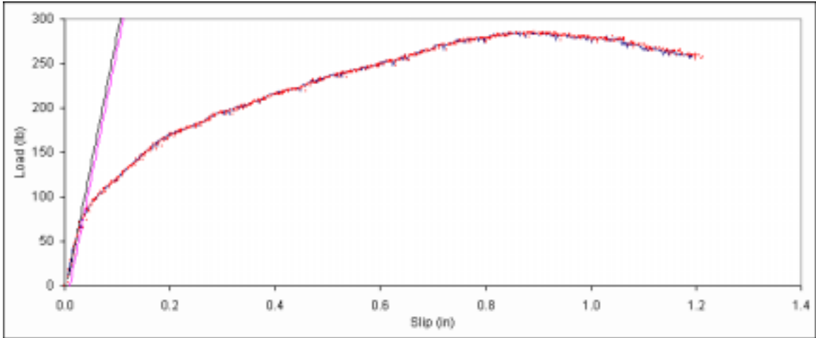
Figure B. 559: Load vs. slip plot for sample F3-12.
