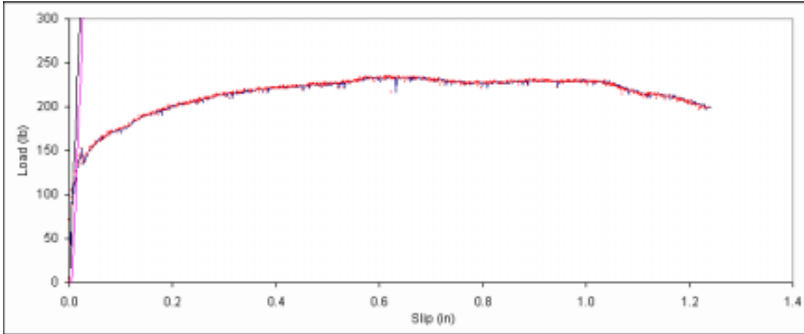
Figure B. 43: Load vs. slip plot for sample A3-14.
