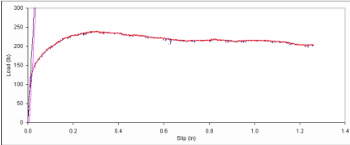
Figure B. 490: Load vs. slip plot for sample E5-15.
