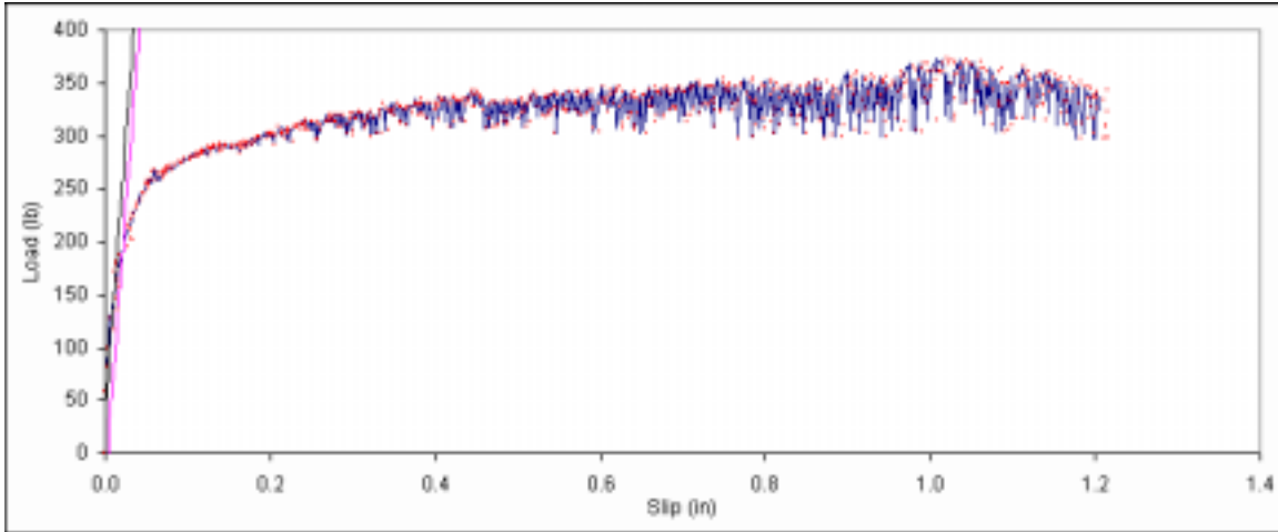
Figure B. 418: Load vs. slip plot for sample E1-3.
