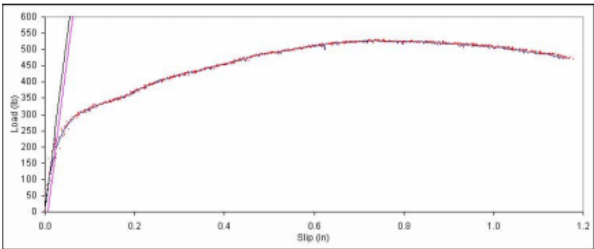
Figure B. 512: Load vs. slip plot for sample E7-8.
