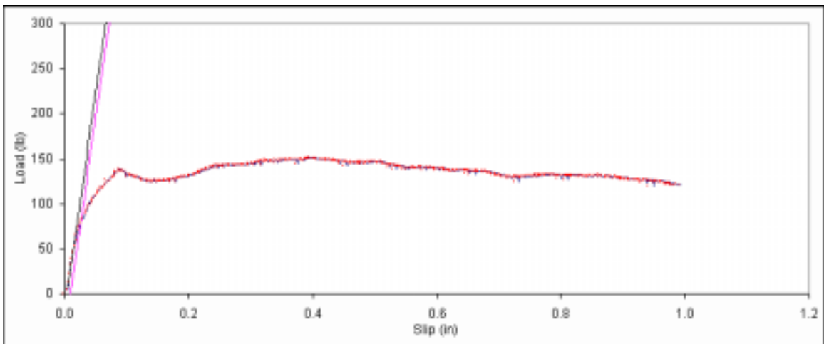
Figure B. 249: Load vs. slip plot for sample C3-13.
