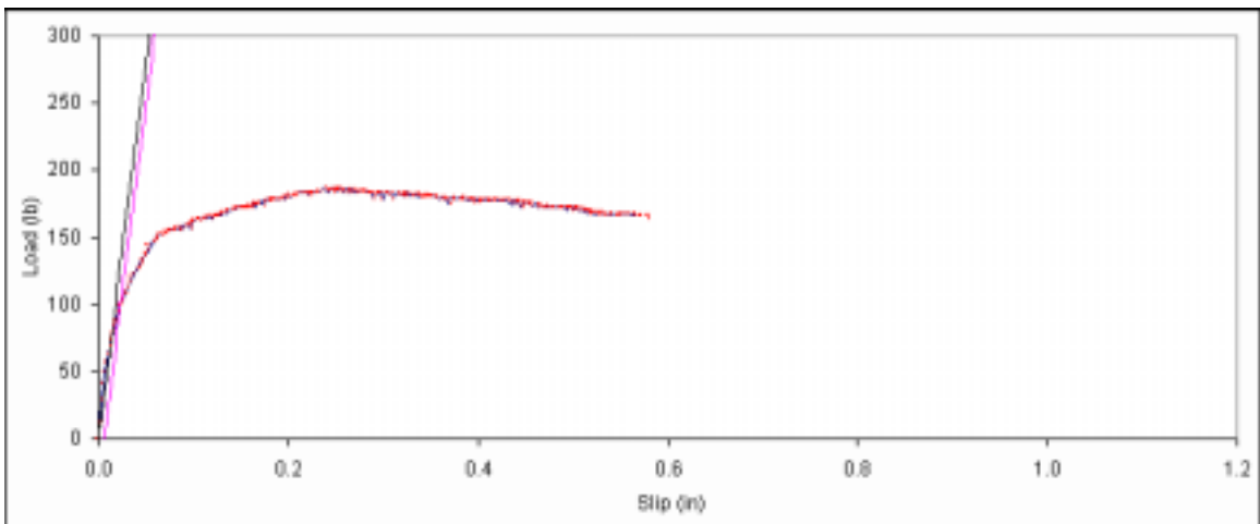
Figure B. 27: Load vs. slip plot for sample A2-13.
