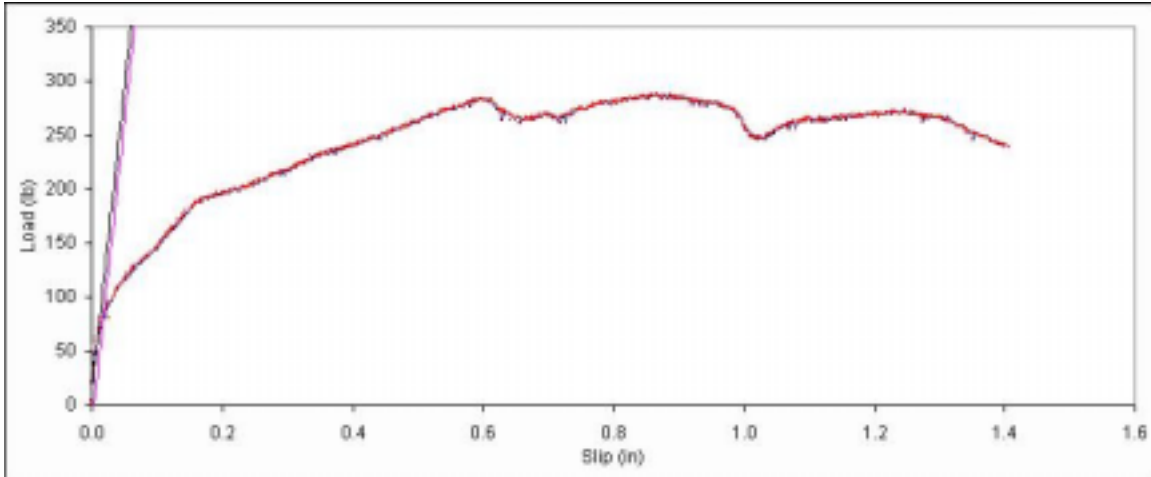
Figure B. 100: Load vs. slip plot for sample A7-12.
