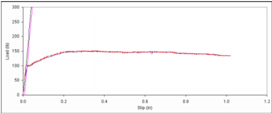
Figure B. 239: Load vs. slip plot for sample C3-2.
