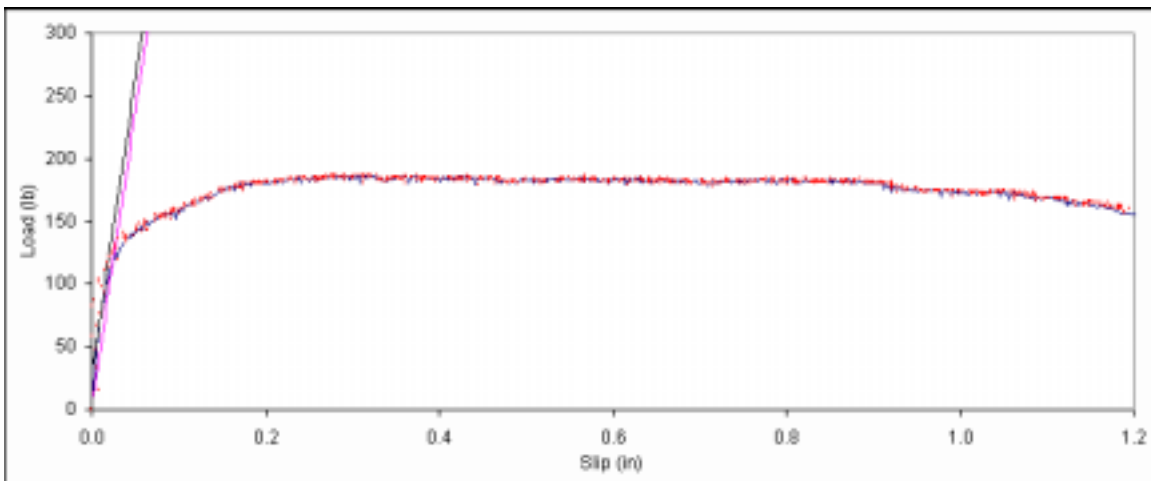
Figure B. 357: Load vs. slip plot for sample D4-2.
