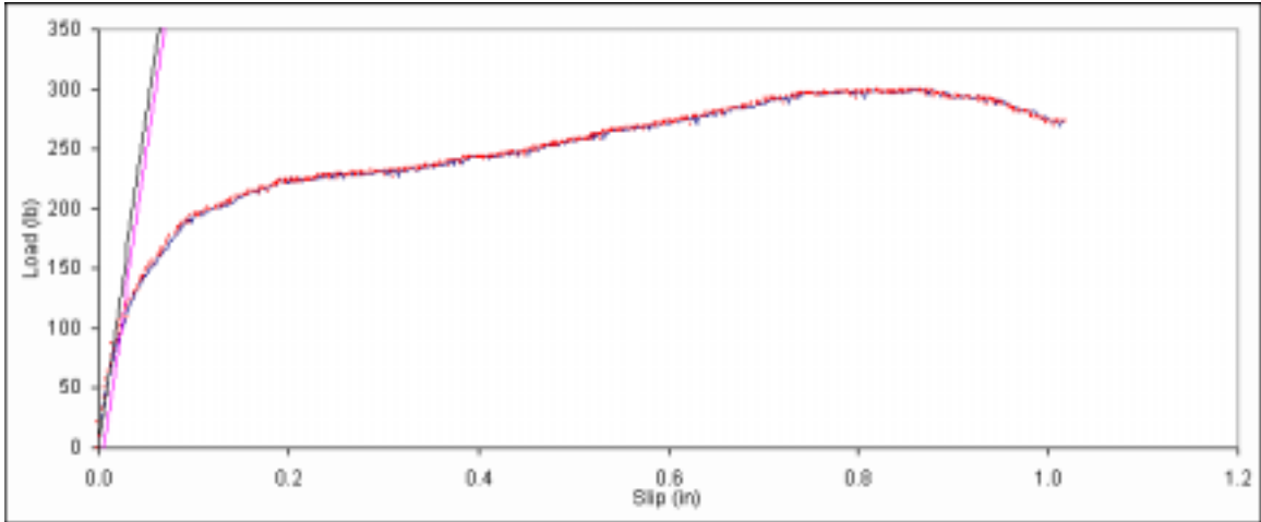
Figure B. 376: Load vs. slip plot for sample D5-6.
