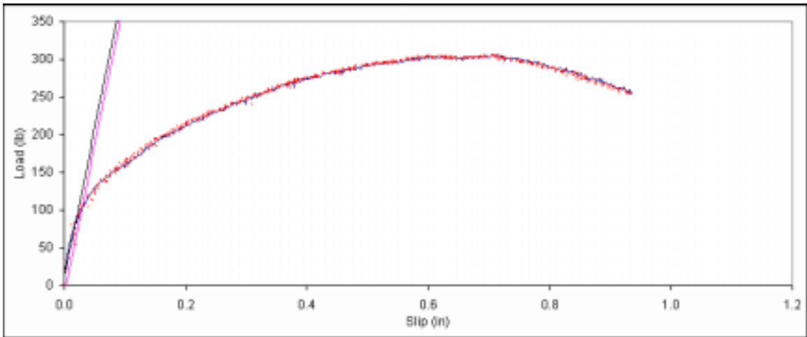
Figure B. 266: Load vs. slip plot for sample C4-15.
