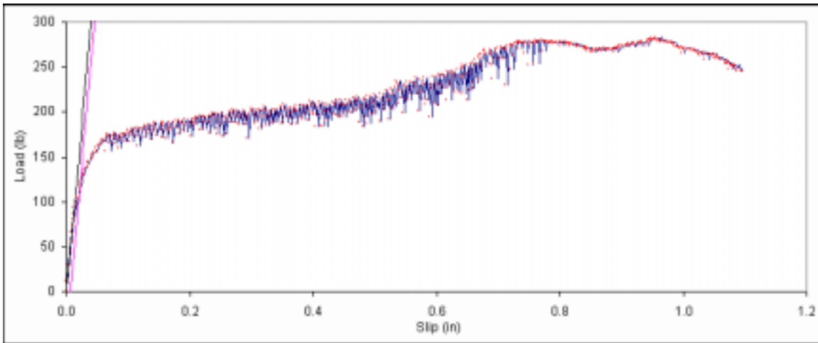
Figure B. 236: Load vs. slip plot for sample C2-14.
