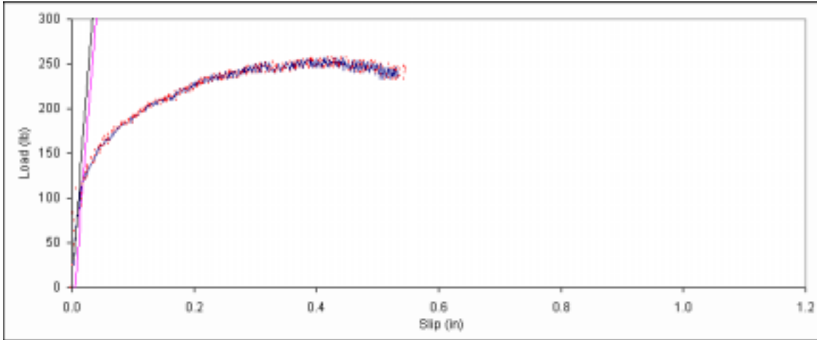
Figure B. 1: Load vs. slip plot for sample A1-1.
