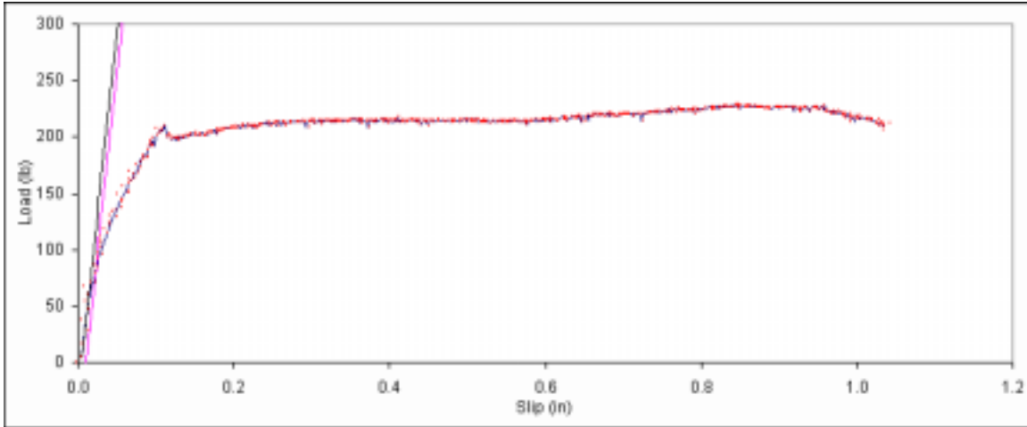
Figure B. 541: Load vs. slip plot for sample F2-8.
