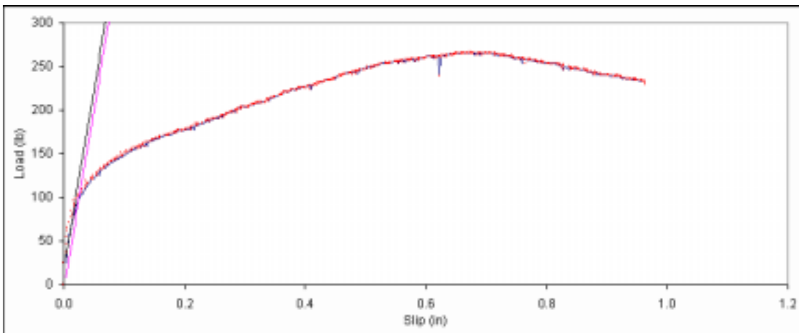
Figure B. 144: Load vs. slip plot for sample B3-12.
