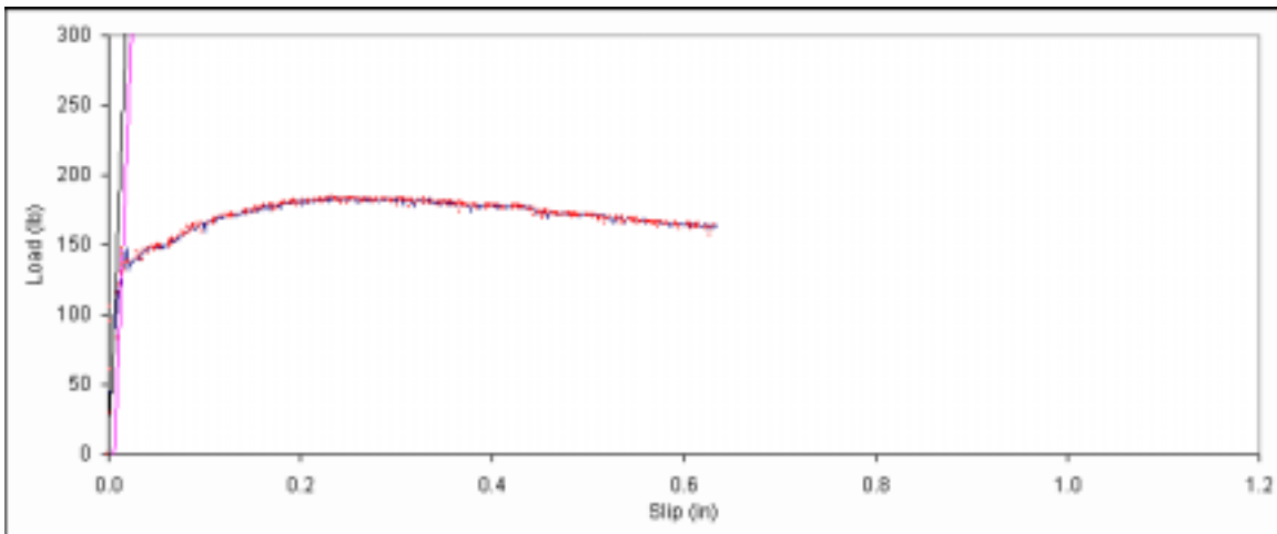
Figure B. 17: Load vs. slip plot for sample A2-3.
