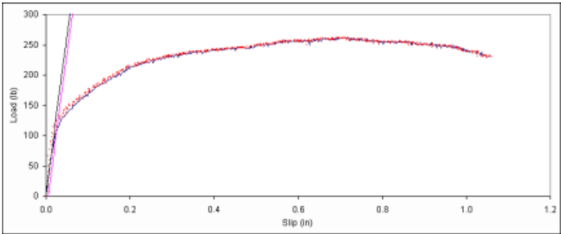
Figure B. 47: Load vs. slip plot for sample A4-3.
