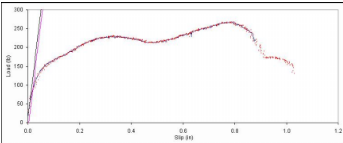
Figure B. 414: Load vs. slip plot for sample D7-14.
