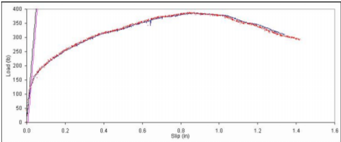
Figure B. 510: Load vs. slip plot for sample E7-6.
