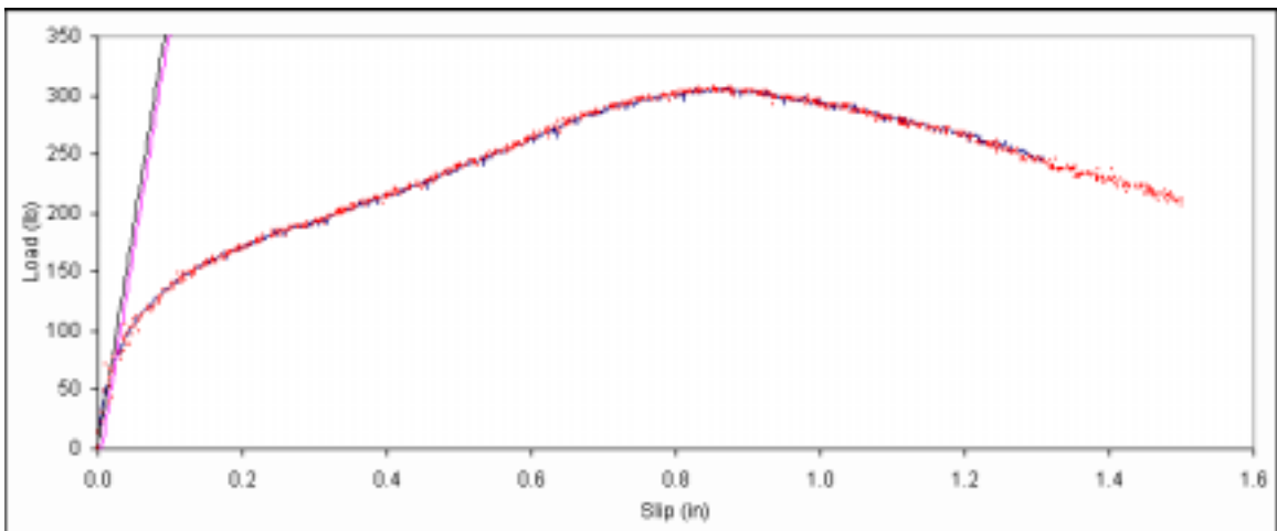
Figure B. 567: Load vs. slip plot for sample F4-5.
