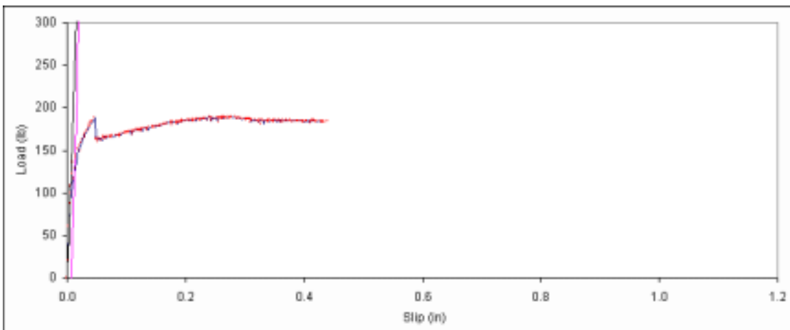
Figure B. 312: Load vs. slip plot for sample D1-1.
