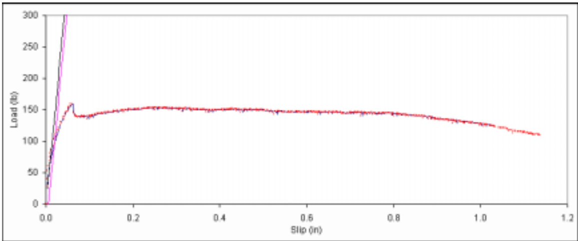
Figure B. 50: Load vs. slip plot for sample A4-6.
