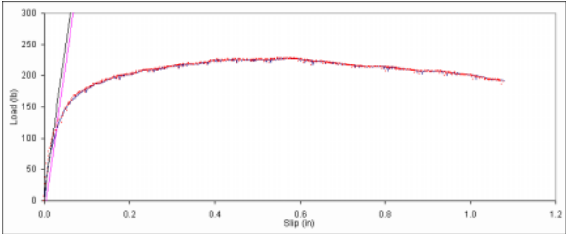
Figure B. 451: Load vs. slip plot for sample E3-6.
