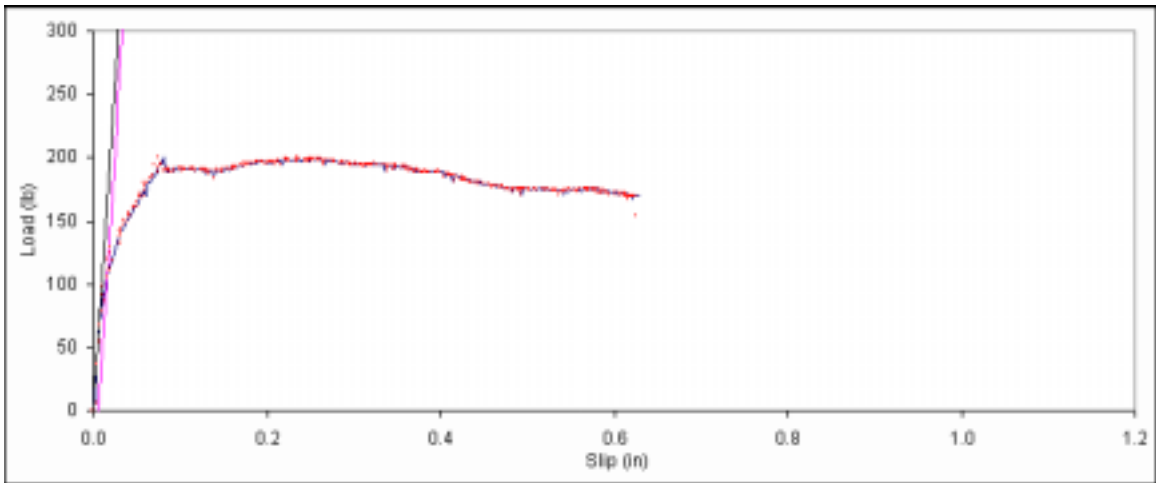
Figure B. 131: Load vs. slip plot for sample B2-14.
