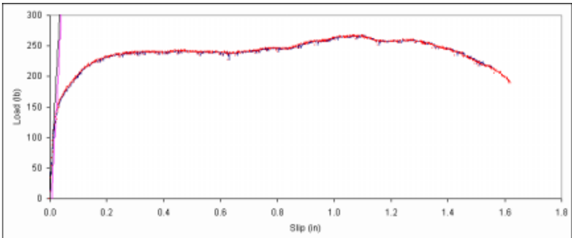
Figure B. 486: Load vs. slip plot for sample E5-11.
