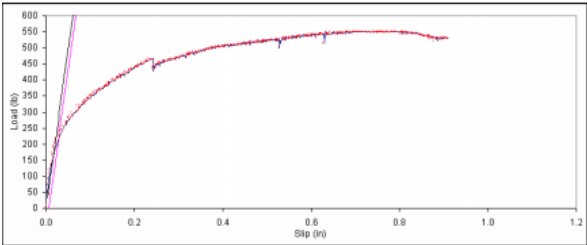
Figure B. 443: Load vs. slip plot for sample E2-13.
