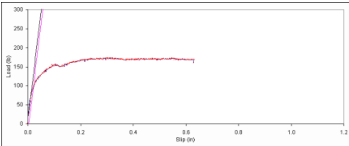
Figure B. 533: Load vs. slip plot for sample F1-15.
