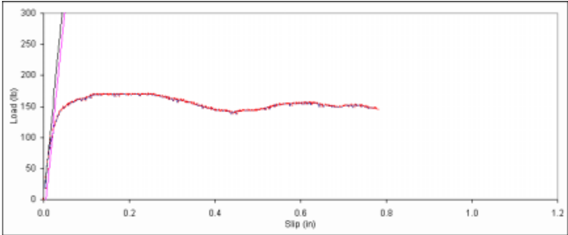
Figure B. 127: Load vs. slip plot for sample B2-10.
