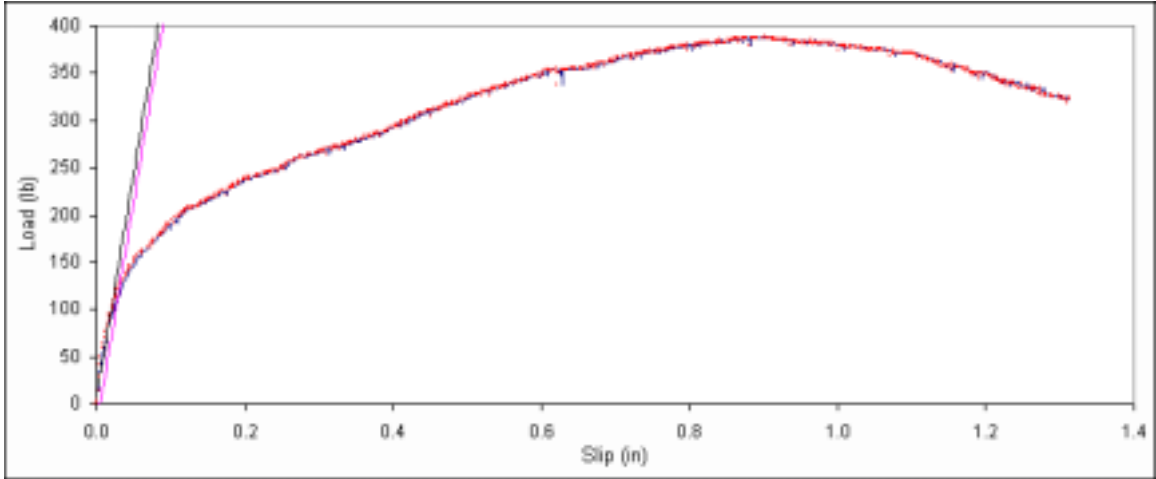
Figure B. 484: Load vs. slip plot for sample E5-9.
