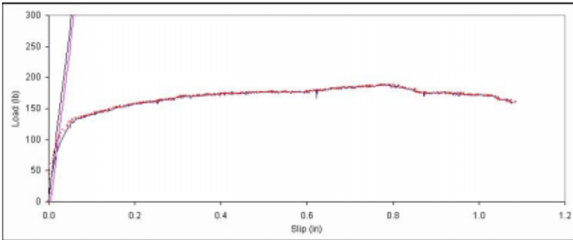
Figure B. 194: Load vs. slip plot for sample B7-2.
