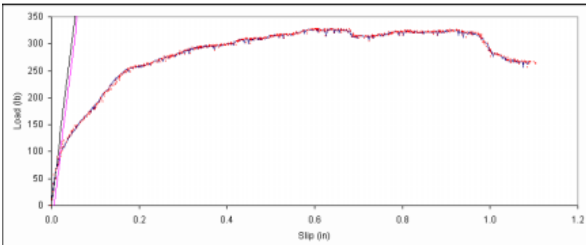
Figure B. 588: Load vs. slip plot for sample F5-11.
