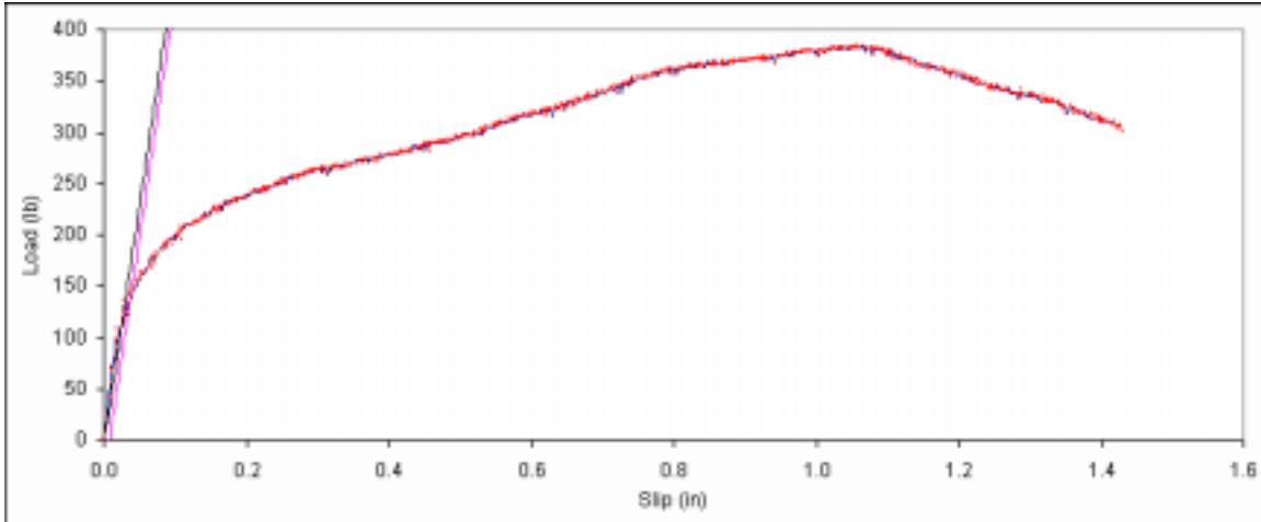
Figure B. 463: Load vs. slip plot for sample E4-3.
