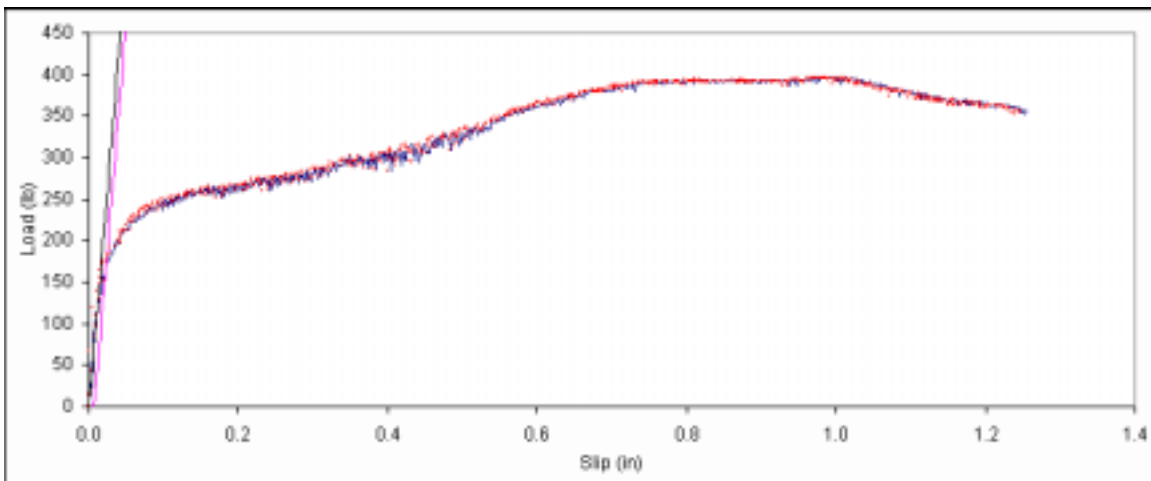
Figure B. 465: Load vs. slip plot for sample E4-5.
