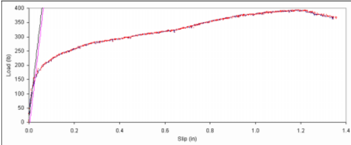
Figure B. 433: Load vs. slip plot for sample E2-3.
