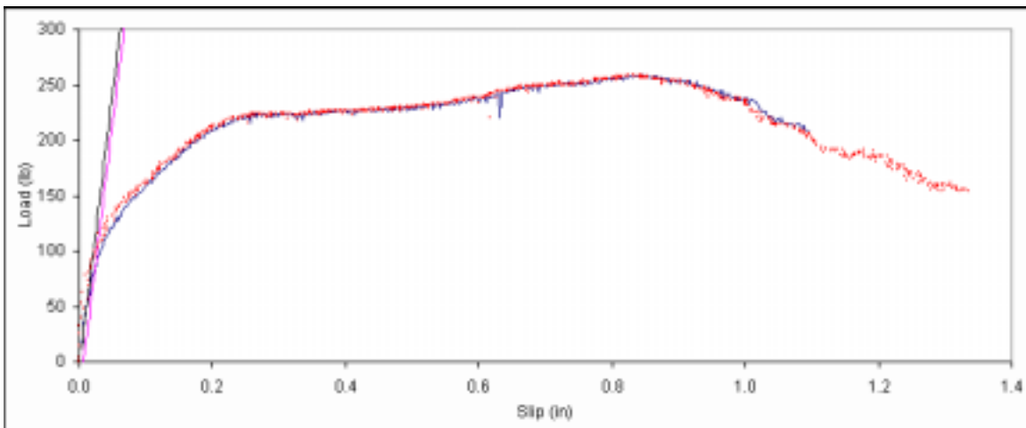
Figure B. 582: Load vs. slip plot for sample F5-5.
