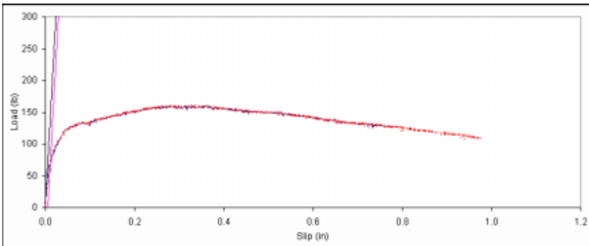
Figure B. 552: Load vs. slip plot for sample F3-5.
