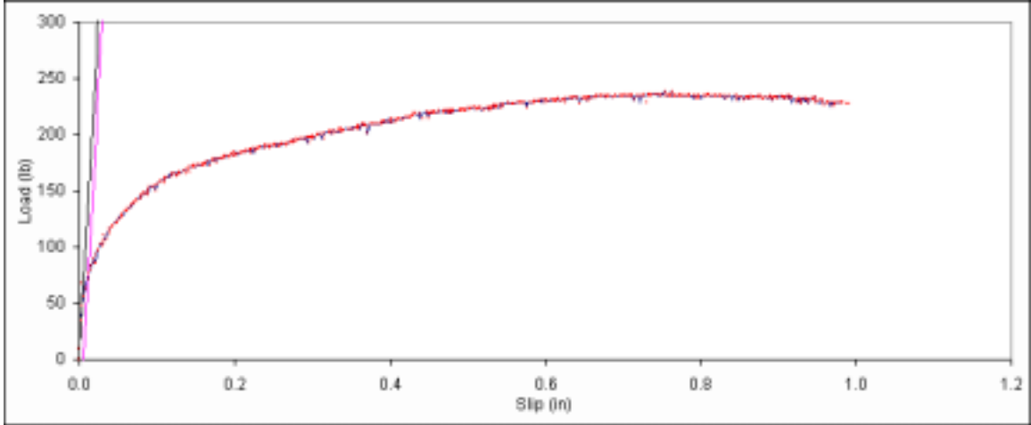
Figure B. 529: Load vs. slip plot for sample F1-10.
