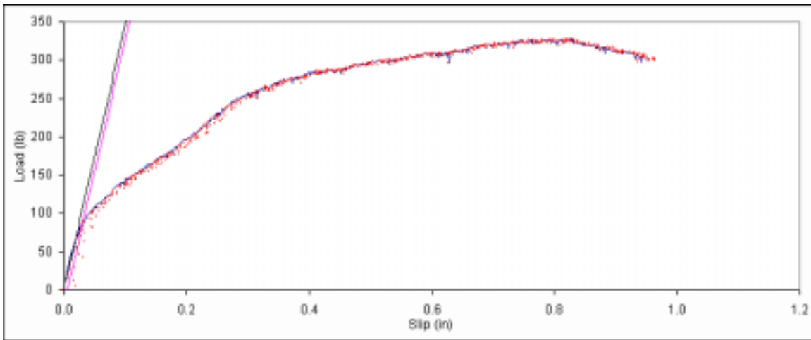
Figure B. 596: Load vs. slip plot for sample F6-4.
