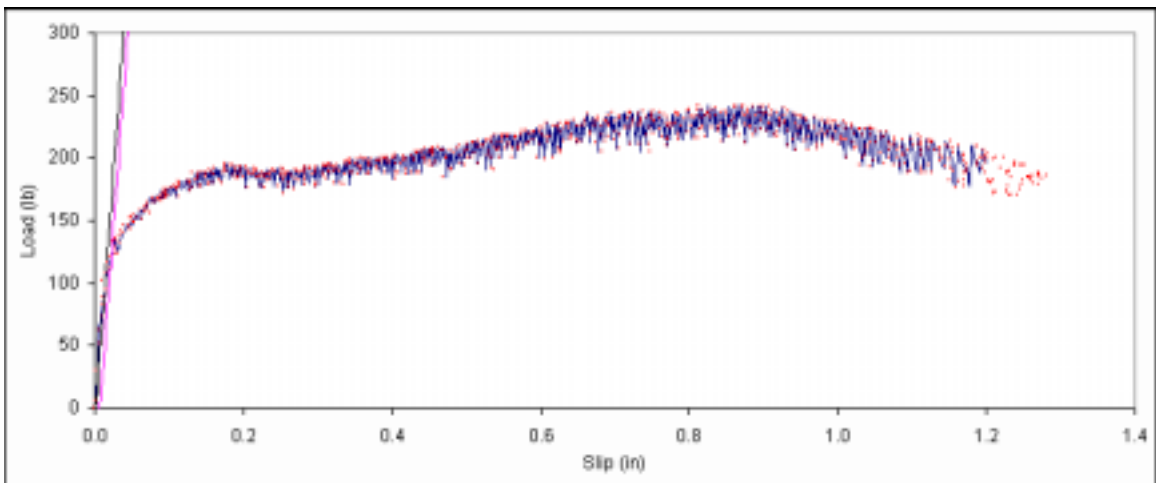
Figure B. 351: Load vs. slip plot for sample D3-11.
