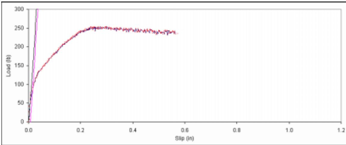
Figure B. 536: Load vs. slip plot for sample F2-3.
