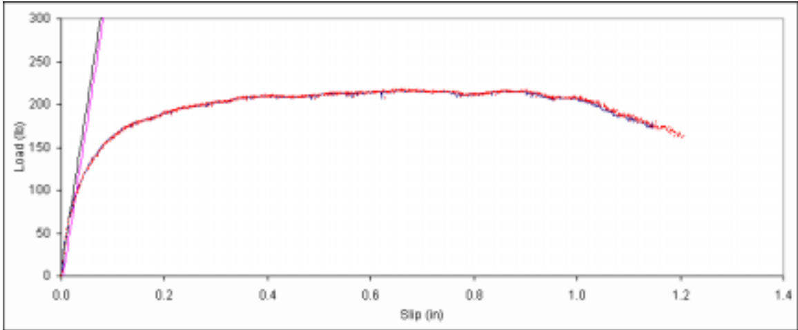
Figure B. 79: Load vs. slip plot for sample A6-5.
