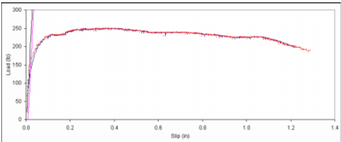
Figure B. 480: Load vs. slip plot for sample E5-5.
