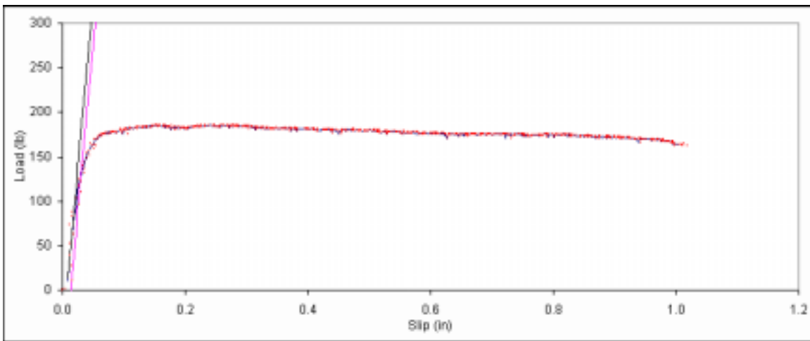
Figure B. 440: Load vs. slip plot for sample E2-10.
