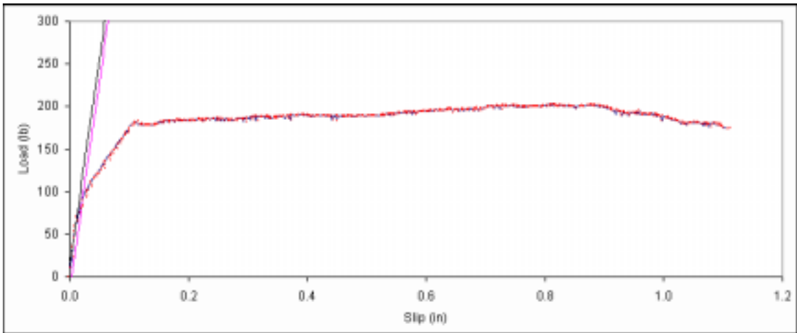
Figure B. 128: Load vs. slip plot for sample B2-11.
