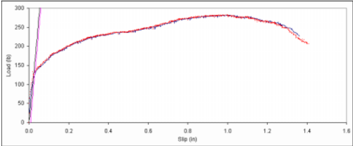
Figure B. 40: Load vs. slip plot for sample A3-11.
