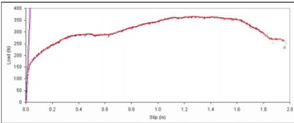
Figure B. 515: Load vs. slip plot for sample E7-11.
