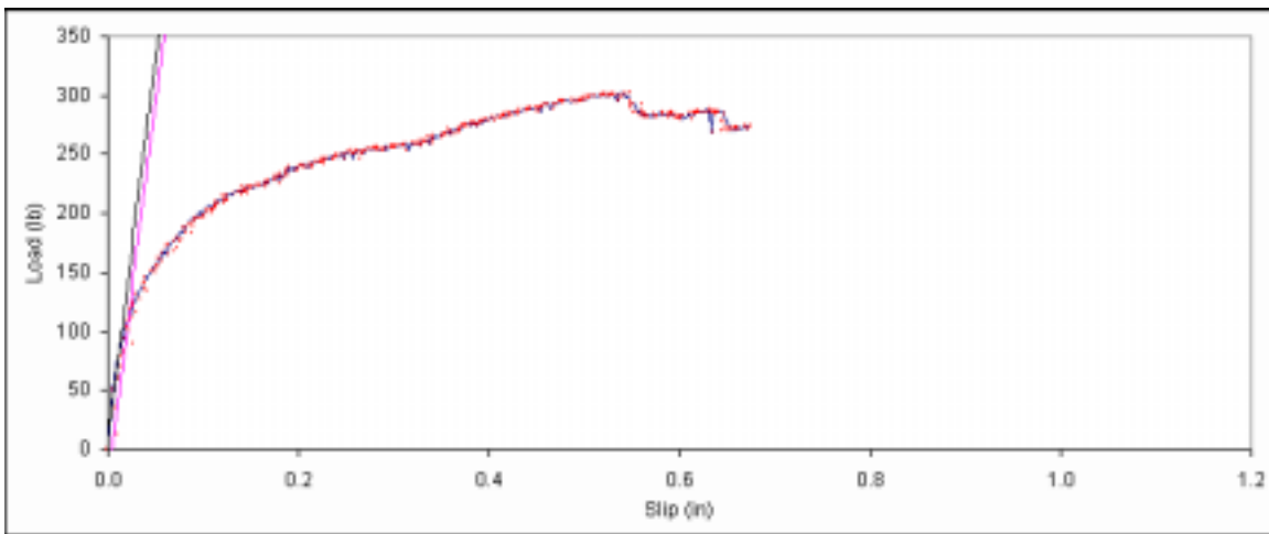
Figure B. 104: Load vs. slip plot for sample B1-2.
