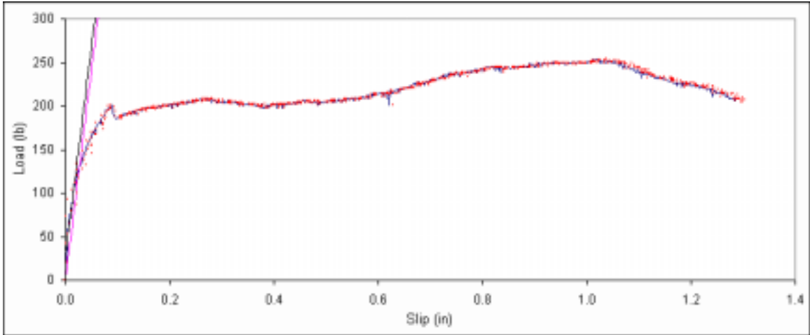
Figure B. 364: Load vs. slip plot for sample D4-9.
