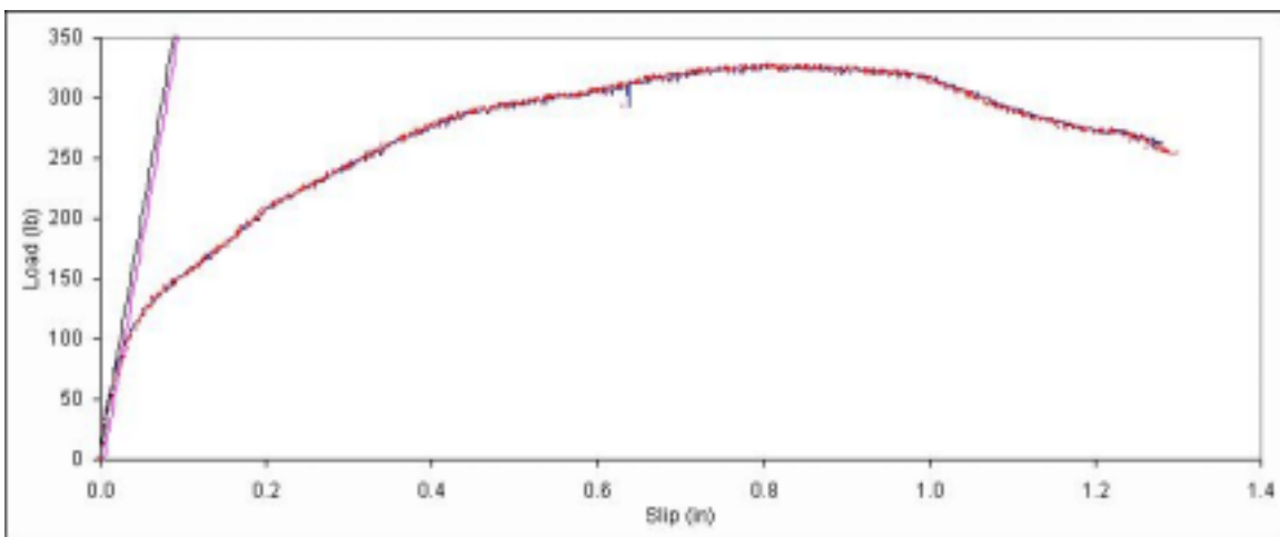
Figure B. 309: Load vs. slip plot for sample C7-13.
