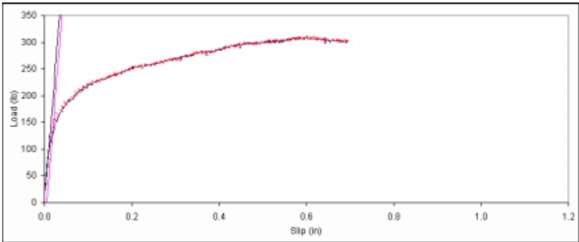
Figure B. 5: Load vs. slip plot for sample A1-5.
