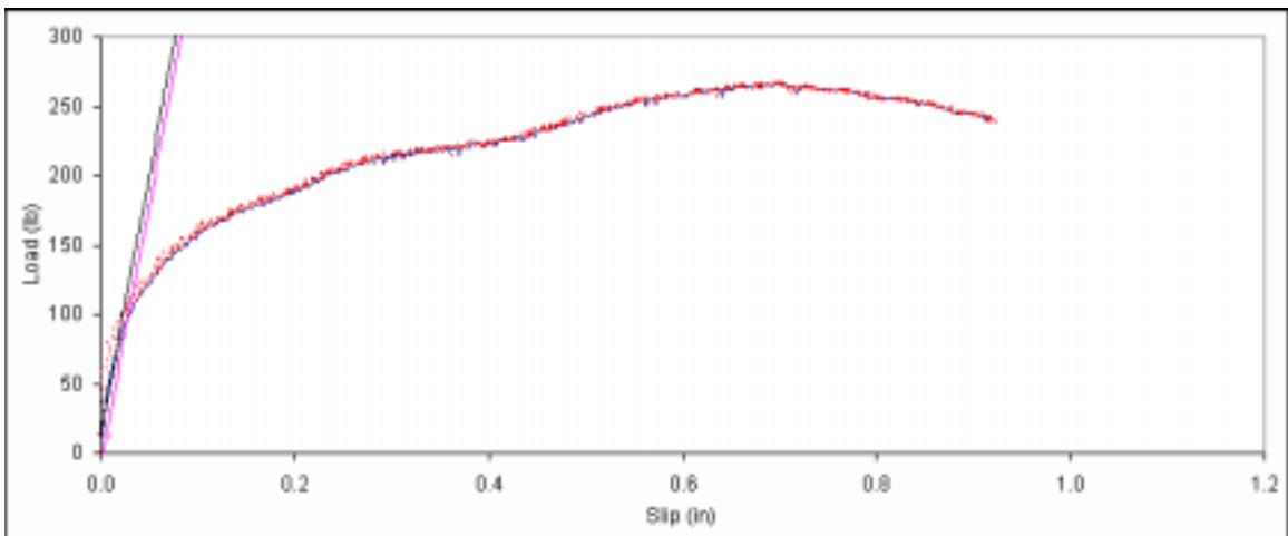
Figure B. 66: Load vs. slip plot for sample A5-7.
