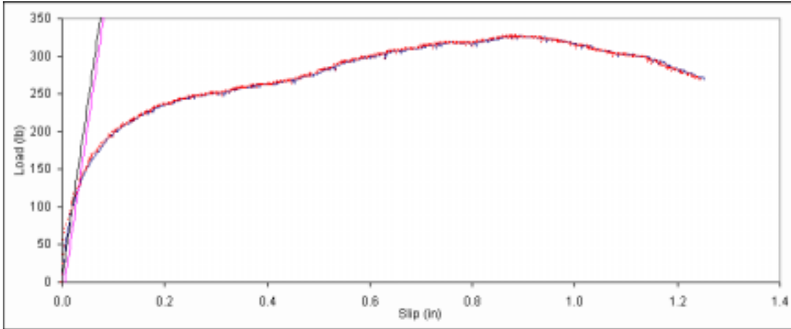
Figure B. 481: Load vs. slip plot for sample E5-6.
