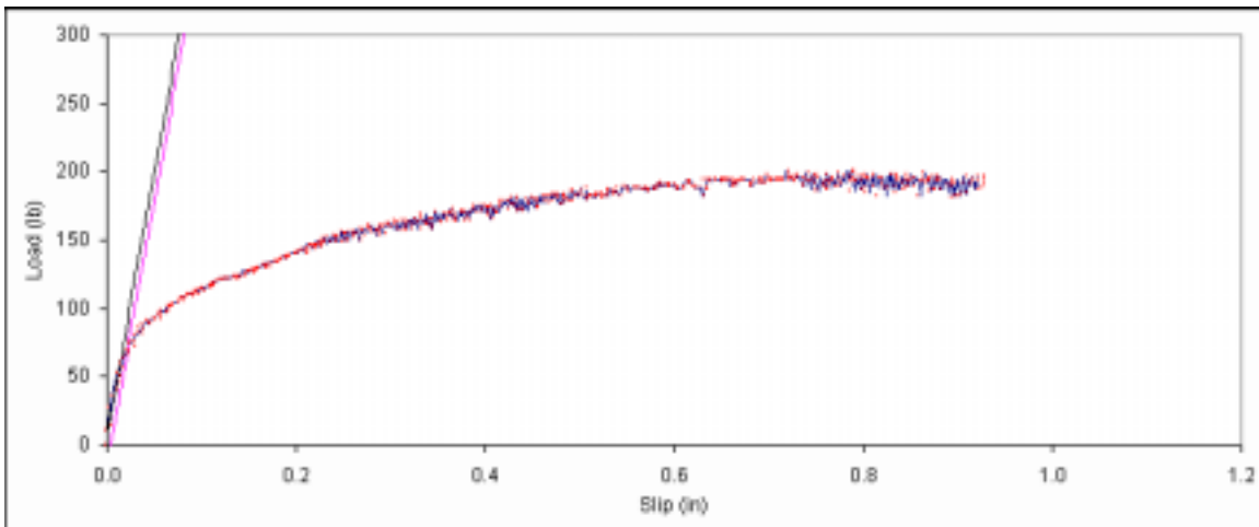
Figure B. 209: Load vs. slip plot for sample C1-2.
