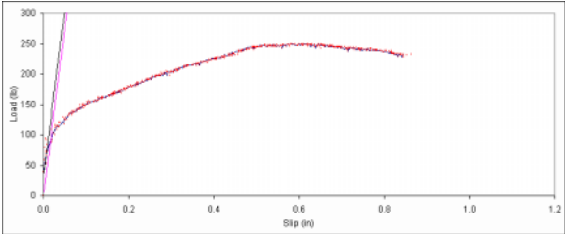
Figure B. 256: Load vs. slip plot for sample C4-5.
