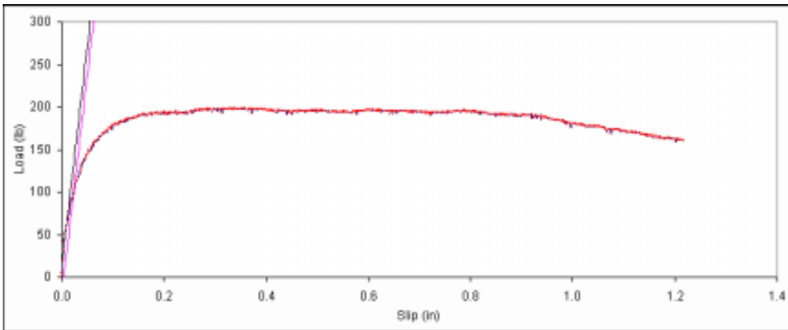
Figure B. 482: Load vs. slip plot for sample E5-7.
