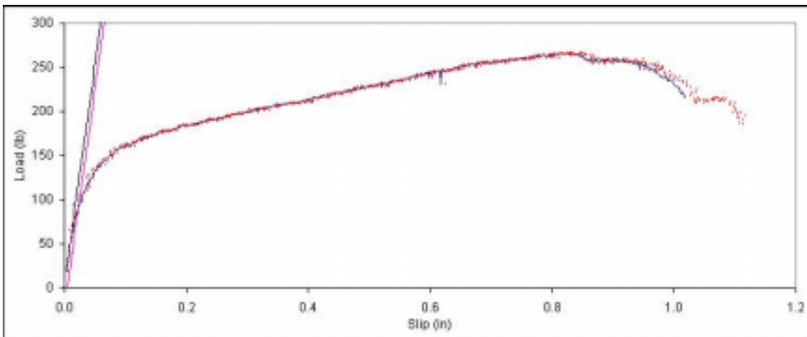
Figure B. 204: Load vs. slip plot for sample B7-12.
