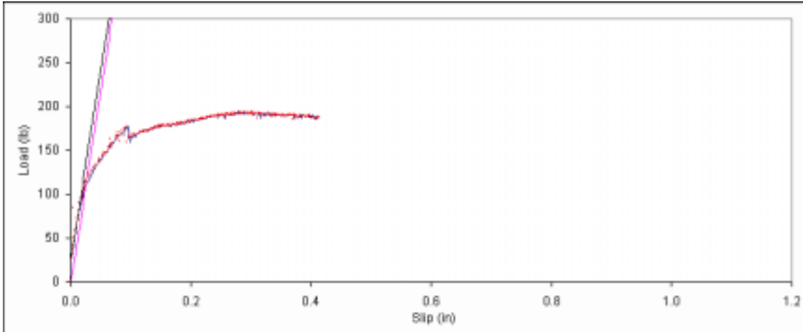
Figure B. 103: Load vs. slip plot for sample B1-1.
