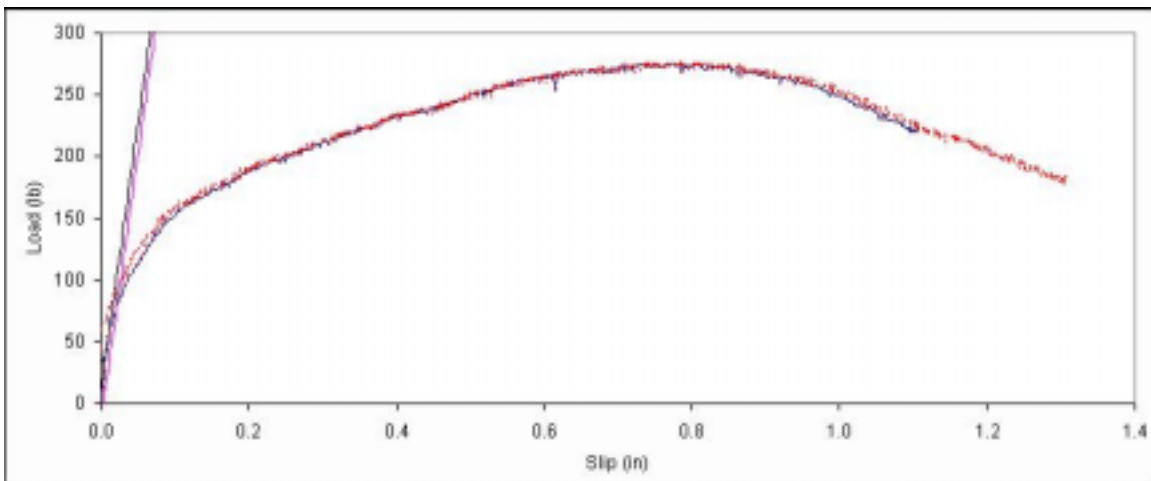
Figure B. 99: Load vs. slip plot for sample A7-11.
