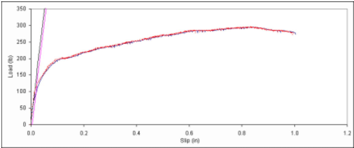
Figure B. 386: Load vs. slip plot for sample D6-1.
