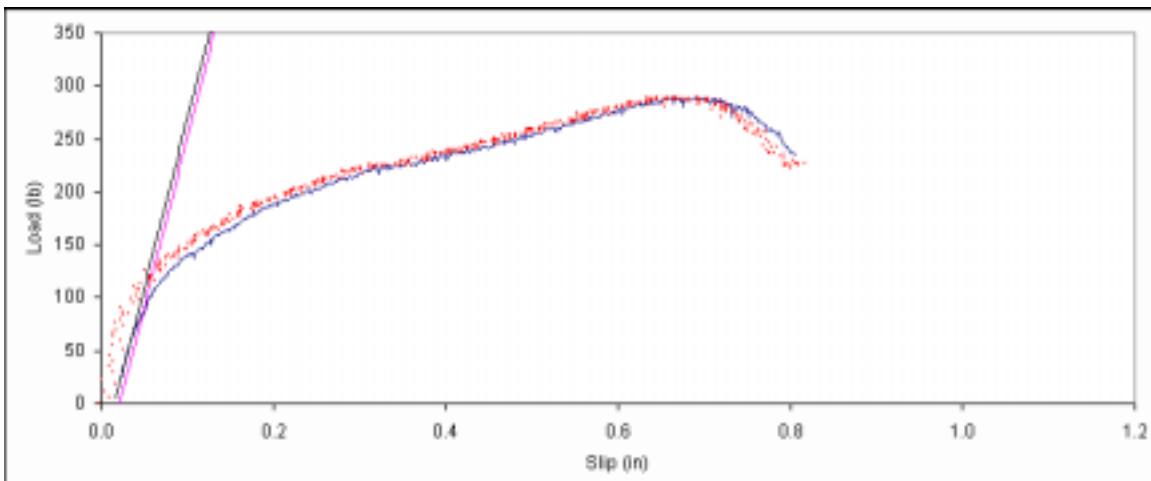
Figure B. 603: Load vs. slip plot for sample F6-11.
