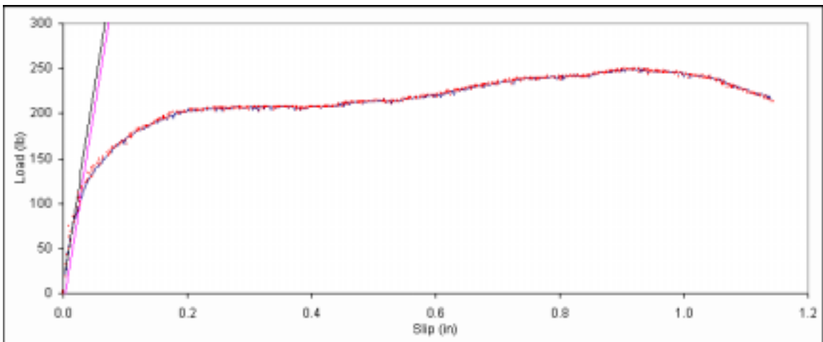
Figure B. 69: Load vs. slip plot for sample A5-10.
