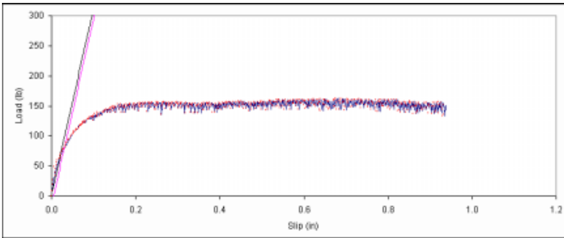
Figure B. 29: Load vs. slip plot for sample A2-15.
