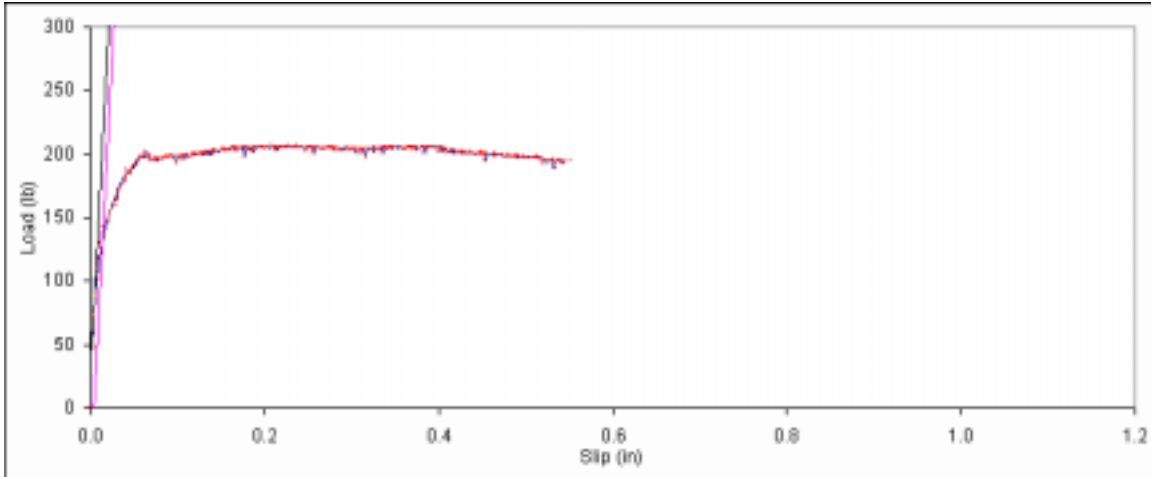
Figure B. 523: Load vs. slip plot for sample F1-4.
