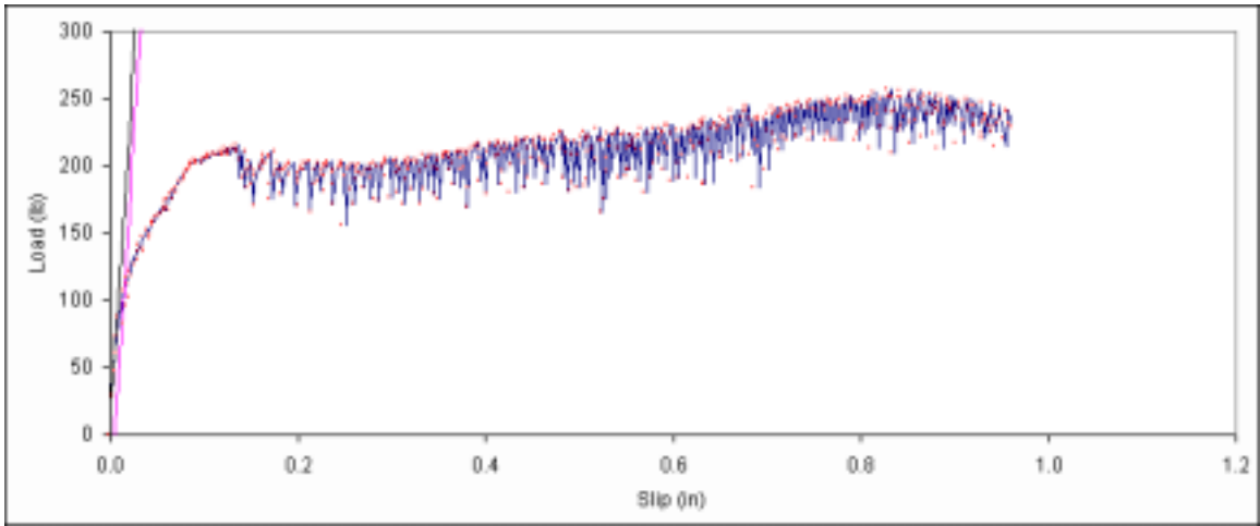
Figure B. 530: Load vs. slip plot for sample F1-11.
