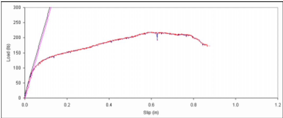
Figure B. 173: Load vs. slip plot for sample B5-11.
