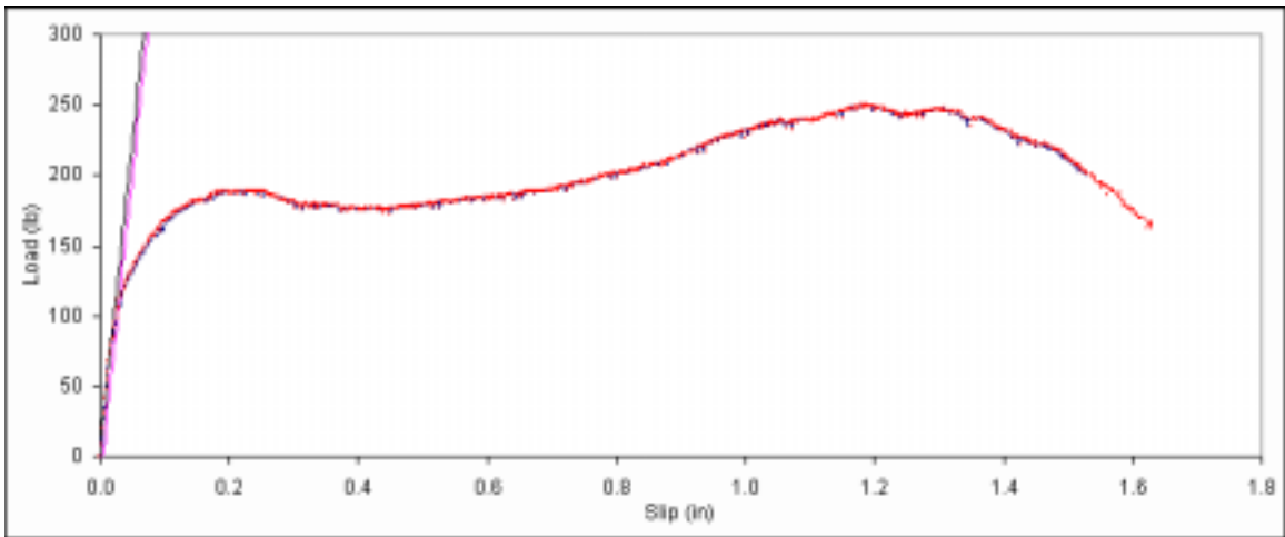
Figure B. 86: Load vs. slip plot for sample A6-13.
