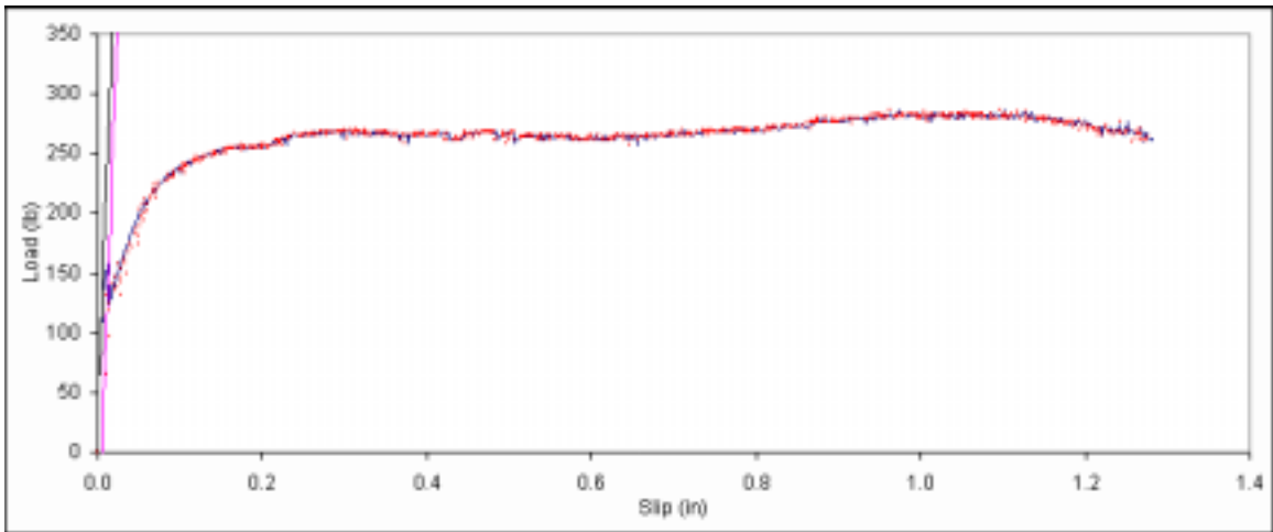
Figure B. 425: Load vs. slip plot for sample E1-10.
