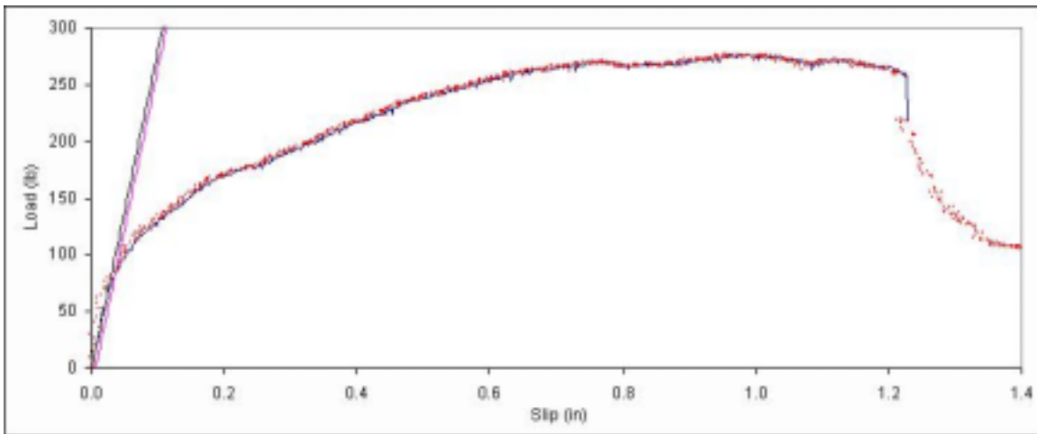
Figure B. 89: Load vs. slip plot for sample A7-1.
