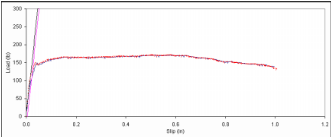
Figure B. 159: Load vs. slip plot for sample B4-12.
