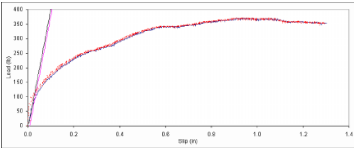
Figure B. 605: Load vs. slip plot for sample F6-13.
