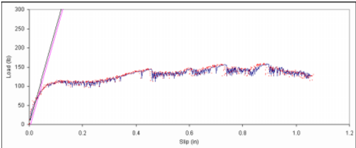
Figure B. 333: Load vs. slip plot for sample D2-8.
