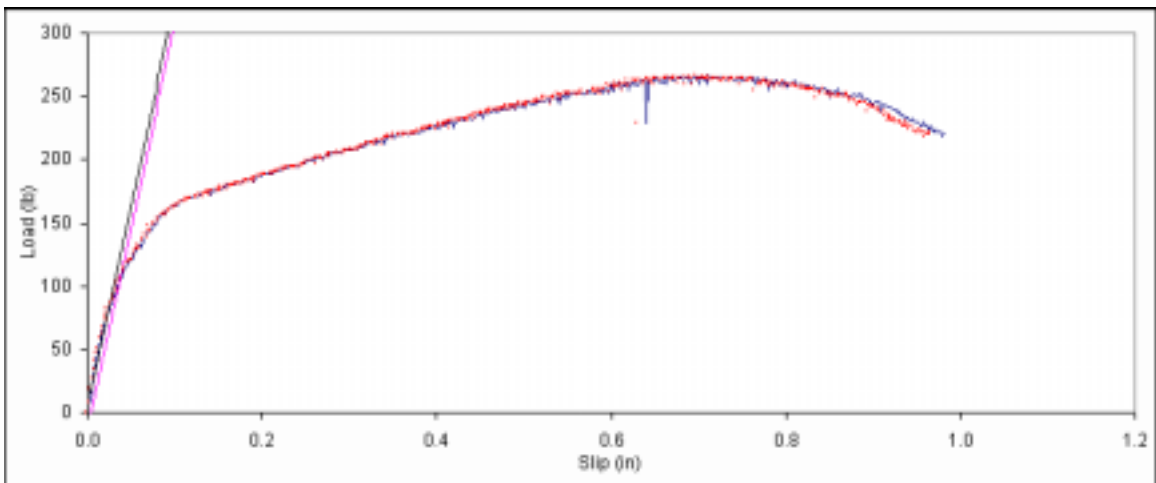
Figure B. 81: Load vs. slip plot for sample A6-8.
