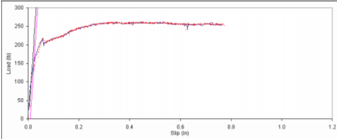
Figure B. 427: Load vs. slip plot for sample E1-12.
