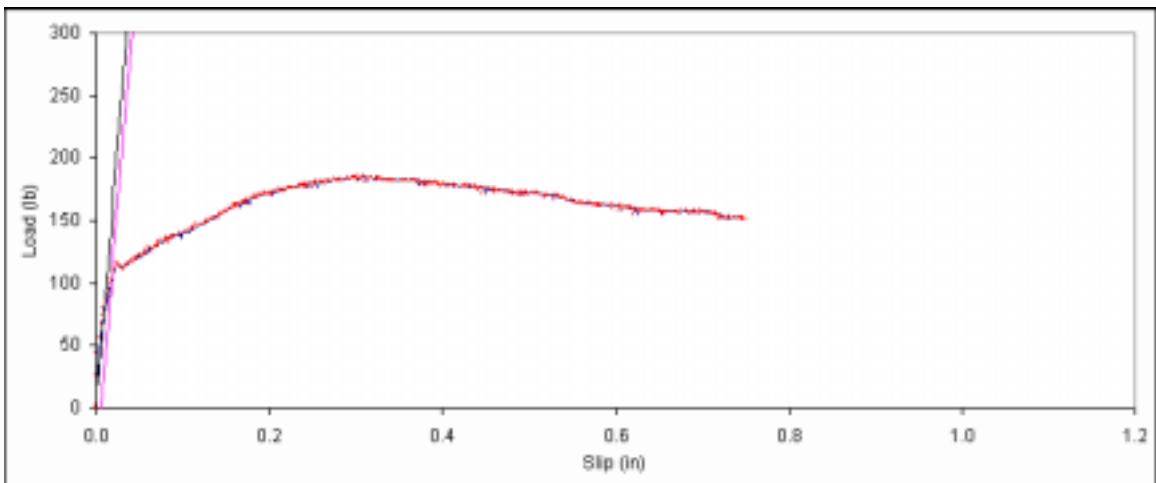
Figure B. 42: Load vs. slip plot for sample A3-13.
