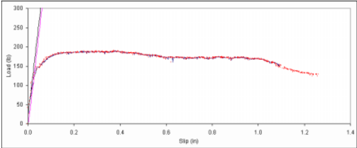
Figure B. 154: Load vs. slip plot for sample B4-7.
