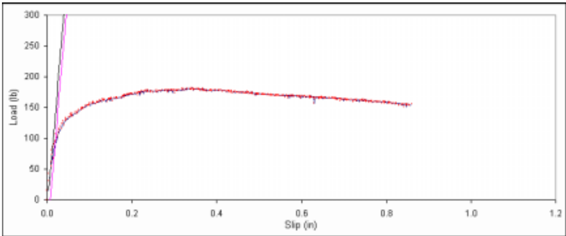
Figure B. 245: Load vs. slip plot for sample C3-9.
