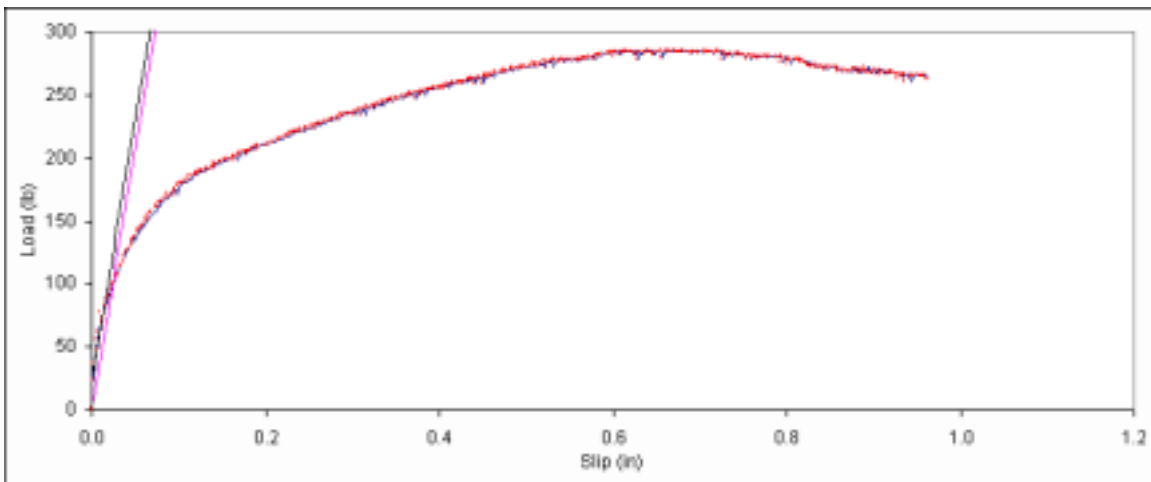
Figure B. 56: Load vs. slip plot for sample A4-12.
