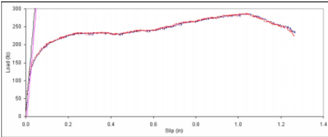
Figure B. 488: Load vs. slip plot for sample E5-13.
