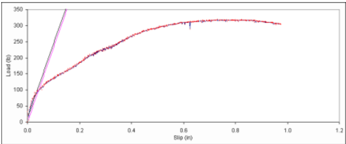
Figure B. 117: Load vs. slip plot for sample B1-15.
