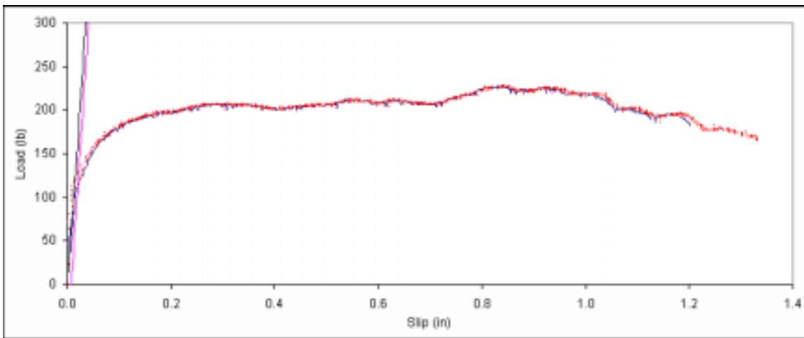
Figure B. 353: Load vs. slip plot for sample D3-13.
