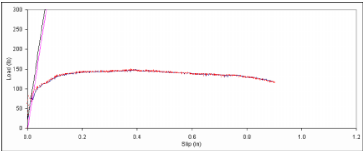
Figure B. 170: Load vs. slip plot for sample B5-8.
