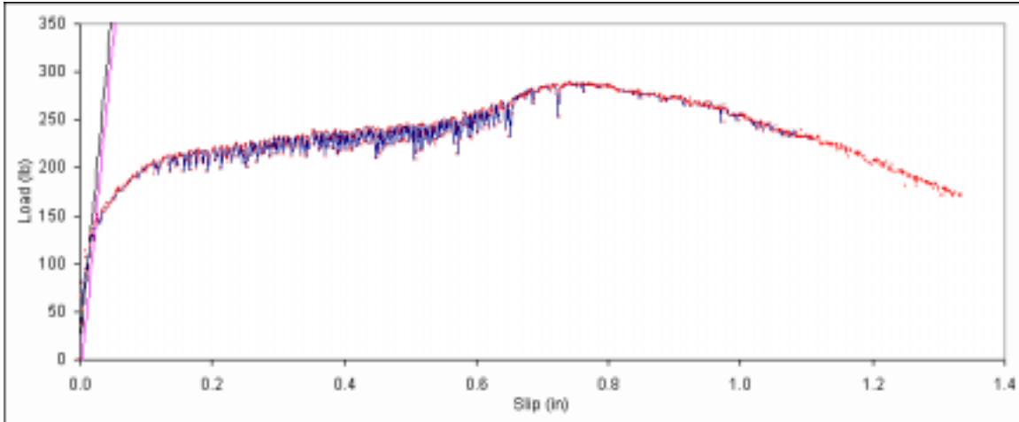
Figure B. 532: Load vs. slip plot for sample F1-13.
