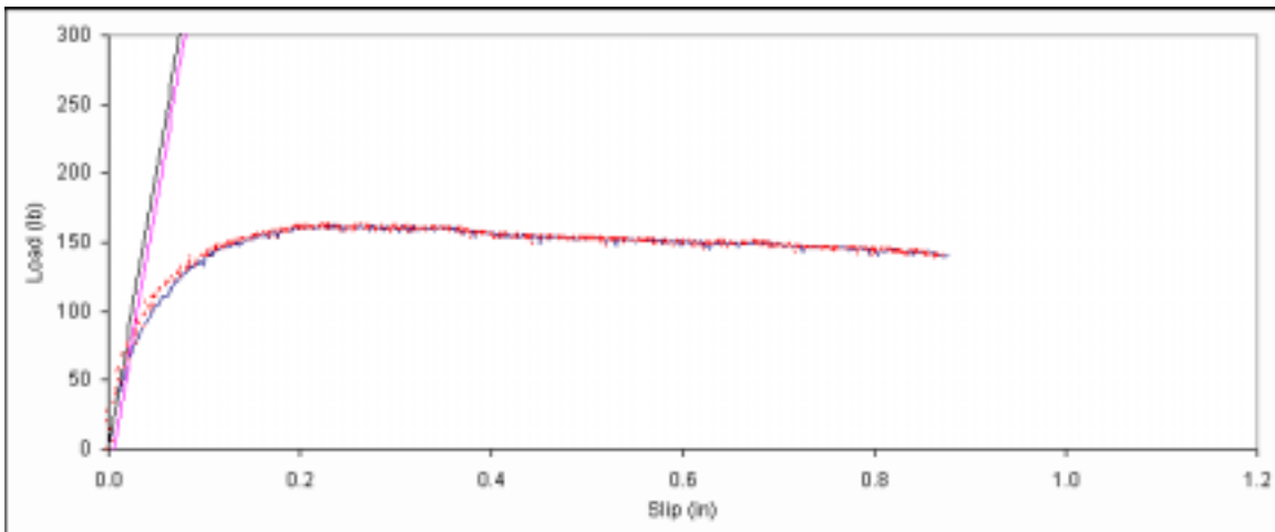
Figure B. 579: Load vs. slip plot for sample F5-2.
