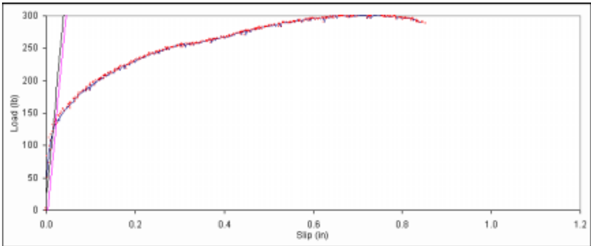
Figure B. 315: Load vs. slip plot for sample D1-4.
