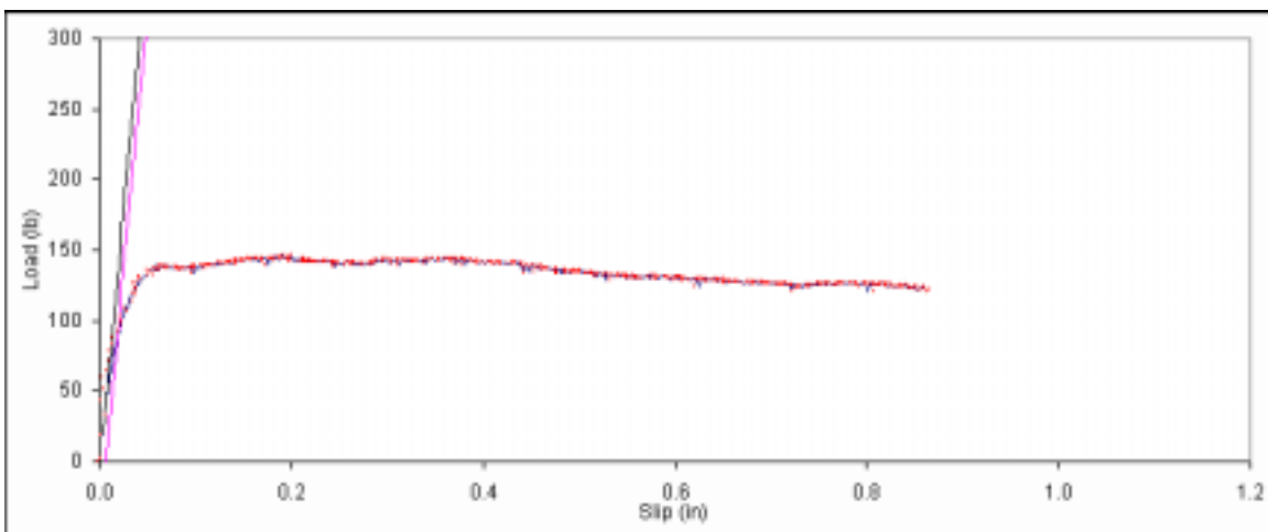
Figure B. 228: Load vs. slip plot for sample C2-6.
