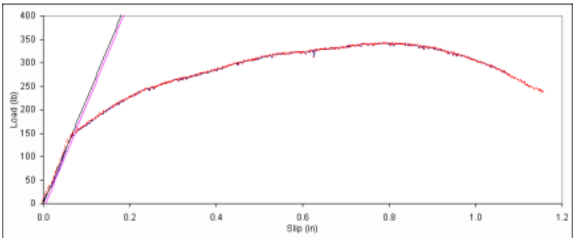
Figure B. 393: Load vs. slip plot for sample D6-8.
