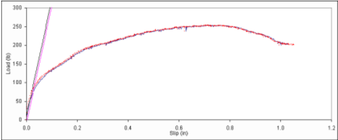
Figure B. 361: Load vs. slip plot for sample D4-6.
