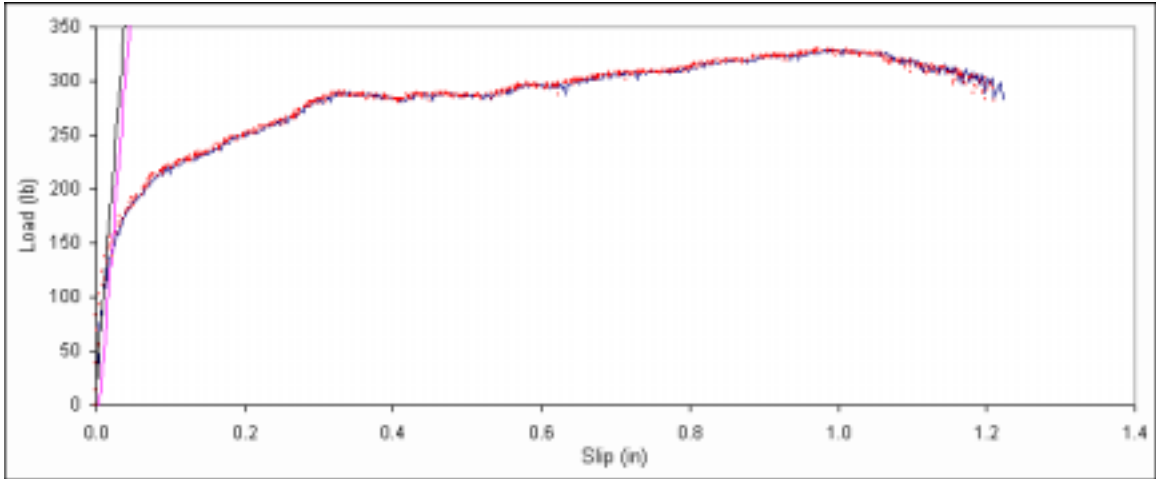
Figure B. 454: Load vs. slip plot for sample E3-9.
