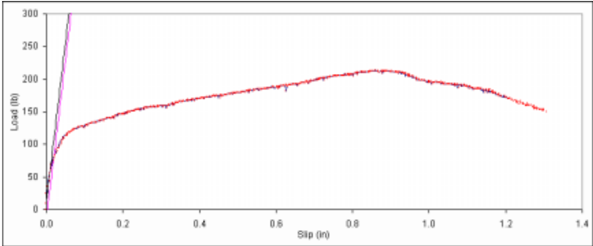
Figure B. 241: Load vs. slip plot for sample C3-4.
