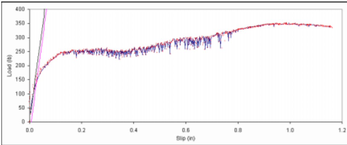
Figure B. 419: Load vs. slip plot for sample E1-4.
