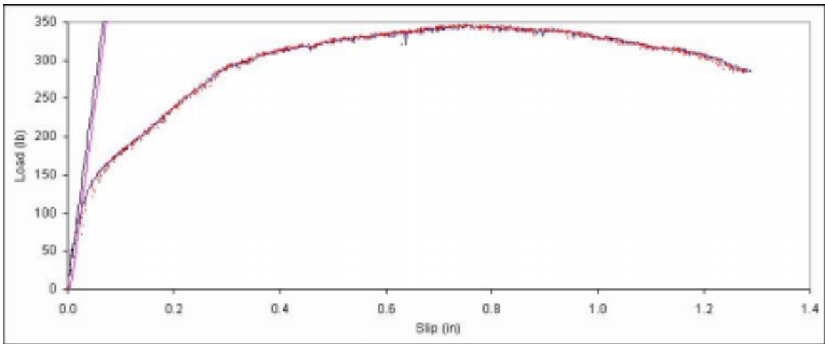
Figure B. 299: Load vs. slip plot for sample C7-3.
