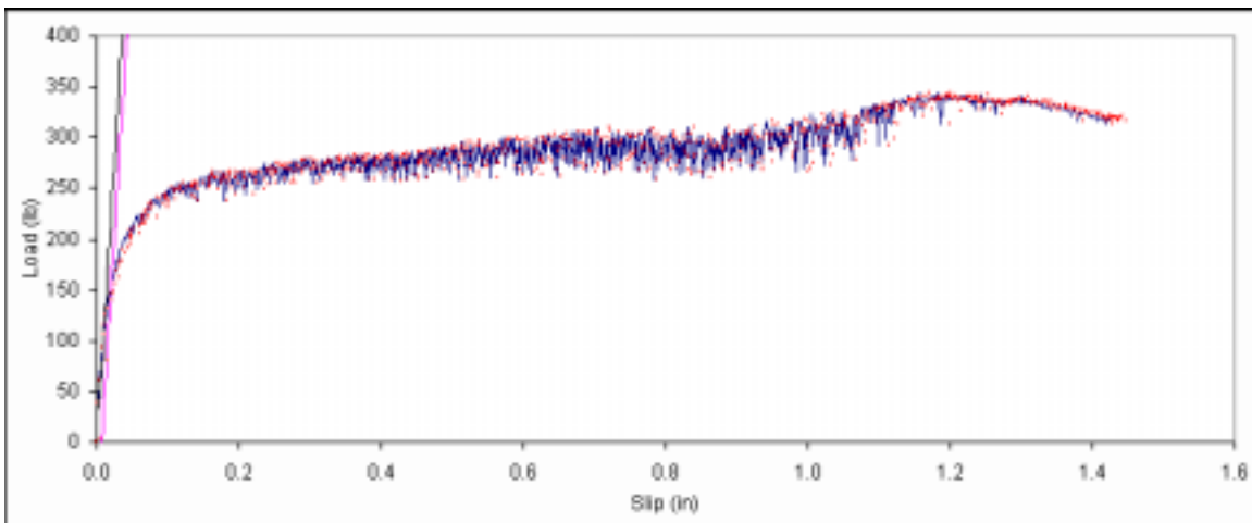
Figure B. 420: Load vs. slip plot for sample E1-5.
