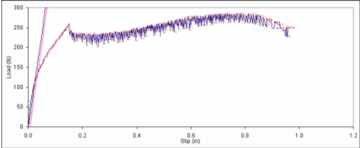
Figure B. 331: Load vs. slip plot for sample D2-6.
