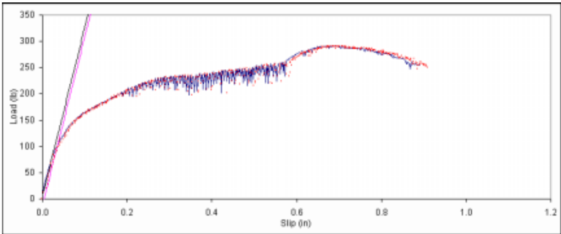
Figure B. 230: Load vs. slip plot for sample C2-8.
