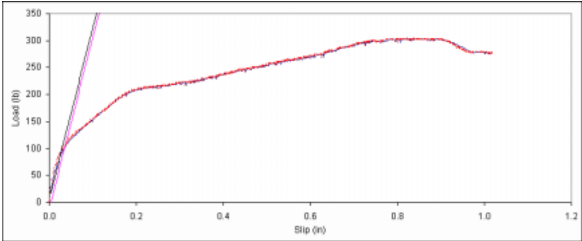
Figure B. 283: Load vs. slip plot for sample C6-2.
