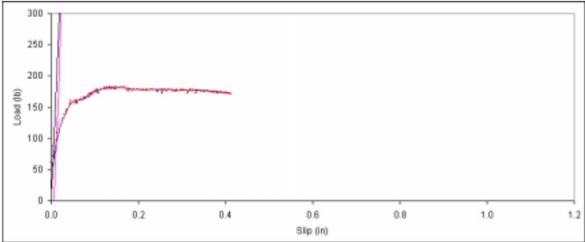
Figure B. 544: Load vs. slip plot for sample F2-11.
