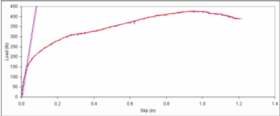
Figure B. 286: Load vs. slip plot for sample C6-5.
