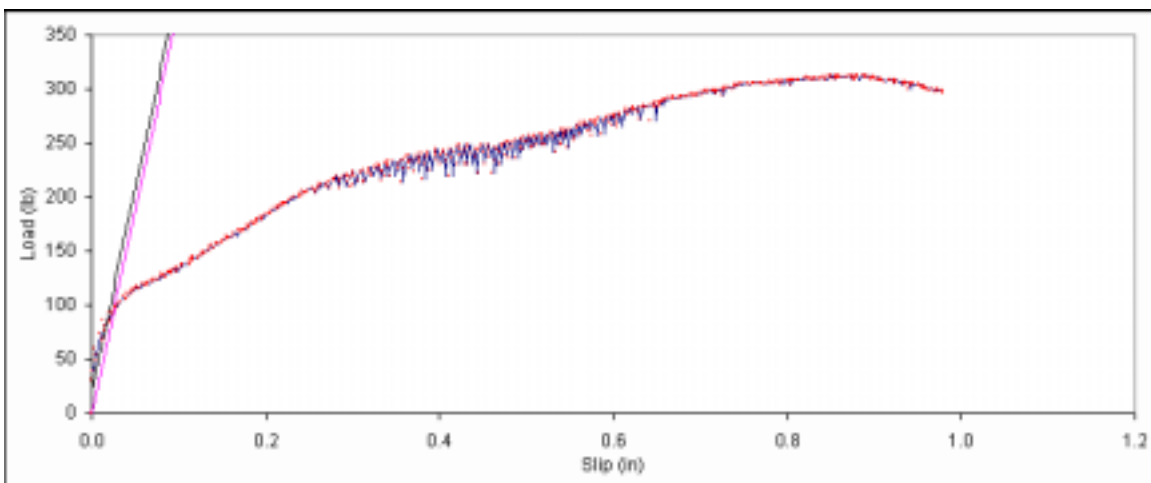
Figure B. 219: Load vs. slip plot for sample C1-12.
