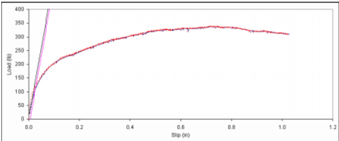
Figure B. 387: Load vs. slip plot for sample D6-2.
