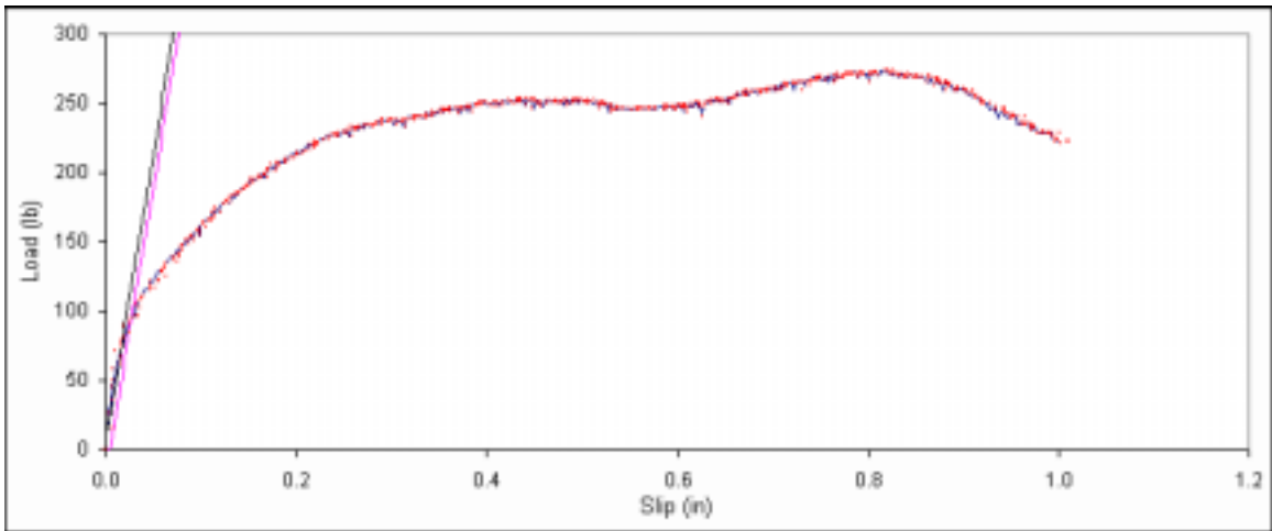
Figure B. 275: Load vs. slip plot for sample C5-9.
