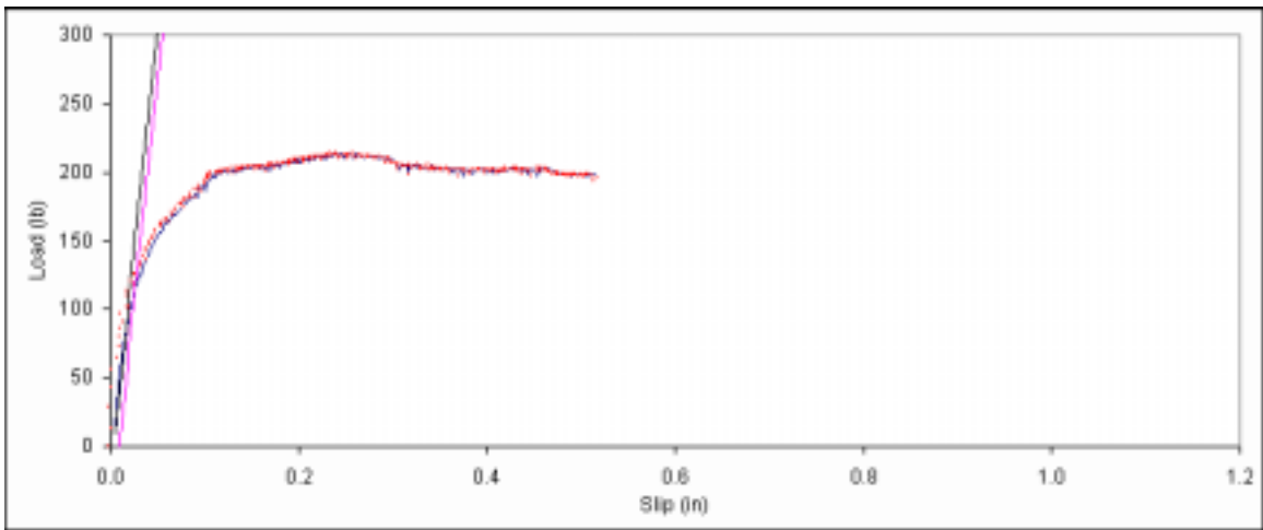
Figure B. 26: Load vs. slip plot for sample A2-12.
