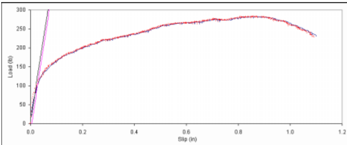
Figure B. 252: Load vs. slip plot for sample C4-1.
