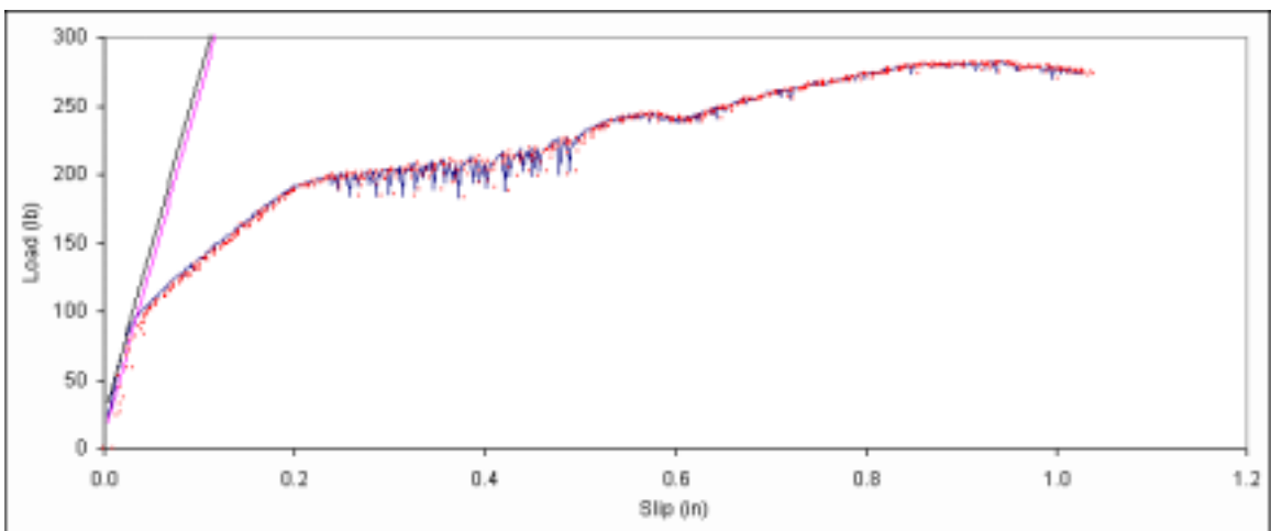
Figure B. 522: Load vs. slip plot for sample F1-3.
