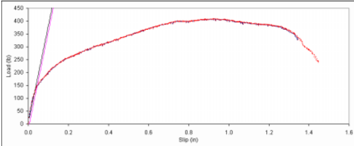
Figure B. 487: Load vs. slip plot for sample E5-12.
