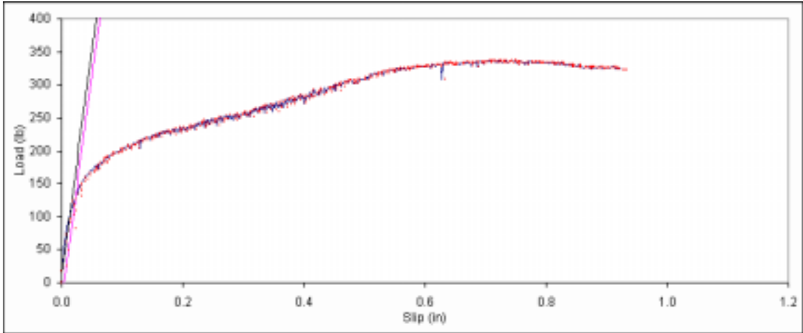
Figure B. 10: Load vs. slip plot for sample A1-10.
