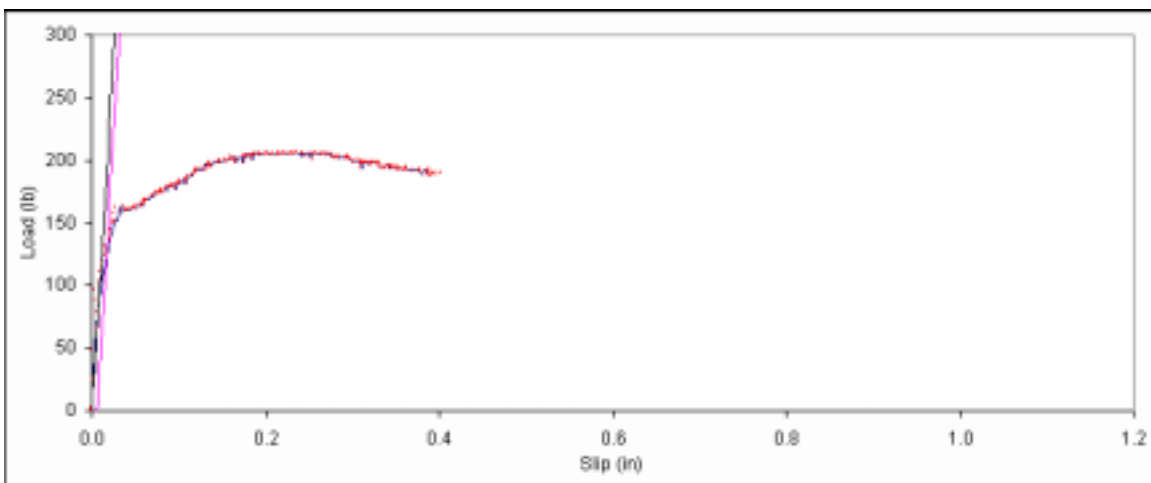
Figure B. 327: Load vs. slip plot for sample D2-2.
