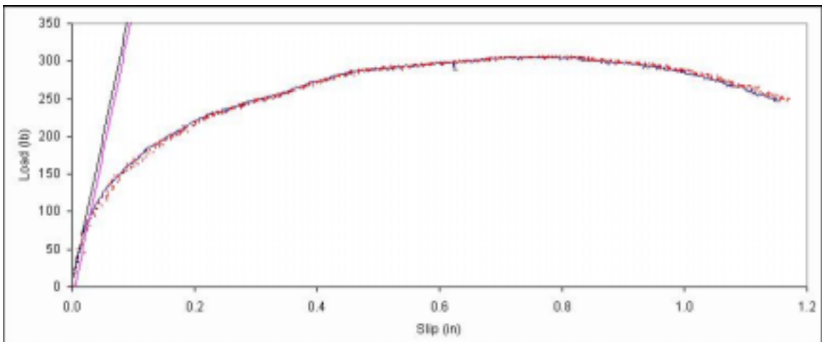
Figure B. 411: Load vs. slip plot for sample D7-11.
