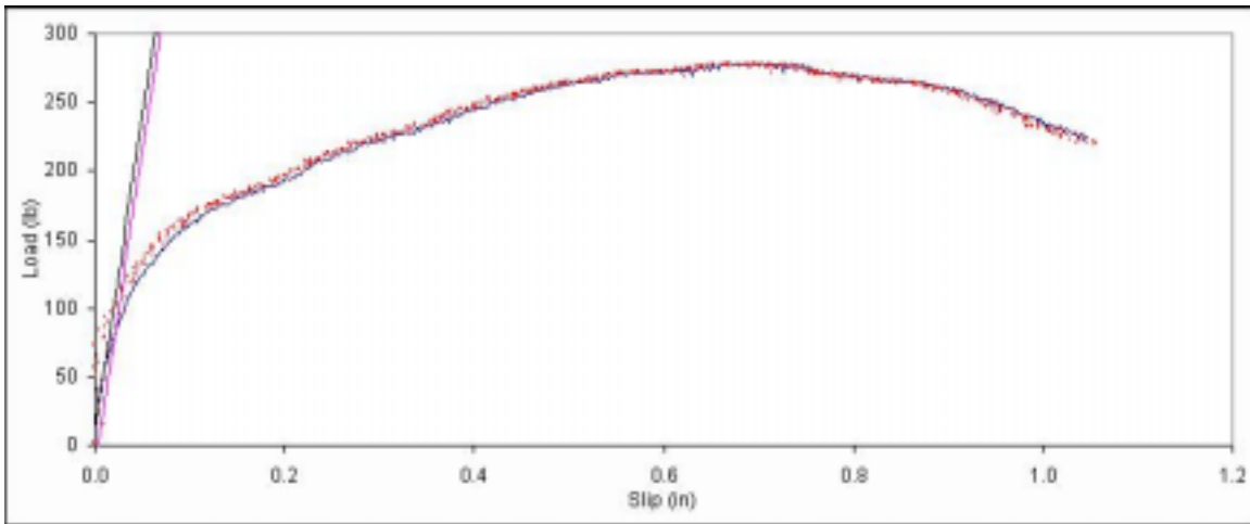
Figure B. 200: Load vs. slip plot for sample B7-8.
