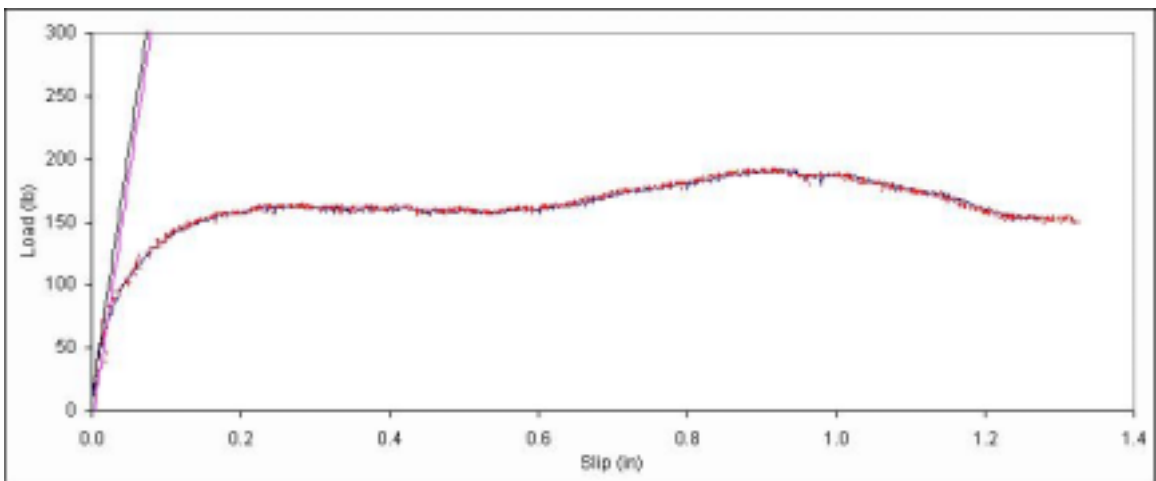
Figure B. 207: Load vs. slip plot for sample B7-15.
