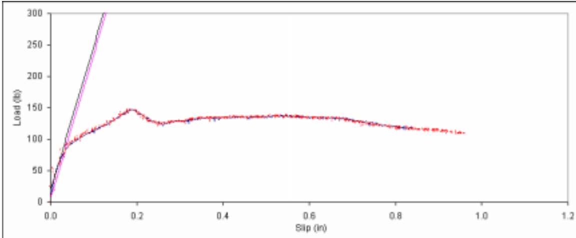
Figure B. 148: Load vs. slip plot for sample B4-1.
