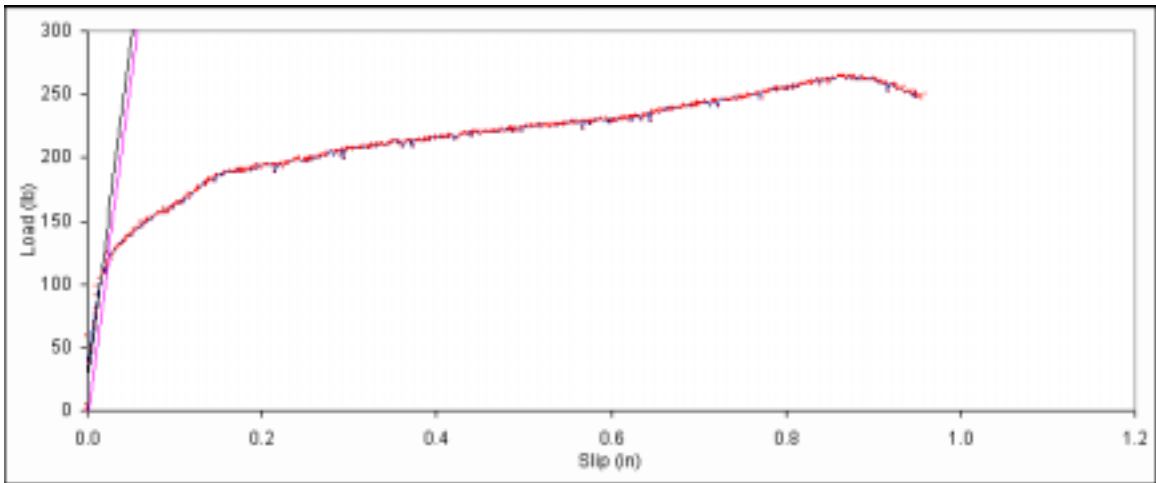
Figure B. 527: Load vs. slip plot for sample F1-8.
