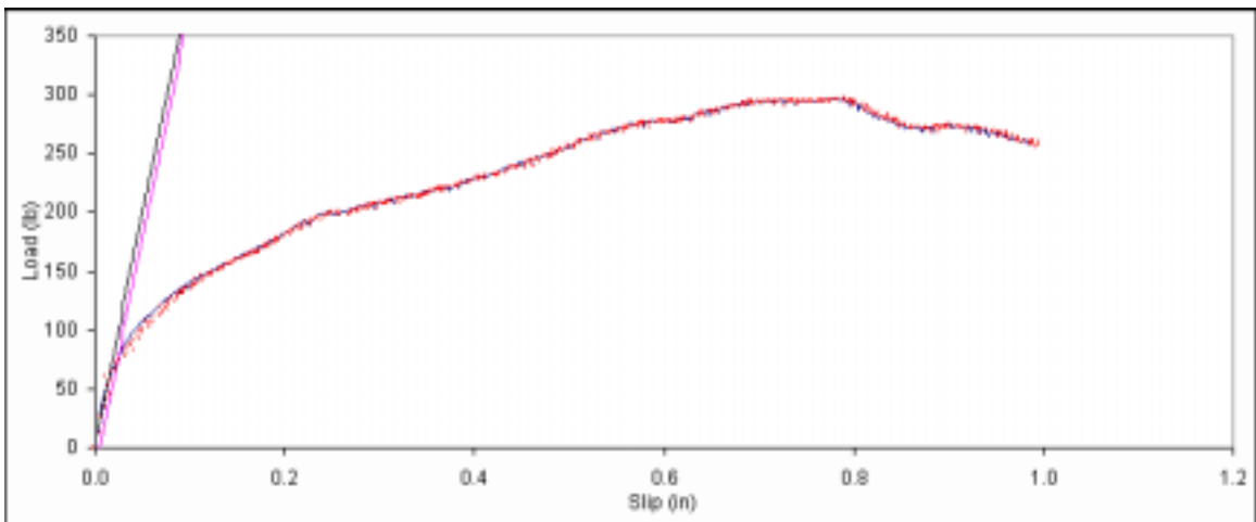
Figure B. 378: Load vs. slip plot for sample D5-8.
