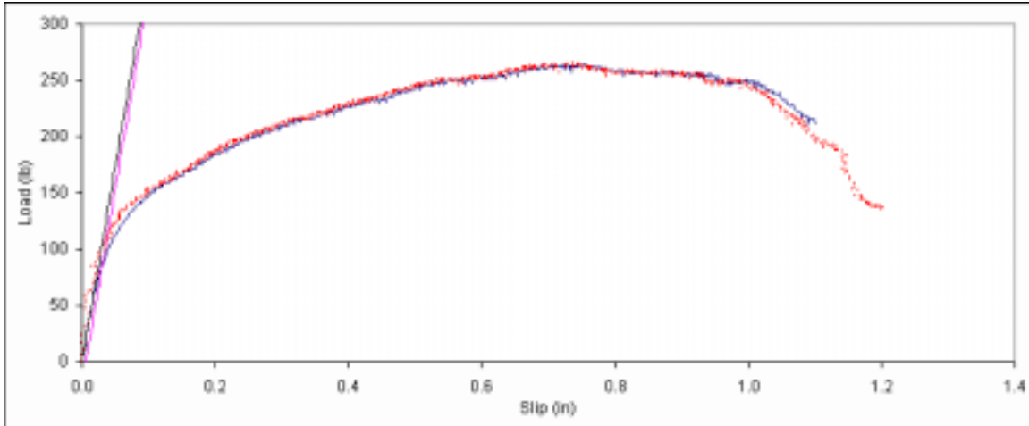
Figure B. 382: Load vs. slip plot for sample D5-12.
