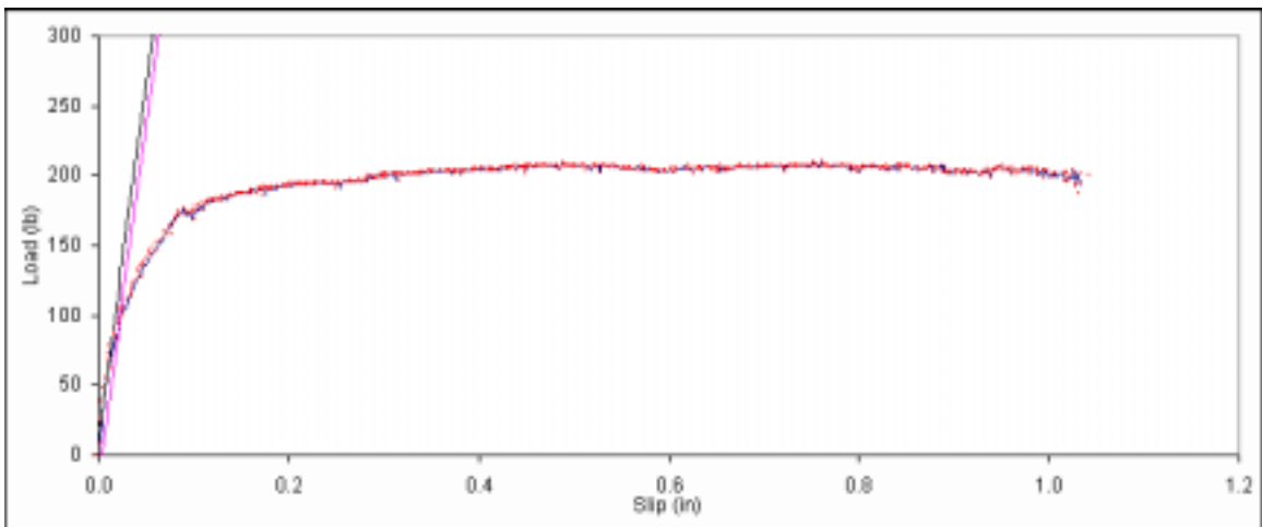
Figure B. 108: Load vs. slip plot for sample B1-6.
