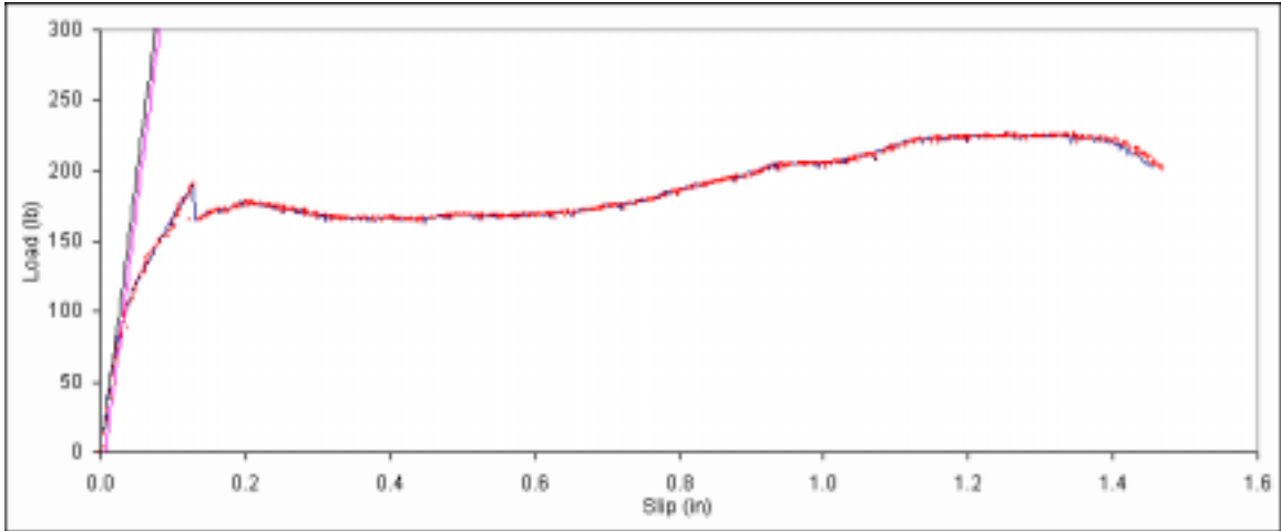
Figure B. 181: Load vs. slip plot for sample B6-4.
