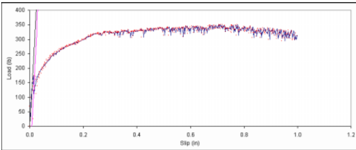
Figure B. 428: Load vs. slip plot for sample E1-13.
