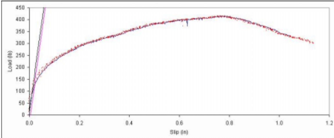
Figure B. 307: Load vs. slip plot for sample C7-11.
