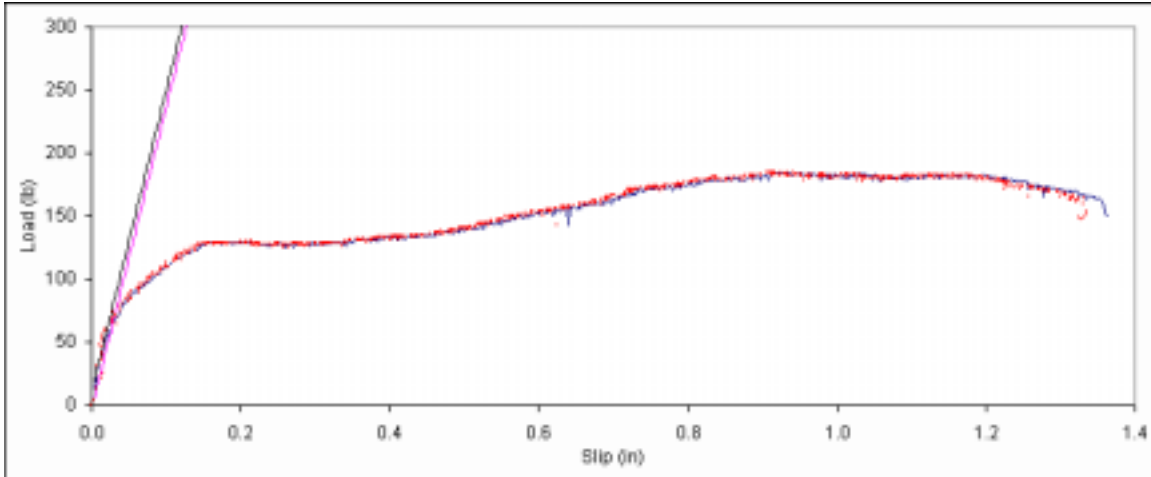
Figure B. 355: Load vs. slip plot for sample D3-15.
