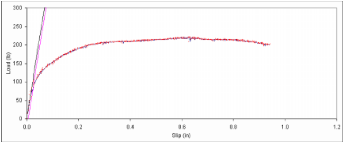
Figure B. 244: Load vs. slip plot for sample C3-7.
