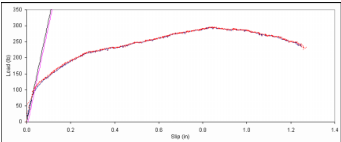
Figure B. 279: Load vs. slip plot for sample C5-13.
