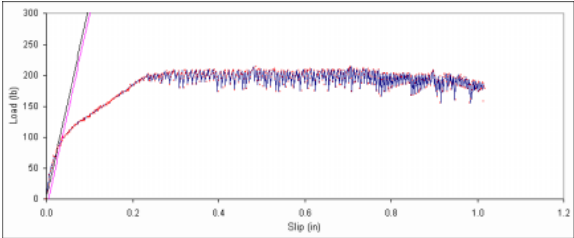
Figure B. 334: Load vs. slip plot for sample D2-9.
