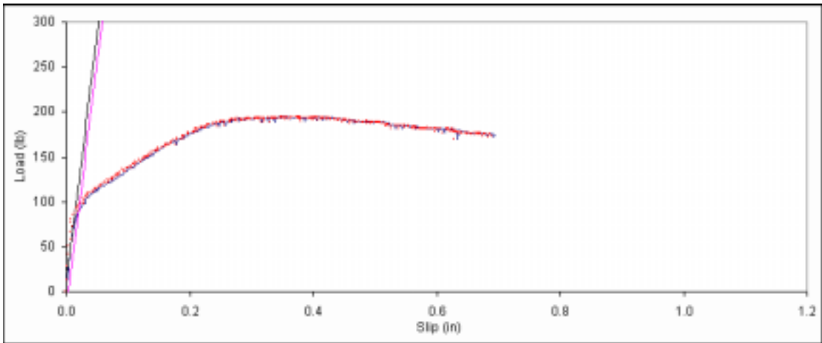
Figure B. 146: Load vs. slip plot for sample B3-14.
