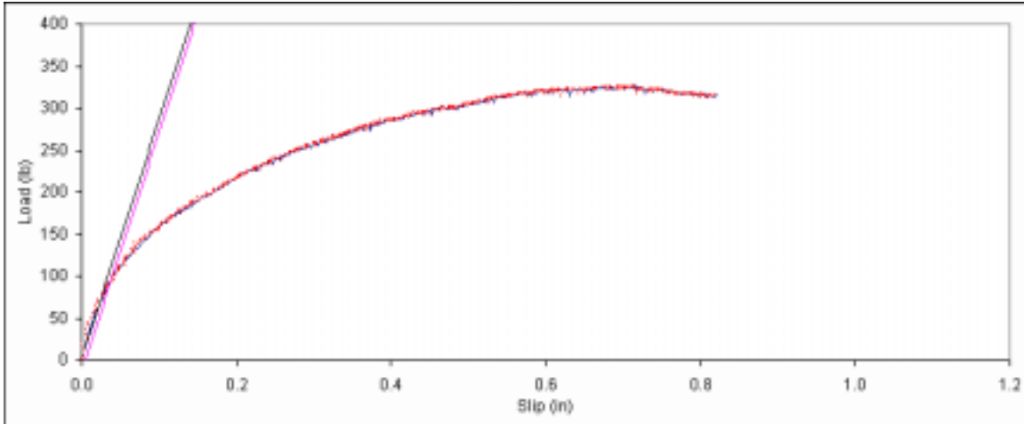
Figure B. 400: Load vs. slip plot for sample D6-15.
