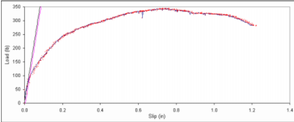
Figure B. 601: Load vs. slip plot for sample F6-9.
