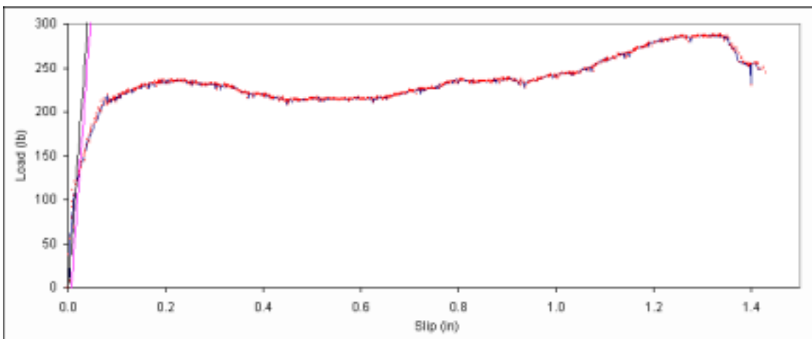
Figure B. 15: Load vs. slip plot for sample A2-1.
