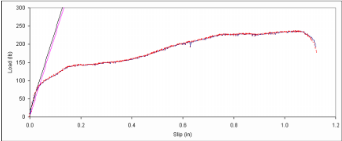
Figure B. 70: Load vs. slip plot for sample A5-11.
