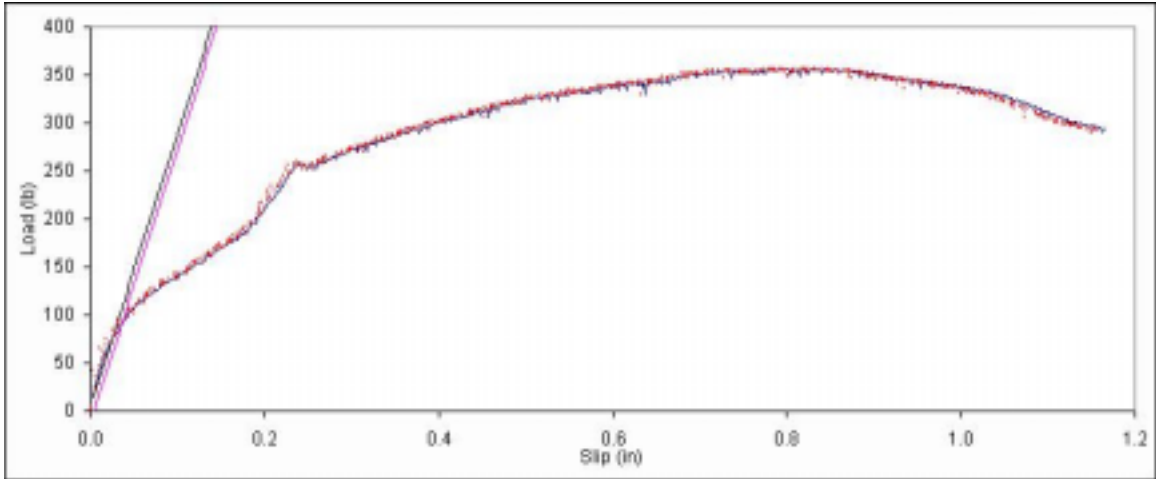
Figure B. 613: Load vs. slip plot for sample F7-6.
