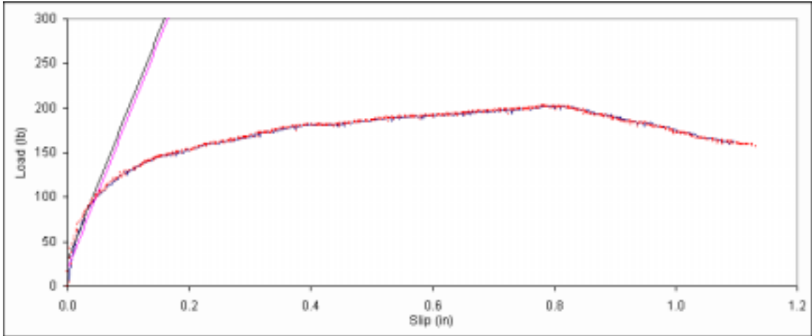
Figure B. 367: Load vs. slip plot for sample D4-12.
