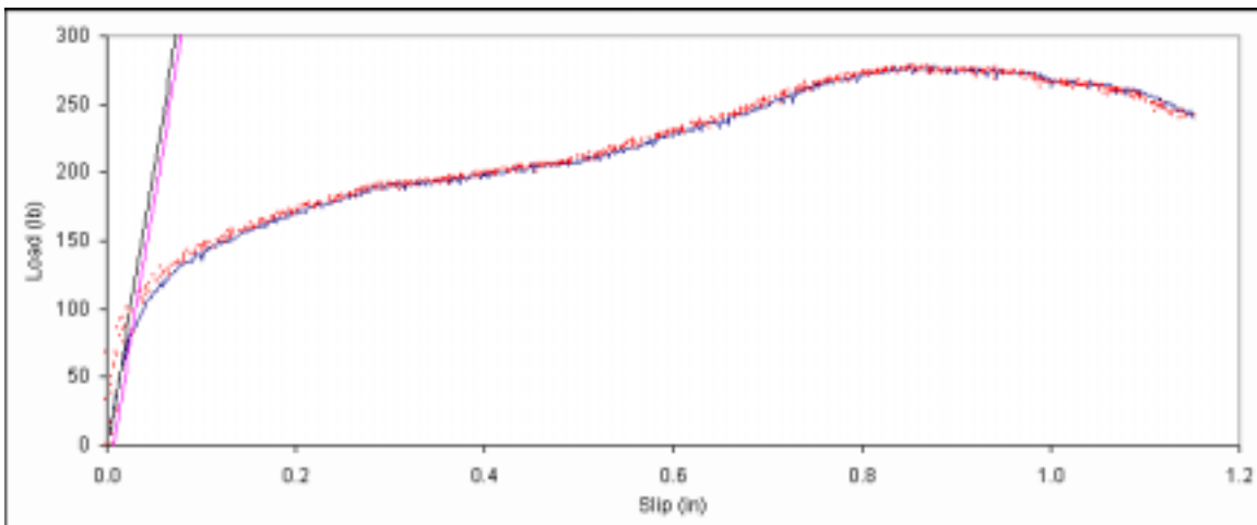
Figure B. 594: Load vs. slip plot for sample F6-2.
