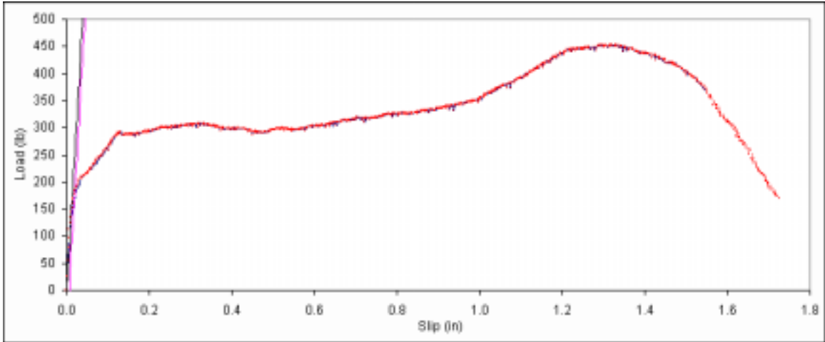
Figure B. 265: Load vs. slip plot for sample C4-14.
