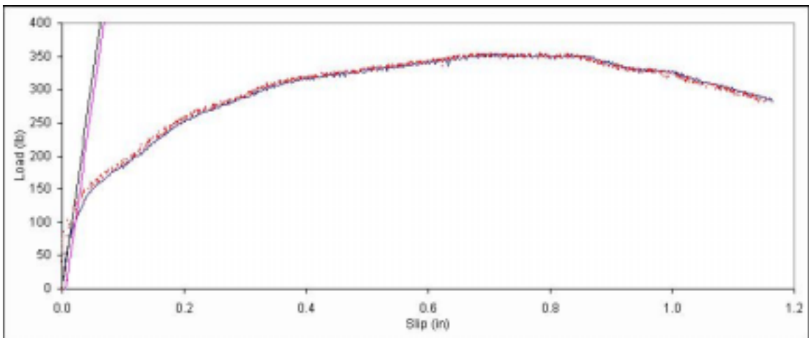
Figure B. 306: Load vs. slip plot for sample C7-10.
