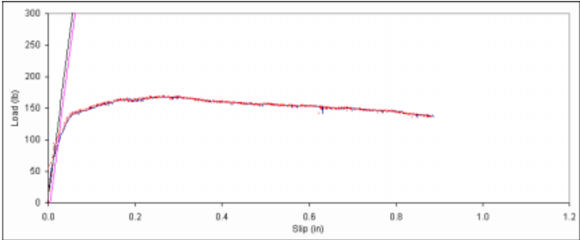
Figure B. 19: Load vs. slip plot for sample A2-5.
