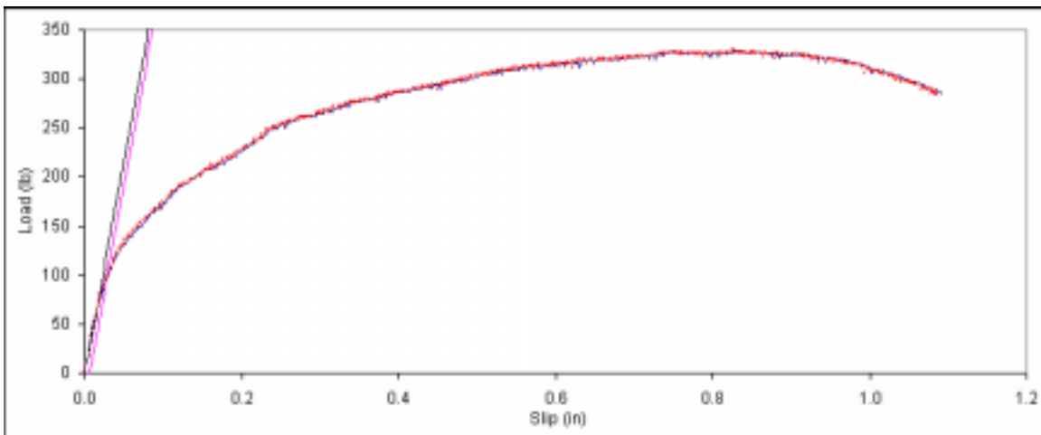
Figure B. 399: Load vs. slip plot for sample D6-14.
