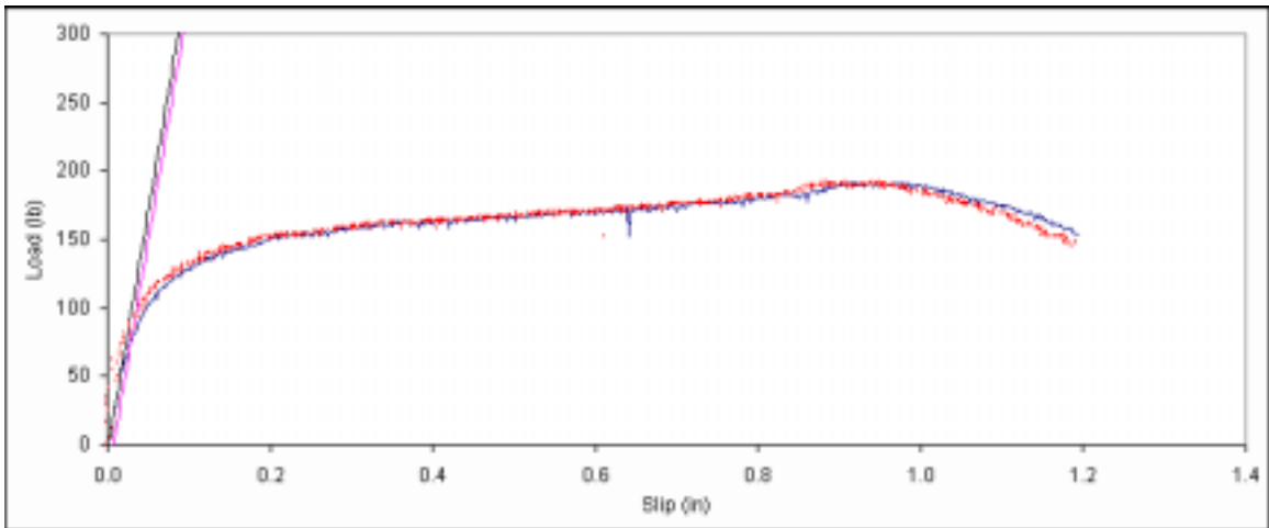
Figure B. 549: Load vs. slip plot for sample F3-2.
