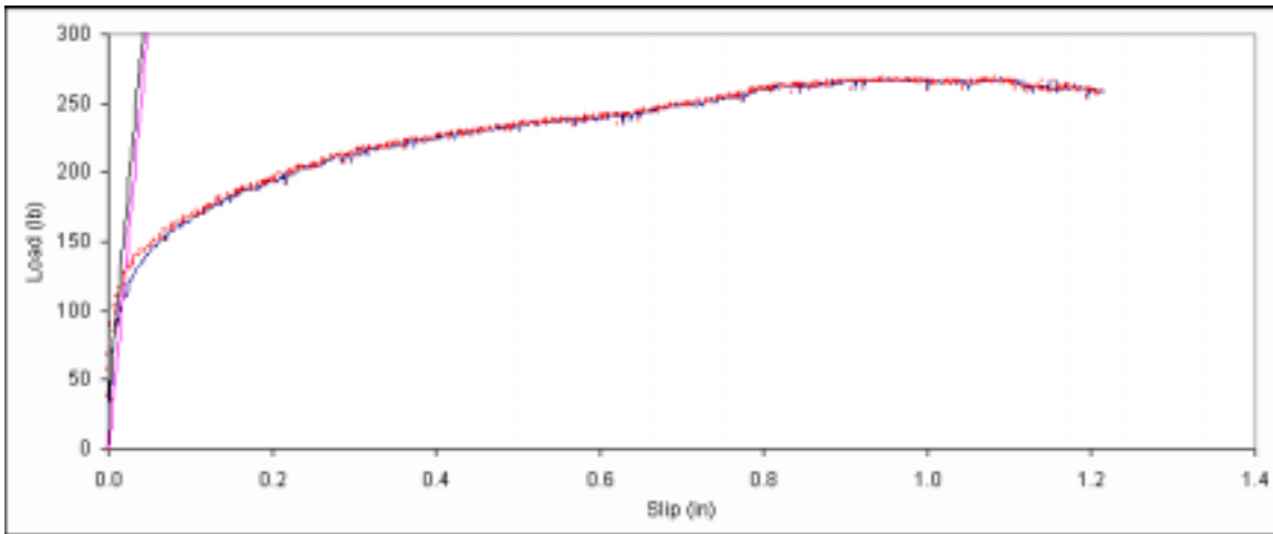
Figure B. 2: Load vs. slip plot for sample A1-2.
