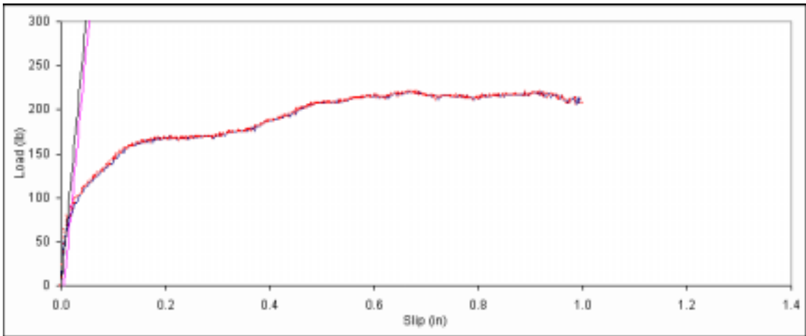
Figure B. 215: Load vs. slip plot for sample C1-8.
