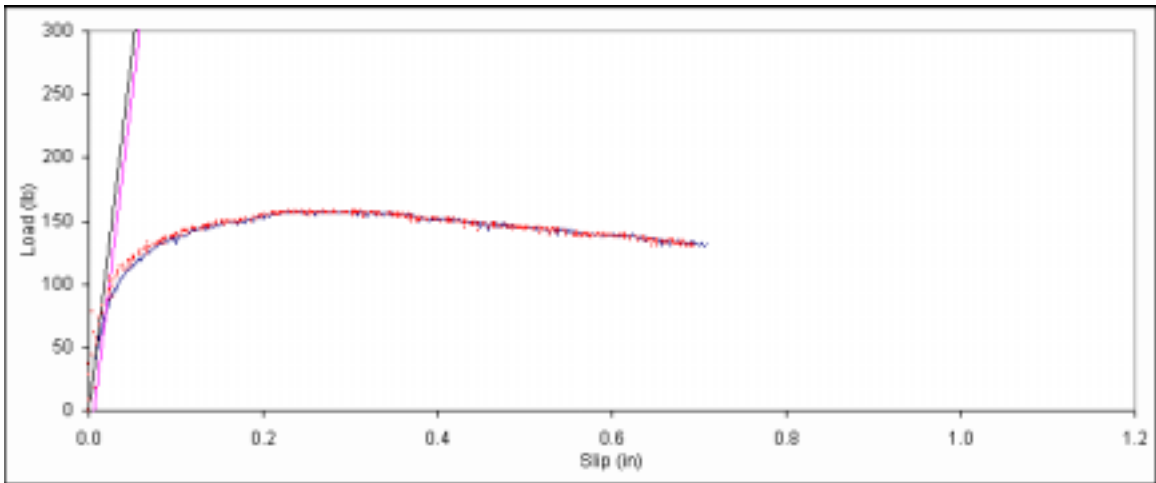
Figure B. 557: Load vs. slip plot for sample F3-10.
