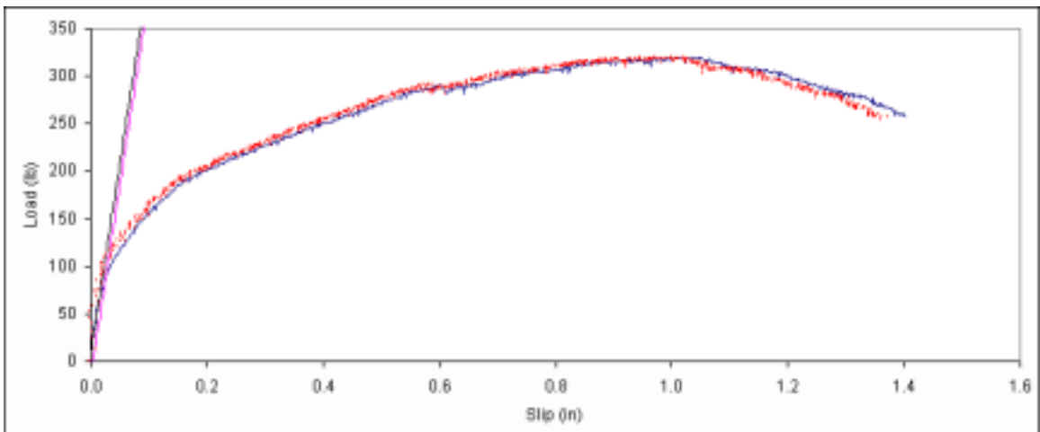
Figure B. 366: Load vs. slip plot for sample D4-11.
