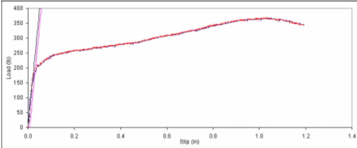
Figure B. 421: Load vs. slip plot for sample E1-6.
