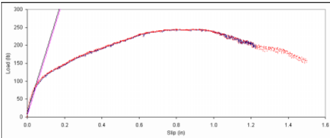
Figure B. 165: Load vs. slip plot for sample B5-3.
