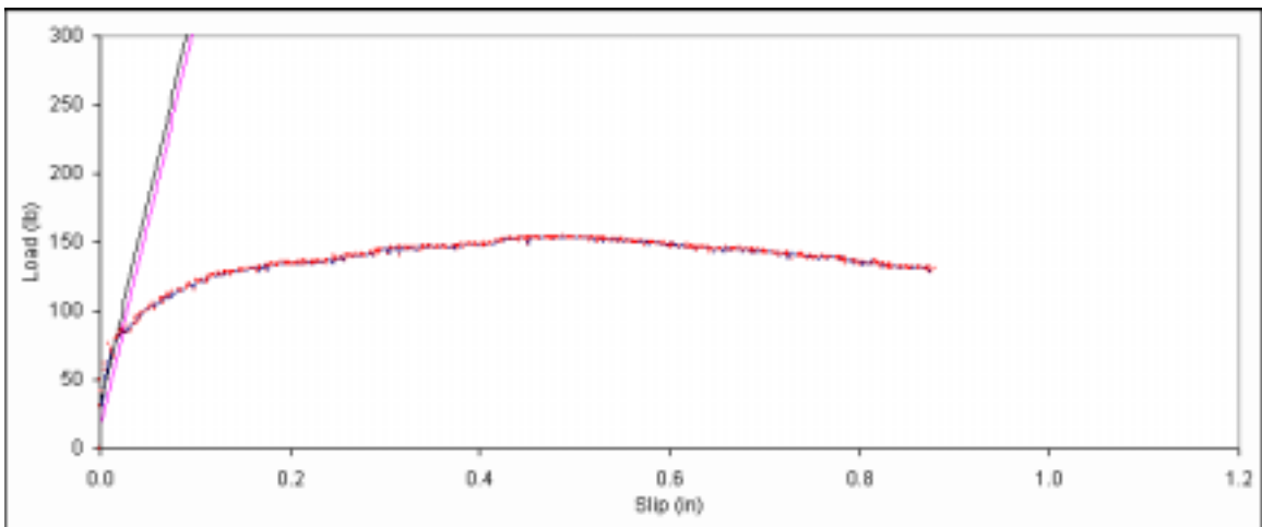
Figure B. 147: Load vs. slip plot for sample B3-15.
