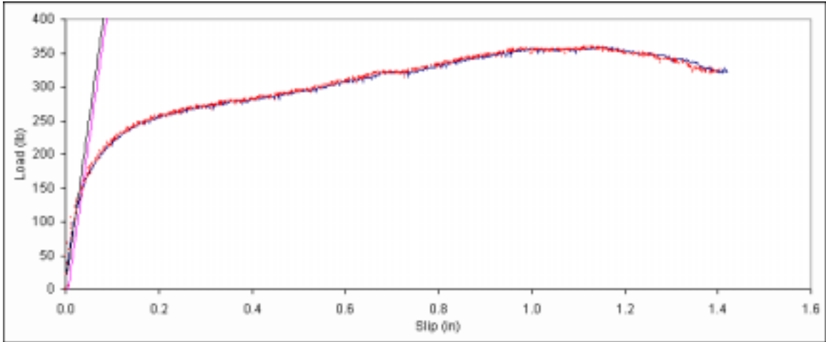
Figure B. 442: Load vs. slip plot for sample E2-12.
