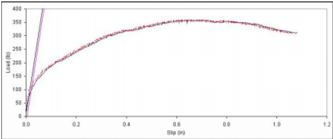
Figure B. 407: Load vs. slip plot for sample D7-7.
