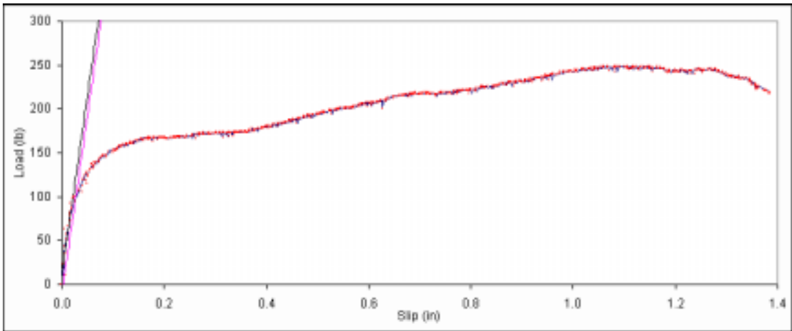
Figure B. 65: Load vs. slip plot for sample A5-6.
