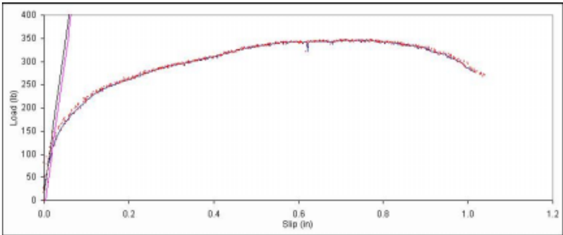
Figure B. 404: Load vs. slip plot for sample D7-4.
