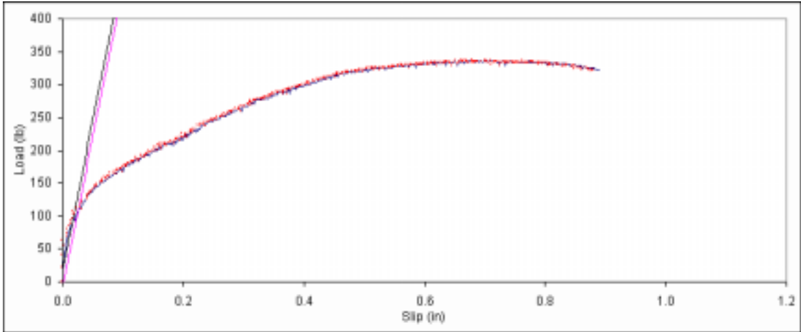
Figure B. 115: Load vs. slip plot for sample B1-13.
