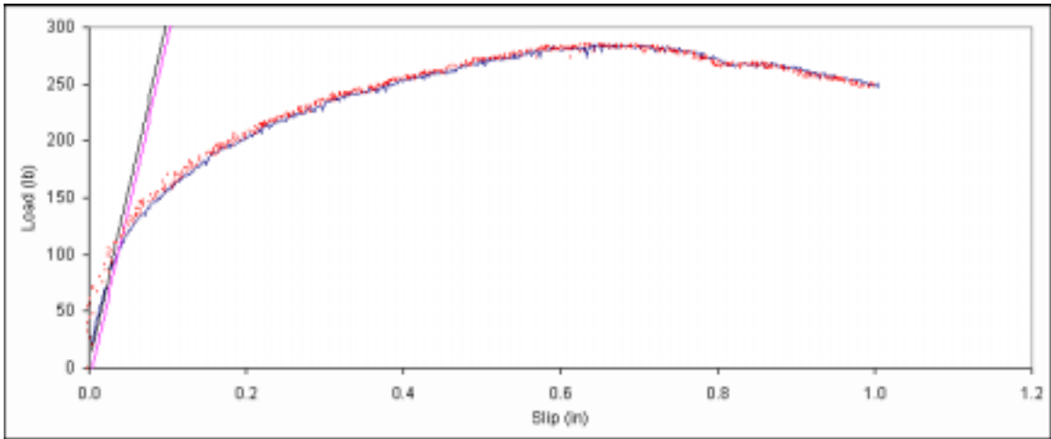
Figure B. 179: Load vs. slip plot for sample B6-2.
