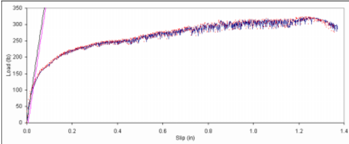
Figure B. 499: Load vs. slip plot for sample E6-10.
