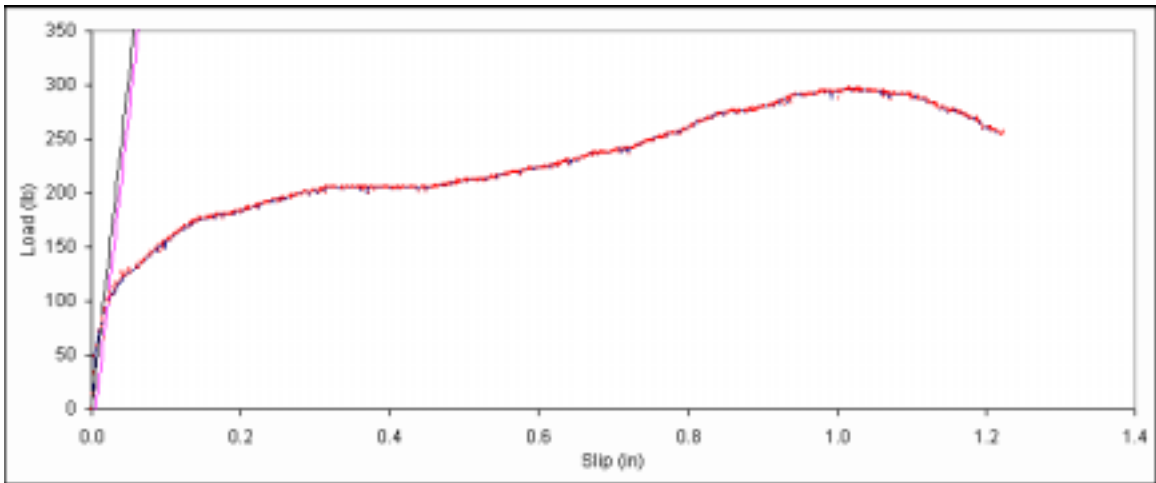
Figure B. 248: Load vs. slip plot for sample C3-12.
