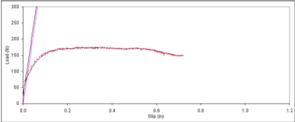
Figure B. 145: Load vs. slip plot for sample B3-13.
