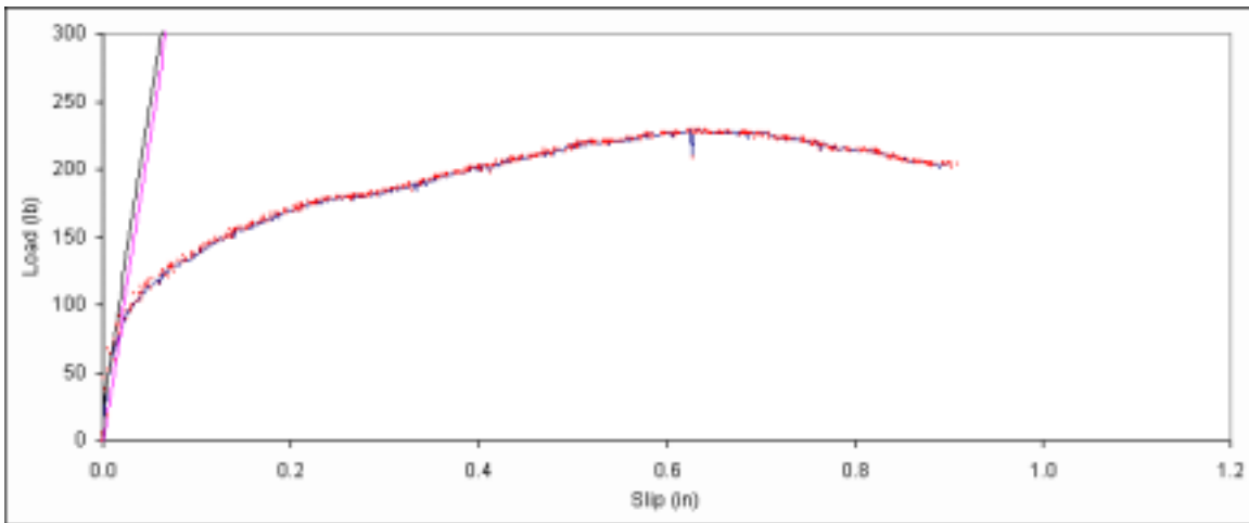
Figure B. 32: Load vs. slip plot for sample A3-3.
