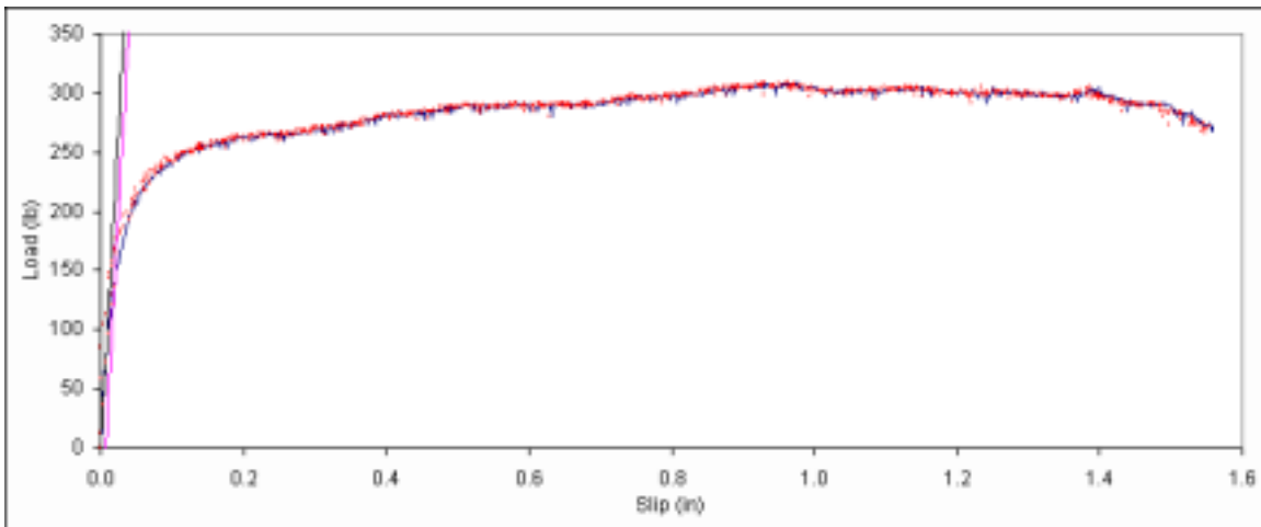
Figure B. 504: Load vs. slip plot for sample E6-15.
