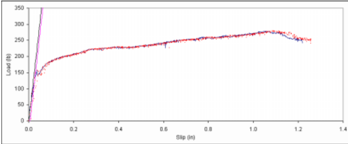
Figure B. 595: Load vs. slip plot for sample F6-3.
