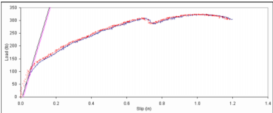
Figure B. 600: Load vs. slip plot for sample F6-8.
