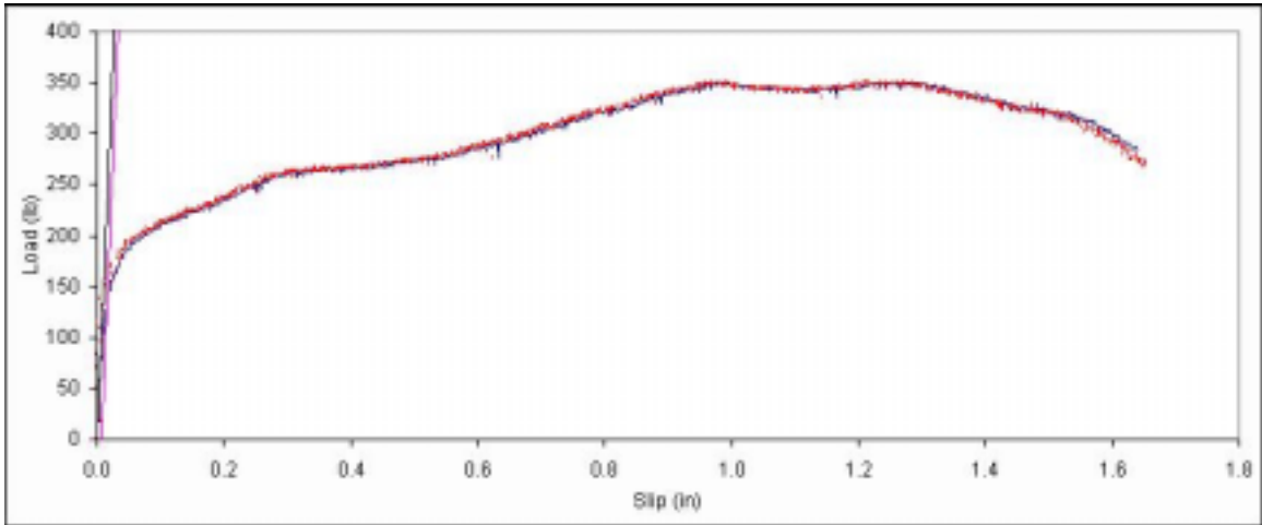
Figure B. 509: Load vs. slip plot for sample E7-5.
