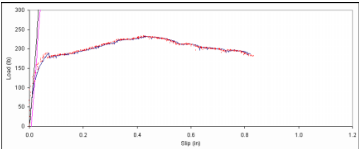
Figure B. 225: Load vs. slip plot for sample C2-3.
