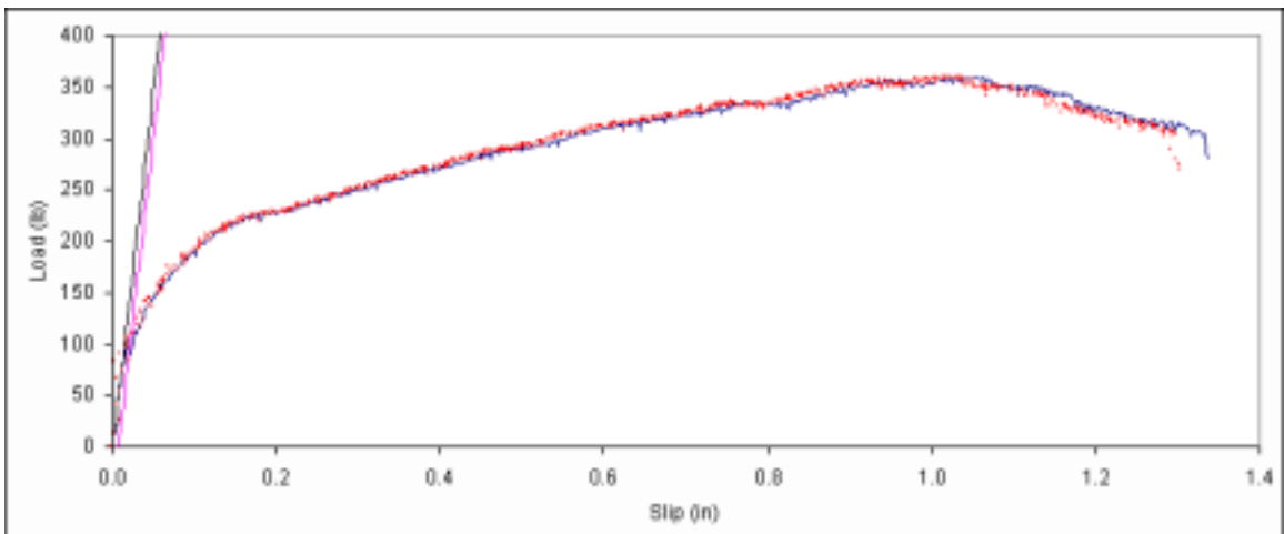
Figure B. 456: Load vs. slip plot for sample E3-11.
