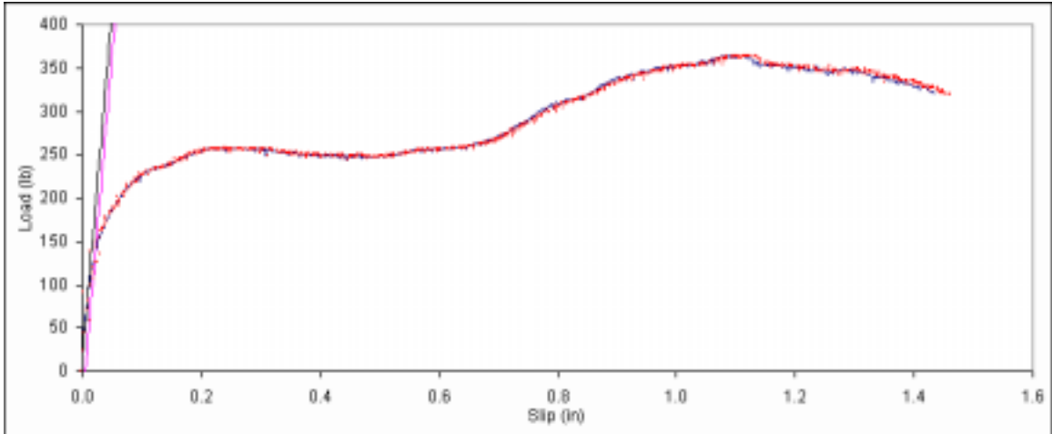
Figure B. 493: Load vs. slip plot for sample E6-4.
