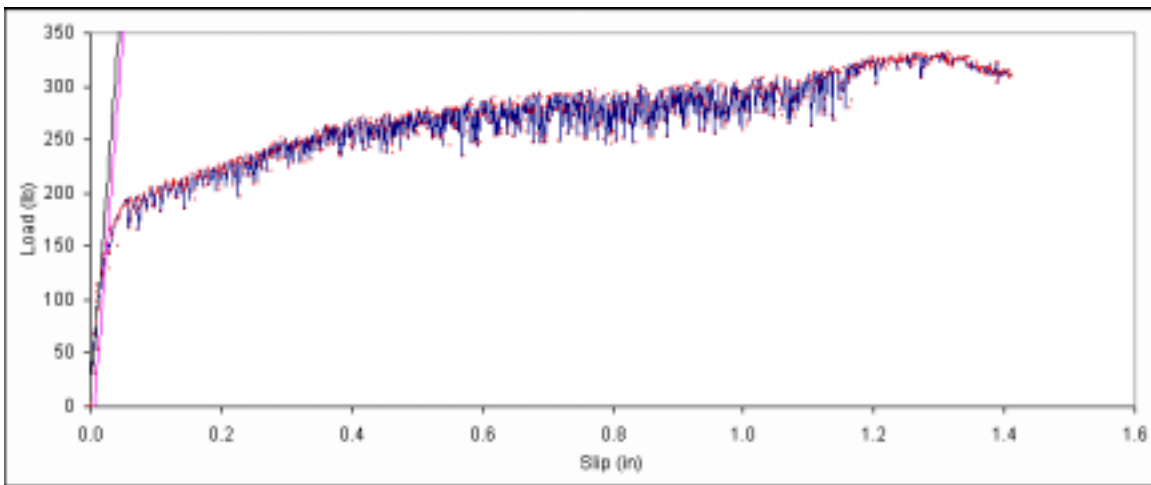
Figure B. 422: Load vs. slip plot for sample E1-7.
