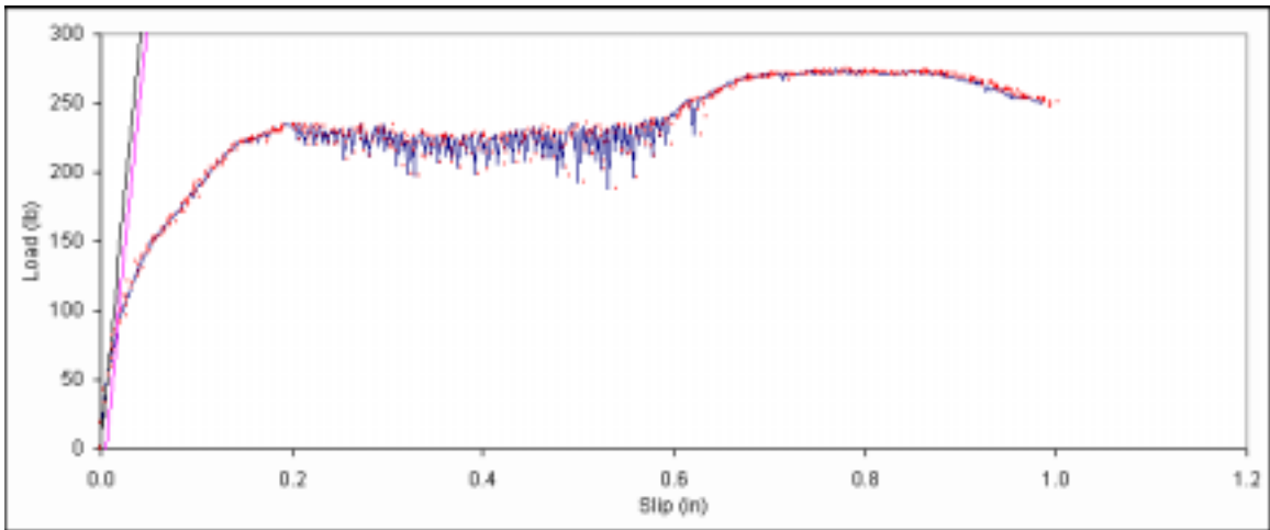
Figure B. 545: Load vs. slip plot for sample F2-12.
