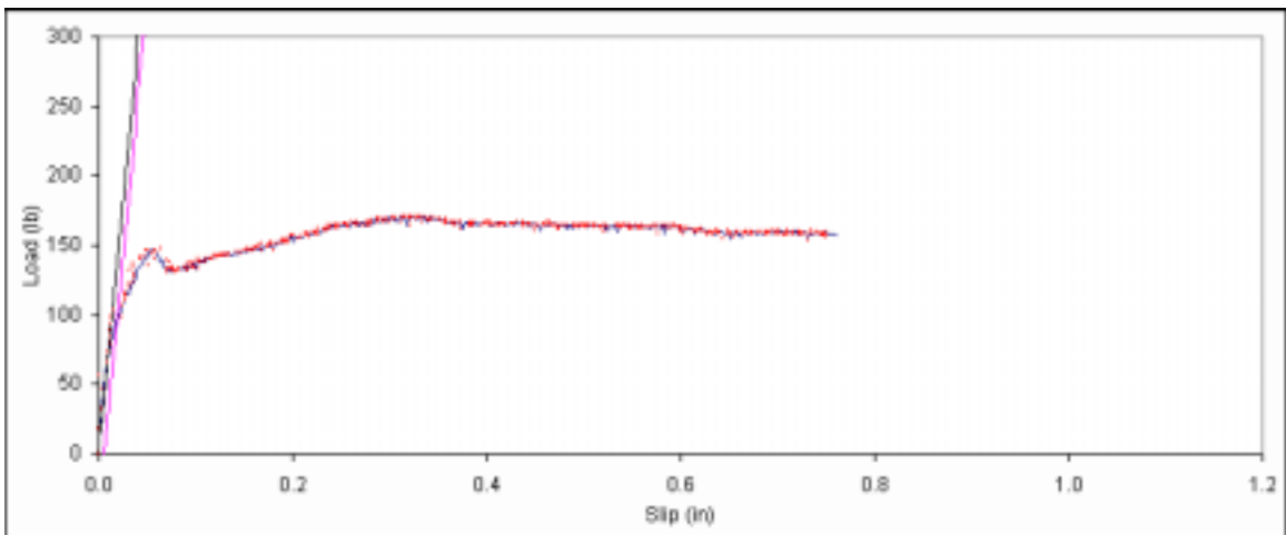
Figure B. 51: Load vs. slip plot for sample A4-7.
