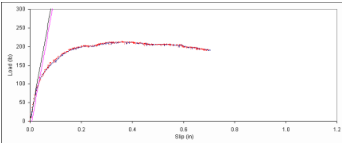
Figure B. 461: Load vs. slip plot for sample E4-1.
