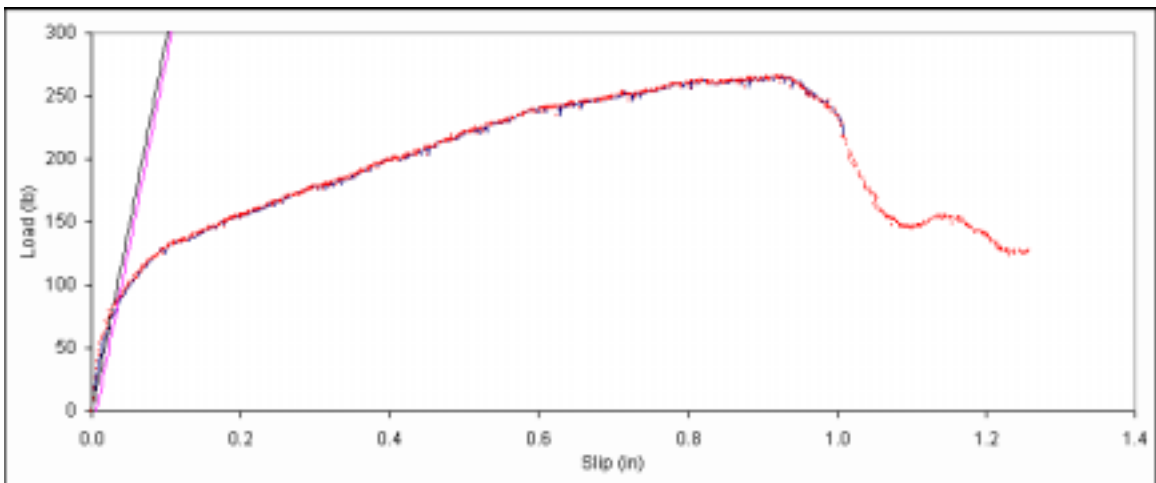
Figure B. 189: Load vs. slip plot for sample B6-12.
