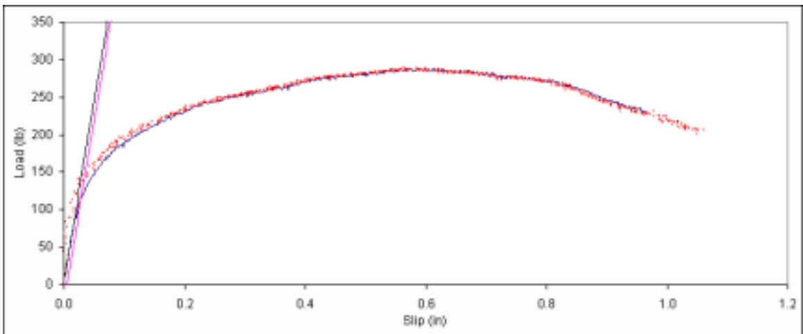
Figure B. 162: Load vs. slip plot for sample B4-15.
