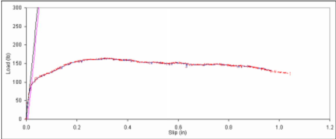
Figure B. 346: Load vs. slip plot for sample D3-6.
