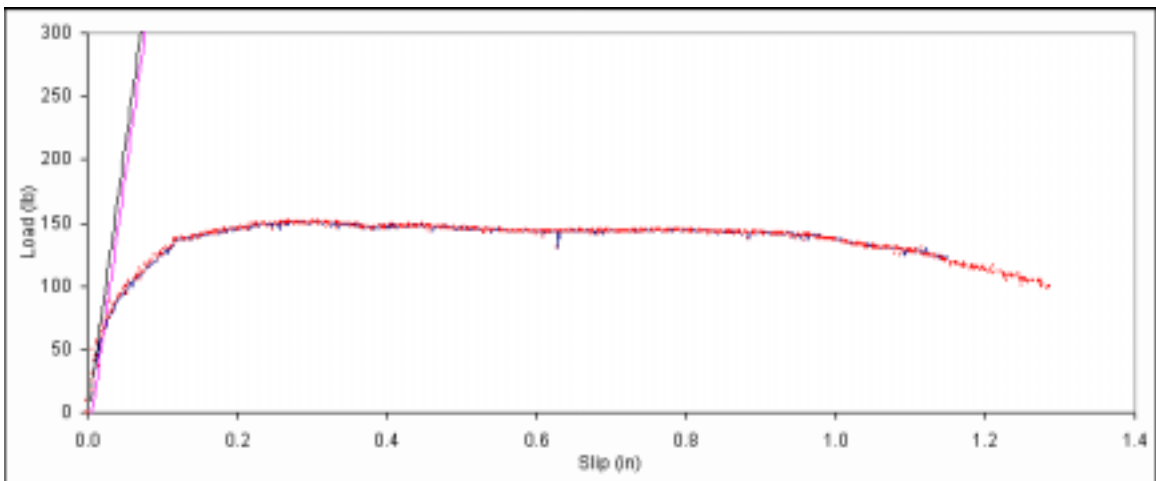
Figure B. 555: Load vs. slip plot for sample F3-8.
