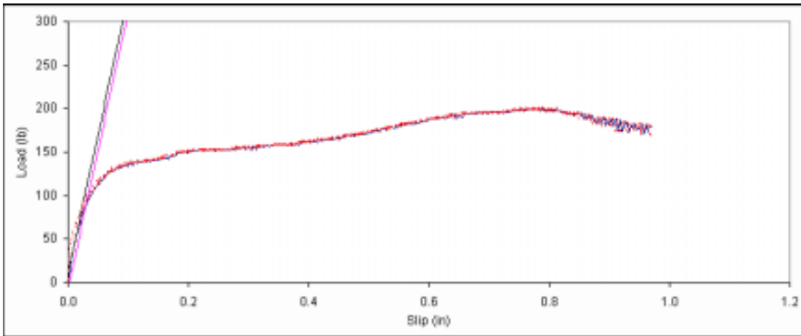
Figure B. 164: Load vs. slip plot for sample B5-2.
