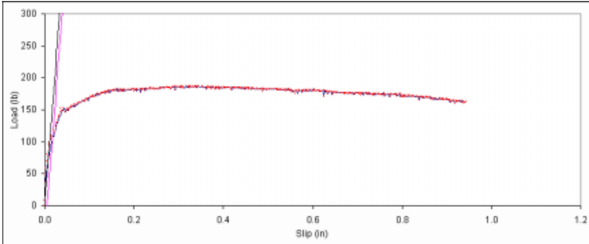
Figure B. 55: Load vs. slip plot for sample A4-11.
