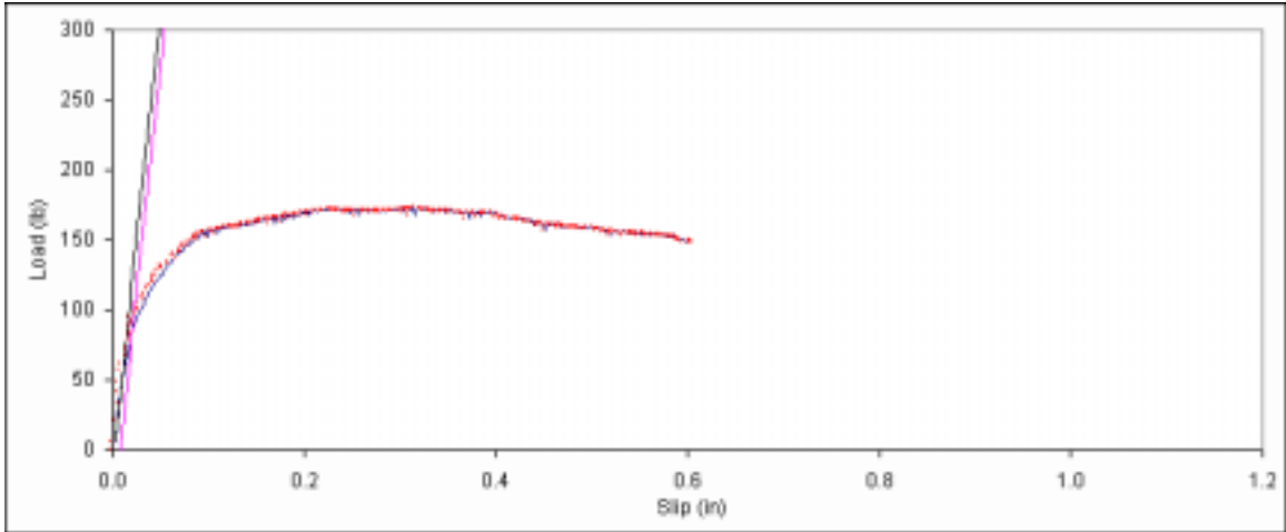
Figure B. 223: Load vs. slip plot for sample C2-1.
