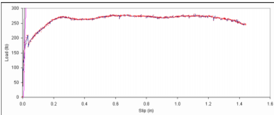
Figure B. 423: Load vs. slip plot for sample E1-8.
