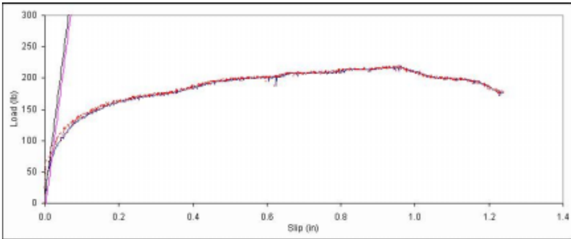
Figure B. 101: Load vs. slip plot for sample A7-13.
