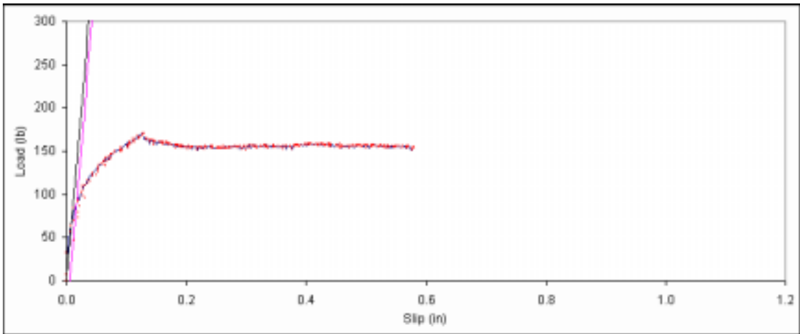
Figure B. 338: Load vs. slip plot for sample D2-13.
