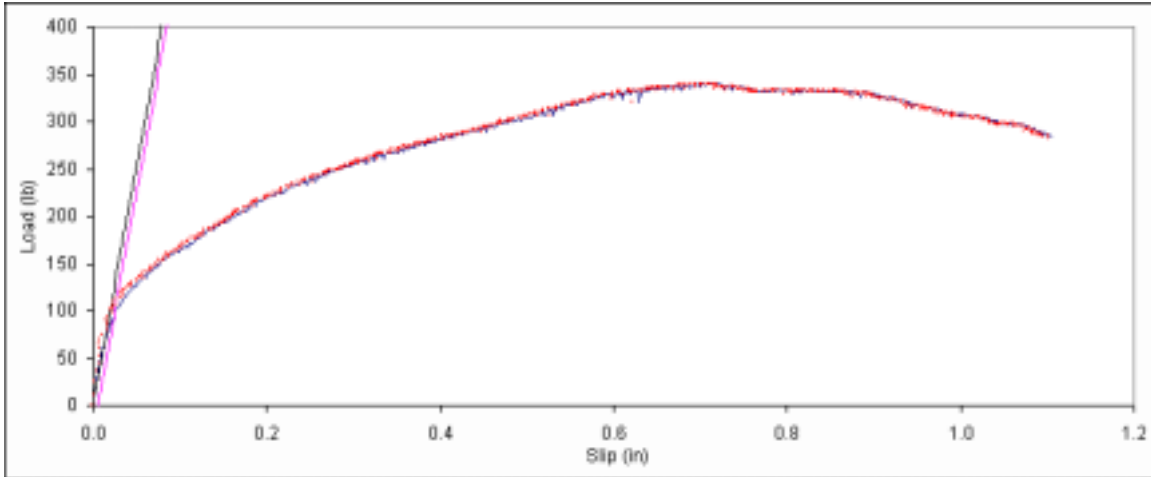
Figure B. 295: Load vs. slip plot for sample C6-14.
