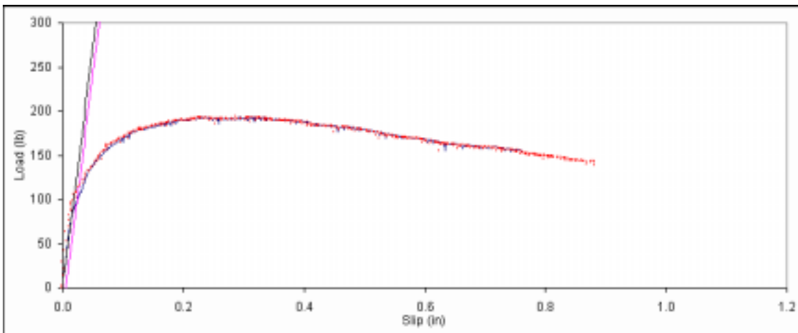
Figure B. 36: Load vs. slip plot for sample A3-7.
