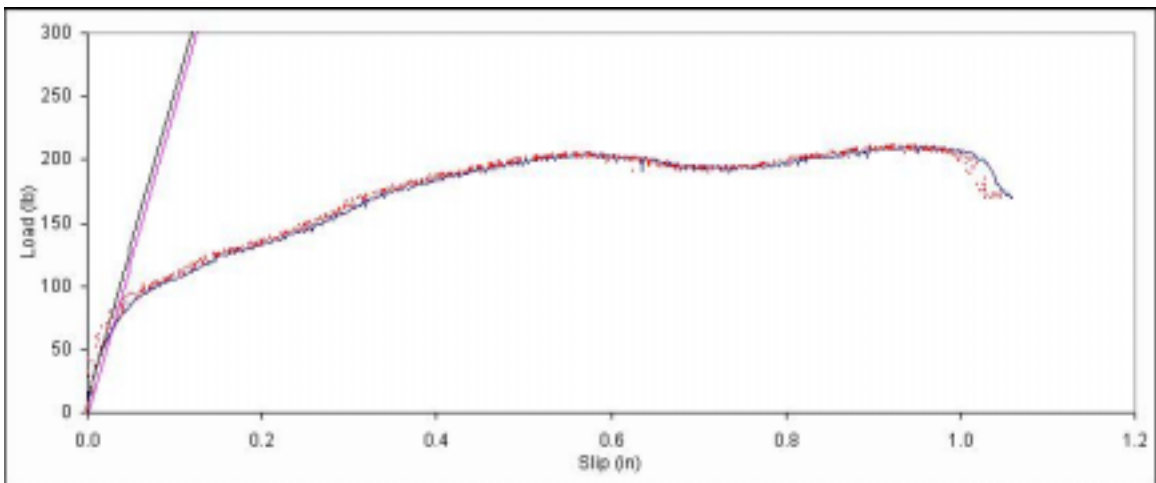
Figure B. 96: Load vs. slip plot for sample A7-8.
