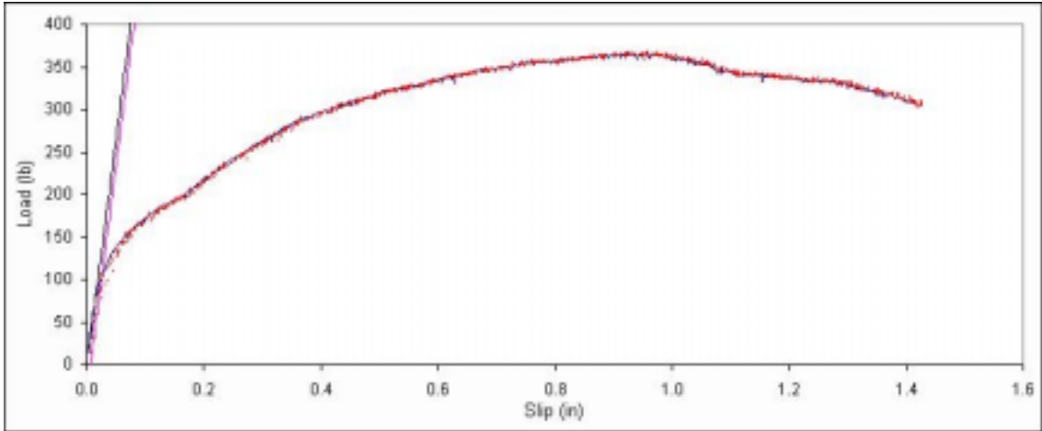
Figure B. 409: Load vs. slip plot for sample D7-9.
