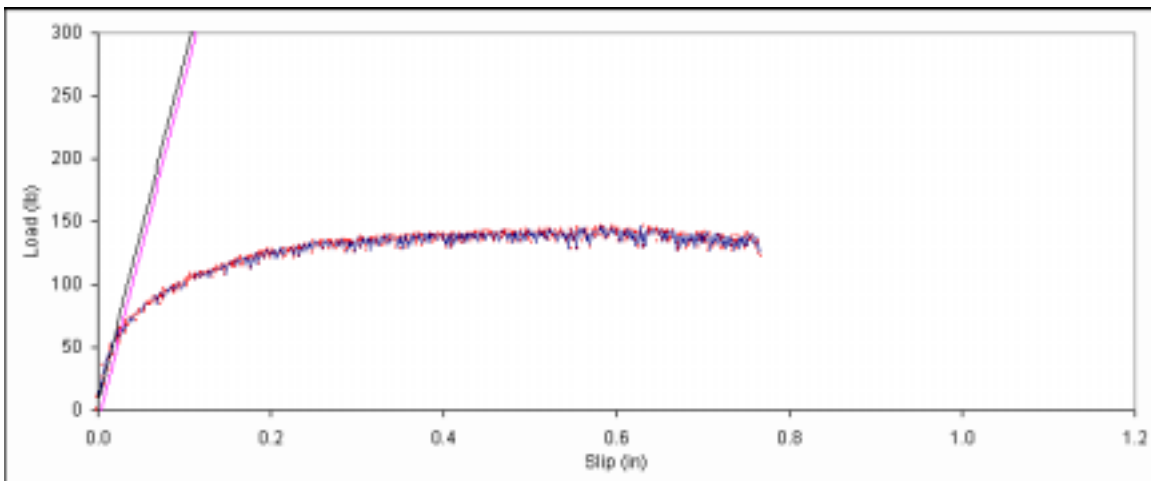
Figure B. 18: Load vs. slip plot for sample A2-4.
