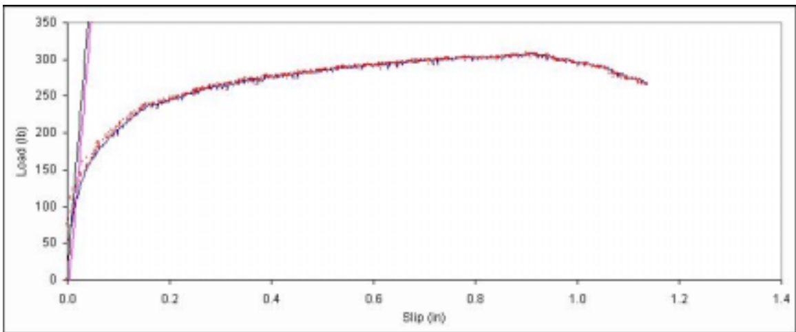
Figure B. 609: Load vs. slip plot for sample F7-2.
