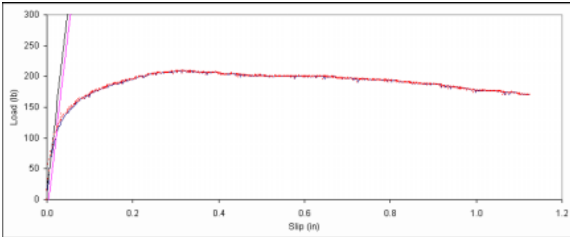
Figure B. 448: Load vs. slip plot for sample E3-3.
