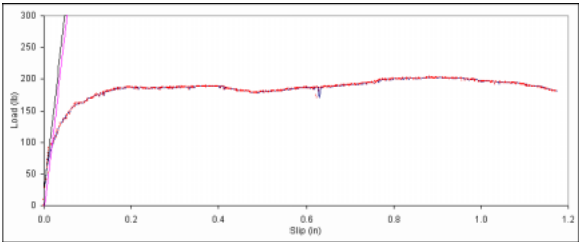
Figure B. 125: Load vs. slip plot for sample B2-8.
