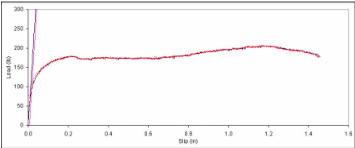
Figure B. 278: Load vs. slip plot for sample C5-12.
