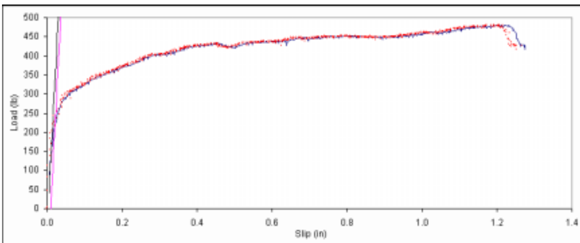
Figure B. 429: Load vs. slip plot for sample E1-14.
