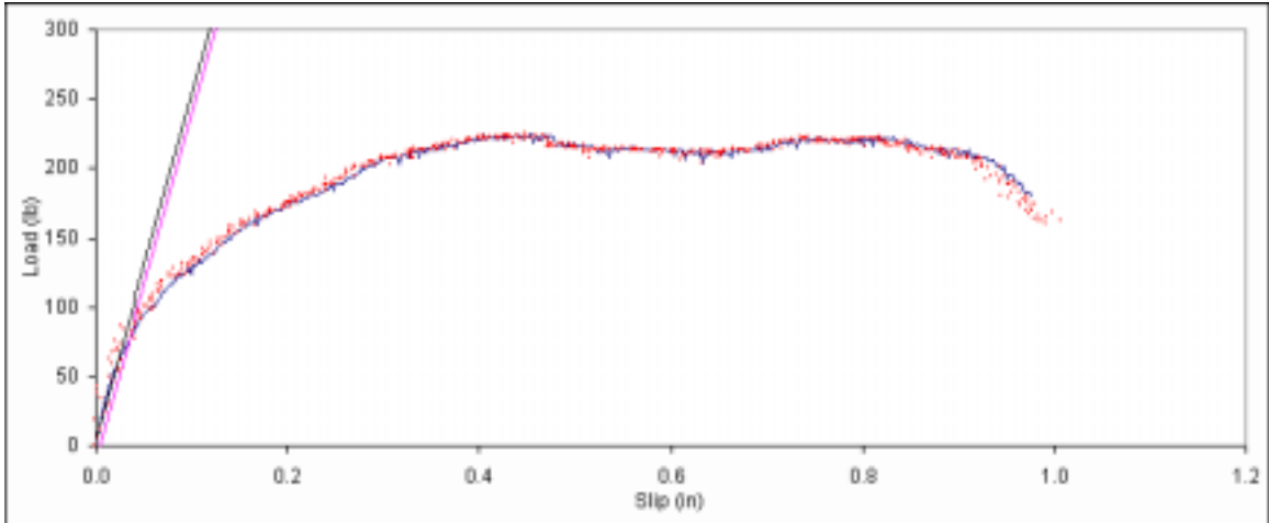
Figure B. 289: Load vs. slip plot for sample C6-8.
