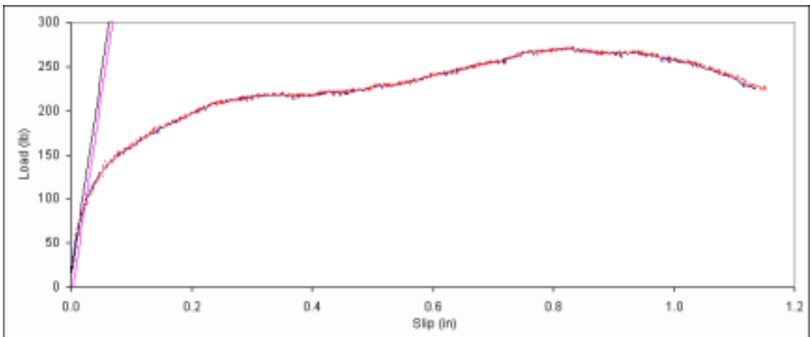
Figure B. 267: Load vs. slip plot for sample C5-1.
