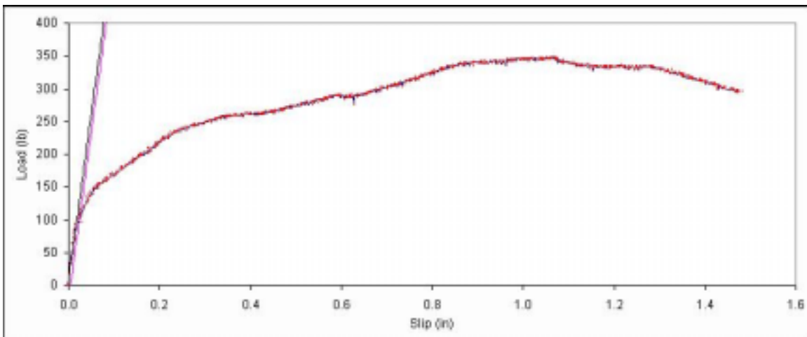
Figure B. 402: Load vs. slip plot for sample D7-2.
