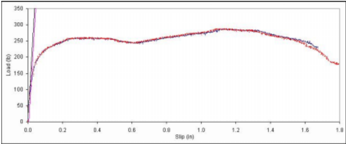
Figure B. 518: Load vs. slip plot for sample E7-14.
