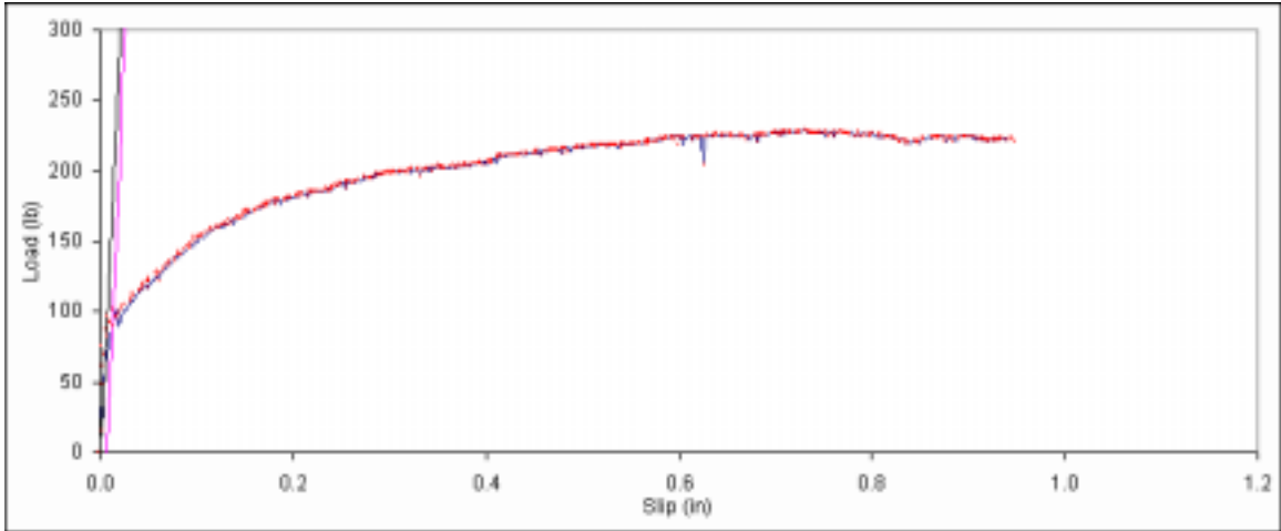
Figure B. 211: Load vs. slip plot for sample C1-4.
