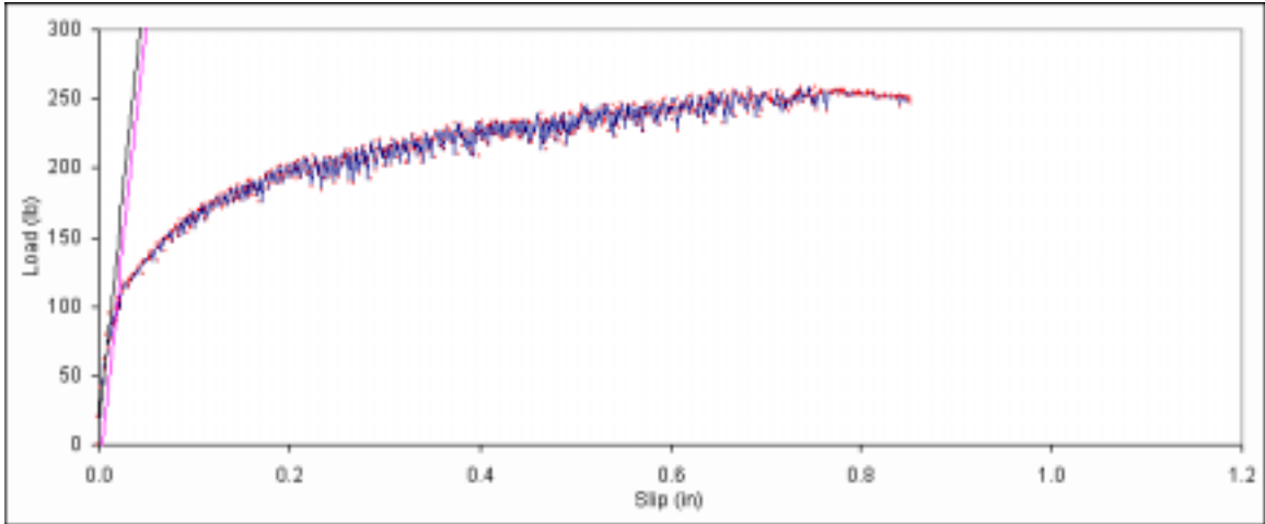
Figure B. 220: Load vs. slip plot for sample C1-13.
