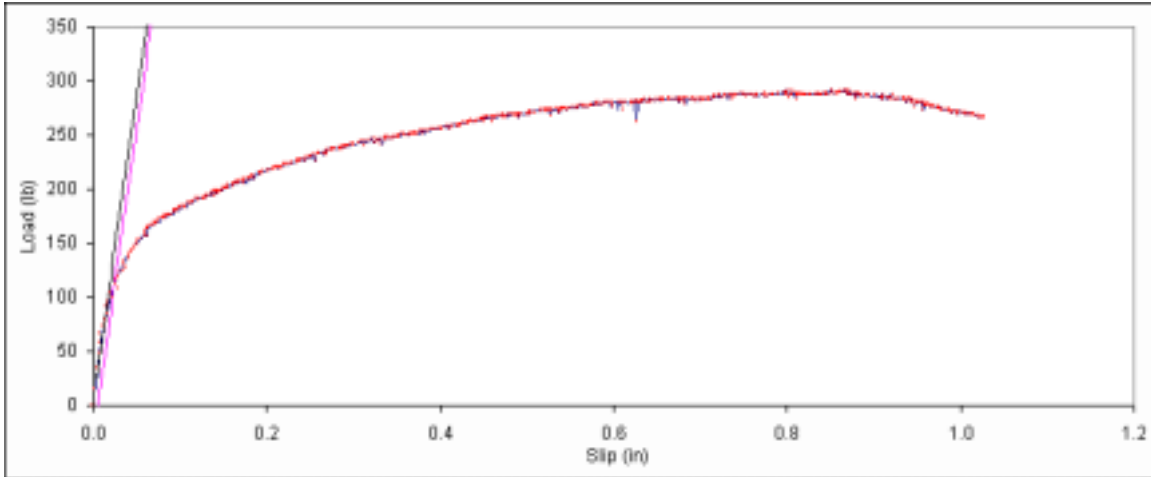
Figure B. 58: Load vs. slip plot for sample A4-14.
