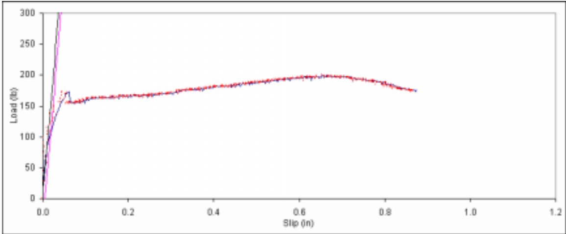
Figure B. 49: Load vs. slip plot for sample A4-5.
