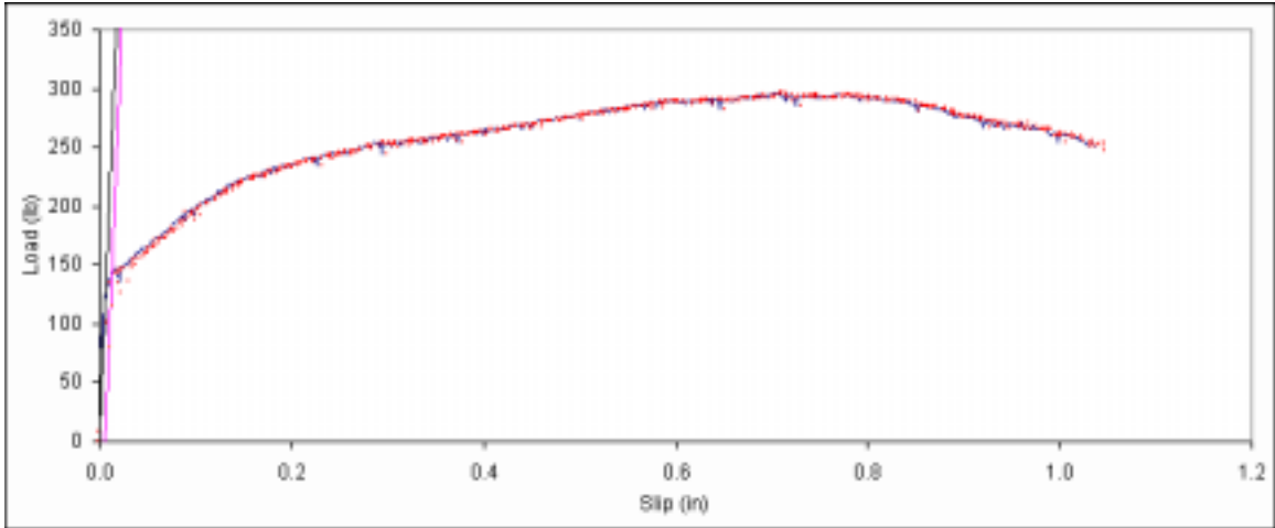
Figure B. 526: Load vs. slip plot for sample F1-7.
