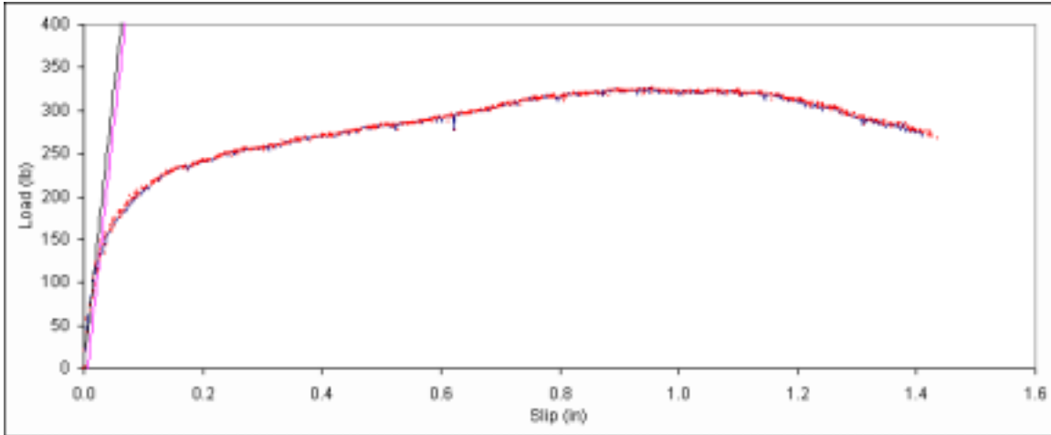
Figure B. 460: Load vs. slip plot for sample E3-15.
