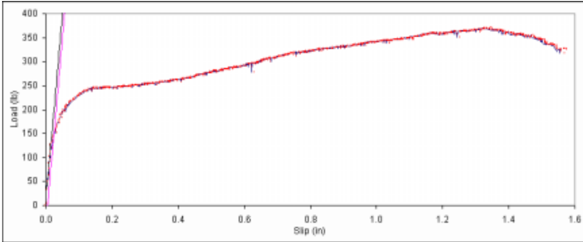
Figure B. 502: Load vs. slip plot for sample E6-13.
