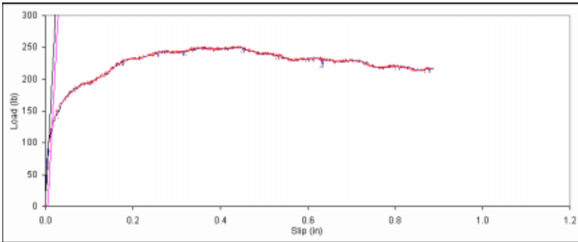
Figure B. 344: Load vs. slip plot for sample D3-4.
