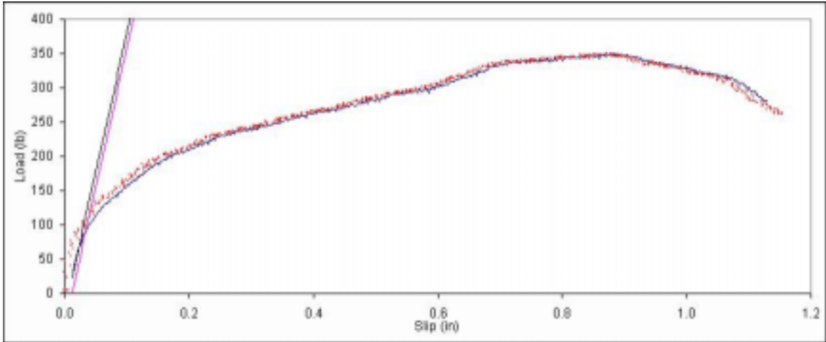
Figure B. 406: Load vs. slip plot for sample D7-6.
