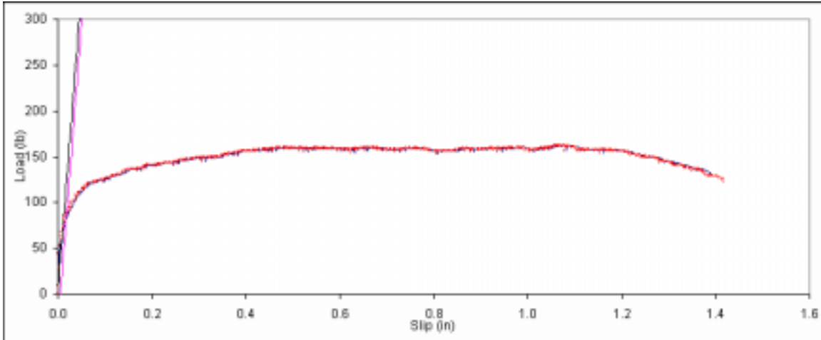
Figure B. 34: Load vs. slip plot for sample A3-5.
