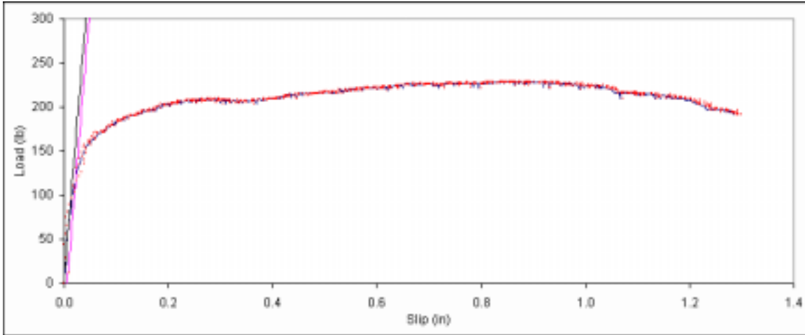
Figure B. 472: Load vs. slip plot for sample E4-12.
