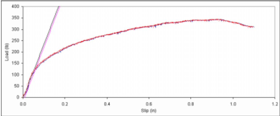
Figure B. 388: Load vs. slip plot for sample D6-3.
