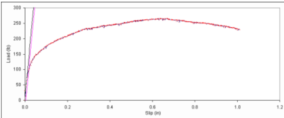
Figure B. 45: Load vs. slip plot for sample A4-1.
