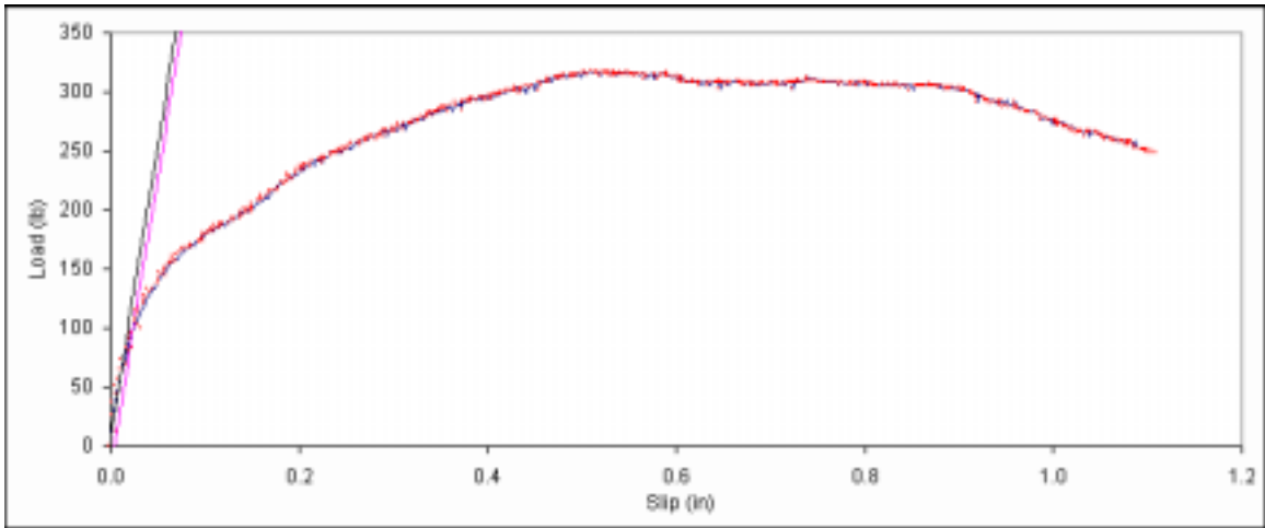
Figure B. 371: Load vs. slip plot for sample D5-1.
