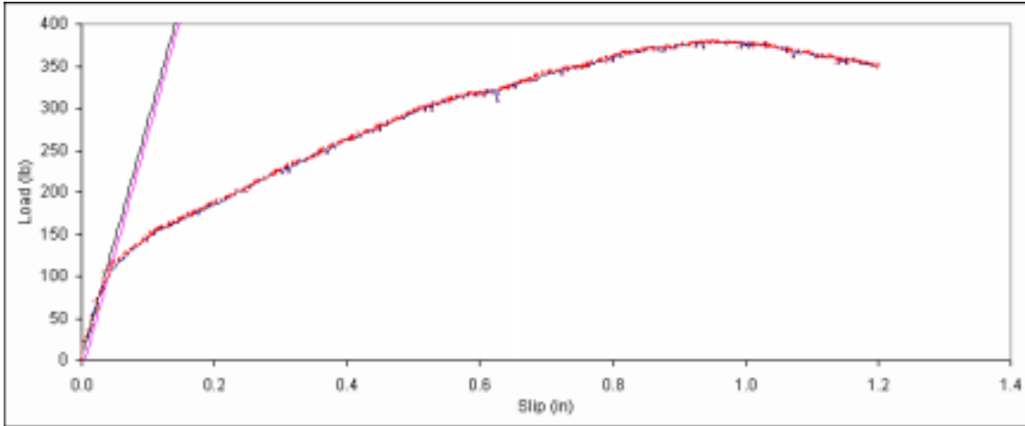
Figure B. 592: Load vs. slip plot for sample F5-15.
