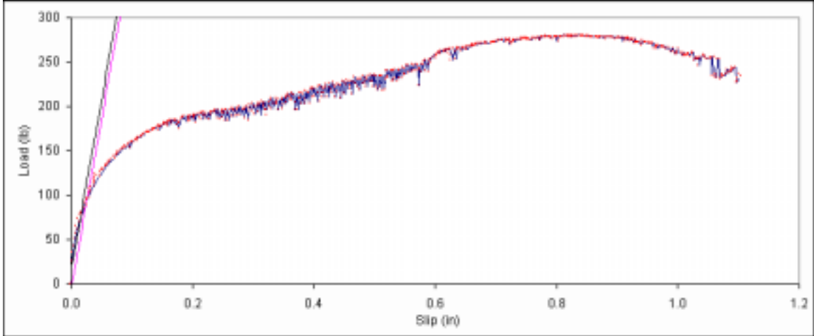
Figure B. 238: Load vs. slip plot for sample C3-1.
