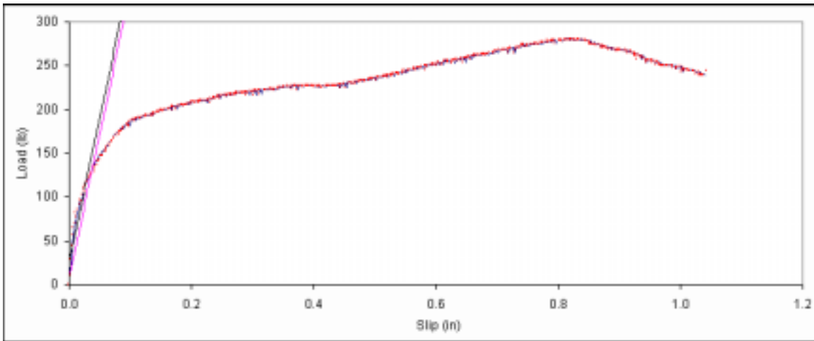
Figure B. 356: Load vs. slip plot for sample D4-1.
