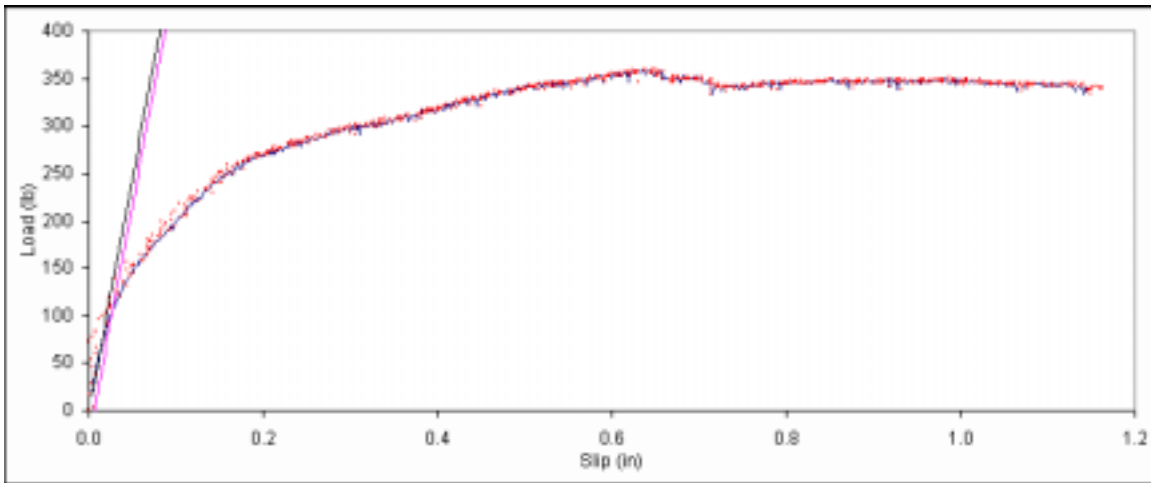
Figure B. 602: Load vs. slip plot for sample F6-10.
