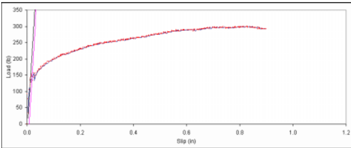
Figure B. 524: Load vs. slip plot for sample F1-5.
