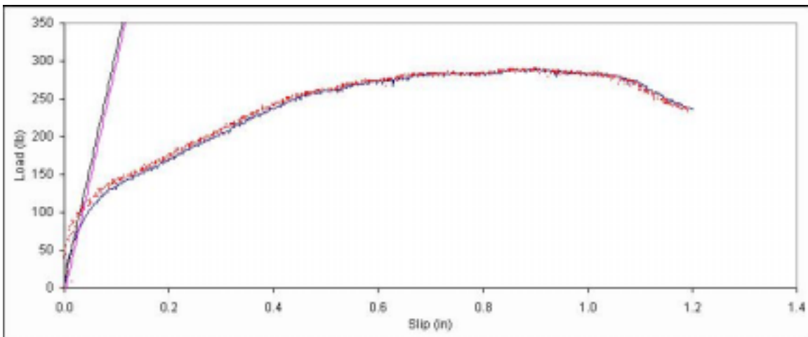
Figure B. 102: Load vs. slip plot for sample A7-15.
