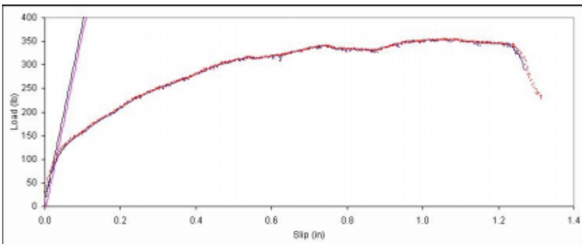
Figure B. 612: Load vs. slip plot for sample F7-5.
