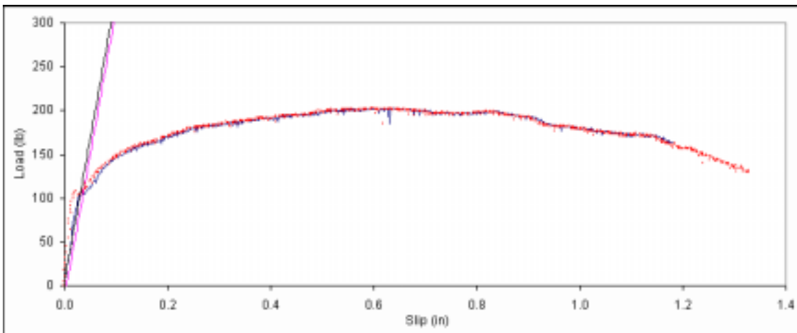
Figure B. 576: Load vs. slip plot for sample F4-14.
