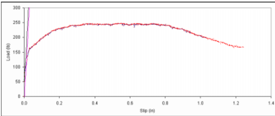
Figure B. 218: Load vs. slip plot for sample C1-11.
