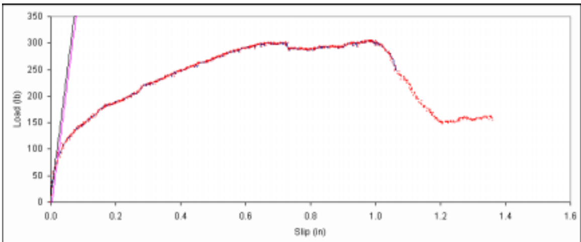
Figure B. 381: Load vs. slip plot for sample D5-11.
