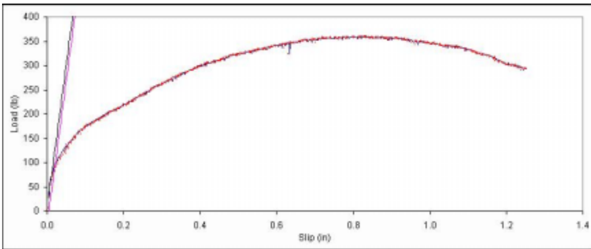
Figure B. 308: Load vs. slip plot for sample C7-12.
