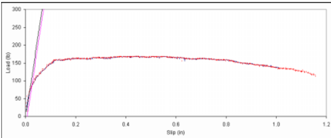
Figure B. 330: Load vs. slip plot for sample D2-5.
