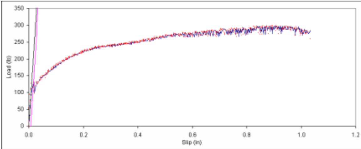
Figure B. 430: Load vs. slip plot for sample E1-15.
