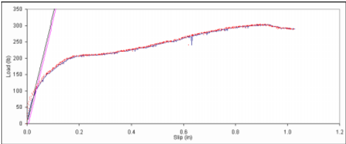
Figure B. 287: Load vs. slip plot for sample C6-6.
