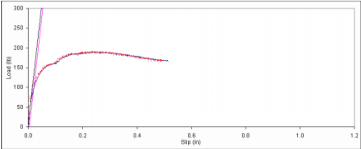
Figure B. 166: Load vs. slip plot for sample B5-4.
