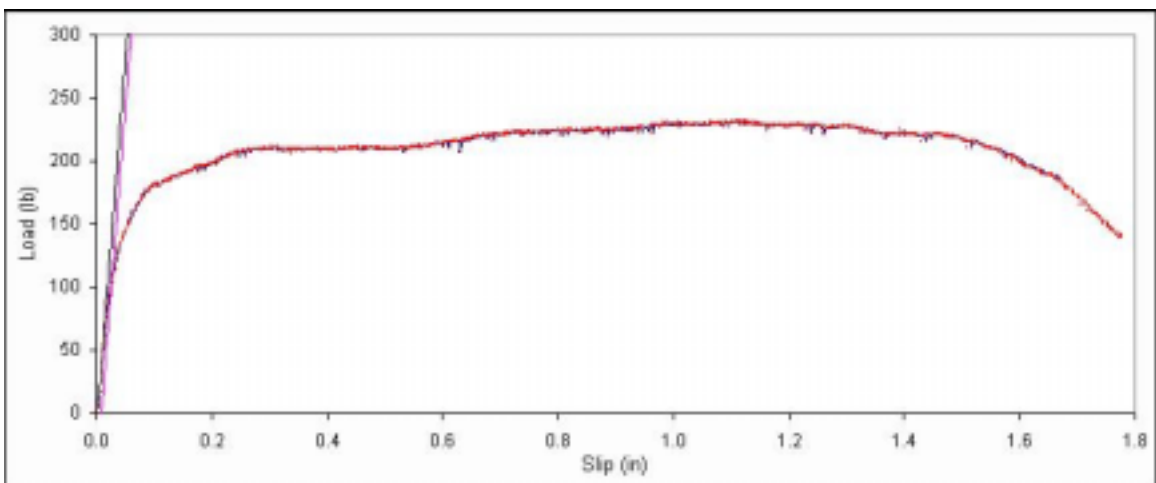
Figure B. 513: Load vs. slip plot for sample E7-9.
