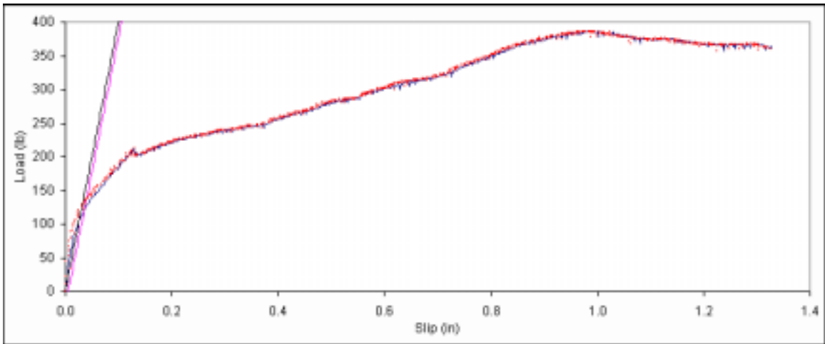
Figure B. 281: Load vs. slip plot for sample C5-15.
