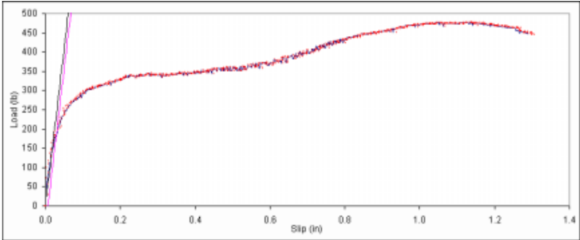
Figure B. 436: Load vs. slip plot for sample E2-6.
