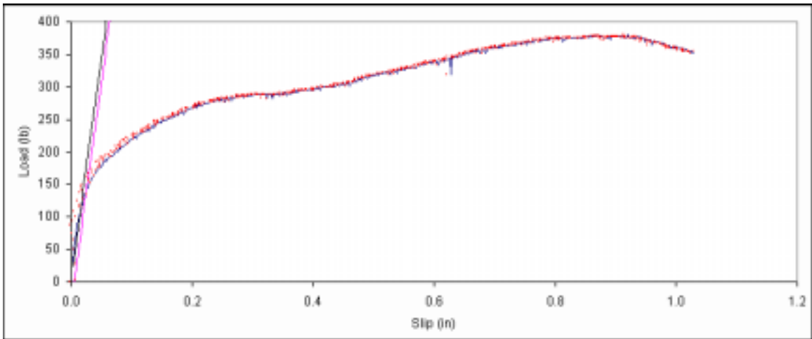
Figure B. 11: Load vs. slip plot for sample A1-11.
