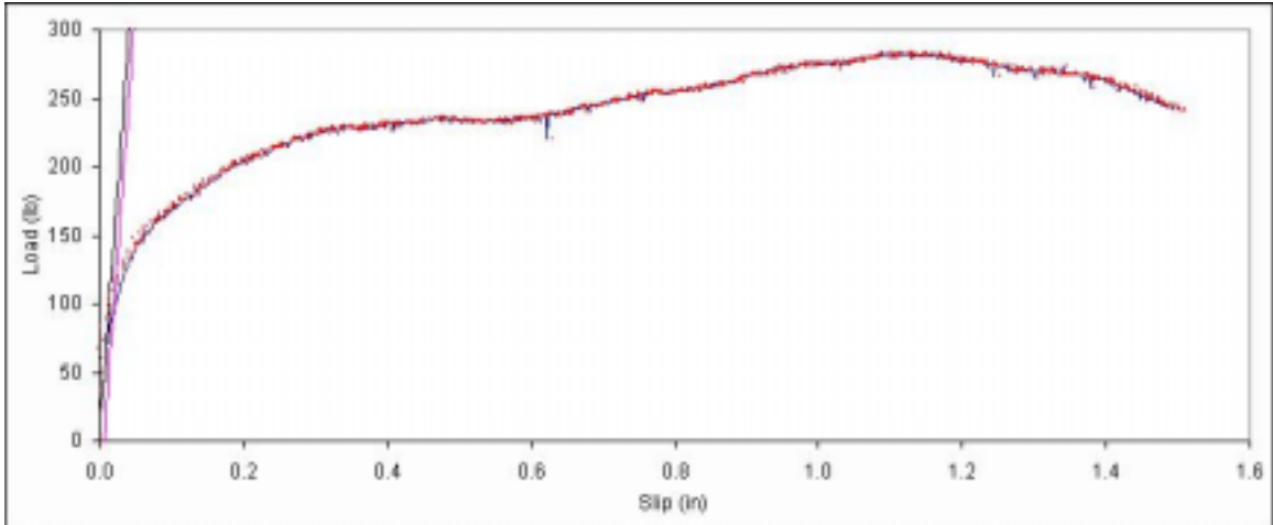
Figure B. 511: Load vs. slip plot for sample E7-7.
