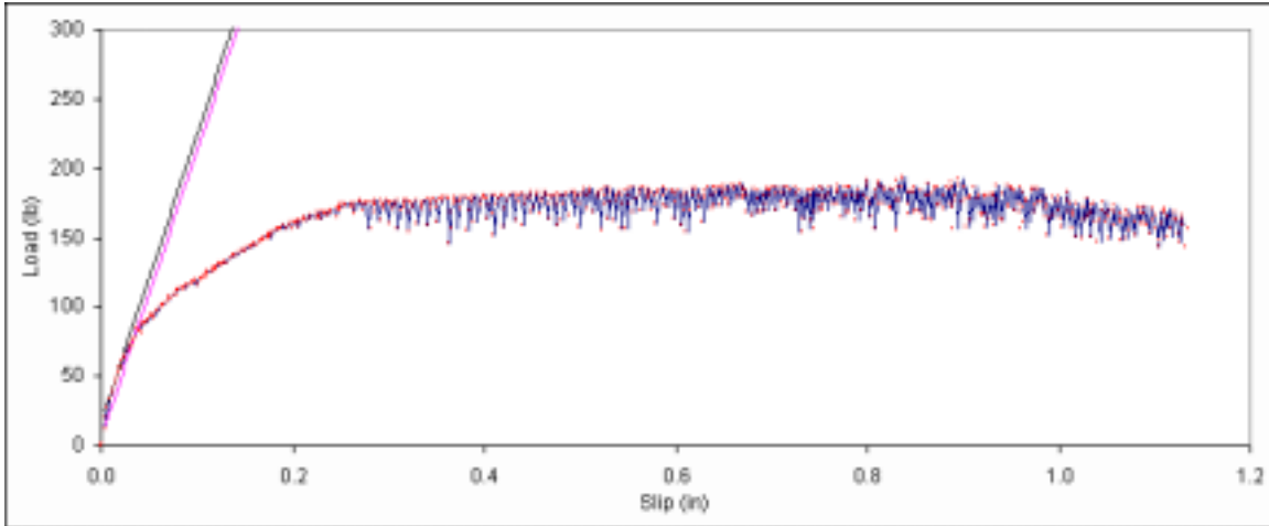
Figure B. 28: Load vs. slip plot for sample A2-14.
