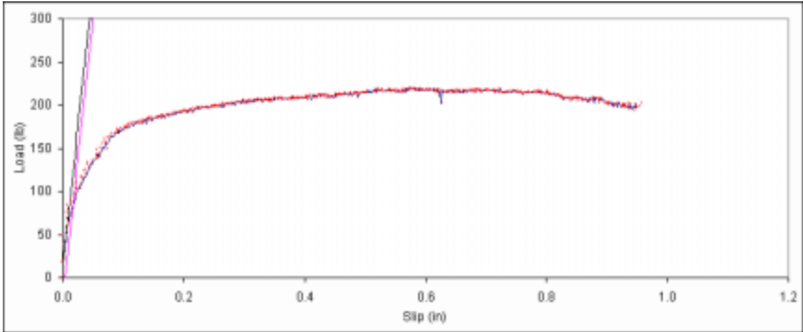
Figure B. 214: Load vs. slip plot for sample C1-7.
