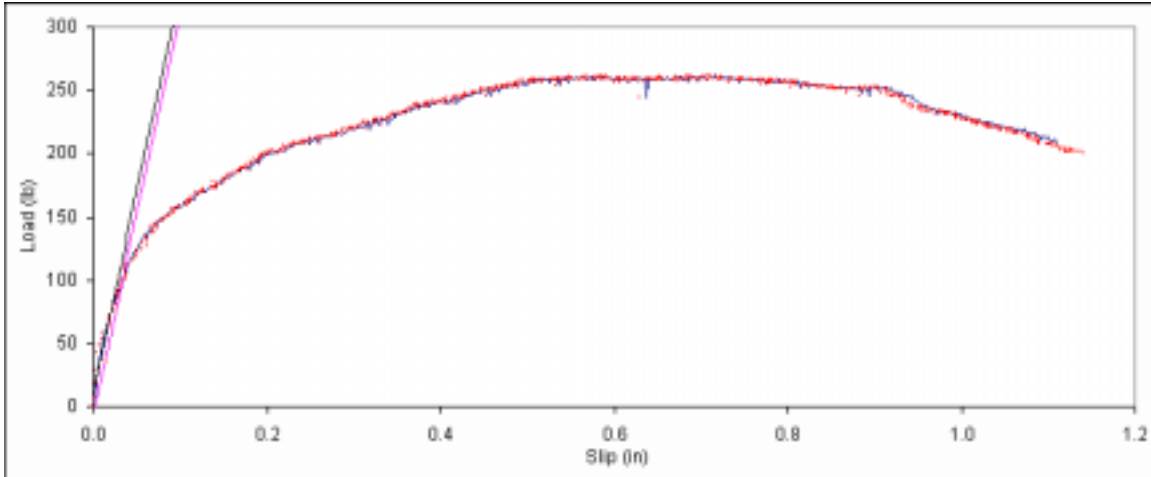
Figure B. 73: Load vs. slip plot for sample A5-14.
