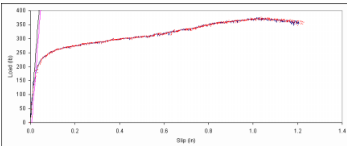
Figure B. 441: Load vs. slip plot for sample E2-11.
