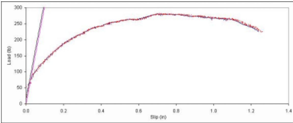
Figure B. 401: Load vs. slip plot for sample D7-1.
