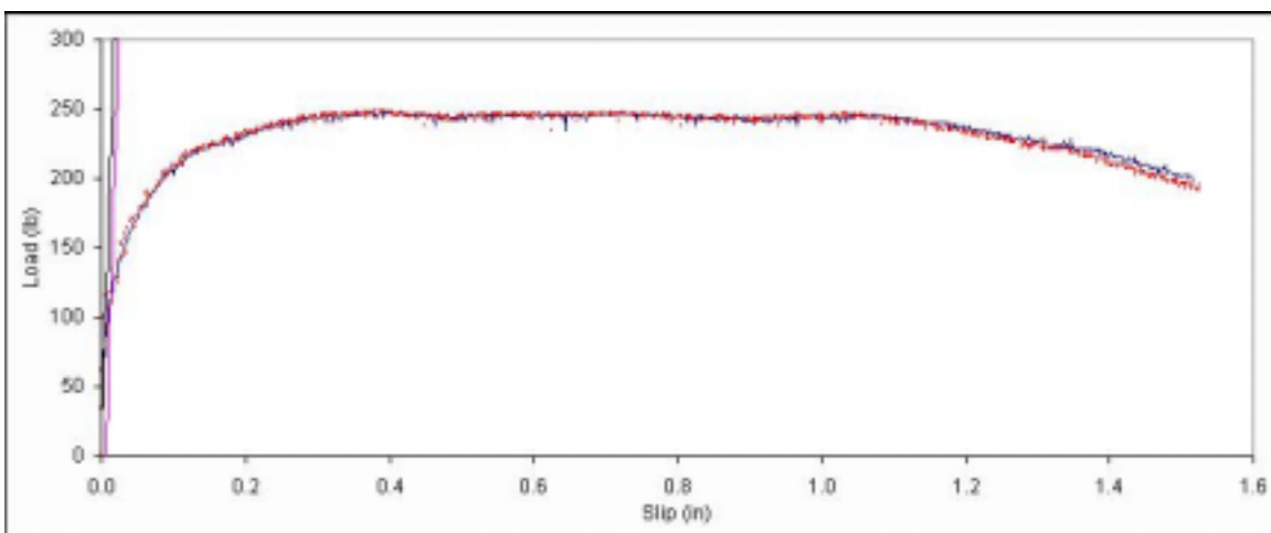
Figure B. 516: Load vs. slip plot for sample E7-12.
