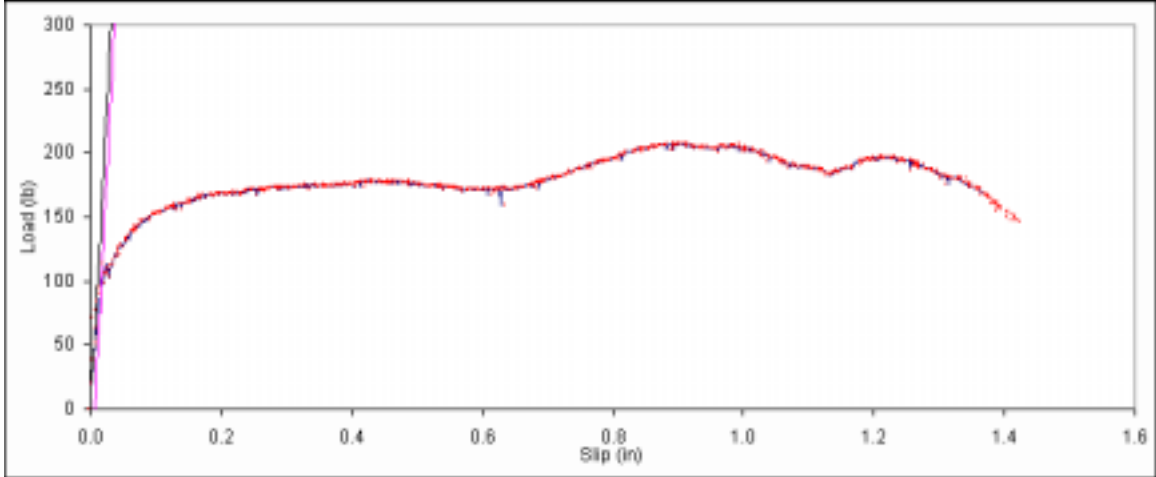
Figure B. 553: Load vs. slip plot for sample F3-6.
