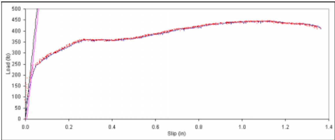
Figure B. 497: Load vs. slip plot for sample E6-8.
