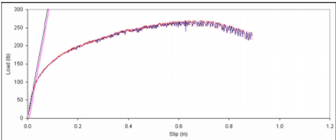
Figure B. 240: Load vs. slip plot for sample C3-3.
