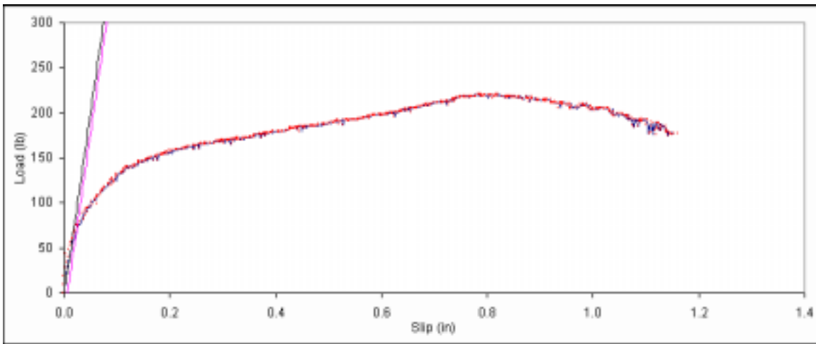
Figure B. 551: Load vs. slip plot for sample F3-4.
