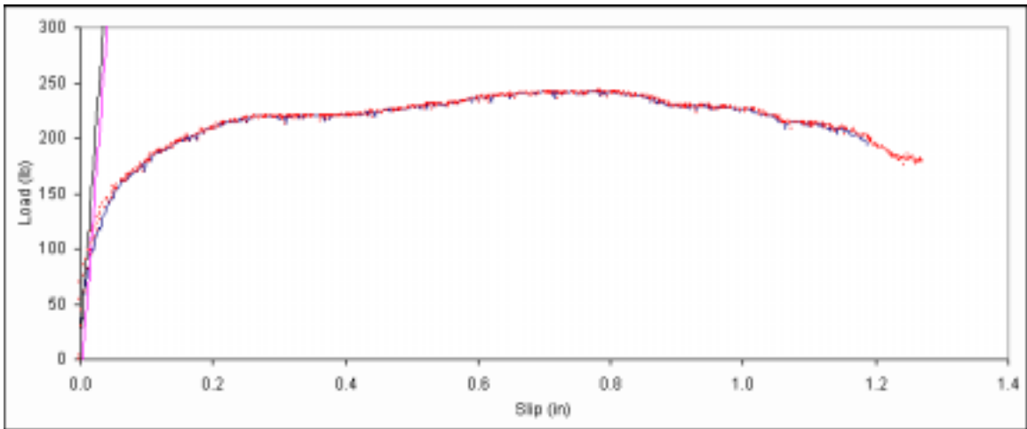
Figure B. 554: Load vs. slip plot for sample F3-7.
