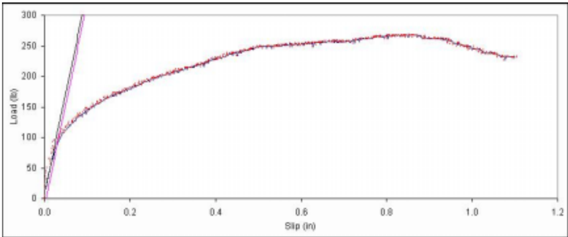
Figure B. 614: Load vs. slip plot for sample F7-7.
