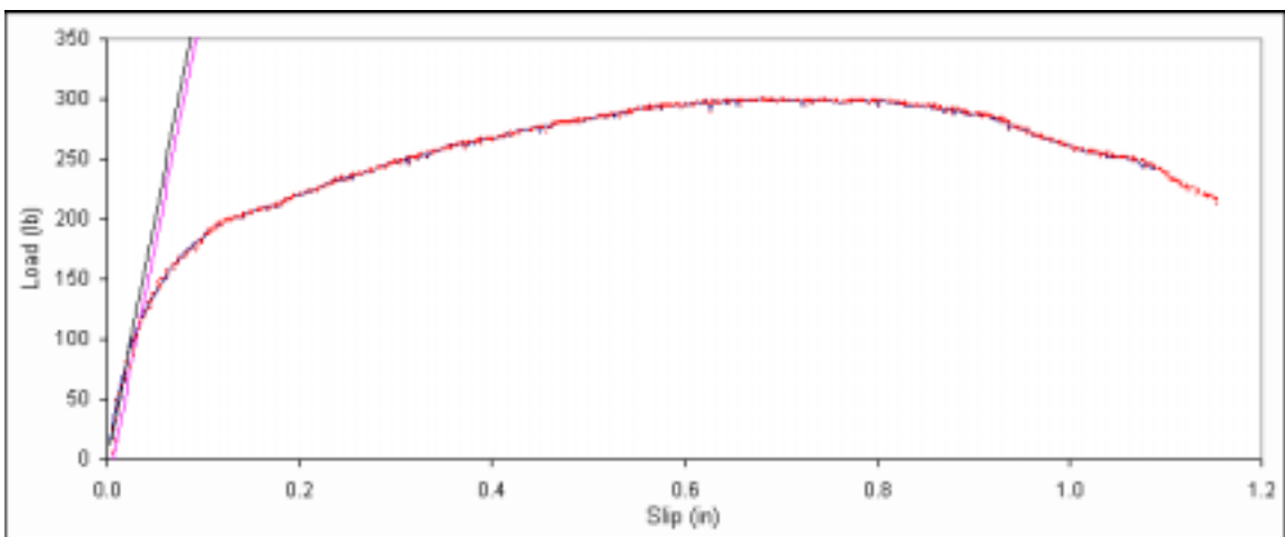
Figure B. 186: Load vs. slip plot for sample B6-9.
