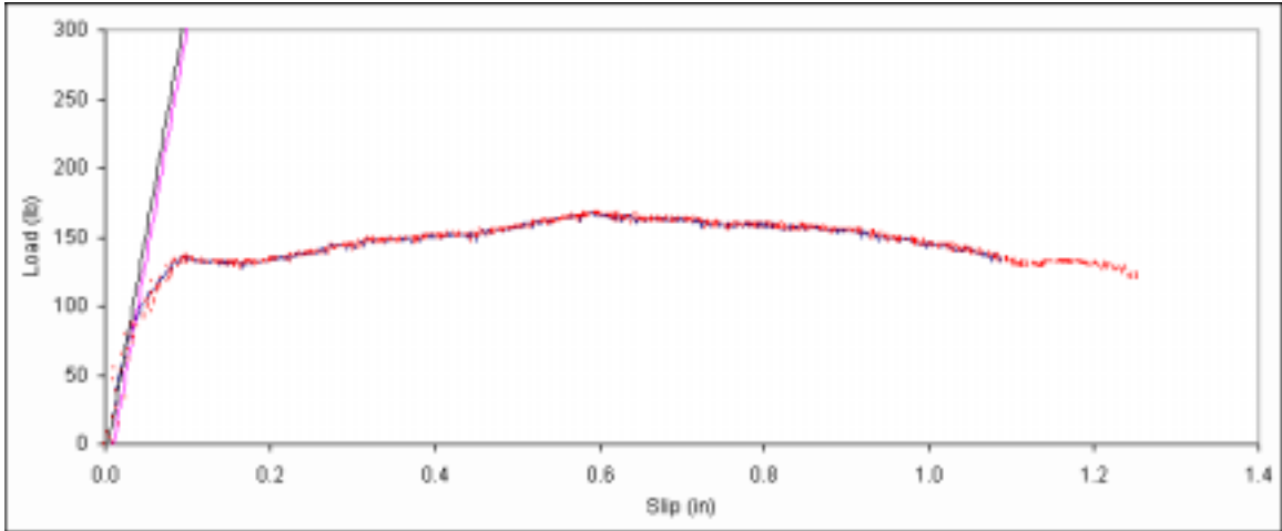
Figure B. 52: Load vs. slip plot for sample A4-8.
