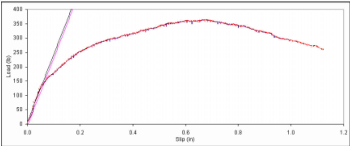
Figure B. 590: Load vs. slip plot for sample F5-13.
