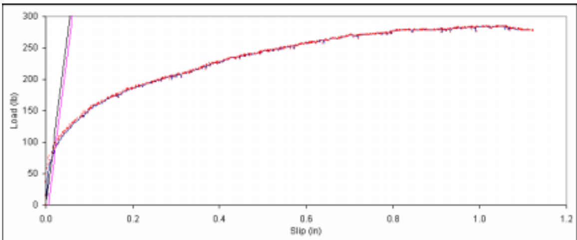
Figure B. 222: Load vs. slip plot for sample C1-15.
