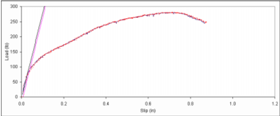
Figure B. 271: Load vs. slip plot for sample C5-5.
