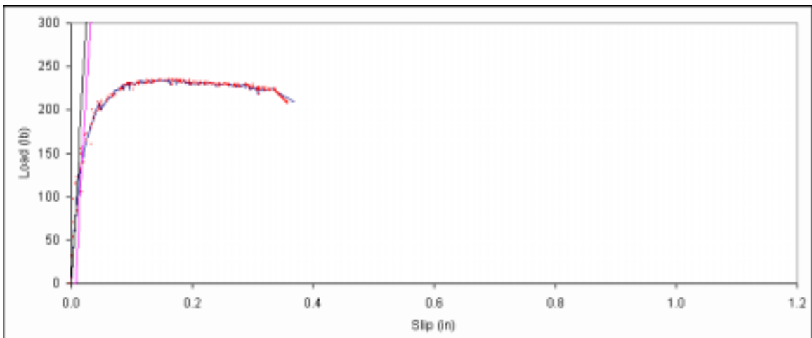
Figure B. 426: Load vs. slip plot for sample E1-11.
