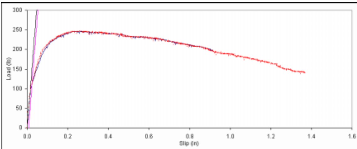
Figure B. 468: Load vs. slip plot for sample E4-8.
