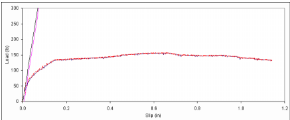
Figure B. 540: Load vs. slip plot for sample F2-7.
