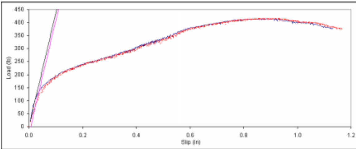
Figure B. 503: Load vs. slip plot for sample E6-14.
