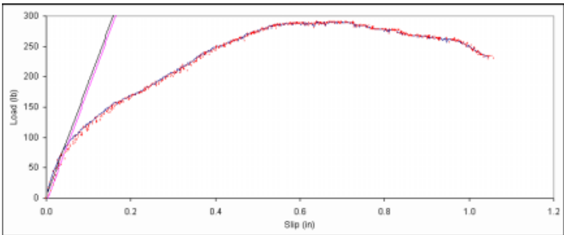
Figure B. 180: Load vs. slip plot for sample B6-3.
