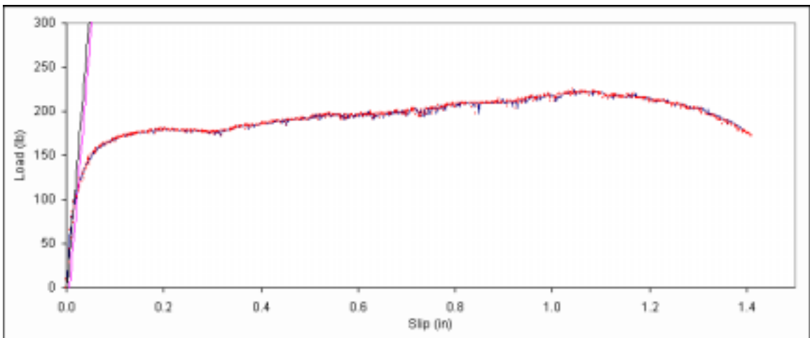
Figure B. 21: Load vs. slip plot for sample A2-7.
