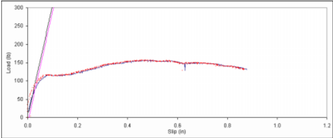
Figure B. 337: Load vs. slip plot for sample D2-12.
