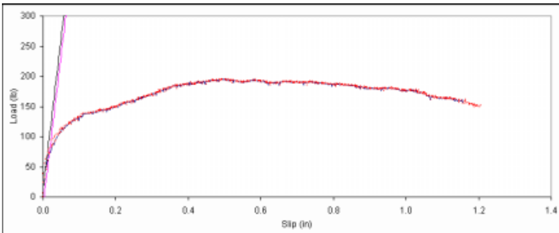
Figure B. 345: Load vs. slip plot for sample D3-5.
