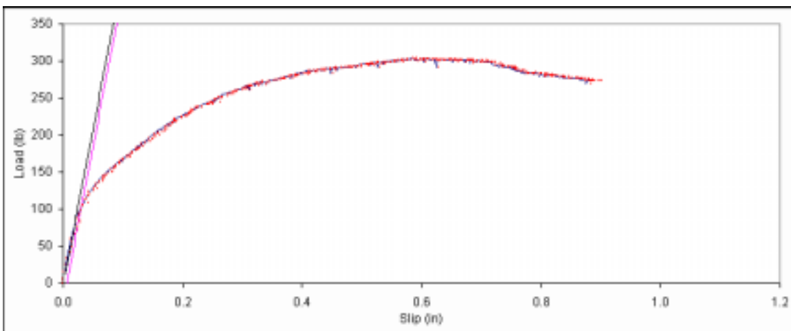
Figure B. 192: Load vs. slip plot for sample B6-15.
