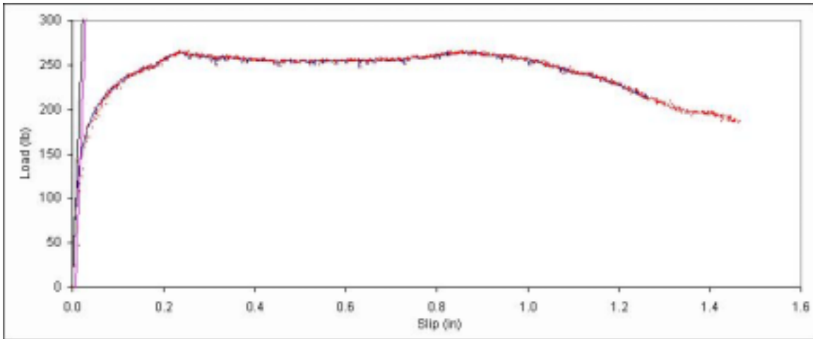
Figure B. 505: Load vs. slip plot for sample E7-1.
