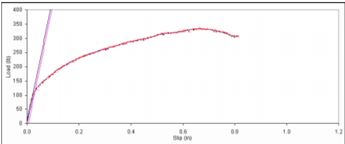
Figure B. 270: Load vs. slip plot for sample C5-4.
