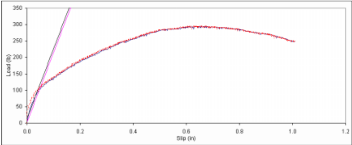
Figure B. 172: Load vs. slip plot for sample B5-10.
