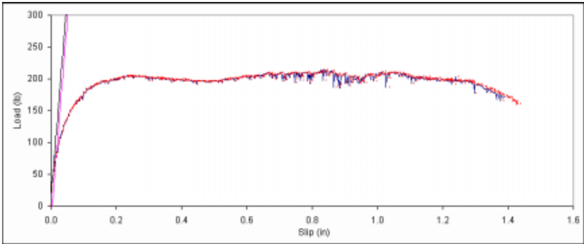
Figure B. 548: Load vs. slip plot for sample F3-1.
