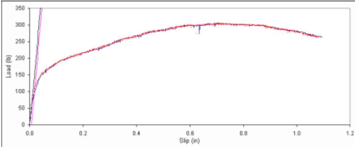
Figure B. 571: Load vs. slip plot for sample F4-9.
