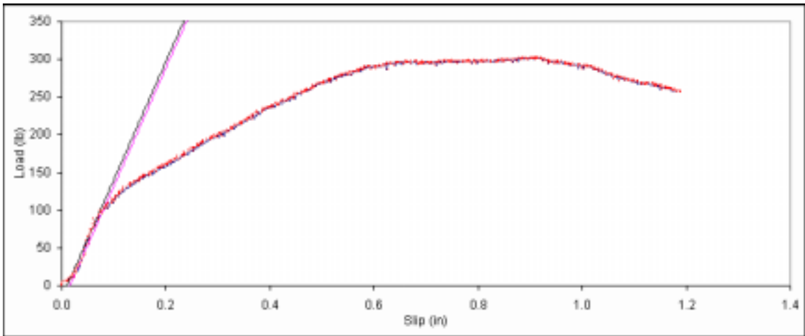
Figure B. 380: Load vs. slip plot for sample D5-10.
