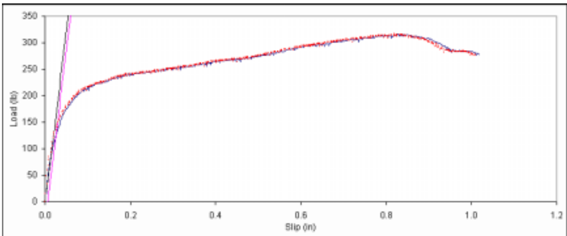
Figure B. 174: Load vs. slip plot for sample B5-12.
