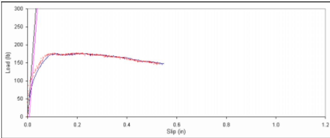
Figure B. 542: Load vs. slip plot for sample F2-9.
