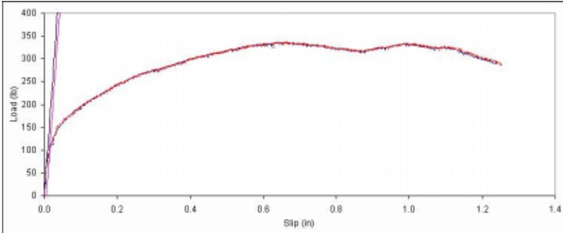
Figure B. 199: Load vs. slip plot for sample B7-7.
