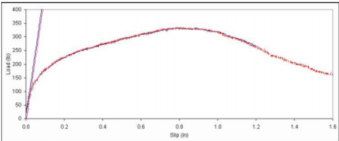
Figure B. 405: Load vs. slip plot for sample D7-5.
