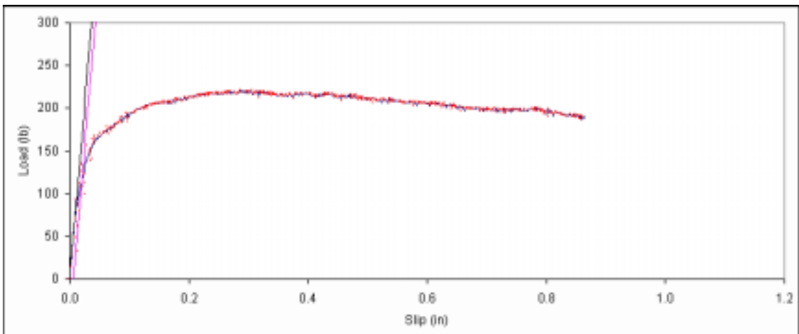
Figure B. 471: Load vs. slip plot for sample E4-11.
