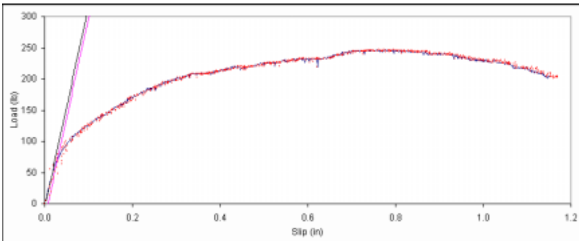
Figure B. 597: Load vs. slip plot for sample F6-5.
