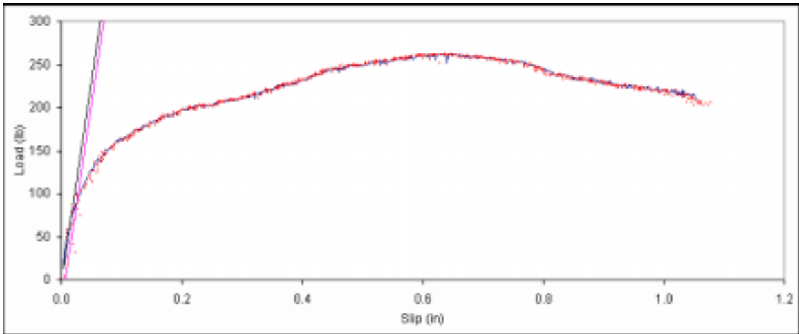
Figure B. 182: Load vs. slip plot for sample B6-5.
