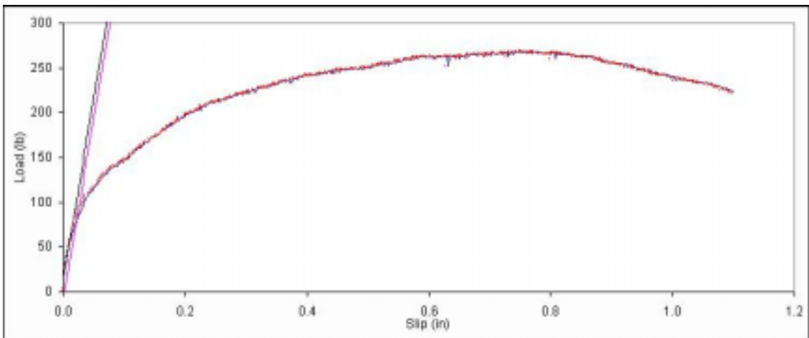
Figure B. 198: Load vs. slip plot for sample B7-6.
