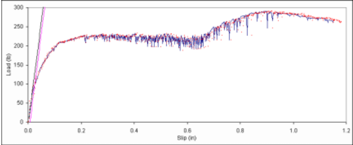
Figure B. 547: Load vs. slip plot for sample F2-15.
