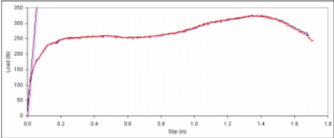
Figure B. 478: Load vs. slip plot for sample E5-3.
