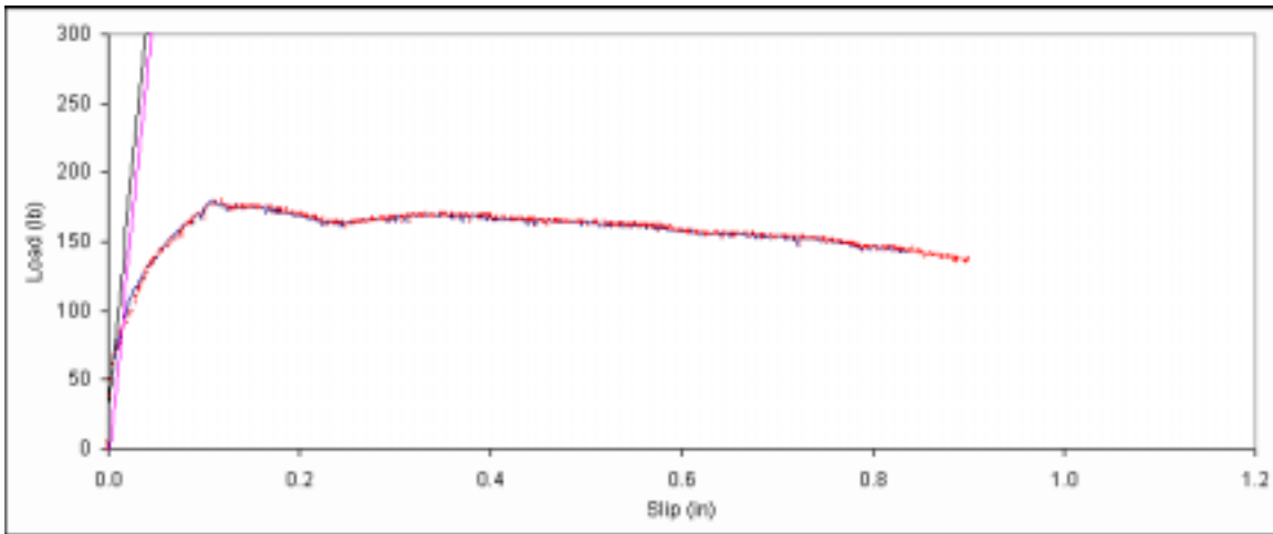
Figure B. 149: Load vs. slip plot for sample B4-2.
