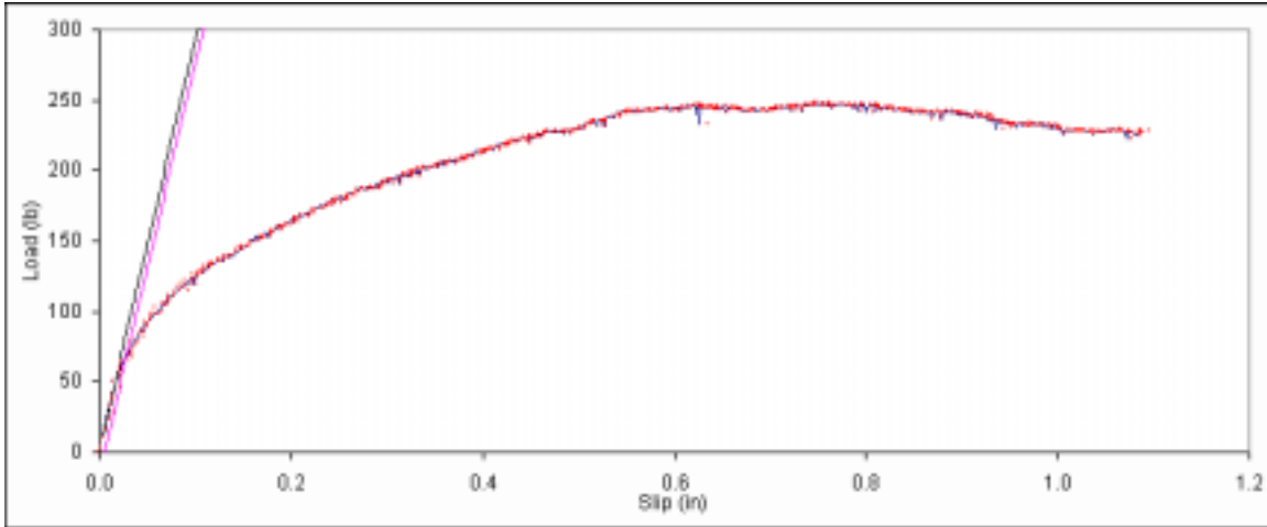
Figure B. 583: Load vs. slip plot for sample F5-6.
