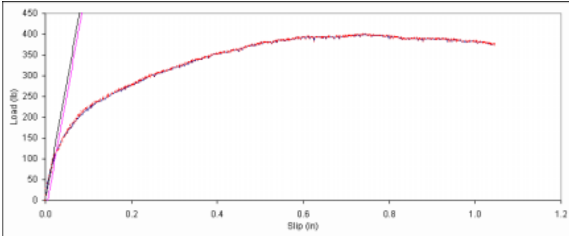
Figure B. 397: Load vs. slip plot for sample D6-12.
