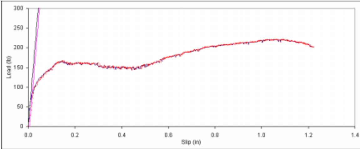
Figure B. 235: Load vs. slip plot for sample C2-13.
