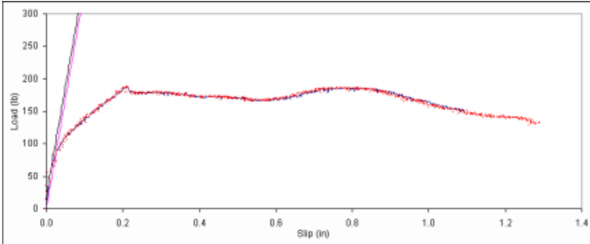
Figure B. 151: Load vs. slip plot for sample B4-4.
