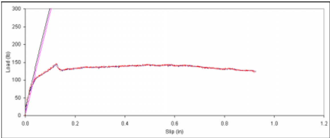
Figure B. 122: Load vs. slip plot for sample B2-5.
