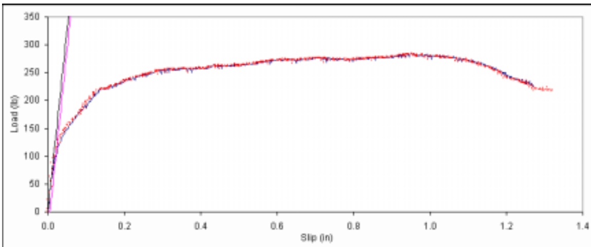
Figure B. 384: Load vs. slip plot for sample D5-14.
