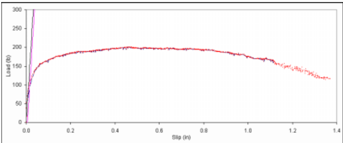
Figure B. 261: Load vs. slip plot for sample C4-10.
