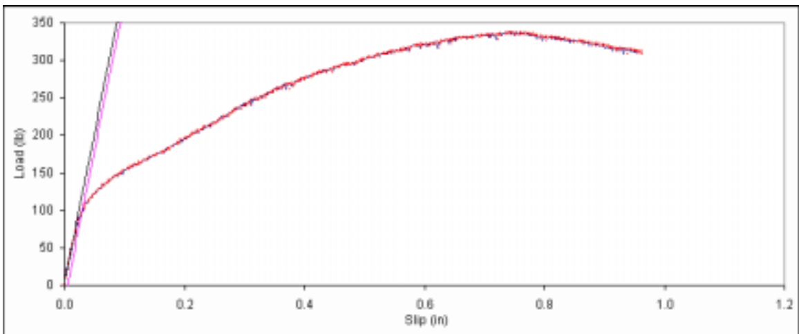
Figure B. 591: Load vs. slip plot for sample F5-14.
