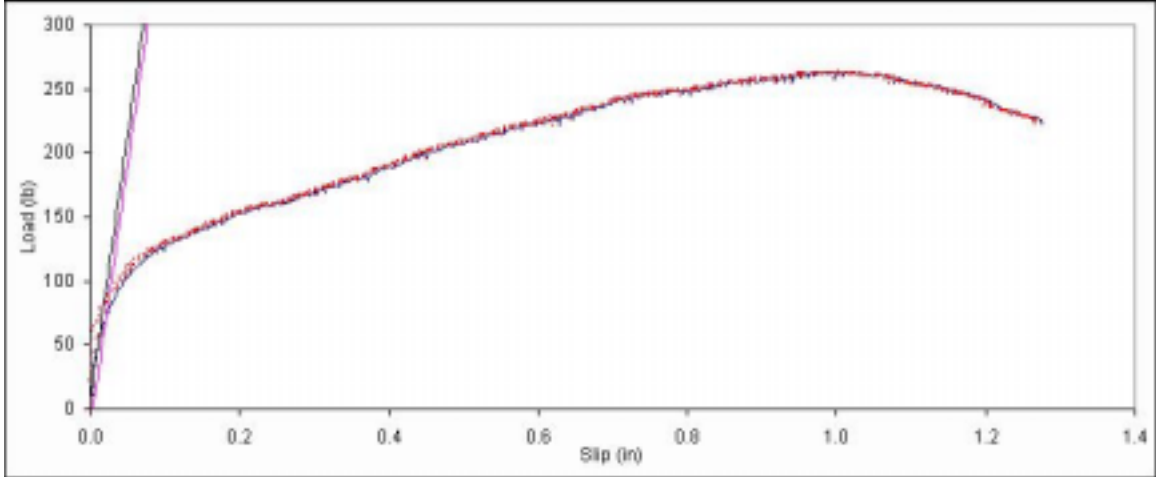
Figure B. 94: Load vs. slip plot for sample A7-6.
