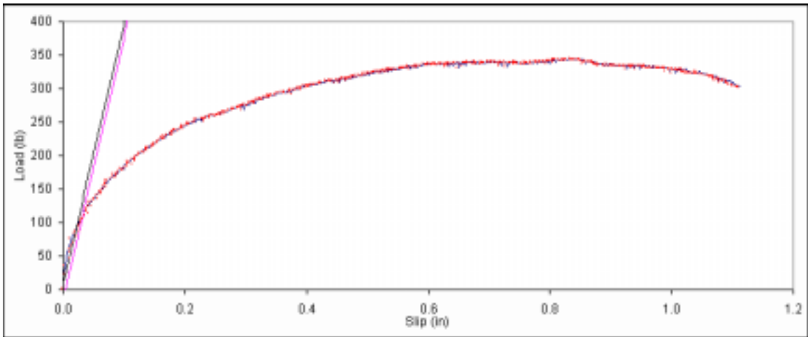
Figure B. 272: Load vs. slip plot for sample C5-6.
