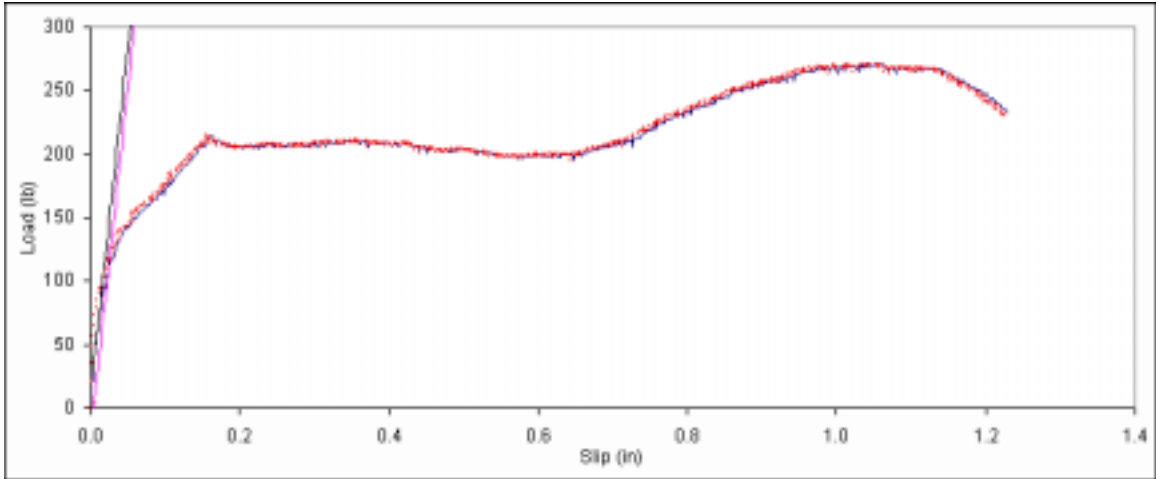
Figure B. 121: Load vs. slip plot for sample B2-4.
