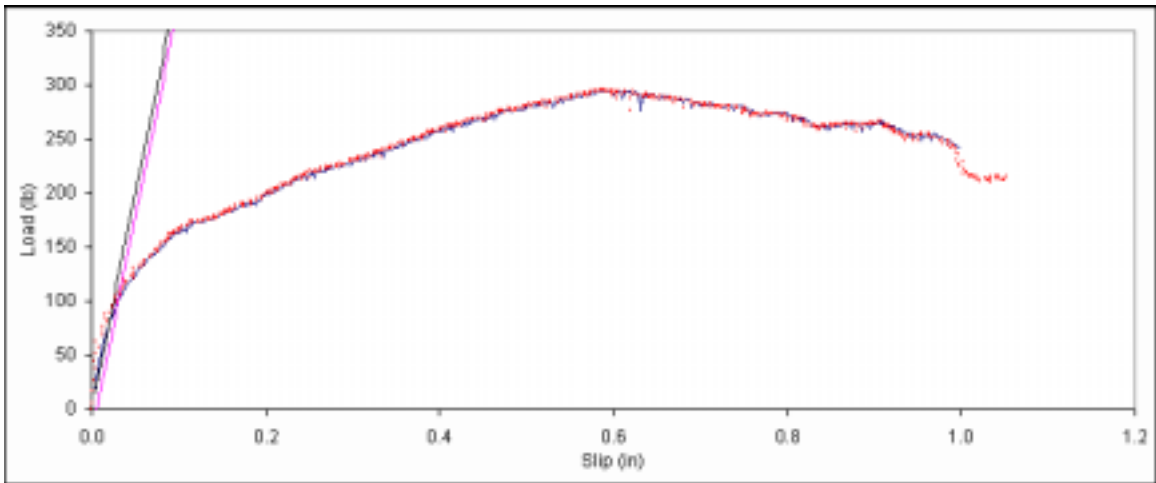
Figure B. 293: Load vs. slip plot for sample C6-12.
