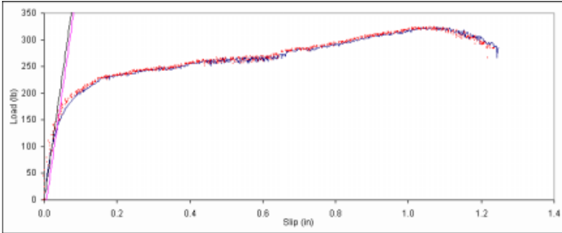
Figure B. 466: Load vs. slip plot for sample E4-6.
