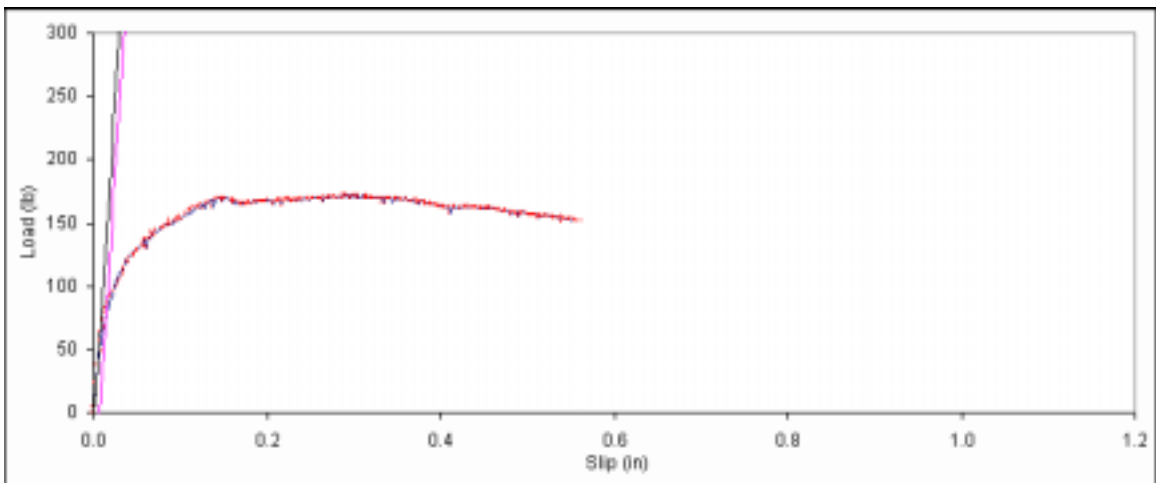
Figure B. 561: Load vs. slip plot for sample F3-14.
