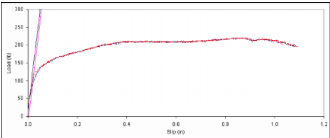
Figure B. 372: Load vs. slip plot for sample D5-2.
