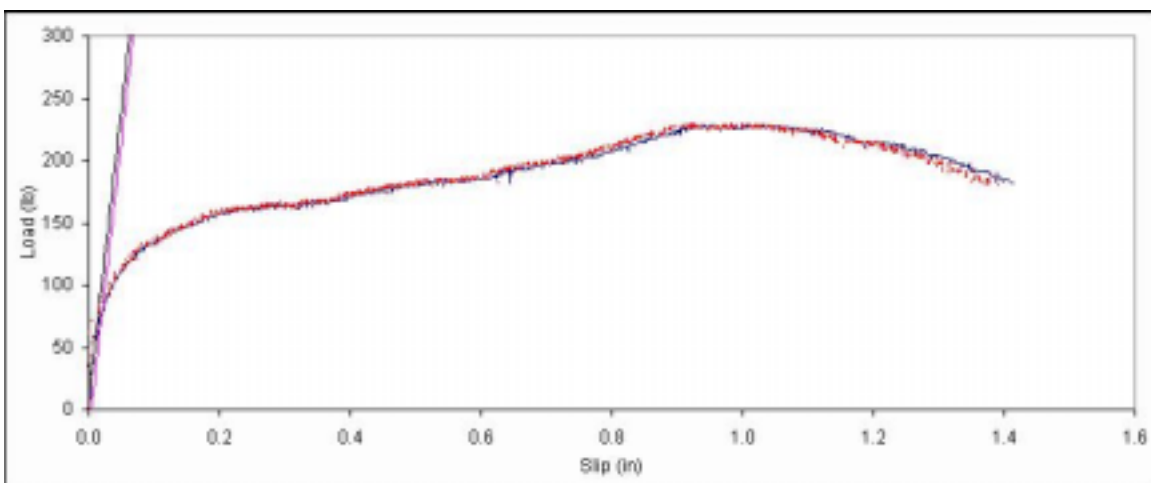
Figure B. 93: Load vs. slip plot for sample A7-5.
