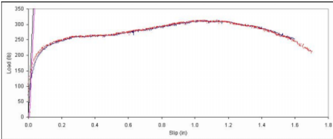
Figure B. 506: Load vs. slip plot for sample E7-2.
