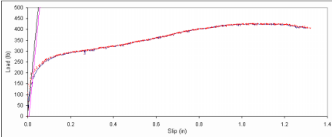
Figure B. 439: Load vs. slip plot for sample E2-9.
