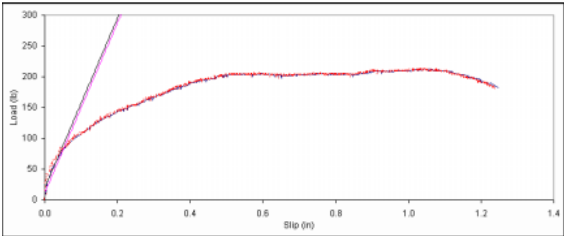
Figure B. 71: Load vs. slip plot for sample A5-12.
