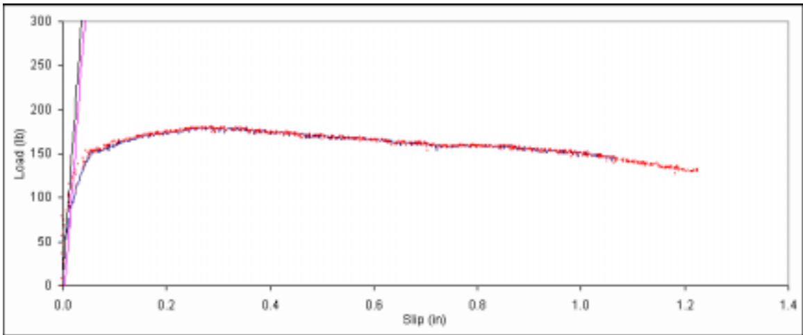
Figure B. 566: Load vs. slip plot for sample F4-4.
