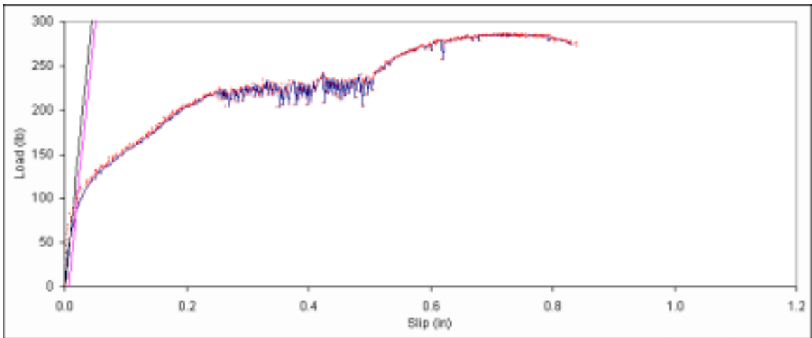
Figure B. 531: Load vs. slip plot for sample F1-12.
