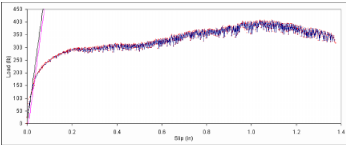
Figure B. 464: Load vs. slip plot for sample E4-4.
