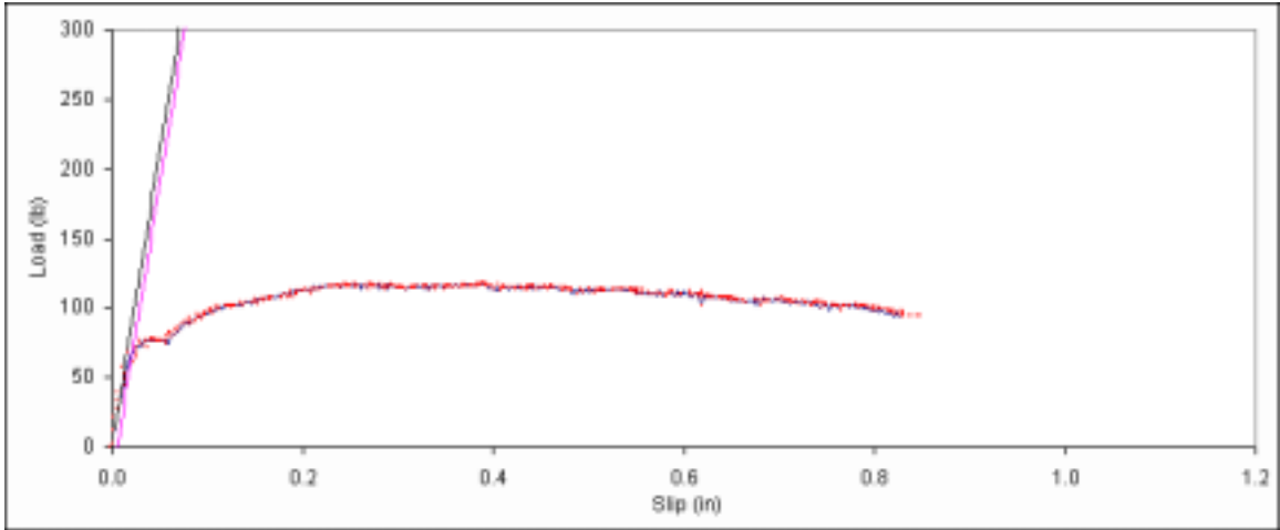
Figure B. 178: Load vs. slip plot for sample B6-1.
