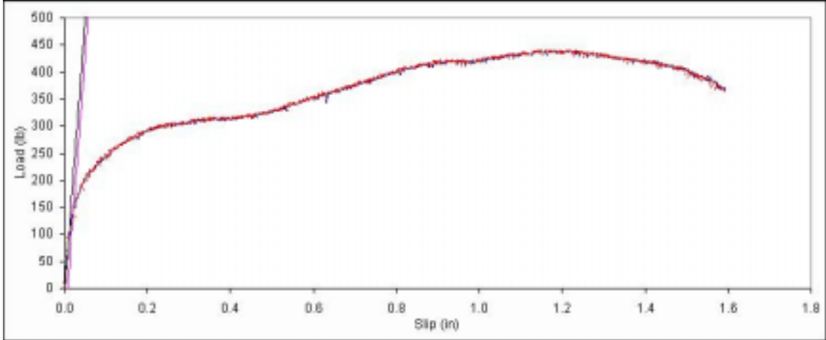
Figure B. 517: Load vs. slip plot for sample E7-13.
