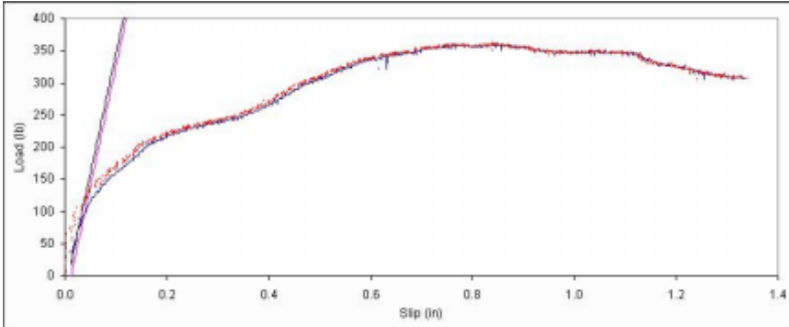
Figure B. 610: Load vs. slip plot for sample F7-3.
