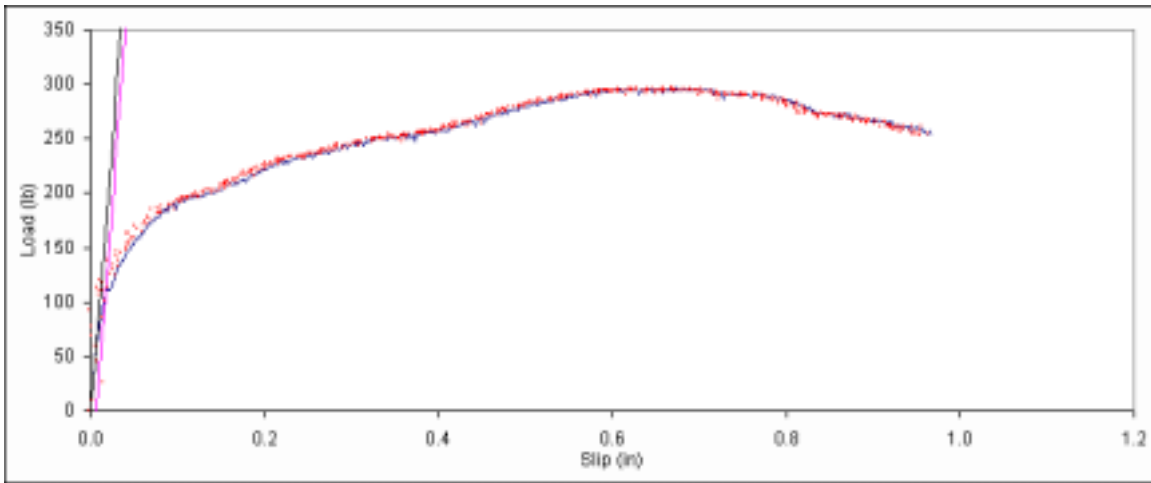
Figure B. 359: Load vs. slip plot for sample D4-4.
