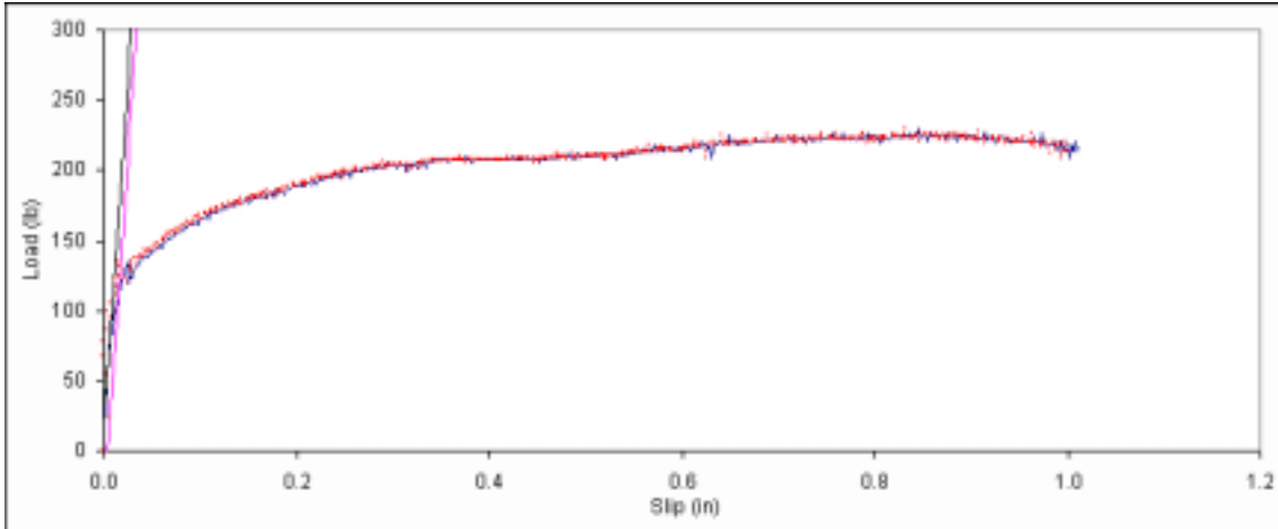
Figure B. 13: Load vs. slip plot for sample A1-14.
