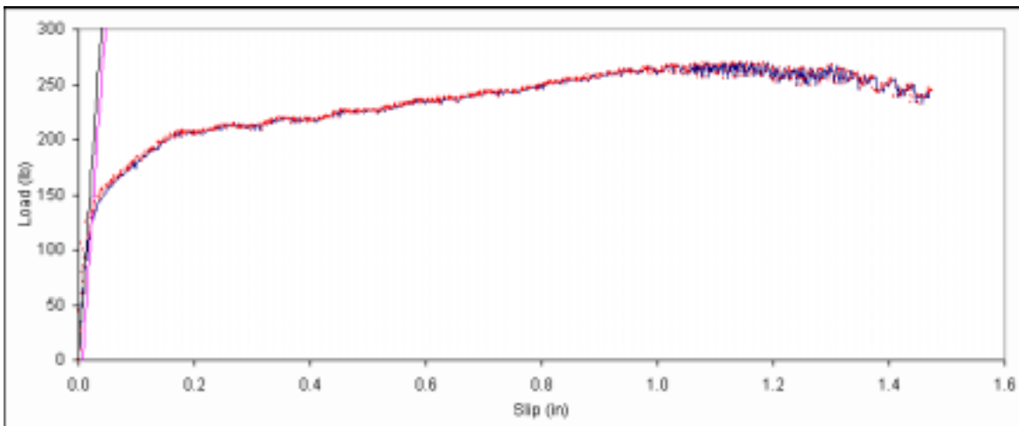
Figure B. 435: Load vs. slip plot for sample E2-5.
