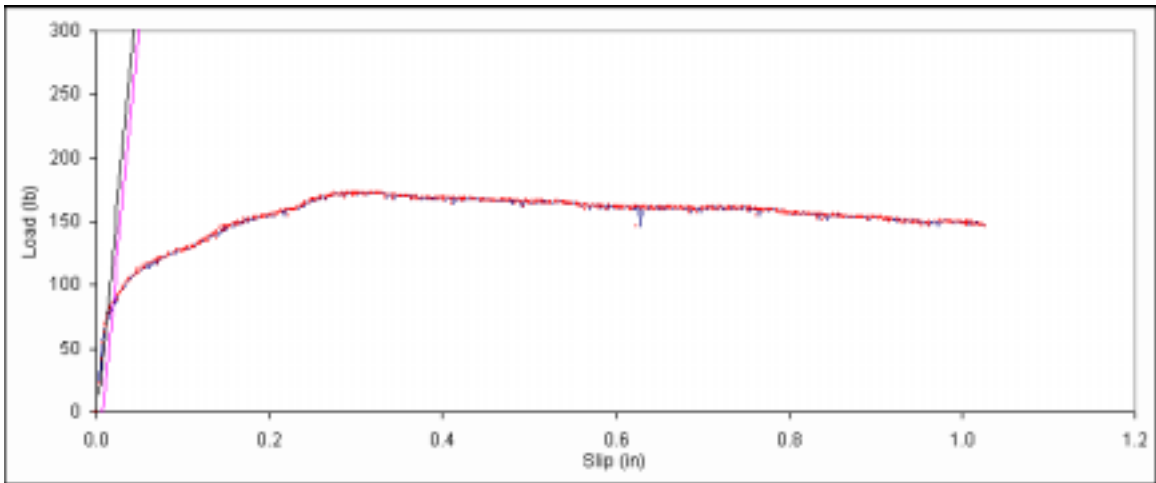
Figure B. 41: Load vs. slip plot for sample A3-12.
