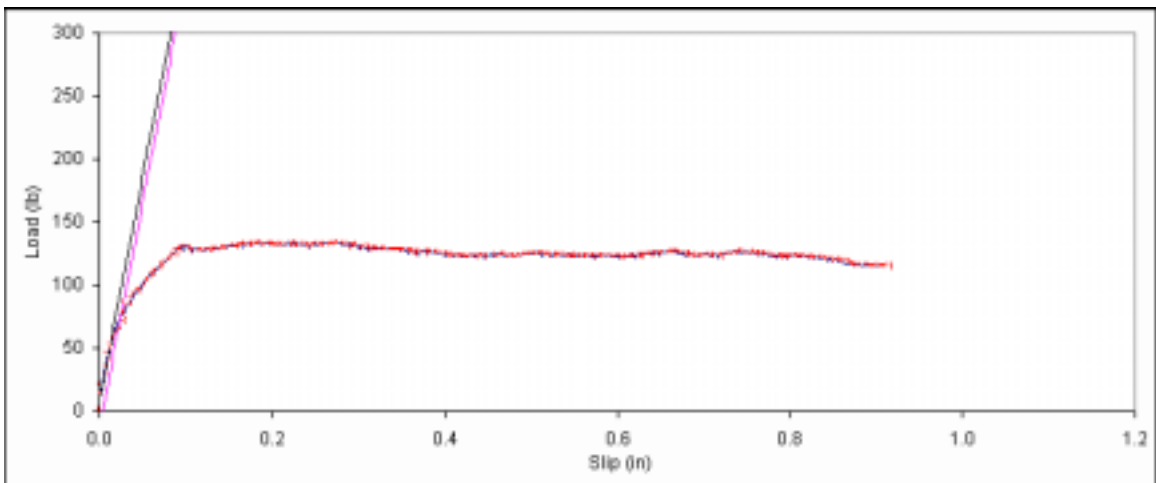
Figure B. 339: Load vs. slip plot for sample D2-14.
