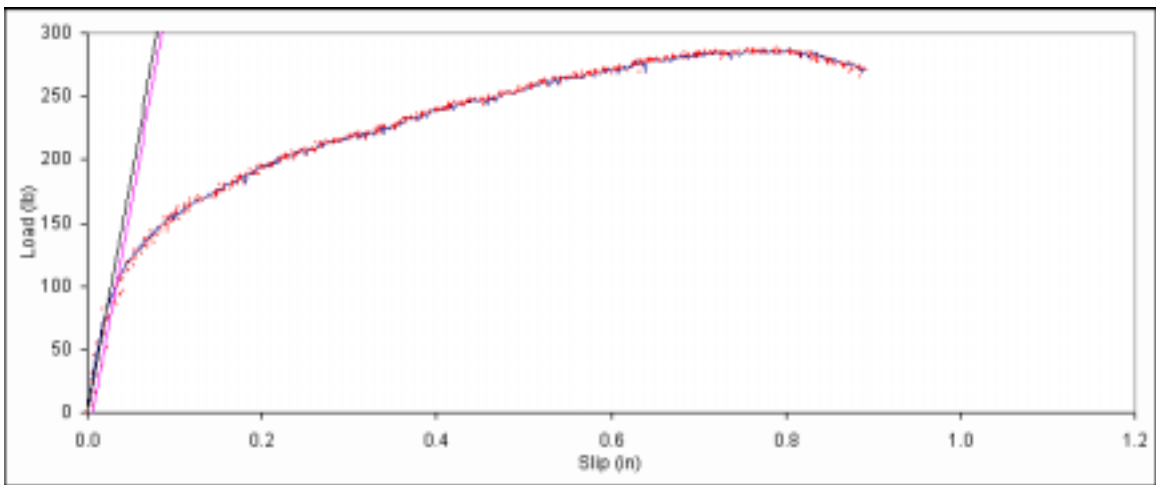
Figure B. 185: Load vs. slip plot for sample B6-8.
