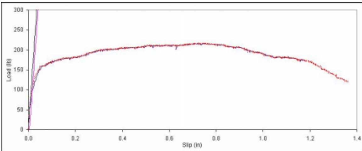
Figure B. 92: Load vs. slip plot for sample A7-4.
