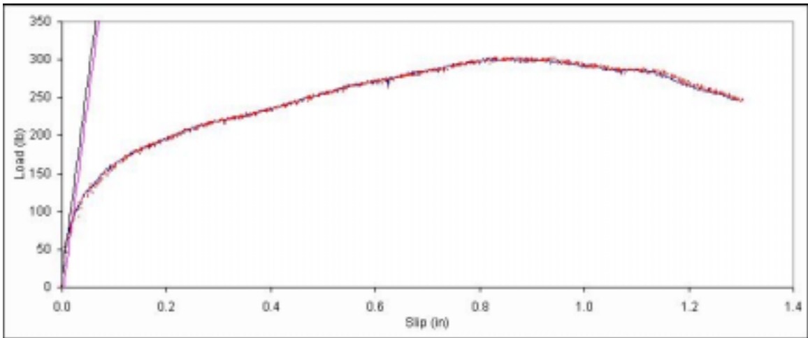
Figure B. 410: Load vs. slip plot for sample D7-10.
