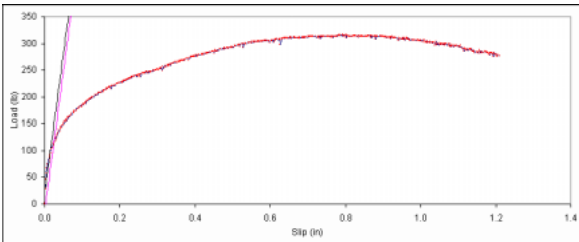
Figure B. 450: Load vs. slip plot for sample E3-5.
