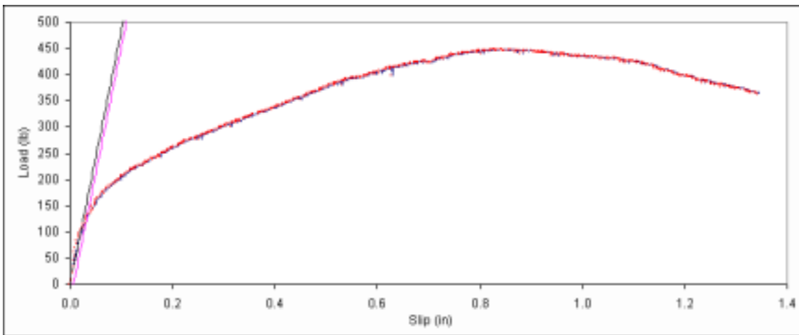
Figure B. 476: Load vs. slip plot for sample E5-1.
