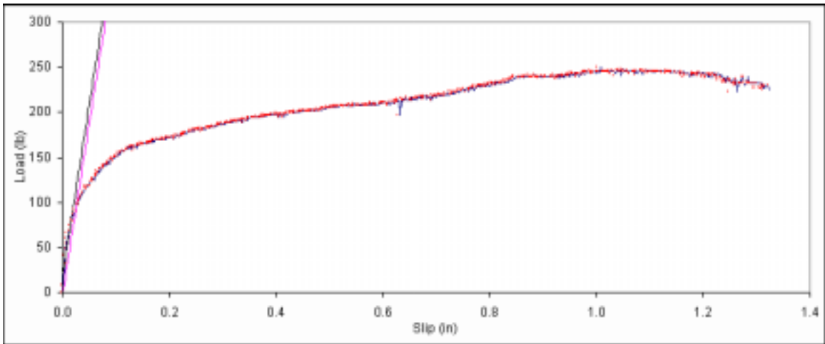
Figure B. 8: Load vs. slip plot for sample A1-8.
