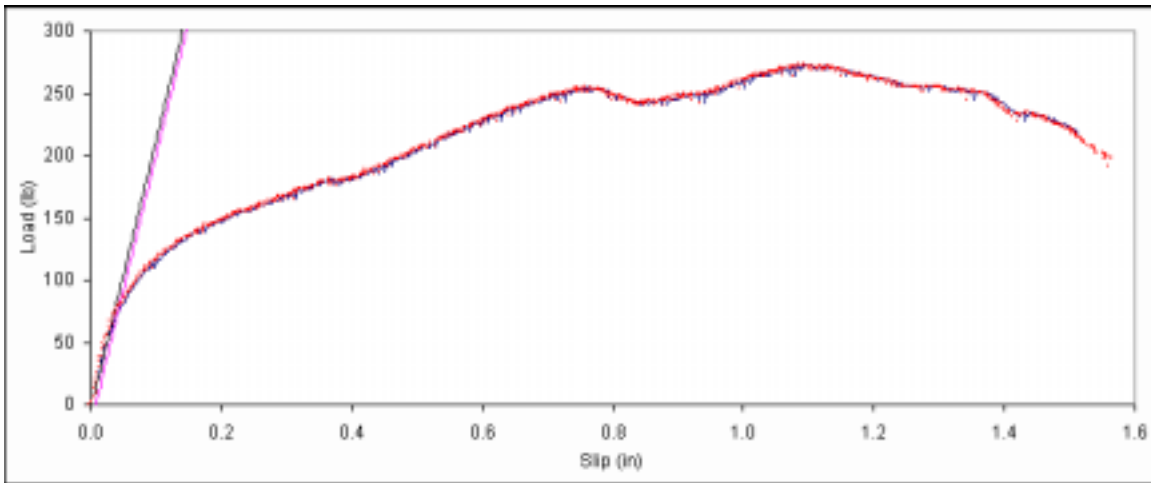
Figure B. 584: Load vs. slip plot for sample F5-7.
