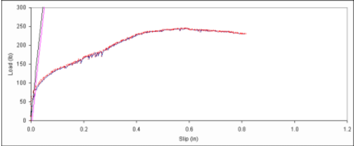
Figure B. 322: Load vs. slip plot for sample D1-12.
