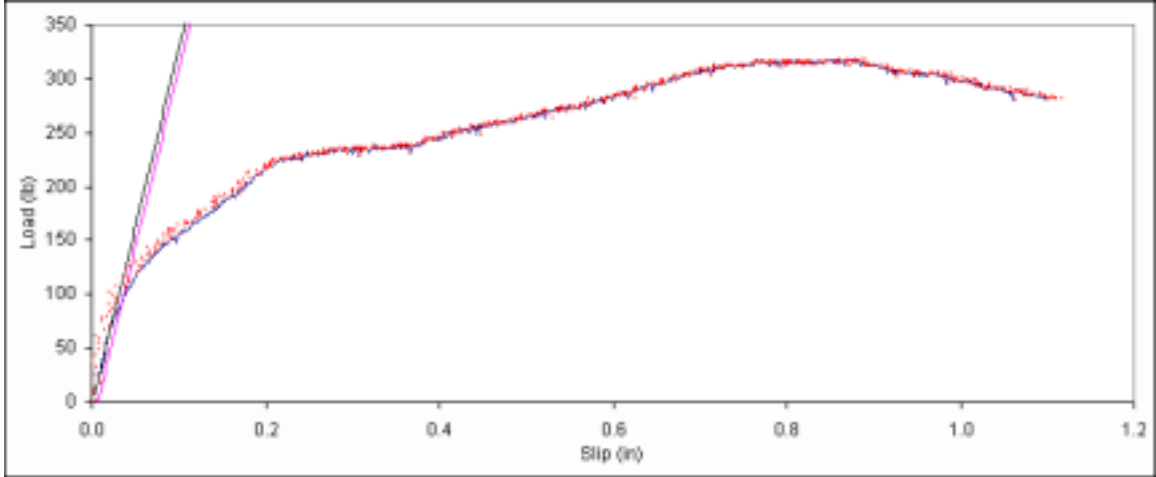
Figure B. 607: Load vs. slip plot for sample F6-15.
