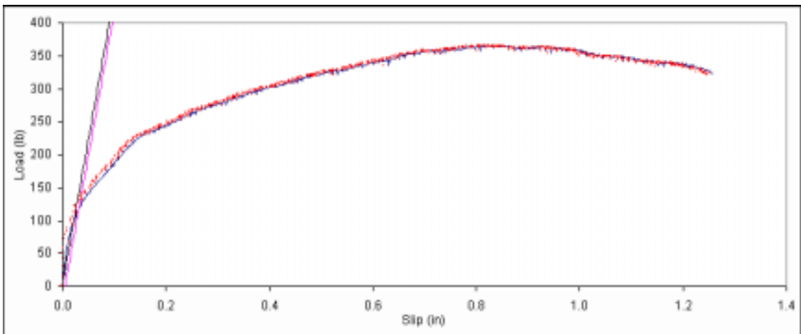
Figure B. 285: Load vs. slip plot for sample C6-4.
