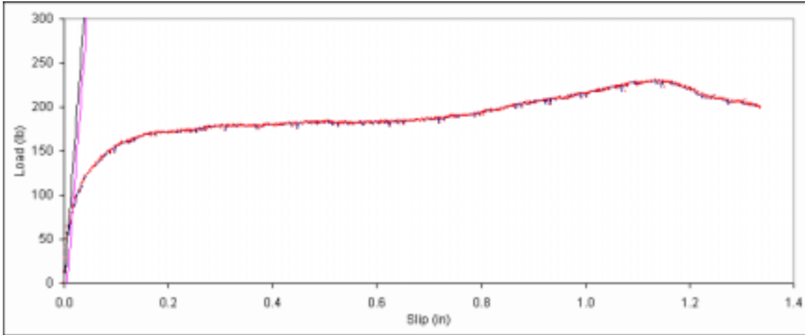
Figure B. 574: Load vs. slip plot for sample F4-12.
