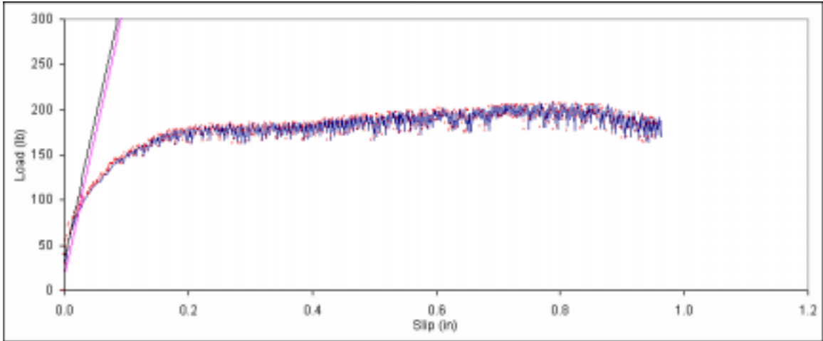
Figure B. 4: Load vs. slip plot for sample A1-4.
