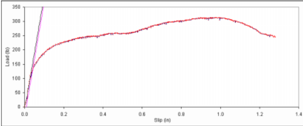
Figure B. 250: Load vs. slip plot for sample C3-14.
