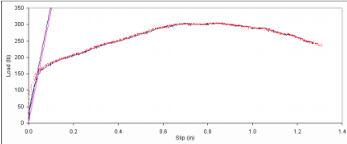
Figure B. 358: Load vs. slip plot for sample D4-3.
