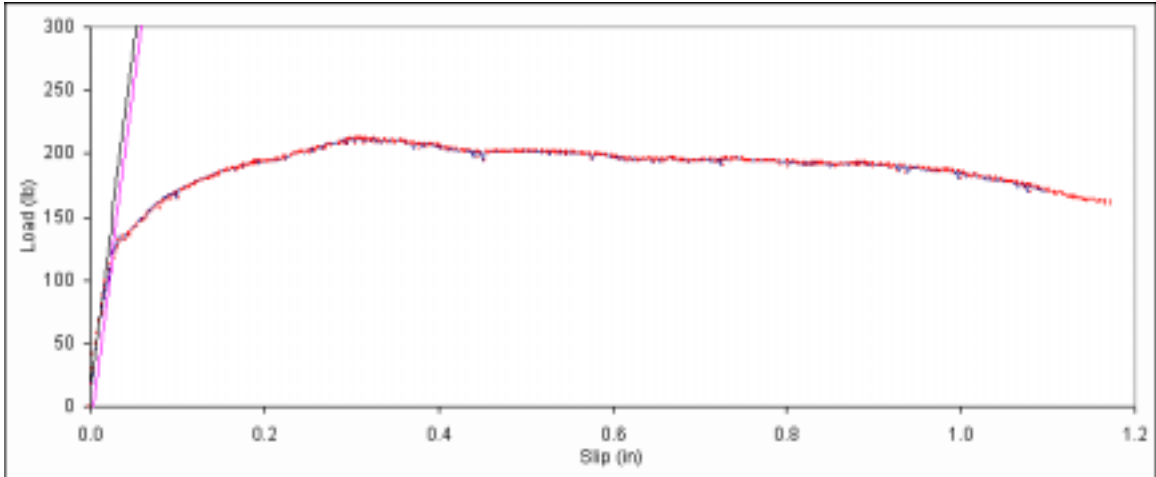
Figure B. 160: Load vs. slip plot for sample B4-13.
