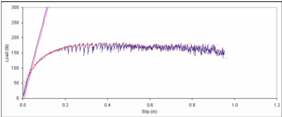
Figure B. 335: Load vs. slip plot for sample D2-10.
