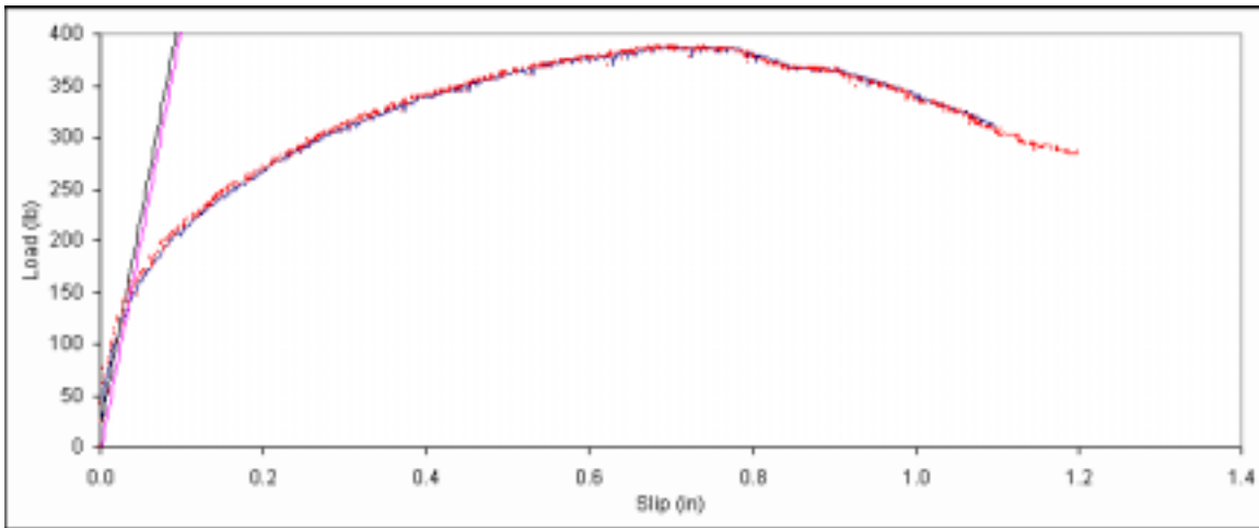
Figure B. 74: Load vs. slip plot for sample A5-15.
