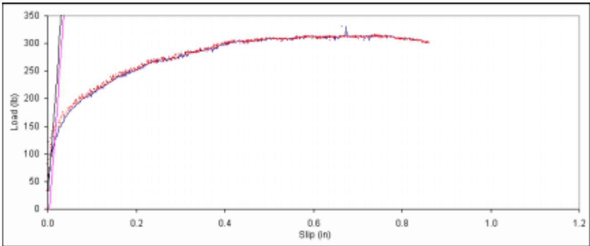
Figure B. 221: Load vs. slip plot for sample C1-14.
