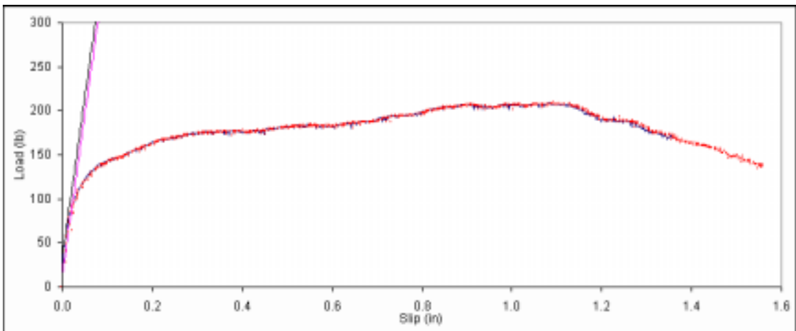
Figure B. 138: Load vs. slip plot for sample B3-6.
