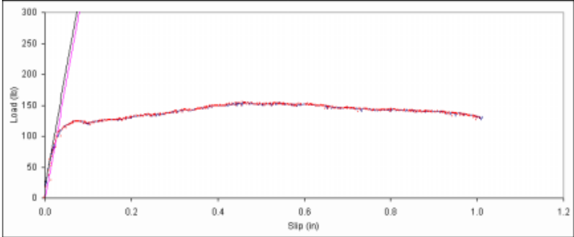
Figure B. 169: Load vs. slip plot for sample B5-7.
