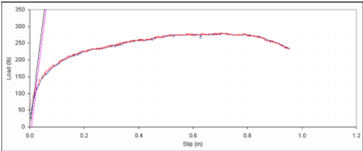
Figure B. 269: Load vs. slip plot for sample C5-3.
