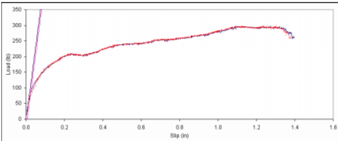
Figure B. 375: Load vs. slip plot for sample D5-5.
