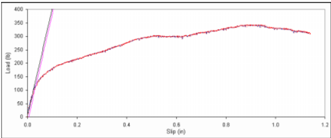
Figure B. 290: Load vs. slip plot for sample C6-9.
