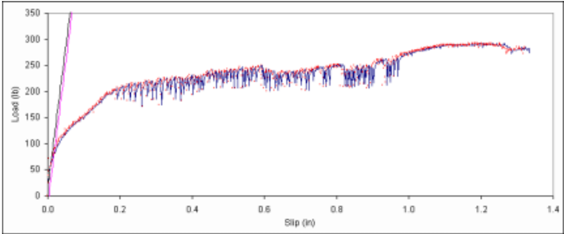
Figure B. 313: Load vs. slip plot for sample D1-2.
