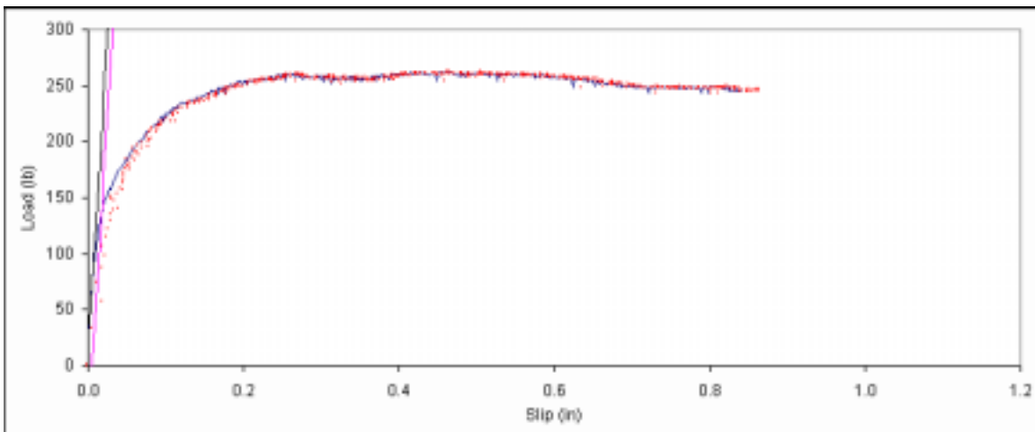
Figure B. 432: Load vs. slip plot for sample E2-2.
