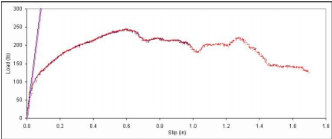
Figure B. 206: Load vs. slip plot for sample B7-14.
