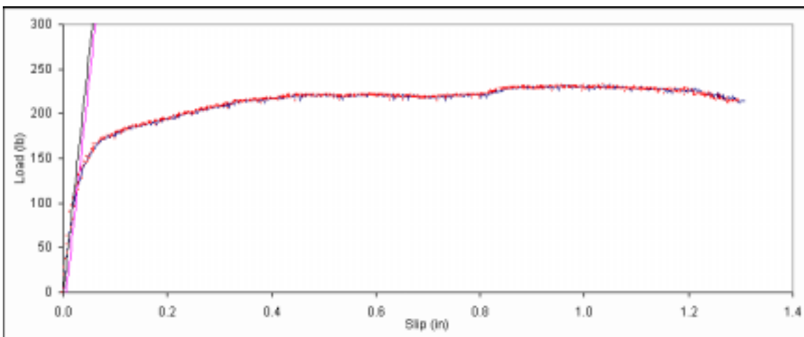
Figure B. 525: Load vs. slip plot for sample F1-6.
