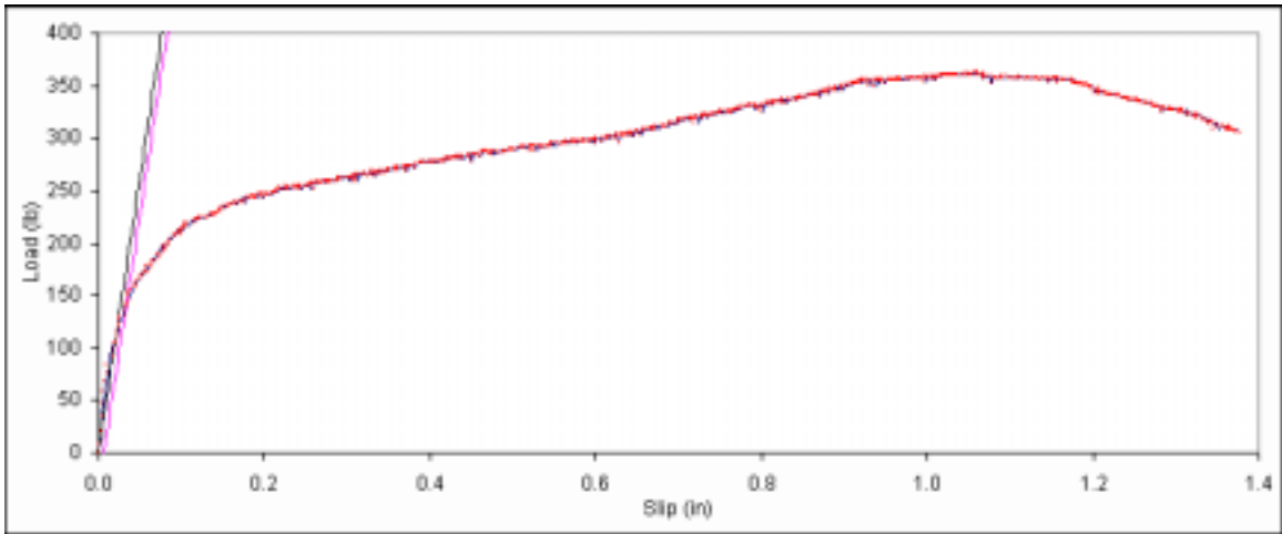
Figure B. 485: Load vs. slip plot for sample E5-10.
