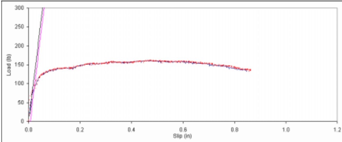
Figure B. 352: Load vs. slip plot for sample D3-12.
