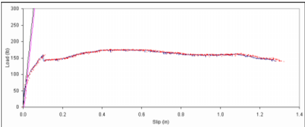
Figure B. 48: Load vs. slip plot for sample A4-4.
