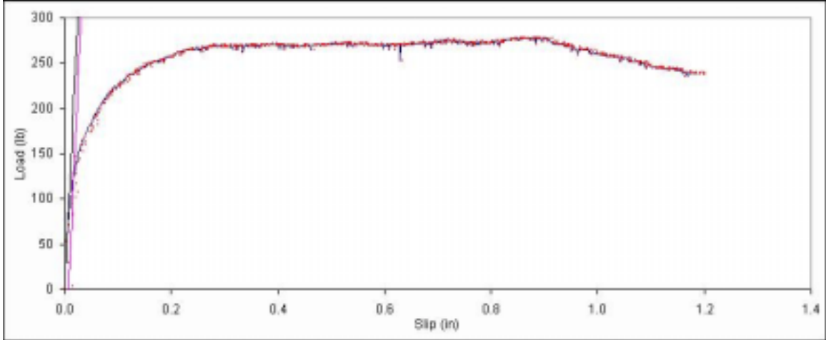
Figure B. 508: Load vs. slip plot for sample E7-4.
