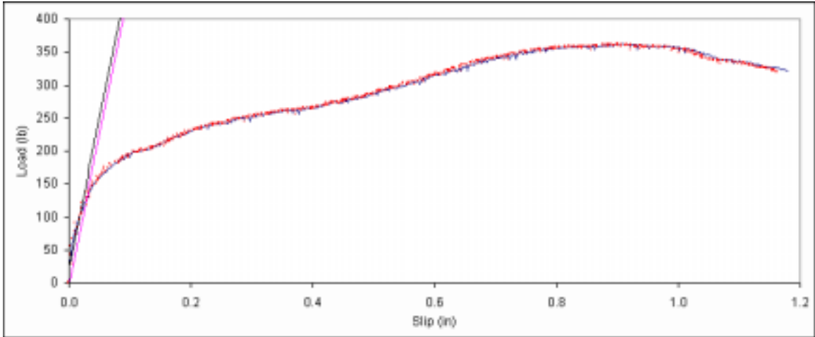
Figure B. 61: Load vs. slip plot for sample A5-2.
