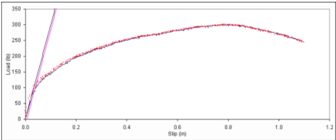
Figure B. 363: Load vs. slip plot for sample D4-8.
