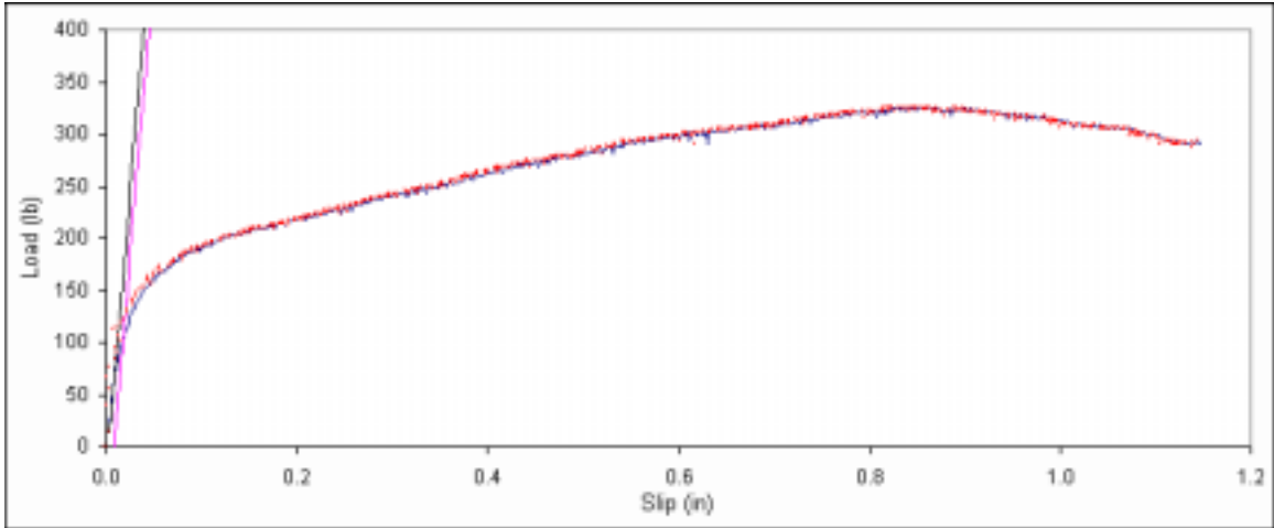
Figure B. 349: Load vs. slip plot for sample D3-9.
