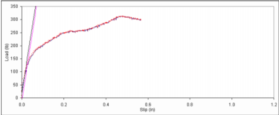
Figure B. 106: Load vs. slip plot for sample B1-4.
