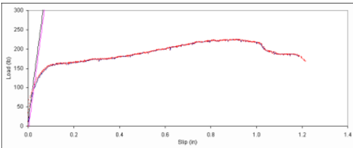
Figure B. 177: Load vs. slip plot for sample B5-15.
