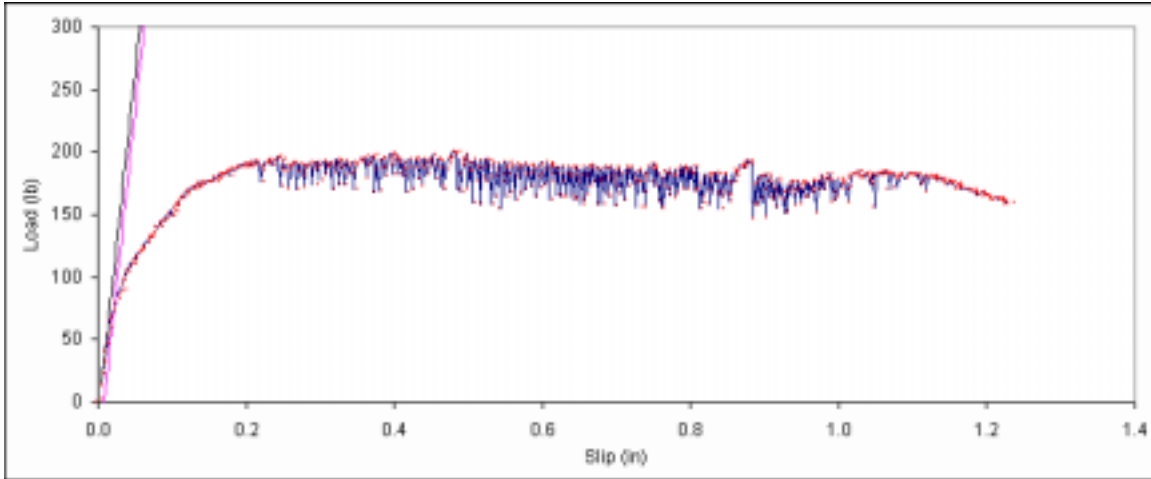
Figure B. 535: Load vs. slip plot for sample F2-2.
