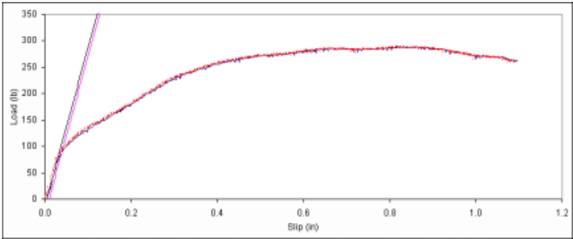
Figure B. 362: Load vs. slip plot for sample D4-7.
