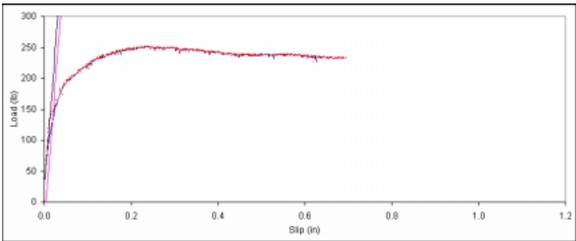
Figure B. 494: Load vs. slip plot for sample E6-5.
