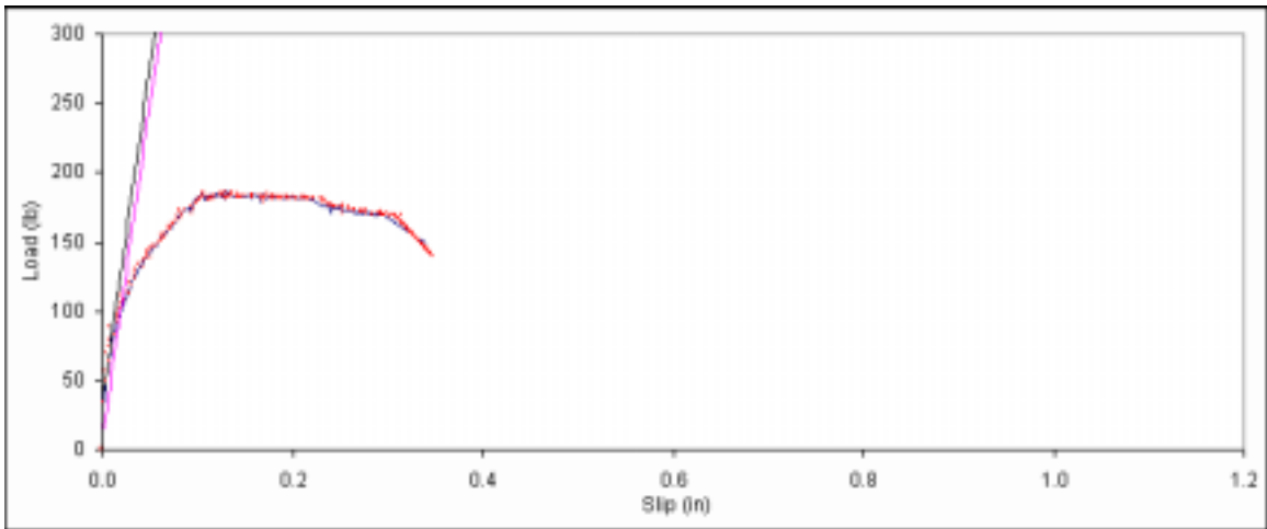
Figure B. 116: Load vs. slip plot for sample B1-14.
