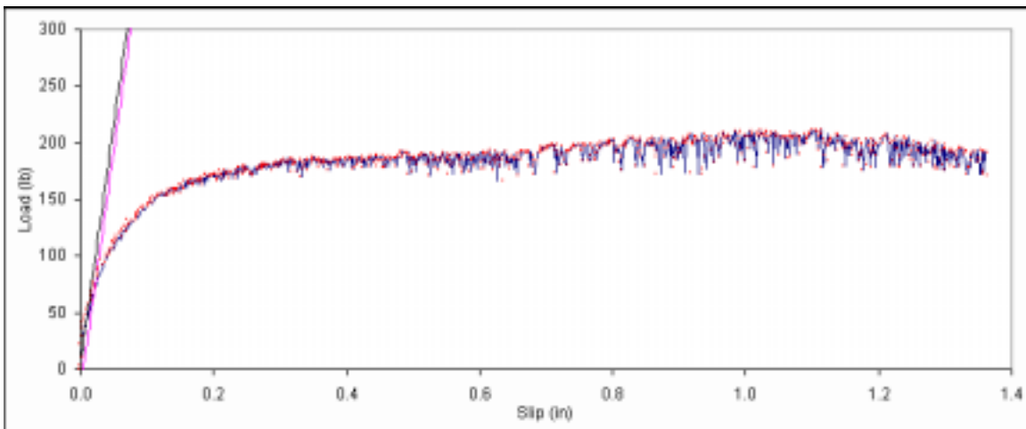
Figure B. 537: Load vs. slip plot for sample F2-4.
