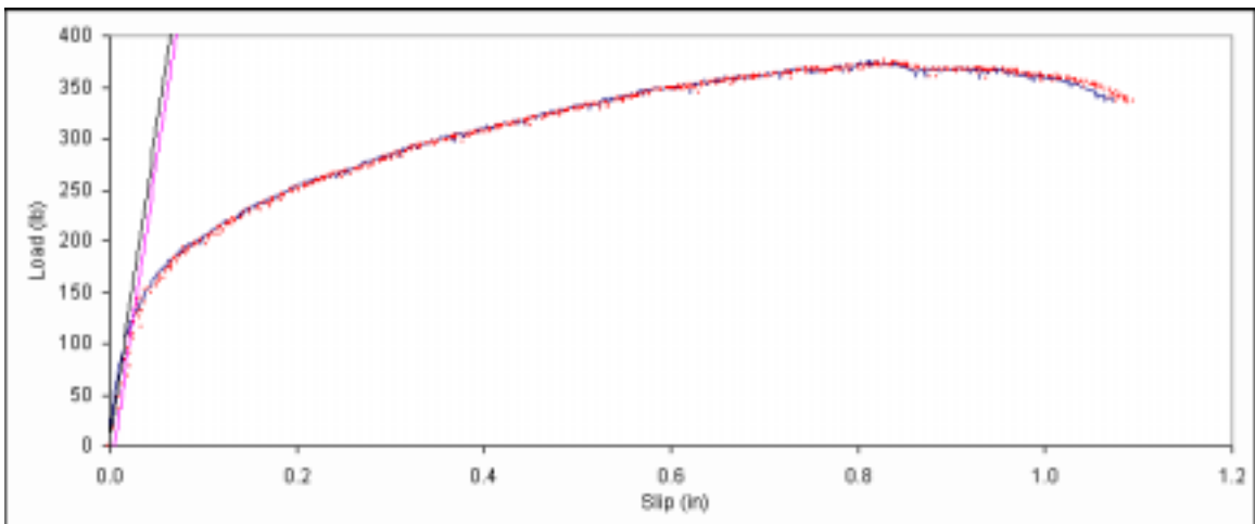
Figure B. 282: Load vs. slip plot for sample C6-1.
