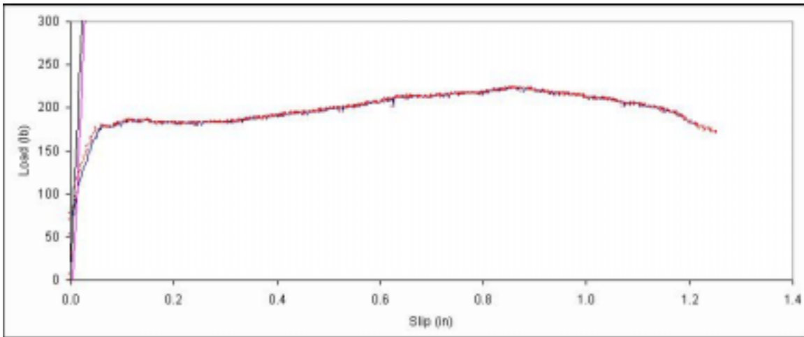
Figure B. 203: Load vs. slip plot for sample B7-11.
