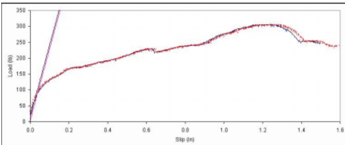
Figure B. 618: Load vs. slip plot for sample F7-11.
