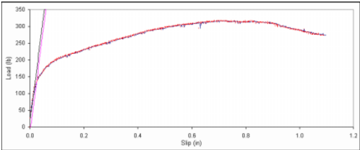
Figure B. 68: Load vs. slip plot for sample A5-9.
