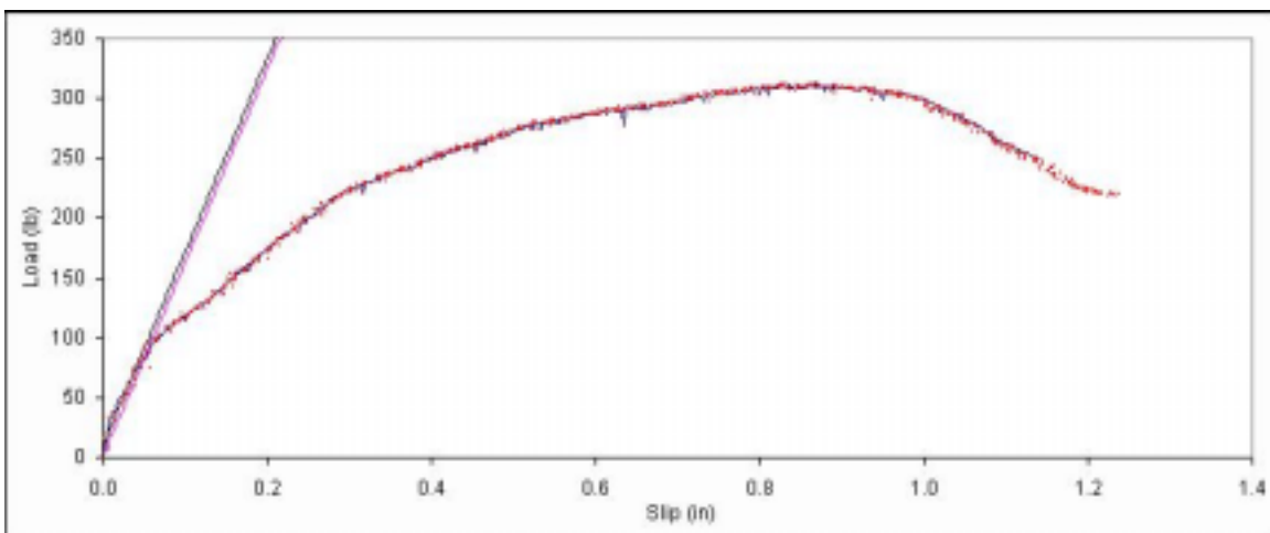
Figure B. 621: Load vs. slip plot for sample F7-14.
