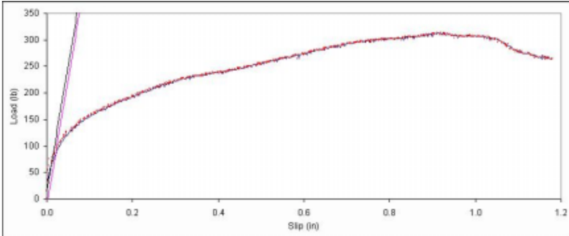
Figure B. 91: Load vs. slip plot for sample A7-3.
