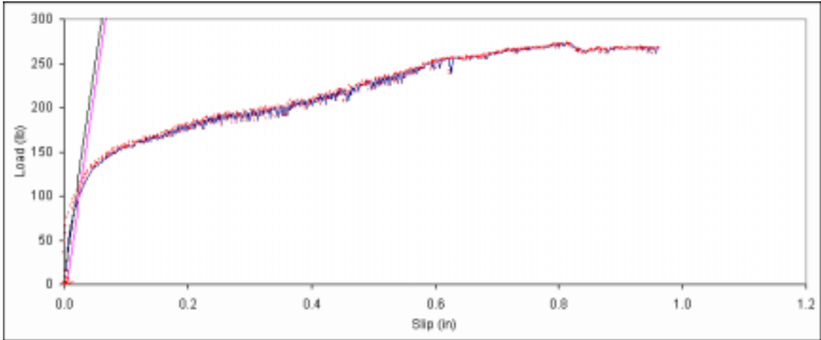
Figure B. 7: Load vs. slip plot for sample A1-7.
