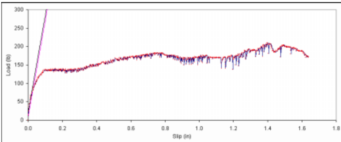
Figure B. 120: Load vs. slip plot for sample B2-3.
