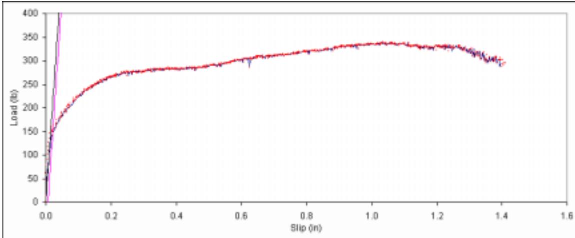
Figure B. 457: Load vs. slip plot for sample E3-12.
