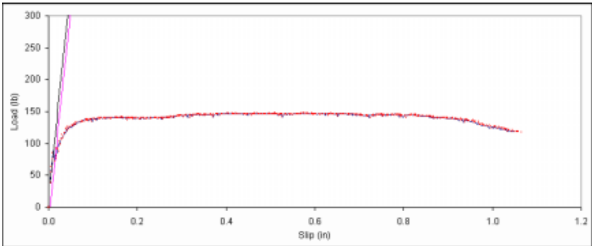
Figure B. 135: Load vs. slip plot for sample B3-3.
