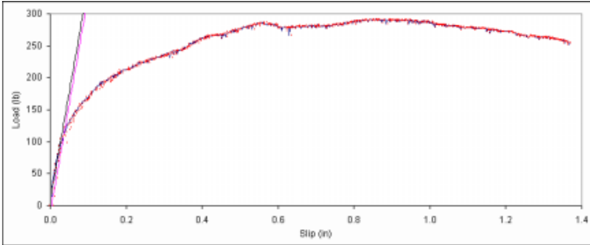
Figure B. 76: Load vs. slip plot for sample A6-2.
