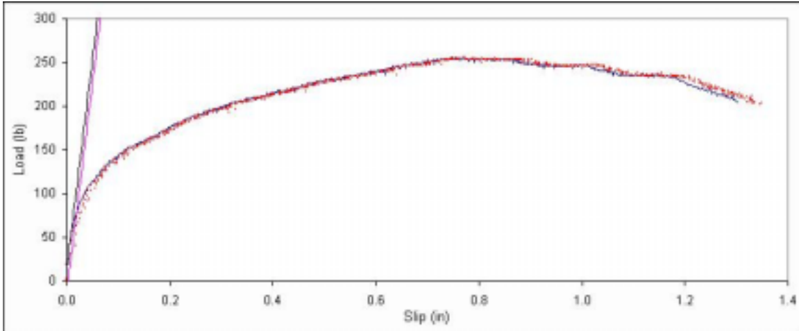
Figure B. 97: Load vs. slip plot for sample A7-9.
