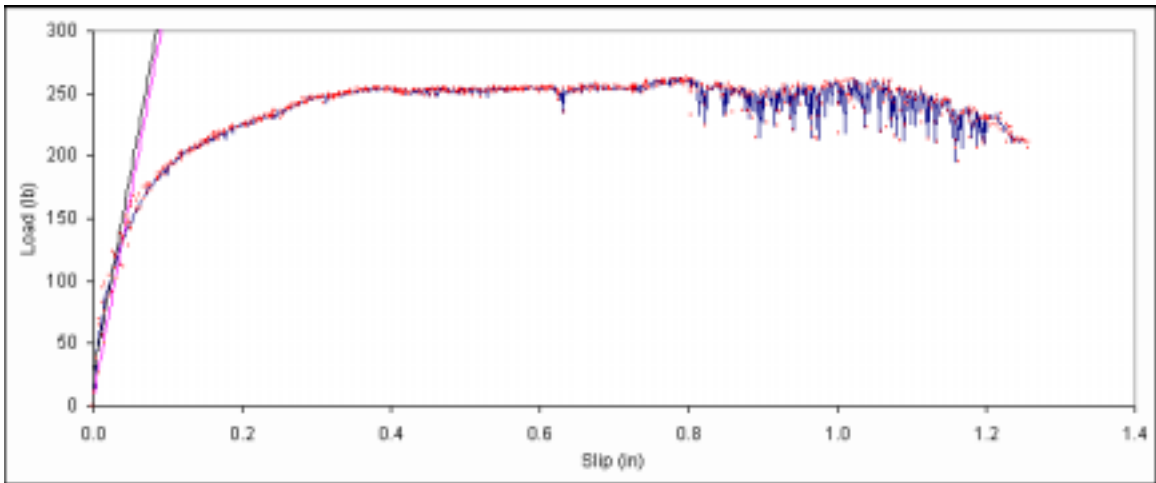
Figure B. 365: Load vs. slip plot for sample D4-10.
