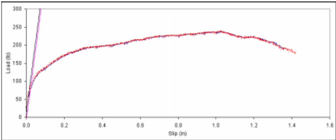
Figure B. 347: Load vs. slip plot for sample D3-7.
