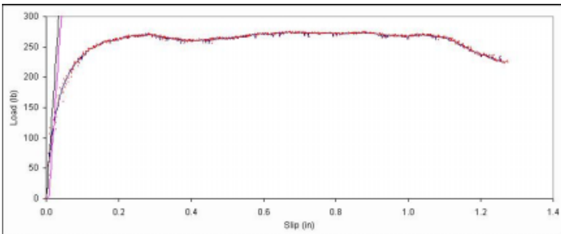
Figure B. 507: Load vs. slip plot for sample E7-3.
