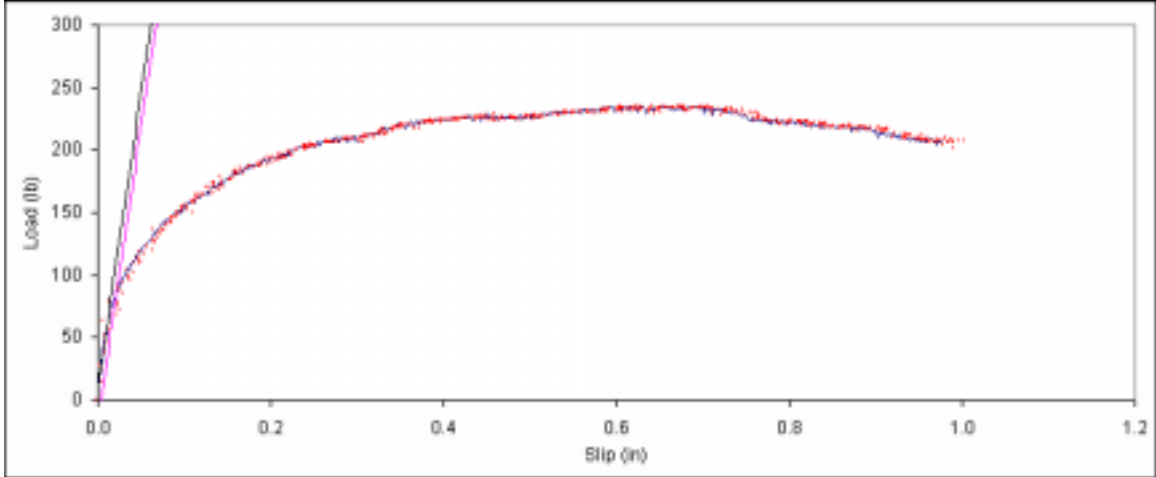
Figure B. 253: Load vs. slip plot for sample C4-2.
