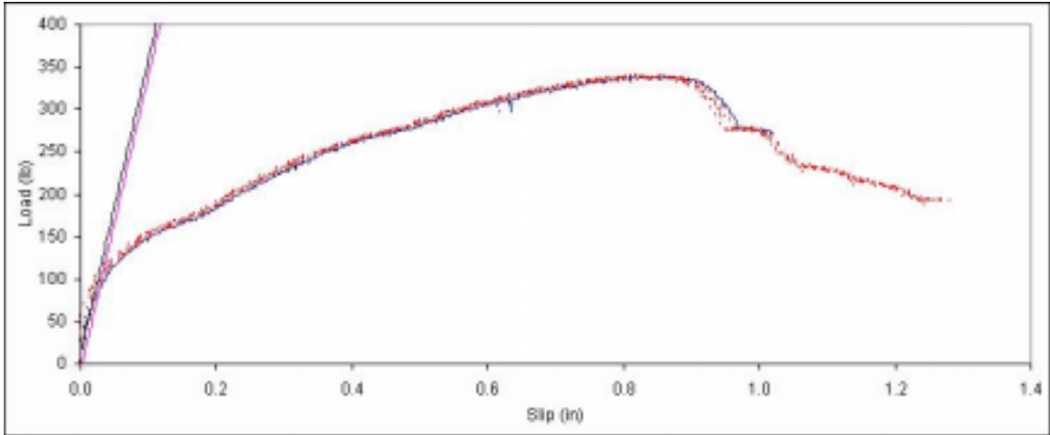
Figure B. 301: Load vs. slip plot for sample C7-5.
