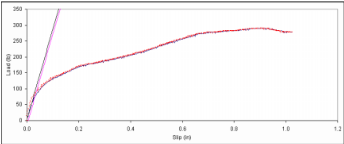
Figure B. 392: Load vs. slip plot for sample D6-7.
