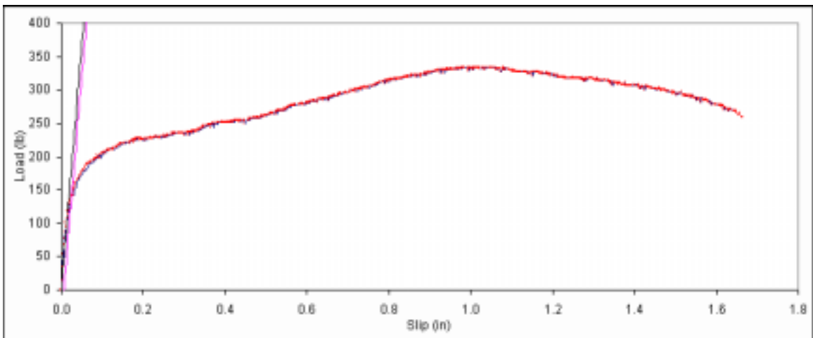
Figure B. 453: Load vs. slip plot for sample E3-8.
