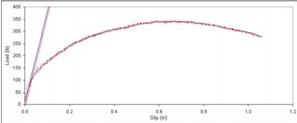
Figure B. 616: Load vs. slip plot for sample F7-9.
