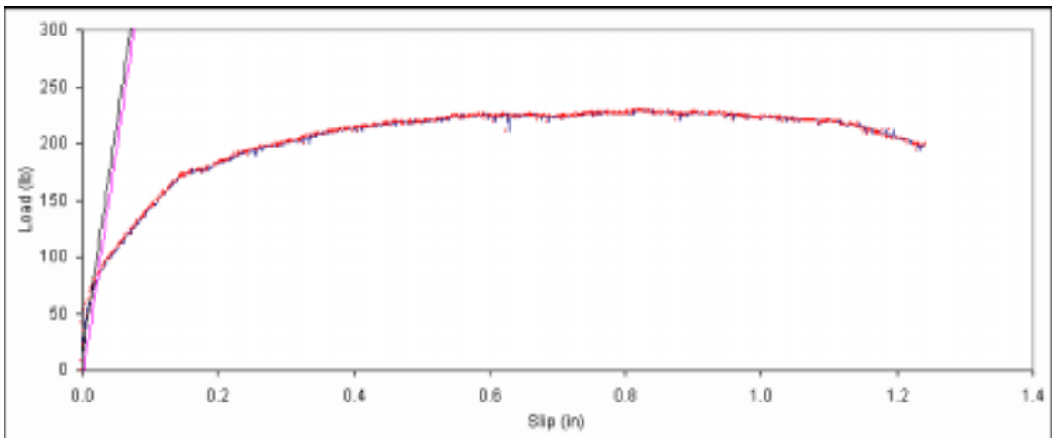
Figure B. 258: Load vs. slip plot for sample C4-7.
