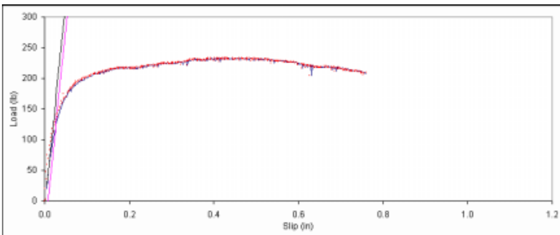
Figure B. 501: Load vs. slip plot for sample E6-12.
