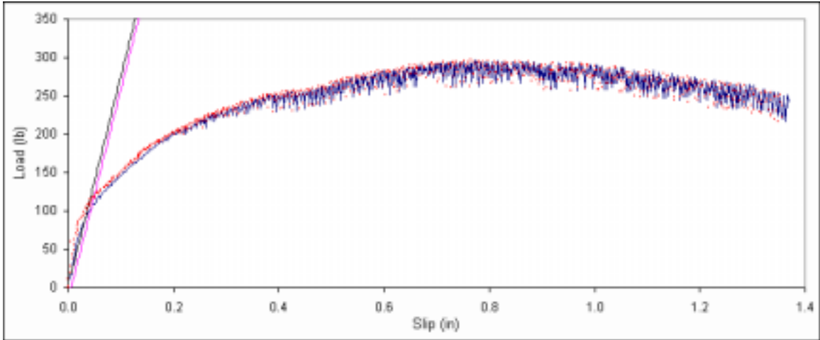
Figure B. 469: Load vs. slip plot for sample E4-9.
