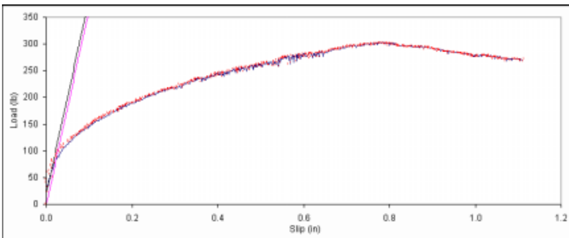
Figure B. 354: Load vs. slip plot for sample D3-14.
