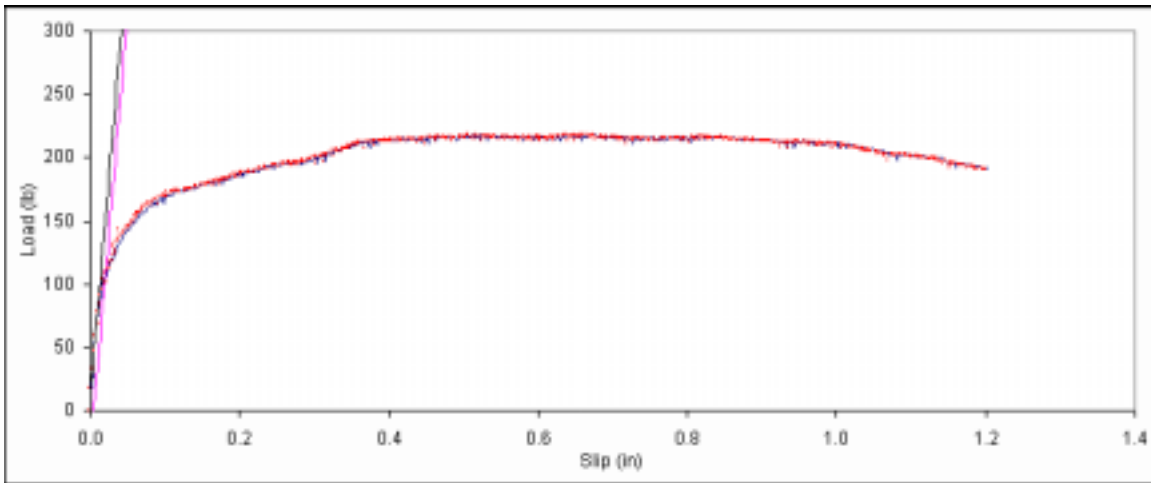
Figure B. 473: Load vs. slip plot for sample E4-13.
