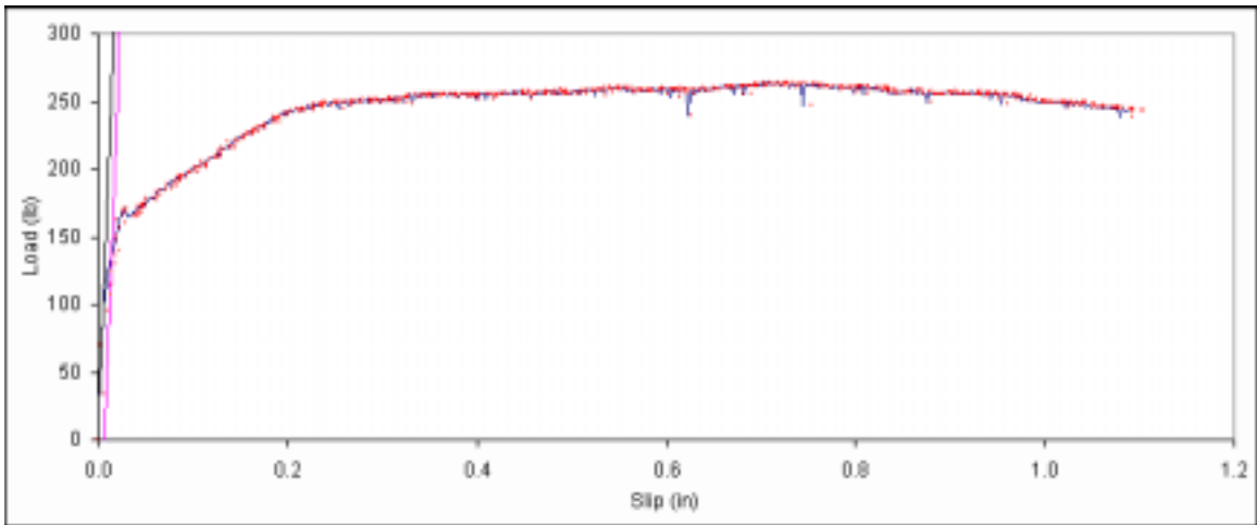
Figure B. 437: Load vs. slip plot for sample E2-7.
