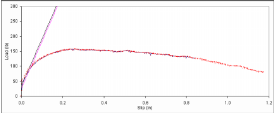
Figure B. 136: Load vs. slip plot for sample B3-4
