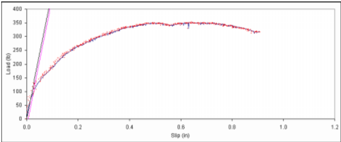
Figure B. 599: Load vs. slip plot for sample F6-7.
