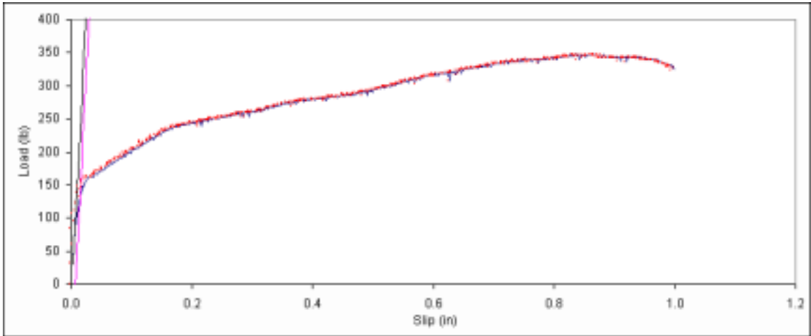
Figure B. 520: Load vs. slip plot for sample F1-1.
