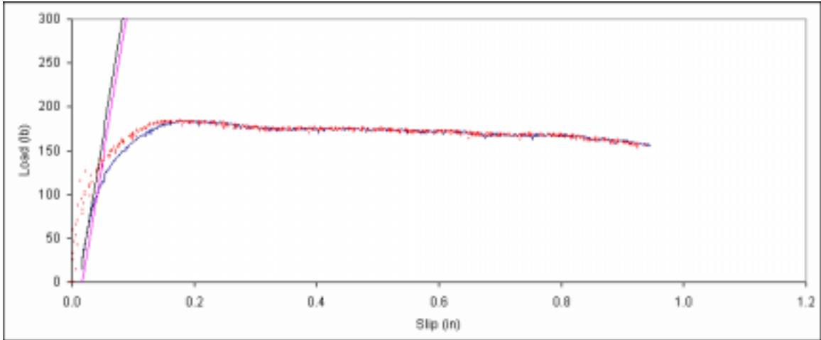
Figure B. 262: Load vs. slip plot for sample C4-11.
