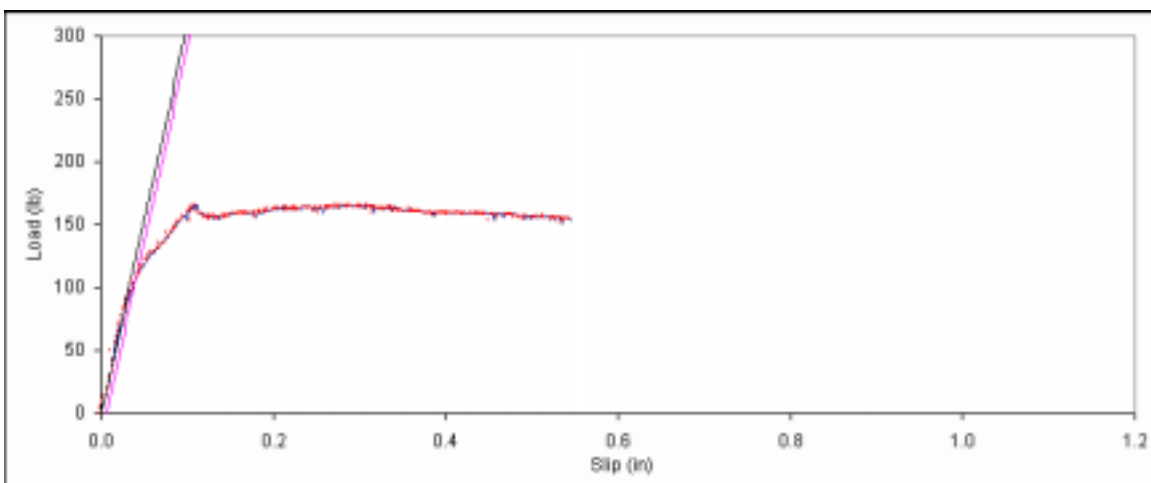
Figure B. 534: Load vs. slip plot for sample F2-1.
