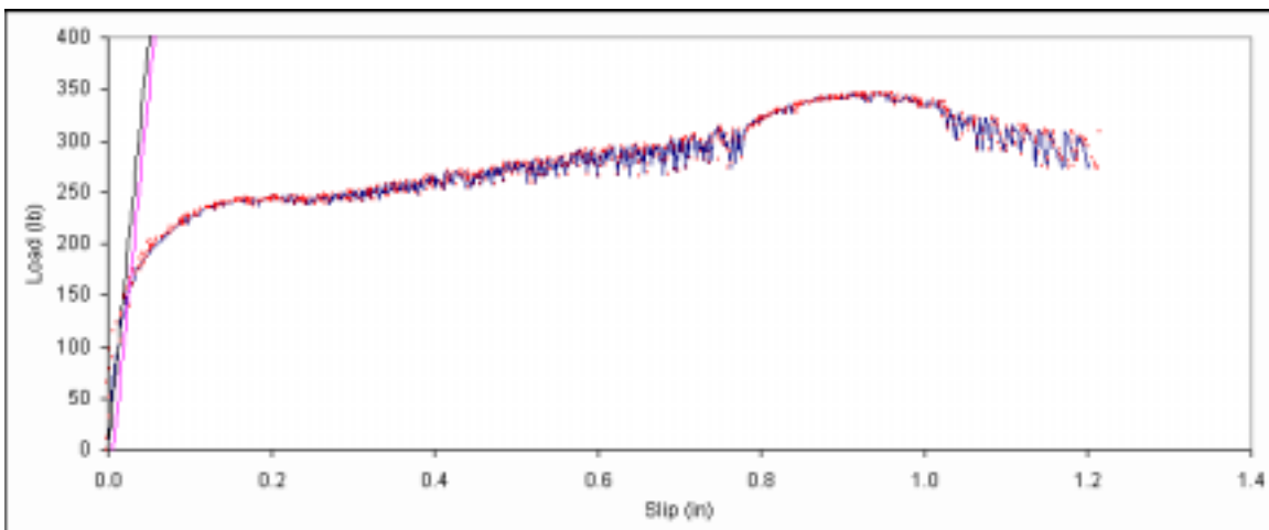
Figure B. 462: Load vs. slip plot for sample E4-2.
