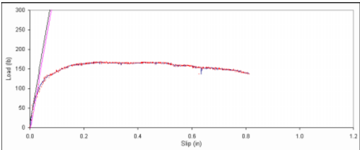
Figure B. 156: Load vs. slip plot for sample B4-9.
