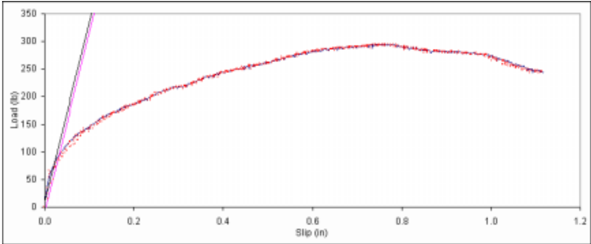
Figure B. 259: Load vs. slip plot for sample C4-8.
