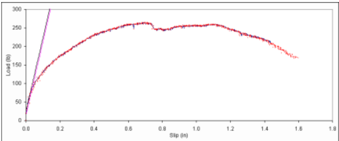
Figure B. 54: Load vs. slip plot for sample A4-10.
