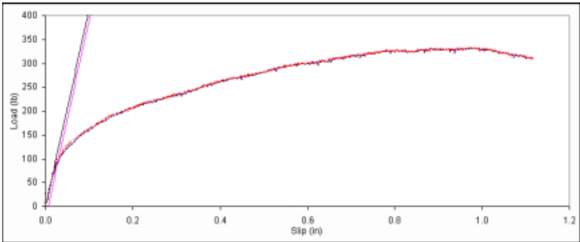
Figure B. 389: Load vs. slip plot for sample D6-4.
