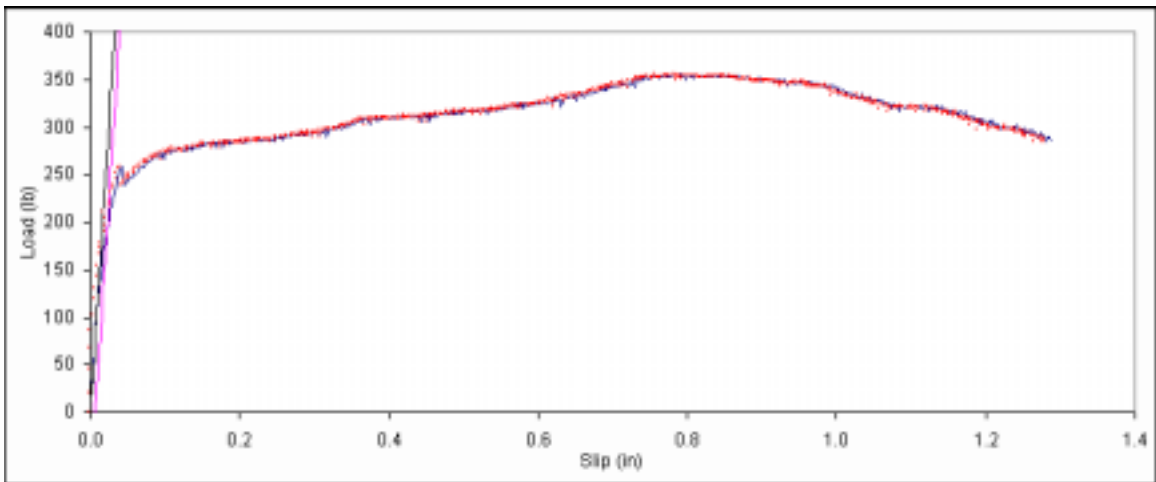
Figure B. 479: Load vs. slip plot for sample E5-4.
