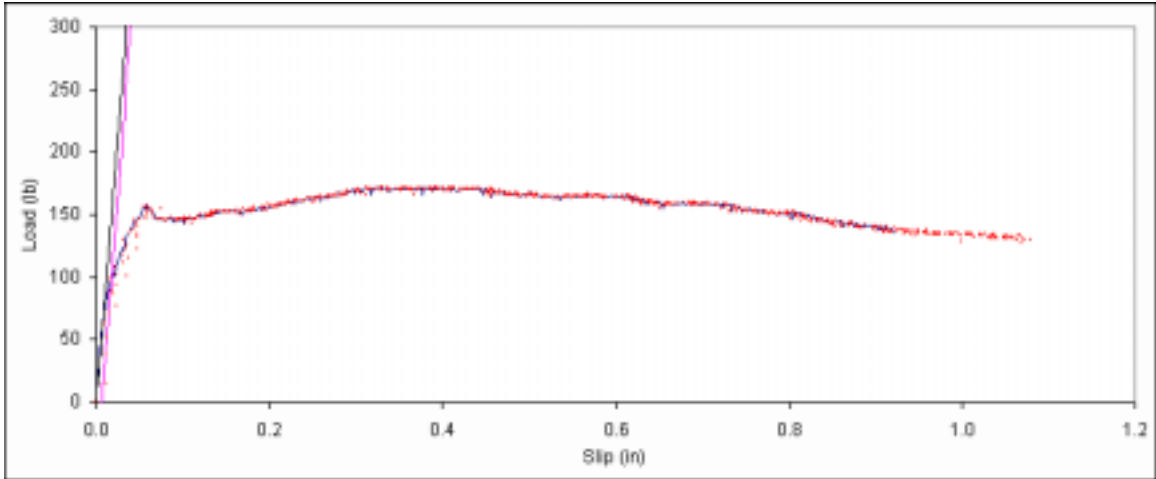
Figure B. 46: Load vs. slip plot for sample A4-2.
