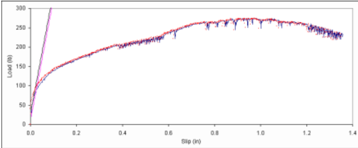
Figure B. 31: Load vs. slip plot for sample A3-2.
