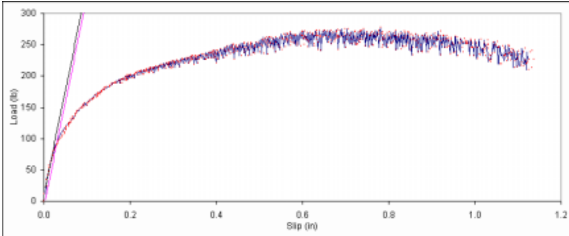
Figure B. 142: Load vs. slip plot for sample B3-10.
