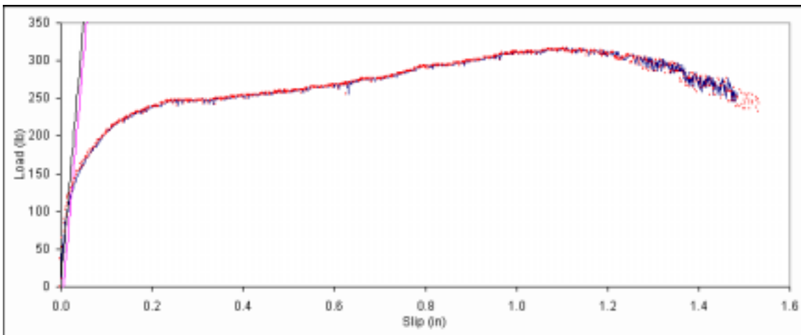
Figure B. 483: Load vs. slip plot for sample E5-8.
