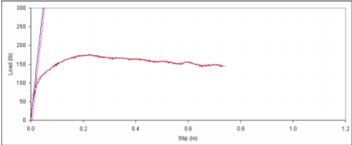
Figure B. 247: Load vs. slip plot for sample C3-11.
