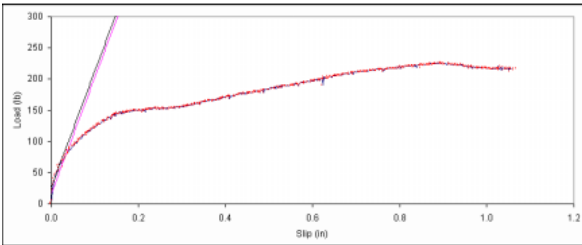
Figure B. 113: Load vs. slip plot for sample B1-11.
