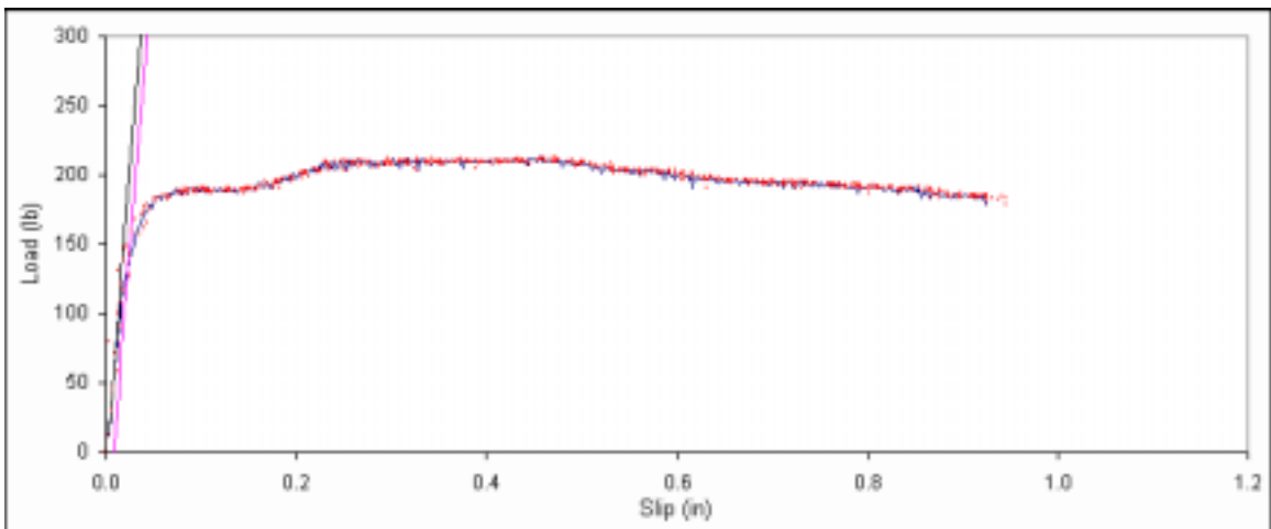
Figure B. 498: Load vs. slip plot for sample E6-9.
