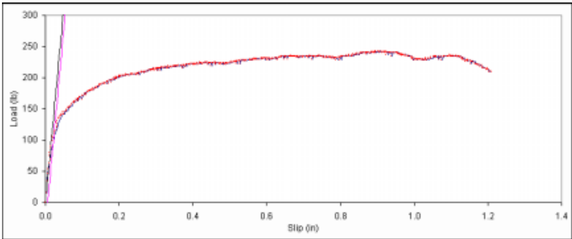
Figure B. 263: Load vs. slip plot for sample C4-12.
