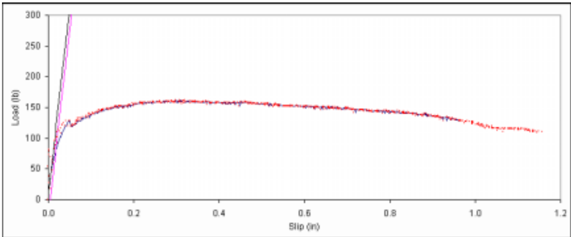
Figure B. 564: Load vs. slip plot for sample F4-2.
