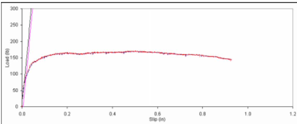
Figure B. 33: Load vs. slip plot for sample A3-4.
