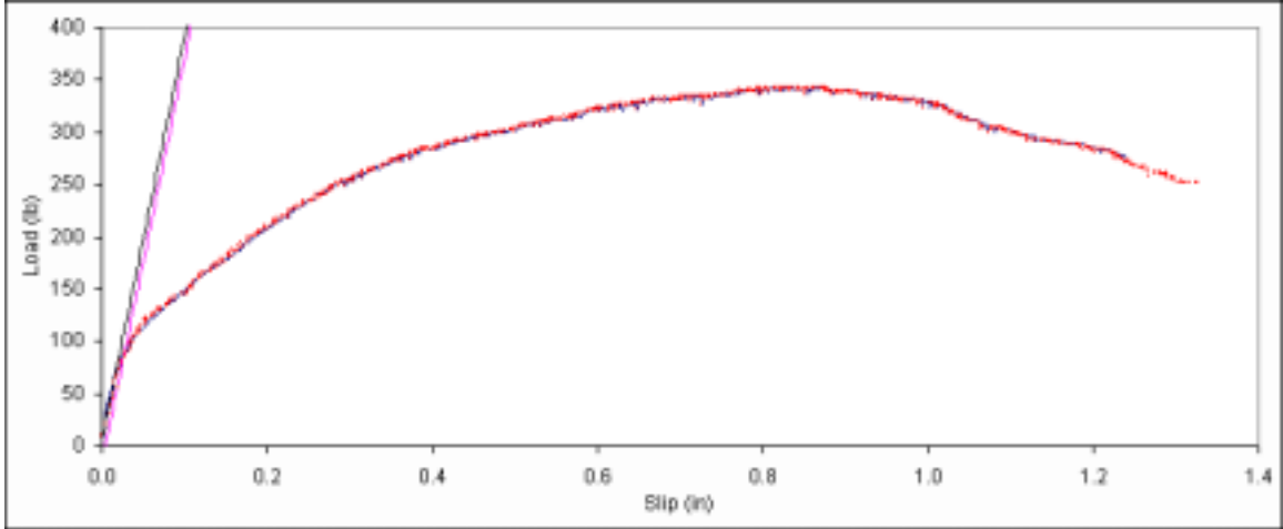
Figure B. 385: Load vs. slip plot for sample D5-15.
