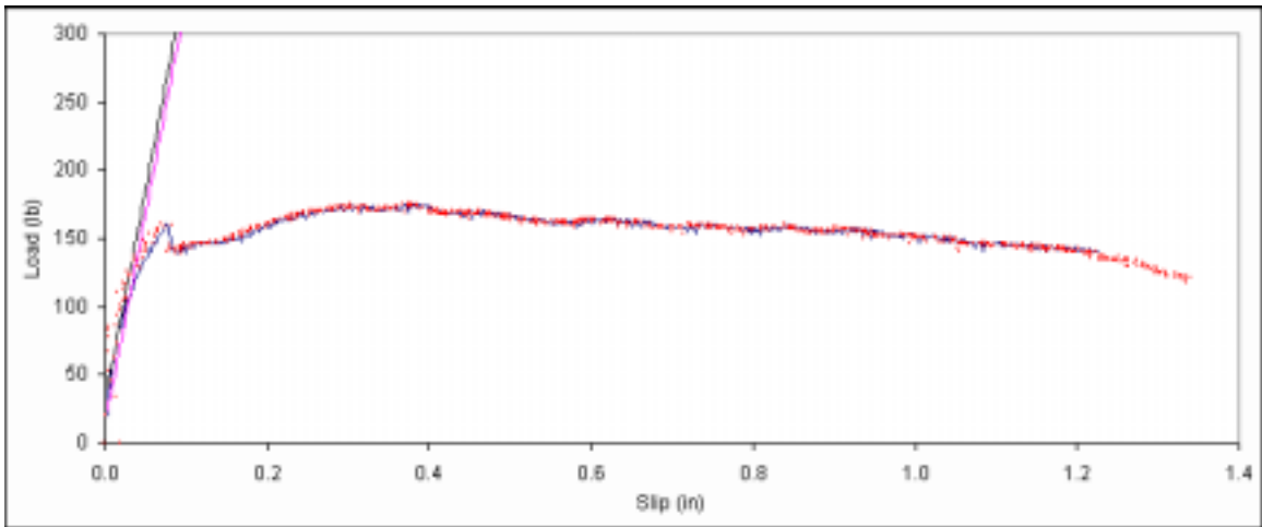
Figure B. 368: Load vs. slip plot for sample D4-13.
