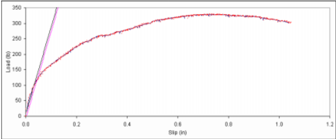
Figure B. 64: Load vs. slip plot for sample A5-5.
