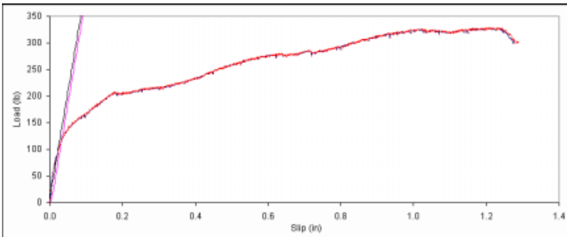
Figure B. 75: Load vs. slip plot for sample A6-1.
