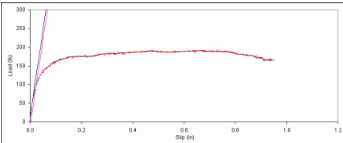
Figure B. 60: Load vs. slip plot for sample A5-1.
