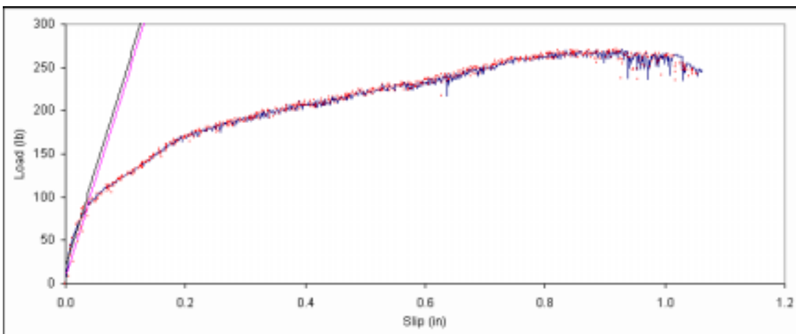
Figure B. 105: Load vs. slip plot for sample B1-3.
