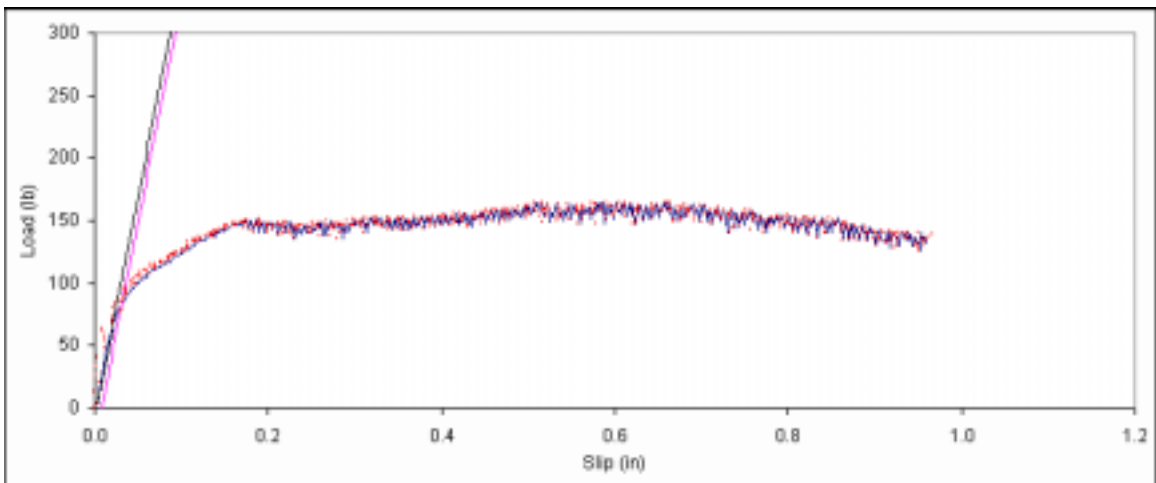
Figure B. 336: Load vs. slip plot for sample D2-11.
