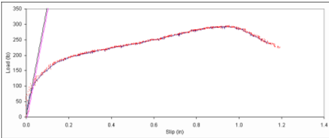
Figure B. 296: Load vs. slip plot for sample C6-15.
