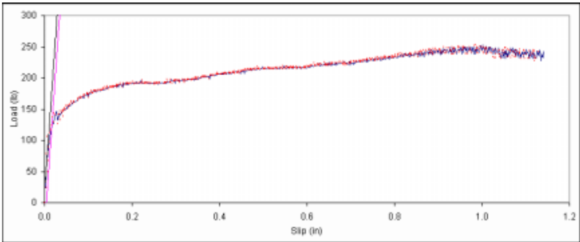
Figure B. 107: Load vs. slip plot for sample B1-5.
