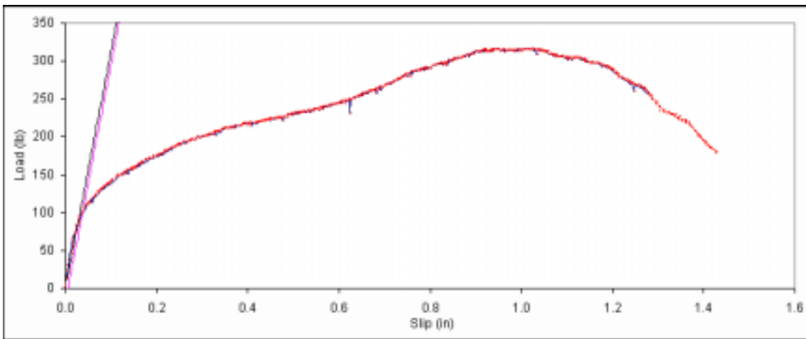
Figure B. 191: Load vs. slip plot for sample B6-14.
