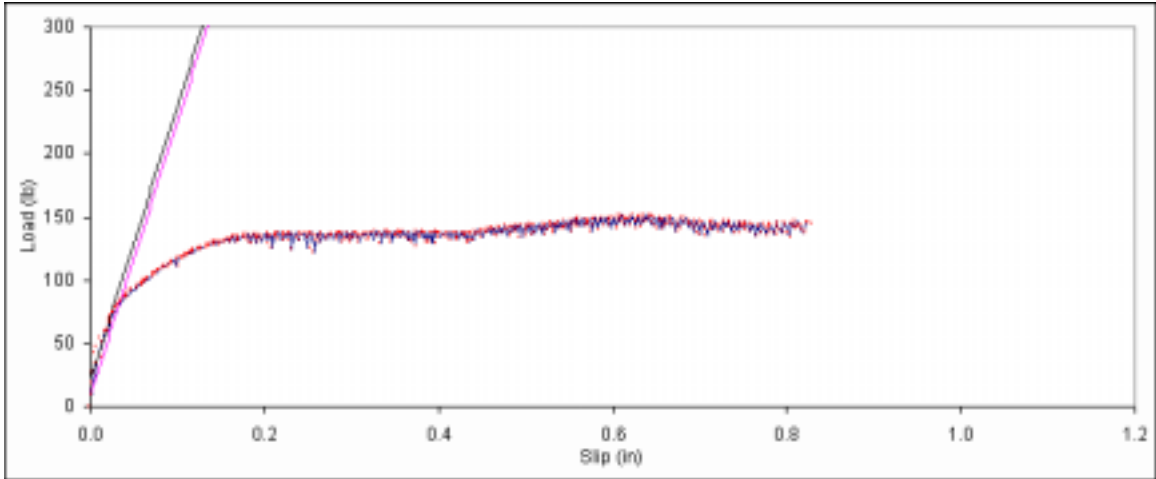
Figure B. 130: Load vs. slip plot for sample B2-13.
