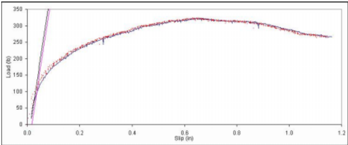
Figure B. 302: Load vs. slip plot for sample C7-6.
