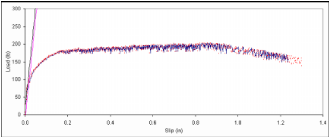
Figure B. 137: Load vs. slip plot for sample B3-5.
