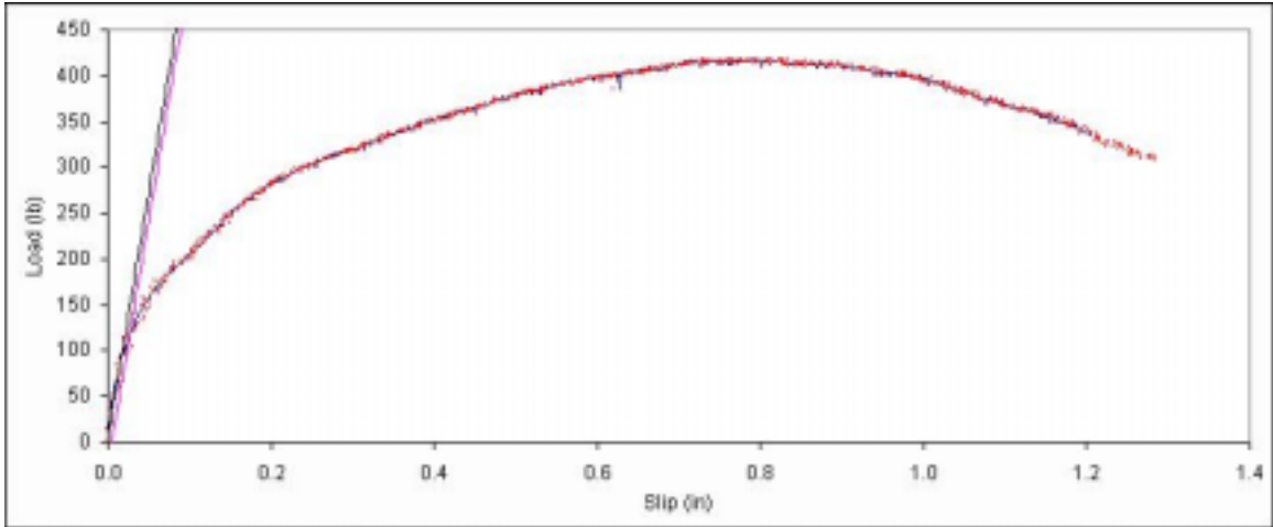
Figure B. 298: Load vs. slip plot for sample C7-2.
