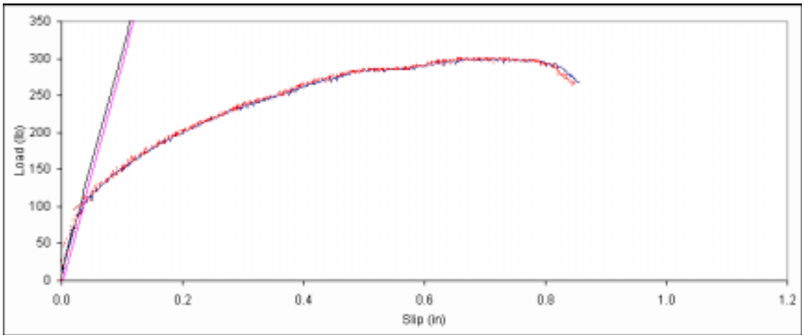
Figure B. 167: Load vs. slip plot for sample B5-5.
