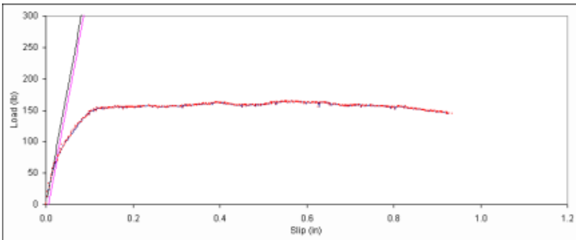
Figure B. 237: Load vs. slip plot for sample C2-15.
