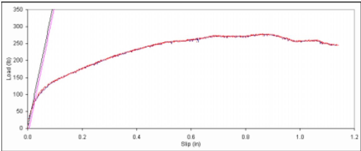
Figure B. 395: Load vs. slip plot for sample D6-10.
