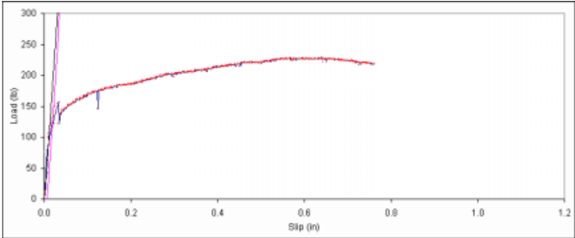
Figure B. 316: Load vs. slip plot for sample D1-5.
