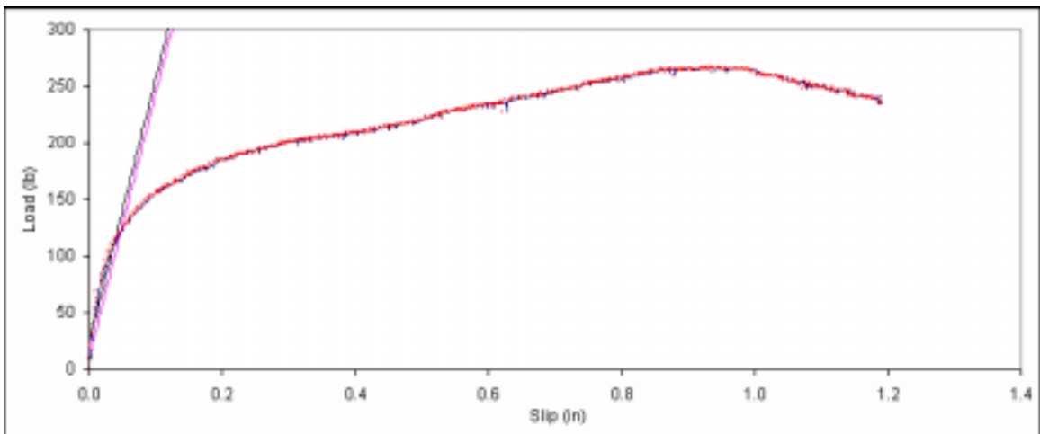
Figure B. 369: Load vs. slip plot for sample D4-14.
