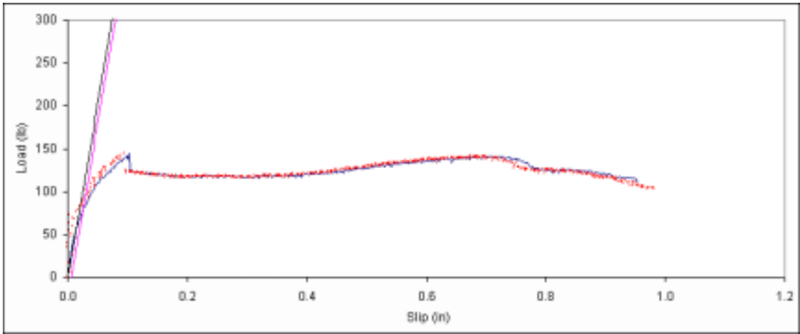
Figure B. 341: Load vs. slip plot for sample D3-1.
