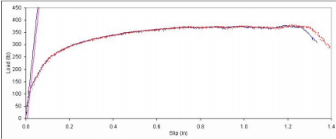
Figure B. 514: Load vs. slip plot for sample E7-10.
