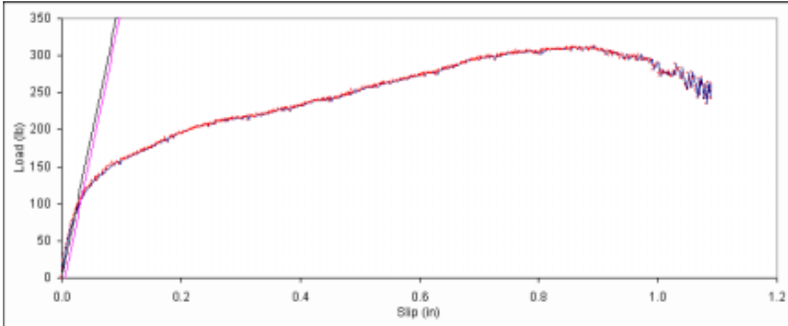
Figure B. 190: Load vs. slip plot for sample B6-13.
