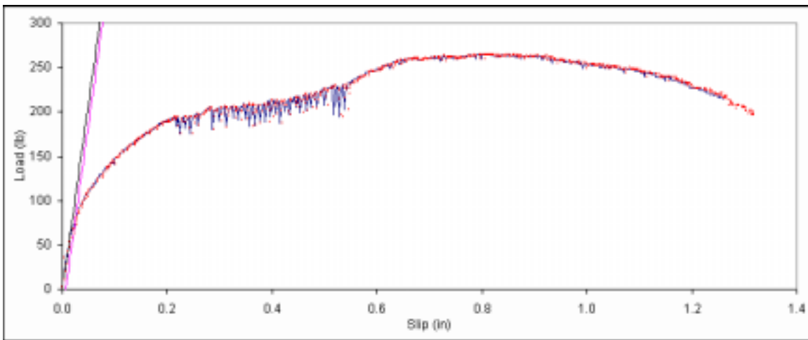
Figure B. 572: Load vs. slip plot for sample F4-10.
