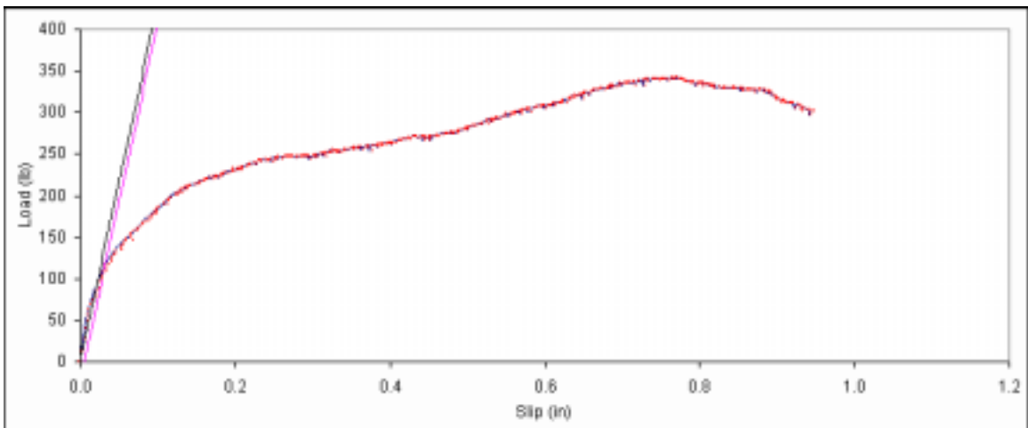
Figure B. 273: Load vs. slip plot for sample C5-7.
