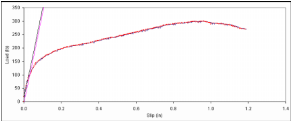
Figure B. 284: Load vs. slip plot for sample C6-3.
