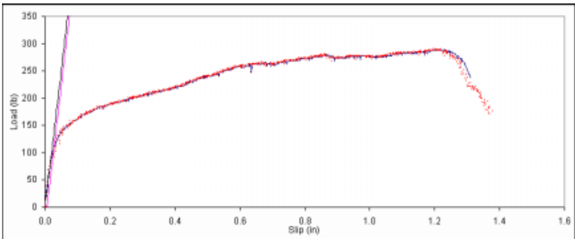
Figure B. 183: Load vs. slip plot for sample B6-6.
