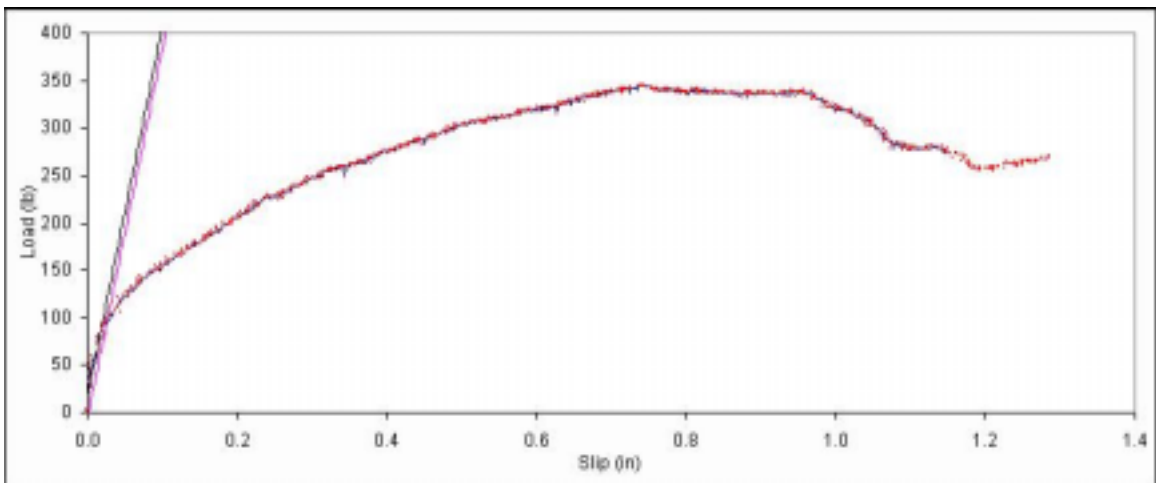
Figure B. 408: Load vs. slip plot for sample D7-8.
