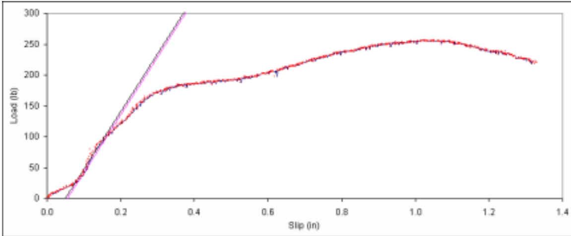
Figure B. 550: Load vs. slip plot for sample F3-3.
