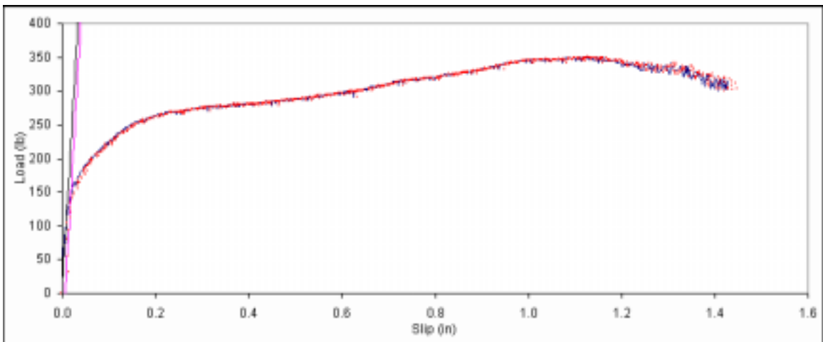
Figure B. 438: Load vs. slip plot for sample E2-8.
