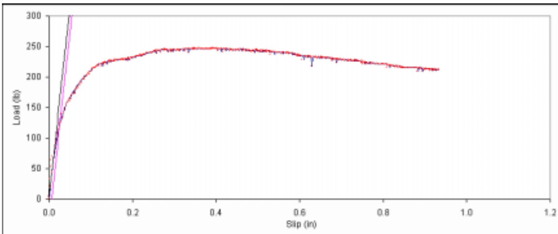
Figure B. 491: Load vs. slip plot for sample E6-1.
