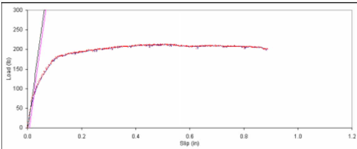
Figure B. 543: Load vs. slip plot for sample F2-10.
