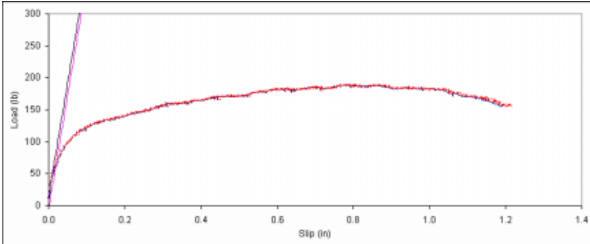
Figure B. 343: Load vs. slip plot for sample D3-3.
