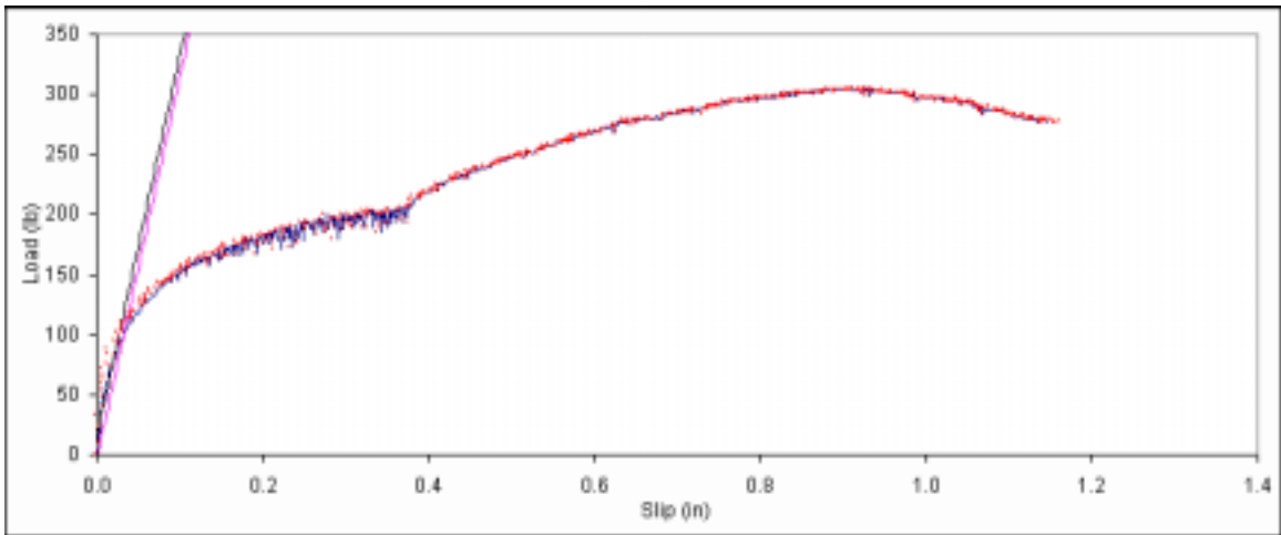
Figure B. 155: Load vs. slip plot for sample B4-8.
