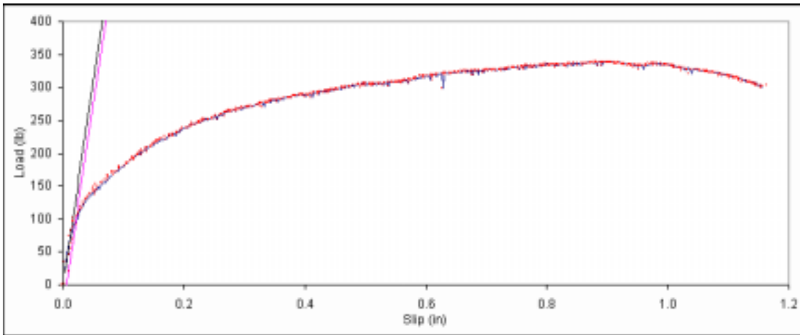
Figure B. 383: Load vs. slip plot for sample D5-13.
