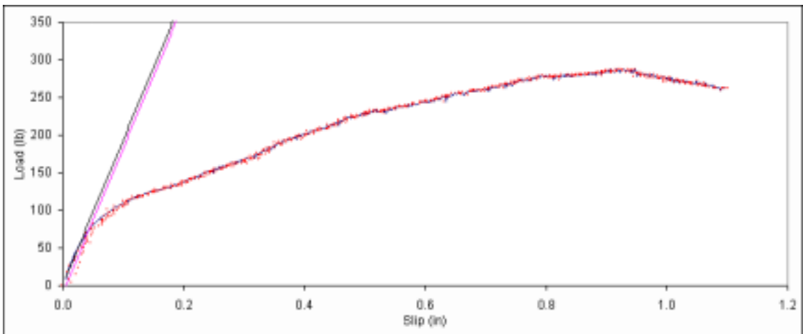
Figure B. 294: Load vs. slip plot for sample C6-13.
