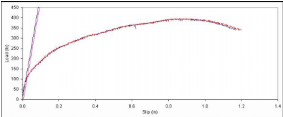
Figure B. 519: Load vs. slip plot for sample E7-15.
