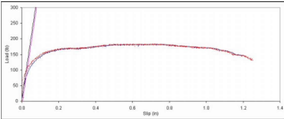
Figure B. 98: Load vs. slip plot for sample A7-10.
