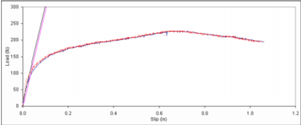
Figure B. 67: Load vs. slip plot for sample A5-8.
