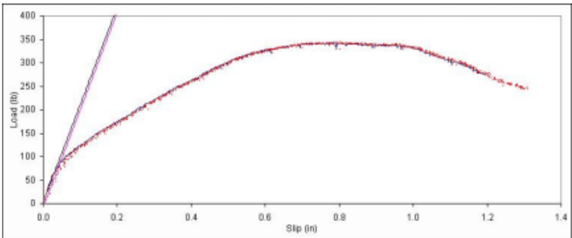
Figure B. 615: Load vs. slip plot for sample F7-8.
