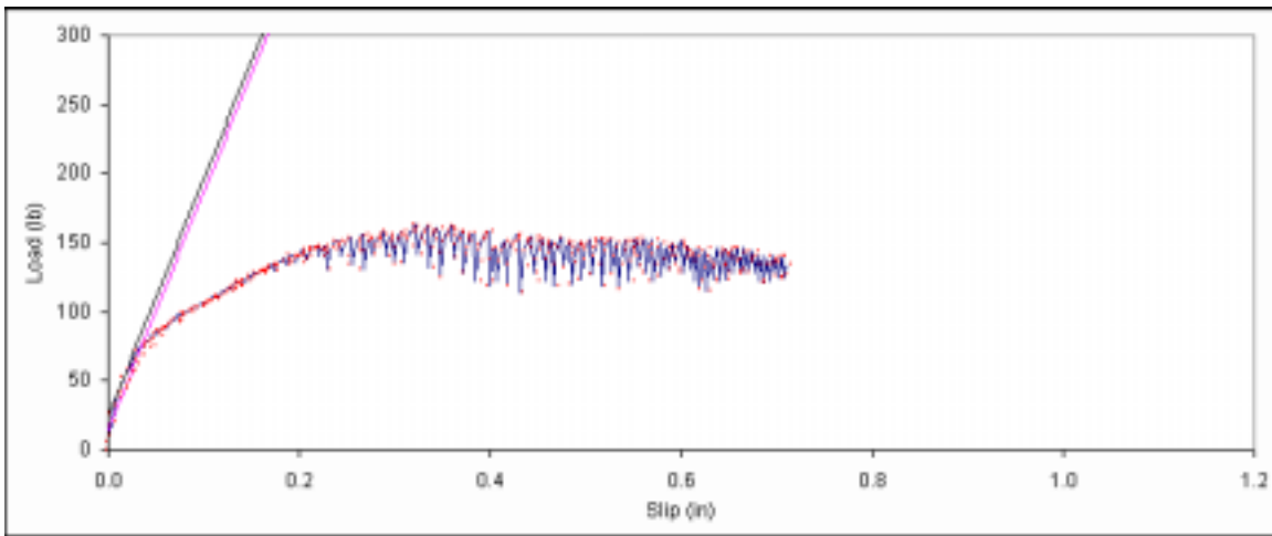
Figure B. 119: Load vs. slip plot for sample B2-2.
