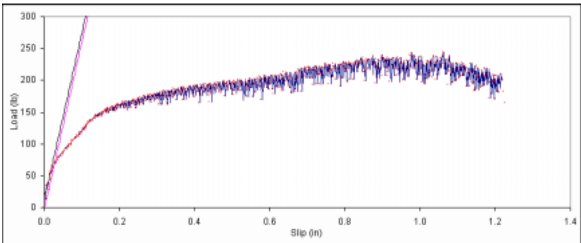
Figure B. 348: Load vs. slip plot for sample D3-8.
