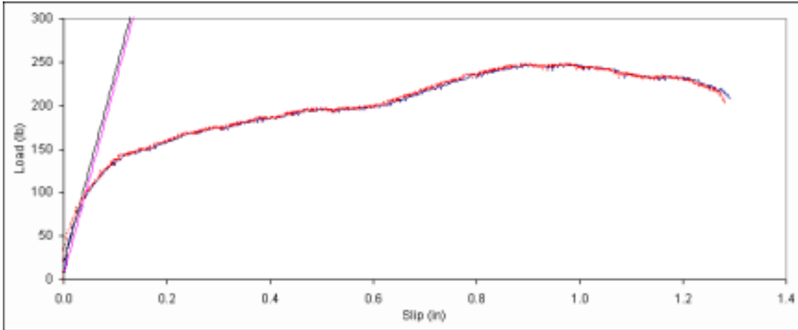
Figure B. 88: Load vs. slip plot for sample A6-15.
