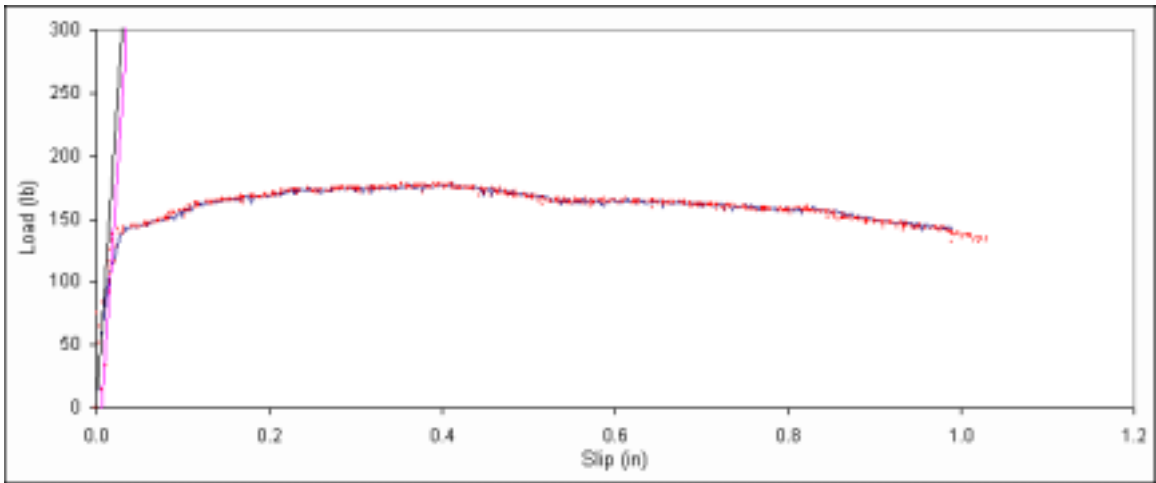
Figure B. 260: Load vs. slip plot for sample C4-9.
