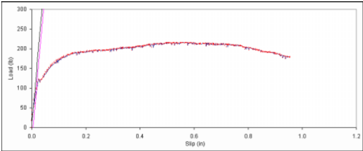
Figure B. 563: Load vs. slip plot for sample F4-1.
