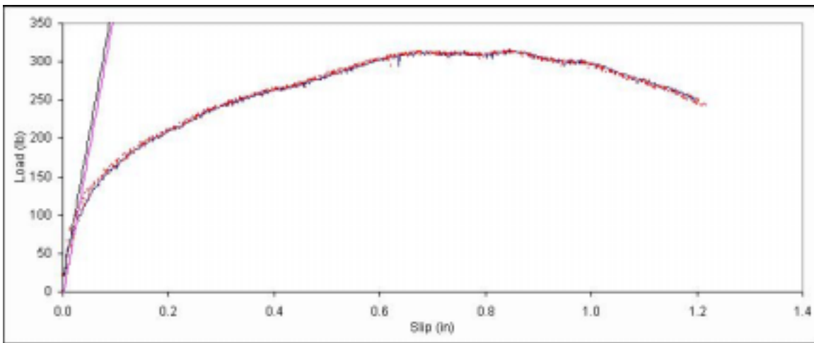
Figure B. 617: Load vs. slip plot for sample F7-10.
