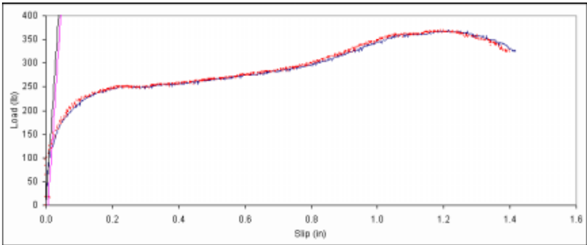
Figure B. 452: Load vs. slip plot for sample E3-7.
