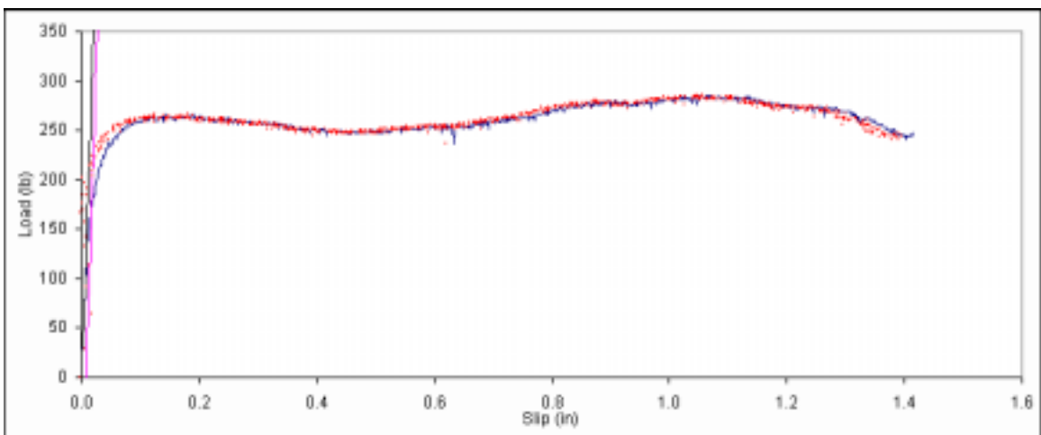
Figure B. 495: Load vs. slip plot for sample E6-6.
