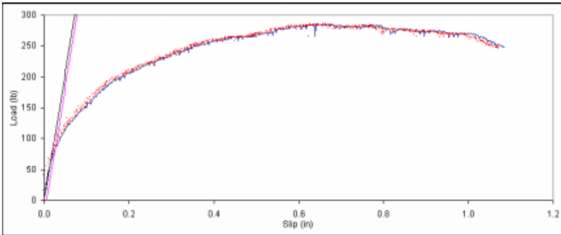
Figure B. 581: Load vs. slip plot for sample F5-4.
