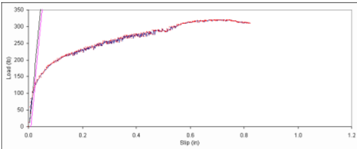
Figure B. 14: Load vs. slip plot for sample A1-15.
