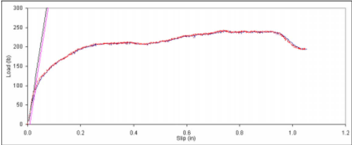
Figure B. 391: Load vs. slip plot for sample D6-6.
