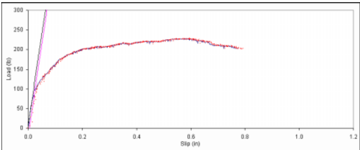
Figure B. 72: Load vs. slip plot for sample A5-13.
