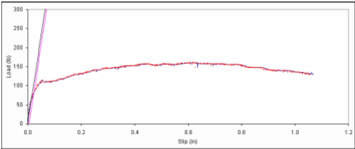
Figure B. 332: Load vs. slip plot for sample D2-7.
