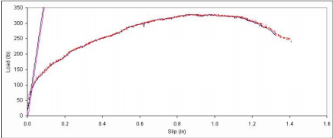
Figure B. 403: Load vs. slip plot for sample D7-3.
