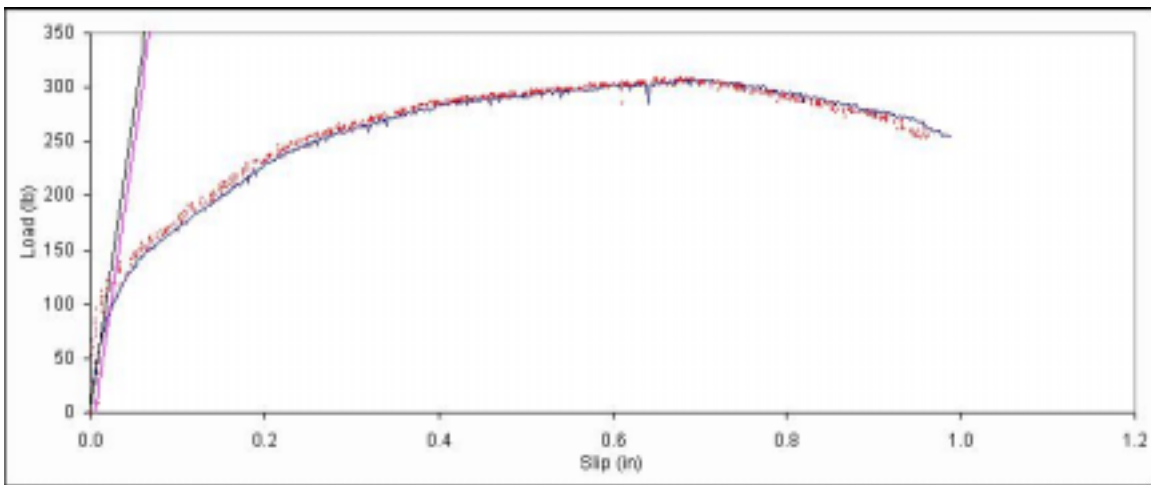
Figure B. 620: Load vs. slip plot for sample F7-13.
