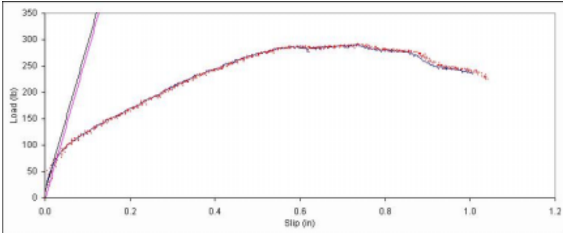
Figure B. 412: Load vs. slip plot for sample D7-12.
