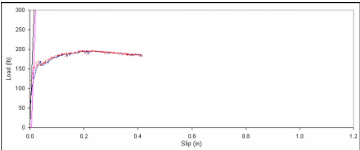
Figure B. 528: Load vs. slip plot for sample F1-9.
