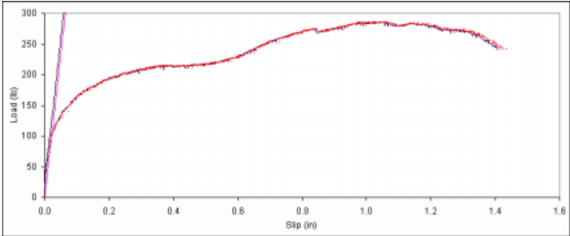
Figure B. 139: Load vs. slip plot for sample B3-7.
