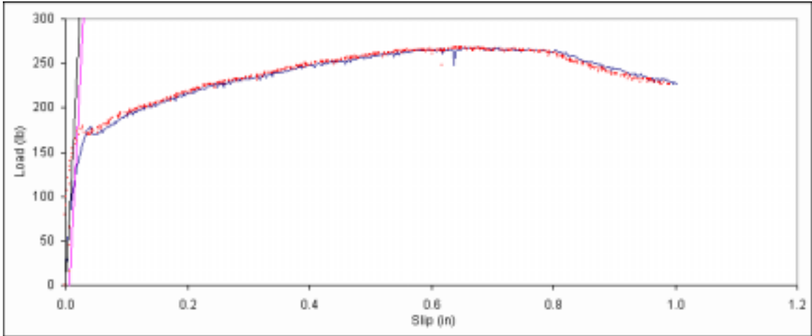
Figure B. 280: Load vs. slip plot for sample C5-14.
