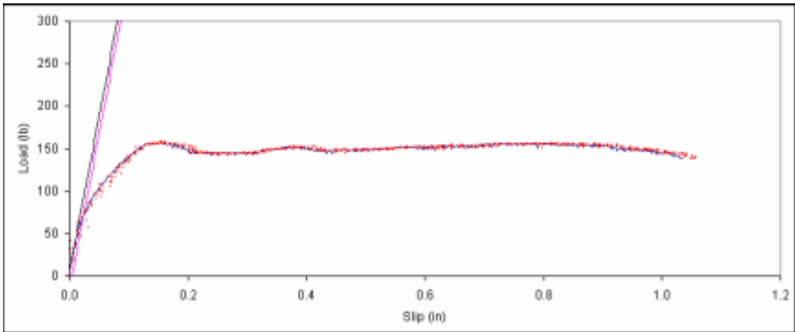
Figure B. 188: Load vs. slip plot for sample B6-11.
