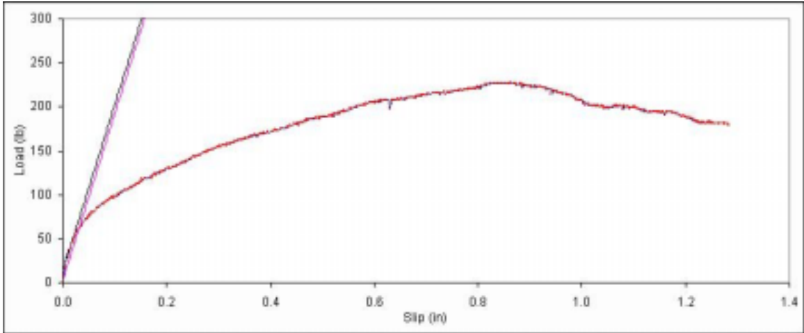
Figure B. 205: Load vs. slip plot for sample B7-13.
