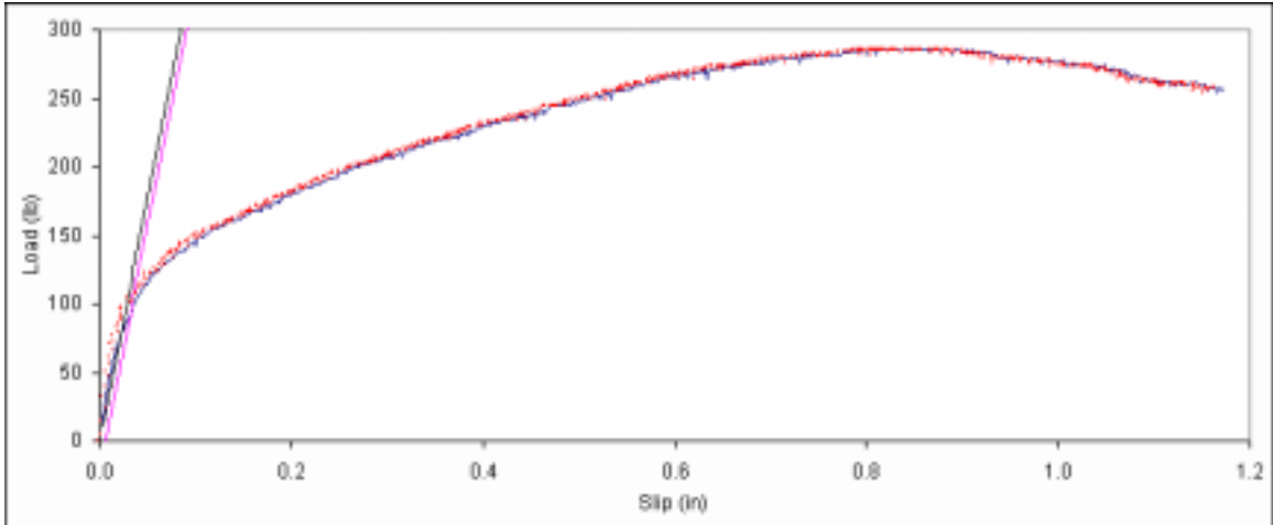
Figure B. 184: Load vs. slip plot for sample B6-7.
