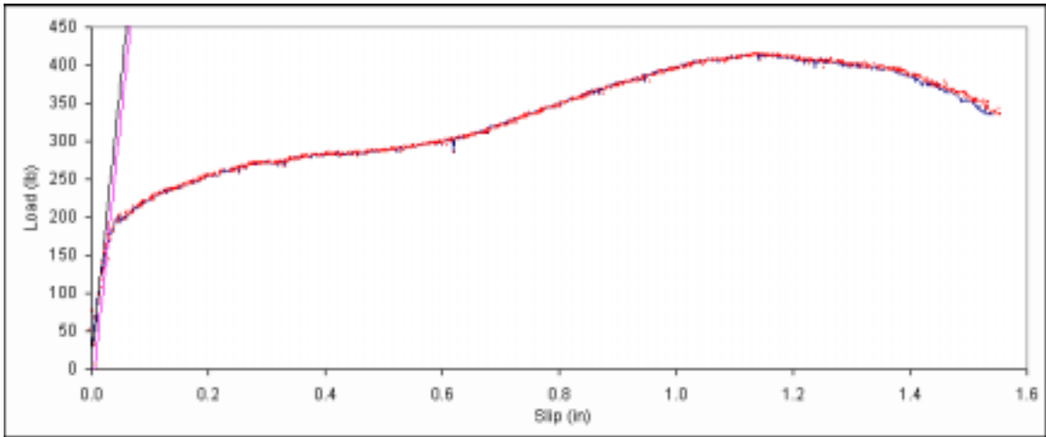
Figure B. 446: Load vs. slip plot for sample E3-1.
