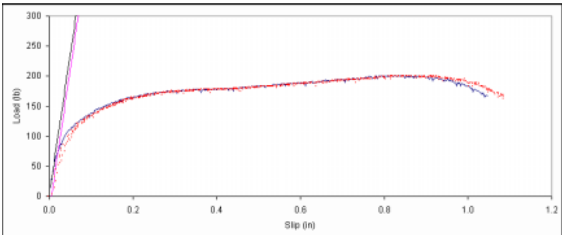
Figure B. 558: Load vs. slip plot for sample F3-11.
