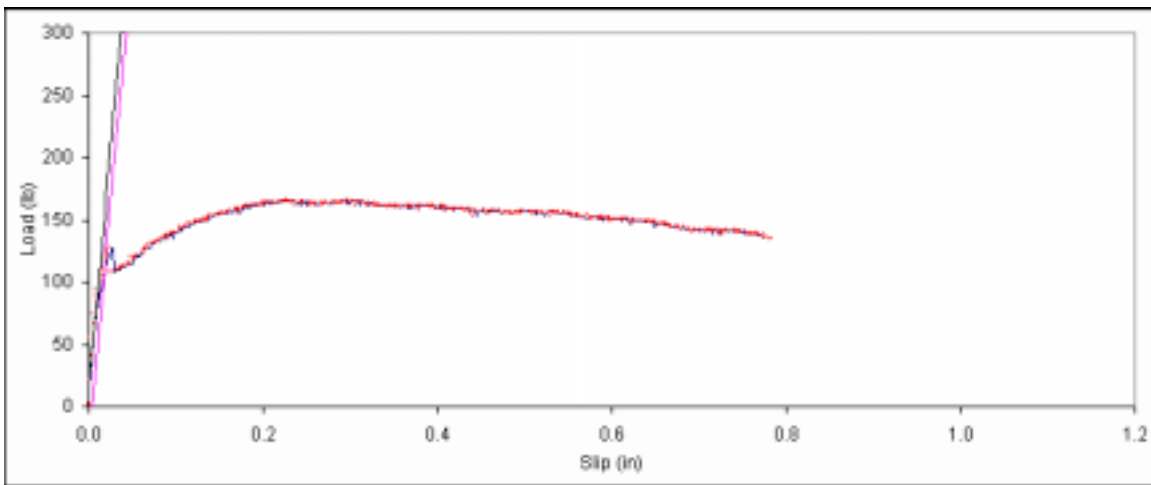
Figure B. 152: Load vs. slip plot for sample B4-5.
