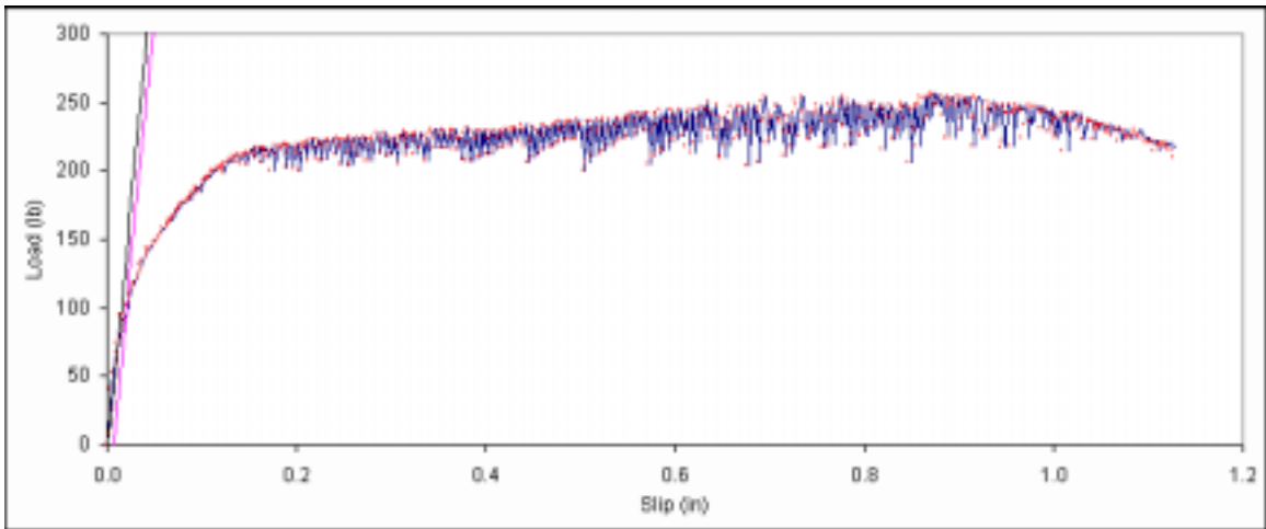
Figure B. 224: Load vs. slip plot for sample C2-2.
