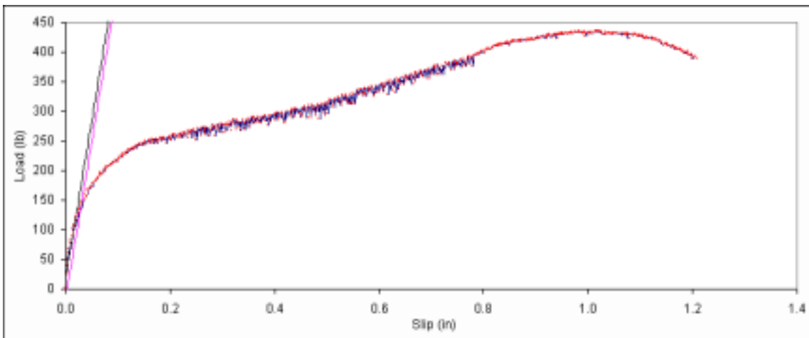
Figure B. 489: Load vs. slip plot for sample E5-14.
