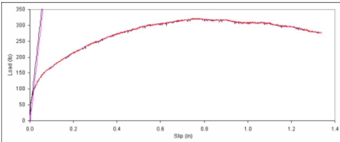
Figure B. 30: Load vs. slip plot for sample A3-1.
