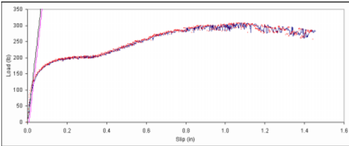
Figure B. 467: Load vs. slip plot for sample E4-7.
