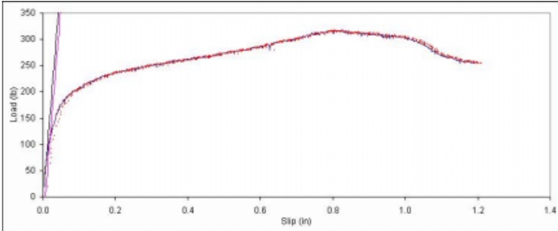
Figure B. 202: Load vs. slip plot for sample B7-10.
