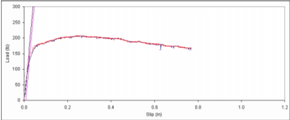
Figure B. 22: Load vs. slip plot for sample A2-8.
