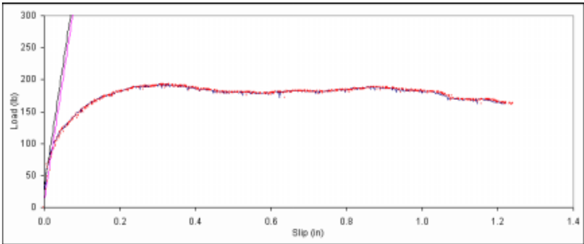
Figure B. 140: Load vs. slip plot for sample B3-8.
