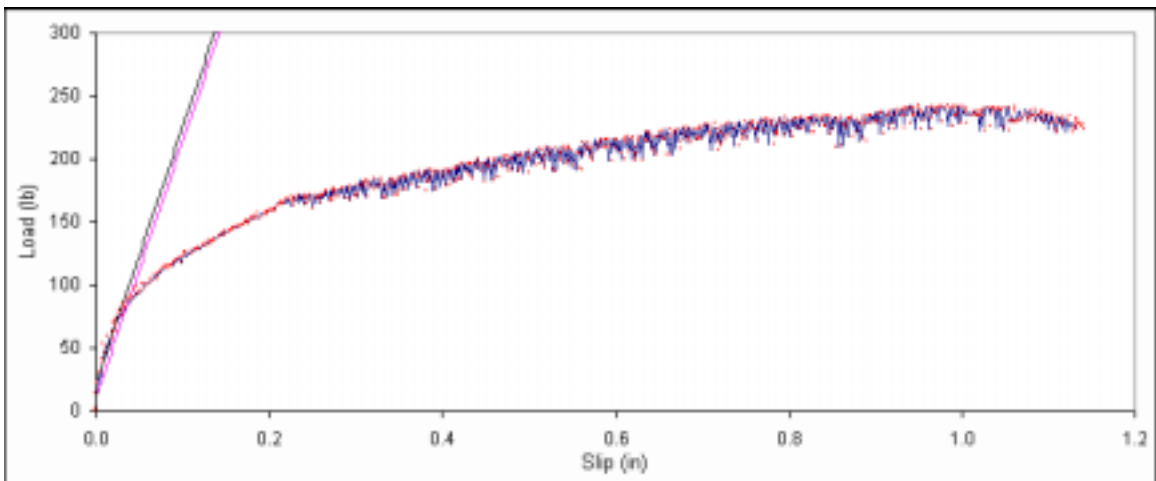
Figure B. 111: Load vs. slip plot for sample B1-9.
