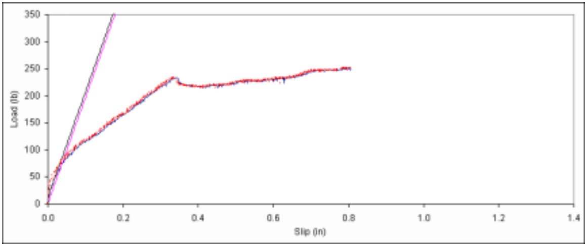
Figure B. 314: Load vs. slip plot for sample D1-3.
