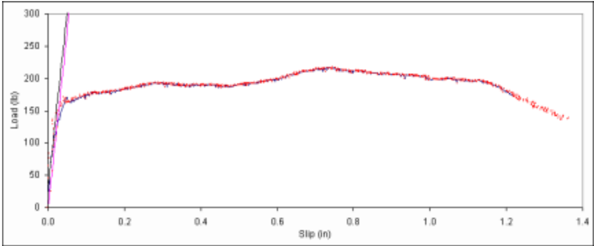
Figure B. 370: Load vs. slip plot for sample D4-15.
