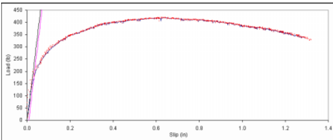
Figure B. 459: Load vs. slip plot for sample E3-14.
