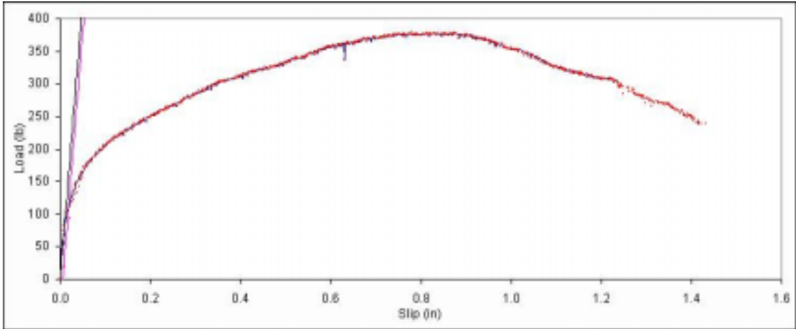
Figure B. 304: Load vs. slip plot for sample C7-8.
