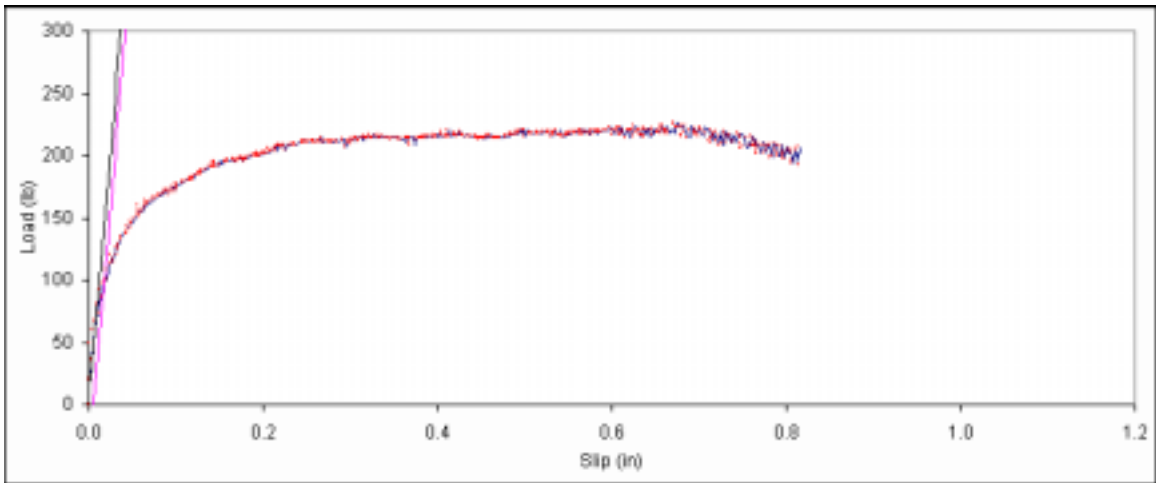
Figure B. 212: Load vs. slip plot for sample C1-5.
