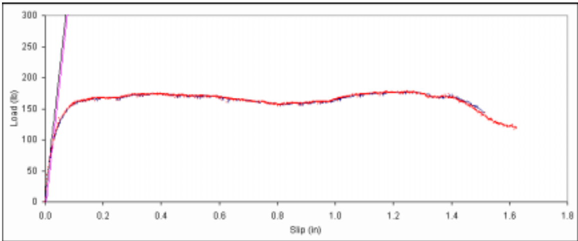
Figure B. 80: Load vs. slip plot for sample A6-7.
