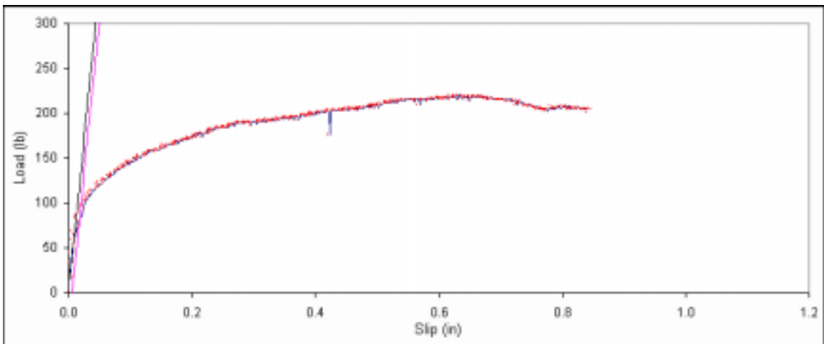
Figure B. 231: Load vs. slip plot for sample C2-9.
