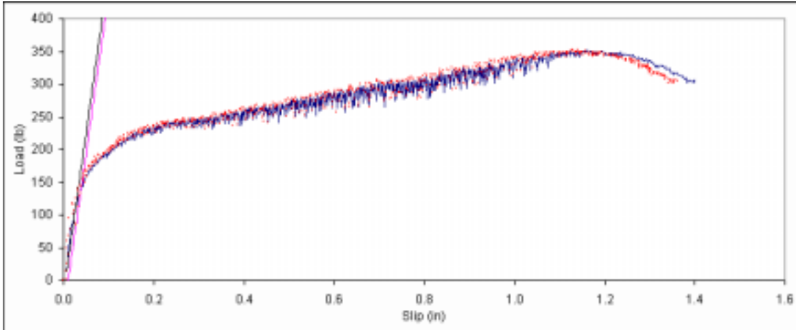
Figure B. 475: Load vs. slip plot for sample E4-15.
