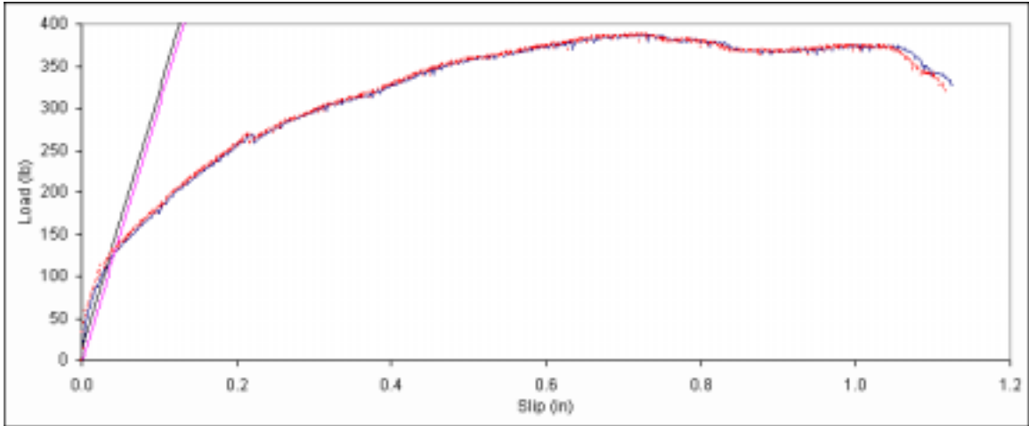
Figure B. 85: Load vs. slip plot for sample A6-12.
