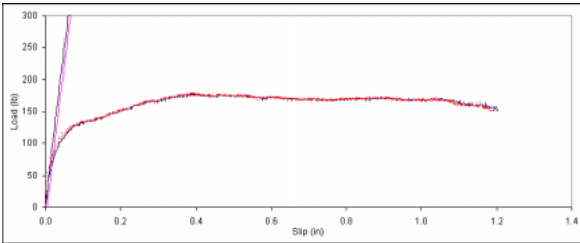
Figure B. 374: Load vs. slip plot for sample D5-4.
