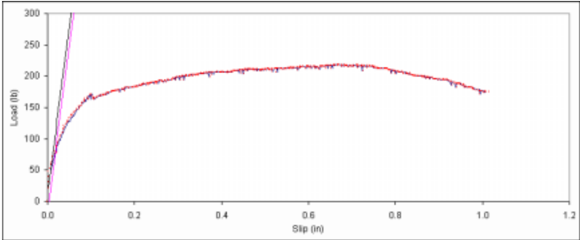
Figure B. 565: Load vs. slip plot for sample F4-3.
