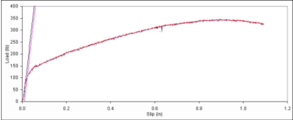
Figure B. 319: Load vs. slip plot for sample D1-8.
