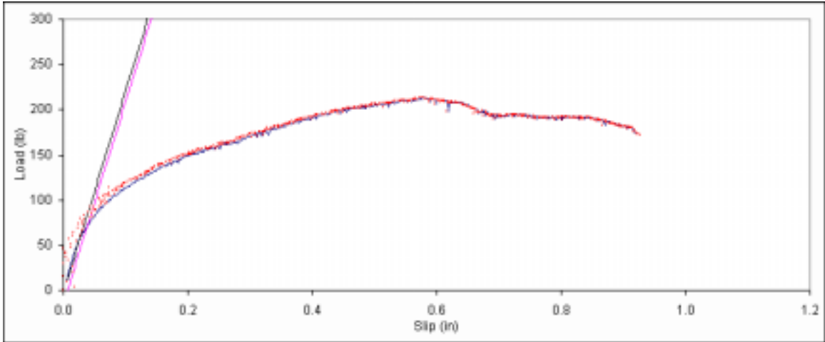
Figure B. 187: Load vs. slip plot for sample B6-10.
