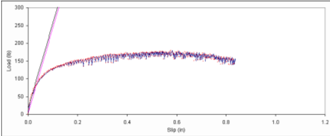
Figure B. 16: Load vs. slip plot for sample A2-2.
