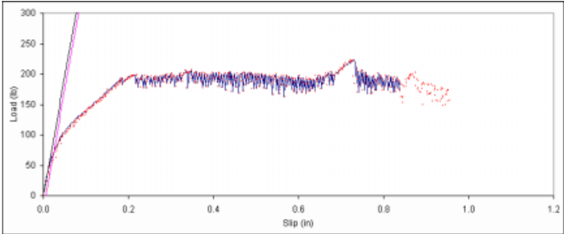
Figure B. 538: Load vs. slip plot for sample F2-5.
