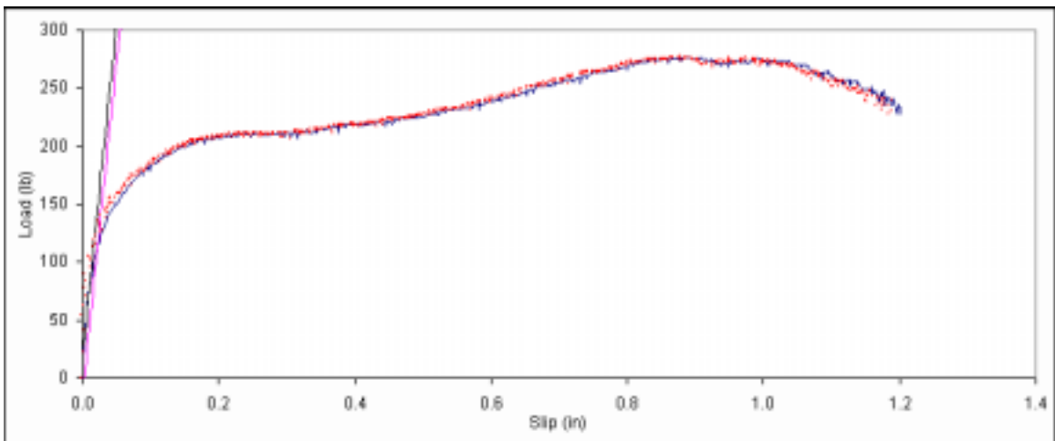
Figure B. 63: Load vs. slip plot for sample A5-4.
