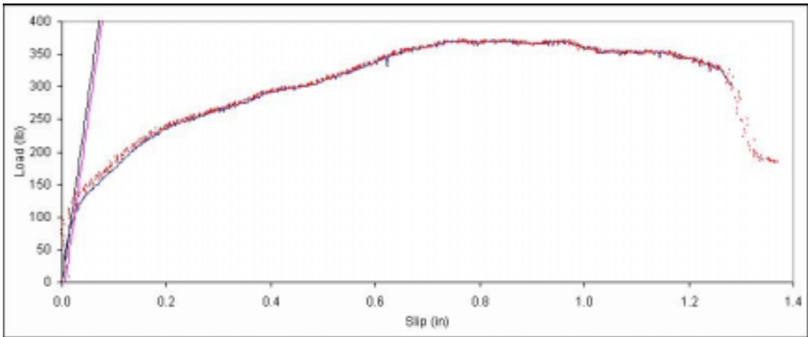
Figure B. 197: Load vs. slip plot for sample B7-5.
