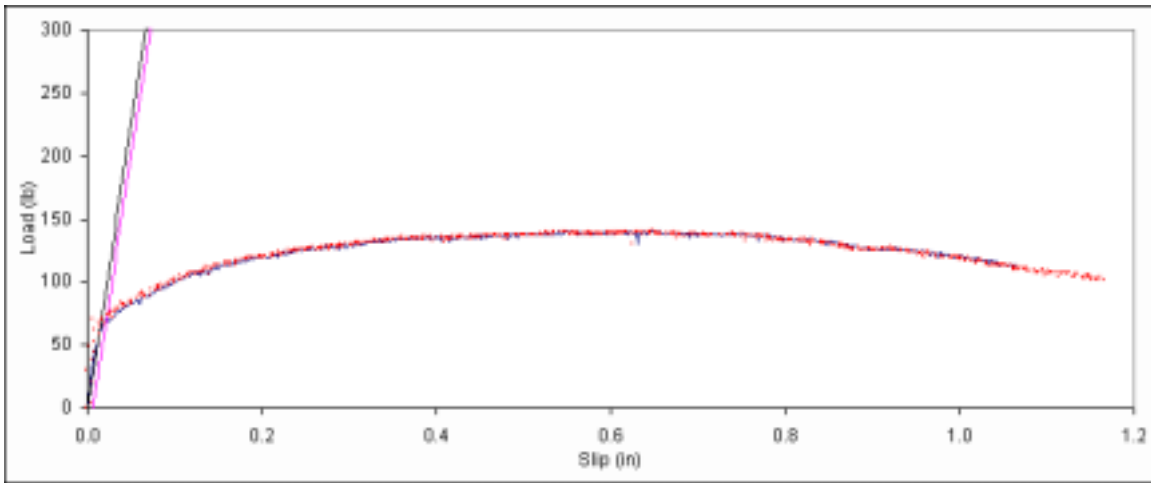
Figure B. 44: Load vs. slip plot for sample A3-15.
