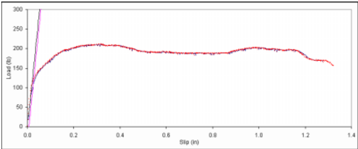
Figure B. 83: Load vs. slip plot for sample A6-10.
