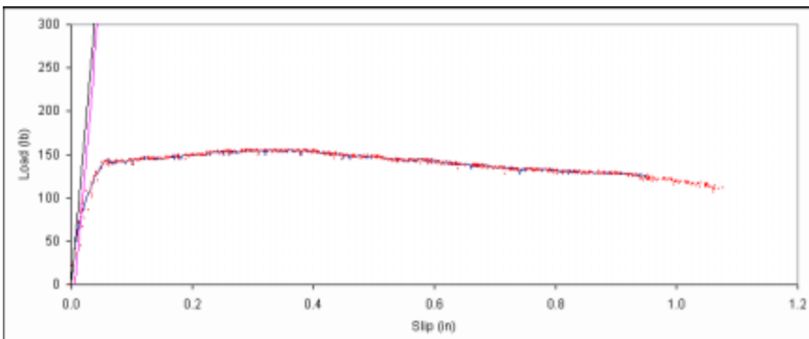
Figure B. 573: Load vs. slip plot for sample F4-11.
