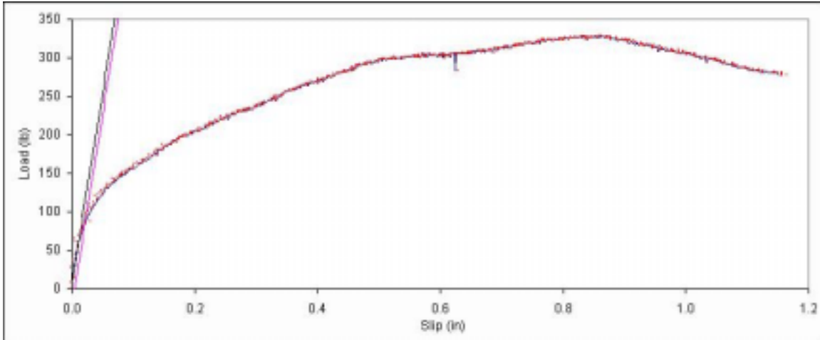
Figure B. 193: Load vs. slip plot for sample B7-1.
