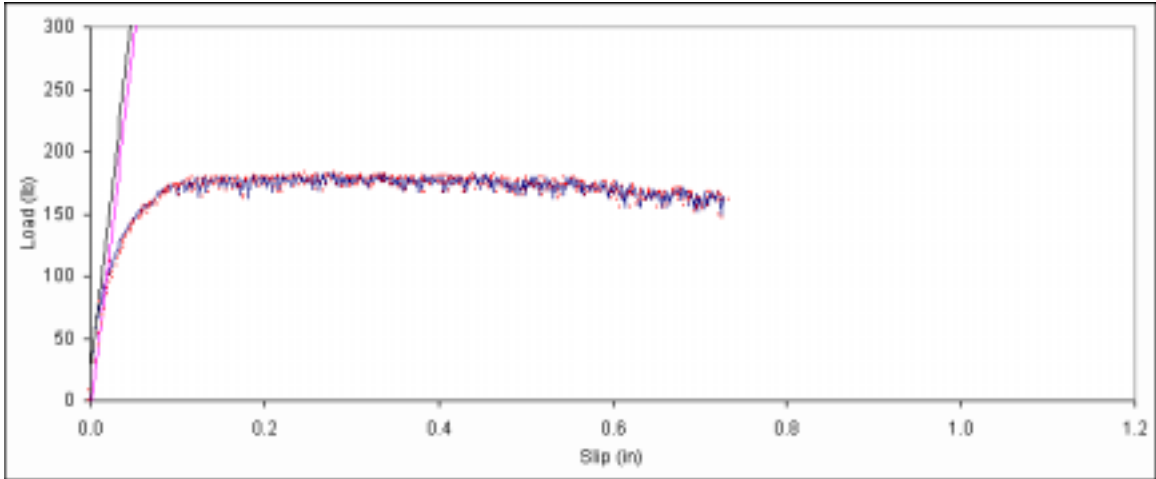
Figure B. 124: Load vs. slip plot for sample B2-7.
