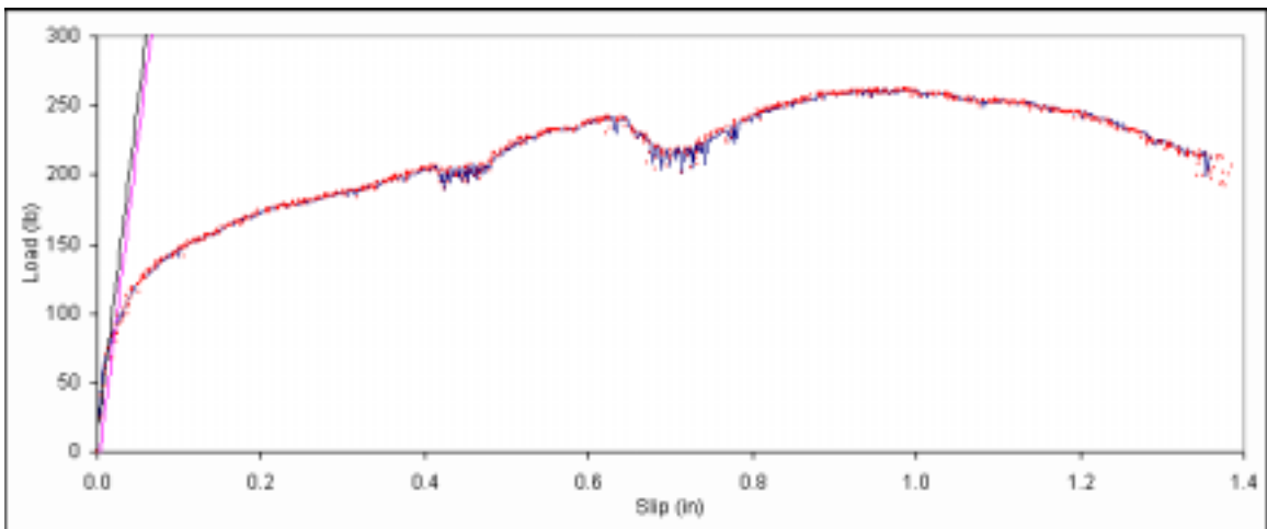
Figure B. 246: Load vs. slip plot for sample C3-10.
