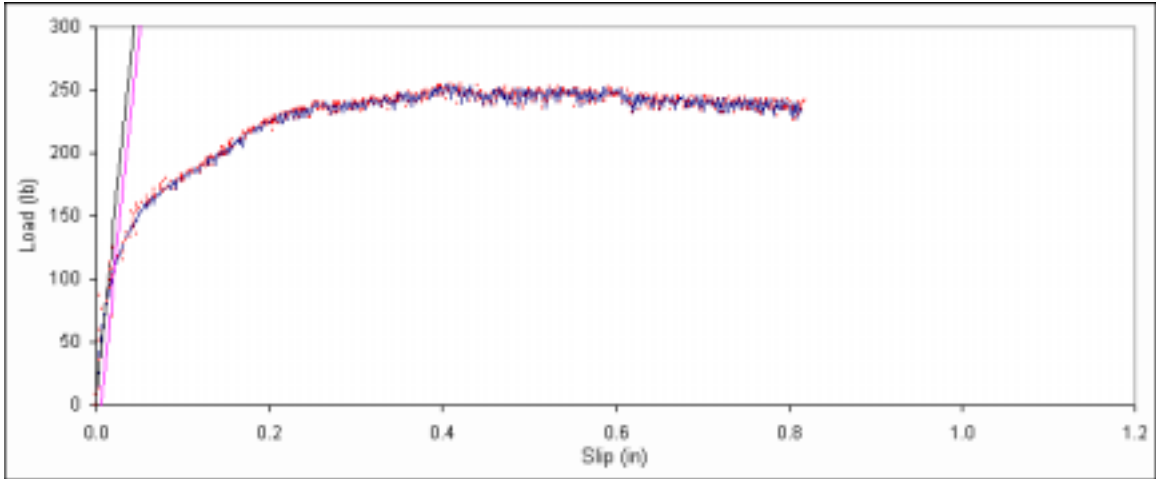
Figure B. 424: Load vs. slip plot for sample E1-9.
