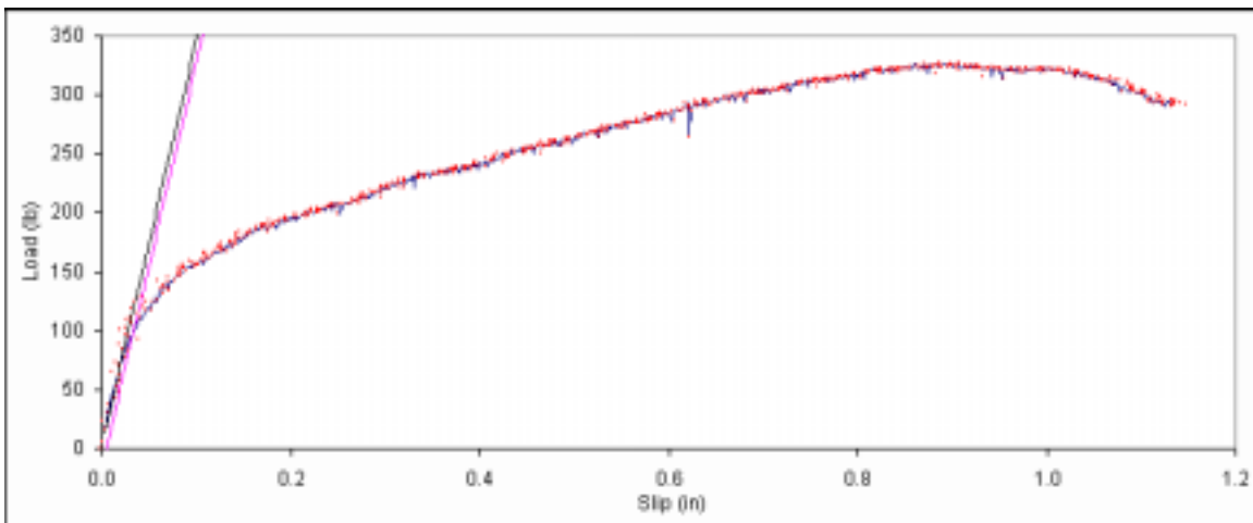
Figure B. 606: Load vs. slip plot for sample F6-14.
