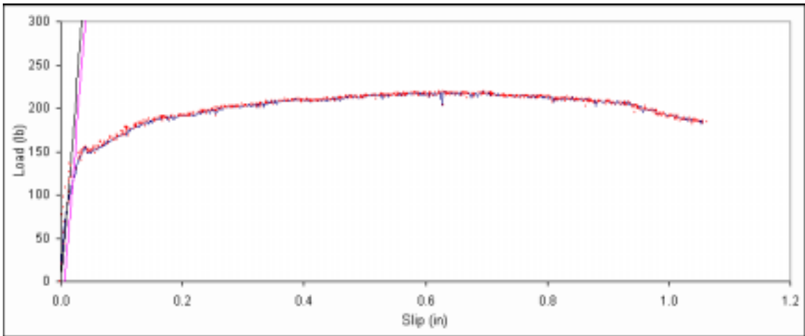
Figure B. 53: Load vs. slip plot for sample A4-9.
