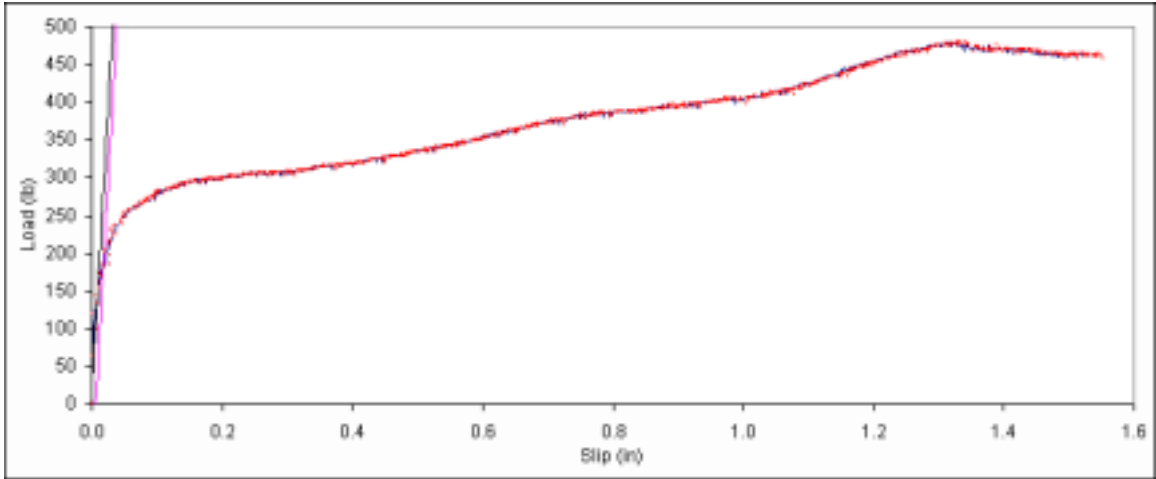
Figure B. 445: Load vs. slip plot for sample E2-15.
