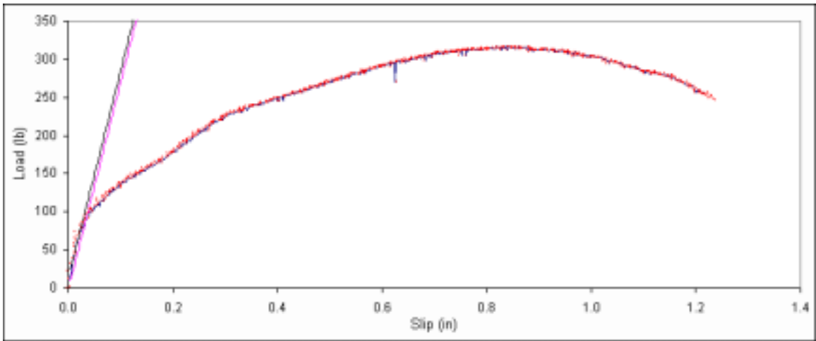
Figure B. 38: Load vs. slip plot for sample A3-9.
