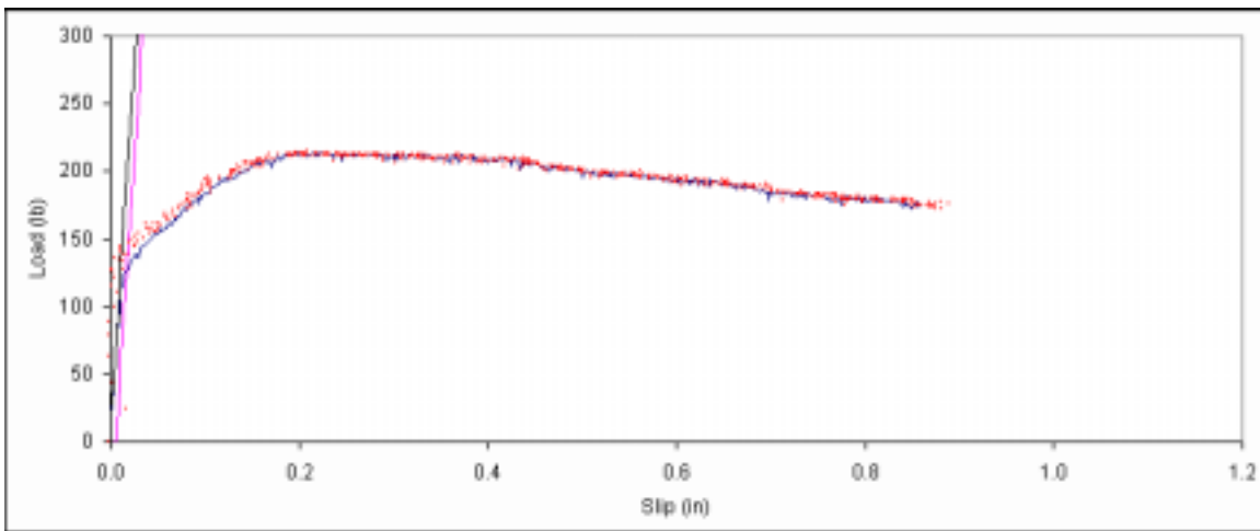
Figure B. 500: Load vs. slip plot for sample E6-11.
