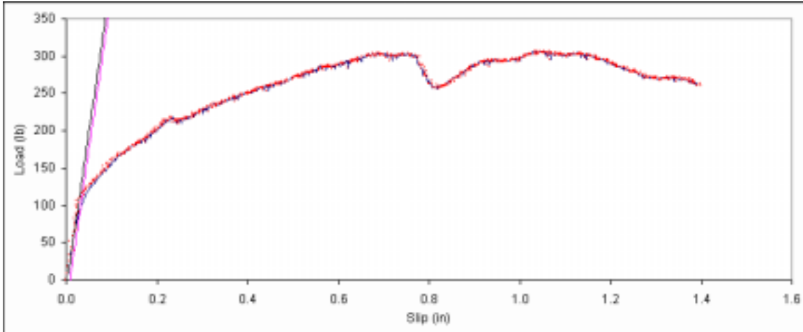
Figure B. 580: Load vs. slip plot for sample F5-3.
