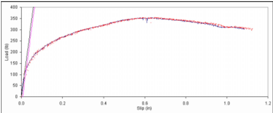
Figure B. 255: Load vs. slip plot for sample C4-4.
