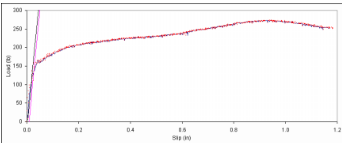
Figure B. 57: Load vs. slip plot for sample A4-13.
