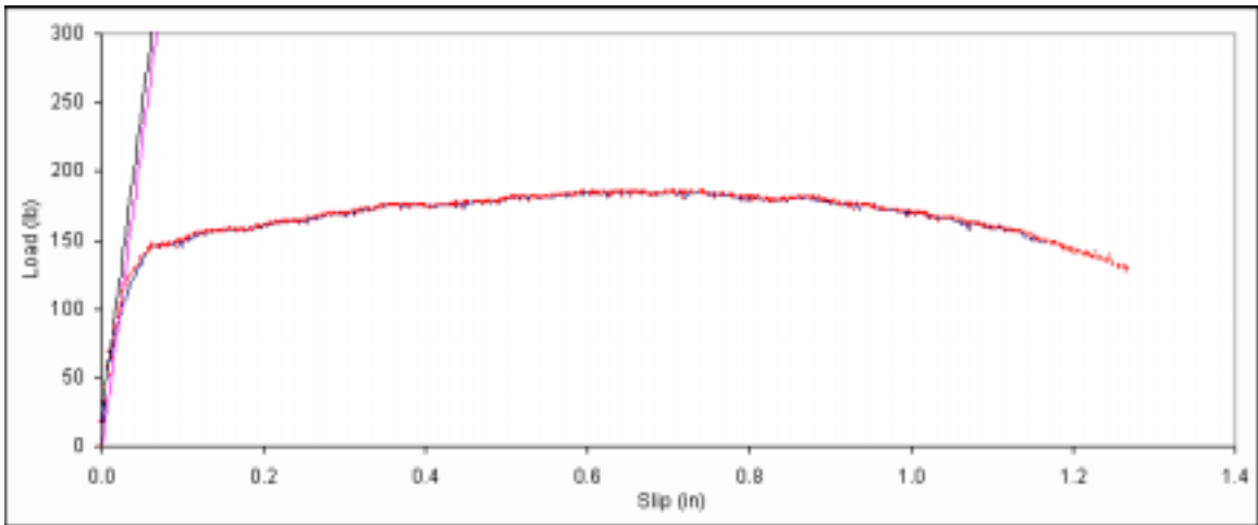
Figure B. 161: Load vs. slip plot for sample B4-14.
