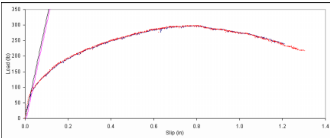
Figure B. 585: Load vs. slip plot for sample F5-8.
