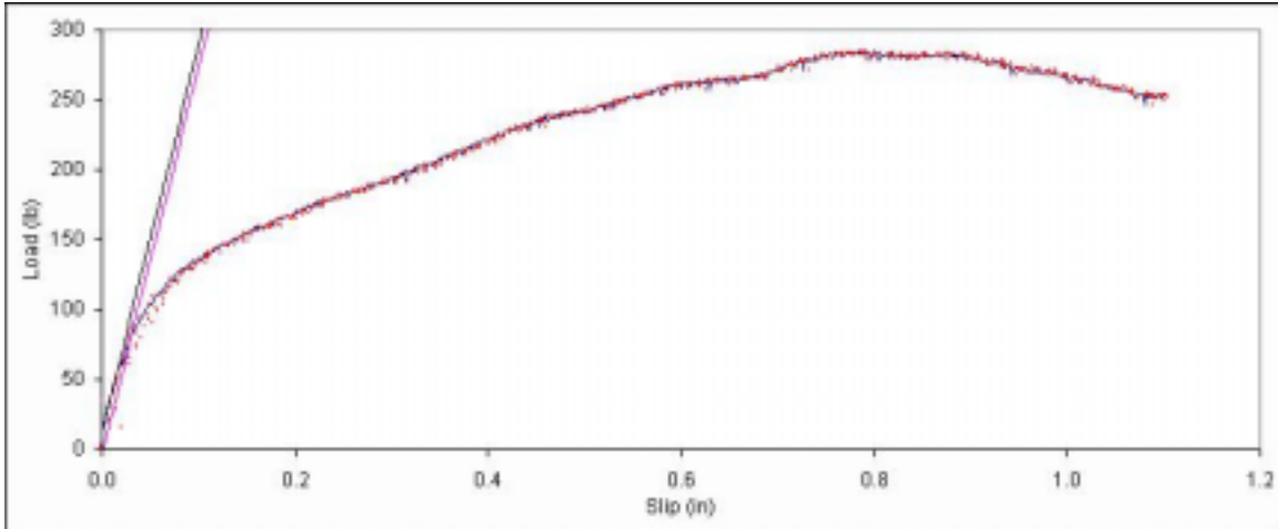
Figure B. 619: Load vs. slip plot for sample F7-12.
