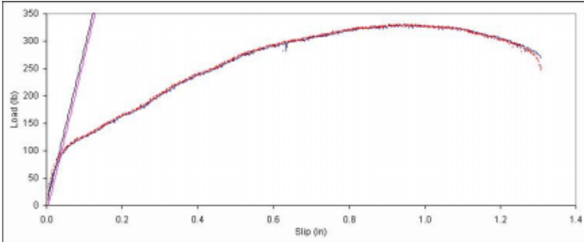
Figure B. 415: Load vs. slip plot for sample D7-15.
