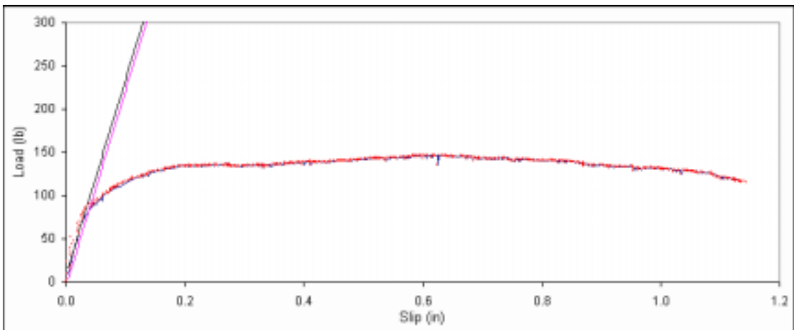
Figure B. 141: Load vs. slip plot for sample B3-9.
