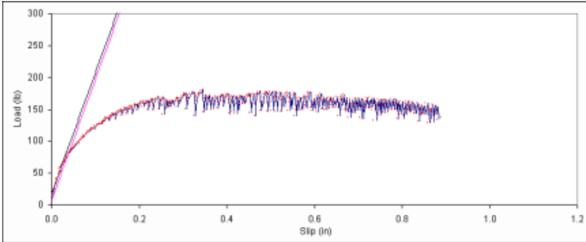
Figure B. 118: Load vs. slip plot for sample B2-1.
