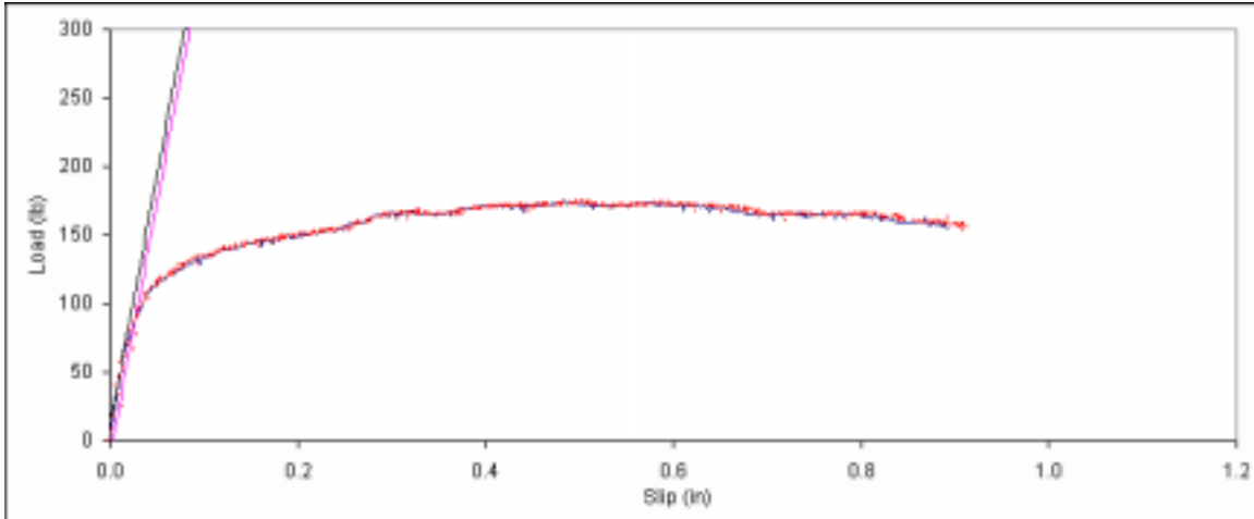
Figure B. 163: Load vs. slip plot for sample B5-1.
