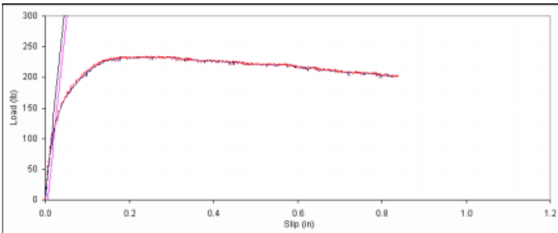
Figure B. 474: Load vs. slip plot for sample E4-14.
