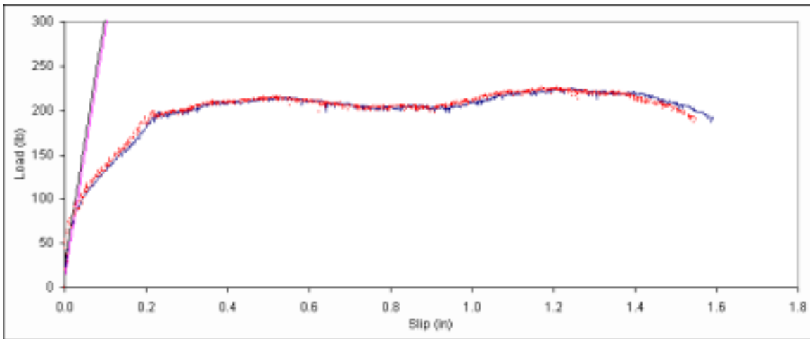
Figure B. 59: Load vs. slip plot for sample A4-15.
