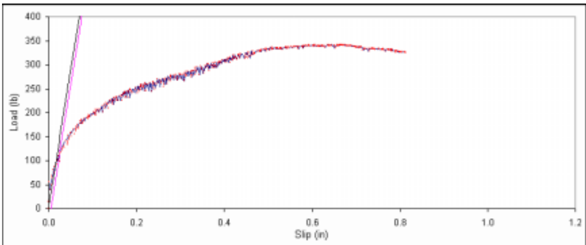
Figure B. 216: Load vs. slip plot for sample C1-9.
