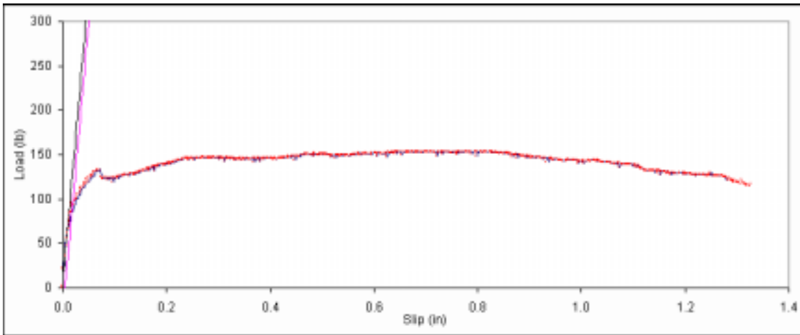
Figure B. 35: Load vs. slip plot for sample A3-6.
