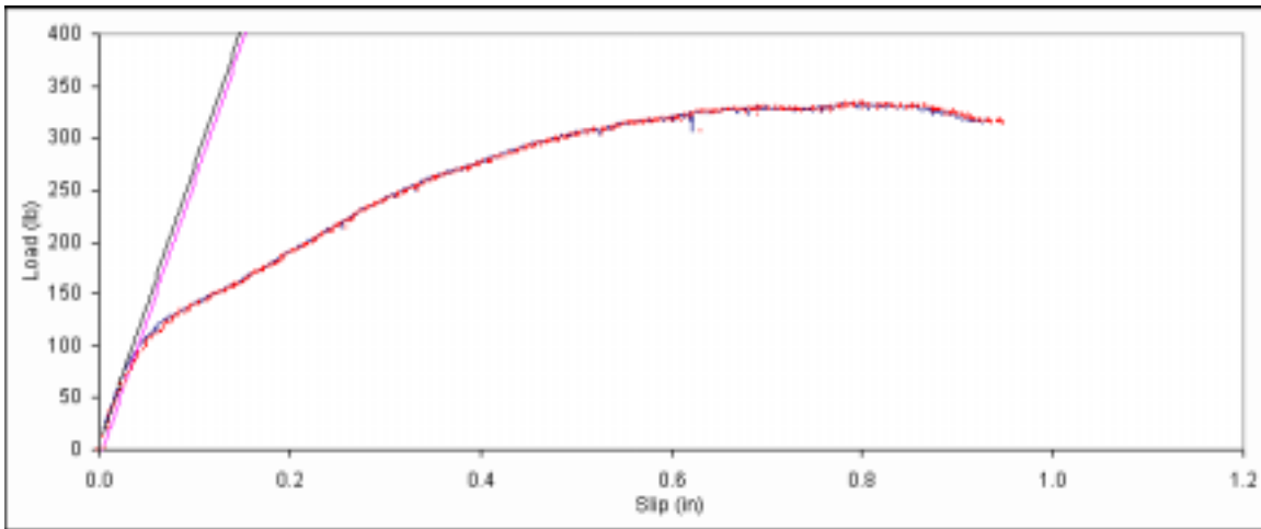
Figure B. 398: Load vs. slip plot for sample D6-13.
