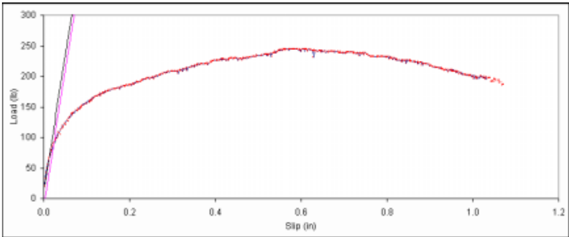
Figure B. 242: Load vs. slip plot for sample C3-5.
