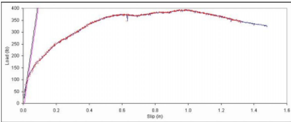
Figure B. 311: Load vs. slip plot for sample C7-15.
