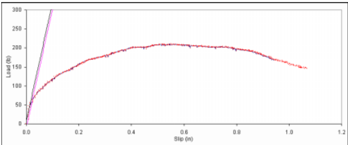
Figure B. 570: Load vs. slip plot for sample F4-8.
