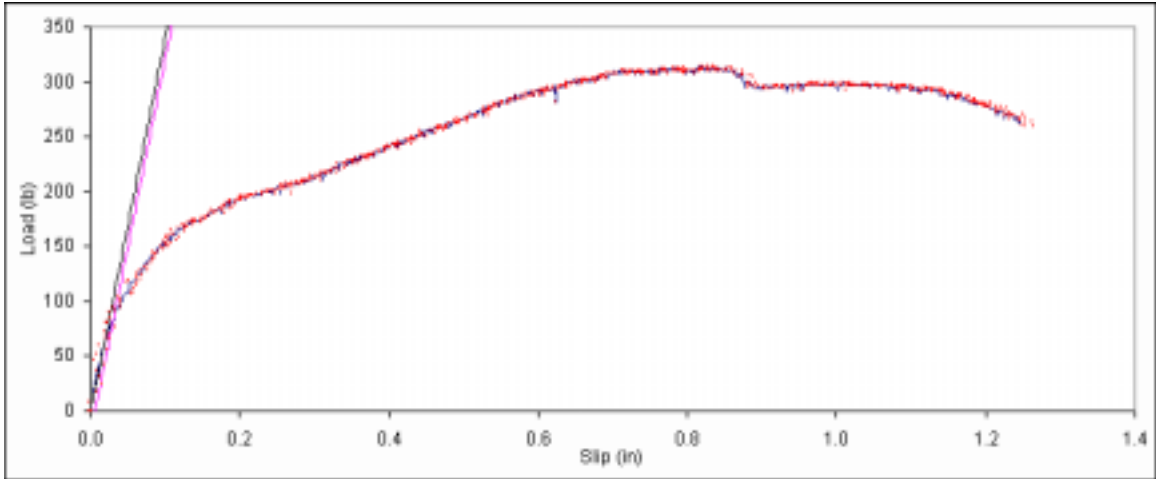
Figure B. 598: Load vs. slip plot for sample F6-6.
