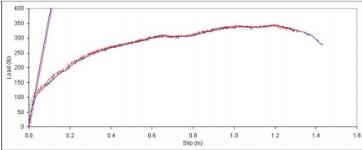
Figure B. 622: Load vs. slip plot for sample F7-15.
