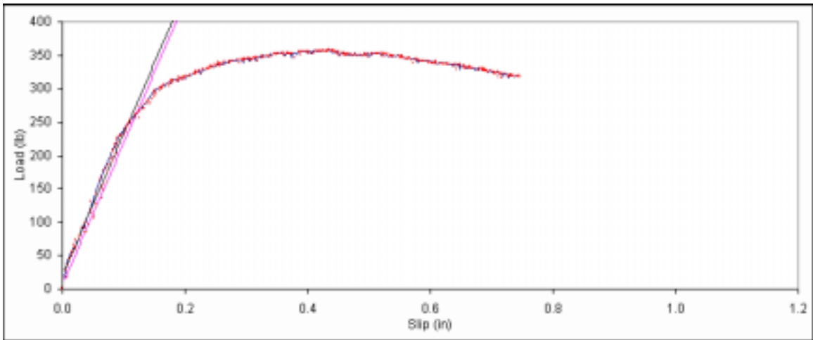
Figure B. 455: Load vs. slip plot for sample E3-10.
