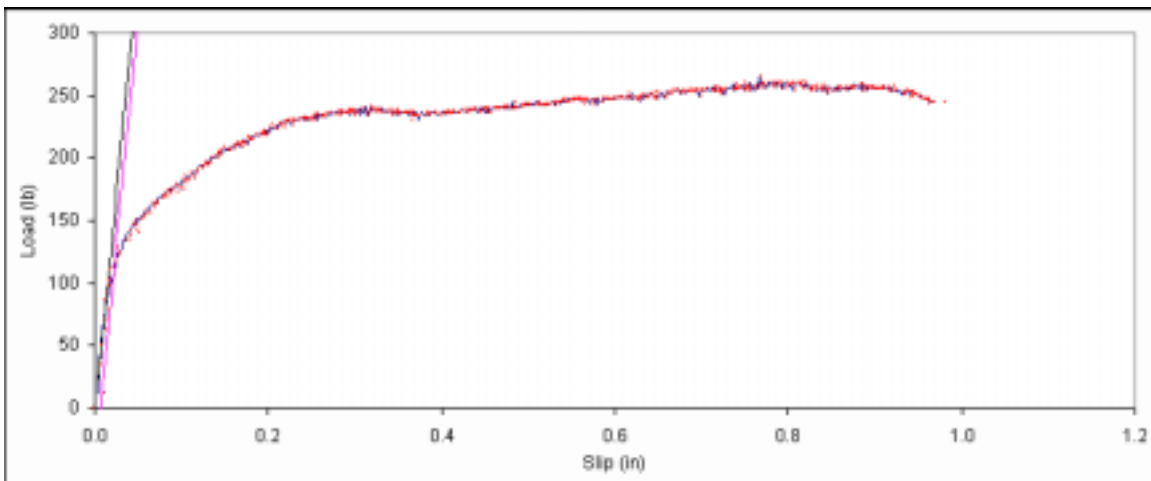
Figure B. 3: Load vs. slip plot for sample A1-3.
