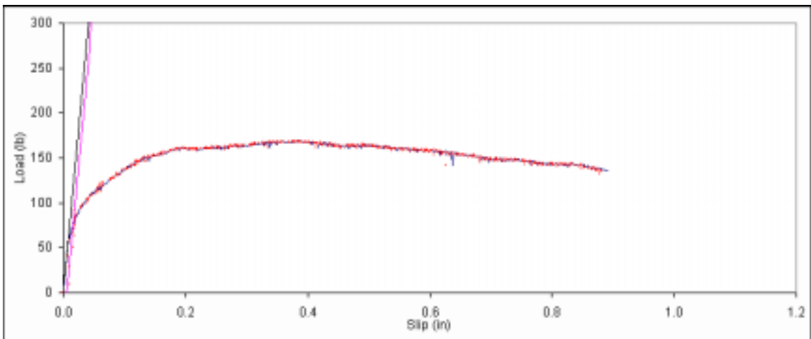
Figure B. 243: Load vs. slip plot for sample C3-6.
