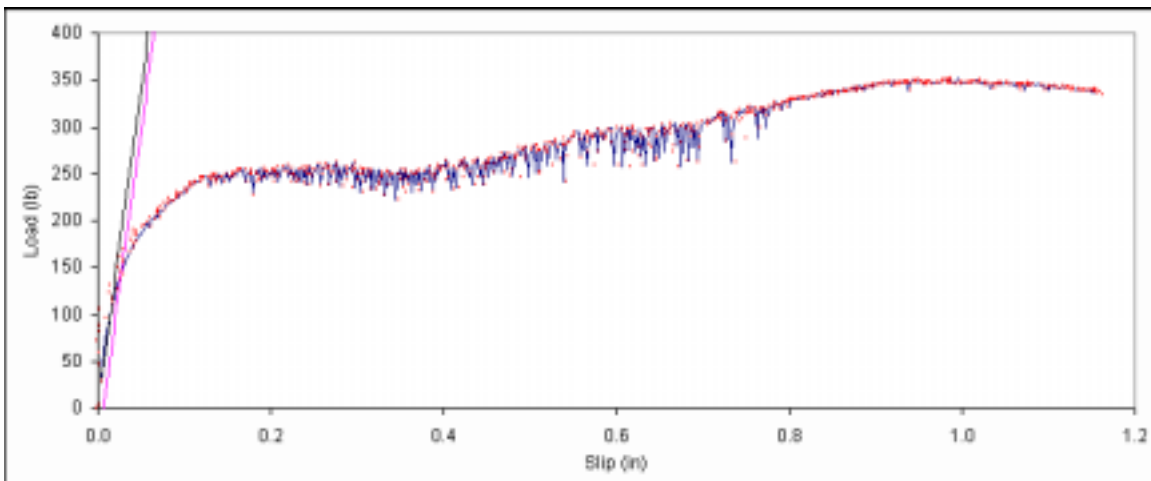
Figure B. 417: Load vs. slip plot for sample E1-2.
