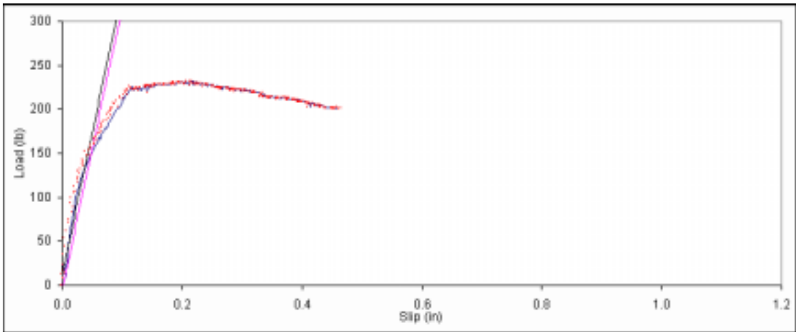
Figure B. 539: Load vs. slip plot for sample F2-6.
