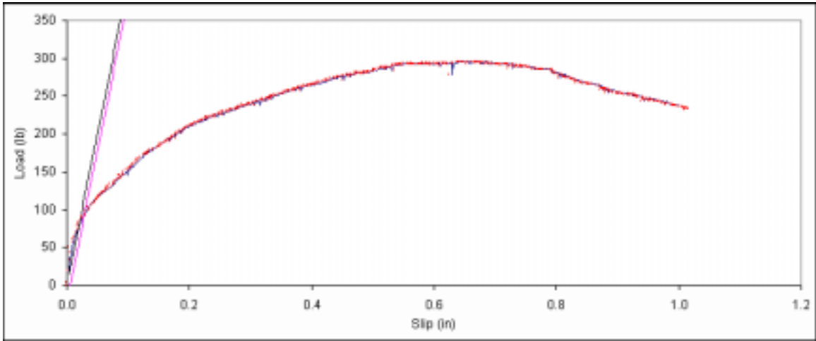
Figure B. 254: Load vs. slip plot for sample C4-3.
