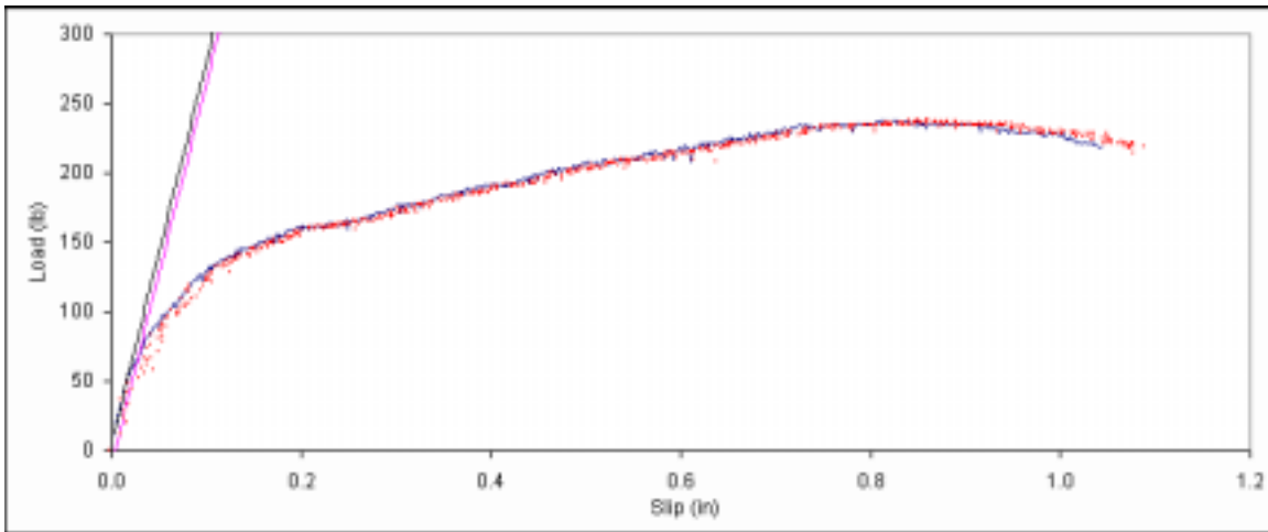
Figure B. 593: Load vs. slip plot for sample F6-1.
