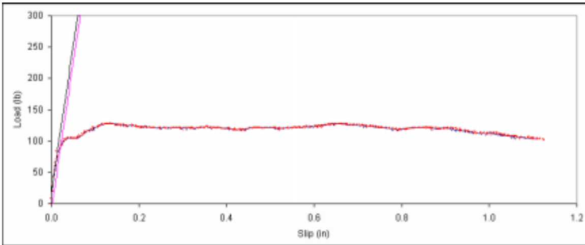
Figure B. 143: Load vs. slip plot for sample B3-11.
