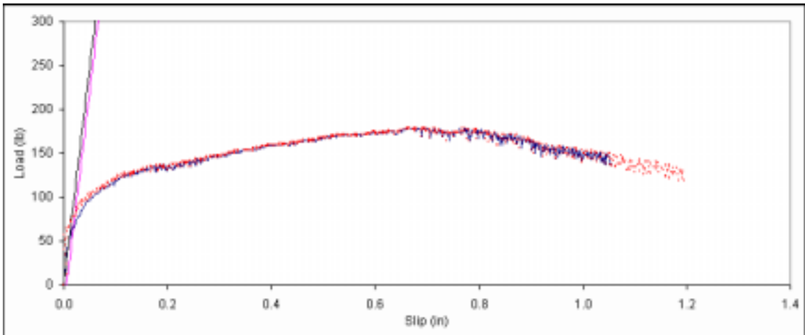
Figure B. 234: Load vs. slip plot for sample C2-12.
