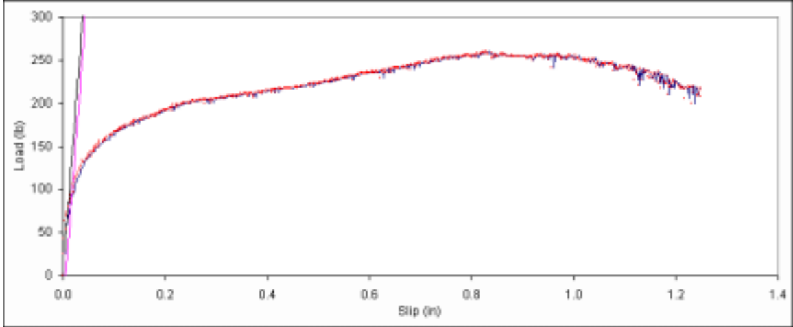
Figure B. 340: Load vs. slip plot for sample D2-15.
