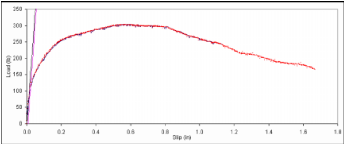
Figure B. 257: Load vs. slip plot for sample C4-6.
