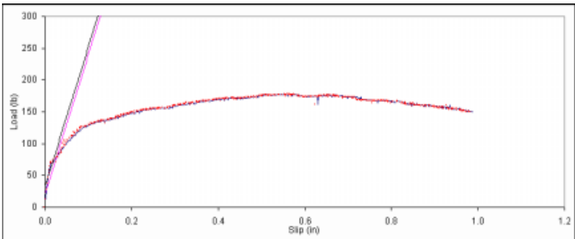
Figure B. 168: Load vs. slip plot for sample B5-6.
