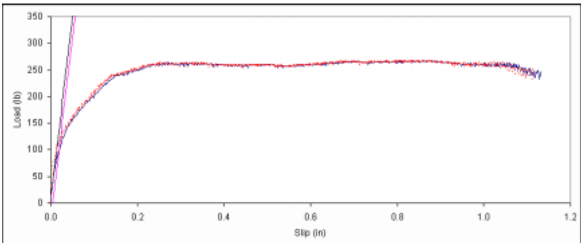
Figure B. 396: Load vs. slip plot for sample D6-11.
