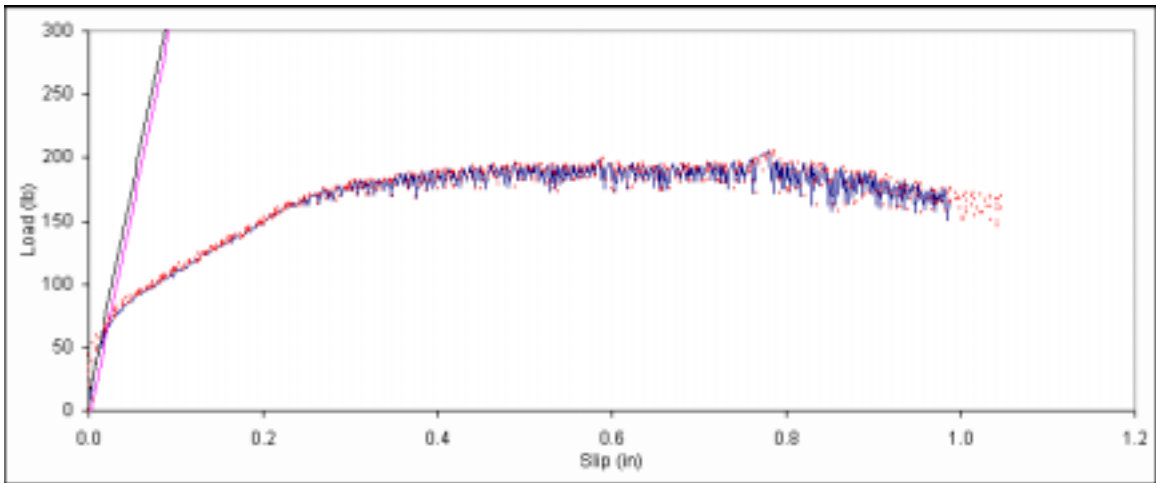
Figure B. 350: Load vs. slip plot for sample D3-10.
