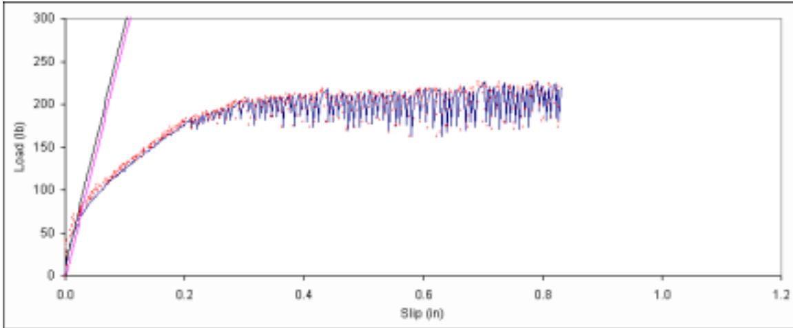
Figure B. 328: Load vs. slip plot for sample D2-3.
