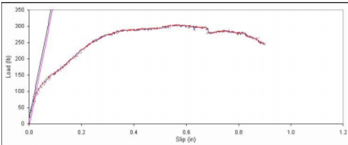
Figure B. 201: Load vs. slip plot for sample B7-9.
