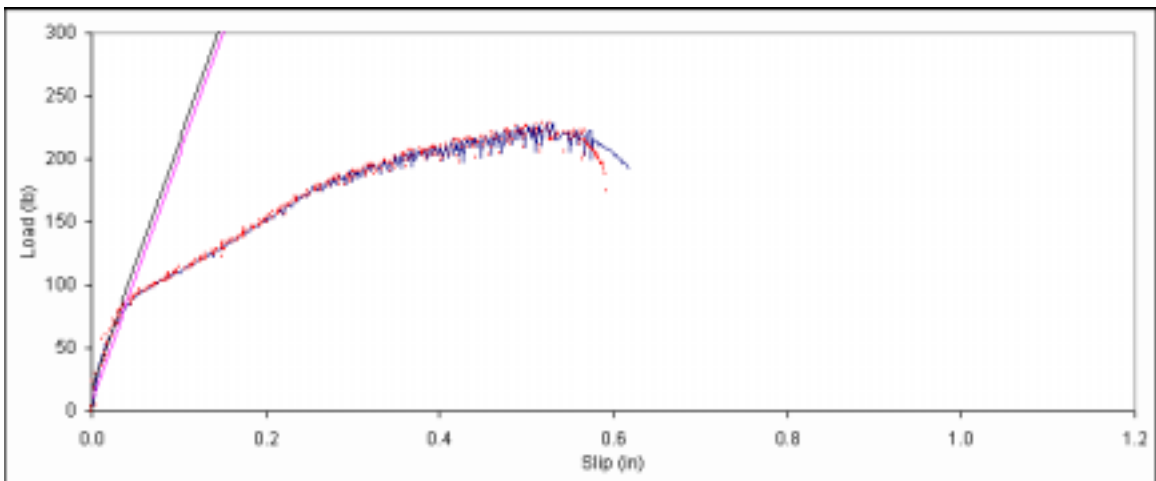
Figure B. 12: Load vs. slip plot for sample A1-12.
