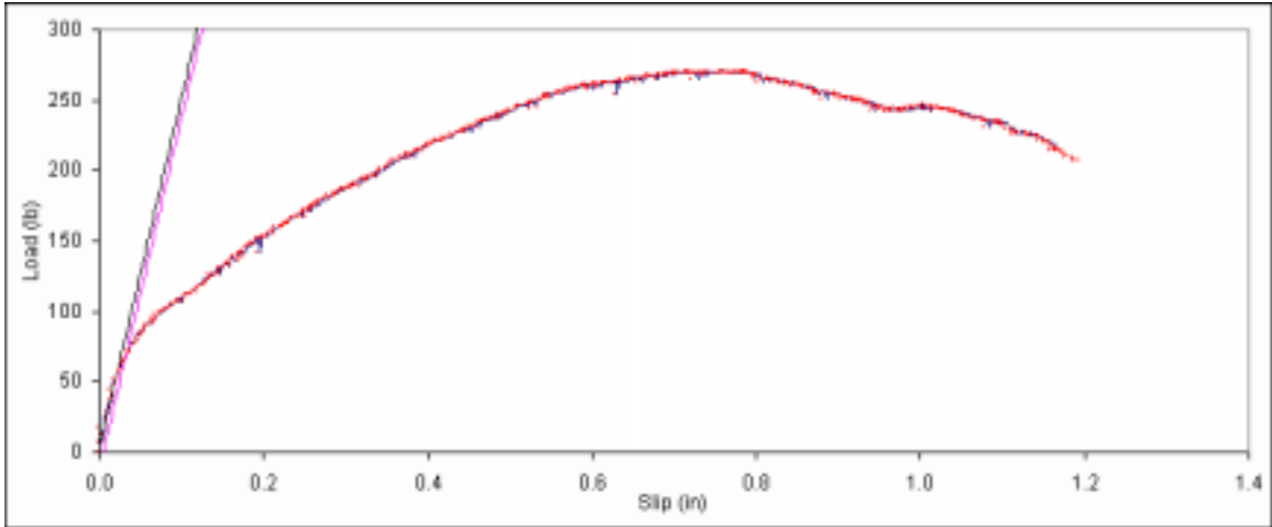
Figure B. 568: Load vs. slip plot for sample F4-6.
