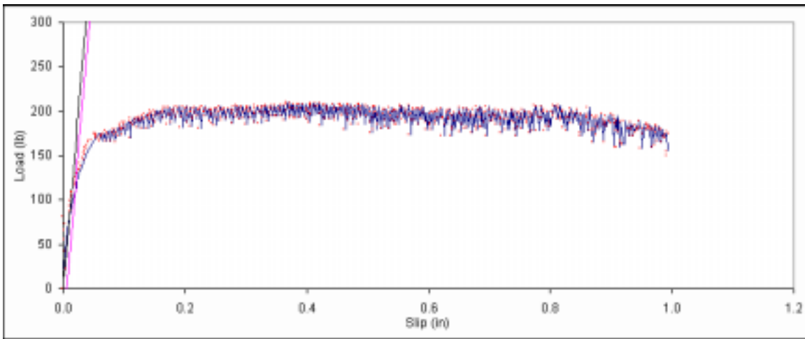
Figure B. 329: Load vs. slip plot for sample D2-4.
