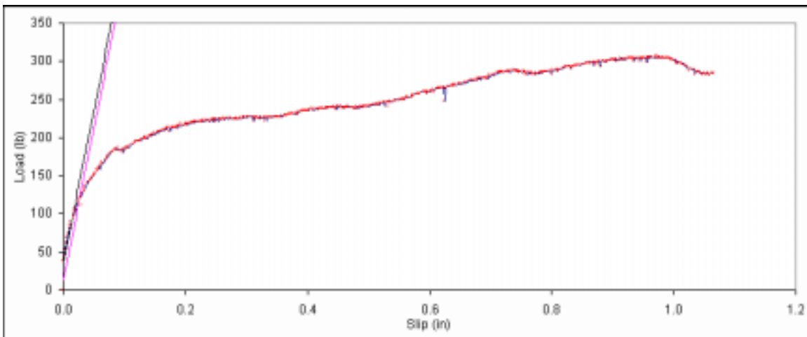
Figure B. 78: Load vs. slip plot for sample A6-4.
