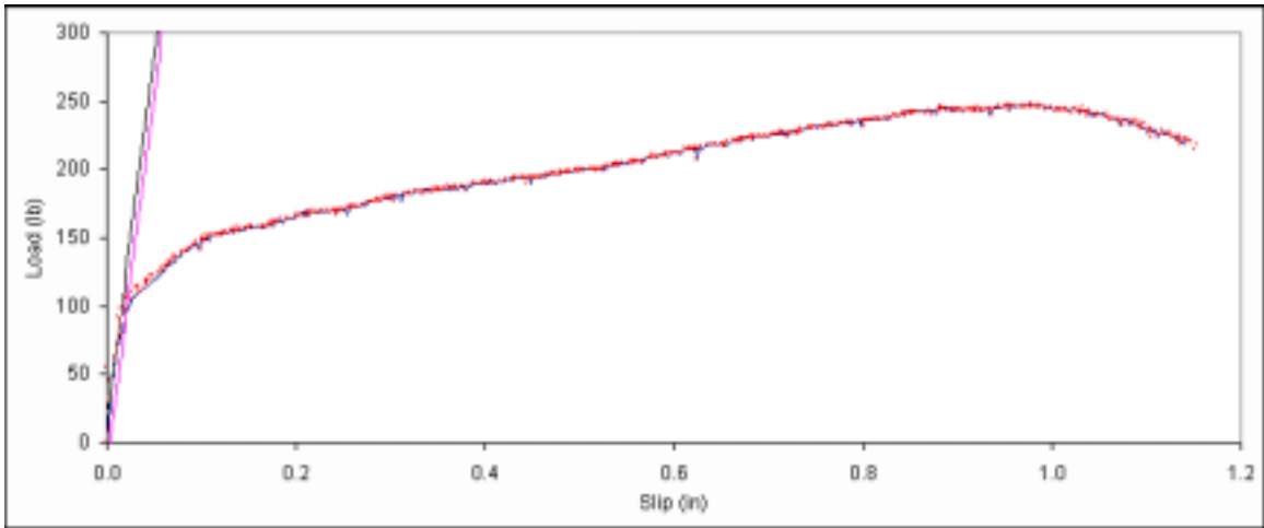
Figure B. 134: Load vs. slip plot for sample B3-2.
