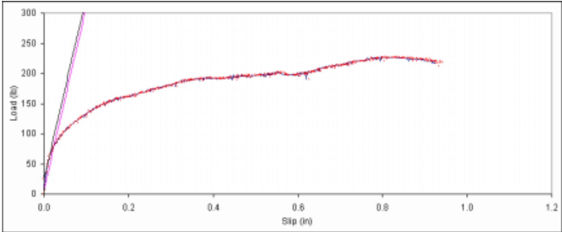
Figure B. 109: Load vs. slip plot for sample B1-7.
