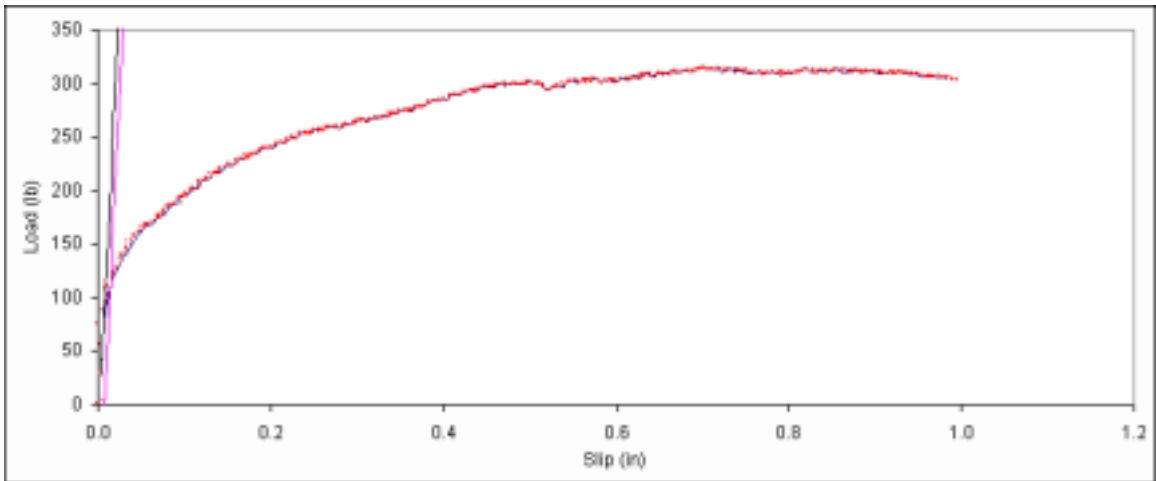
Figure B. 521: Load vs. slip plot for sample F1-2.
