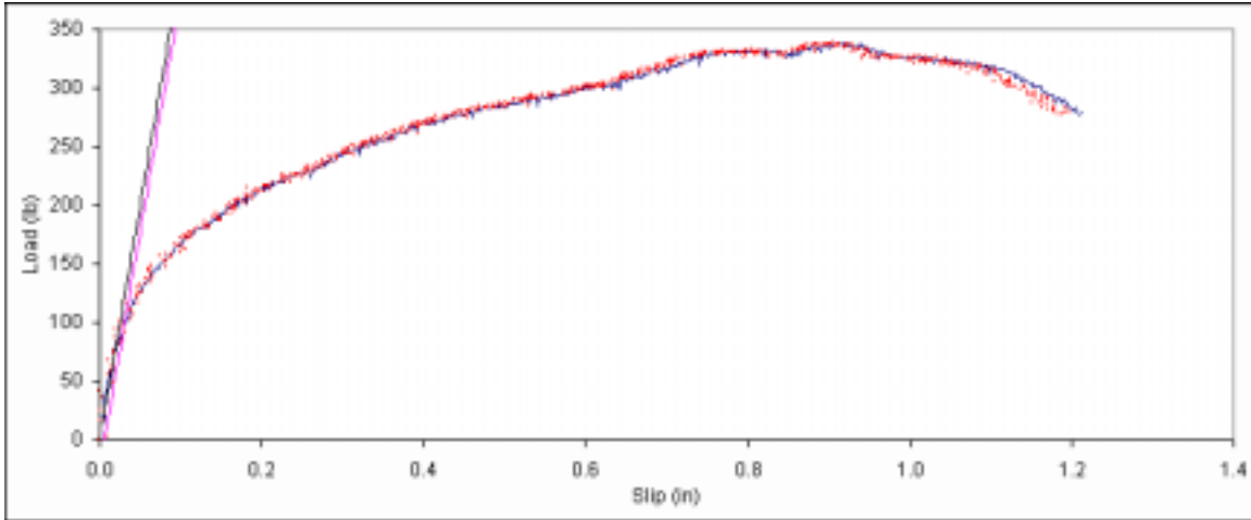
Figure B. 604: Load vs. slip plot for sample F6-12.
