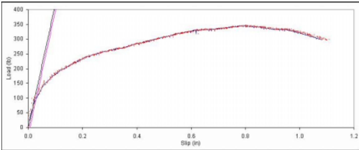
Figure B. 413: Load vs. slip plot for sample D7-13.
