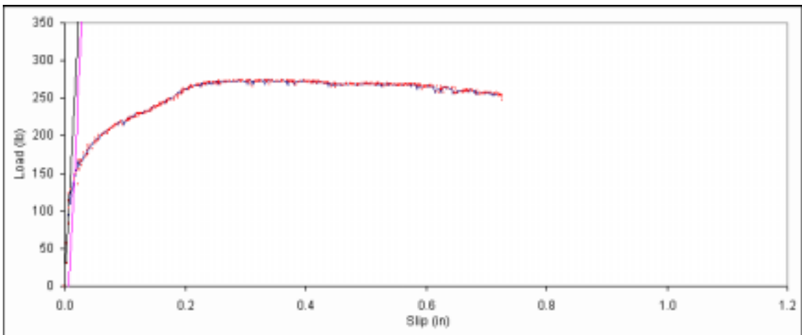
Figure B. 444: Load vs. slip plot for sample E2-14.
