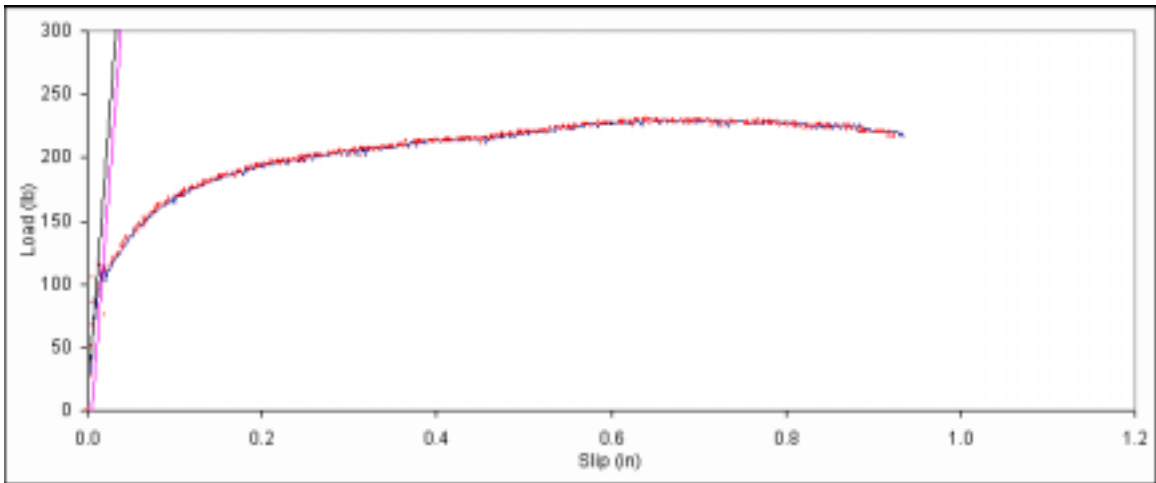
Figure B. 110: Load vs. slip plot for sample B1-8.
