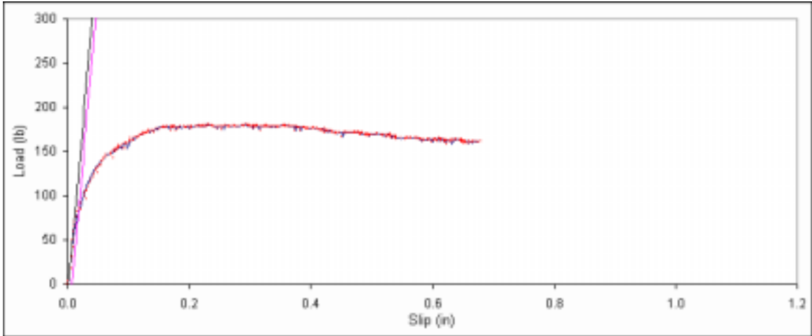
Figure B. 556: Load vs. slip plot for sample F3-9.
