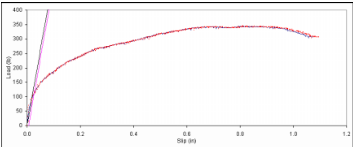
Figure B. 276: Load vs. slip plot for sample C5-10.
