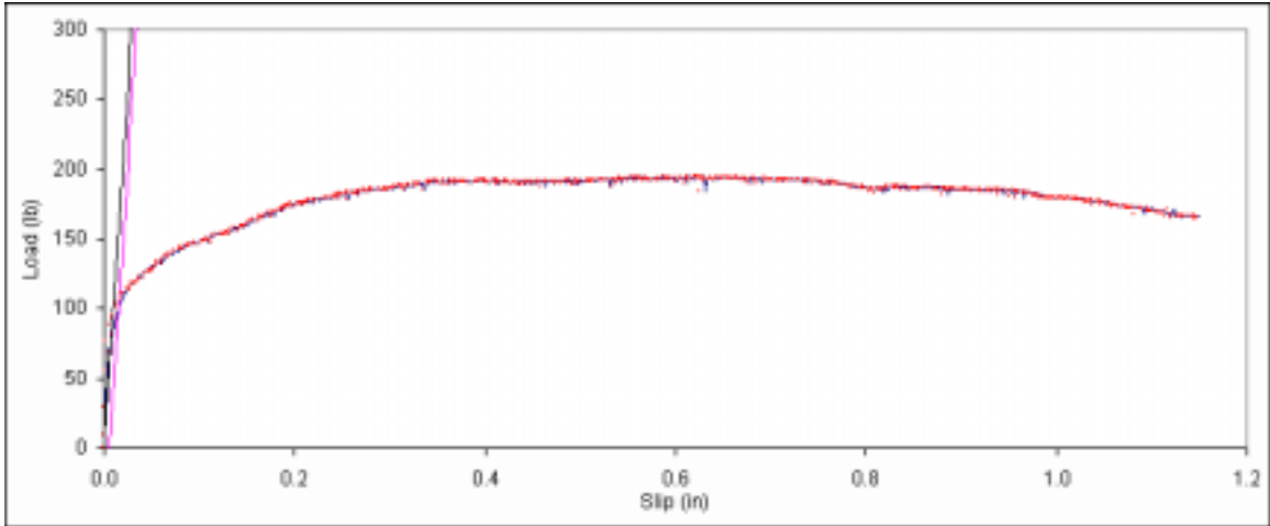
Figure B. 37: Load vs. slip plot for sample A3-8.
