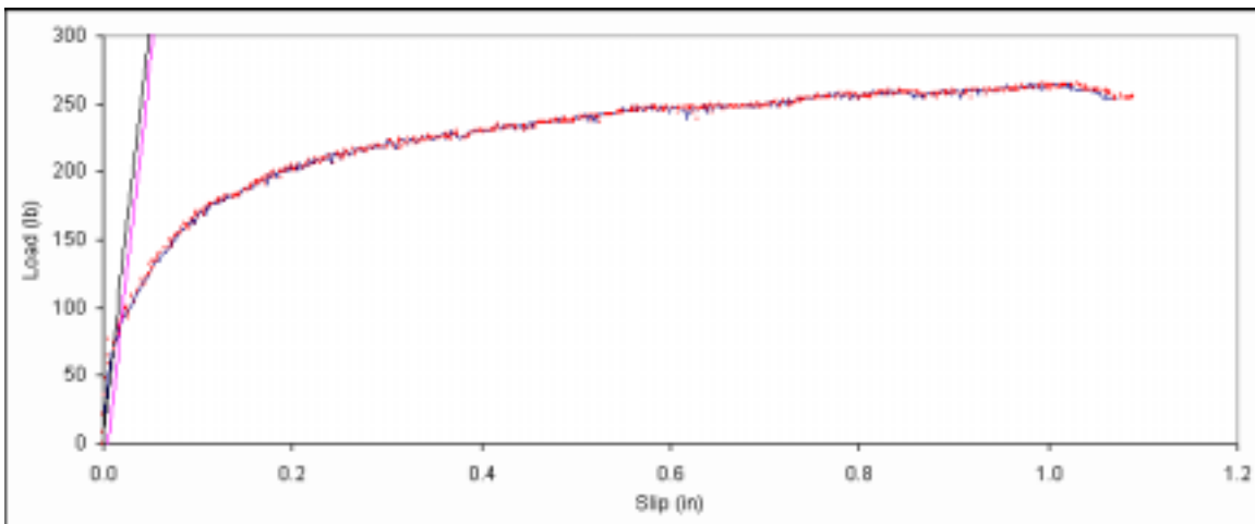
Figure B. 210: Load vs. slip plot for sample C1-3.
