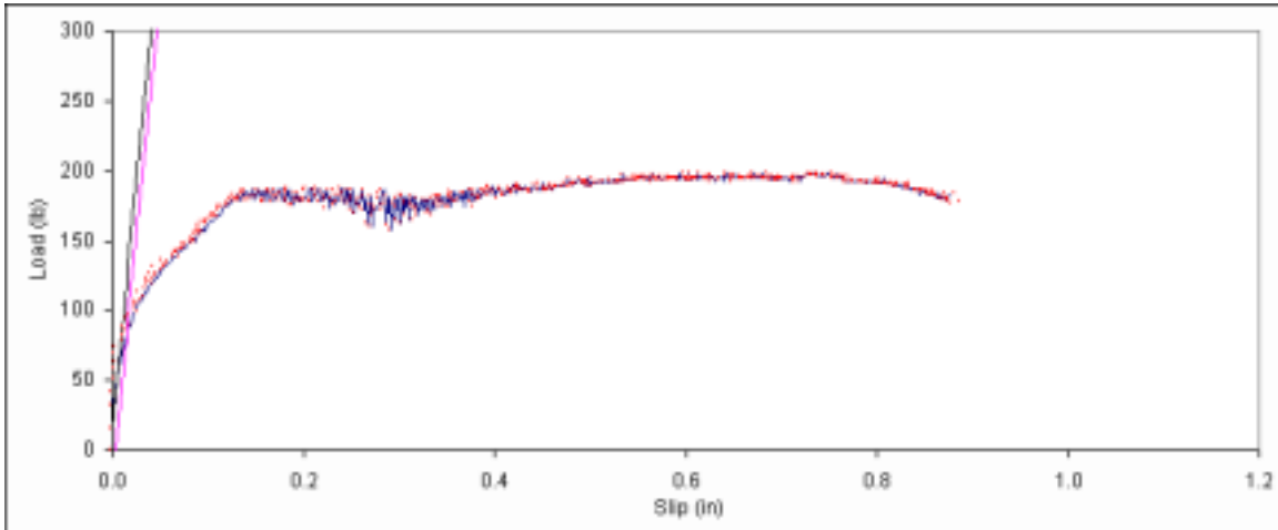
Figure B. 208: Load vs. slip plot for sample C1-1.
