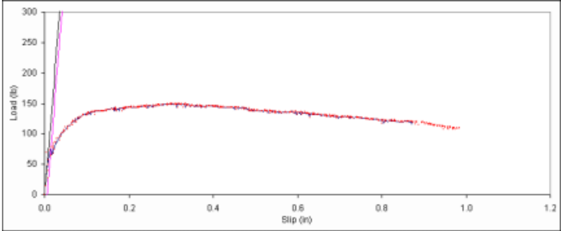
Figure B. 562: Load vs. slip plot for sample F3-15.
