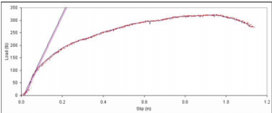
Figure B. 303: Load vs. slip plot for sample C7-7.
