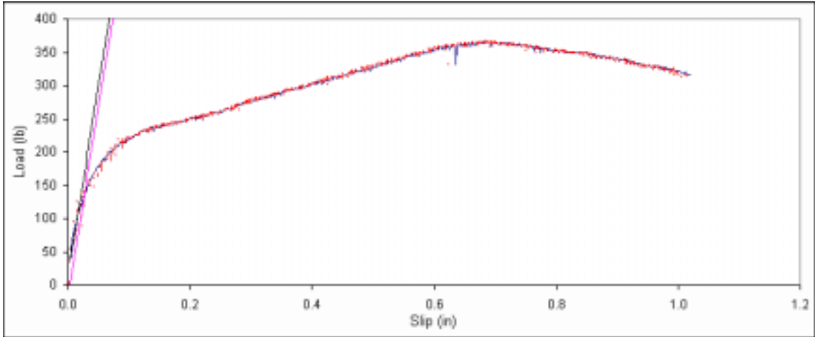
Figure B. 82: Load vs. slip plot for sample A6-9.
