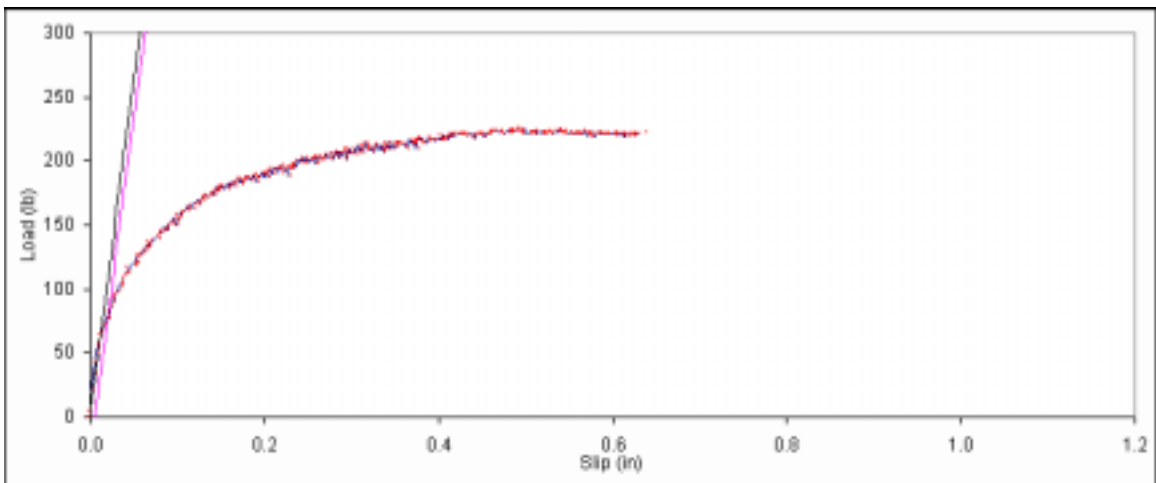
Figure B. 213: Load vs. slip plot for sample C1-6.
