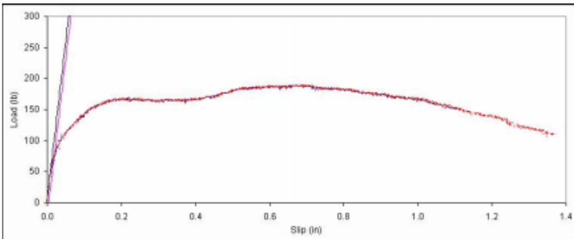
Figure B. 195: Load vs. slip plot for sample B7-3.
