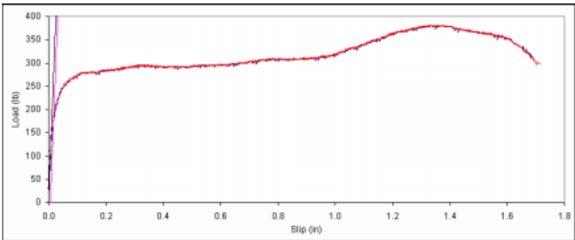
Figure B. 447: Load vs. slip plot for sample E3-2.
