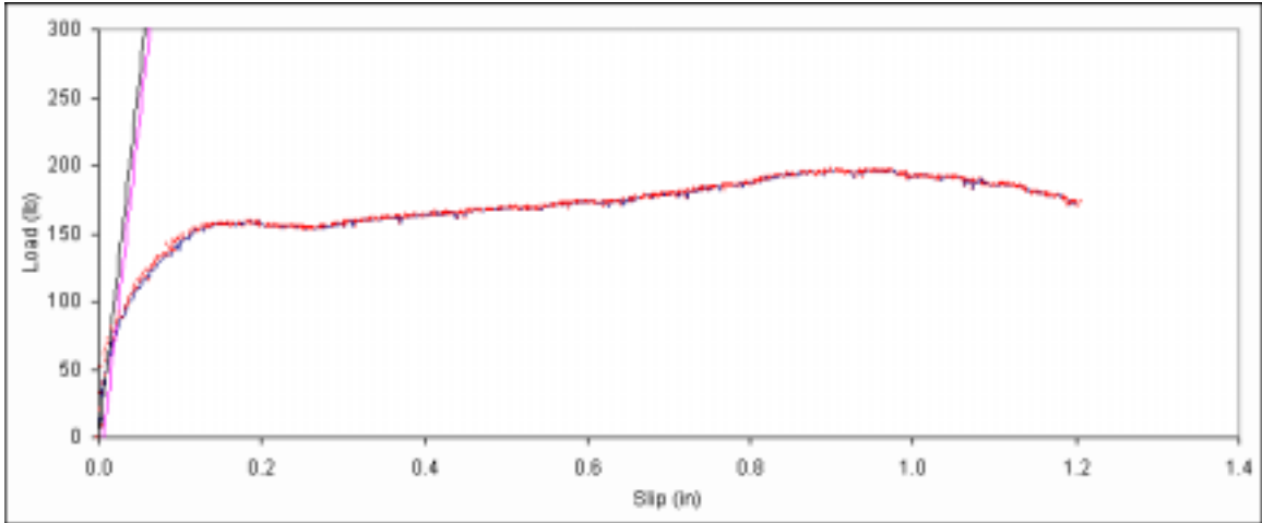
Figure B. 229: Load vs. slip plot for sample C2-7.
