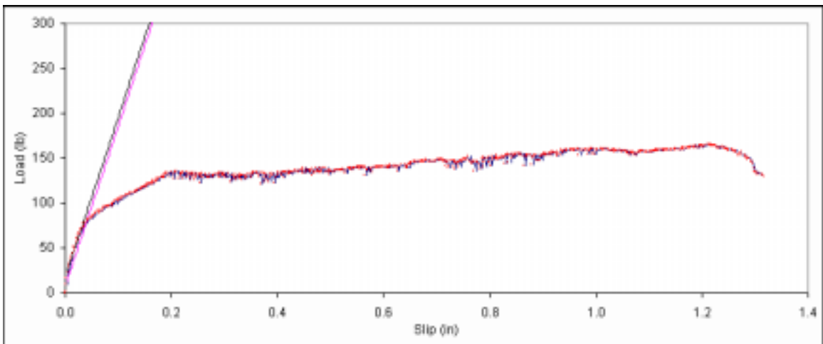
Figure B. 129: Load vs. slip plot for sample B2-12.
