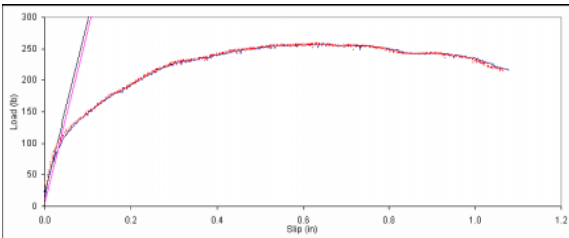
Figure B. 153: Load vs. slip plot for sample B4-6.
