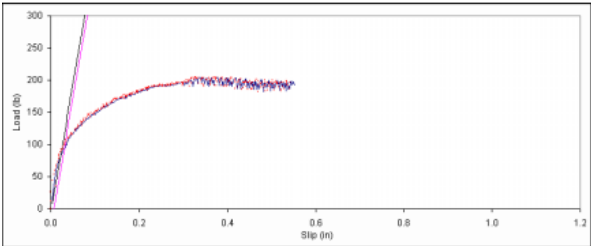
Figure B. 324: Load vs. slip plot for sample D1-14.
