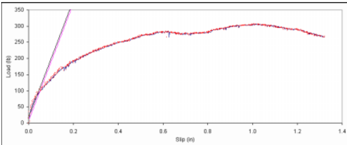
Figure B. 150: Load vs. slip plot for sample B4-3.
