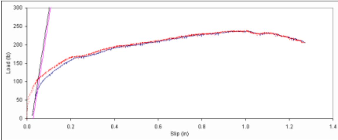
Figure B. 577: Load vs. slip plot for sample F4-15.
