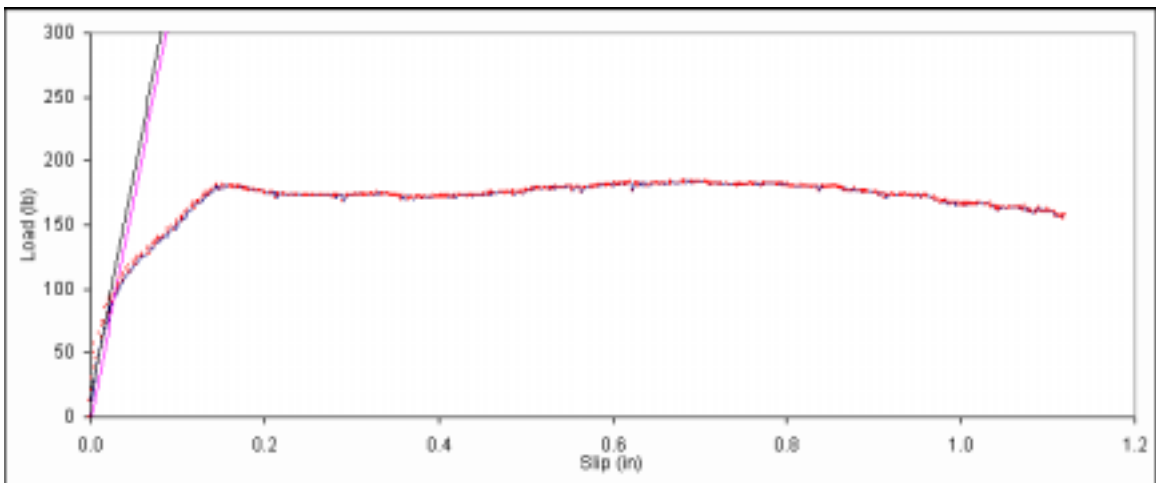
Figure B. 123: Load vs. slip plot for sample B2-6.
