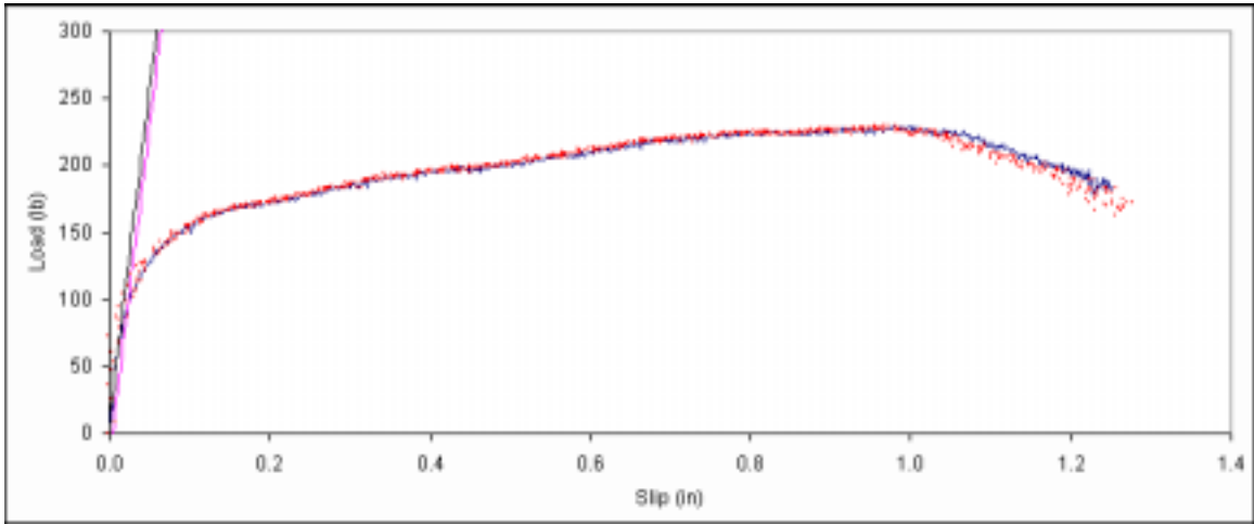
Figure B. 158: Load vs. slip plot for sample B4-11.
