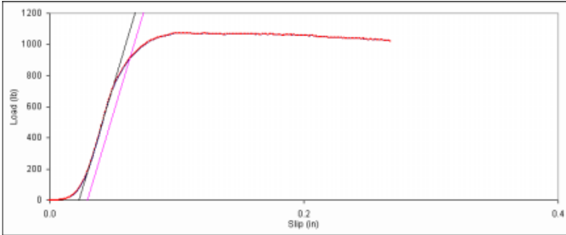
Figure D. 34: Bearing embedment plot for main member sample 8d-14.
