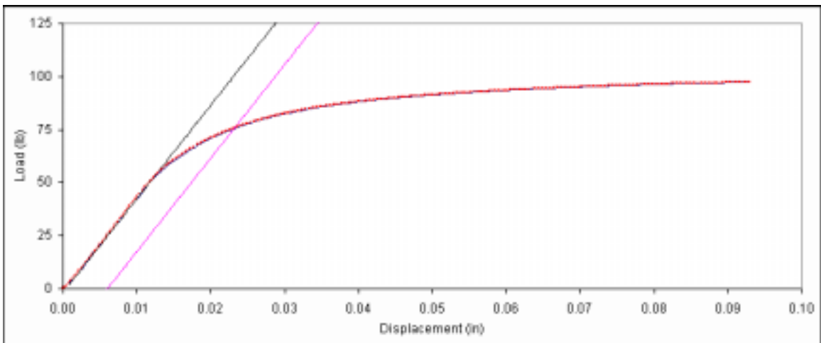
Figure D. 165: Bearing embedment plot for fastener sample 6d-5.
