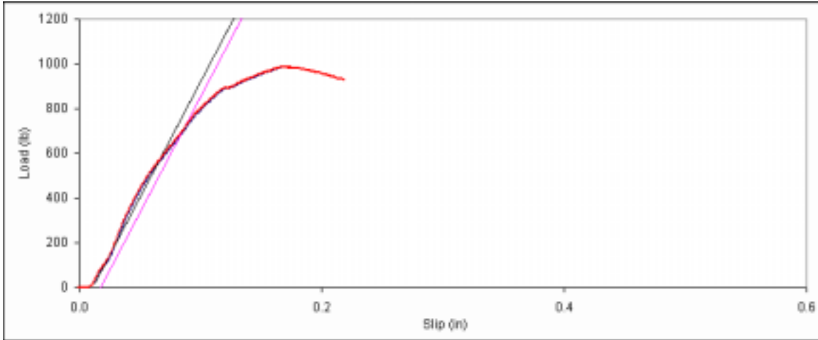
Figure D. 121: Bearing embedment plot for side member sample E-1.
