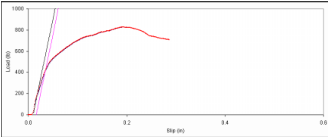
Figure D. 140: Bearing embedment plot for side member sample E-20.
