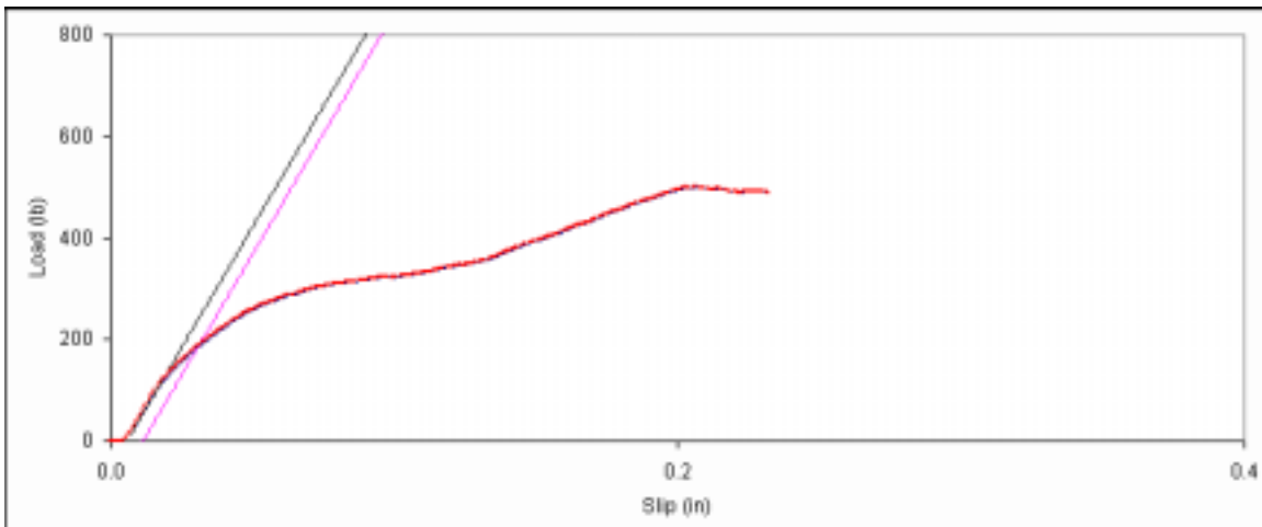
Figure D. 71: Bearing embedment plot for side member sample B-11.
