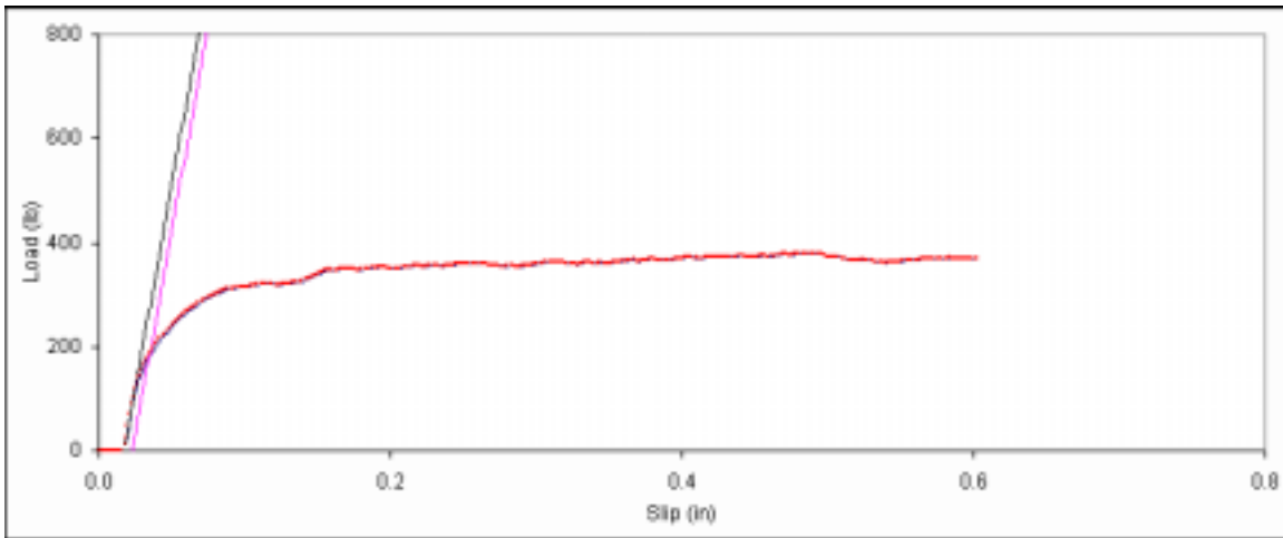
Figure D. 65: Bearing embedment plot for side member sample B-5.
