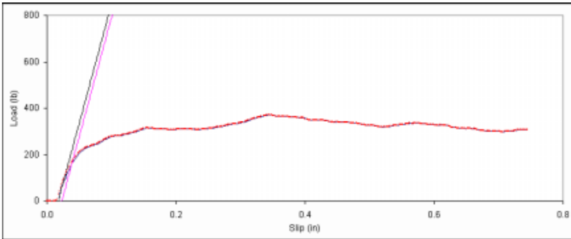
Figure D. 98: Bearing embedment plot for side member sample C-18.
