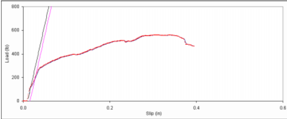
Figure D. 94: Bearing embedment plot for side member sample C-14.
