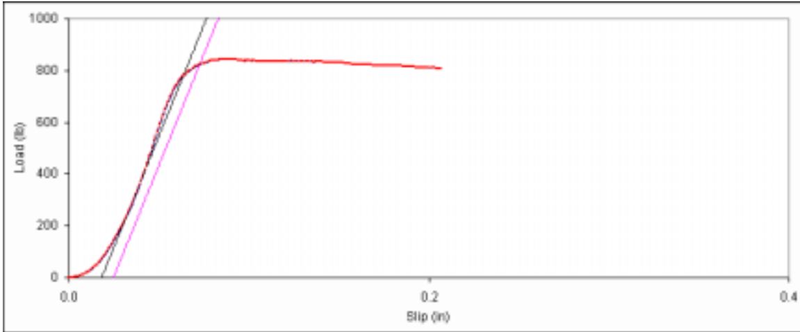
Figure D. 25: Bearing embedment plot for main member sample 8d-5.
