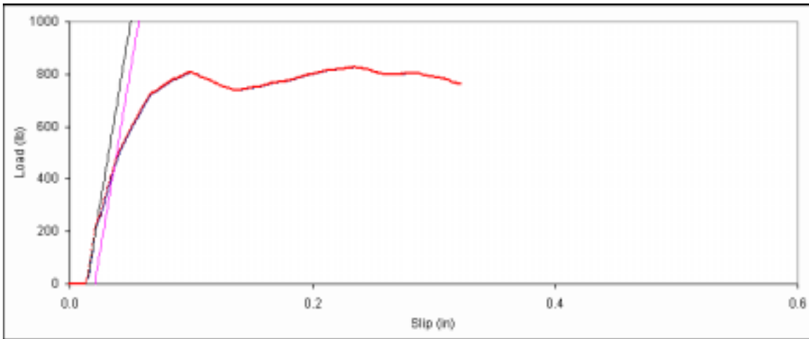
Figure D. 125: Bearing embedment plot for side member sample E-5.
