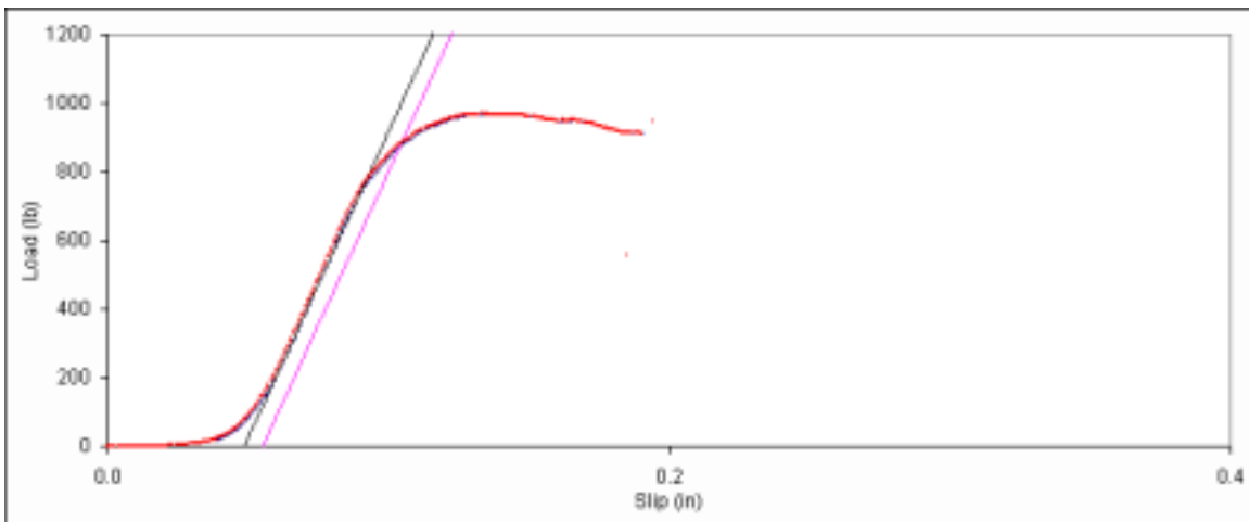
Figure D. 30: Bearing embedment plot for main member sample 8d-10.
