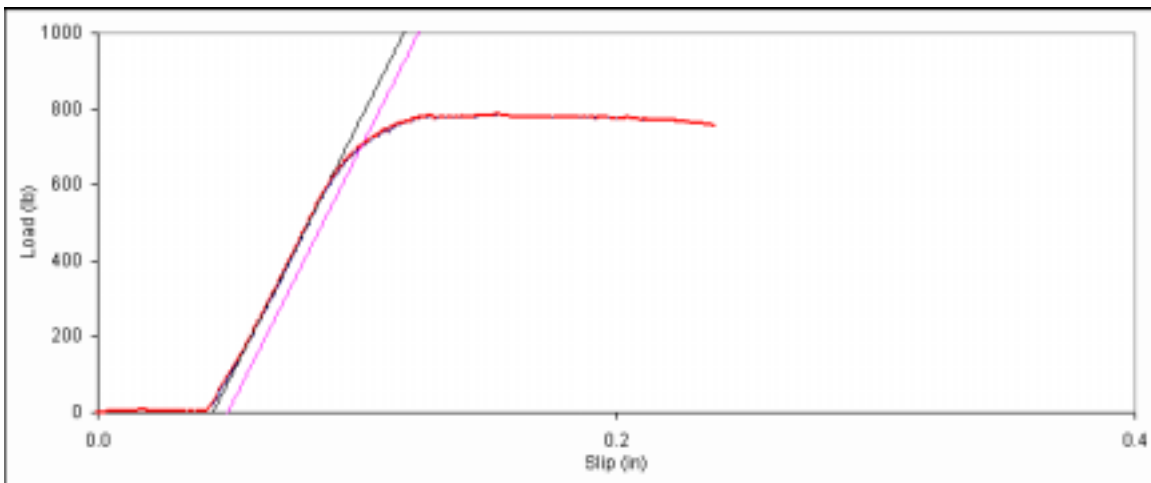
Figure D. 6: Bearing embedment plot for main member sample 6d-6.
