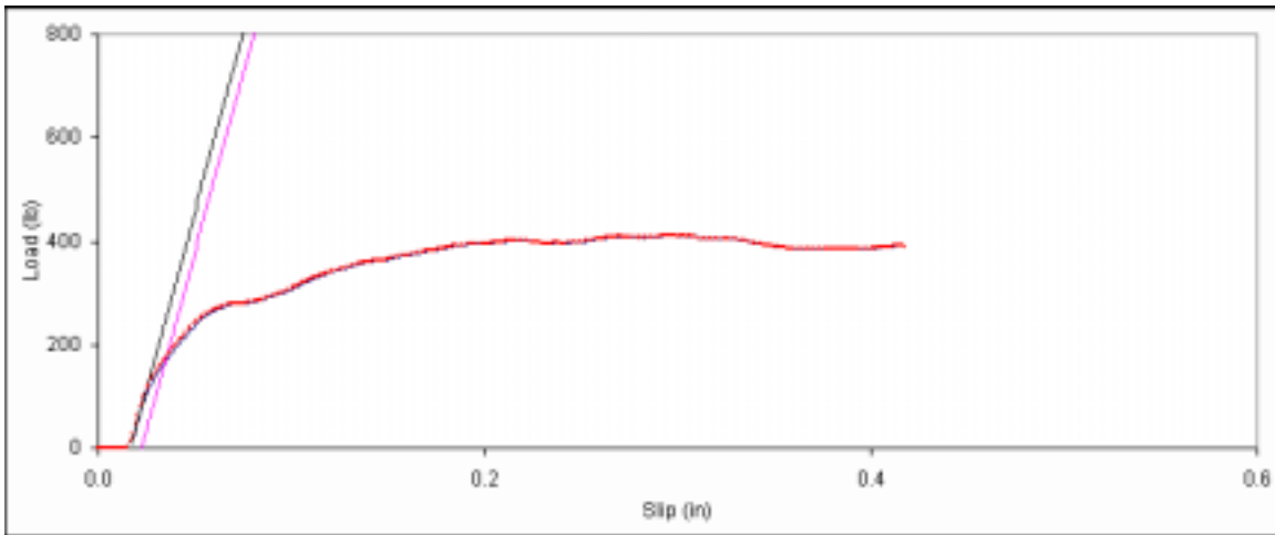
Figure D. 80: Bearing embedment plot for side member sample B-20.
