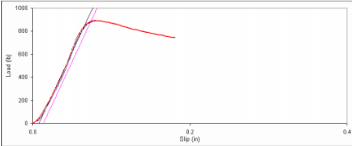
Figure D. 7: Bearing embedment plot for main member sample 6d-7.
