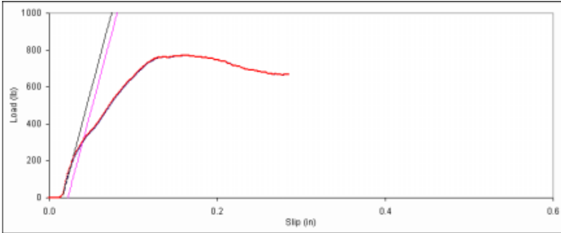
Figure D. 133: Bearing embedment plot for side member sample E-13.
