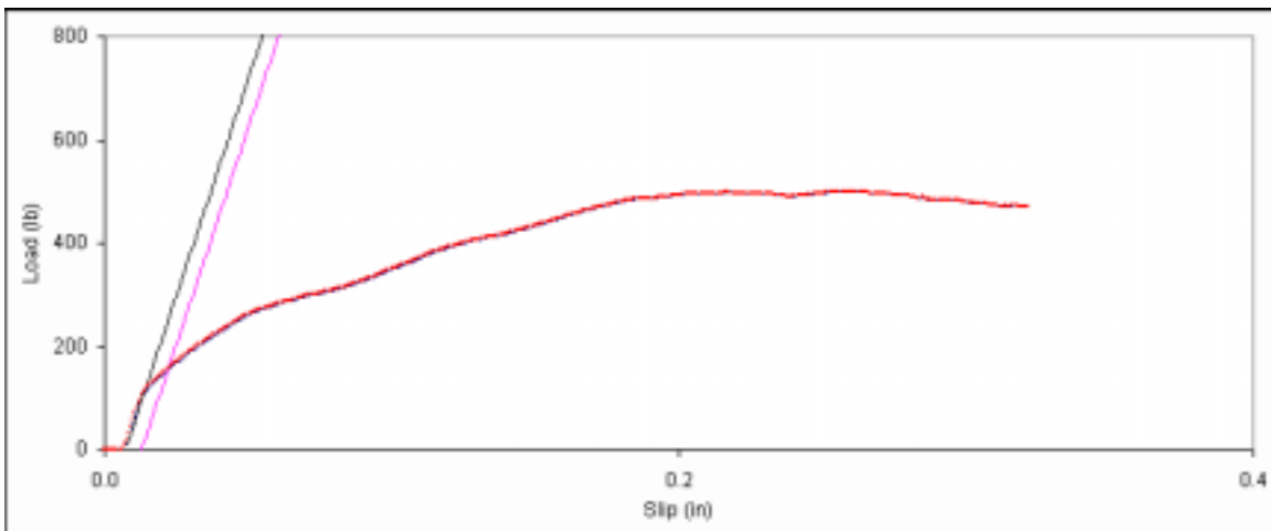
Figure D. 78: Bearing embedment plot for side member sample B-18.
