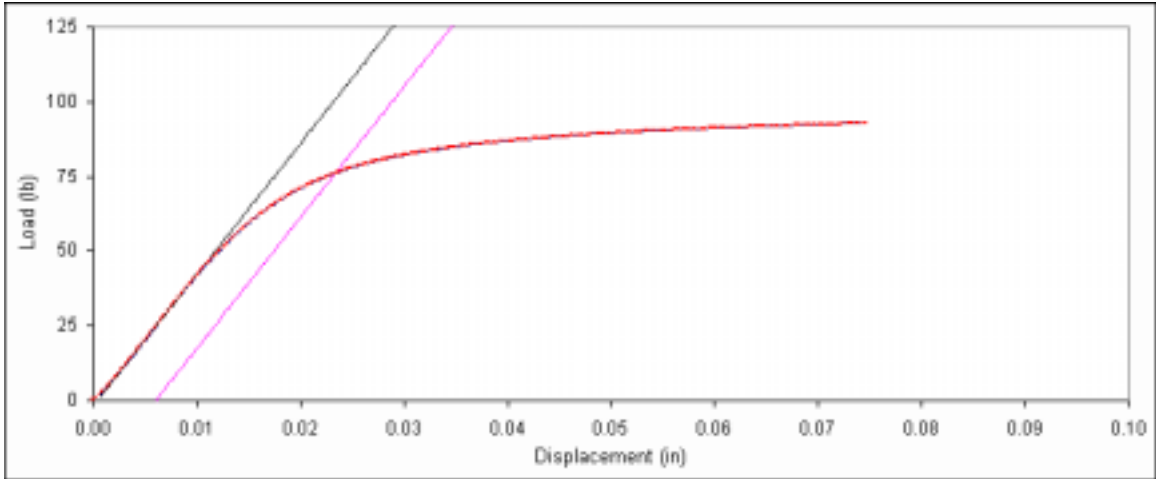
Figure D. 169: Bearing embedment plot for fastener sample 6d-9.
