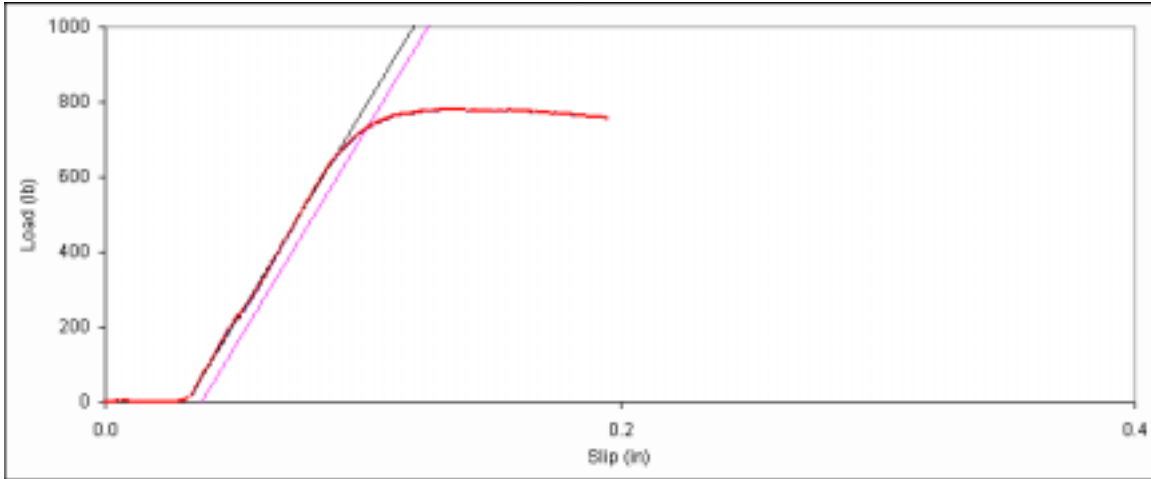
Figure D. 1: Bearing embedment plot for main member sample 6d-1.
