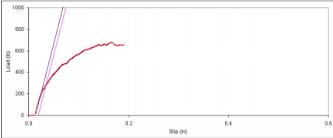
Figure D. 145: Bearing embedment plot for side member sample F-5.
