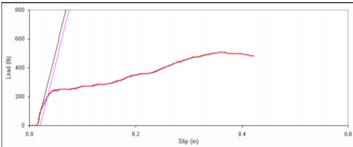
Figure D. 69: Bearing embedment plot for side member sample B-9.
