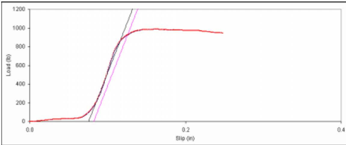
Figure D. 35: Bearing embedment plot for main member sample 8d-15.
