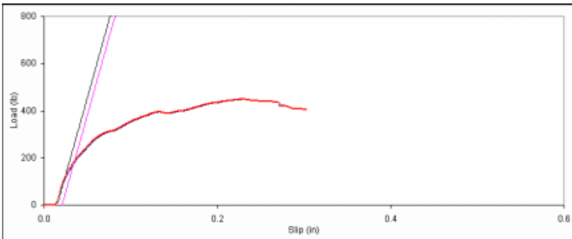
Figure D. 120: Bearing embedment plot for side member sample D-20.
