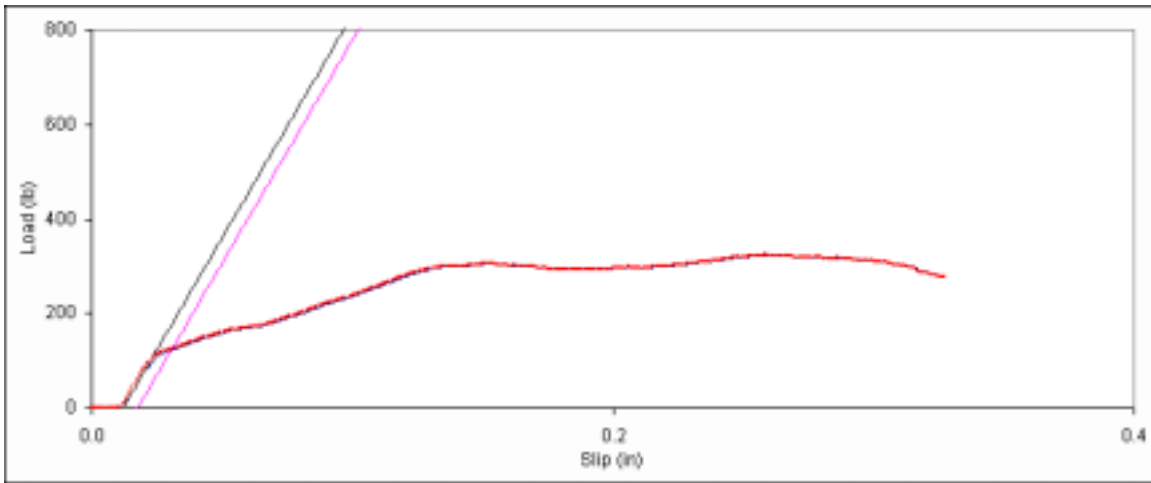
Figure D. 95: Bearing embedment plot for side member sample C-15.
