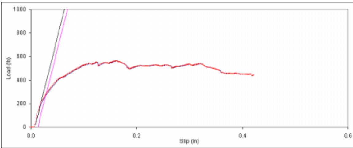
Figure D. 146: Bearing embedment plot for side member sample F-6.
