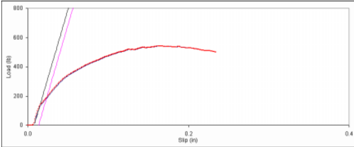
Figure D. 64: Bearing embedment plot for side member sample B-4.
