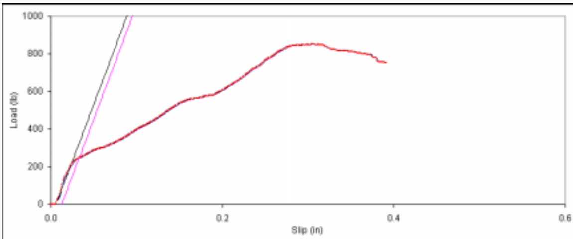
Figure D. 132: Bearing embedment plot for side member sample E-12.
