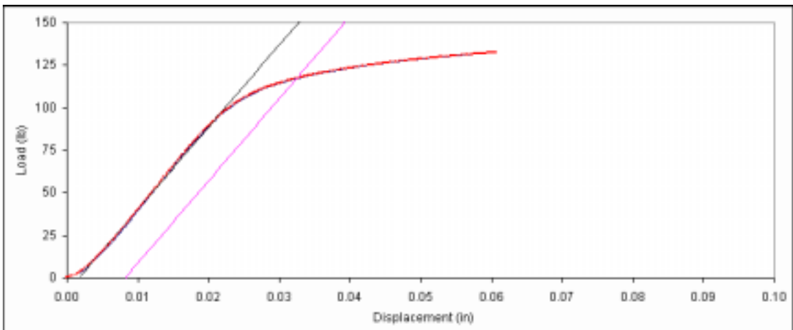
Figure D. 171: Bearing embedment plot for fastener sample 8d-1.
