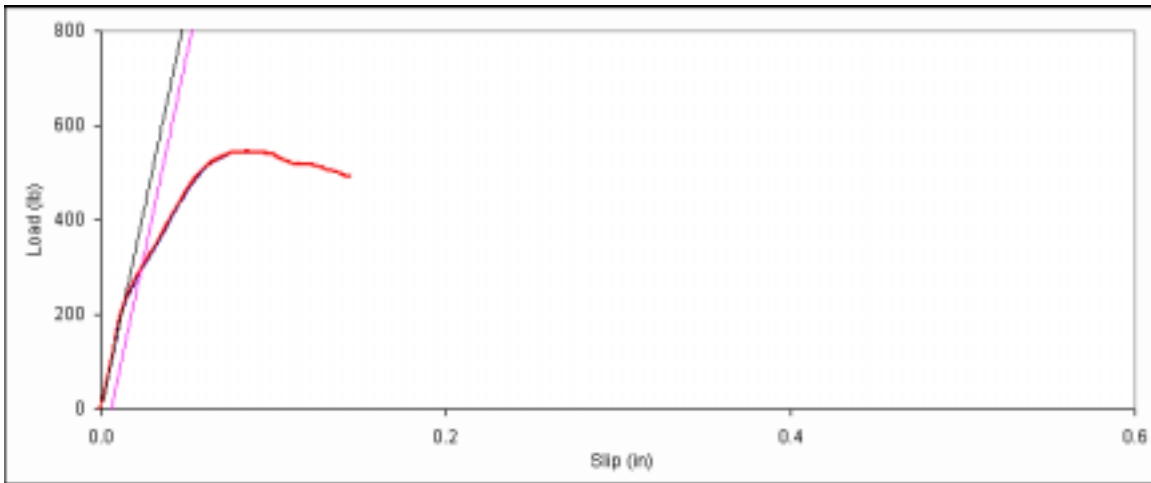
Figure D. 101: Bearing embedment plot for side member sample D-1.
