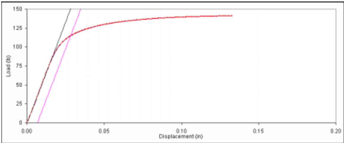
Figure D. 176: Bearing embedment plot for fastener sample 8d-6.
