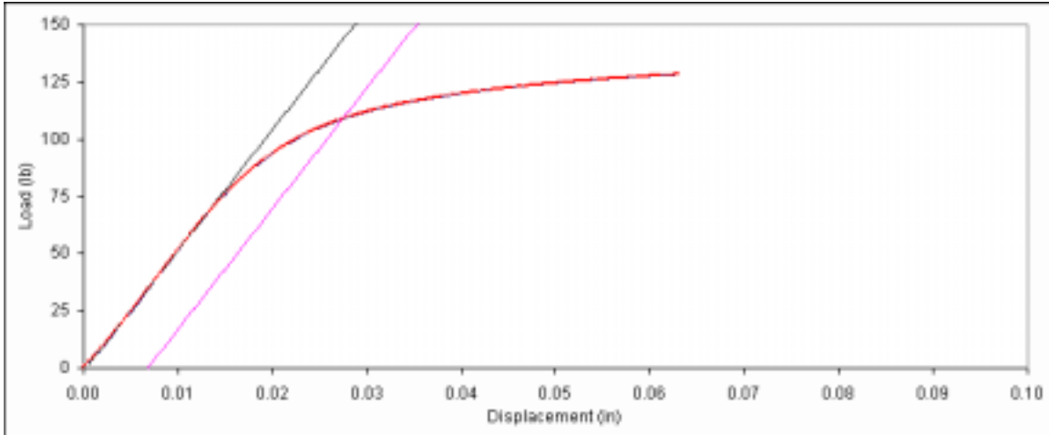
Figure D. 172: Bearing embedment plot for fastener sample 8d-2.
