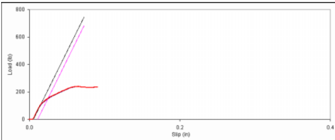
Figure D. 96: Bearing embedment plot for side member sample C-16.
