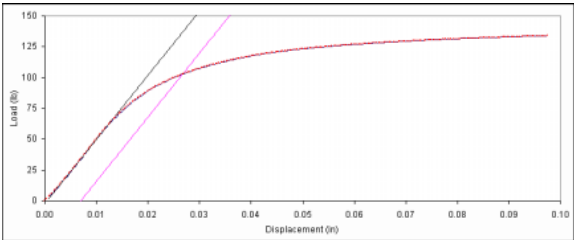
Figure D. 177: Bearing embedment plot for fastener sample 8d-7.
