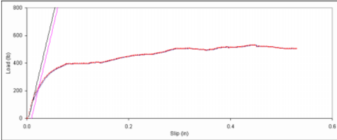
Figure D. 55: Bearing embedment plot for side member sample A-15.
