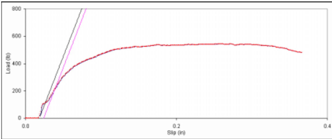
Figure D. 50: Bearing embedment plot for side member sample A-10.
