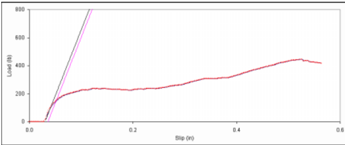
Figure D. 77: Bearing embedment plot for side member sample B-17.
