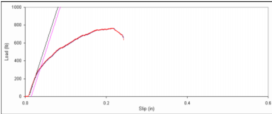
Figure D. 149: Bearing embedment plot for side member sample F-9.
