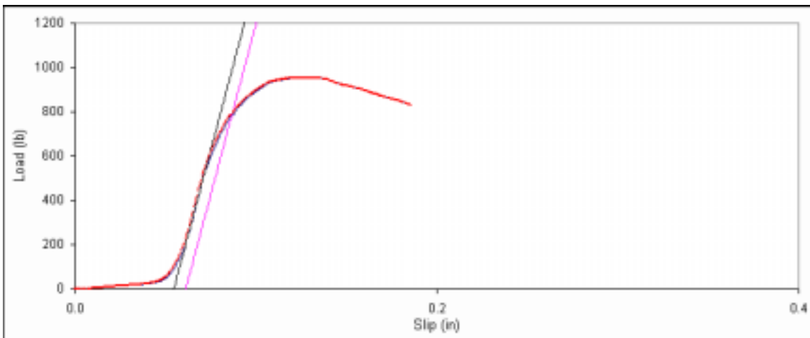
Figure D. 39: Bearing embedment plot for main member sample 8d-19.
