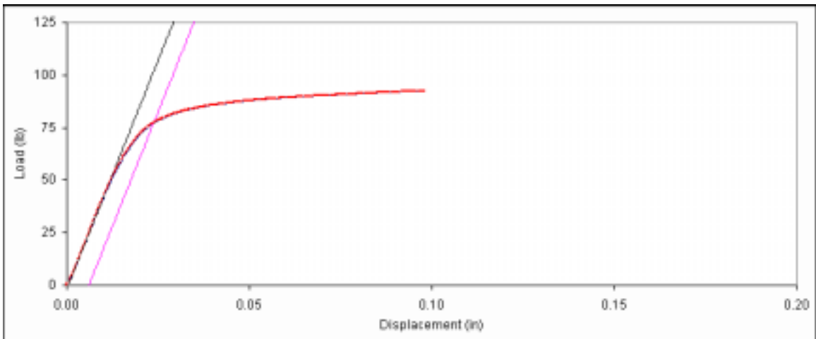
Figure D. 168: Bearing embedment plot for fastener sample 6d-8.
