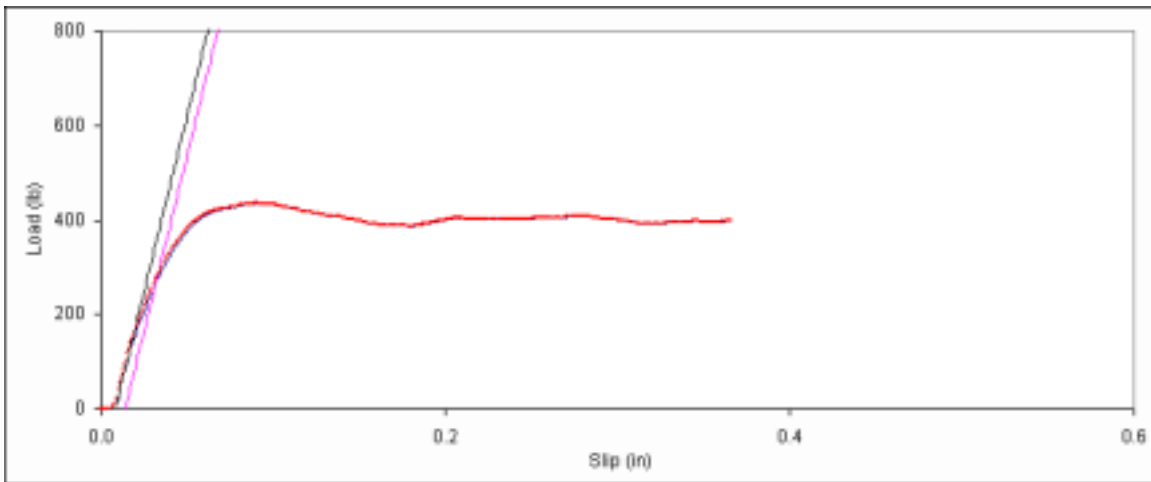
Figure D. 41: Bearing embedment plot for side member sample A-1.
