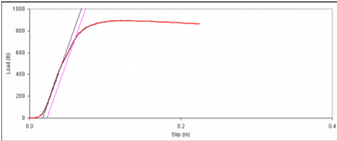
Figure D. 17: Bearing embedment plot for main member sample 6d-17.
