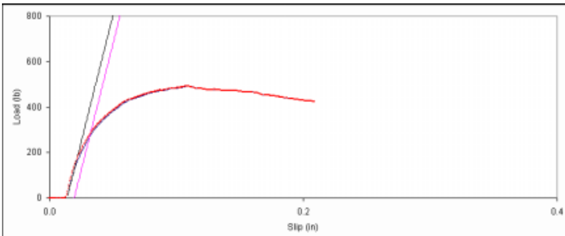
Figure D. 51: Bearing embedment plot for side member sample A-11.
