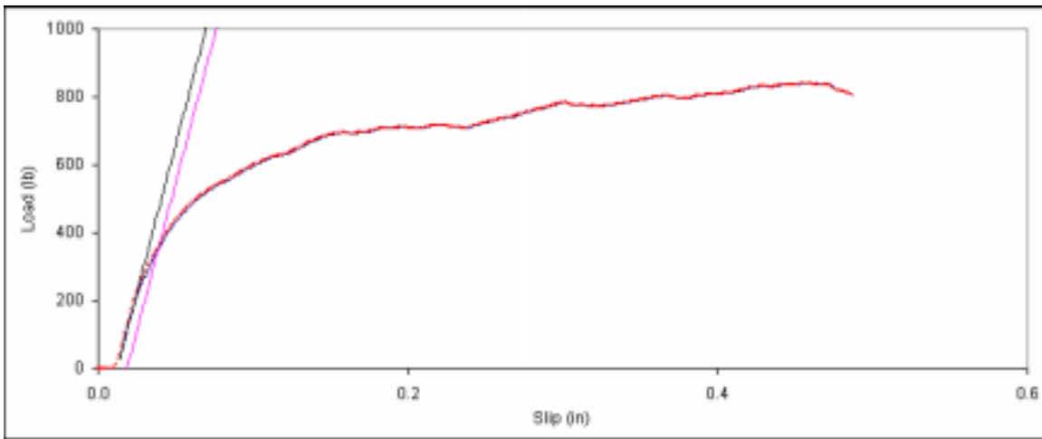
Figure D. 137: Bearing embedment plot for side member sample E-17.
