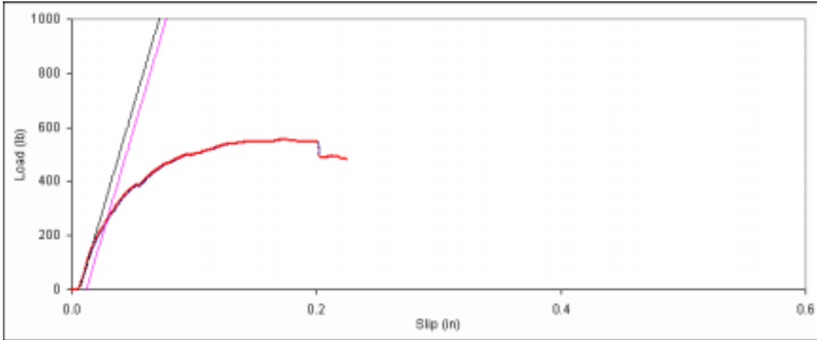
Figure D. 154: Bearing embedment plot for side member sample F-14.
