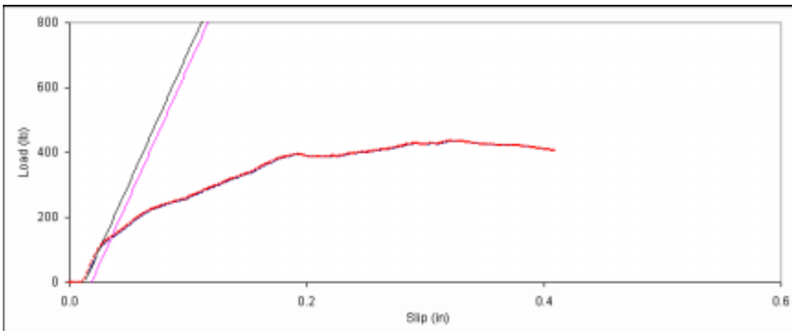
Figure D. 111: Bearing embedment plot for side member sample D-11.
