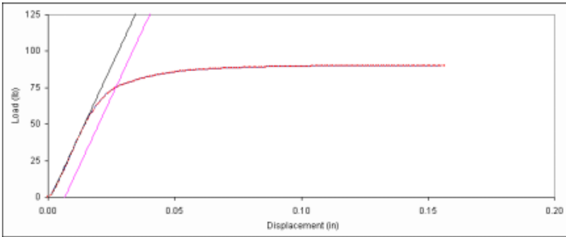
Figure D. 161: Bearing embedment plot for fastener sample 6d-1.
