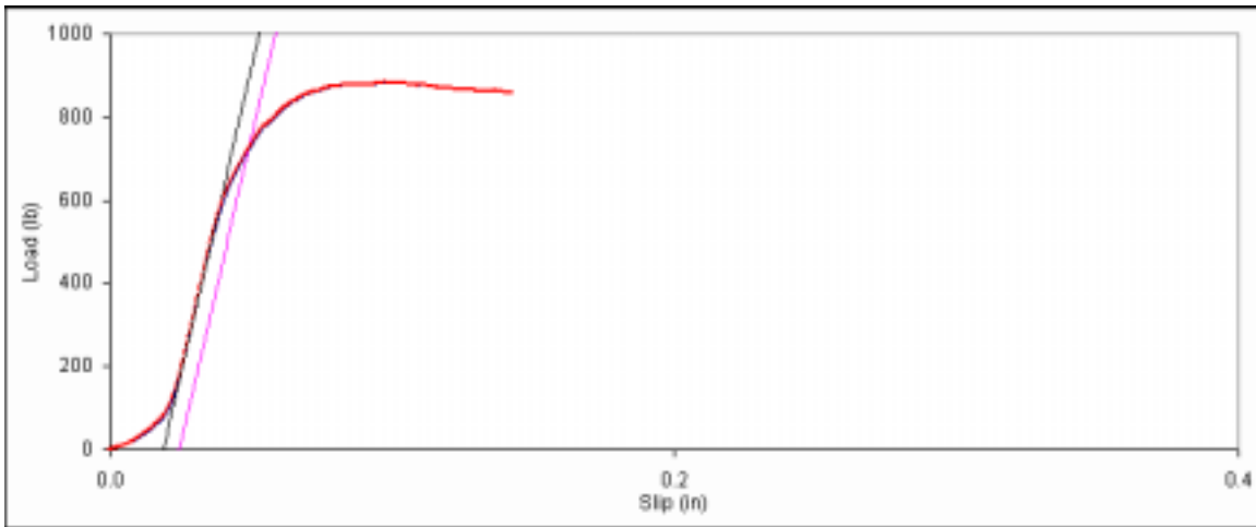
Figure D. 14: Bearing embedment plot for main member sample 6d-14.
