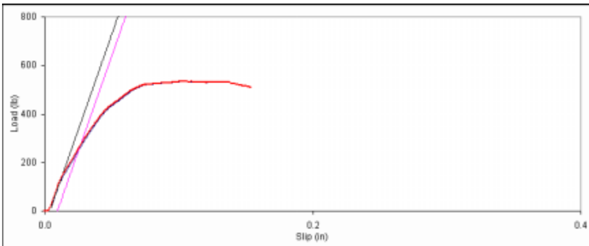
Figure D. 48: Bearing embedment plot for side member sample A-8.
