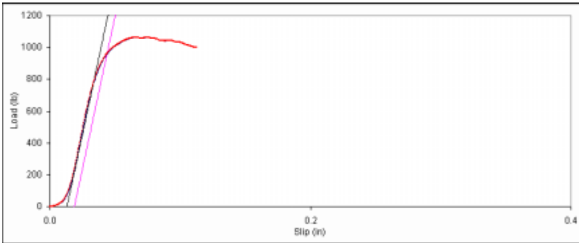
Figure D. 8: Bearing embedment plot for main member sample 6d-8.
