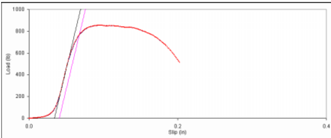
Figure D. 24: Bearing embedment plot for main member sample 8d-4.
