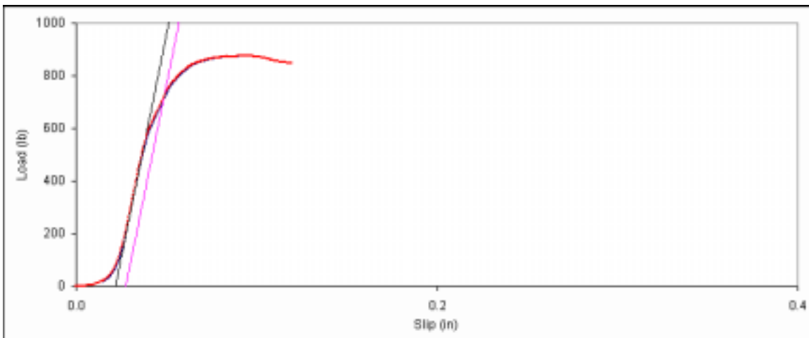
Figure D. 12: Bearing embedment plot for main member sample 6d-12.
