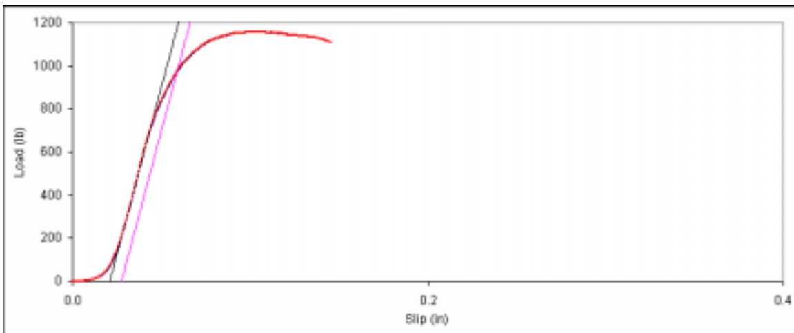
Figure D. 33: Bearing embedment plot for main member sample 8d-13.
