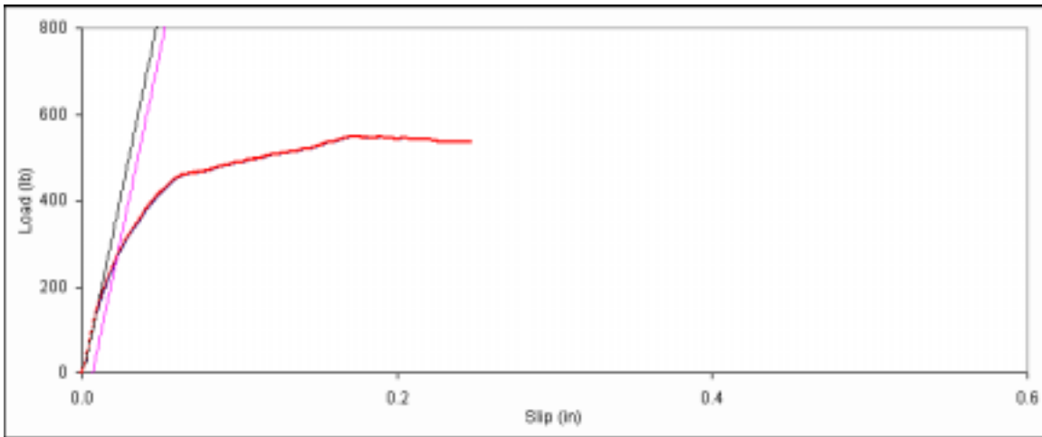
Figure D. 104: Bearing embedment plot for side member sample D-4.
