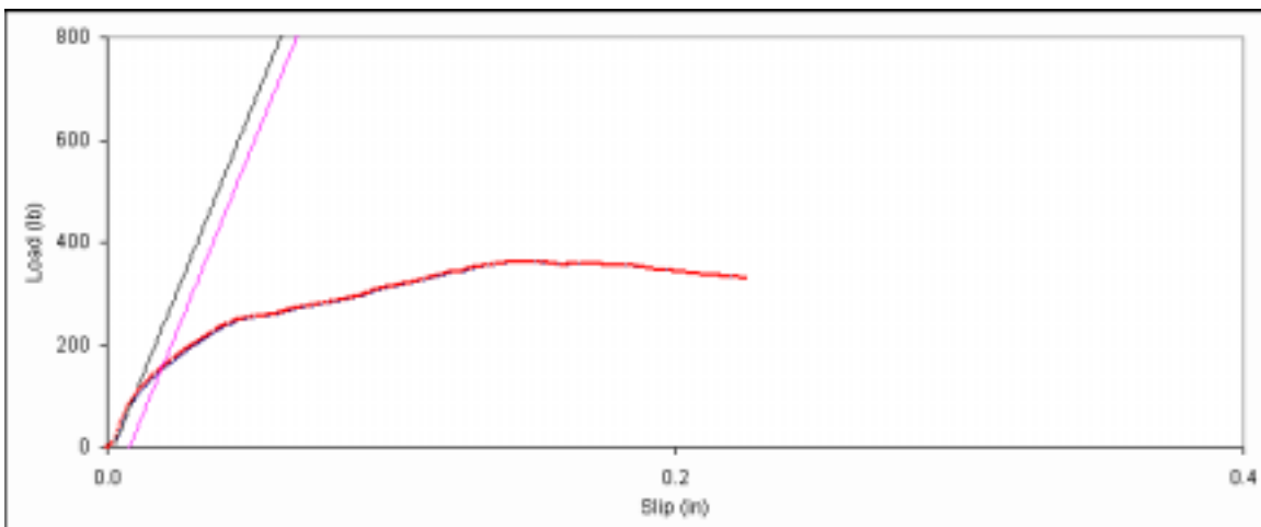
Figure D. 42: Bearing embedment plot for side member sample A-2.
