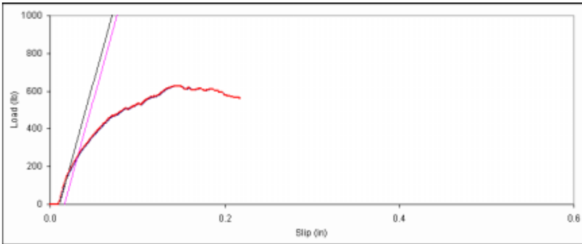
Figure D. 155: Bearing embedment plot for side member sample F-15.
