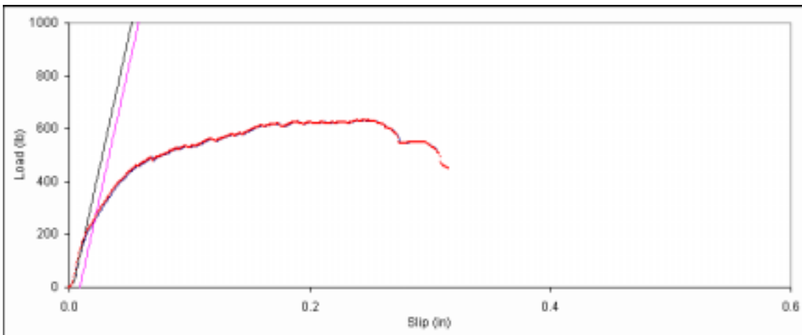
Figure D. 150: Bearing embedment plot for side member sample F-10.
