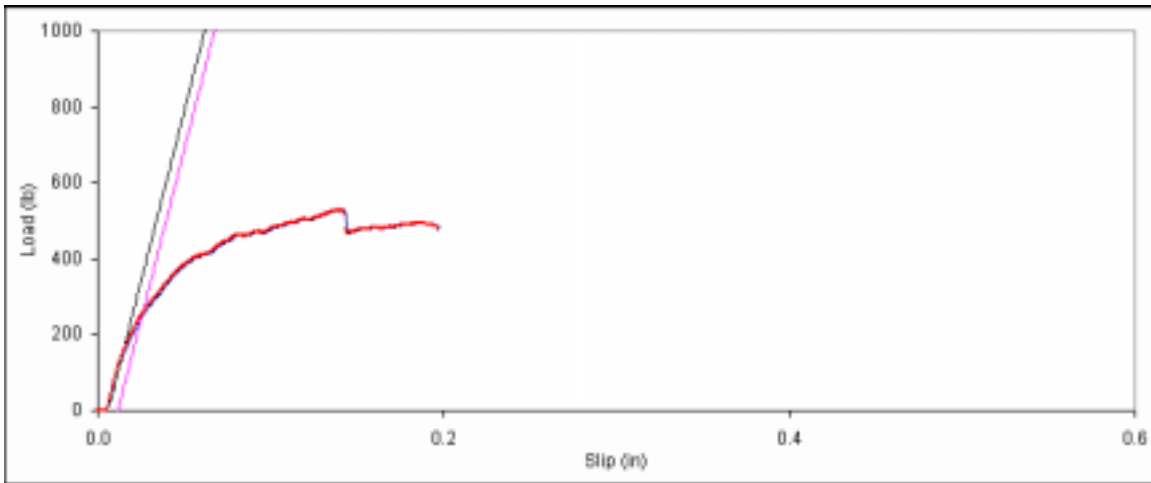
Figure D. 158: Bearing embedment plot for side member sample F-18.
