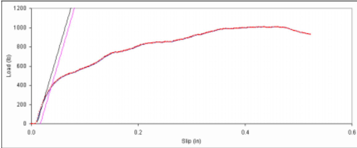
Figure D. 127: Bearing embedment plot for side member sample E-7.
