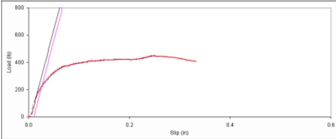
Figure D. 112: Bearing embedment plot for side member sample D-12.
