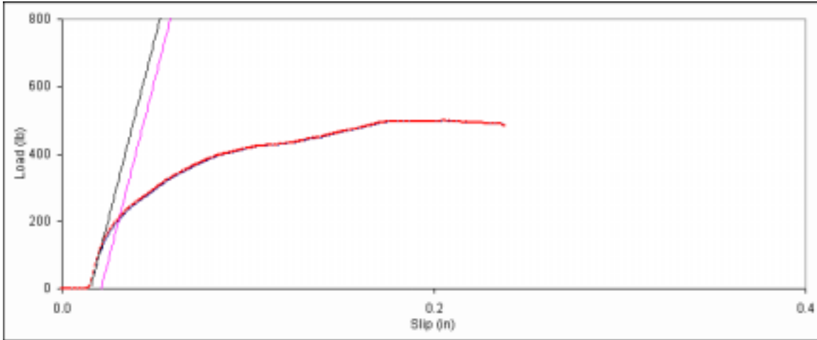
Figure D. 88: Bearing embedment plot for side member sample C-8.
