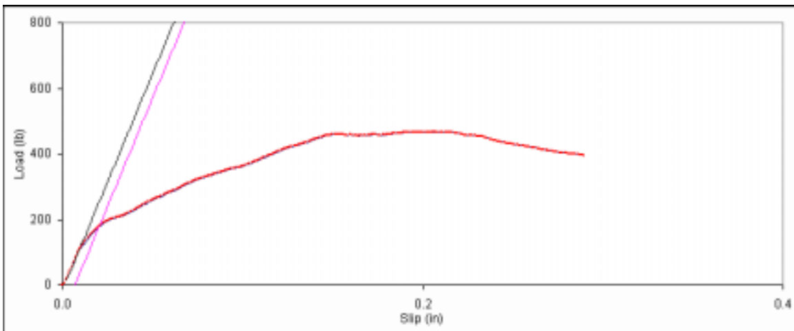
Figure D. 99: Bearing embedment plot for side member sample C-19.
