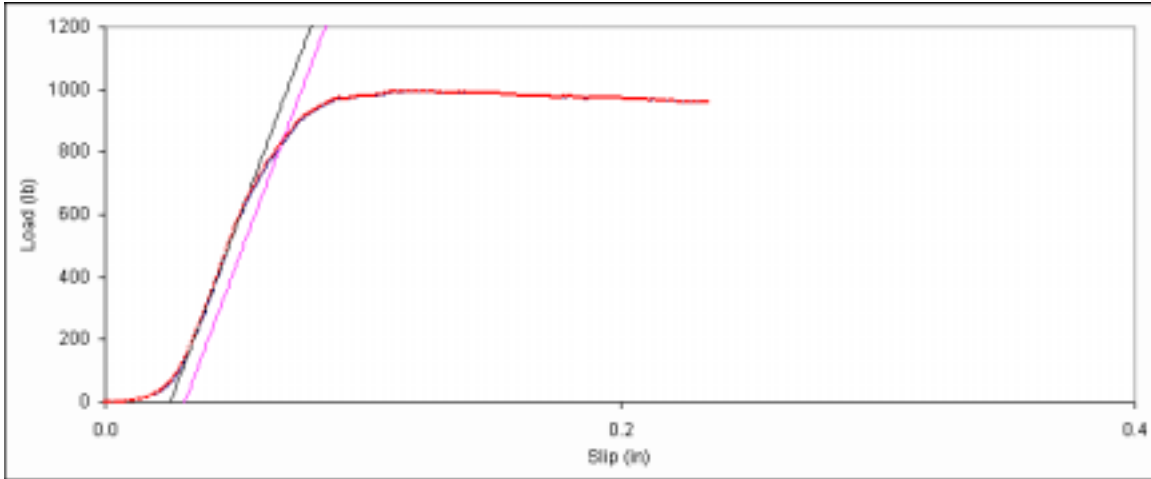
Figure D. 13: Bearing embedment plot for main member sample 6d-13.
