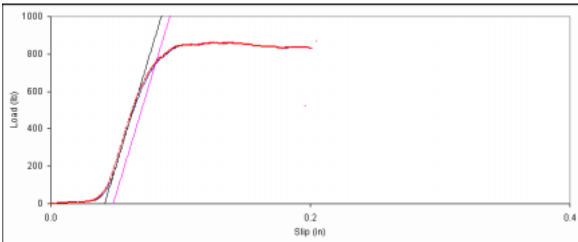
Figure D. 27: Bearing embedment plot for main member sample 8d-7.
