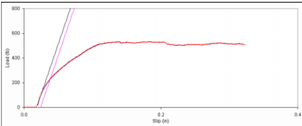
Figure D. 72: Bearing embedment plot for side member sample B-12.
