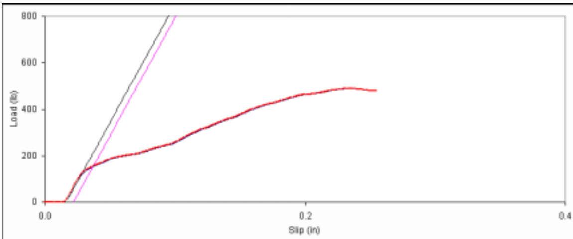
Figure D. 87: Bearing embedment plot for side member sample C-7.
