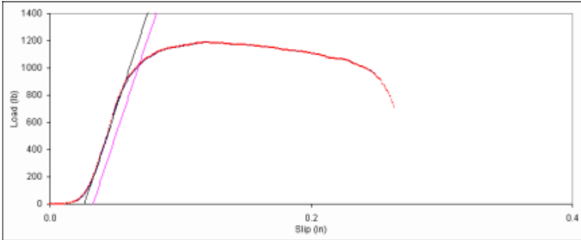
Figure D. 40: Bearing embedment plot for main member sample 8d-20.
