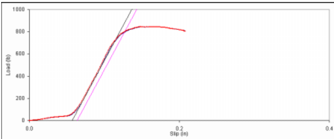
Figure D. 36: Bearing embedment plot for main member sample 8d-16.
