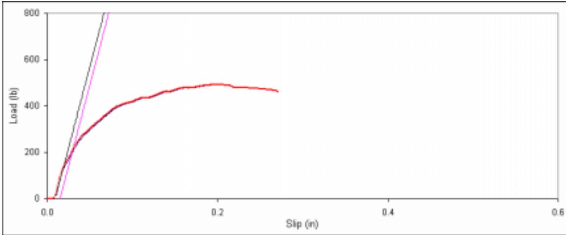
Figure D. 109: Bearing embedment plot for side member sample D-9.
