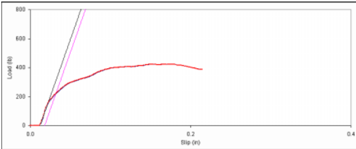
Figure D. 62: Bearing embedment plot for side member sample B-2.
