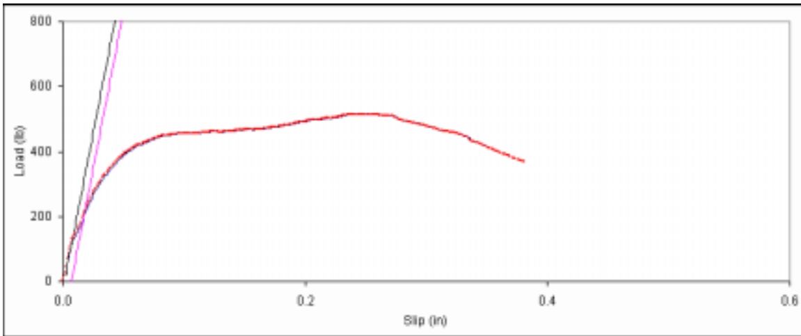
Figure D. 107: Bearing embedment plot for side member sample D-7.
