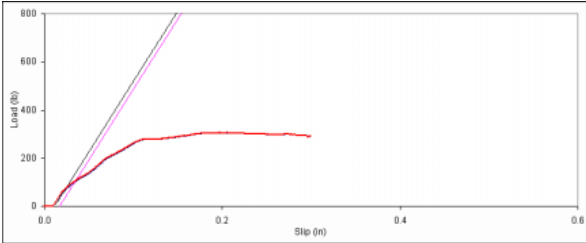
Figure D. 118: Bearing embedment plot for side member sample D-18.
