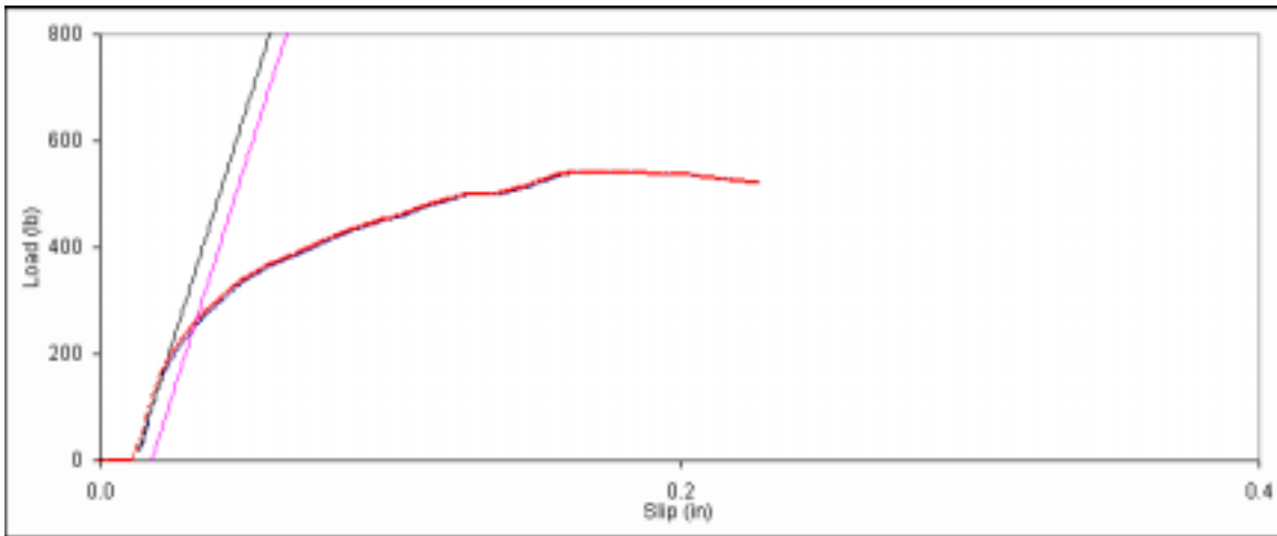
Figure D. 86: Bearing embedment plot for side member sample C-6.
