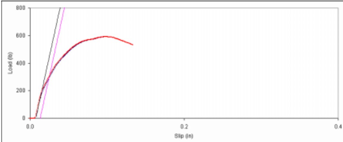
Figure D. 91: Bearing embedment plot for side member sample C-11.
