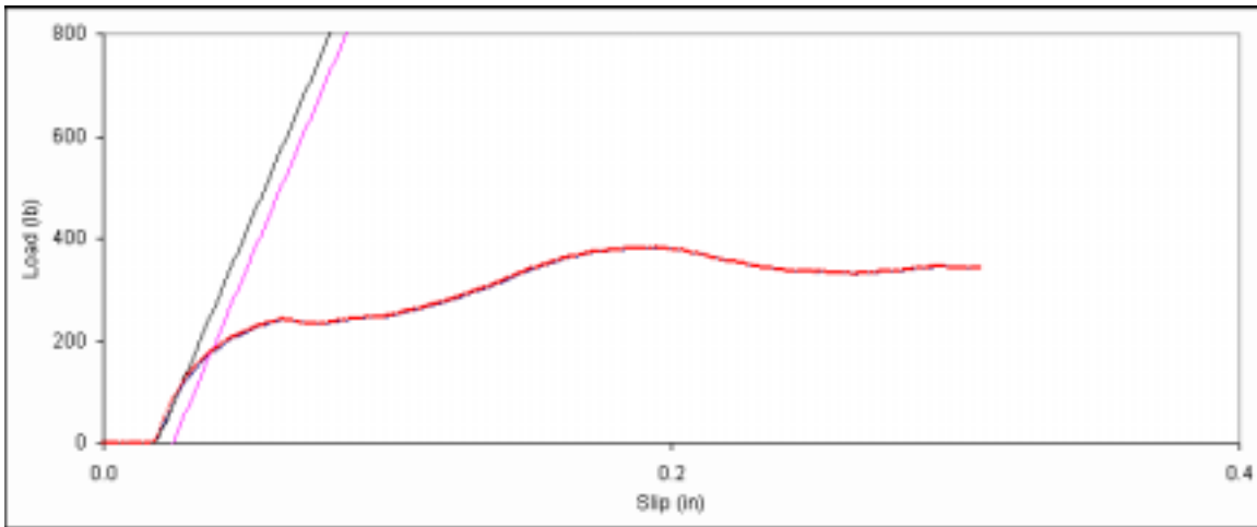
Figure D. 83: Bearing embedment plot for side member sample C-3.
