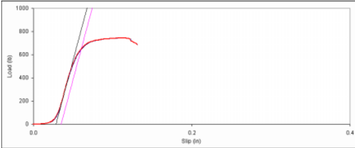
Figure D. 22: Bearing embedment plot for main member sample 8d-2.
