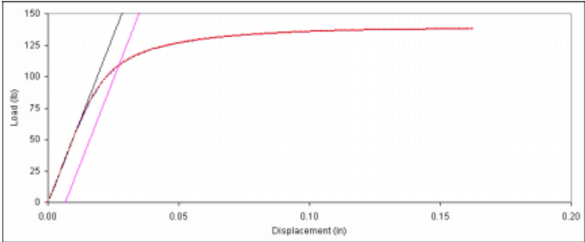
Figure D. 178: Bearing embedment plot for fastener sample 8d-8.
