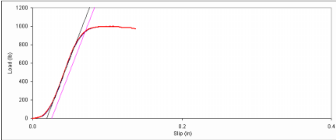
Figure D. 31: Bearing embedment plot for main member sample 8d-11.
