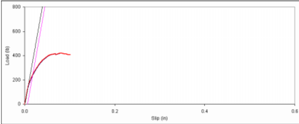
Figure D. 103: Bearing embedment plot for side member sample D-3.
