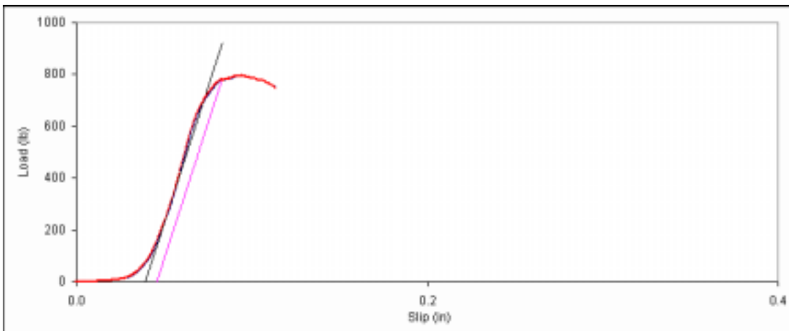
Figure D. 21: Bearing embedment plot for main member sample 8d-1.
