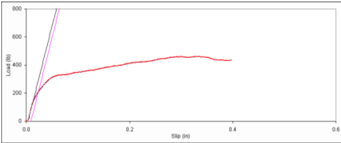
Figure D. 110: Bearing embedment plot for side member sample D-10.
