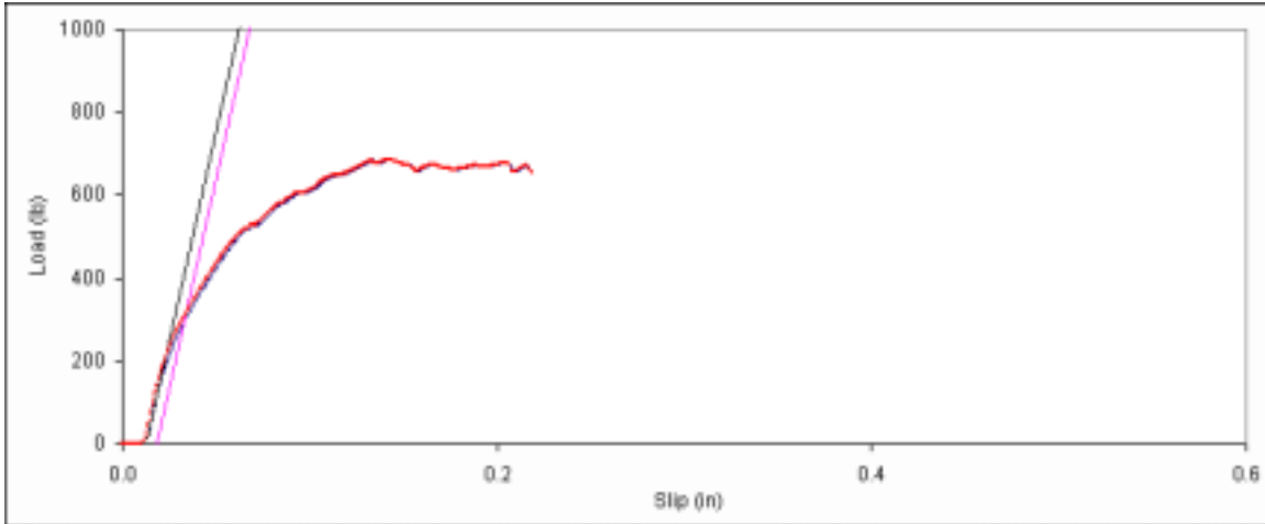
Figure D. 151: Bearing embedment plot for side member sample F-11.
