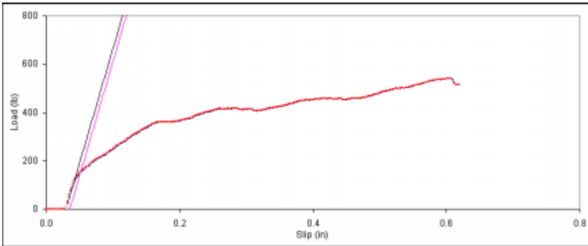
Figure D. 53: Bearing embedment plot for side member sample A-13.
