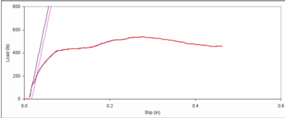
Figure D. 97: Bearing embedment plot for side member sample C-17.
