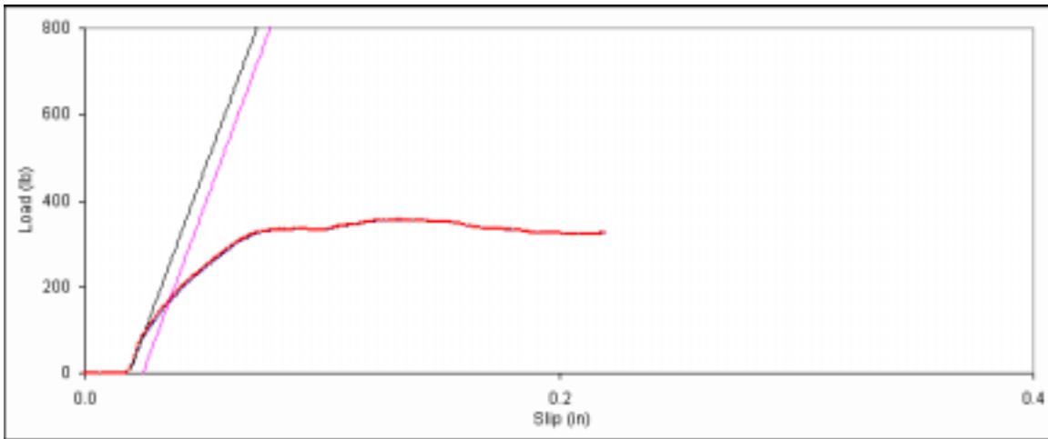
Figure D. 74: Bearing embedment plot for side member sample B-14.
