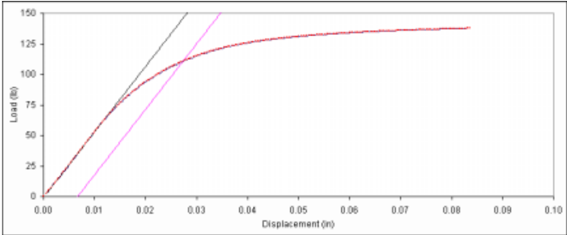
Figure D. 175: Bearing embedment plot for fastener sample 8d-5.
