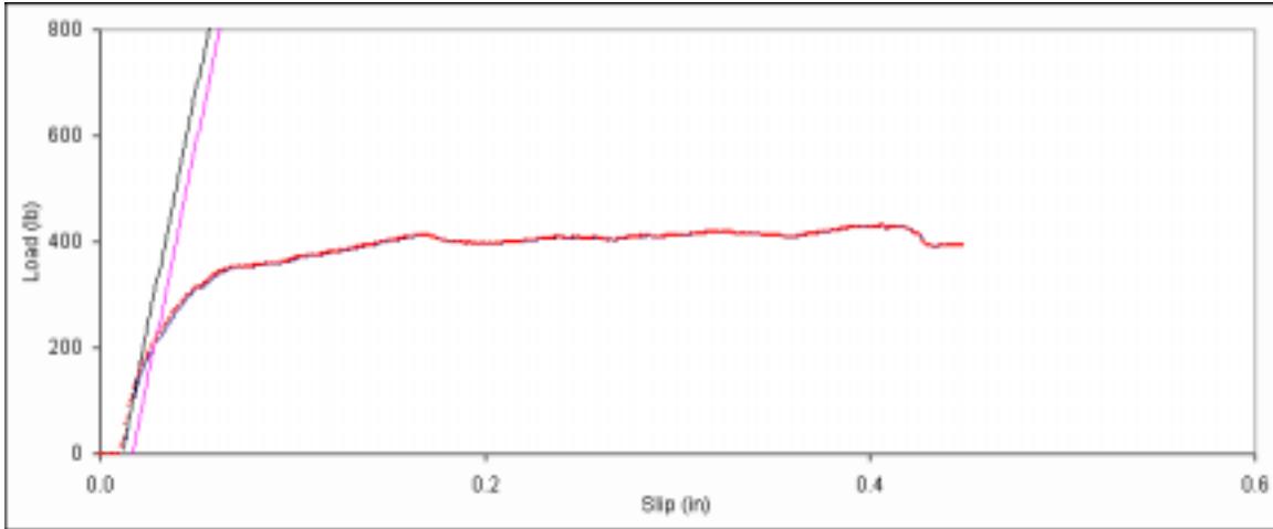
Figure D. 46: Bearing embedment plot for side member sample A-6.
