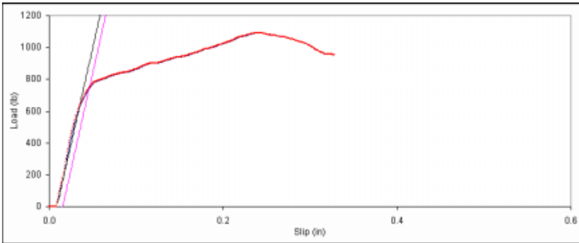
Figure D. 128: Bearing embedment plot for side member sample E-8.
