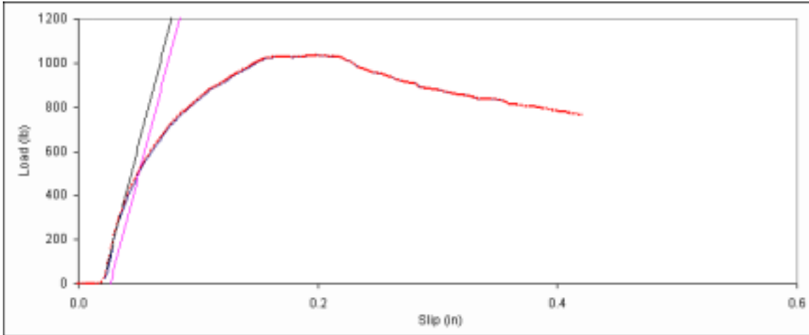
Figure D. 136: Bearing embedment plot for side member sample E-16.
