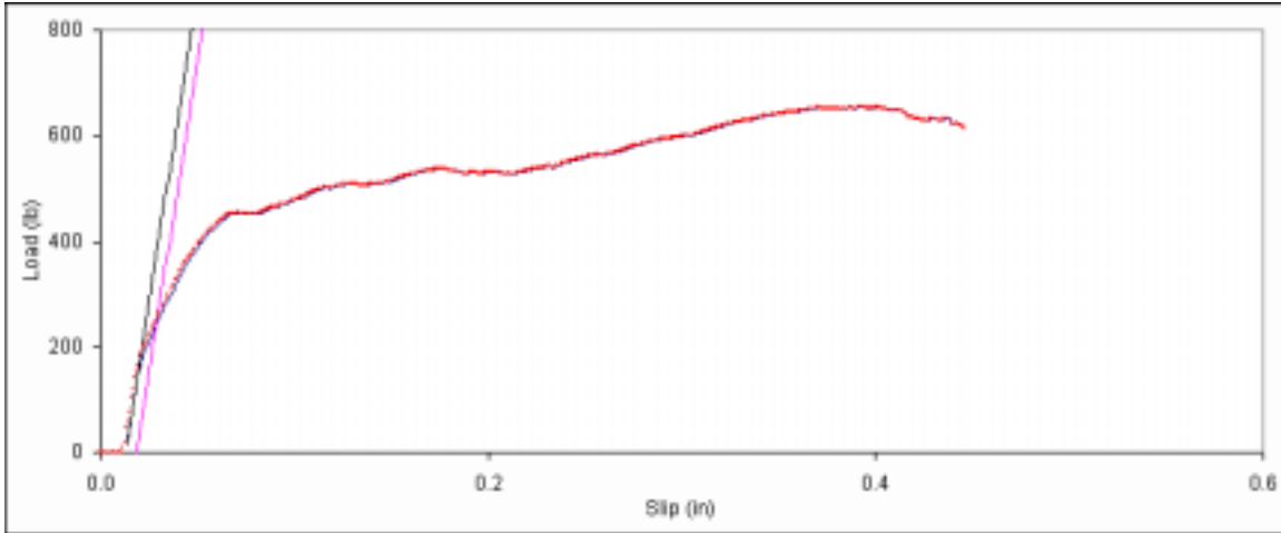
Figure D. 73: Bearing embedment plot for side member sample B-13.
