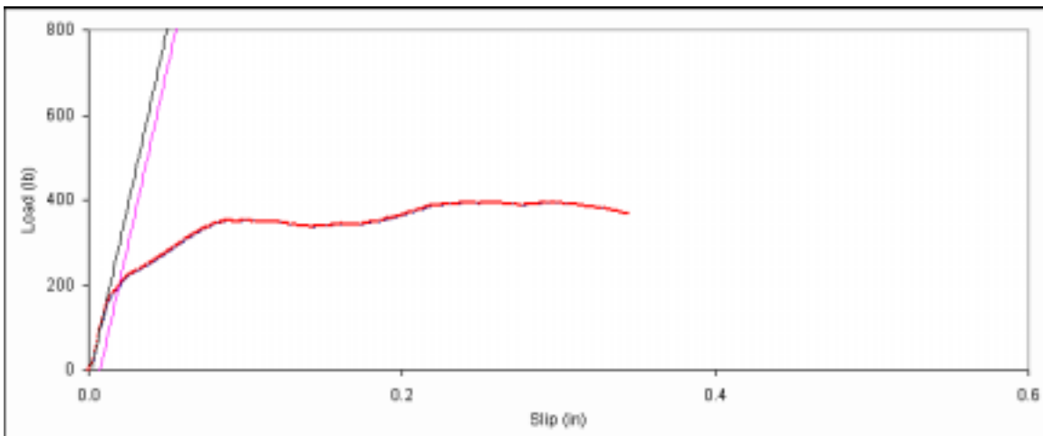
Figure D. 102: Bearing embedment plot for side member sample D-2.
