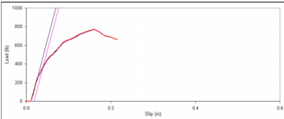
Figure D. 129: Bearing embedment plot for side member sample E-9.
