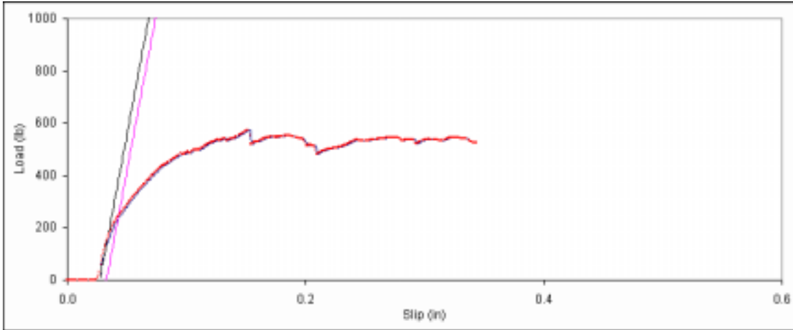
Figure D. 148: Bearing embedment plot for side member sample F-8.
