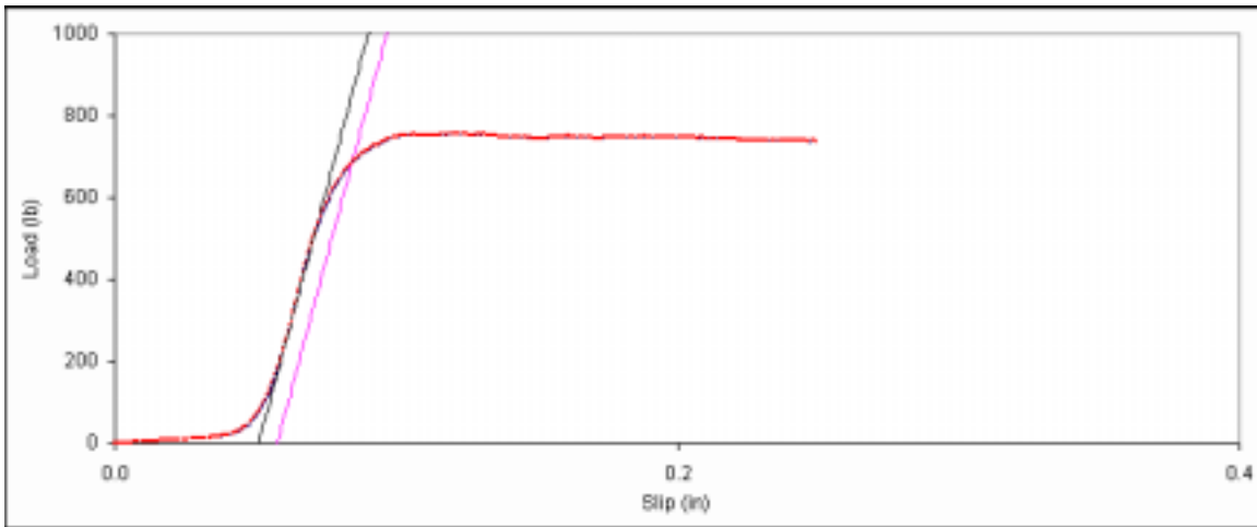
Figure D. 23: Bearing embedment plot for main member sample 8d-3.
