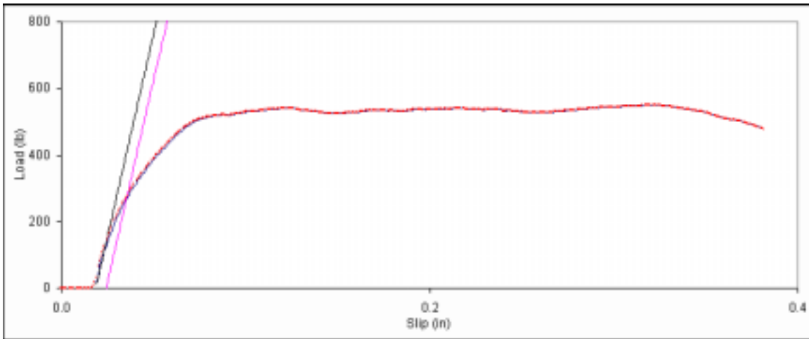
Figure D. 59: Bearing embedment plot for side member sample A-19.
