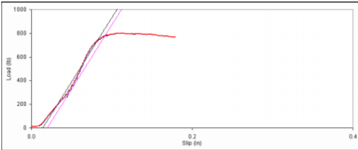
Figure D. 2: Bearing embedment plot for main member sample 6d-2.
