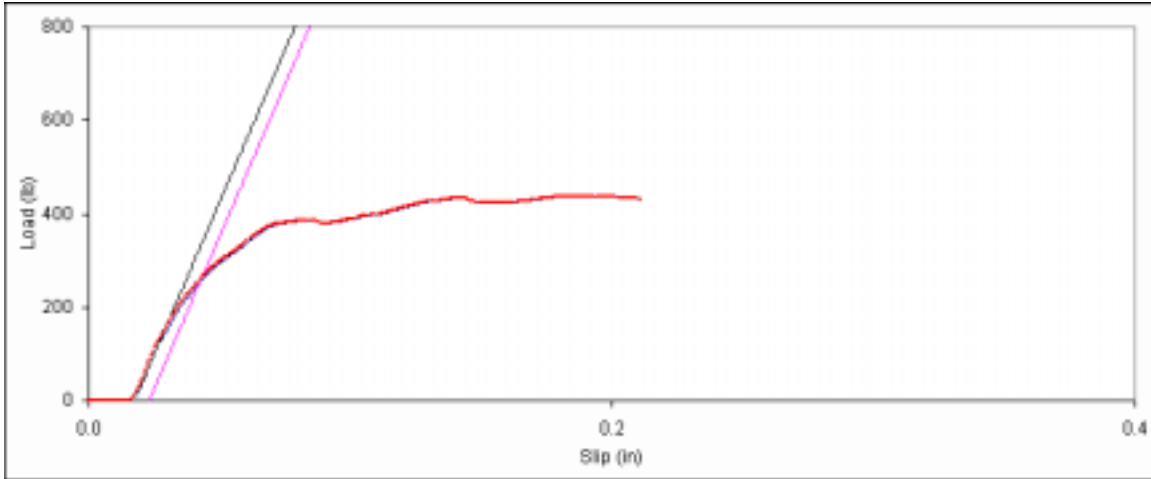
Figure D. 85: Bearing embedment plot for side member sample C-5.
