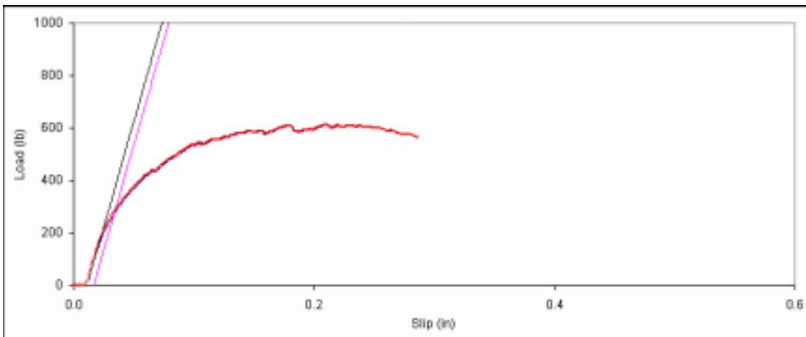
Figure D. 153: Bearing embedment plot for side member sample F-13.
