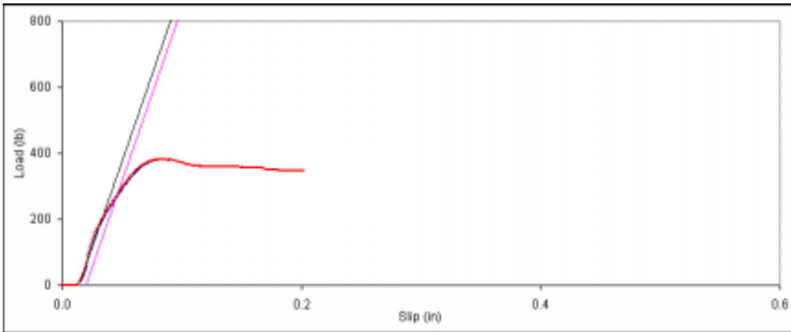
Figure D. 116: Bearing embedment plot for side member sample D-16.
