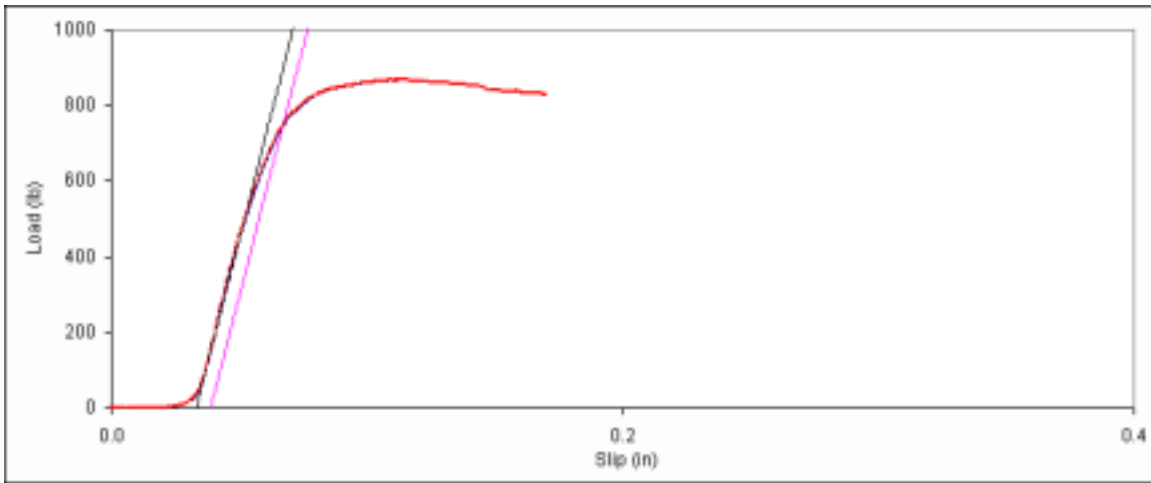
Figure D. 11: Bearing embedment plot for main member sample 6d-11.
