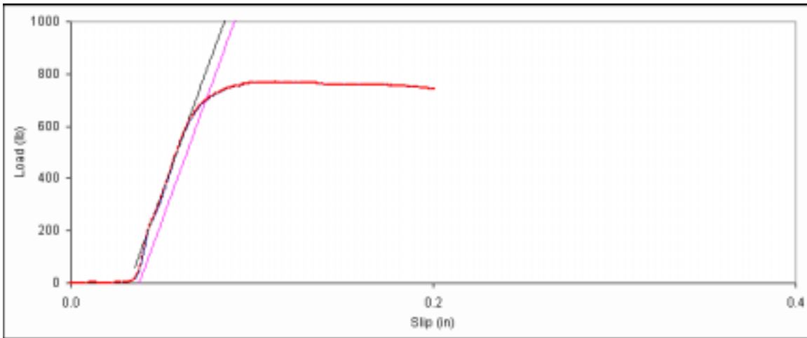
Figure D. 5: Bearing embedment plot for main member sample 6d-5.
