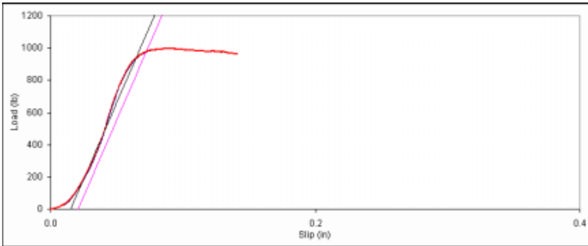
Figure D. 20: Bearing embedment plot for main member sample 6d-20.
