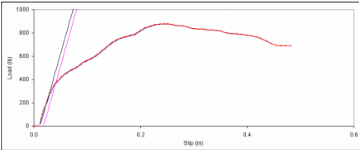
Figure D. 122: Bearing embedment plot for side member sample E-2.
