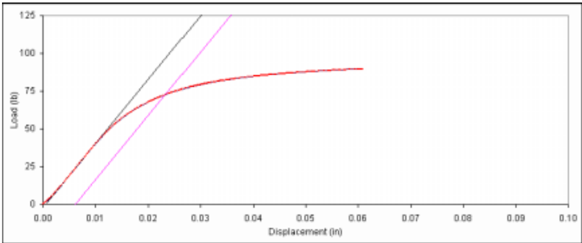
Figure D. 170: Bearing embedment plot for fastener sample 6d-10.
