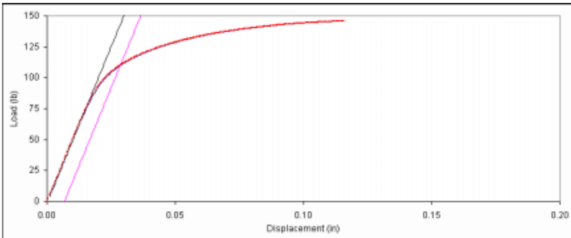
Figure D. 173: Bearing embedment plot for fastener sample 8d-3.
