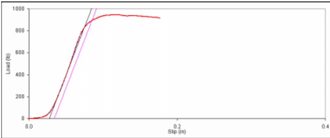
Figure D. 26: Bearing embedment plot for main member sample 8d-6.
