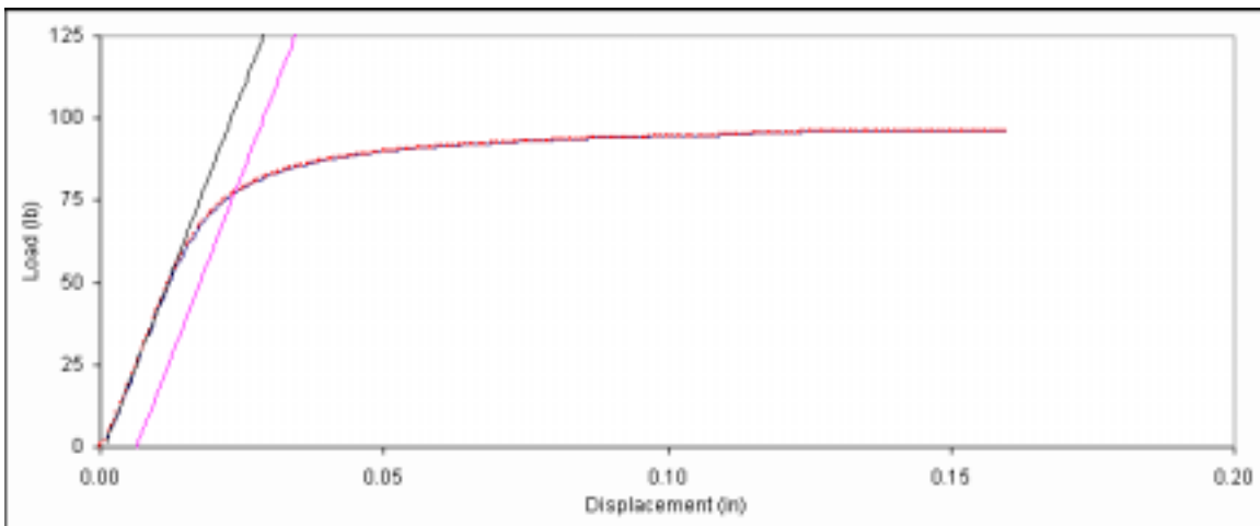
Figure D. 162: Bearing embedment plot for fastener sample 6d-2.
