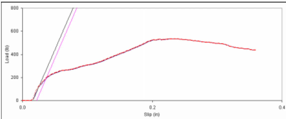
Figure D. 57: Bearing embedment plot for side member sample A-17.
