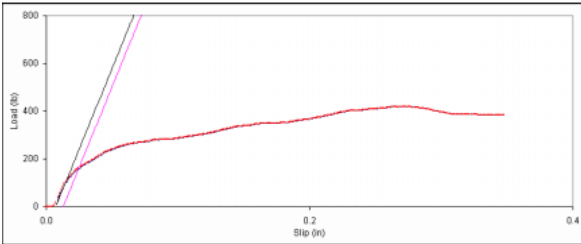
Figure D. 92: Bearing embedment plot for side member sample C-12.
