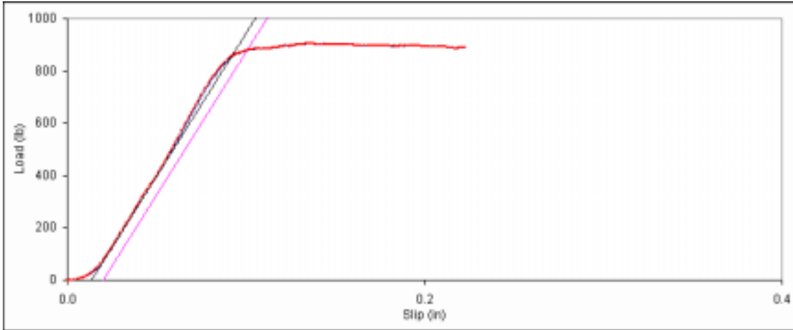
Figure D. 28: Bearing embedment plot for main member sample 8d-8.
