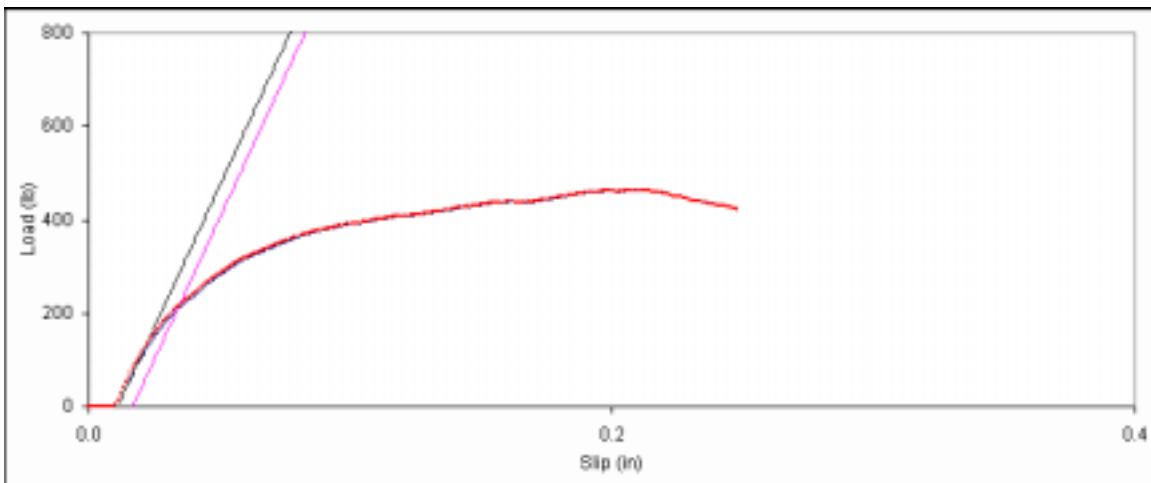
Figure D. 45: Bearing embedment plot for side member sample A-5.
