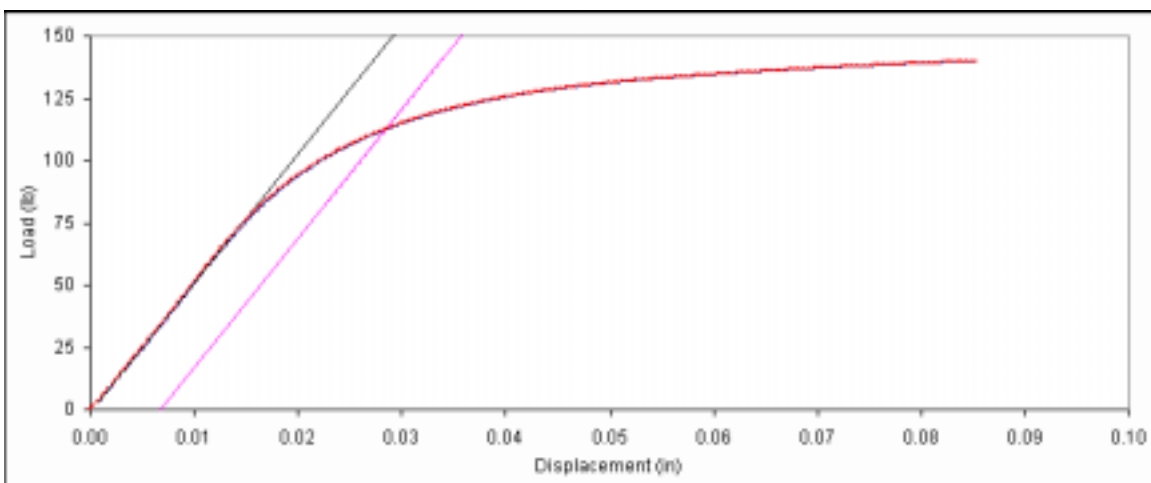
Figure D. 174: Bearing embedment plot for fastener sample 8d-4.
