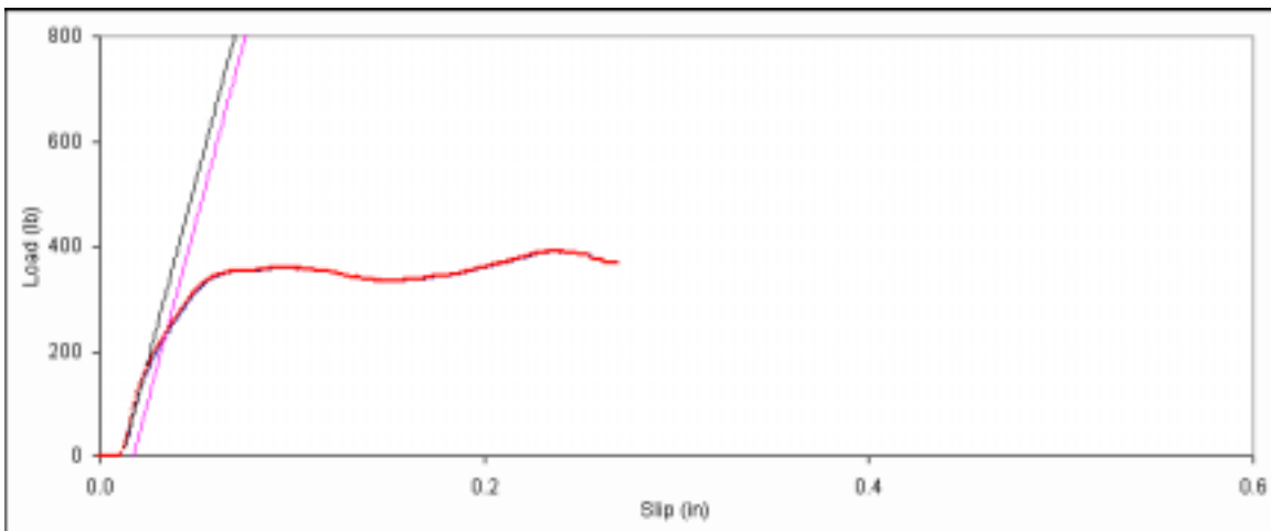
Figure D. 114: Bearing embedment plot for side member sample D-14.
