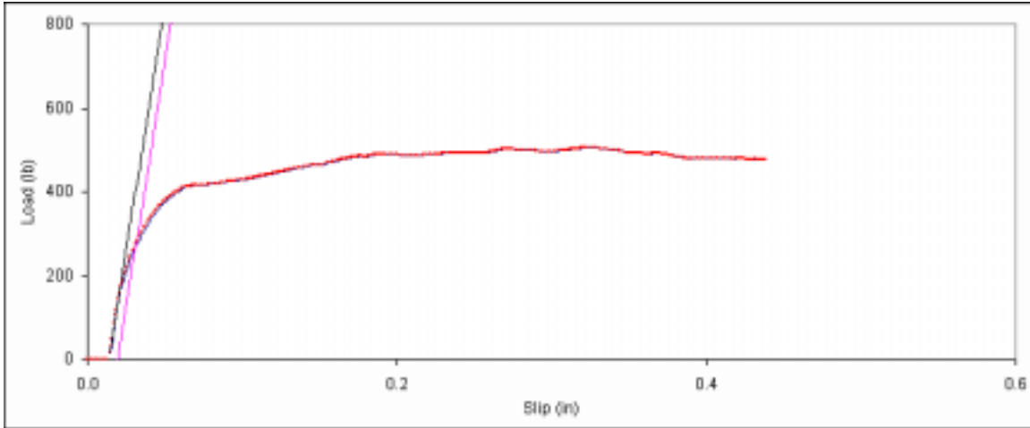
Figure D. 82: Bearing embedment plot for side member sample C-2.
