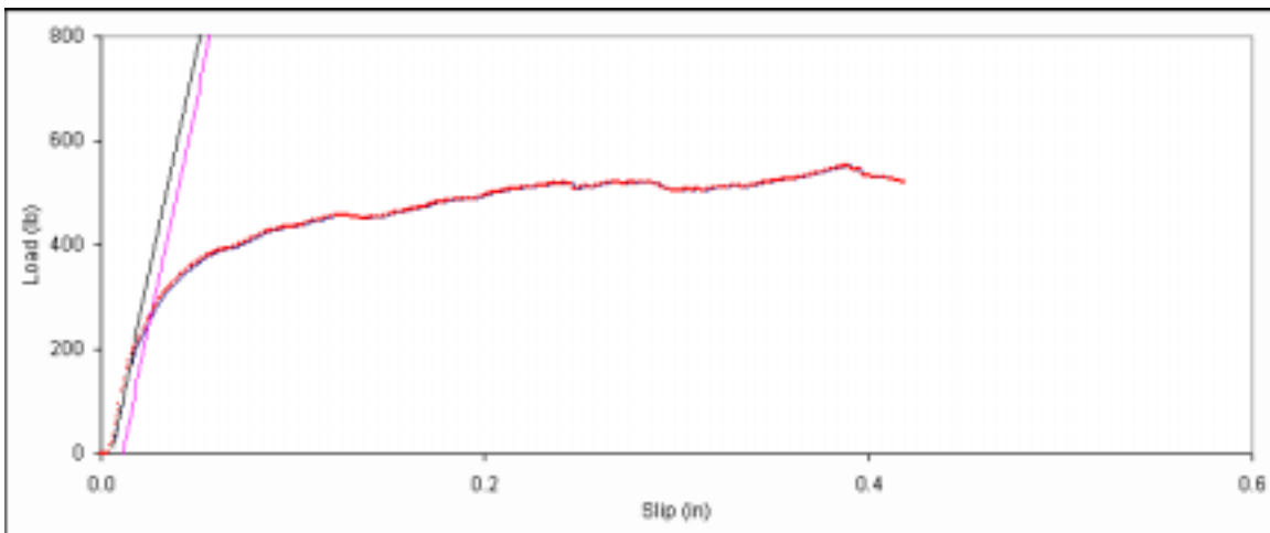
Figure D. 75: Bearing embedment plot for side member sample B-15.
