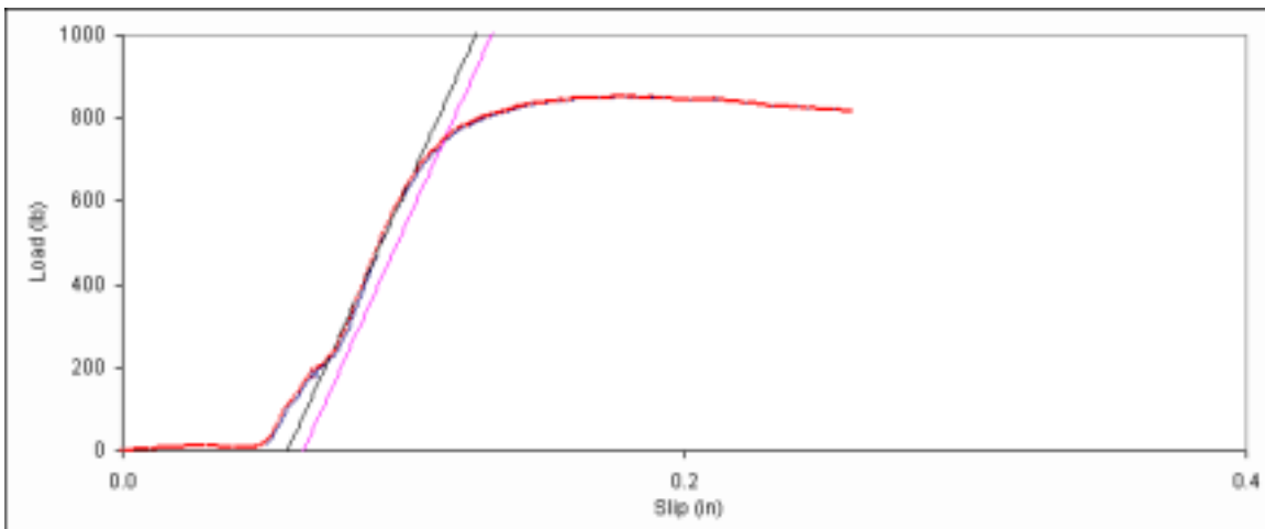
Figure D. 9: Bearing embedment plot for main member sample 6d-9.
