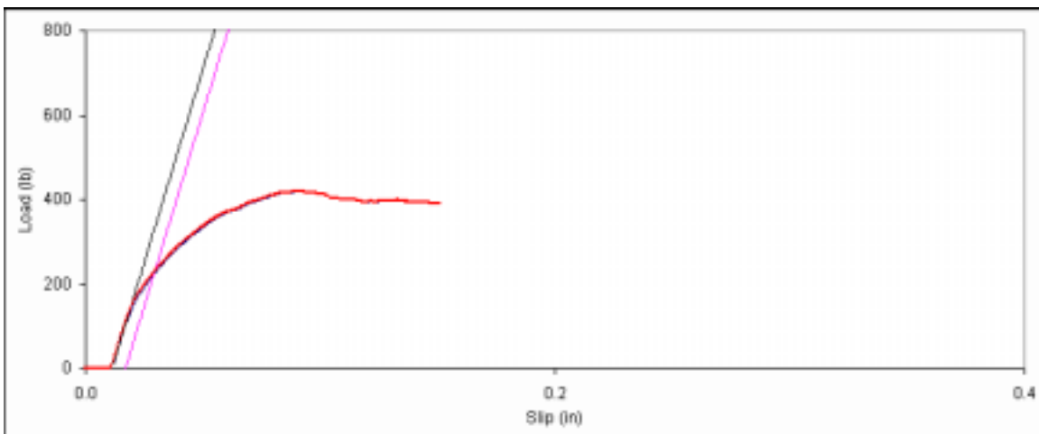
Figure D. 63: Bearing embedment plot for side member sample B-3.
