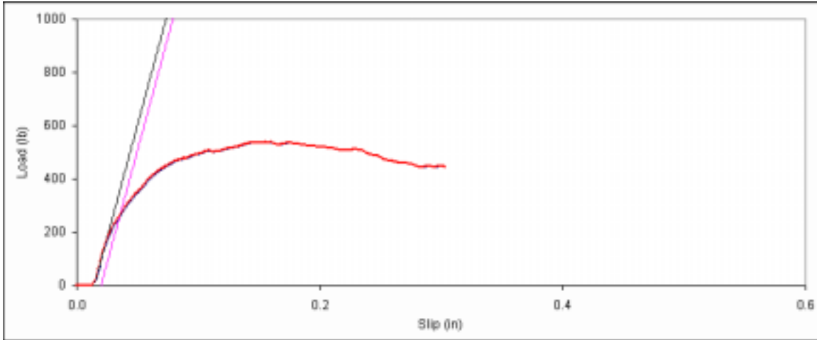
Figure D. 142: Bearing embedment plot for side member sample F-2.
