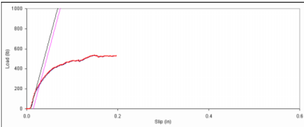
Figure D. 144: Bearing embedment plot for side member sample F-4.
