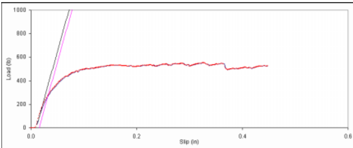
Figure D. 156: Bearing embedment plot for side member sample F-16.
