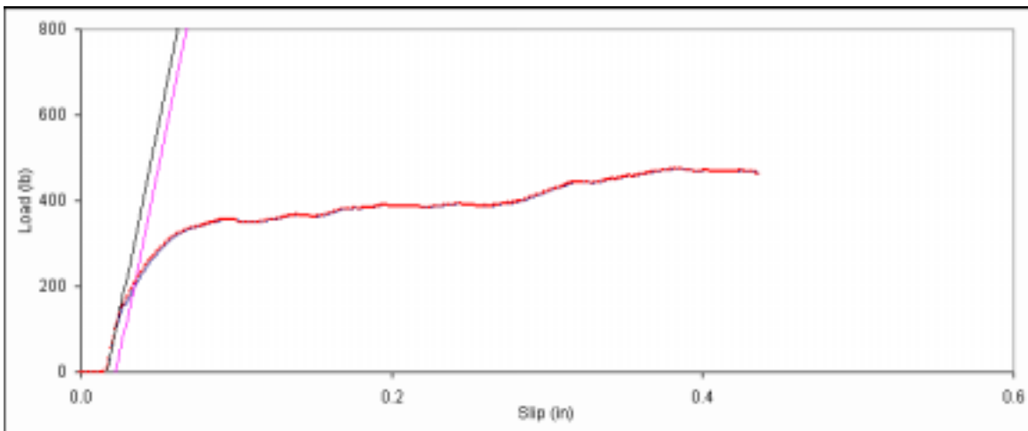
Figure D. 66: Bearing embedment plot for side member sample B-6.
