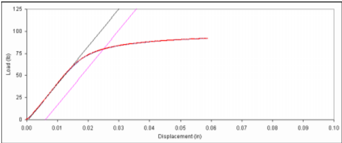
Figure D. 164: Bearing embedment plot for fastener sample 6d-4.
