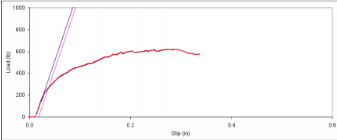
Figure D. 157: Bearing embedment plot for side member sample F-17.
