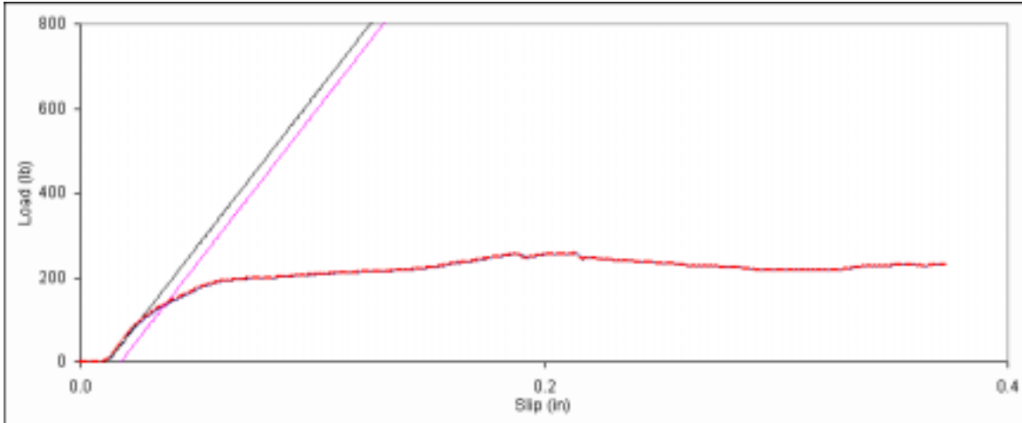
Figure D. 79: Bearing embedment plot for side member sample B-19.
