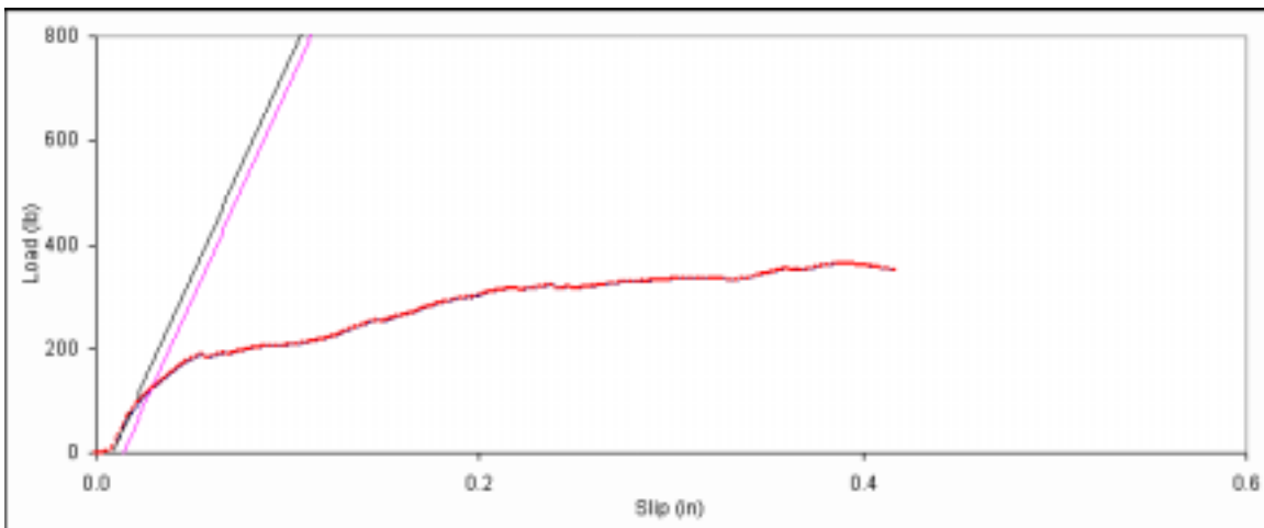
Figure D. 108: Bearing embedment plot for side member sample D-8.
