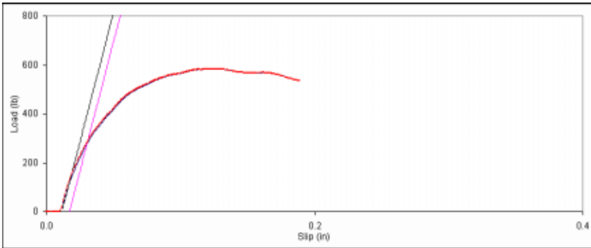
Figure D. 44: Bearing embedment plot for side member sample A-4.
