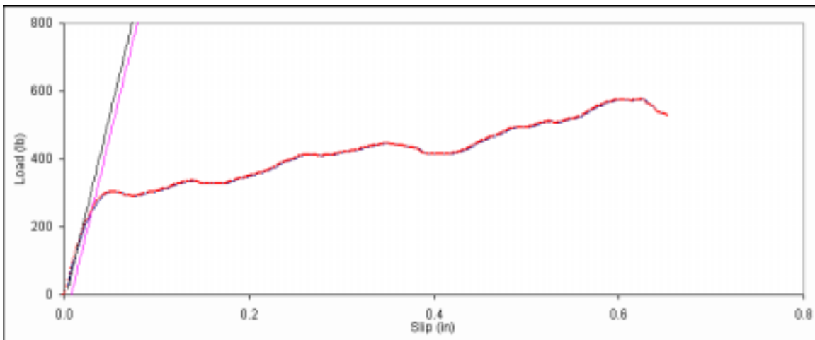
Figure D. 84: Bearing embedment plot for side member sample C-4.
