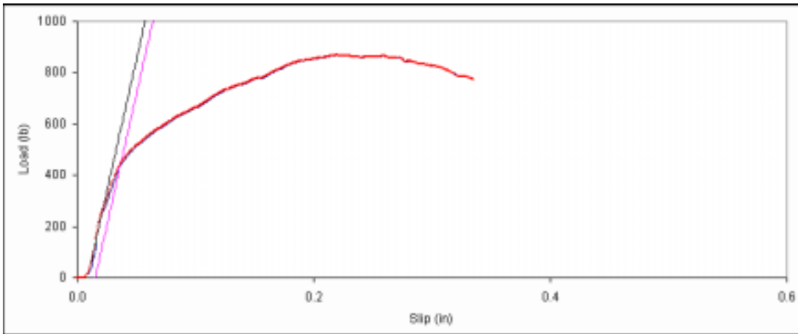
Figure D. 131: Bearing embedment plot for side member sample E-11.
