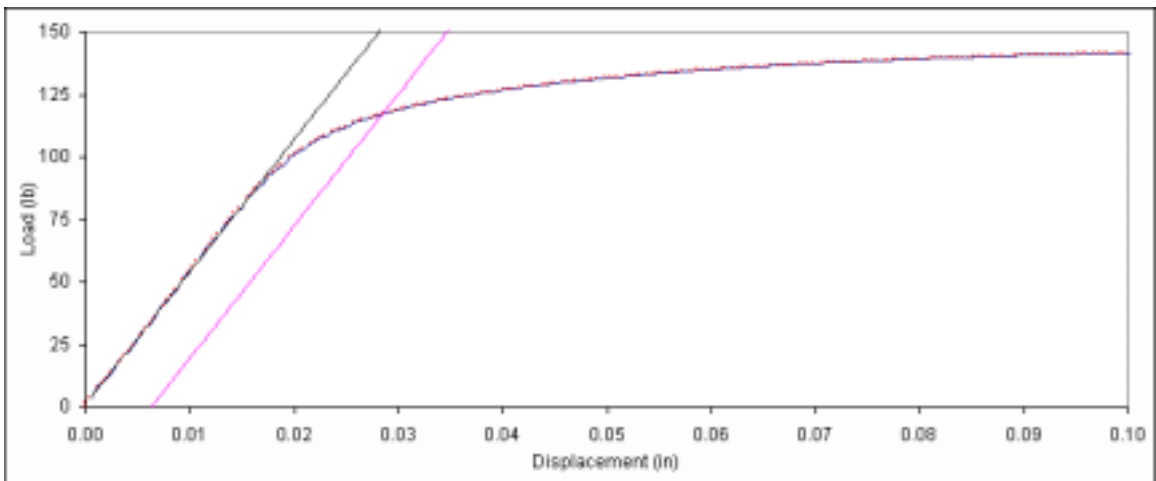
Figure D. 180: Bearing embedment plot for fastener sample 8d-10.
