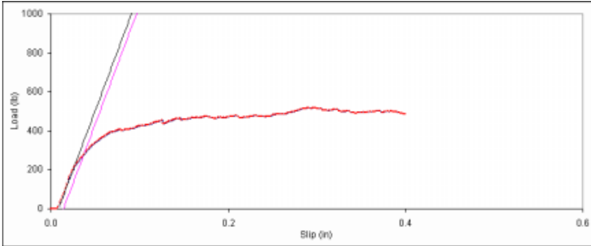
Figure D. 160: Bearing embedment plot for side member sample F-20.
