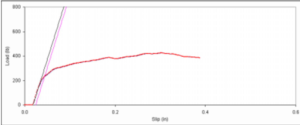
Figure D. 58: Bearing embedment plot for side member sample A-18.
