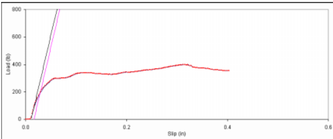
Figure D. 90: Bearing embedment plot for side member sample C-10.
