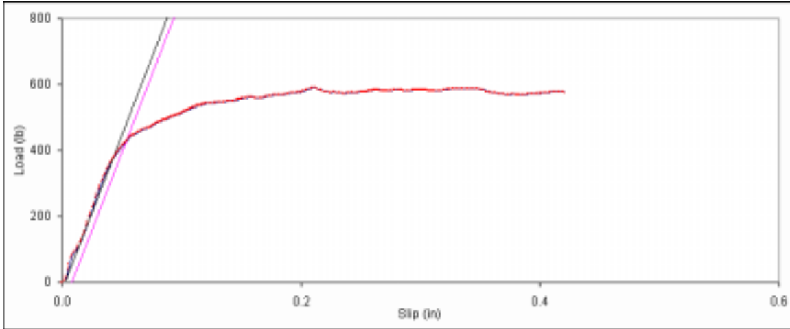
Figure D. 106: Bearing embedment plot for side member sample D-6.
