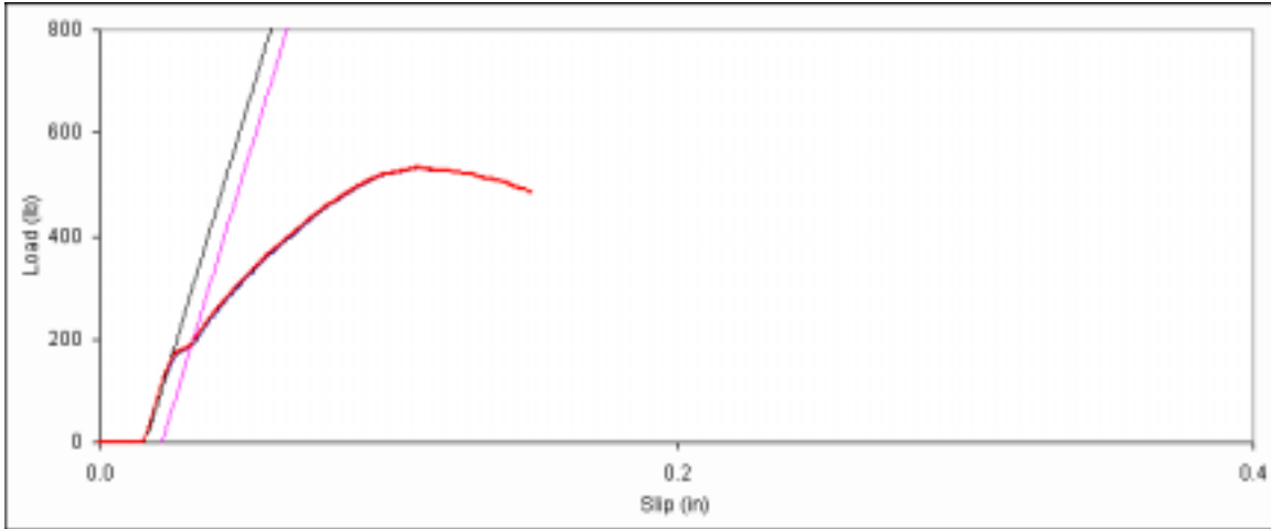
Figure D. 67: Bearing embedment plot for side member sample B-7.
