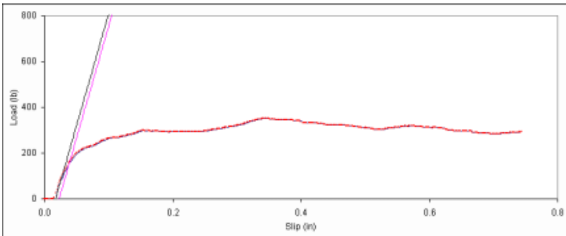
Figure D. 81: Bearing embedment plot for side member sample C-1.
