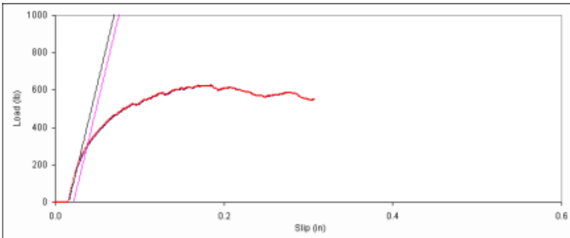
Figure D. 141: Bearing embedment plot for side member sample F-1.
