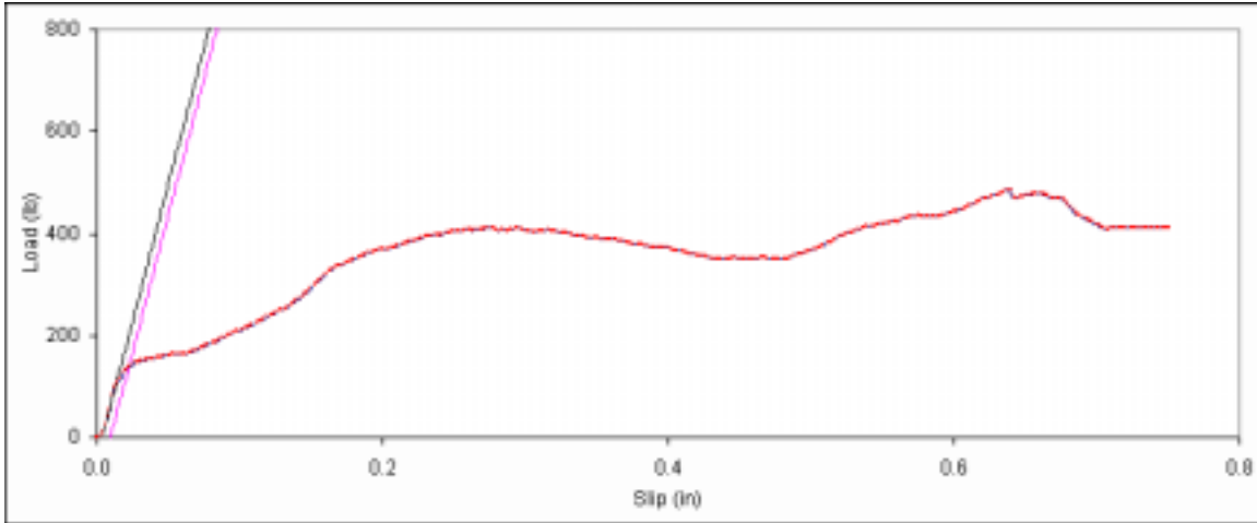
Figure D. 100: Bearing embedment plot for side member sample C-20.
