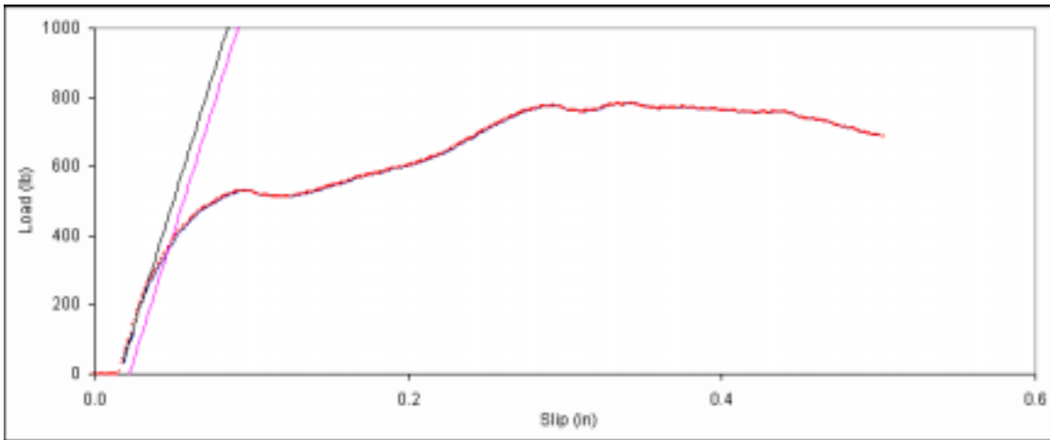
Figure D. 134: Bearing embedment plot for side member sample E-14.
