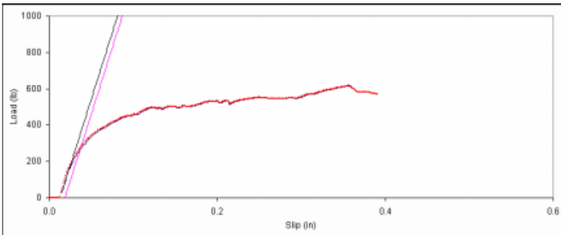
Figure D. 147: Bearing embedment plot for side member sample F-7.
