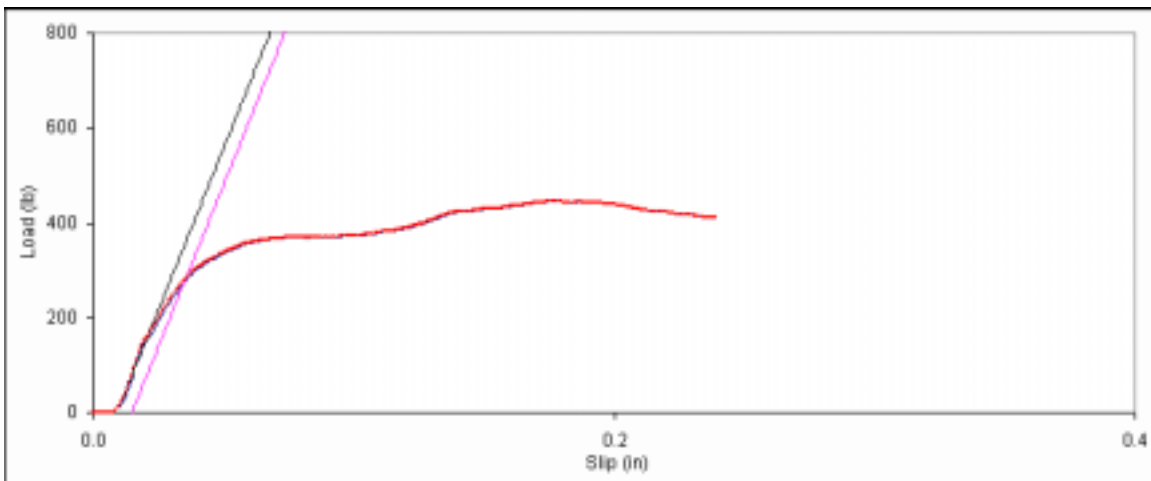
Figure D. 54: Bearing embedment plot for side member sample A-14.
