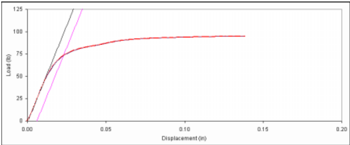
Figure D. 167: Bearing embedment plot for fastener sample 6d-7.
