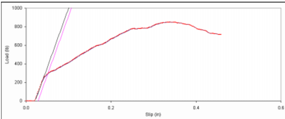
Figure D. 123: Bearing embedment plot for side member sample E-3.
