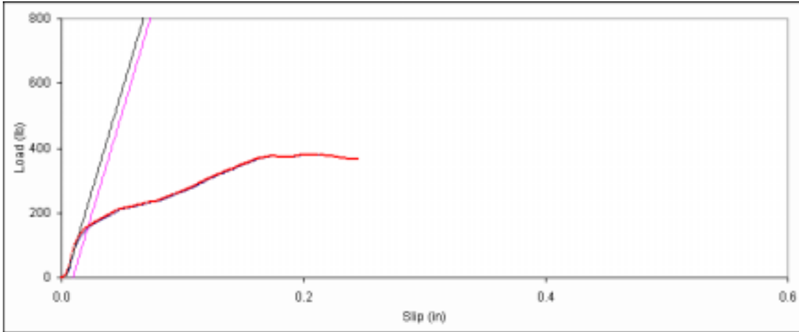
Figure D. 115: Bearing embedment plot for side member sample D-15.
