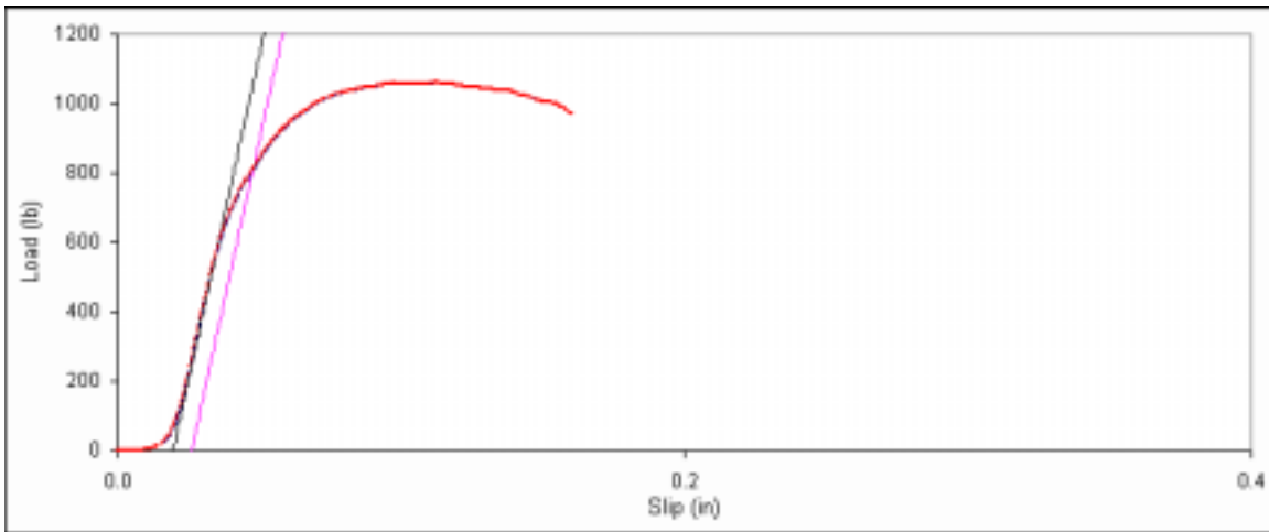
Figure D. 29: Bearing embedment plot for main member sample 8d-9.
