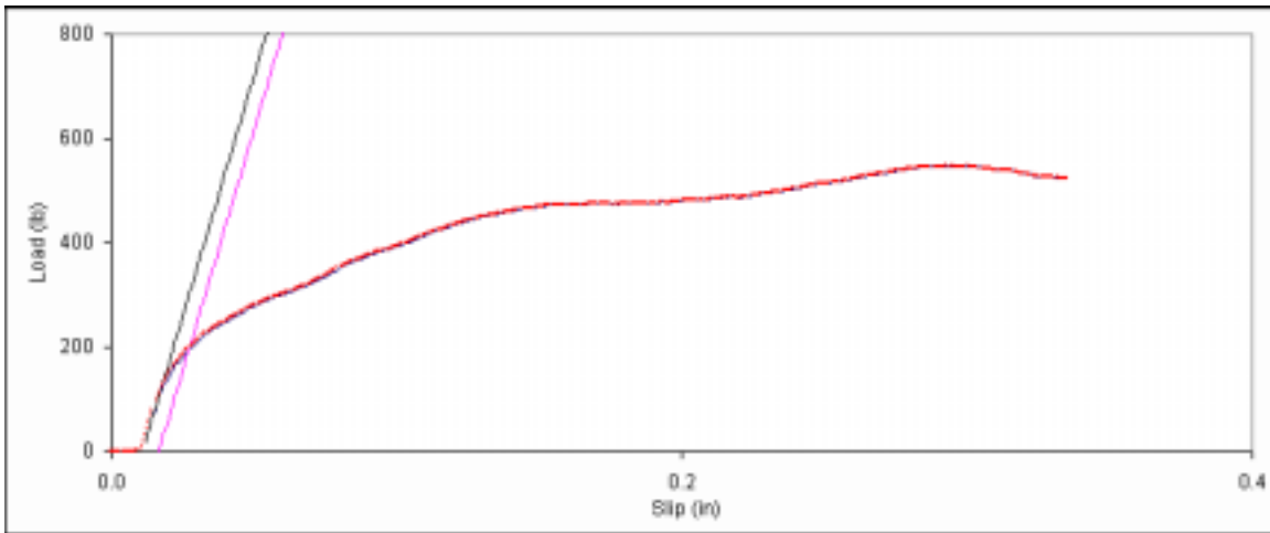
Figure D. 56: Bearing embedment plot for side member sample A-16.
