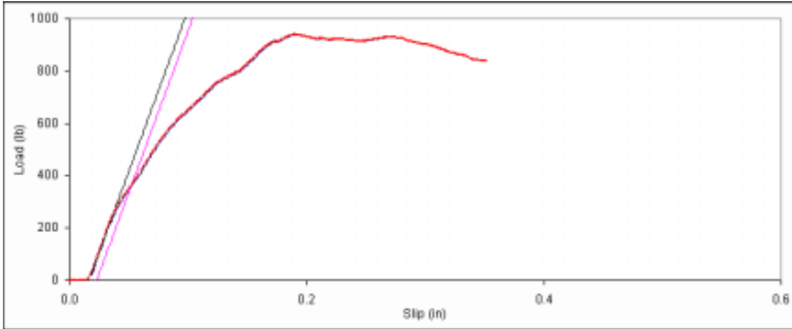
Figure D. 124: Bearing embedment plot for side member sample E-4.
