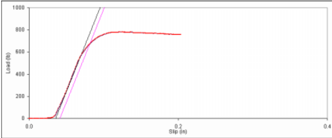
Figure D. 4: Bearing embedment plot for main member sample 6d-4.
