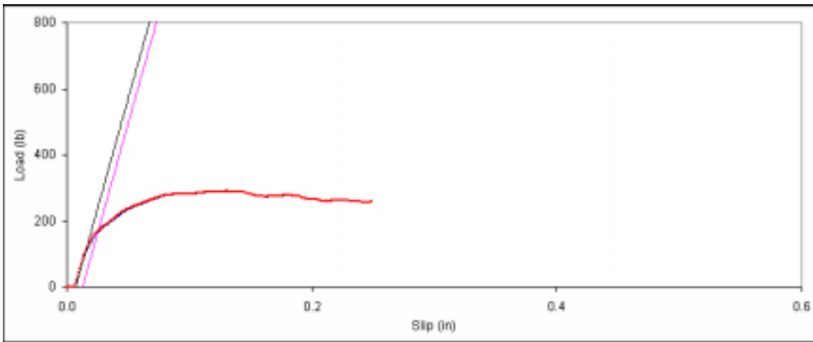
Figure D. 113: Bearing embedment plot for side member sample D-13.
