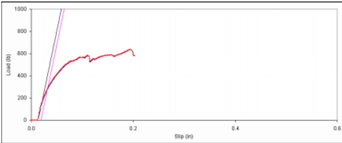
Figure D. 143: Bearing embedment plot for side member sample F-3.
