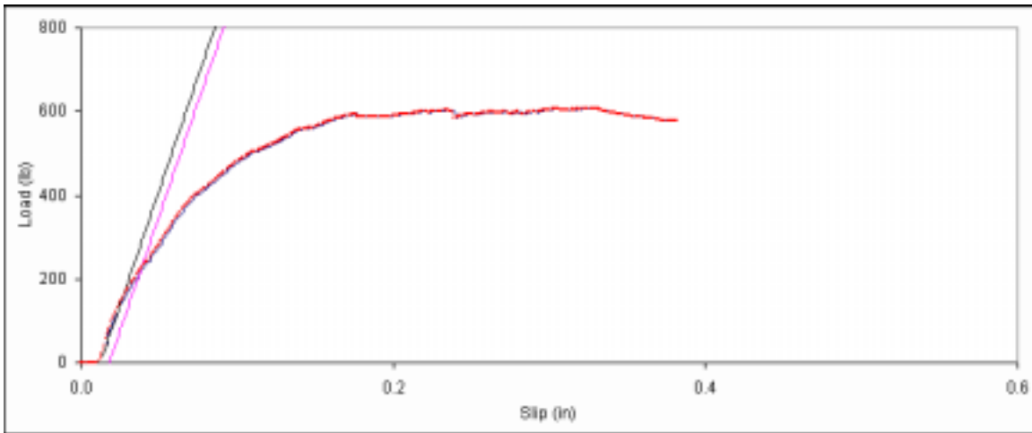
Figure D. 47: Bearing embedment plot for side member sample A-7.
