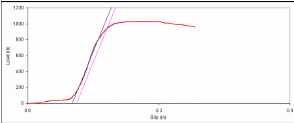
Figure D. 32: Bearing embedment plot for main member sample 8d-12.
