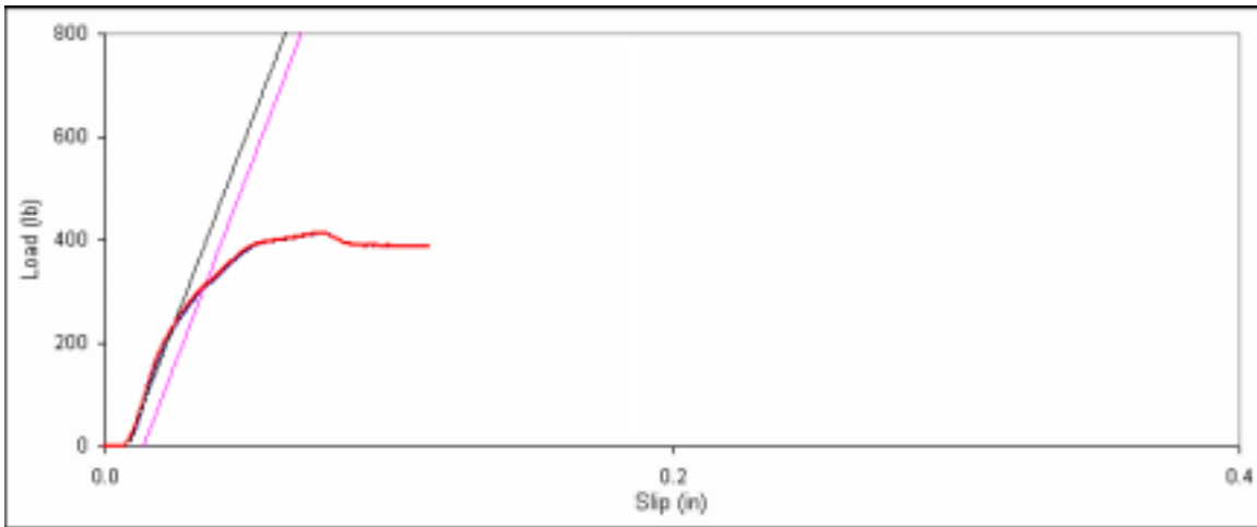
Figure D. 89: Bearing embedment plot for side member sample C-9.
