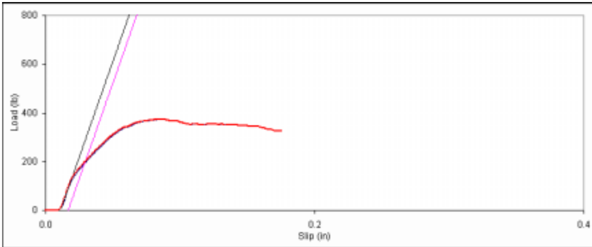
Figure D. 70: Bearing embedment plot for side member sample B-10.
