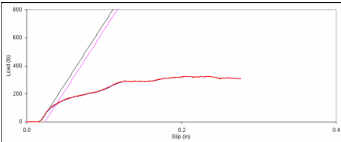
Figure D. 93: Bearing embedment plot for side member sample C-13.
