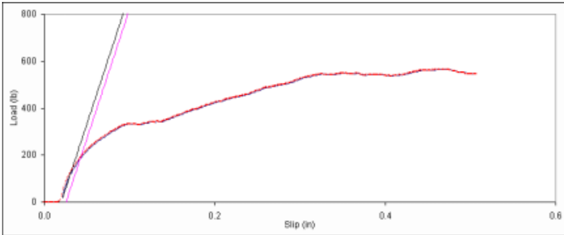
Figure D. 61: Bearing embedment plot for side member sample B-1.
