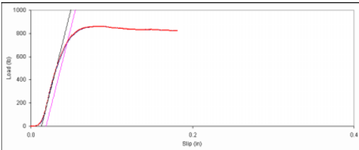
Figure D. 15: Bearing embedment plot for main member sample 6d-15.
