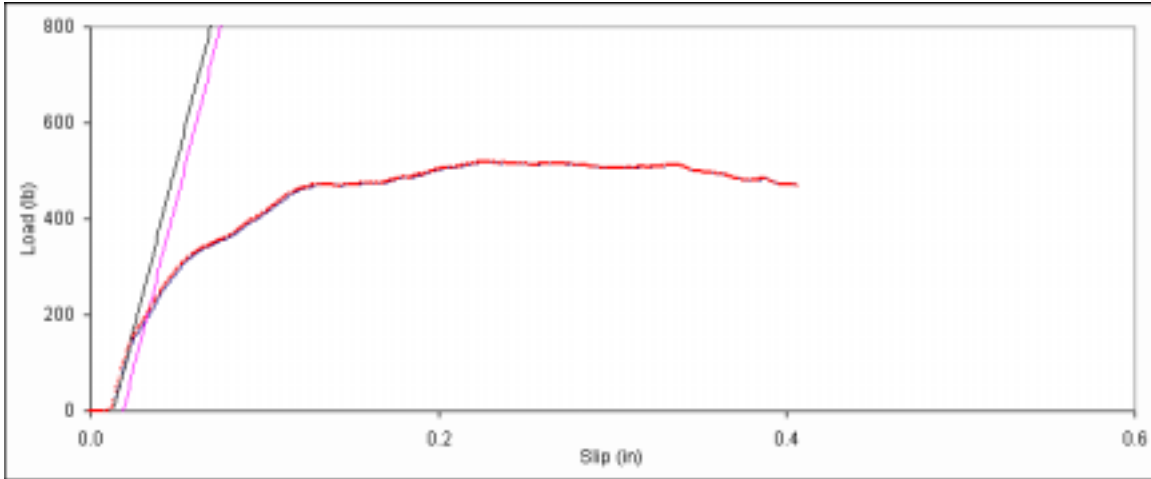
Figure D. 49: Bearing embedment plot for side member sample A-9.
