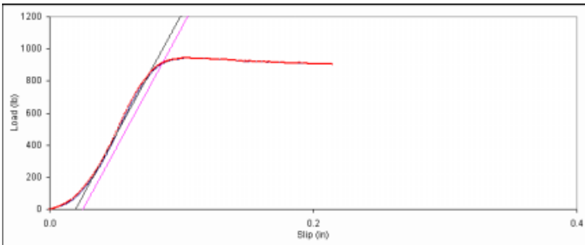
Figure D. 18: Bearing embedment plot for main member sample 6d-18.
