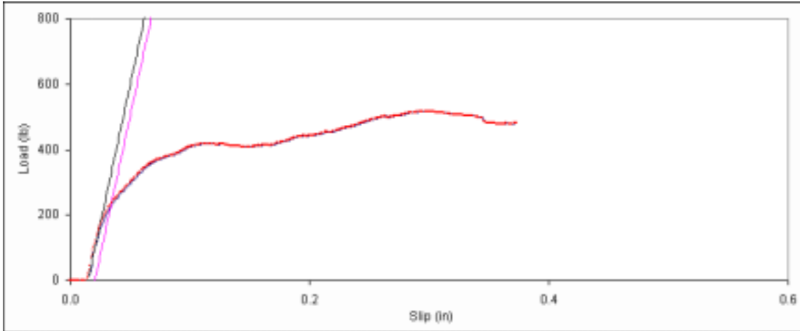
Figure D. 76: Bearing embedment plot for side member sample B-16.
