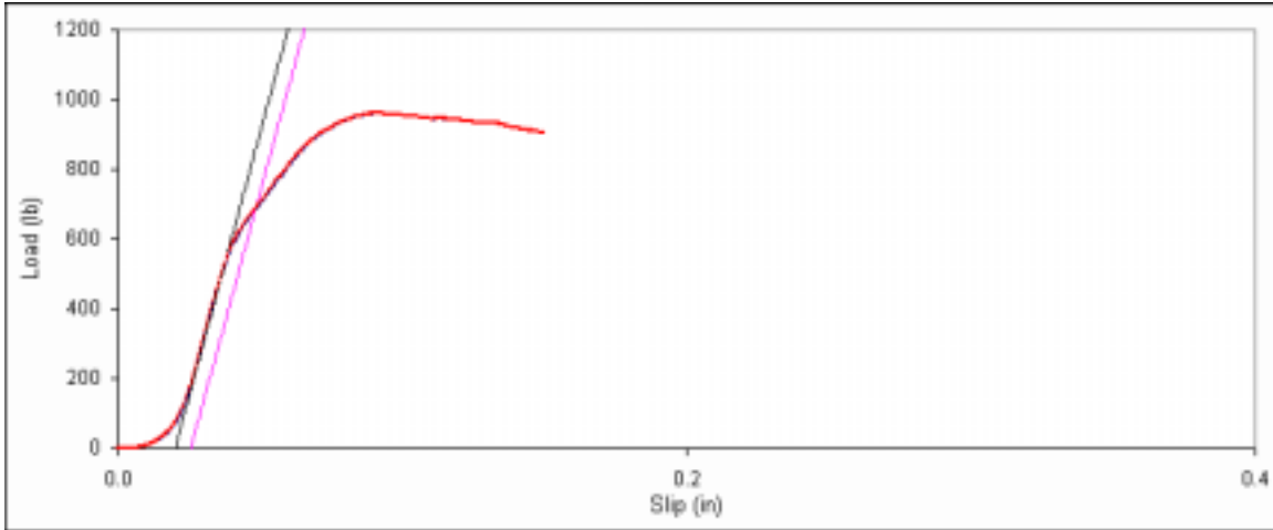
Figure D. 19: Bearing embedment plot for main member sample 6d-19.
