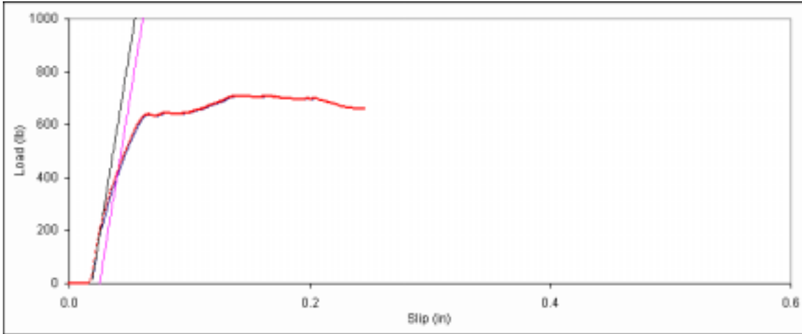
Figure D. 130: Bearing embedment plot for side member sample E-10.
