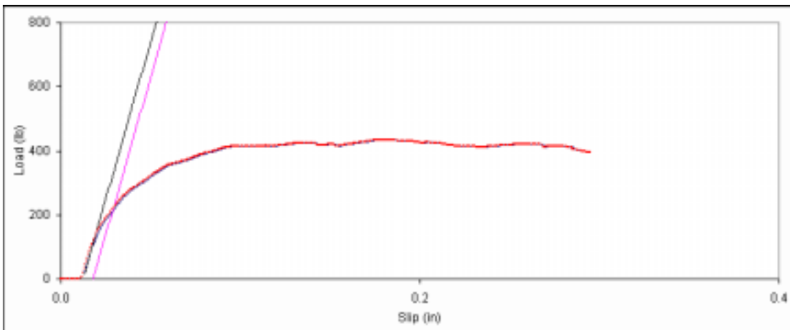
Figure D. 60: Bearing embedment plot for side member sample A-20.
