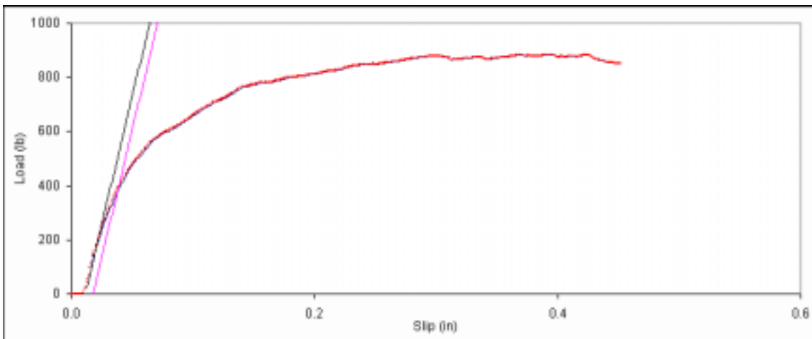
Figure D. 126: Bearing embedment plot for side member sample E-6.
