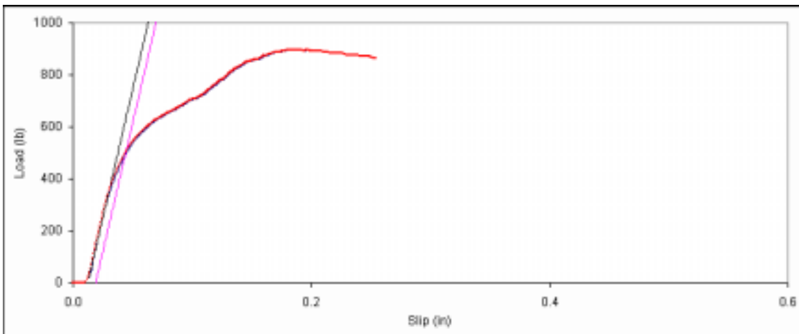
Figure D. 138: Bearing embedment plot for side member sample E-18.
