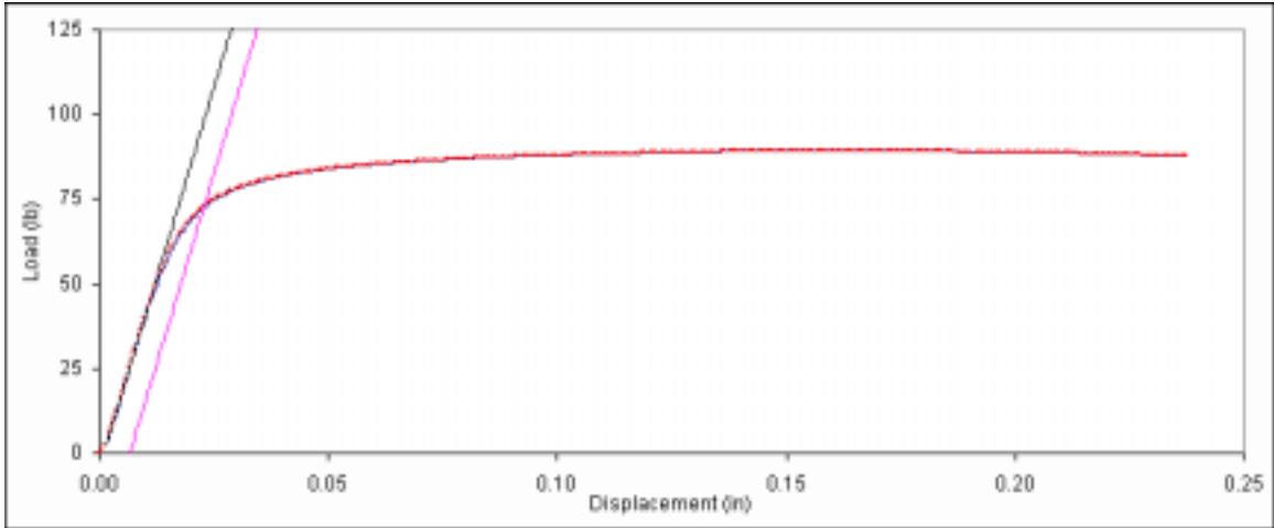
Figure D. 166: Bearing embedment plot for fastener sample 6d-6.
