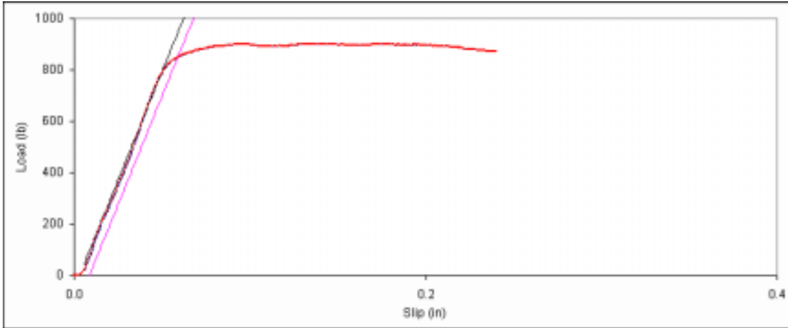
Figure D. 10: Bearing embedment plot for main member sample 6d-10.
