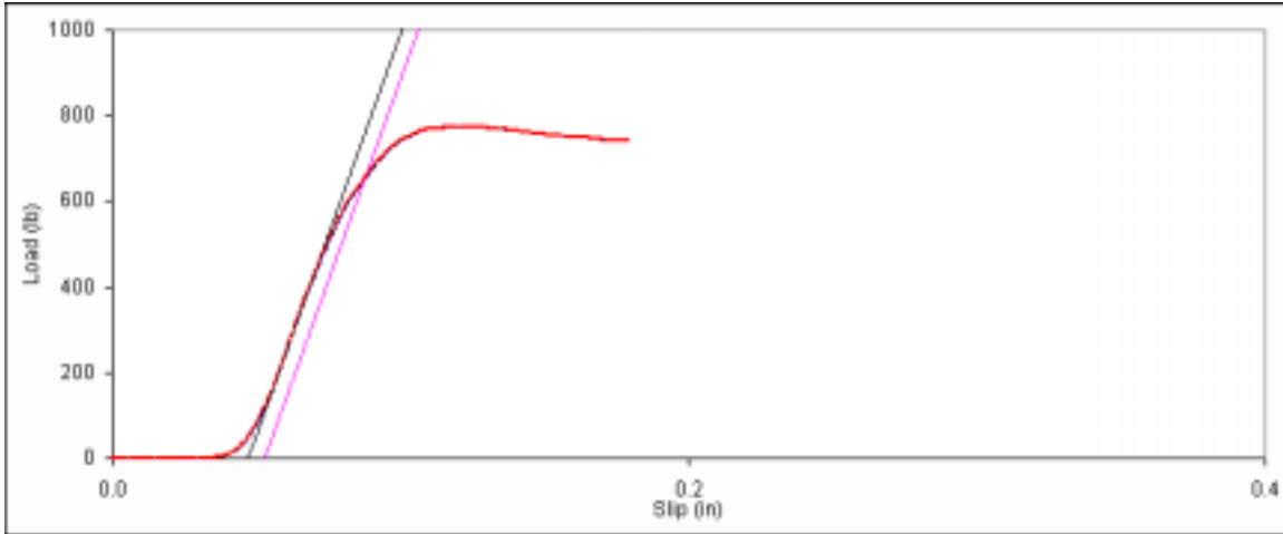
Figure D. 16: Bearing embedment plot for main member sample 6d-16.
