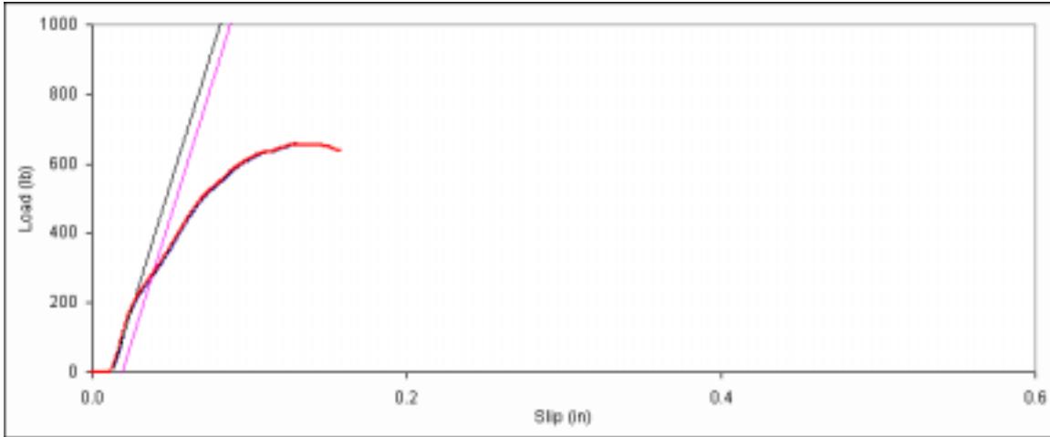
Figure D. 139: Bearing embedment plot for side member sample E-19.
