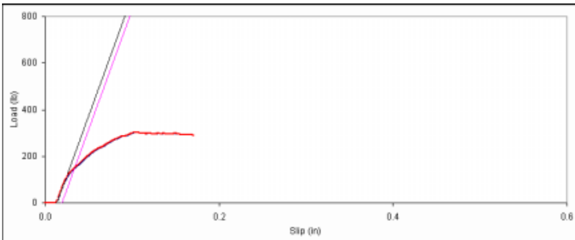
Figure D. 117: Bearing embedment plot for side member sample D-17.
