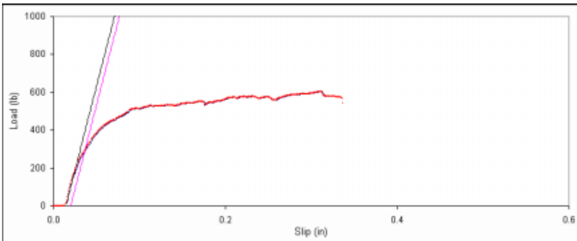
Figure D. 159: Bearing embedment plot for side member sample F-19.
