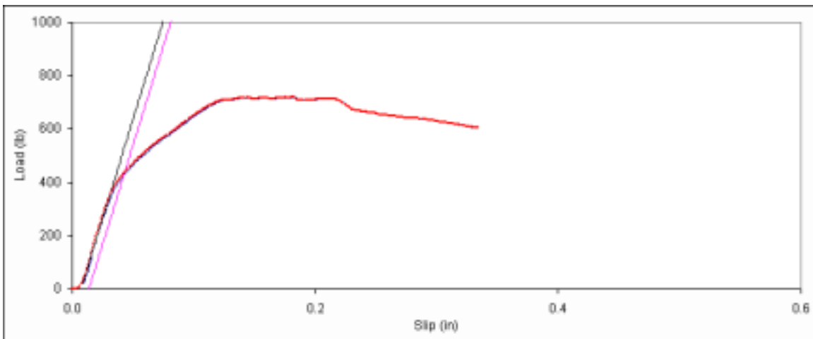
Figure D. 135: Bearing embedment plot for side member sample E-15.
