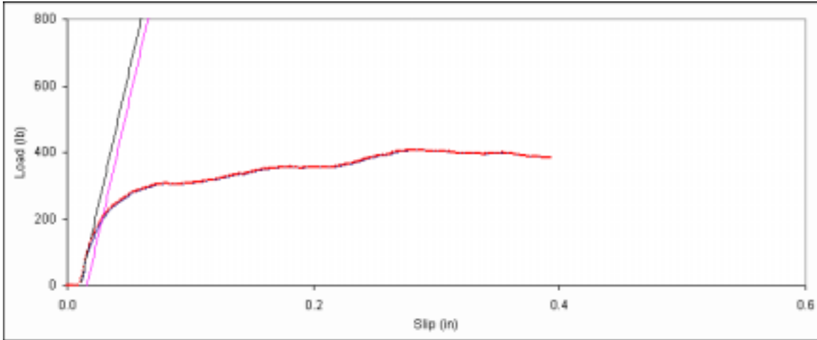
Figure D. 43: Bearing embedment plot for side member sample A-3.
