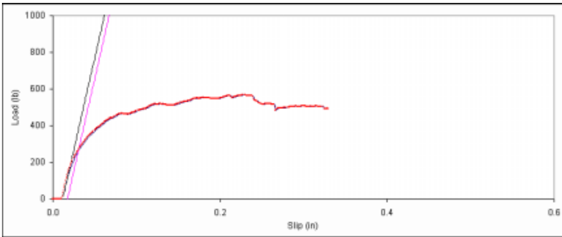
Figure D. 152: Bearing embedment plot for side member sample F-12.
