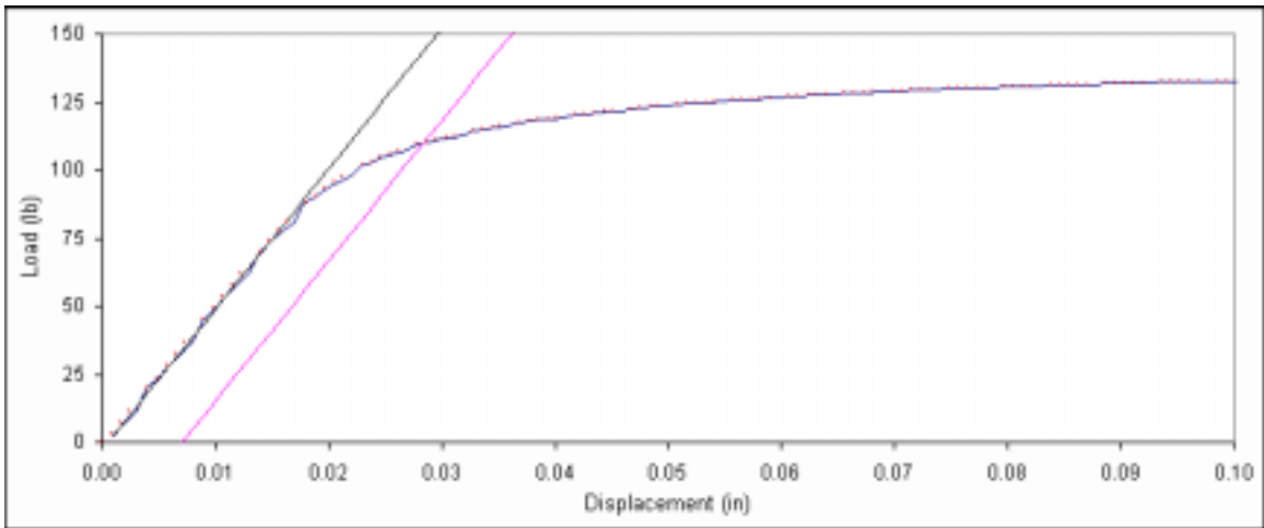
Figure D. 179: Bearing embedment plot for fastener sample 8d-9.
