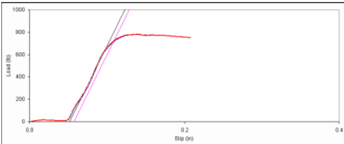
Figure D. 3: Bearing embedment plot for main member sample 6d-3.
