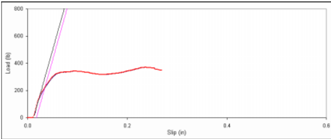
Figure D. 119: Bearing embedment plot for side member sample D-19.
