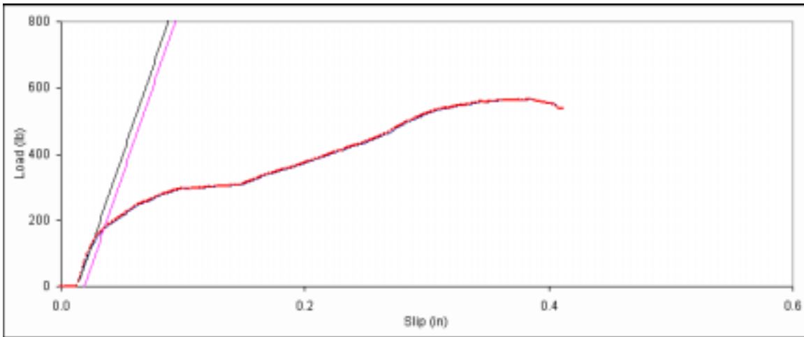
Figure D. 68: Bearing embedment plot for side member sample B-8.
