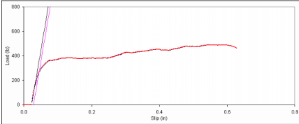
Figure D. 52: Bearing embedment plot for side member sample A-12.
