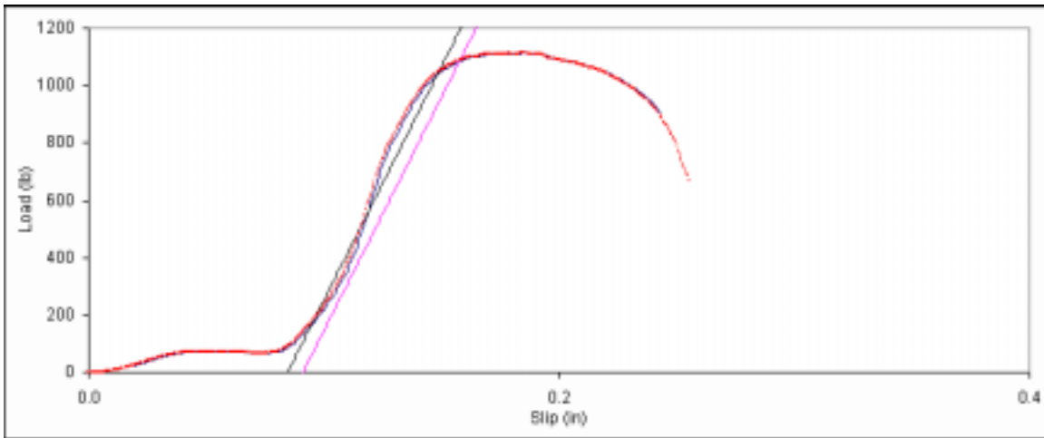
Figure D. 38: Bearing embedment plot for main member sample 8d-18.
