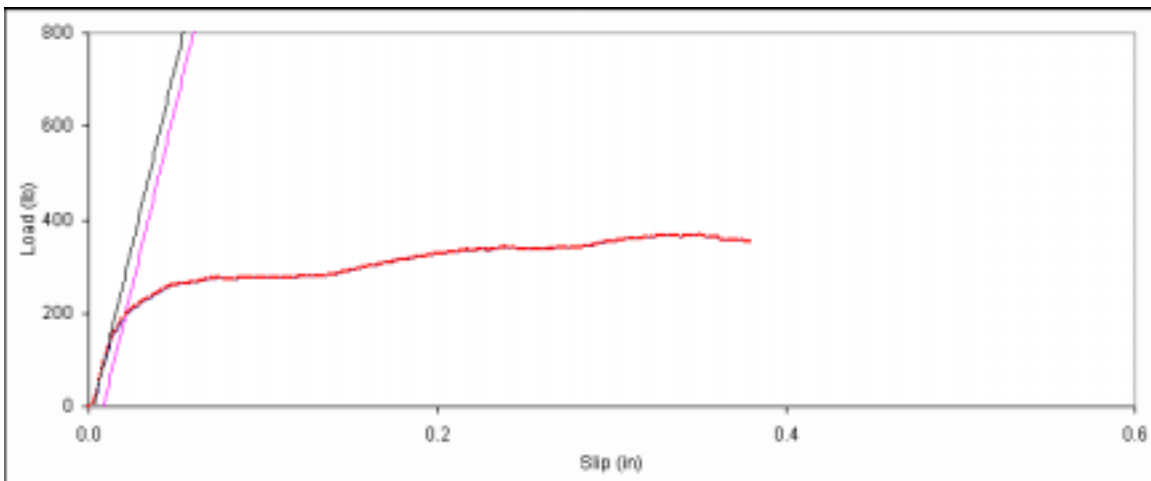
Figure D. 105: Bearing embedment plot for side member sample D-5.
