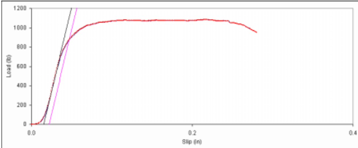
Figure D. 37: Bearing embedment plot for main member sample 8d-17.
