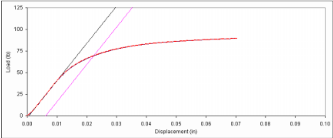
Figure D. 163: Bearing embedment plot for fastener sample 6d-3.
