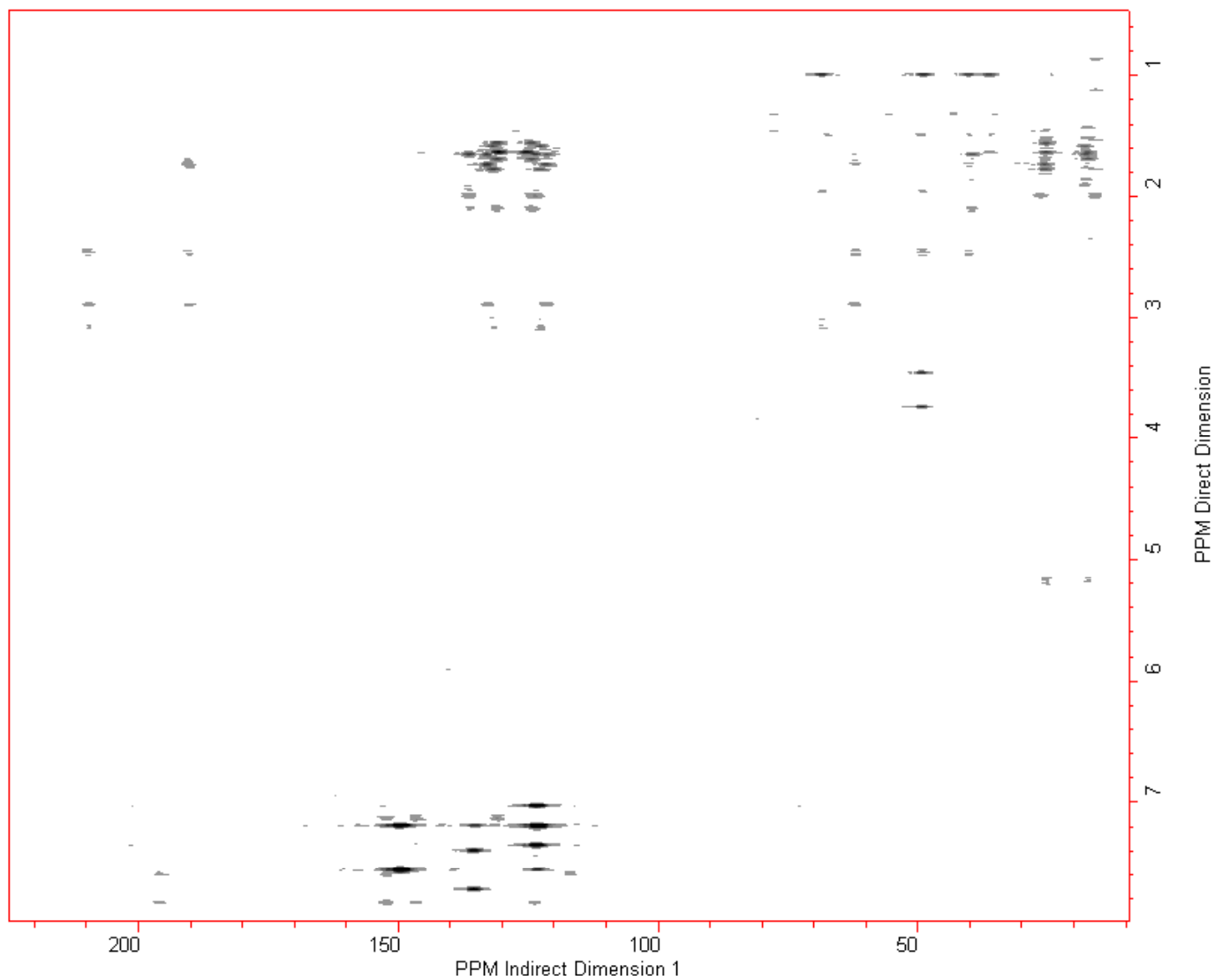
HMBC Spectrum of Garcinia Compound B /Guttiferone G in d 5 -pyridine.
