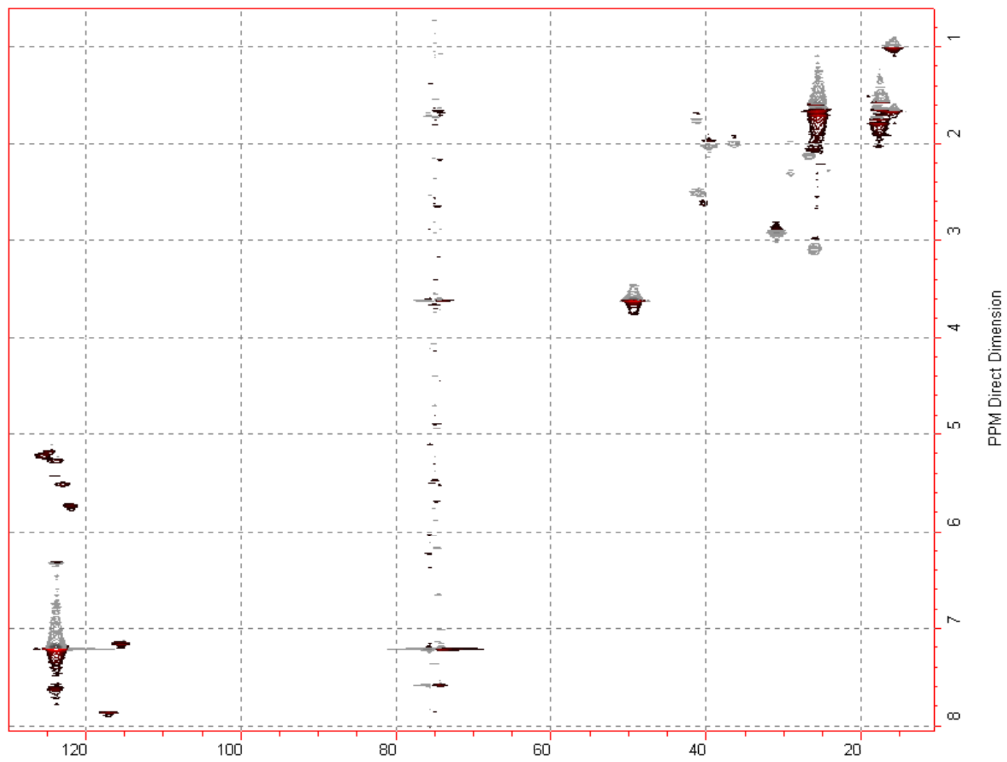
Gradient Selected HSQC Spectrum of Garcinia Compound B /Guttiferone G in d_5 -pyridine.
