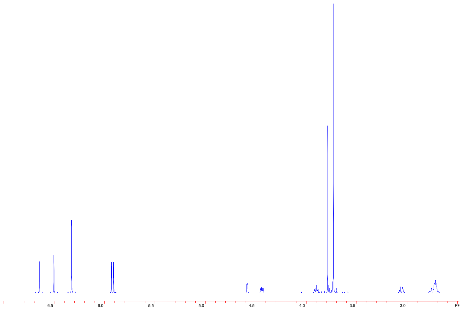
^1\text{H} NMR Spectrum of Authentic Sample of Deoxypodophyllotoxin in \text{CDCl}_3 .
