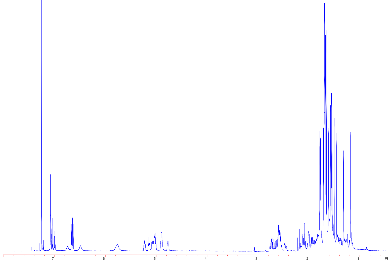
^1\text{H} NMR Spectrum of Garcinia Compound A/Guttiferone A in \text{CDCl}_3 .
