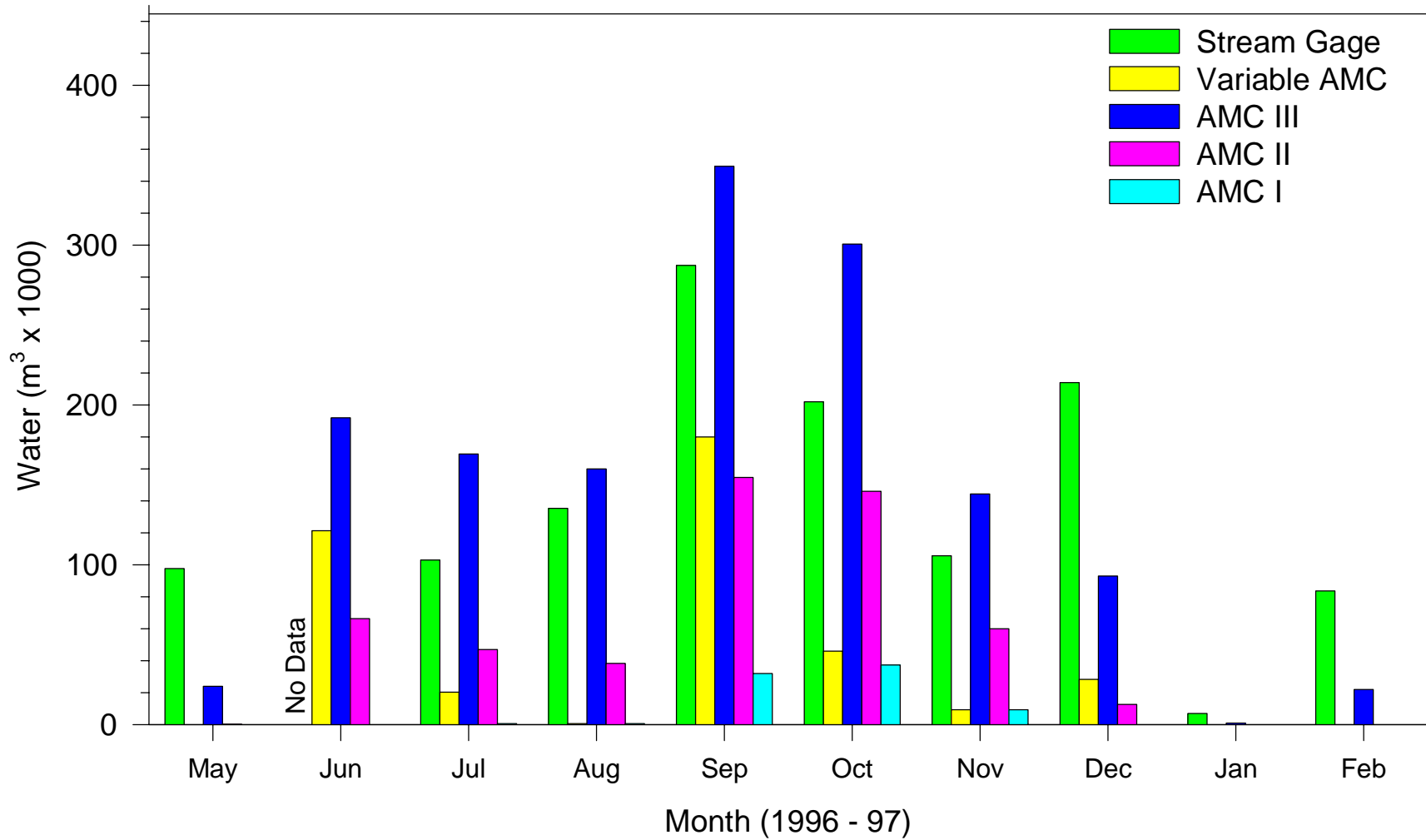
Figure 10. Runoff volumes calculated by the SCS runoff method for a range of antecedent moisture conditions (AMC) for Cockrell Branch watershed (W1) using on-site precipitation. May 1-9, Jun 19-30, Jul 1-3, Jan 16-31, and Feb 26-29 are not included.
