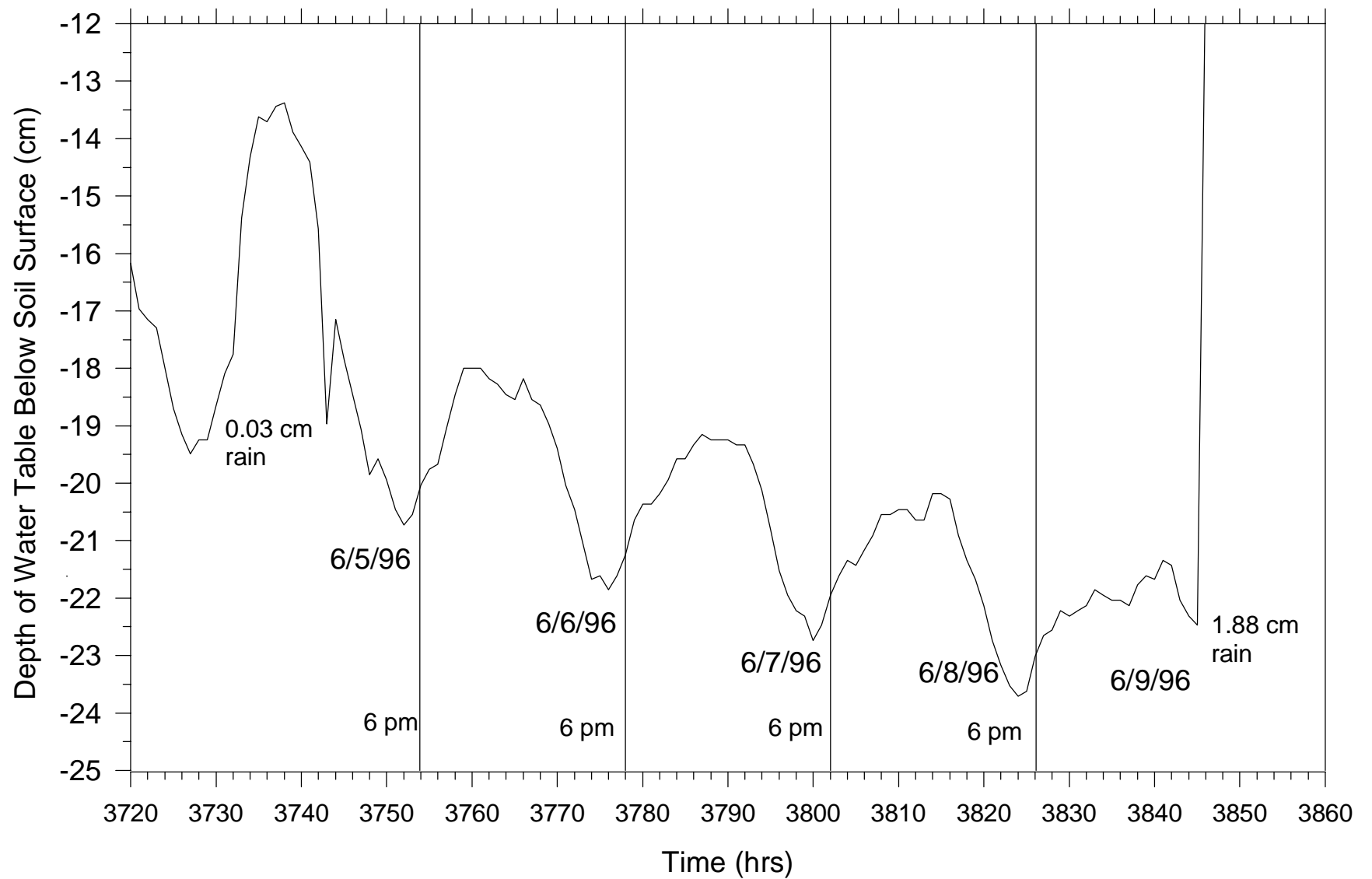
Figure 11. Sample diurnal cycles of groundwater levels in the observation well for June 5-9, 1996.
