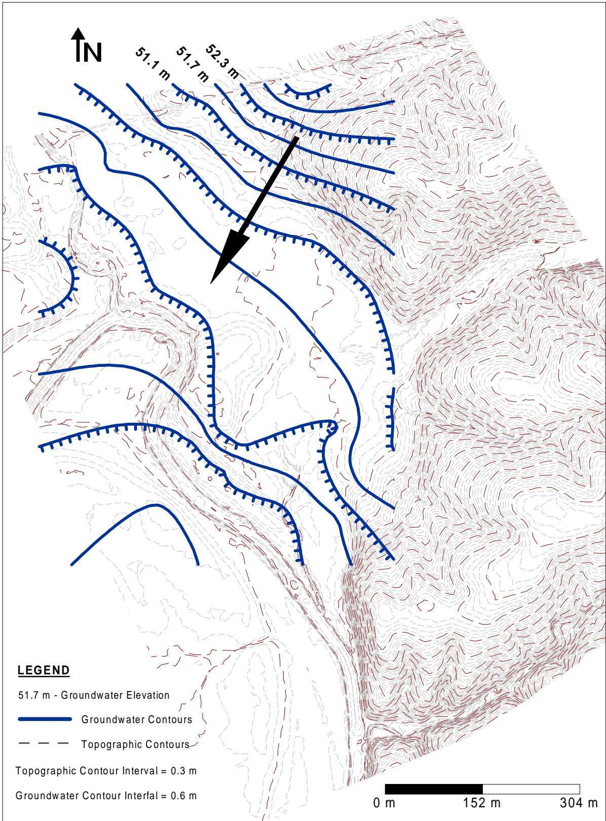
Figure 12. Groundwater potentiometric contours at the Manassas wetland site for July 9, 1996. Note: Overall flow direction is indicated by large arrow and flow is perpendicular to equipotential contours as shown by hatch lines.
