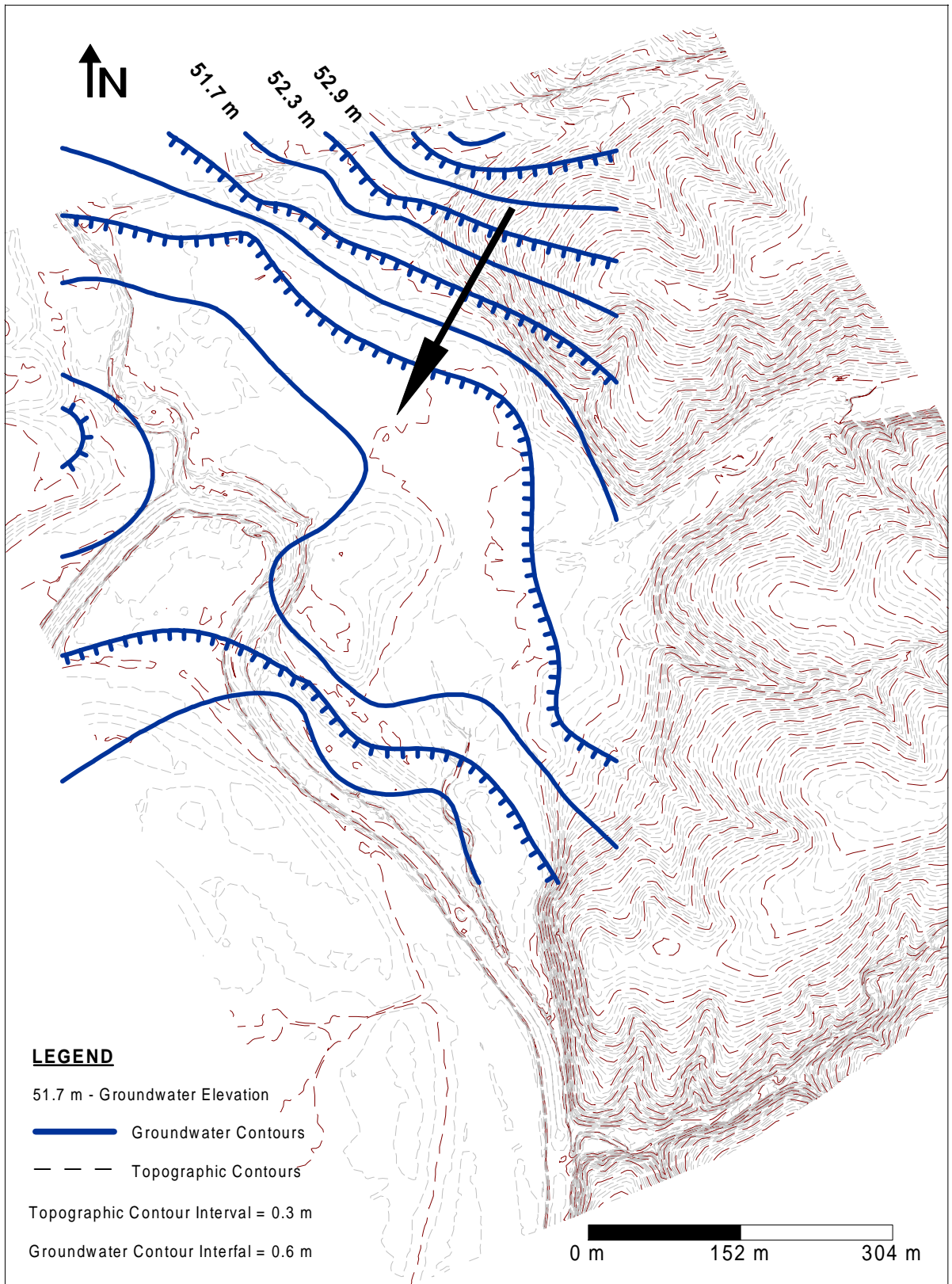
Figure 13. Groundwater potentiometric contours at the Manassas wetland for May 10, 1996. Note: Overall flow direction is indicated by large arrow and flow is perpendicular to equipotential contours as shown by hatch lines.
