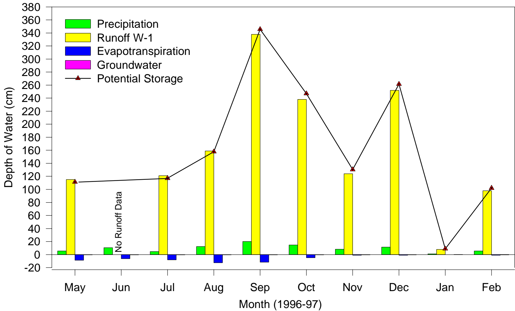
Figure 14. Potential storage and water balance components for the Manassas wetland from on-site measurements. May 1-9, Jun 1-30, Jul 1-3, Jan 16-31, and Feb 26-29 are not included in the total.
