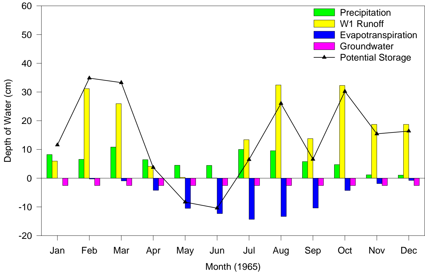
Figure 17. Potential storage in the Manassas wetland calculated using the modified Pierce model for a historically dry year.
