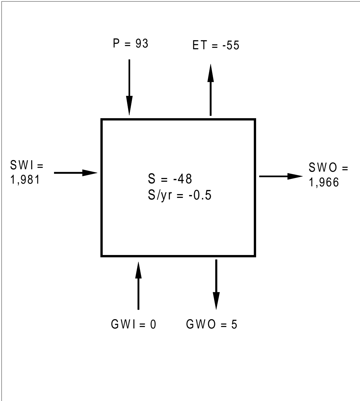
Figure 18. On-site measured water budget for the Manassas wetland. P = precipitation, ET = evapotranspiration, SWI = surface water inflows, SWO = surface water outflow, GWI = groundwater inflow, GWO = groundwater outflow, and S = change in storage. All values are expressed in cm/10 month period unless otherwise noted. Note: The months of May, June, July, January, and February did not include 9, 12, 3, 5, and 3 days of data, respectively.
