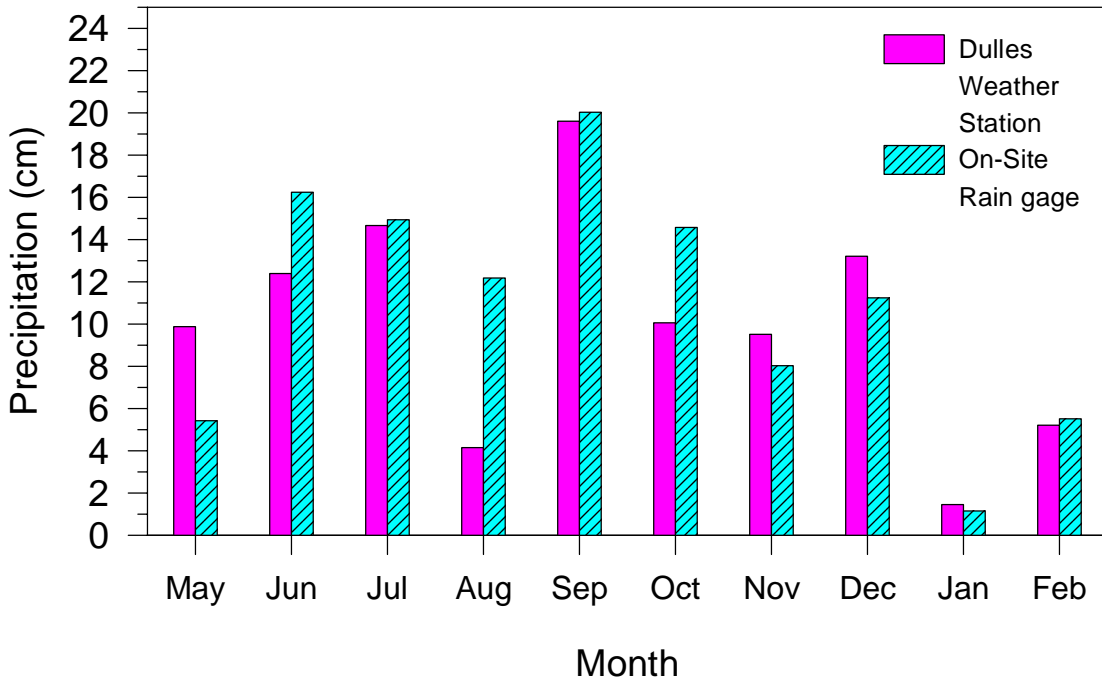
Figure 3a. Monthly precipitation totals from on-site rain gage and from the Dulles weather station. May 1-8, January 17-31, and February 26-28 are not included in the totals.
