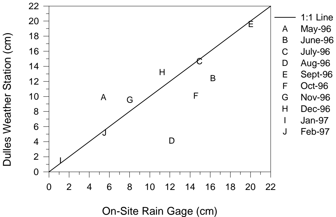
Figure 3b. Double mass curve showing the difference between monthly precipitation totals from the on-site rain gage and Dulles weather station.
