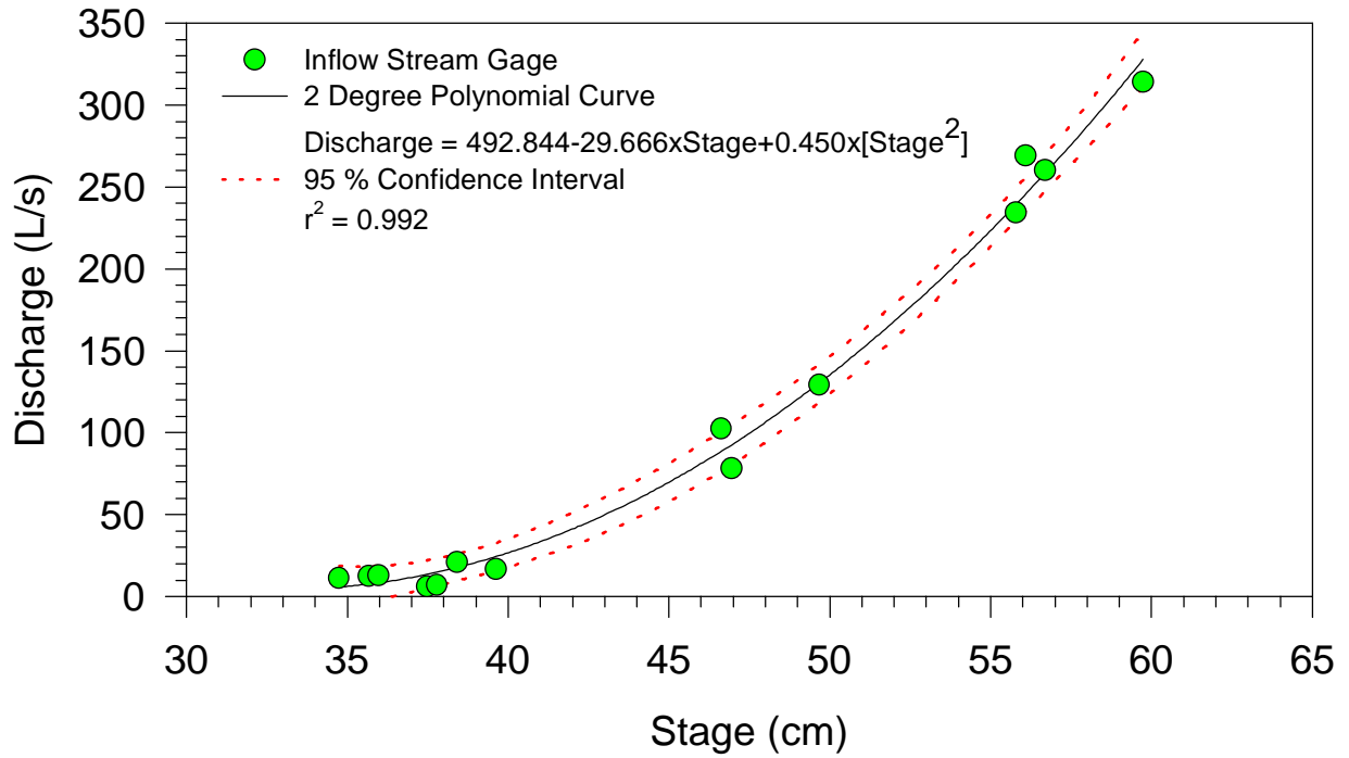
Figure 4a. Inflow rating curve developed from measured stream stage and discharge data.
