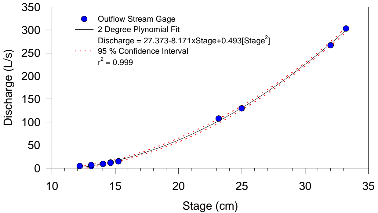
Figure 4b. Outflow rating curve developed from measured stream stage and discharge data.
