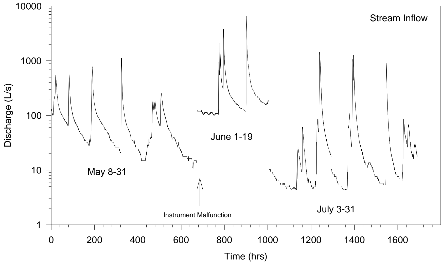
Figure 5. Partial record of the discharge at the inflow stage recorder on Cockrell Branch for May, June, and July showing the anomaly for the month of June.
