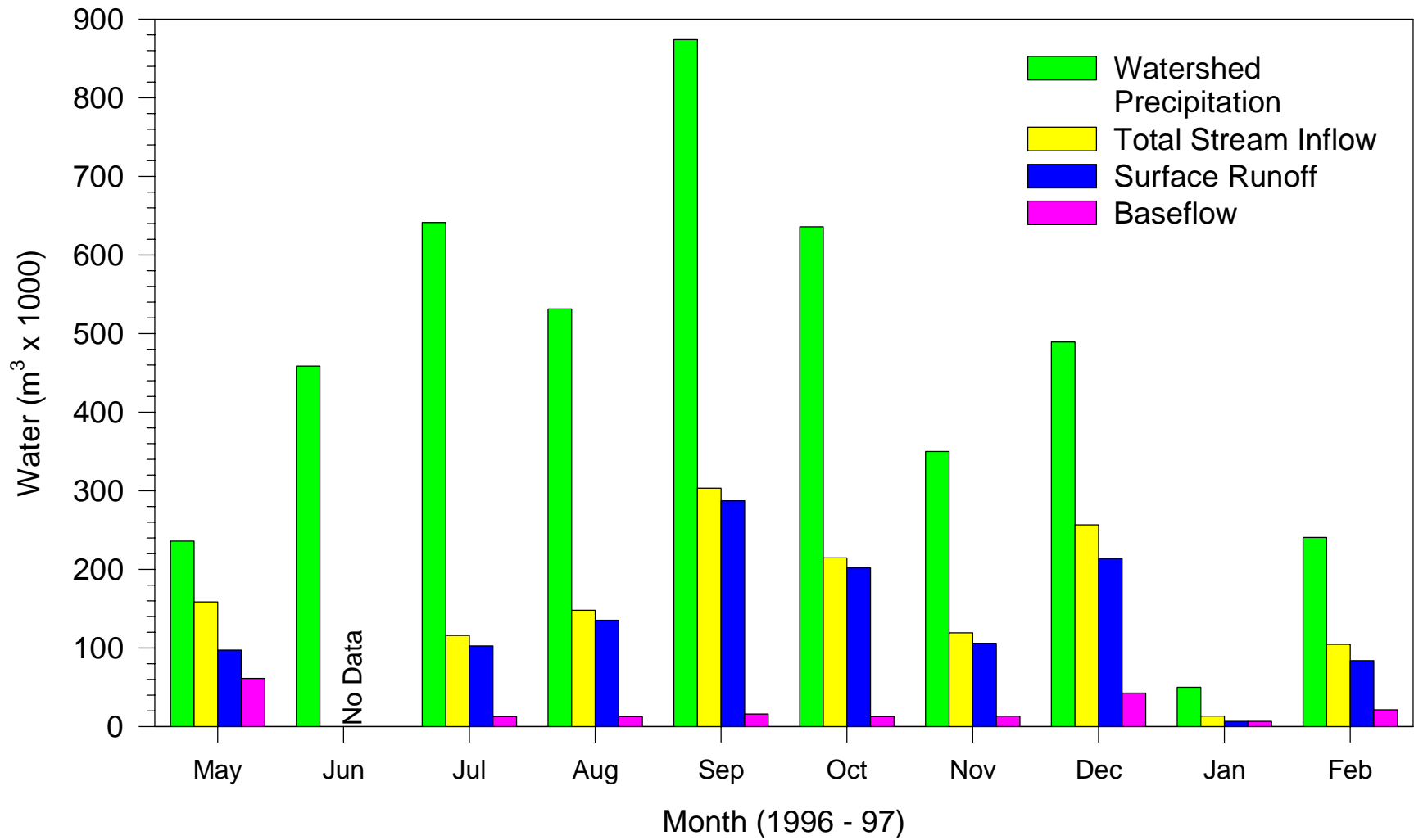
Figure 7. Monthly volume of precipitation over Cockrell Branch watershed (W1), and stream inflow, disaggregated into its surface runoff and baseflow components. May 1-9, Jun 1-30, Jul 1-3, Jan 16-31, and Feb 26-29 are not included in the totals.
