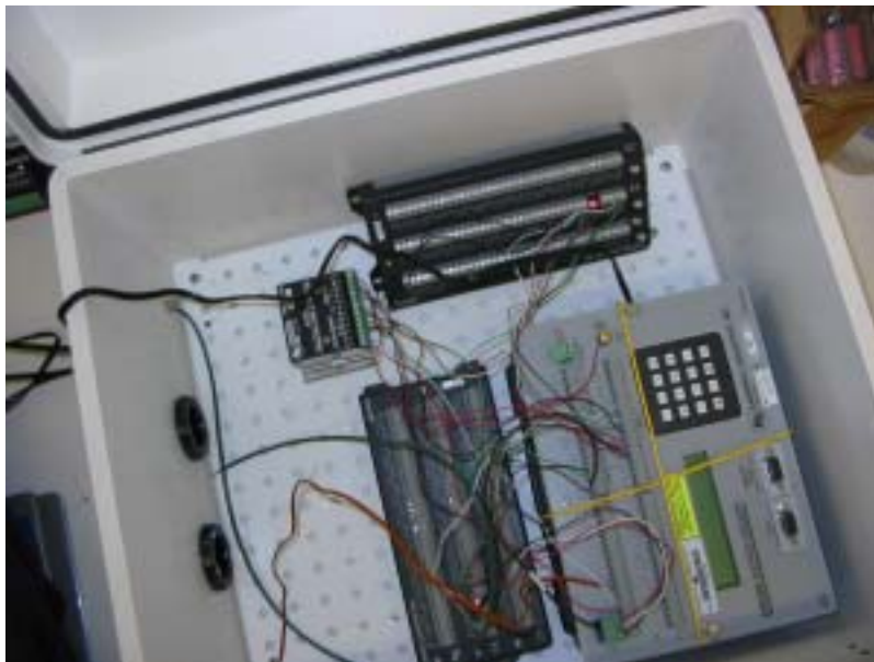
Figure 11. CR23X Micrologger and Instrumentation Components
