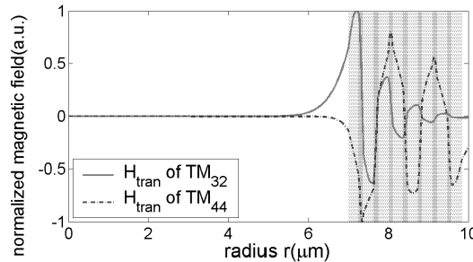
Fig. 4. The radial dependence of the magnetic field of the cladding modes. The fields of both modes are evanescent in the core. The field of TM_{32} mode decays quickly in the cladding due to the Bragg reflection. While the field of TM_{44} mode is propagating in the cladding layer and is confined by TIR at the outer surface. Here we use r_{co} = 7 \mu m and N_{Bragg} = 7 .
