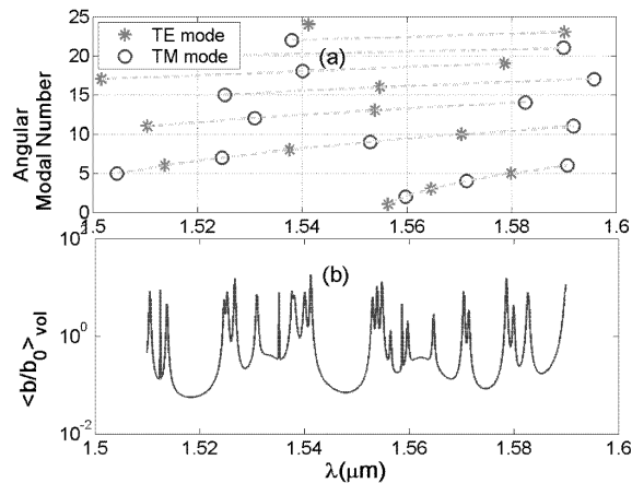
Fig. 6. (a) Spectrum of the onion resonator eigenmodes with modal number l \leq 24 . (b). Spectral dependence of the ensemble averaged damping rate. r_{co} = 7\mu\text{m} and N_{\text{Bragg}} = 4 are used in the calculation.
