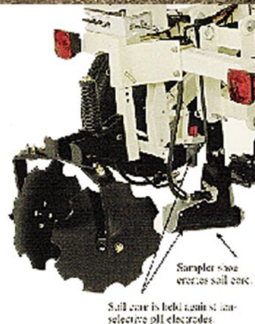
Figure 15. Veris Mobile Sensor Platform (MSP) equipped with “pH Manager” ( www.veristech.com/products/soilph.aspx ).
