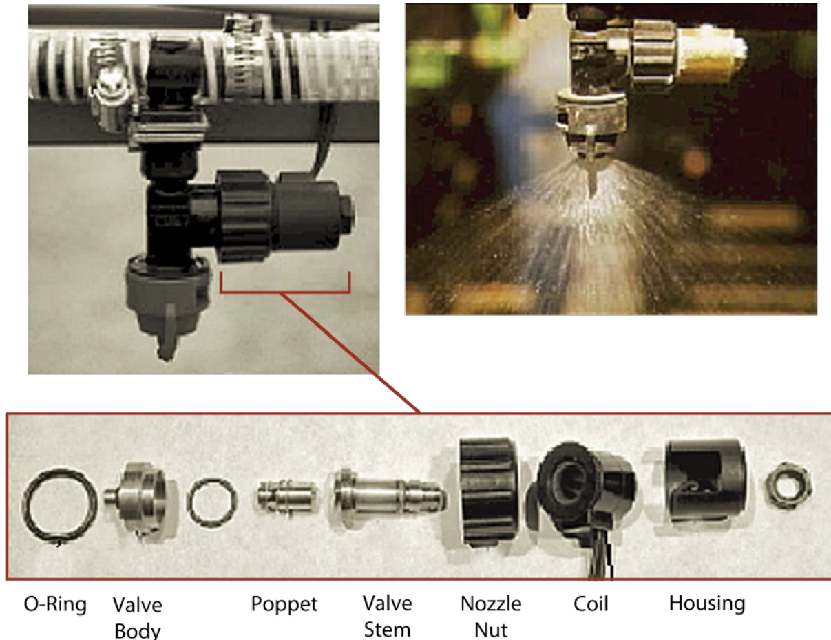
Figure 7. Fast-acting, electrical, solenoid-controlled nozzle assembly.
