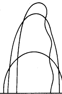
FIG. 7. The shape of extraordinary bubbles for \epsilon = 0.1 and \alpha = 0.5, 0.78, and 0.84 . The more vertically elongated bubbles correspond to larger values of \alpha .
