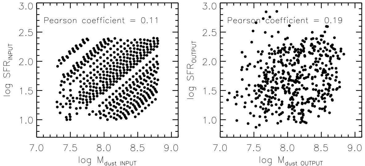
Fig. C.1. Distribution of mock SFR and M_{\text{dust}} in input (left panel) and output (right panel) of the simulation described in text. The measure of the SFR and M_{\text{dust}} does not introduce a correlation in an initially uncorrelated distribution. The value of the Pearson coefficient is printed in both cases.
