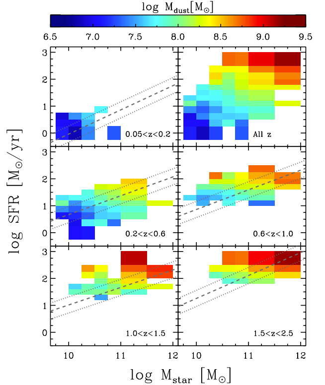
Fig. 4. Average dust mass values, as indicated by the colour according to the colour bar, for bins of different SFR and M_{\text{star}} in different redshift intervals and at all redshifts ( upper right panel ). Dashed lines represent MS relations of star-forming galaxies as taken from the literature; the local MS is from Peng et al. (2010) (computed using Brinchmann et al. 2004 data), rescaled to a Salpeter IMF, while the relations at higher redshifts are from Santini et al. (2009). Dotted lines represent the \pm 1\sigma ( =0.3 dex) scatter of the MS relation.
