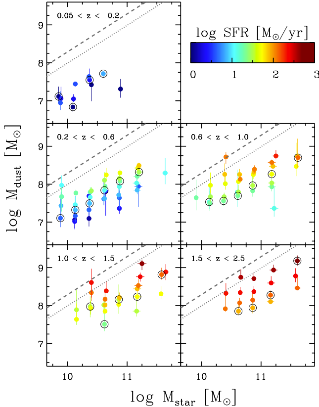
Fig. 3. Dust mass vs. stellar mass in different redshift ranges. Symbols are colour coded according to their SFR, as shown by the colour bar. At each M_{\text{star}} , black open circles mark the bin which lies closest to the MS (in each M_{\text{star}} interval), and in every case within 0.3 dex from it. The correlations between M_{\text{dust}} and M_{\text{star}} are rather flat when the data points are separated by means of their SFR. The dashed lines correspond to an amount of dust equal to the maximum metal mass M_Z = y_Z \times M_{\text{star}}^{\text{tot}} , where y_Z \sim 0.014 , assuming the extreme case of a condensation efficiency of 100%, while the dotted line shows the case when only 50% of the metals are depleted into dust grains (see text).
