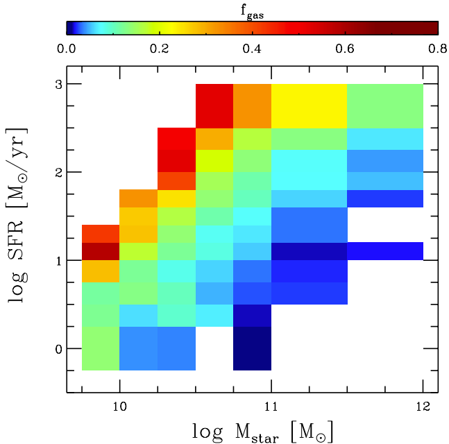
Fig. 9. Average gas fractions, as indicated by the upper colour bar, in bins of M_{\text{star}} and SFR.
