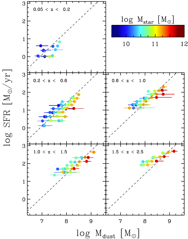
Fig. 2. SFR vs. dust mass in different redshift ranges. Galaxies are colour coded according to their stellar mass, as shown by the colour bar. The dashed lines corresponds to the integrated Schmidt-Kennicutt law fitted by Daddi et al. (2010), under the assumption of Solar metallicity (see text) and converted to a Salpeter IMF.
