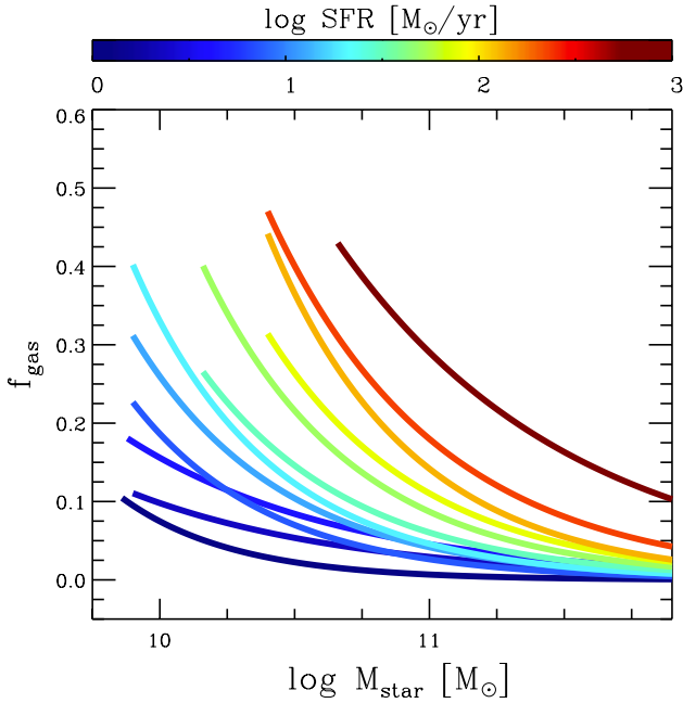
Fig. 10. Parameterization of the gas fraction as a function of stellar mass at all redshifts in different SFR intervals, using the functional shape given in Eq. (9) (see text). Curves of different colours refer to different SFR bins, as shown by the colour bar.
