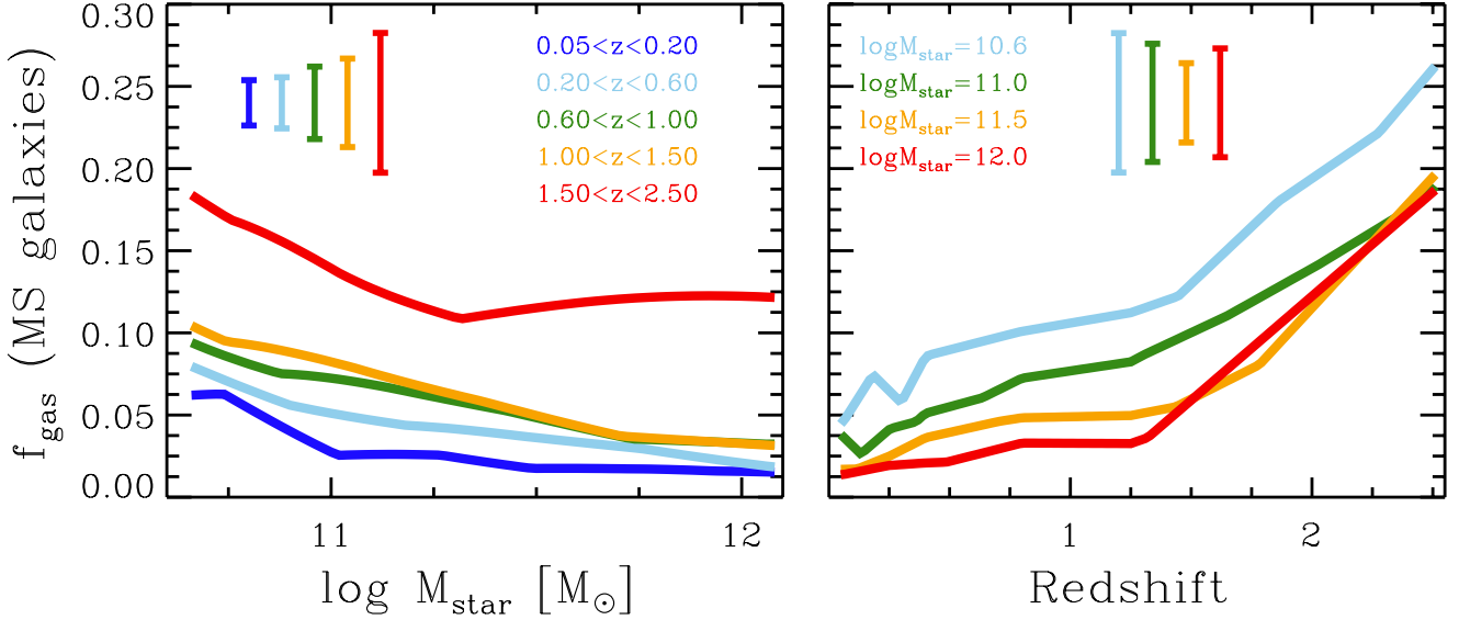
Fig. 12. Left: gas fraction vs. M_{\text{star}} at different redshifts (in different colours according to the legend) for main sequence (MS) galaxies. Right: gas fraction vs. redshift at different M_{\text{star}} (in different colours according to the legend) for MS galaxies. Curves are obtained by interpolating the f_{\text{gas}} parameterizations reported in Fig. 10 and Table 1 and the MS relations (see text for details) at M_{\text{star}} above the minimum sampled M_{\text{star}} common to all SFR bins. Mean uncertainties on gas fraction associated to MS galaxies in each redshift ( left ) or stellar mass ( right ) bin are plotted.
