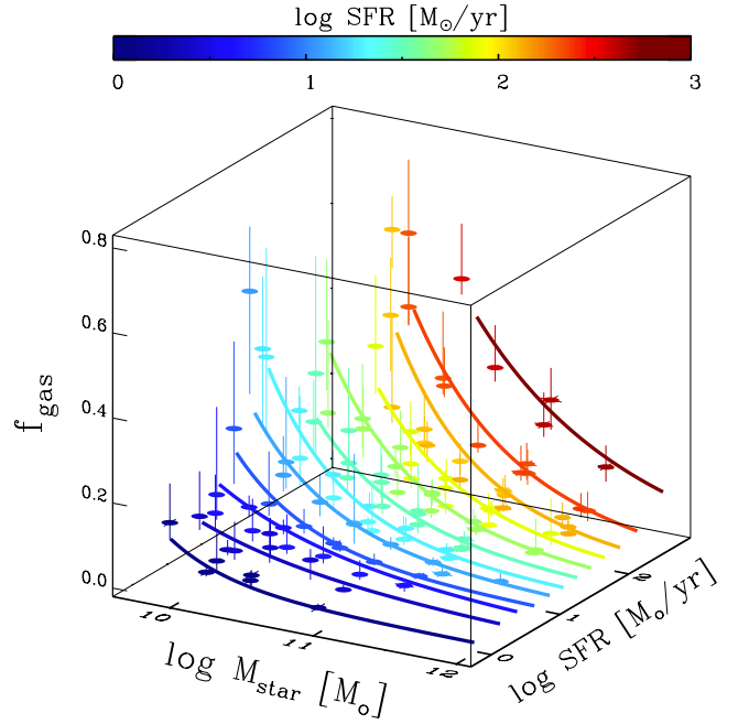
Fig. 11. Representation of the 3D fundamental f_{\text{gas}}-M_{\text{star}}-SFR relation. The colour code indicates the average SFR of each bin. The best-fit relations shown in Fig. 8 are overplotted.
