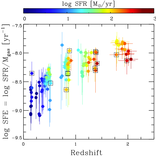
Fig. 7. Redshift evolution of the star formation efficiency (SFE, or inverse of the depletion time). Different colours refer to different SFRs, as shown by the colour bar. Black boxes are as in Fig. 6.
