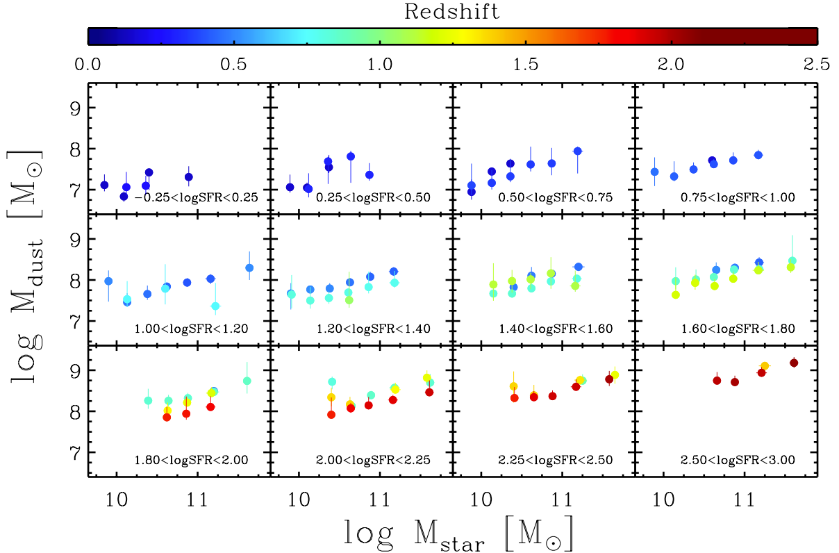
Fig. 5. Dust mass vs. stellar mass in panels of different SFR. The symbol colour indicates the mean redshift of each bin, as coded by the colour bar. No evolution with redshift is observed within uncertainties at a given M_{\text{star}} and SFR.
