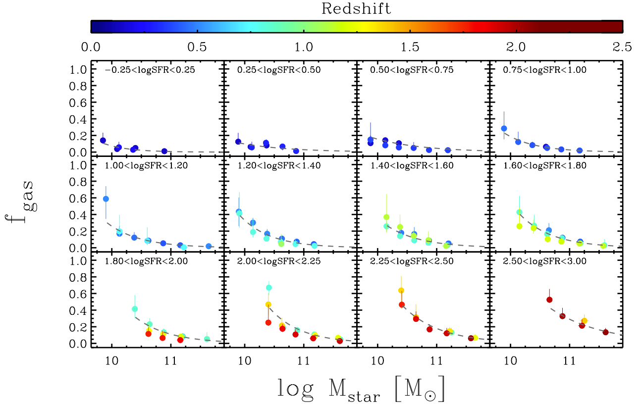
Fig. 8. Gas fraction vs. stellar mass in panels of different average SFR. The colour of the symbols reflects the mean redshift of each bin, as indicated by the colour bar. No evolution with redshift is observed, within uncertainties, at given SFR and M_{\text{star}} . Grey dashed curves are the best-fits to the data assuming the functional shape in Eq. (9). Best-fit parameters for each SFR interval are summarized in Table 1.
